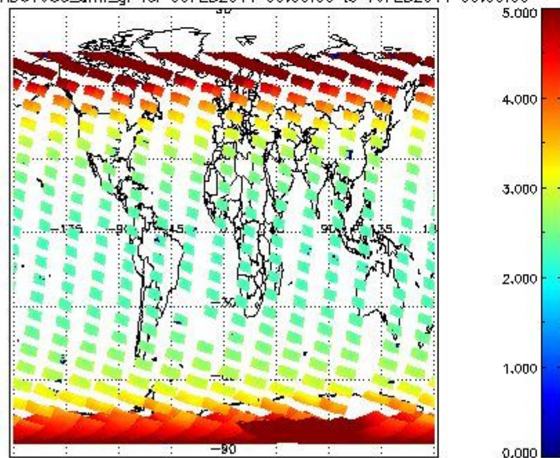
SCIOL2P_NADUV003_amf_gr for 09FEB2011 00:00:00 to 10FEB2011 00:00:00
