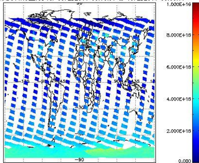
SCIOL2P_NADUV1N02_vcd for 09FEB2011 00:00:00 to 10FEB2011 00:00:00
