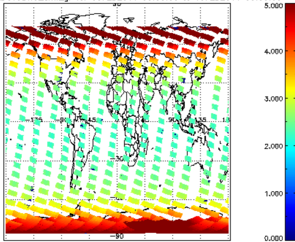
SCIOL2P_NADUV3BRO_amf_gr for 09FEB2011 00:00:00 to 10FEB2011 00:00:00
