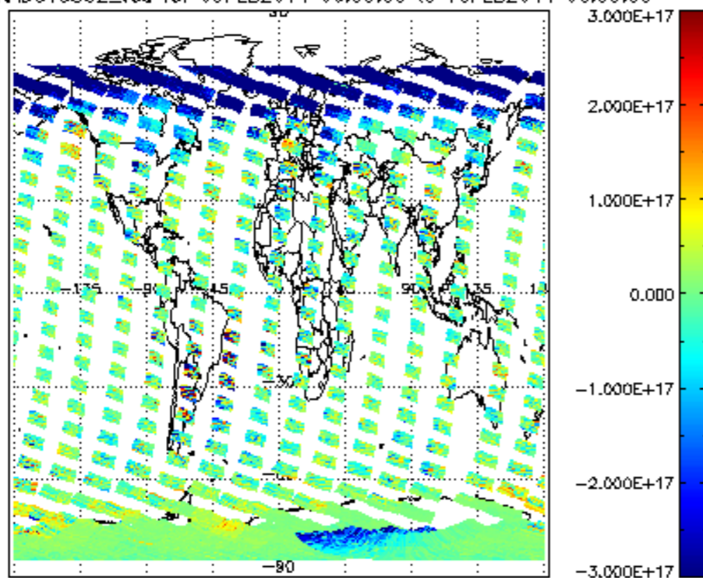
SCIOL2P_NADUV5S02_vcd for 09FEB2011 00:00:00 to 10FEB2011 00:00:00
