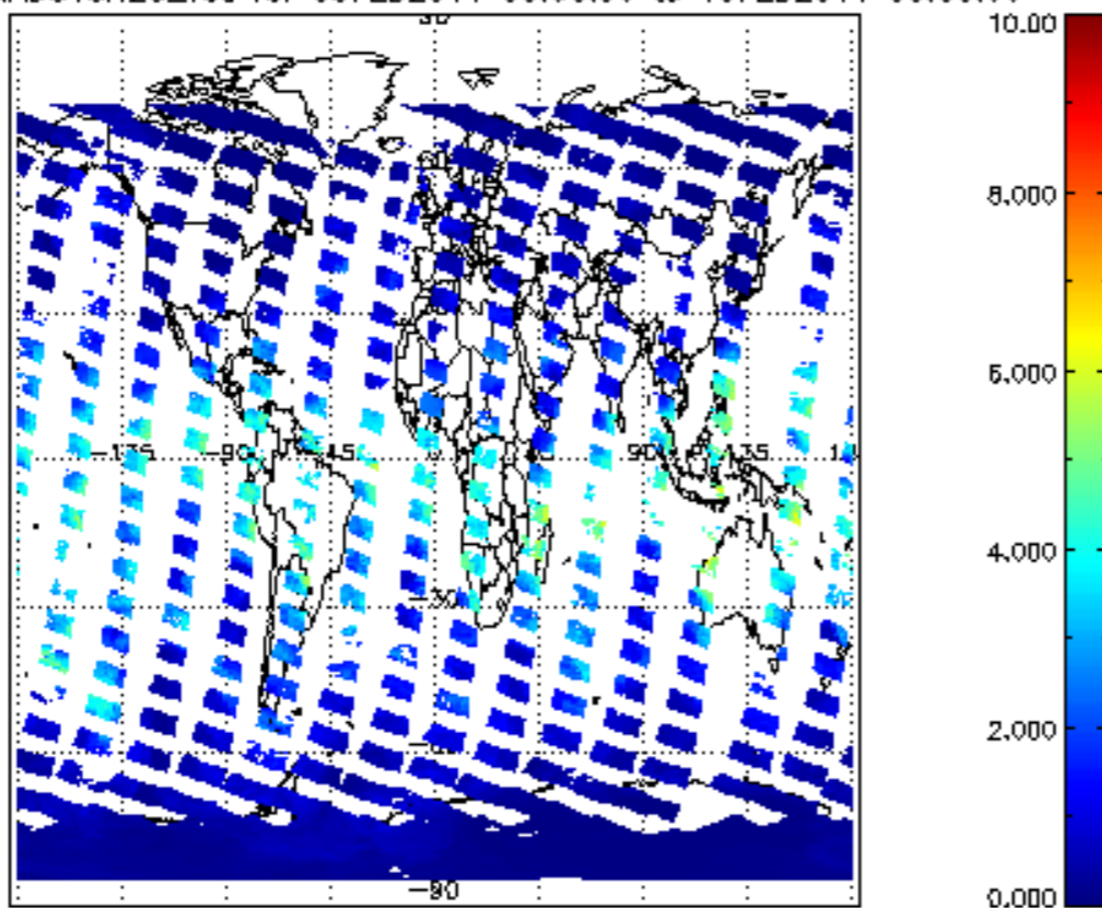
SCIOL2P_NADUV8H2O_vcd for 09FEB2011 00:00:00 to 10FEB2011 00:00:00
