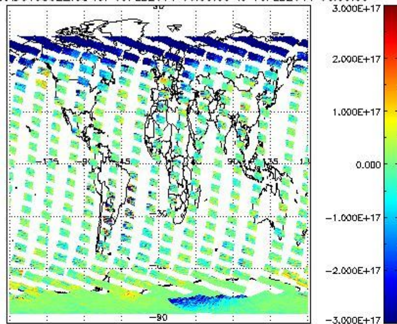
SCIOL2P_NADUV5S02_vcd for 09FEB2011 00:00:00 to 10FEB2011 00:00:00
