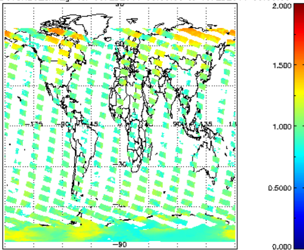
SCIOL2P_NADUV8H2O_amf_gr for 09FEB2011 00:00:00 to 10FEB2011 00:00:00
