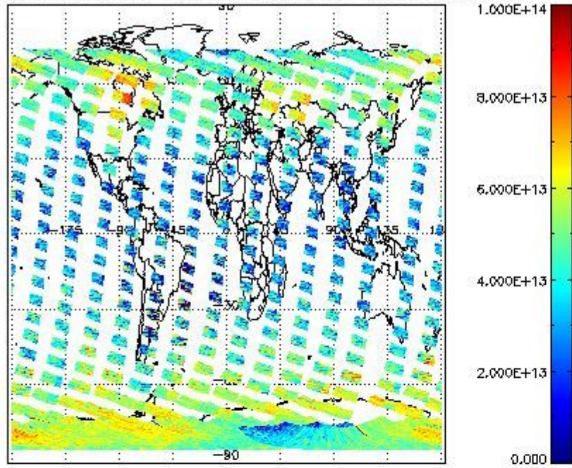
SCIOL2P_NADUV3BRO_vcd for 09FEB2011 00:00:00 to 10FEB2011 00:00:00
