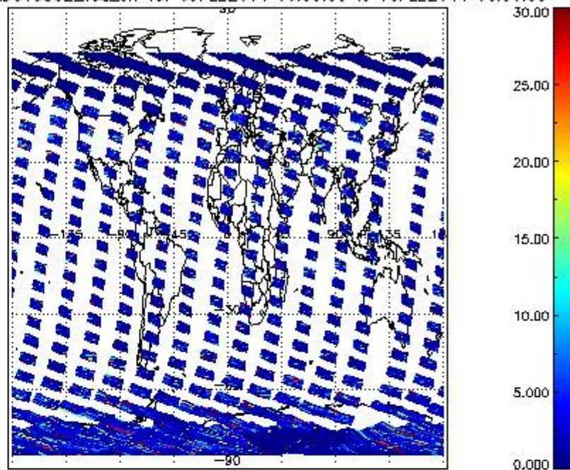
SCIOL2P_NADUV5S02_vcd_err for 09FEB2011 00:00:00 to 10FEB2011 00:00:00
