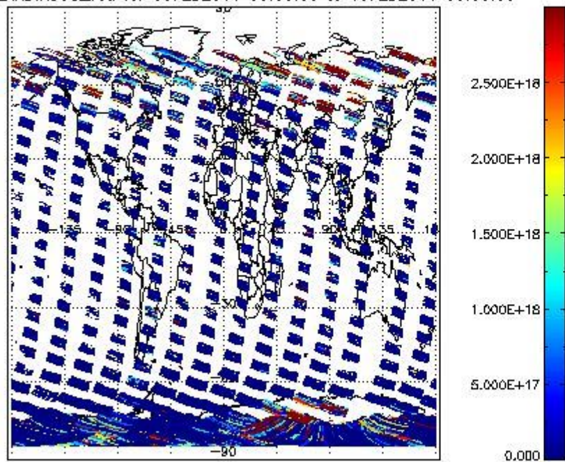
SCIO2P_NADIR3CO_vcd for 09FEB2011 00:00:00 to 10FEB2011 00:00:00
