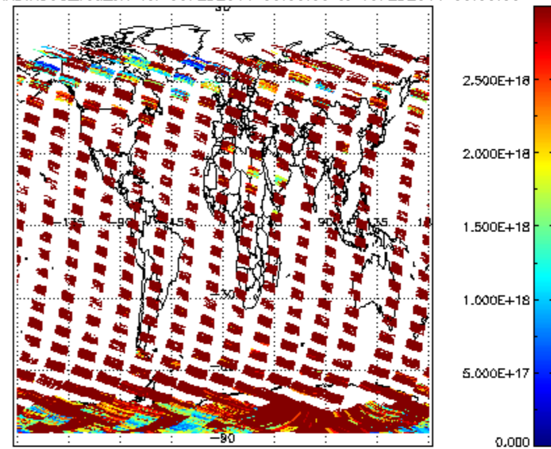
SCIOL2P_NADIR3CO_vcd_err for 09FEB2011 00:00:00 to 10FEB2011 00:00:00
