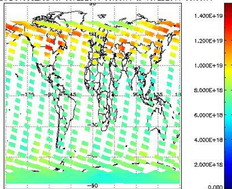
SCIOL2P_NADUV003_vcd for 09FEB2011 00:00:00 to 10FEB2011 00:00:00
