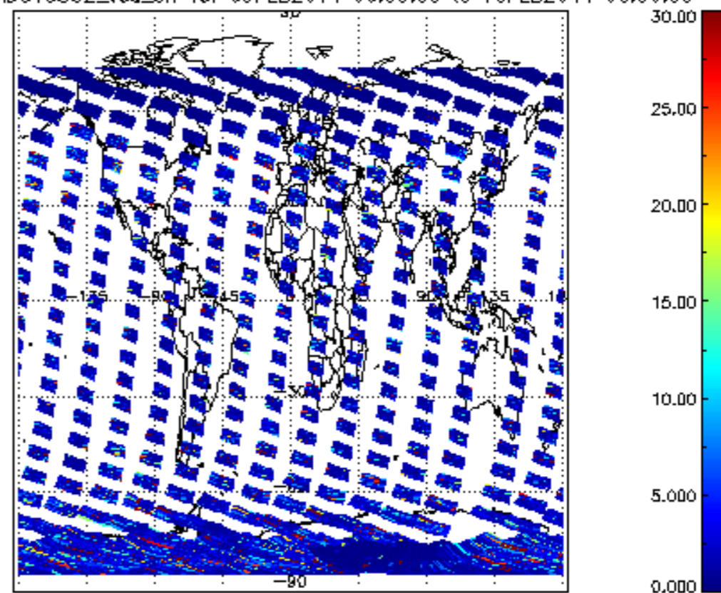
SCIOL2P_NADUV5S02_vcd_err for 09FEB2011 00:00:00 to 10FEB2011 00:00:00
