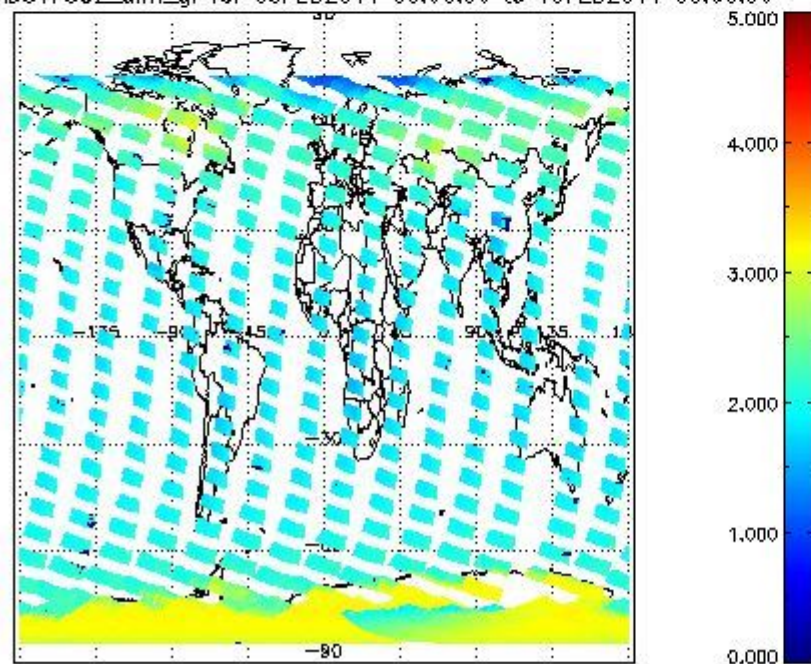
SCIOL2P_NADUV7S02_amf_gr for 09FEB2011 00:00:00 to 10FEB2011 00:00:00
