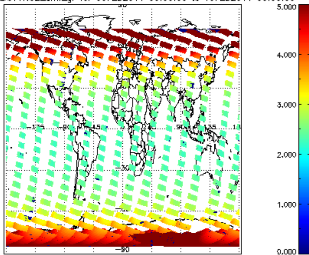
SCIOL2P_NADUV1N02_amf_gr for 09FEB2011 00:00:00 to 10FEB2011 00:00:00
