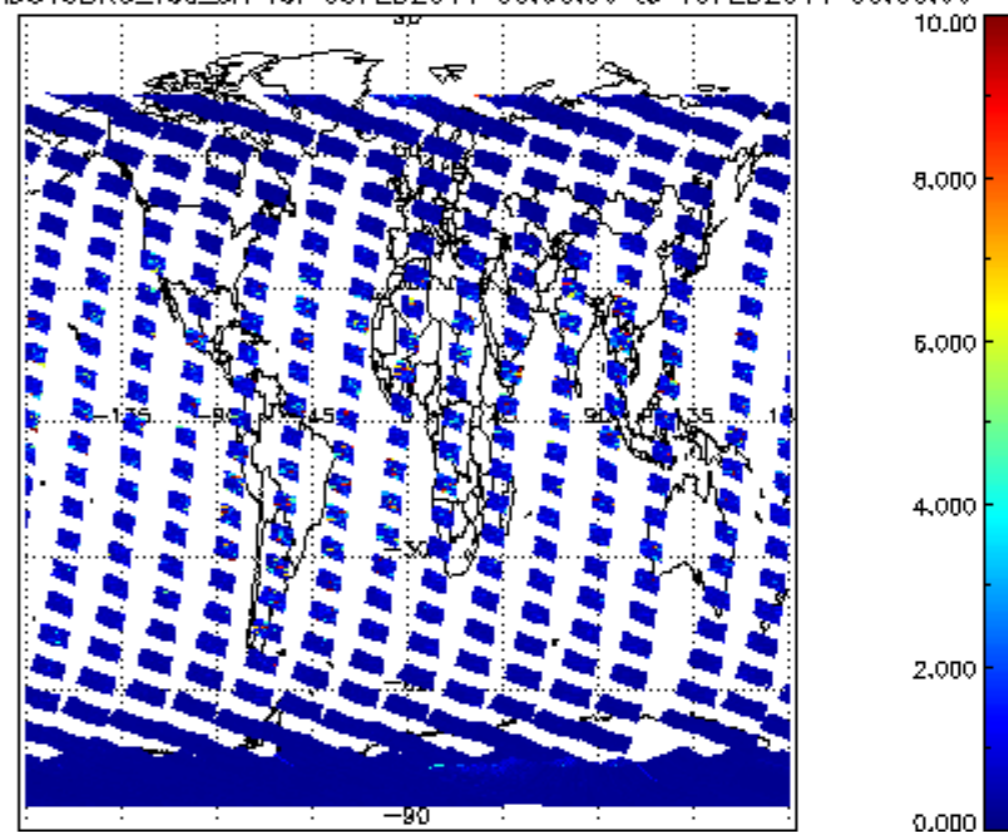
SCIOL2P_NADUV3BRO_vcd_err for 09FEB2011 00:00:00 to 10FEB2011 00:00:00
