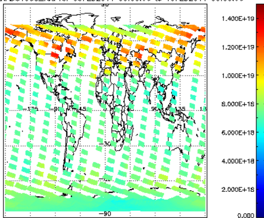
SCIOL2P_NADUV003_vcd for 09FEB2011 00:00:00 to 10FEB2011 00:00:00
