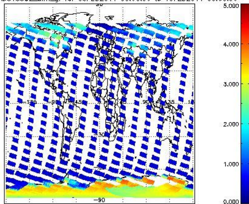
SCIOL2P_NADUV5S02_amf_gr for 09FEB2011 00:00:00 to 10FEB2011 00:00:00
