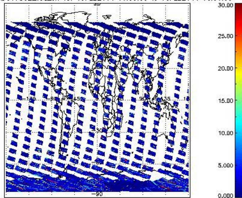
SCIOL2P_NADUV7S02_vcd_err for 09FEB2011 00:00:00 to 10FEB2011 00:00:00
