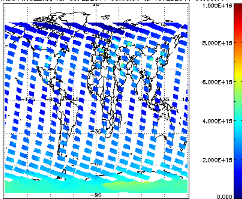
SCIOL2P_NADUV1N02_vcd for 09FEB2011 00:00:00 to 10FEB2011 00:00:00
