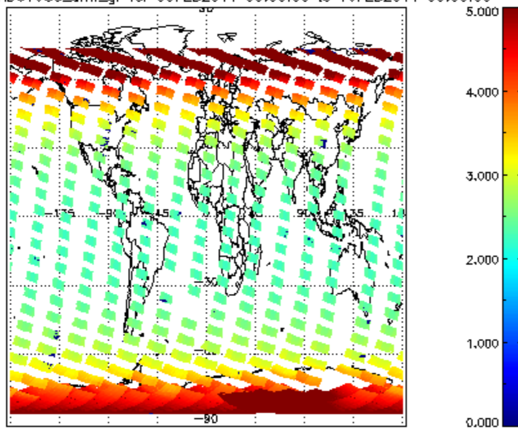
SCIOL2P_NADUV003_amf_gr for 09FEB2011 00:00:00 to 10FEB2011 00:00:00
