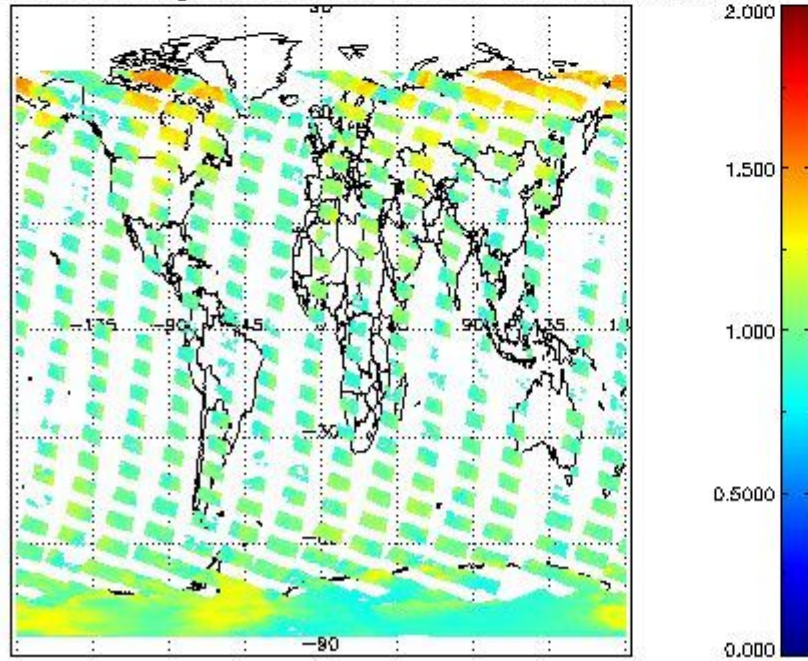
SCIOL2P_NADUV8H2O_amf_gr for 09FEB2011 00:00:00 to 10FEB2011 00:00:00
