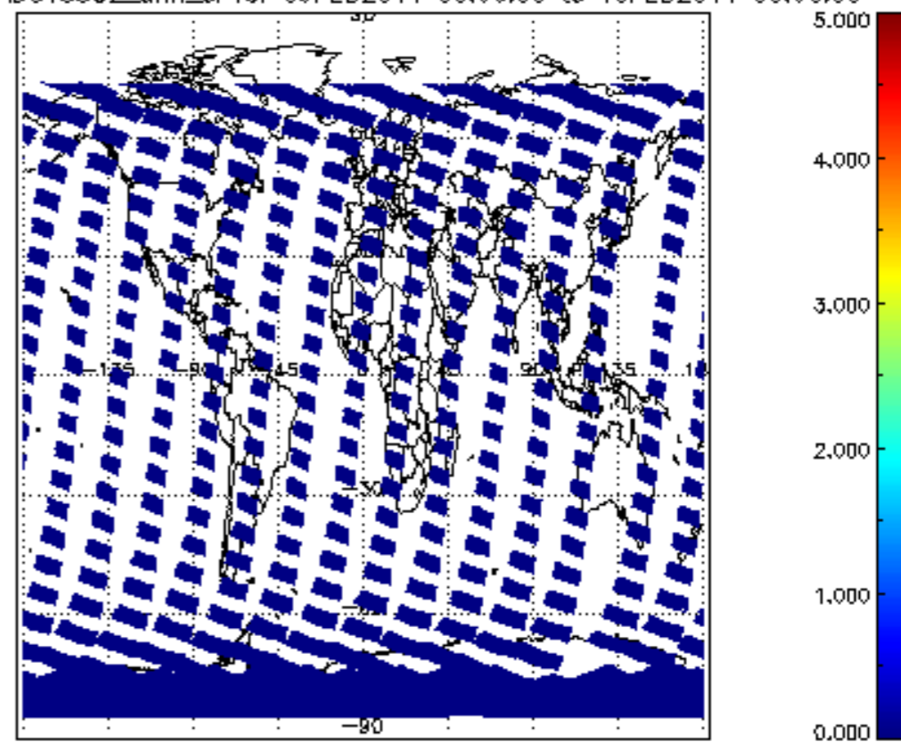
SCIOL2P_NADUV5S02_amf_cl for 09FEB2011 00:00:00 to 10FEB2011 00:00:00
