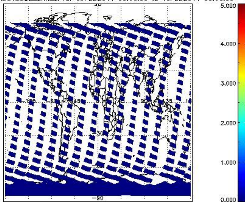
SCIOL2P_NADUV5S02_amf_cl for 09FEB2011 00:00:00 to 10FEB2011 00:00:00
