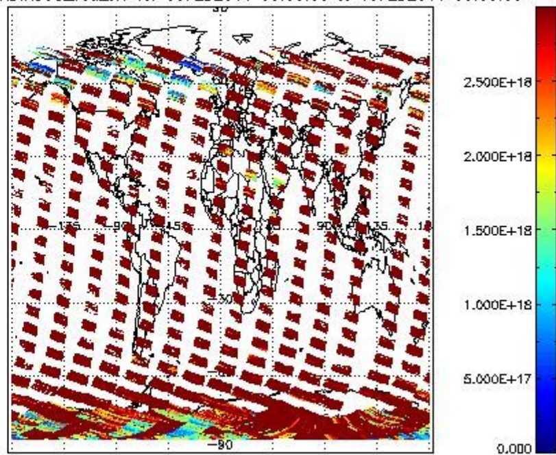
SCIO2P_NADIR3CO_vcd_err for 09FEB2011 00:00:00 to 10FEB2011 00:00:00
