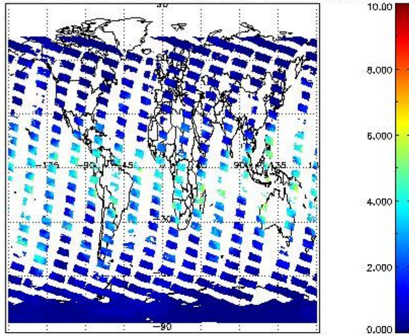
SCIOL2P_NADUV8H2O_vcd for 09FEB2011 00:00:00 to 10FEB2011 00:00:00
