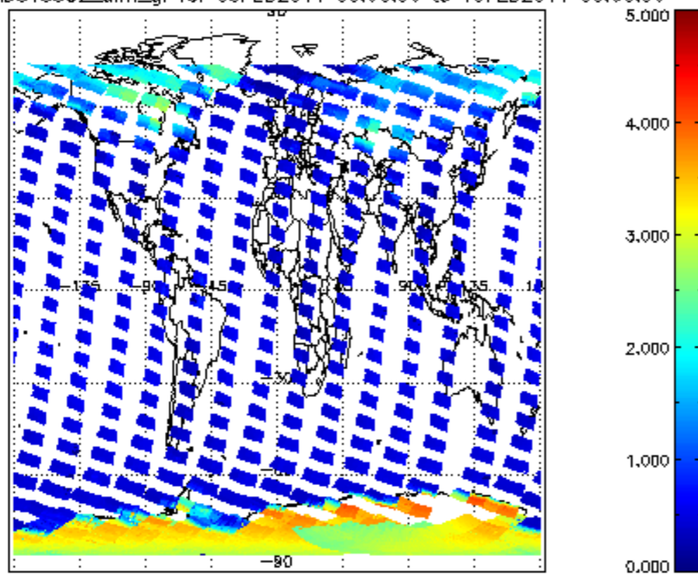
SCIOL2P_NADUV5S02_amf_gr for 09FEB2011 00:00:00 to 10FEB2011 00:00:00
