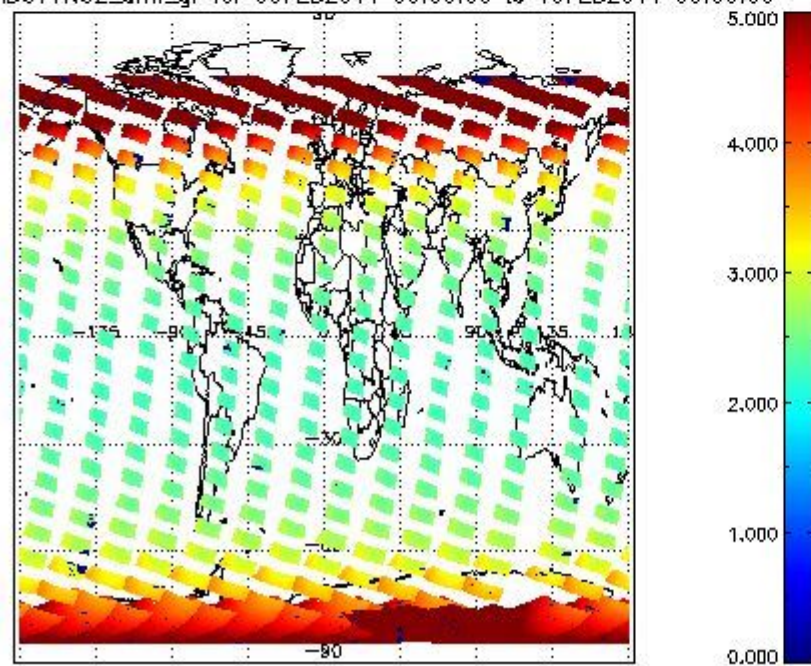
SCIOL2P_NADUV1N02_amf_gr for 09FEB2011 00:00:00 to 10FEB2011 00:00:00
