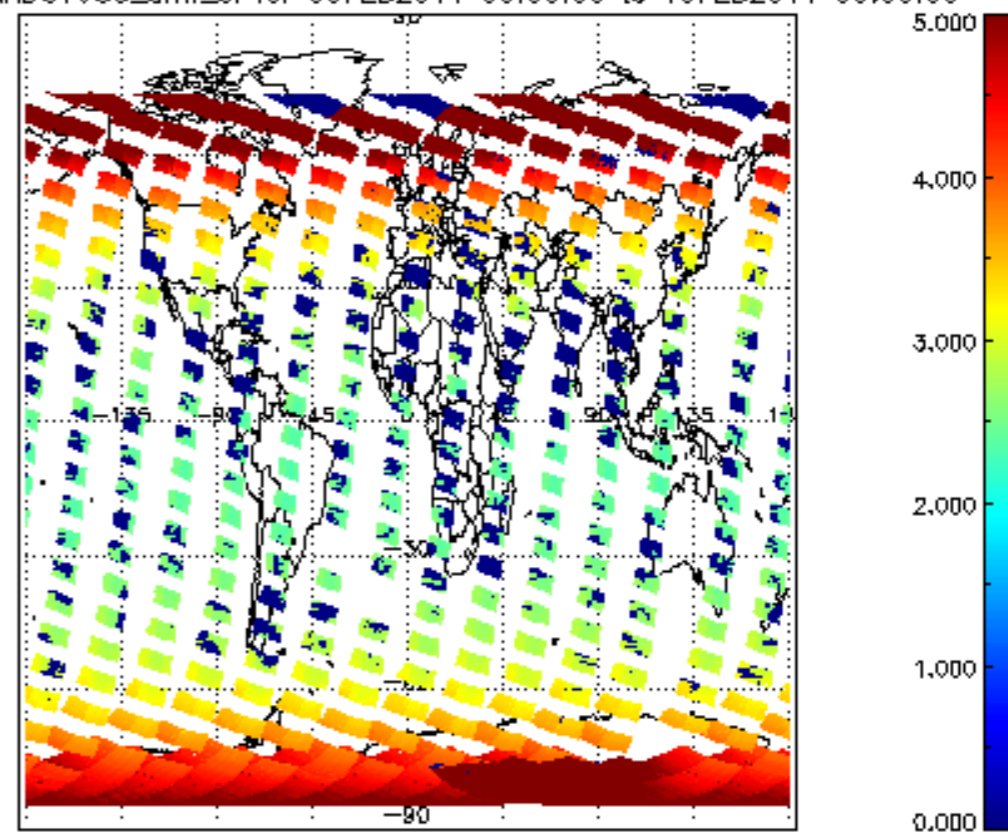
SCIOL2P_NADUV003_amf_cl for 09FEB2011 00:00:00 to 10FEB2011 00:00:00
