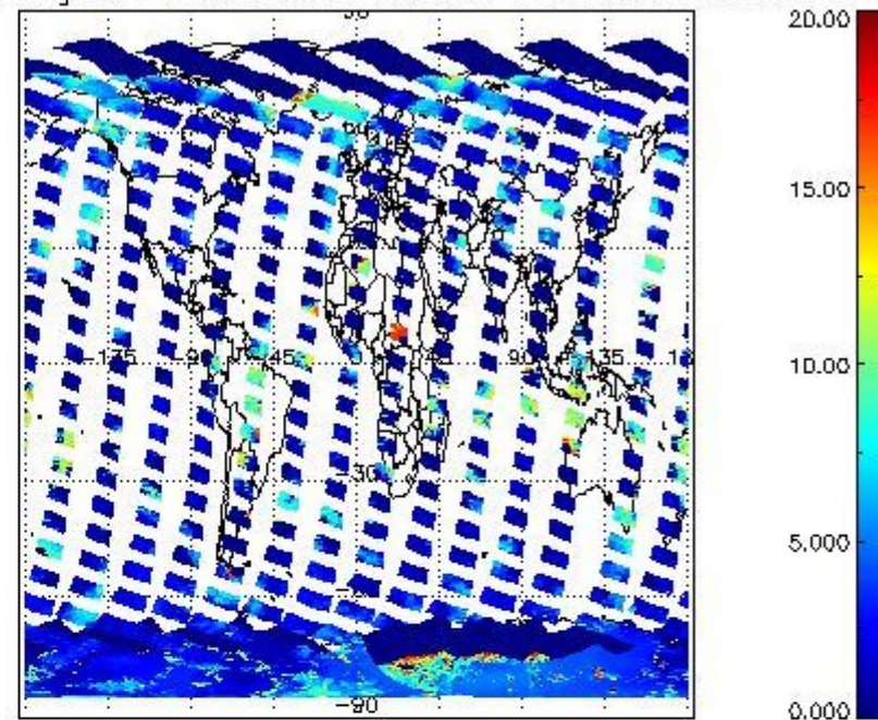
cL_top_height for 09FEB2011 00:00:00 to 10FEB2011 00:00:00
