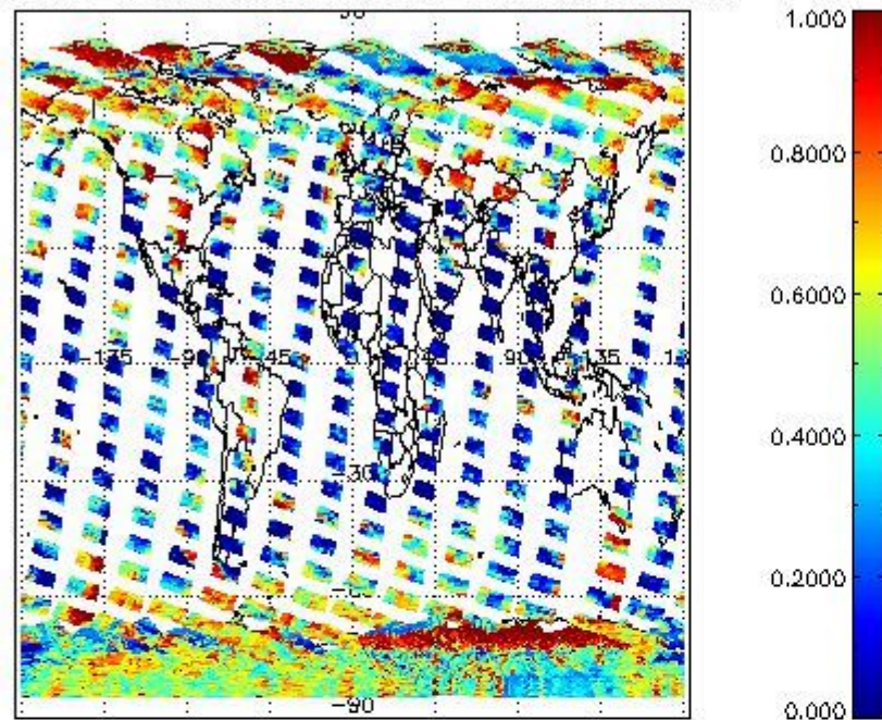
cL_frac for 09FEB2011 00:00:00 to 10FEB2011 00:00:00
