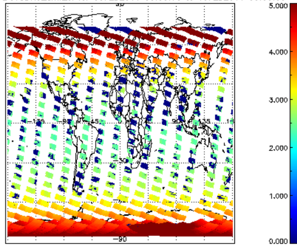
SCIOL2P_NADUV3BRO_amf_cl for 09FEB2011 00:00:00 to 10FEB2011 00:00:00
