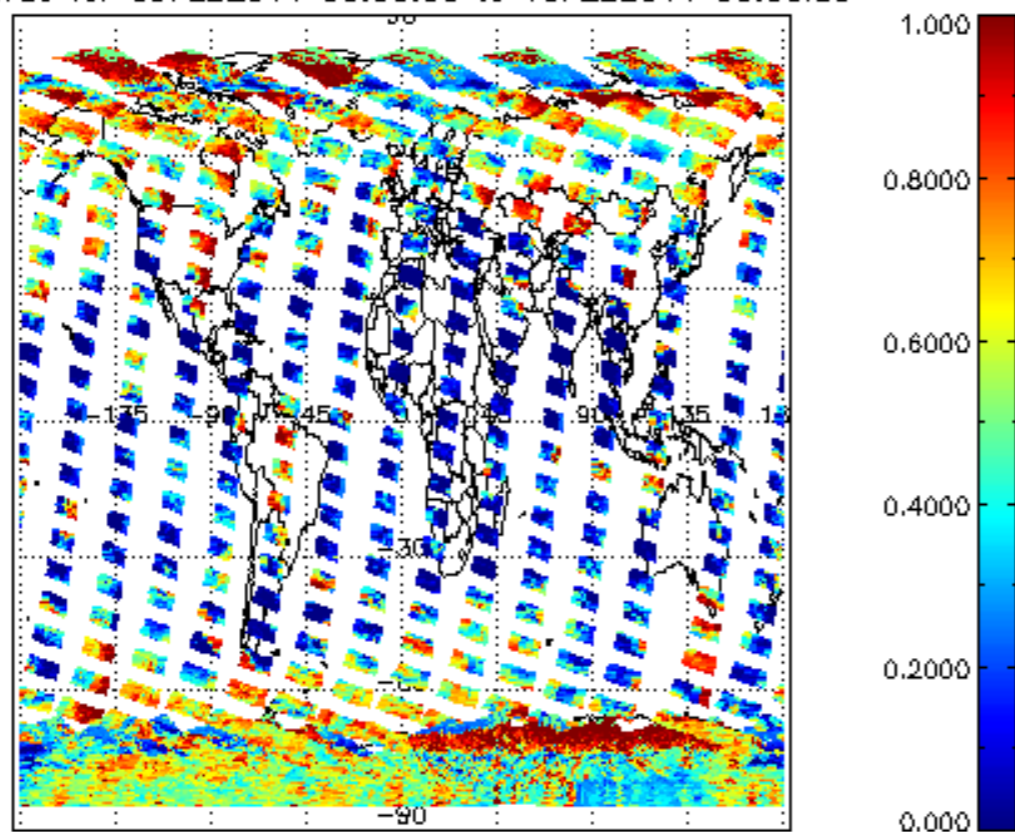
cL_frac for 09FEB2011 00:00:00 to 10FEB2011 00:00:00
