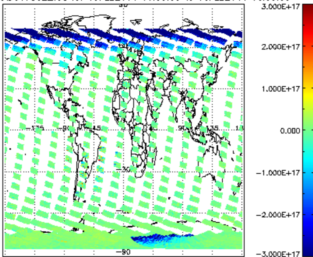
SCIOL2P_NADUV7S02_vcd for 09FEB2011 00:00:00 to 10FEB2011 00:00:00
