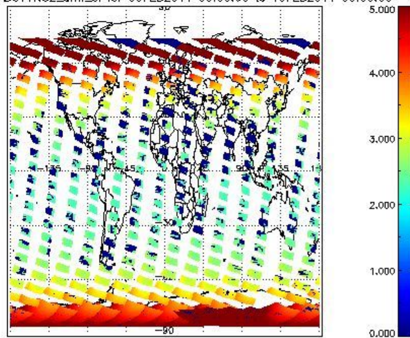
SCIOL2P_NADUV1N02_amf_cl for 09FEB2011 00:00:00 to 10FEB2011 00:00:00
