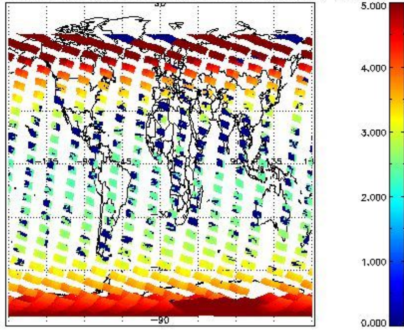
SCIOL2P_NADUV3BRO_amf_cl for 09FEB2011 00:00:00 to 10FEB2011 00:00:00
