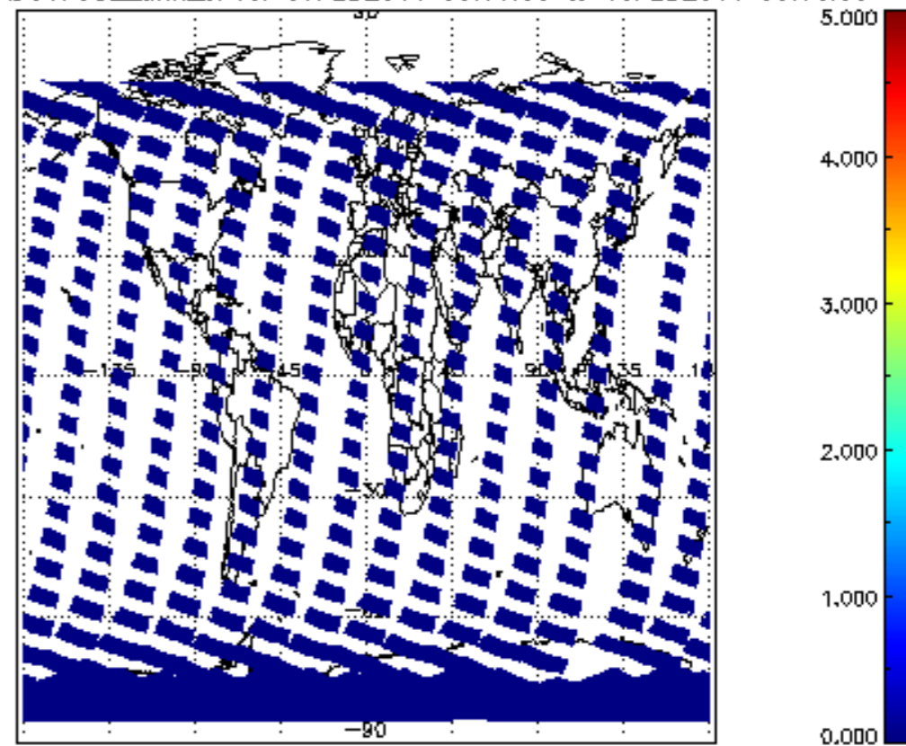
SCIOL2P_NADUV7S02_amf_cl for 09FEB2011 00:00:00 to 10FEB2011 00:00:00
