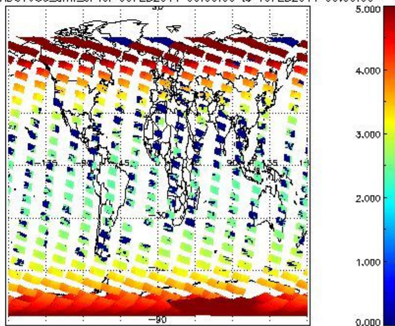
SCIOL2P_NADUV003_amf_cl for 09FEB2011 00:00:00 to 10FEB2011 00:00:00
