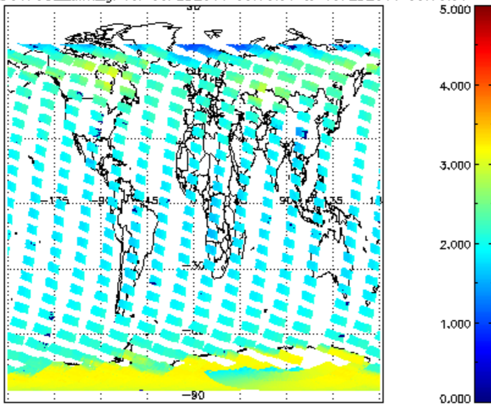
SCIOL2P_NADUV7S02_amf_gr for 09FEB2011 00:00:00 to 10FEB2011 00:00:00
