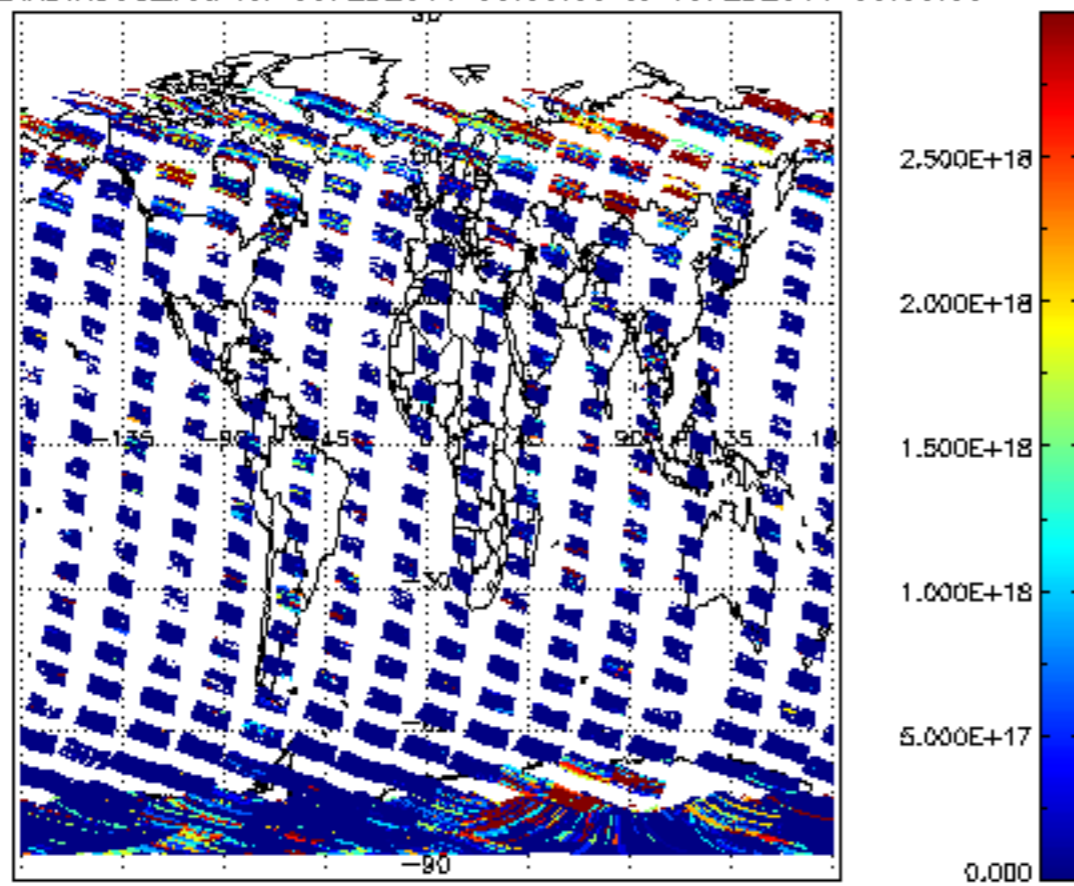
SCIOL2P_NADIR3CO_vcd for 09FEB2011 00:00:00 to 10FEB2011 00:00:00
