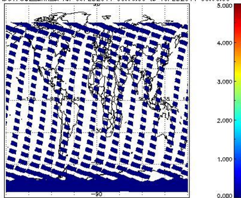
SCIOL2P_NADUV7S02_amf_cl for 09FEB2011 00:00:00 to 10FEB2011 00:00:00
