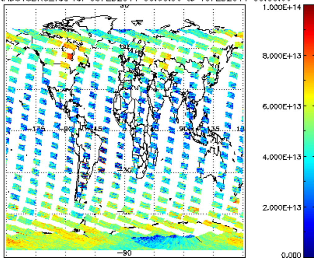
SCIOL2P_NADUV3BRO_vcd for 09FEB2011 00:00:00 to 10FEB2011 00:00:00
