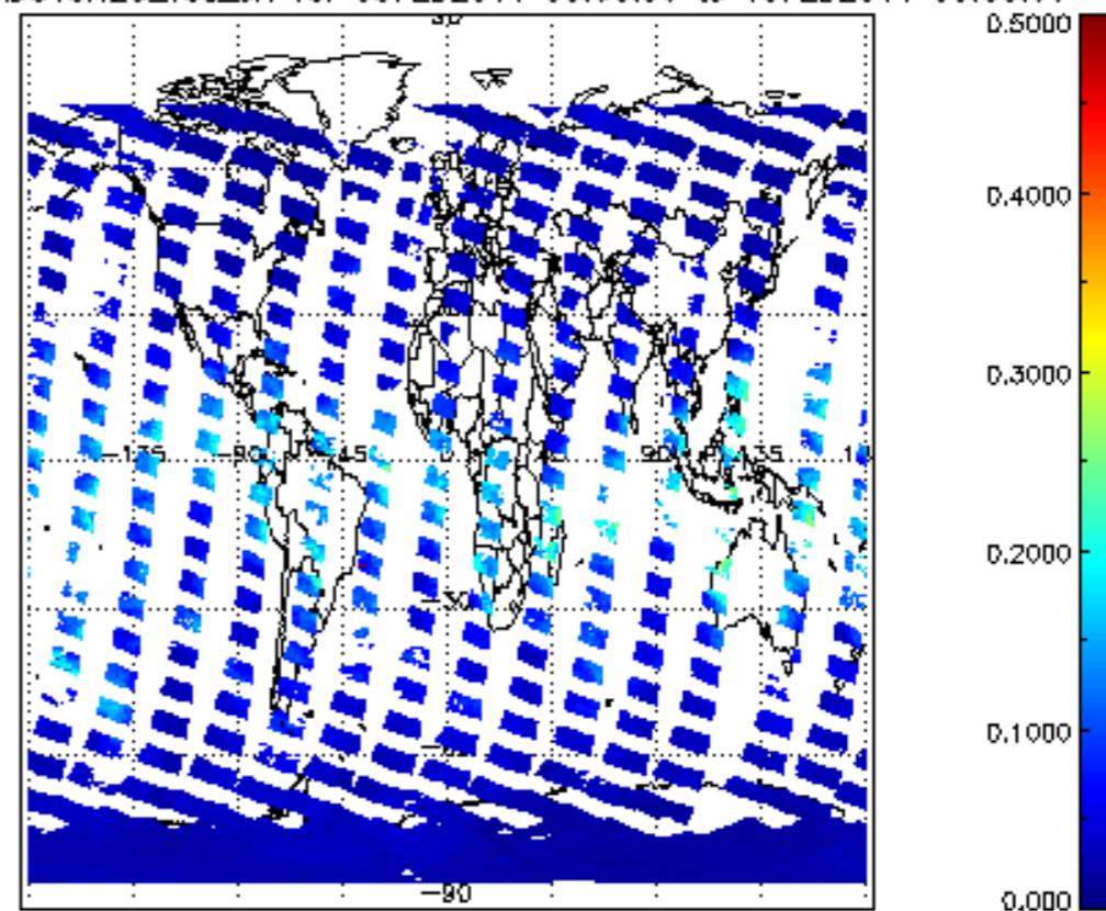
SCIOL2P_NADUV8H2O_vcd_err for 09FEB2011 00:00:00 to 10FEB2011 00:00:00
