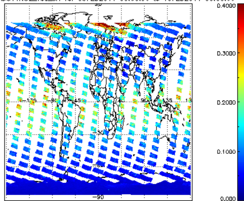
SCIOL2P_NADUV1N02_vcd_err for 09FEB2011 00:00:00 to 10FEB2011 00:00:00
