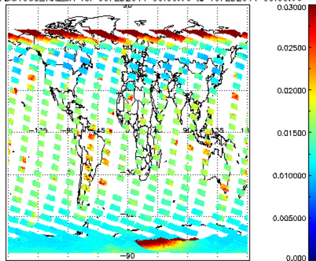
SCIOL2P_NADUV003_vcd_err for 09FEB2011 00:00:00 to 10FEB2011 00:00:00
