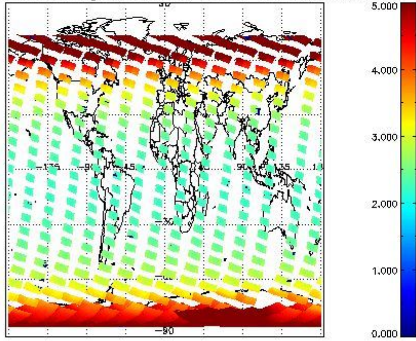
SCIOL2P_NADUV3BRO_amf_gr for 09FEB2011 00:00:00 to 10FEB2011 00:00:00
