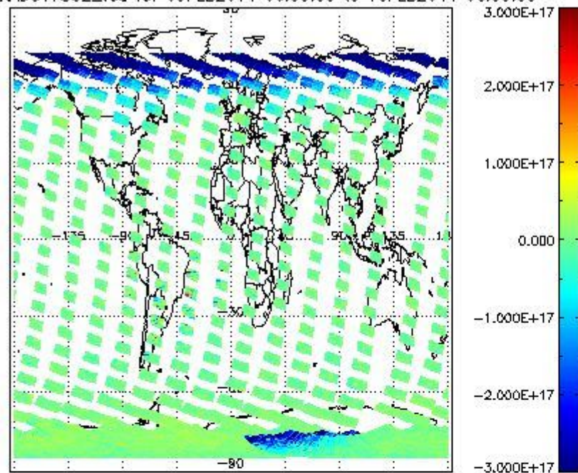
SCIOL2P_NADUV7S02_vcd for 09FEB2011 00:00:00 to 10FEB2011 00:00:00
