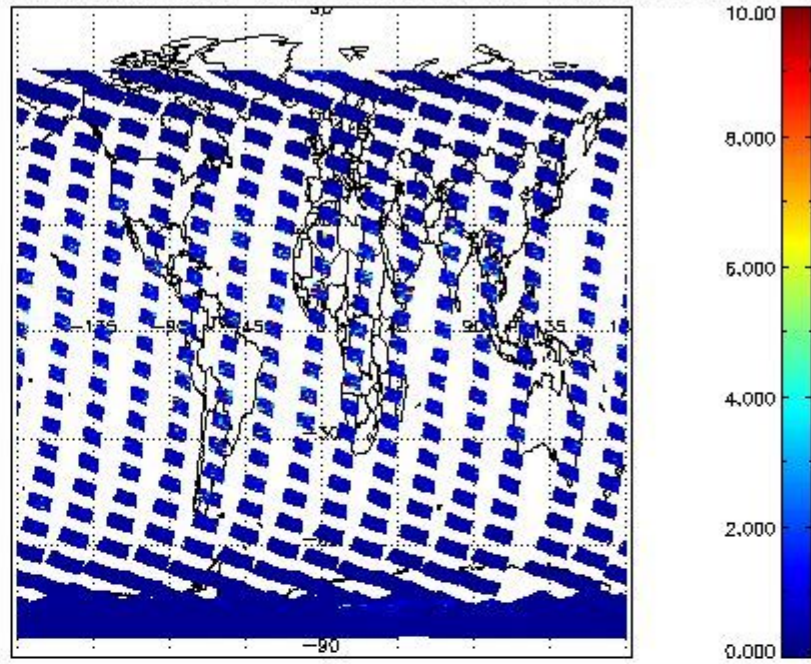
SCIOL2P_NADUV3BRO_vcd_err for 09FEB2011 00:00:00 to 10FEB2011 00:00:00
