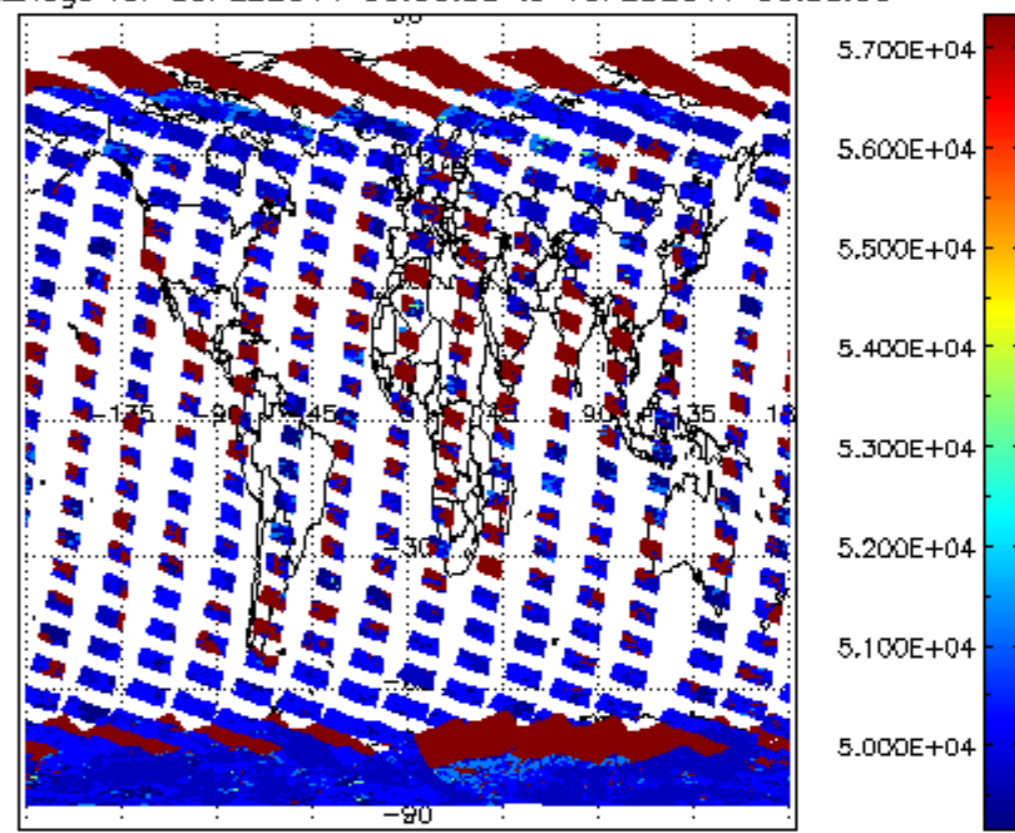
cloud_flags for 09FEB2011 00:00:00 to 10FEB2011 00:00:00
