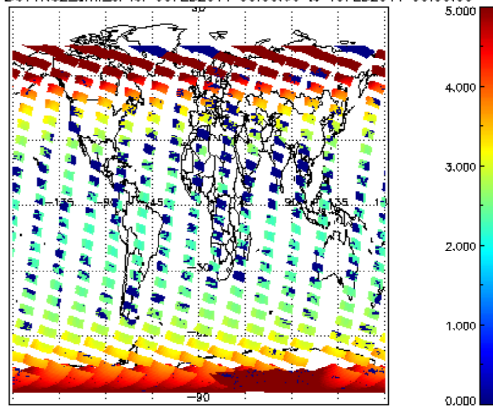
SCIOL2P_NADUV1N02_amf_cl for 09FEB2011 00:00:00 to 10FEB2011 00:00:00
