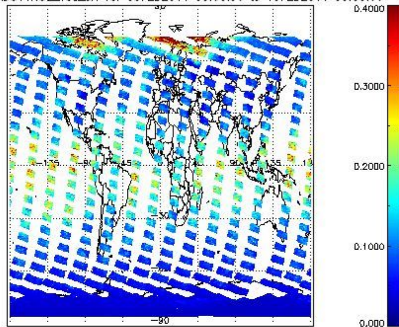
SCIOL2P_NADUV1N02_vcd_err for 09FEB2011 00:00:00 to 10FEB2011 00:00:00
