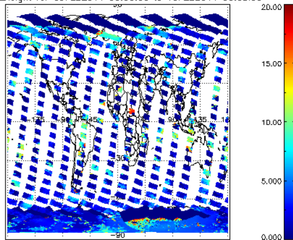
cL_top_height for 09FEB2011 00:00:00 to 10FEB2011 00:00:00
