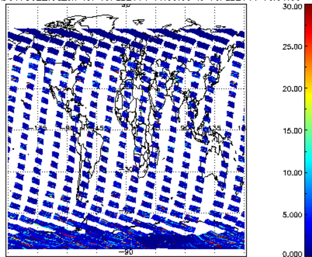
SCIOL2P_NADUV7S02_vcd_err for 09FEB2011 00:00:00 to 10FEB2011 00:00:00
