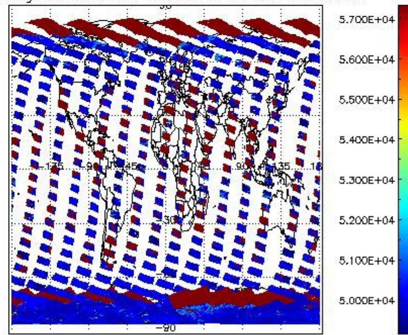
cloud_flags for 09FEB2011 00:00:00 to 10FEB2011 00:00:00
