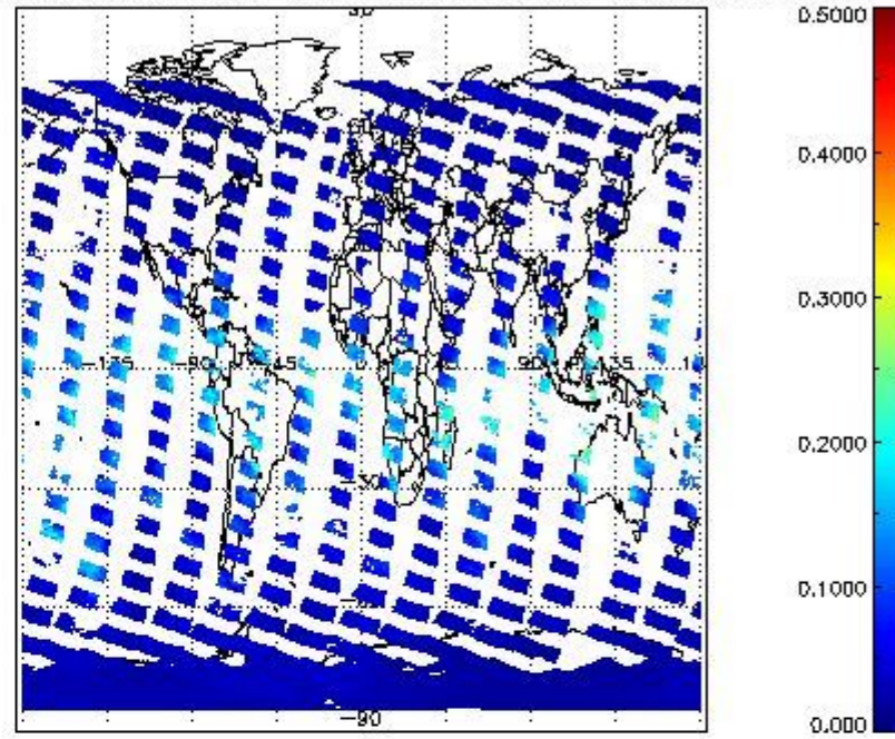
SCIOL2P_NADUV8H2O_vcd_err for 09FEB2011 00:00:00 to 10FEB2011 00:00:00
