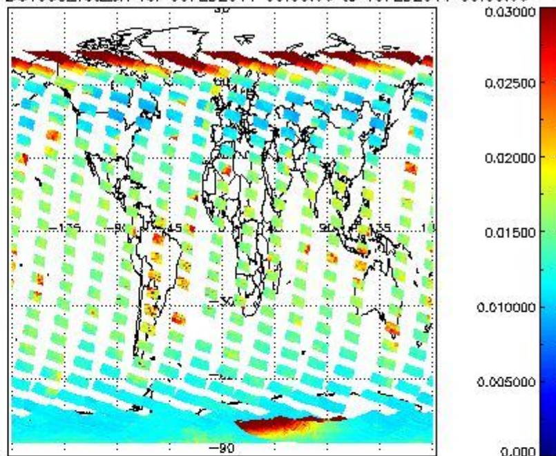
SCIOL2P_NADUV003_vcd_err for 09FEB2011 00:00:00 to 10FEB2011 00:00:00
