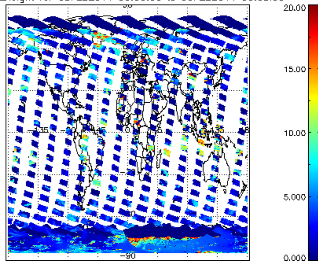
cL_top_height for 08FEB2011 00:00:00 to 09FEB2011 00:00:00
