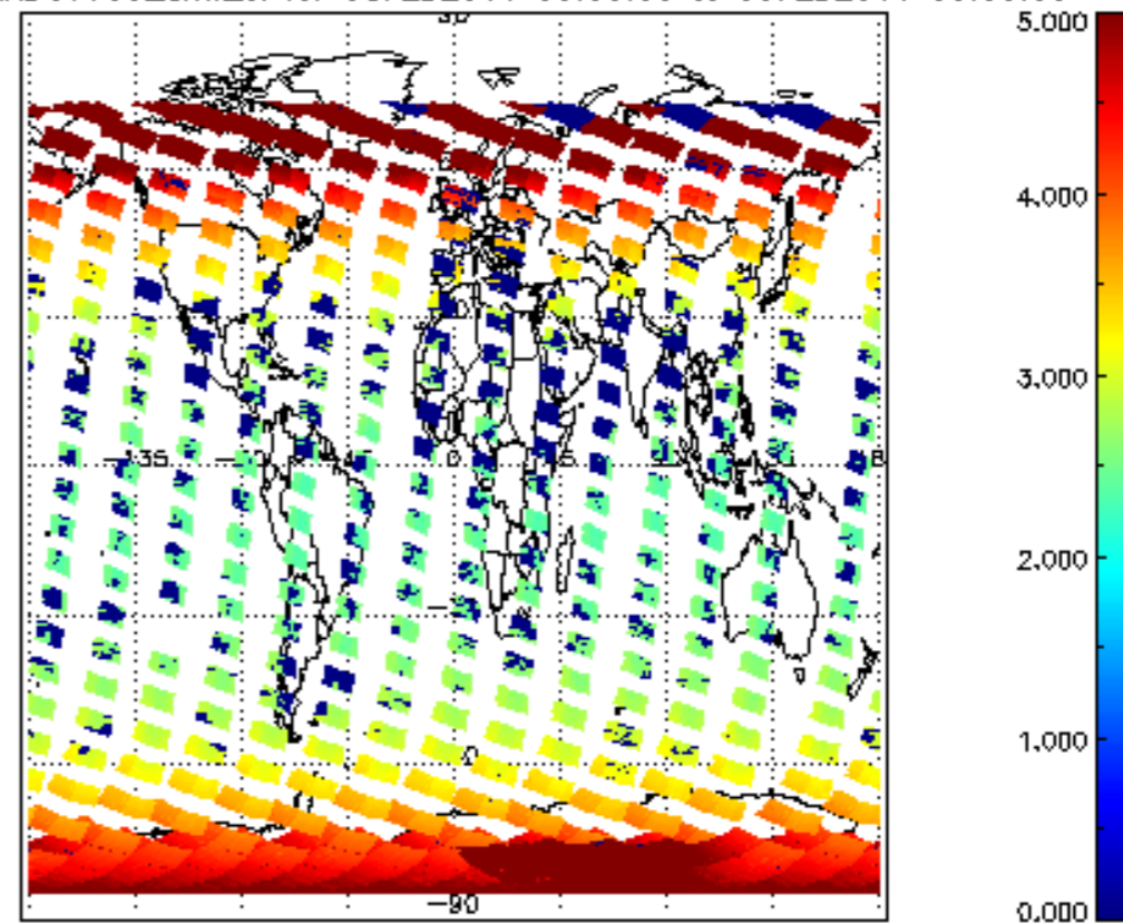
SCIOL2P_NADUV003_amf_cl for 08FEB2011 00:00:00 to 09FEB2011 00:00:00
