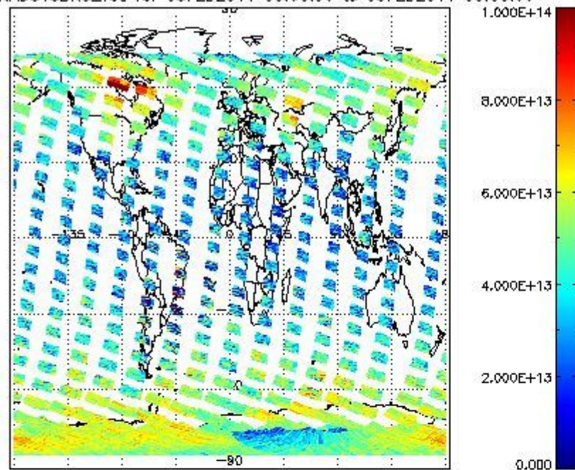
SCIOL2P_NADUV3BRO_vcd for 08FEB2011 00:00:00 to 09FEB2011 00:00:00
