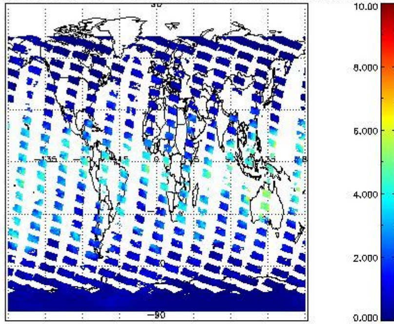
SCIOL2P_NADUV8H2O_vcd for 08FEB2011 00:00:00 to 09FEB2011 00:00:00
