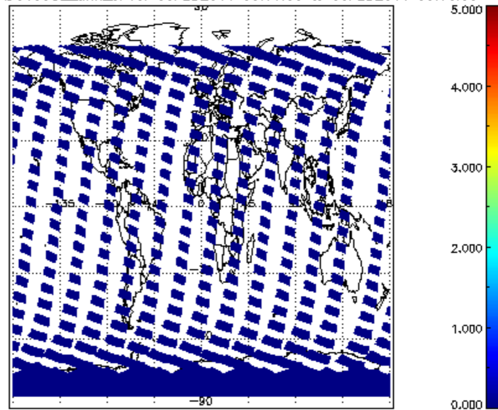
SCIOL2P_NADUV5S02_amf_cl for 08FEB2011 00:00:00 to 09FEB2011 00:00:00
