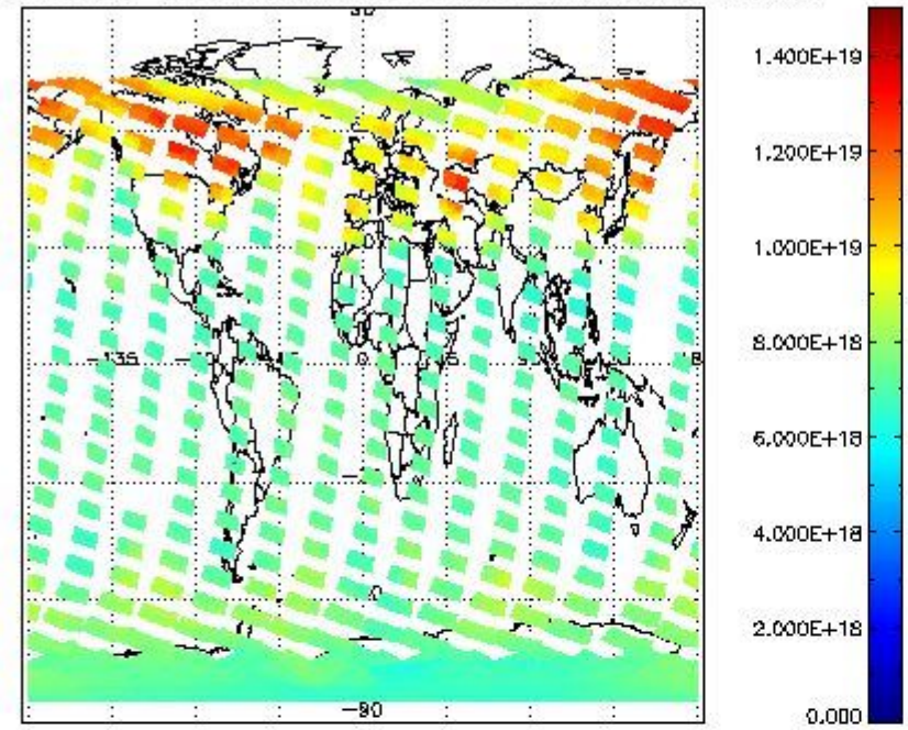
SCIOL2P_NADUV003_vcd for 08FEB2011 00:00:00 to 09FEB2011 00:00:00
