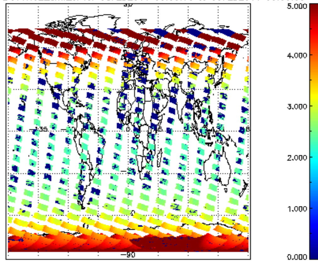
SCIOL2P_NADUV1N02_amf_cl for 08FEB2011 00:00:00 to 09FEB2011 00:00:00
