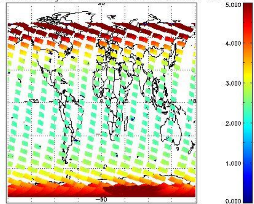
SCIOL2P_NADUV003_amf_gr for 08FEB2011 00:00:00 to 09FEB2011 00:00:00
