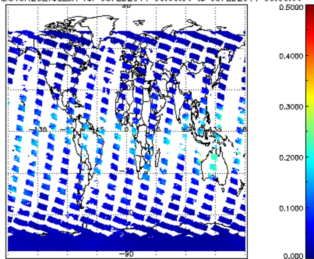
SCIOL2P_NADUV8H20_vcd_err for 08FEB2011 00:00:00 to 09FEB2011 00:00:00
