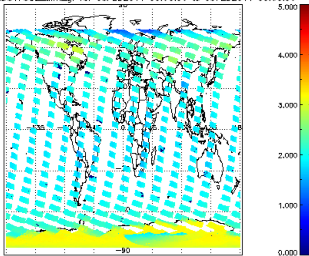
SCIOL2P_NADUV7S02_amf_gr for 08FEB2011 00:00:00 to 09FEB2011 00:00:00
