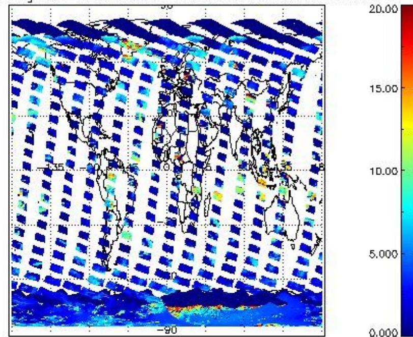
cL_top_height for 08FEB2011 00:00:00 to 09FEB2011 00:00:00
