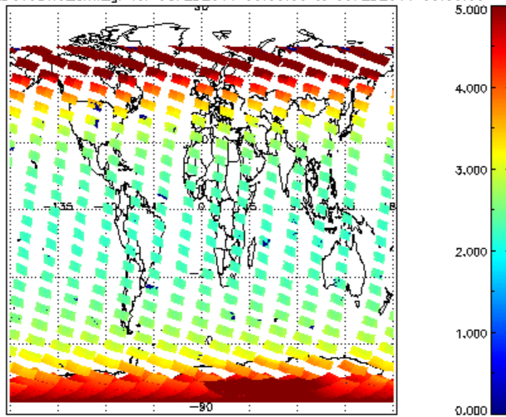
SCIOL2P_NADUV3BRO_amf_gr for 08FEB2011 00:00:00 to 09FEB2011 00:00:00
