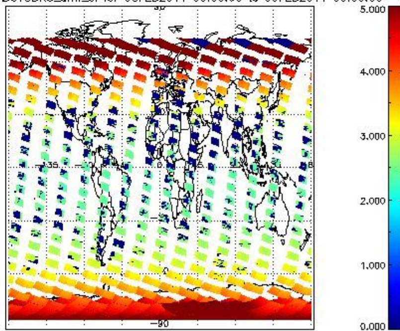
SCIOL2P_NADUV3BRO_amf_cl for 08FEB2011 00:00:00 to 09FEB2011 00:00:00
