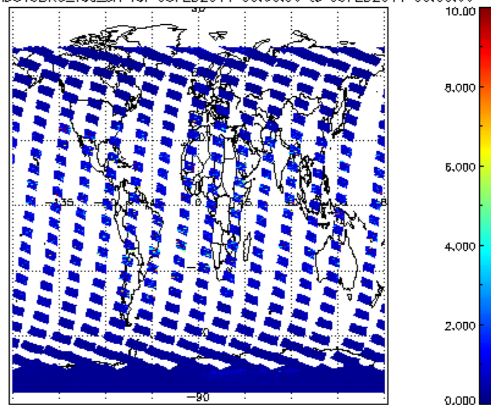
SCIOL2P_NADUV3BRO_vcd_err for 08FEB2011 00:00:00 to 09FEB2011 00:00:00
