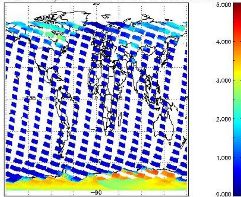
SCIOL2P_NADUV5S02_amf_gr for 08FEB2011 00:00:00 to 09FEB2011 00:00:00
