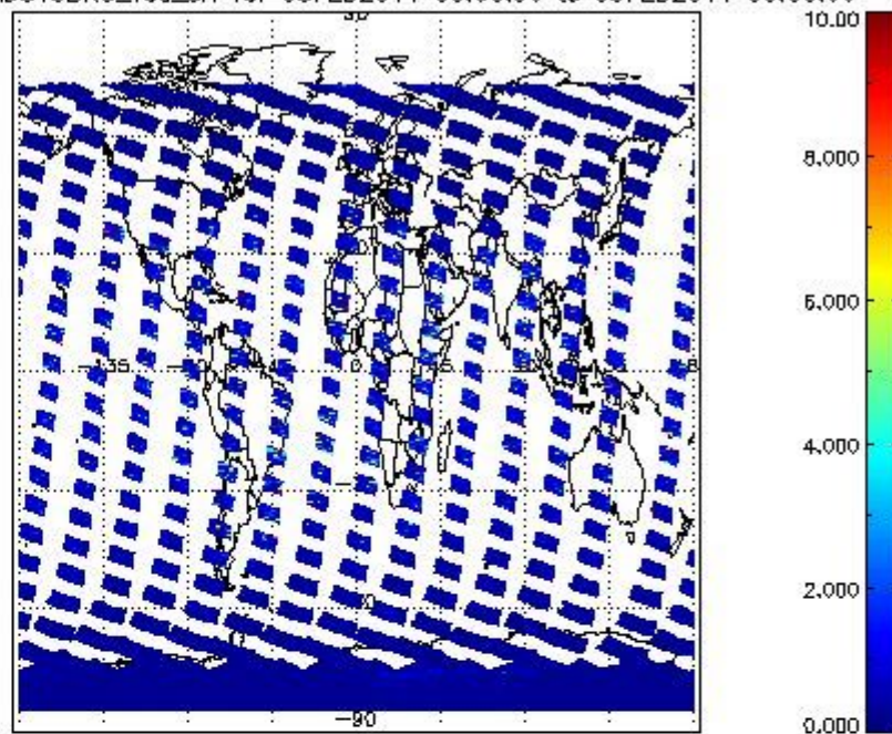
SCIOL2P_NADUV3BRO_vcd_err for 08FEB2011 00:00:00 to 09FEB2011 00:00:00
