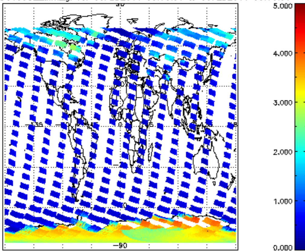
SCIOL2P_NADUV5S02_amf_gr for 08FEB2011 00:00:00 to 09FEB2011 00:00:00
