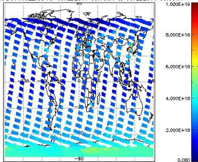
SCIOL2P_NADUV1N02_vcd for 08FEB2011 00:00:00 to 09FEB2011 00:00:00
