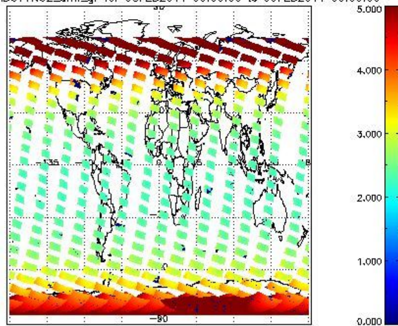
SCIOL2P_NADUV1N02_amf_gr for 08FEB2011 00:00:00 to 09FEB2011 00:00:00
