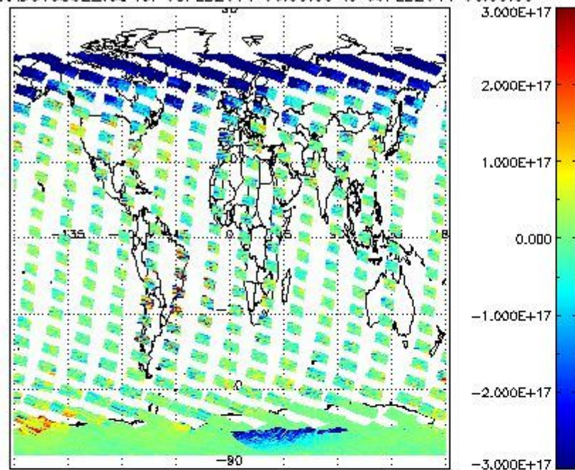
SCIOL2P_NADUV5S02_vcd for 08FEB2011 00:00:00 to 09FEB2011 00:00:00
