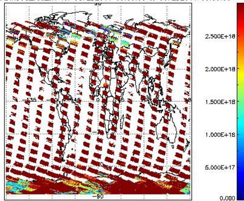
SCIDL2P_NADIR3CO_vcd_err for 08FEB2011 00:00:00 to 09FEB2011 00:00:00
