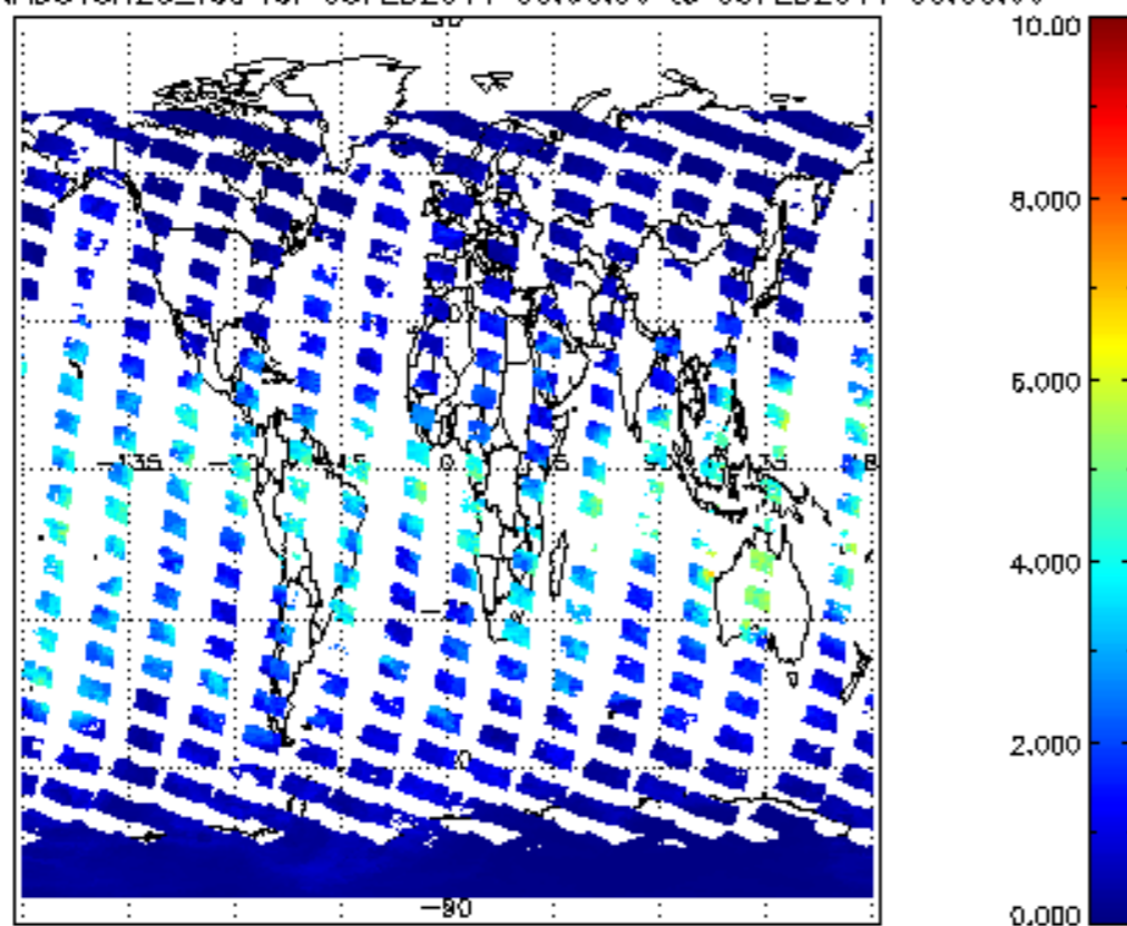
SCIOL2P_NADUV8H20_vcd for 08FEB2011 00:00:00 to 09FEB2011 00:00:00
