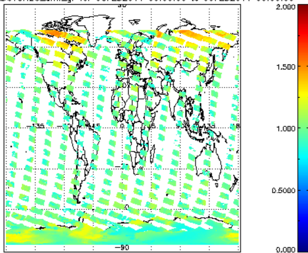
SCIOL2P_NADUV8H20_amf_gr for 08FEB2011 00:00:00 to 09FEB2011 00:00:00
