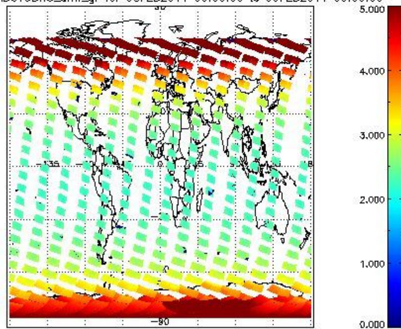
SCIOL2P_NADUV3BRO_amf_gr for 08FEB2011 00:00:00 to 09FEB2011 00:00:00
