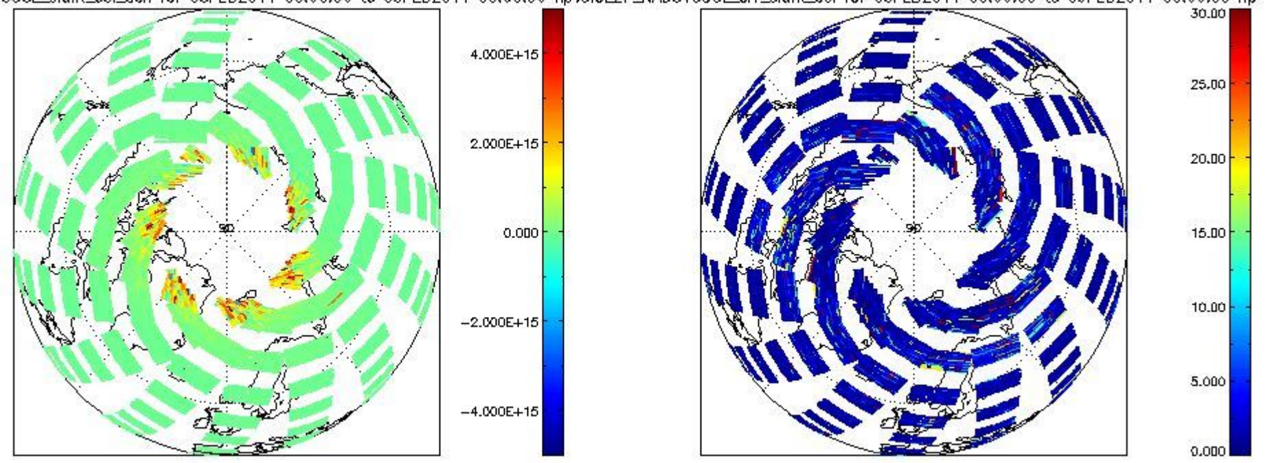
CIOL2P_NADUV60CL_slant_col_den for 08FEB2011 00:00:00 to 09FEB2011 00:00:00 np; CIOL2P_NADUV60CL_err_slant_col for 08FEB2011 00:00:00 to 09FEB2011 00:00:00 np
