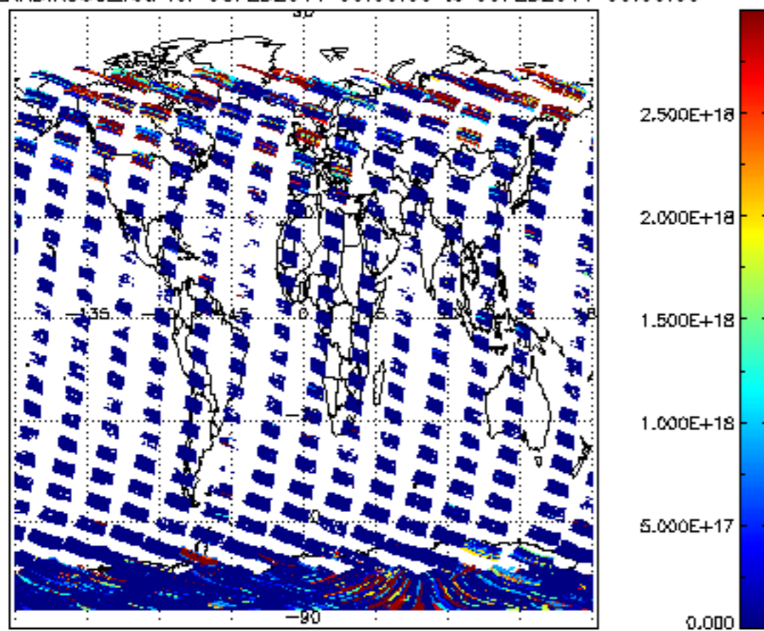
SCIOL2P_NADIR3CO_vcd for 08FEB2011 00:00:00 to 09FEB2011 00:00:00
