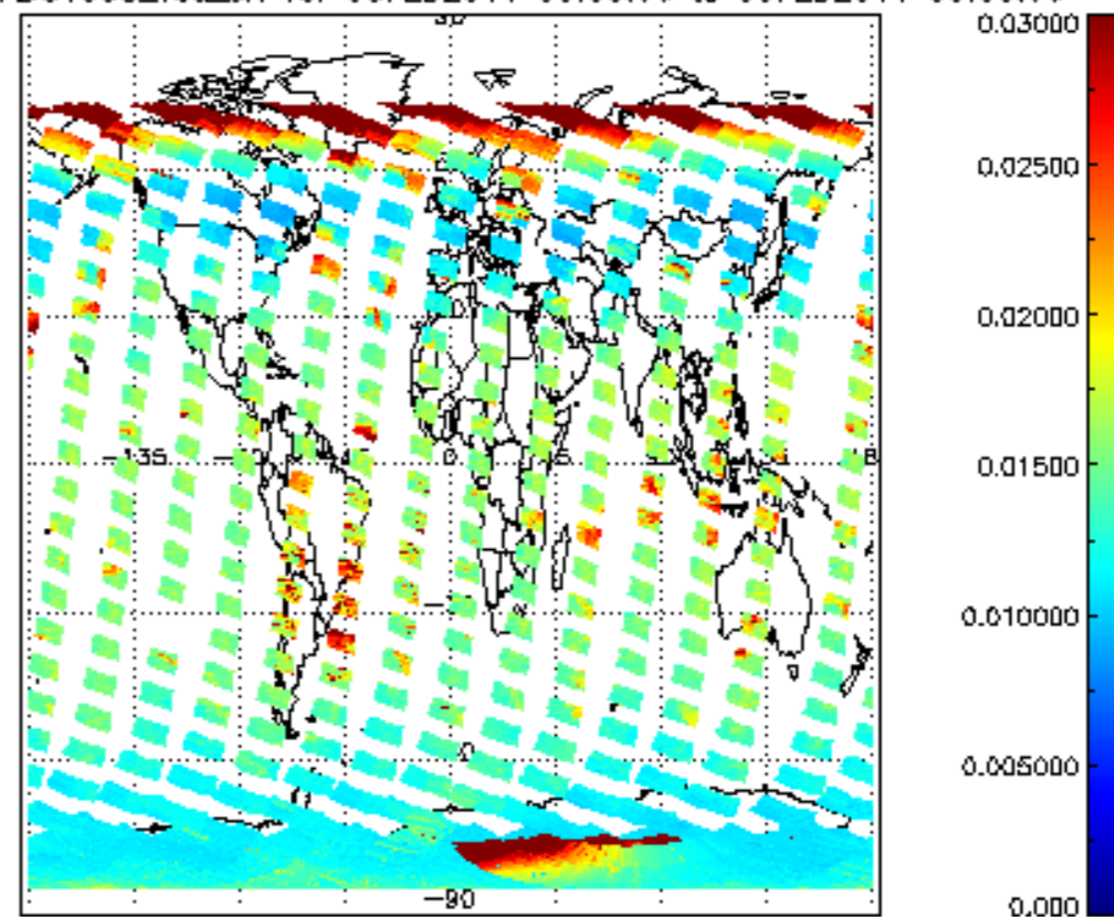
SCIOL2P_NADUV003_vcd_err for 08FEB2011 00:00:00 to 09FEB2011 00:00:00
