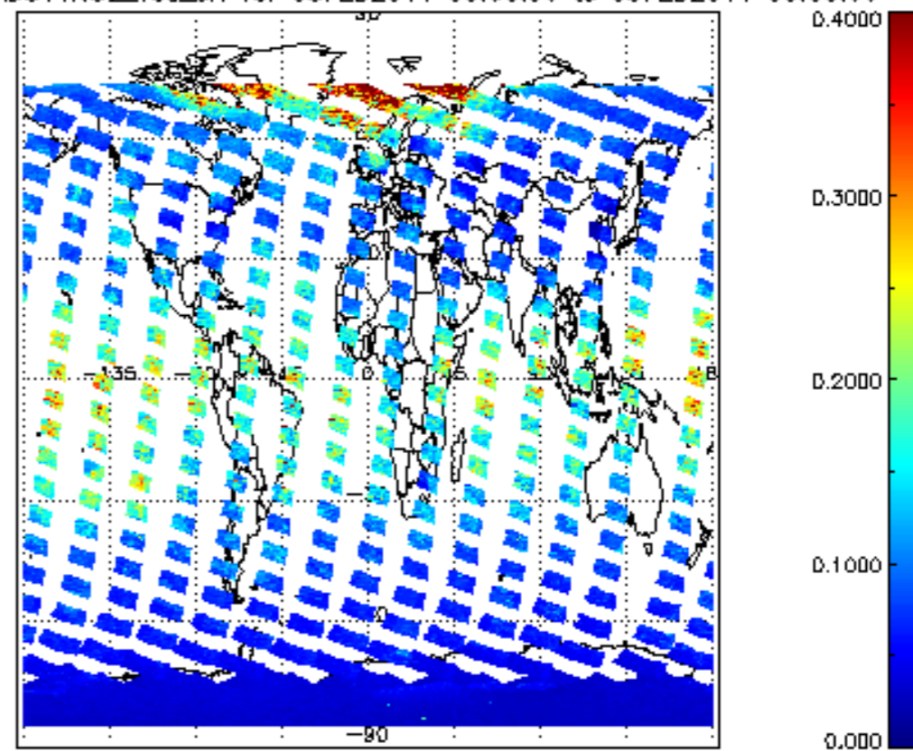
SCIOL2P_NADUV1N02_vcd_err for 08FEB2011 00:00:00 to 09FEB2011 00:00:00
