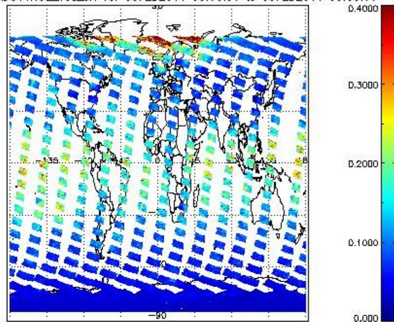
SCIOL2P_NADUV1N02_vcd_err for 08FEB2011 00:00:00 to 09FEB2011 00:00:00
