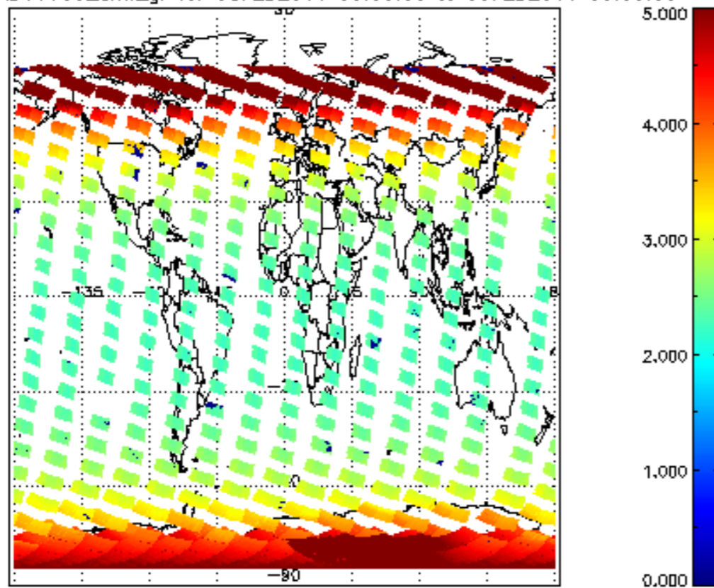
SCIOL2P_NADUV003_amf_gr for 08FEB2011 00:00:00 to 09FEB2011 00:00:00
