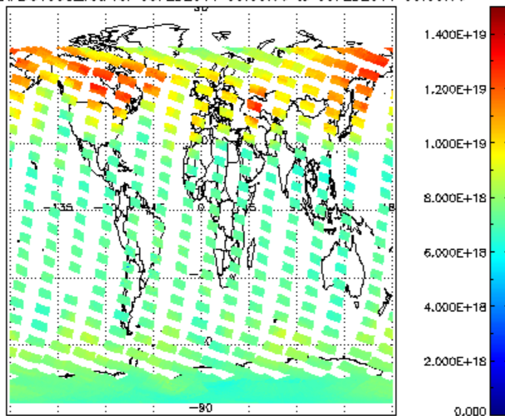
SCIOL2P_NADUV003_vcd for 08FEB2011 00:00:00 to 09FEB2011 00:00:00
