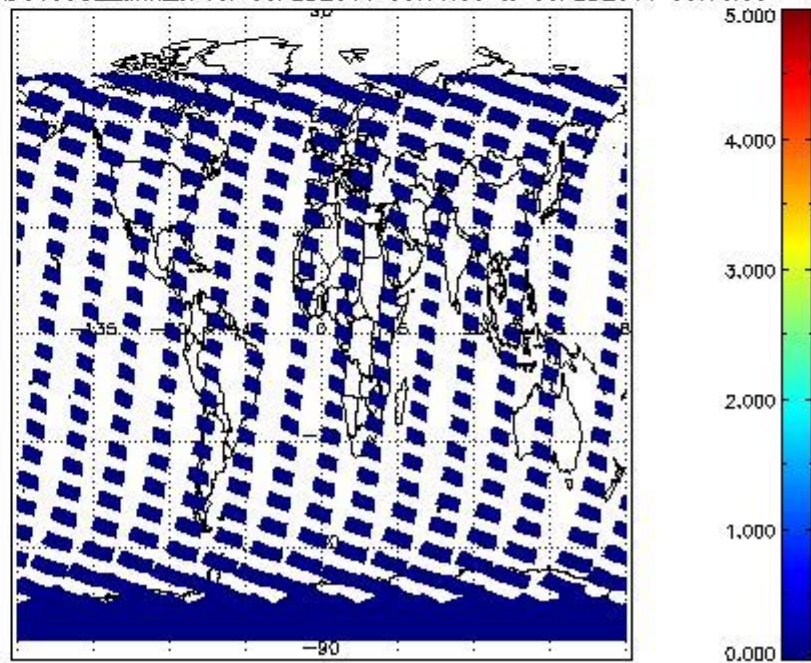
SCIOL2P_NADUV5S02_amf_cl for 08FEB2011 00:00:00 to 09FEB2011 00:00:00
