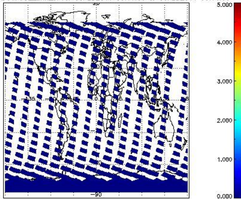
SCIOL2P_NADUV7S02_amf_cl for 08FEB2011 00:00:00 to 09FEB2011 00:00:00
