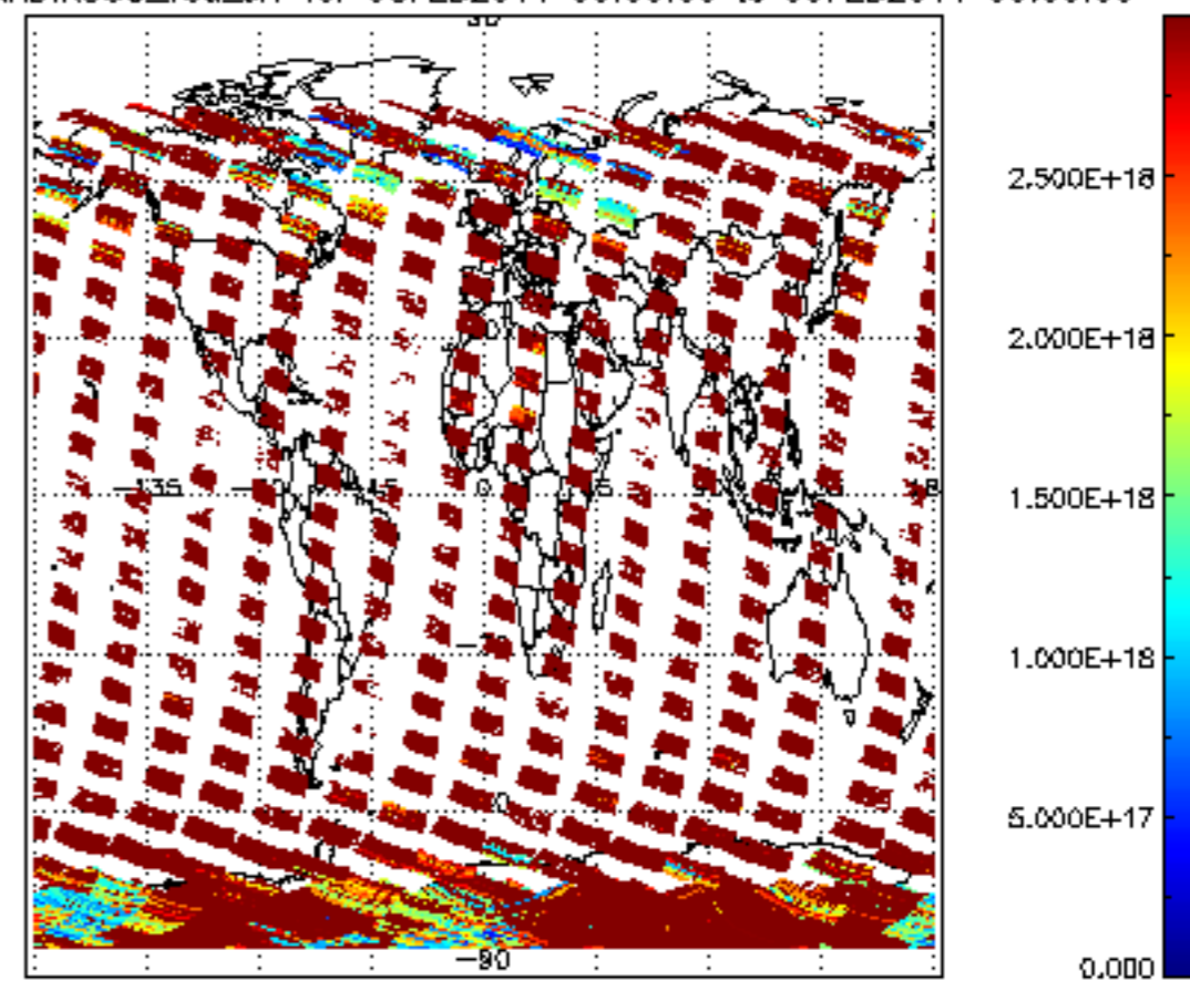
SCIOL2P_NADIR3CO_vcd_err for 08FEB2011 00:00:00 to 09FEB2011 00:00:00
