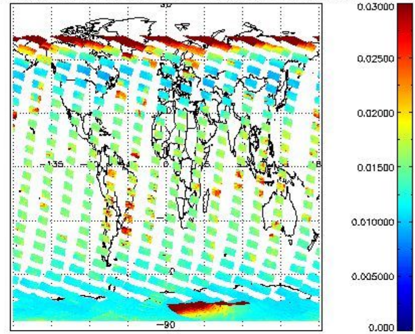
SCIOL2P_NADUV003_vcd_err for 08FEB2011 00:00:00 to 09FEB2011 00:00:00
