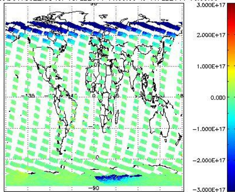
SCIOL2P_NADUV7S02_vcd for 08FEB2011 00:00:00 to 09FEB2011 00:00:00
