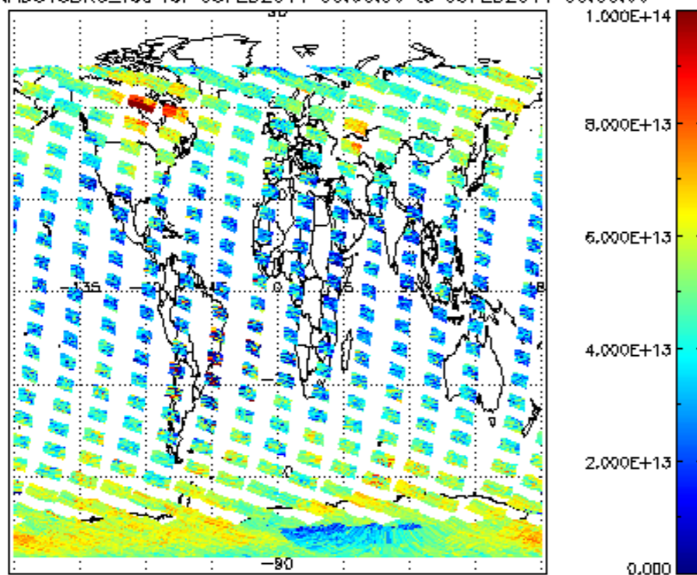
SCIOL2P_NADUV3BRO_vcd for 08FEB2011 00:00:00 to 09FEB2011 00:00:00
