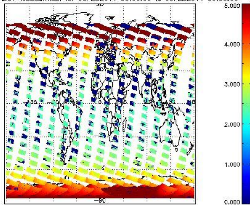
SCIOL2P_NADUV1N02_amf_cl for 08FEB2011 00:00:00 to 09FEB2011 00:00:00
