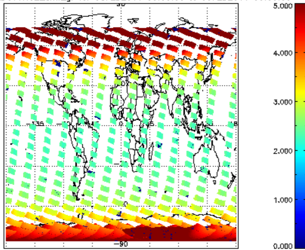
SCIOL2P_NADUV1N02_amf_gr for 08FEB2011 00:00:00 to 09FEB2011 00:00:00
