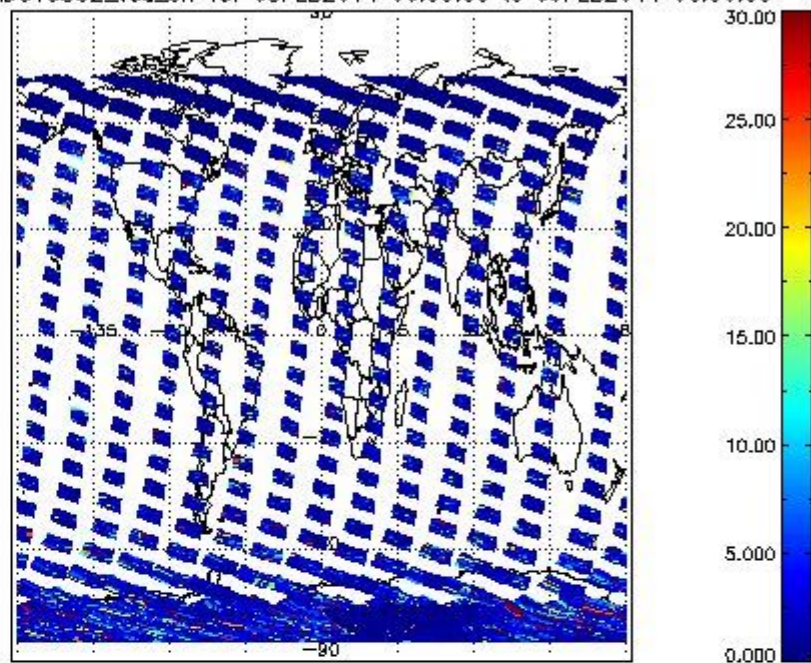
SCIOL2P_NADUV5S02_vcd_err for 08FEB2011 00:00:00 to 09FEB2011 00:00:00
