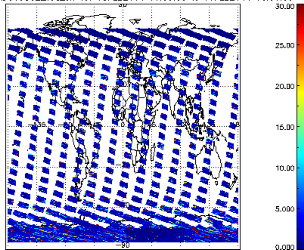
SCIOL2P_NADUV5S02_vcd_err for 08FEB2011 00:00:00 to 09FEB2011 00:00:00
