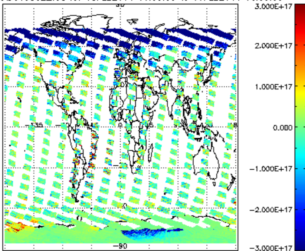
SCIOL2P_NADUV5S02_vcd for 08FEB2011 00:00:00 to 09FEB2011 00:00:00
