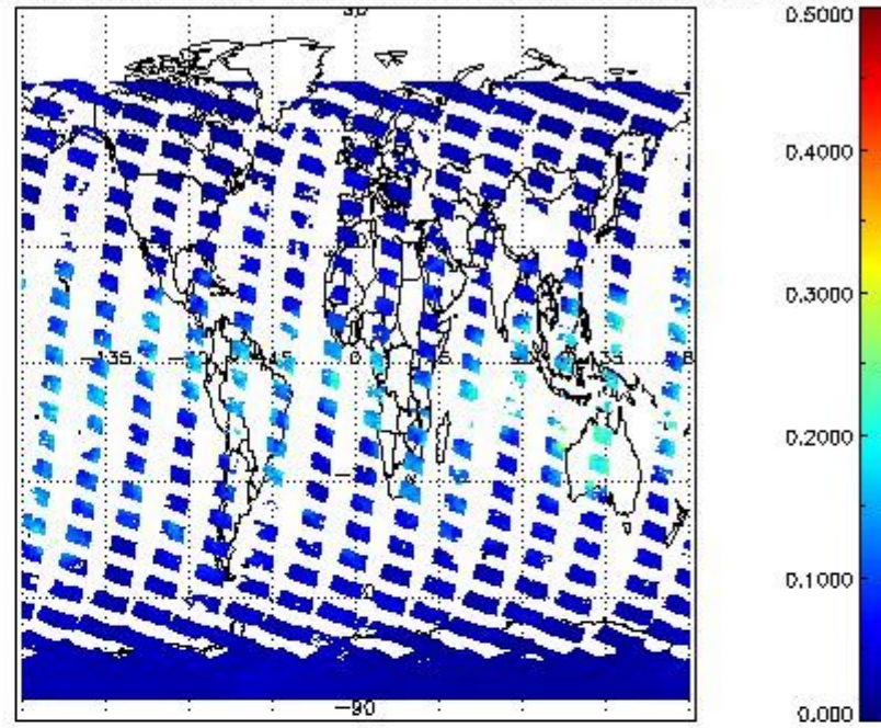
SCIOL2P_NADUV8H2O_vcd_err for 08FEB2011 00:00:00 to 09FEB2011 00:00:00
