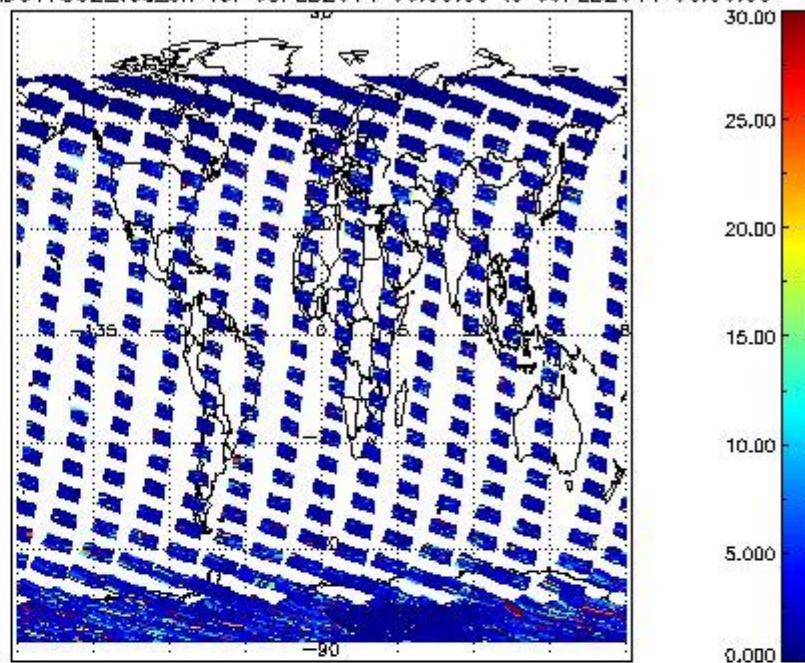
SCIOL2P_NADUV7S02_vcd_err for 08FEB2011 00:00:00 to 09FEB2011 00:00:00
