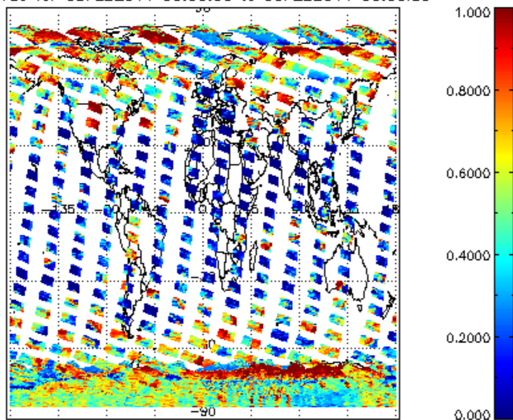
cL_frac for 08FEB2011 00:00:00 to 09FEB2011 00:00:00
