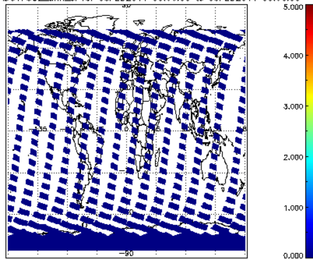
SCIOL2P_NADUV7S02_amf_cl for 08FEB2011 00:00:00 to 09FEB2011 00:00:00
