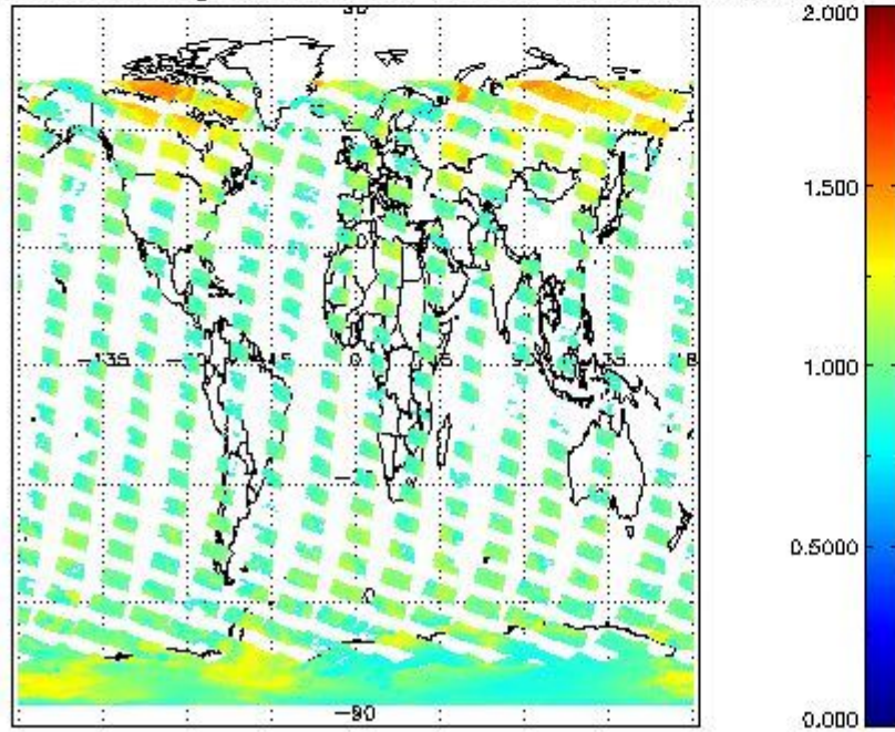
SCIOL2P_NADUV8H2O_amf_gr for 08FEB2011 00:00:00 to 09FEB2011 00:00:00
