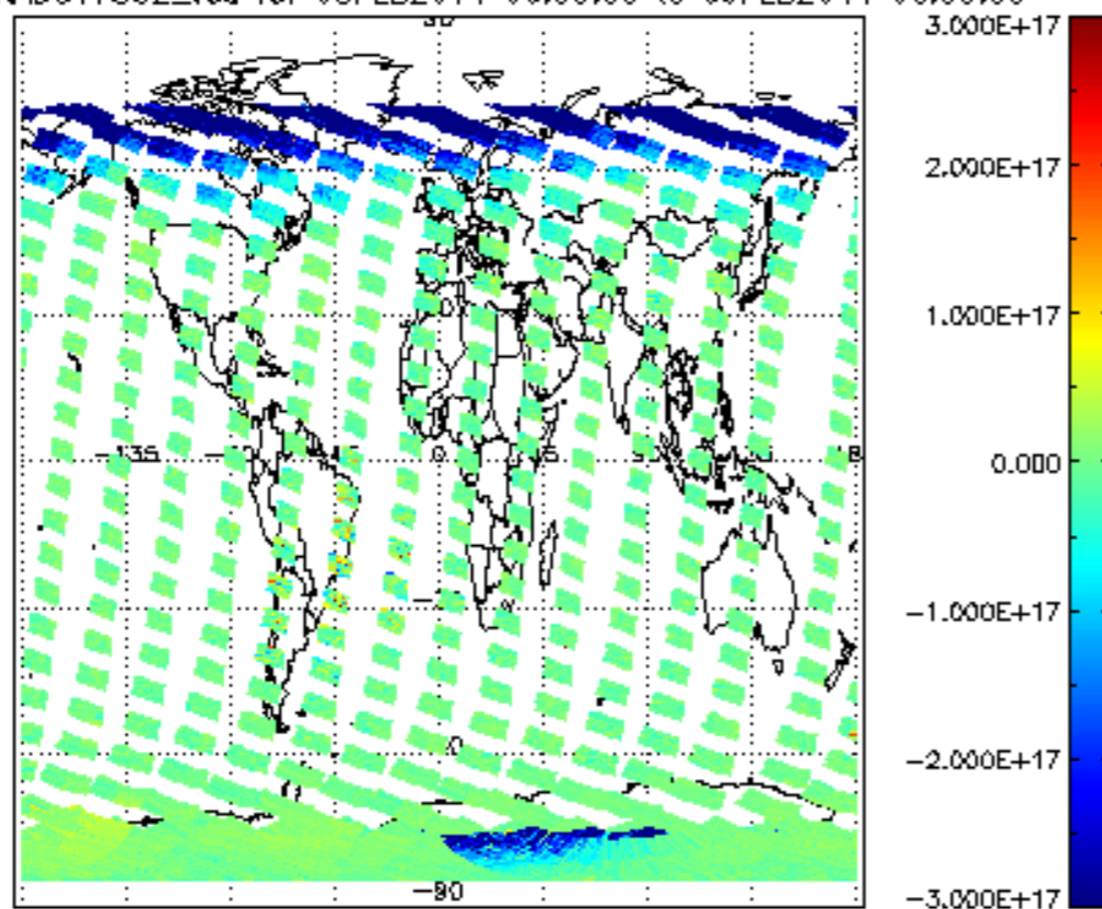
SCIOL2P_NADUV7S02_vcd for 08FEB2011 00:00:00 to 09FEB2011 00:00:00
