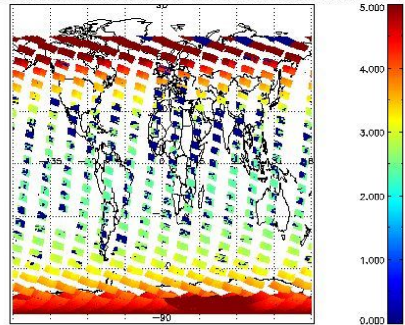
SCIOL2P_NADUV003_amf_cl for 08FEB2011 00:00:00 to 09FEB2011 00:00:00
