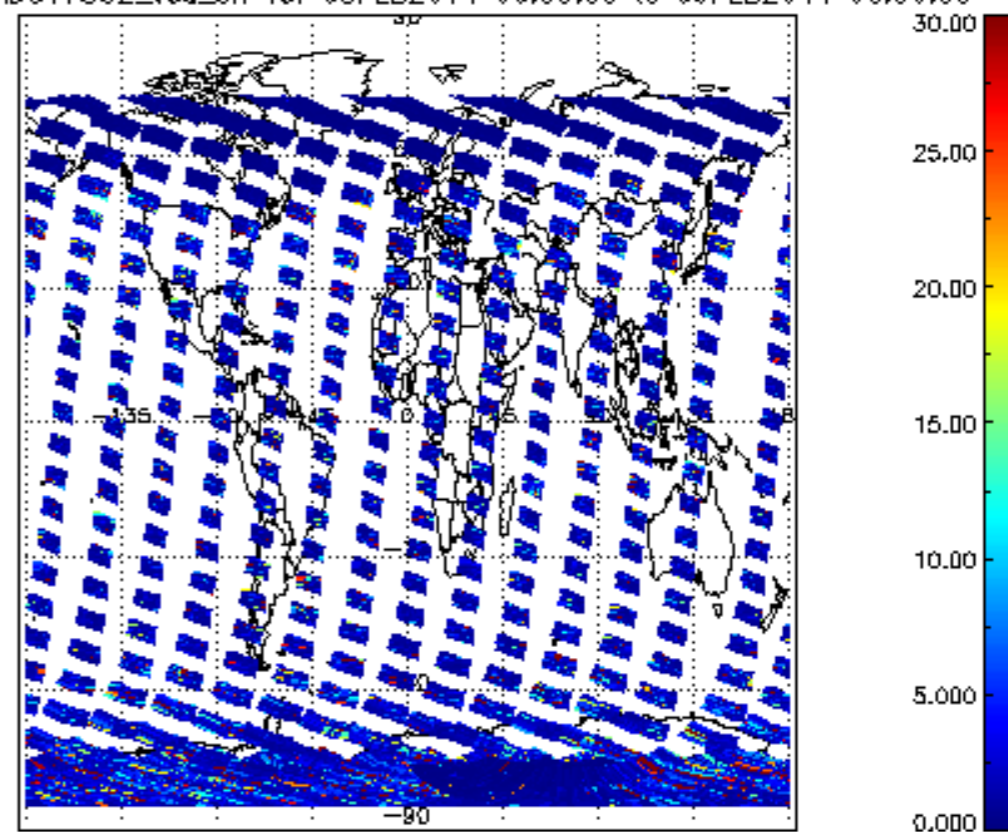
SCIOL2P_NADUV7S02_vcd_err for 08FEB2011 00:00:00 to 09FEB2011 00:00:00
