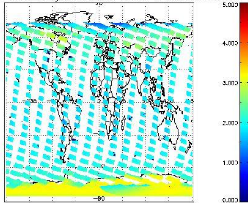
SCIOL2P_NADUV7S02_amf_gr for 08FEB2011 00:00:00 to 09FEB2011 00:00:00
