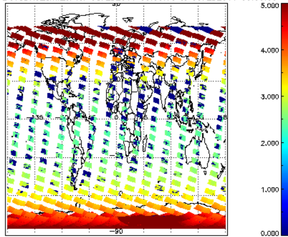
SCIOL2P_NADUV3BRO_amf_cl for 08FEB2011 00:00:00 to 09FEB2011 00:00:00
