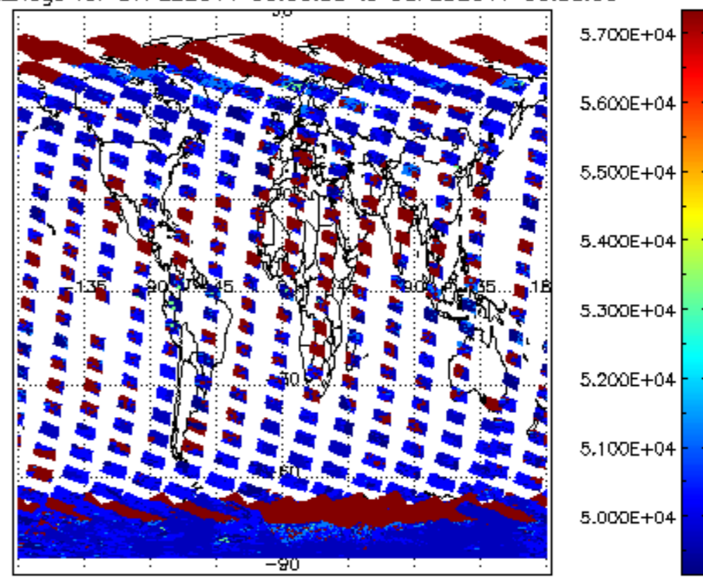
cloud_flags for 07FEB2011 00:00:00 to 08FEB2011 00:00:00
