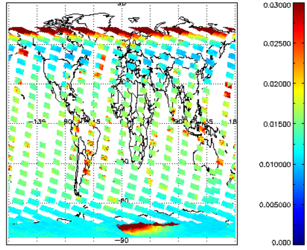
SCIOL2P_NADUV003_vcd_err for 07FEB2011 00:00:00 to 08FEB2011 00:00:00
