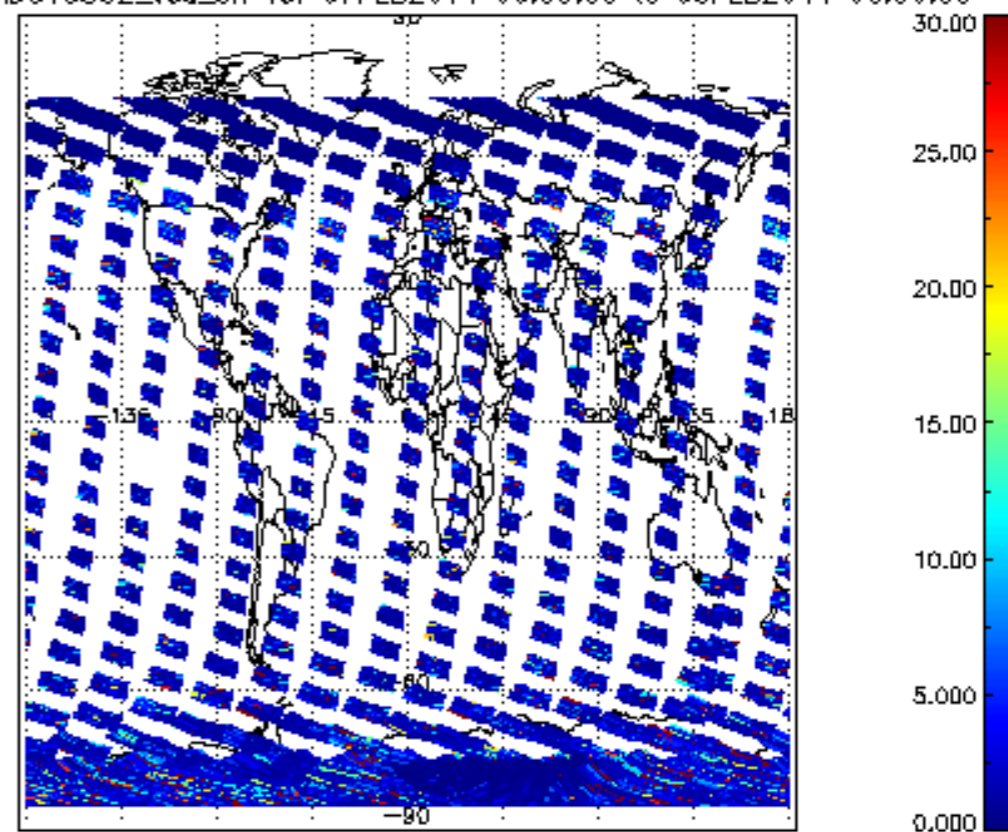
SCIOL2P_NADUV5S02_vcd_err for 07FEB2011 00:00:00 to 08FEB2011 00:00:00
