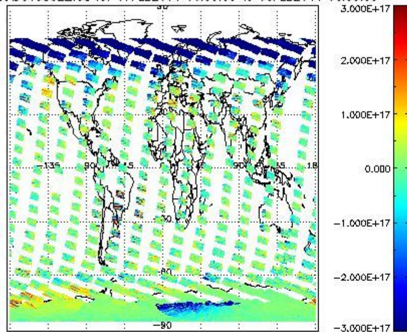
SCIOL2P_NADUV5S02_vcd for 07FEB2011 00:00:00 to 08FEB2011 00:00:00
