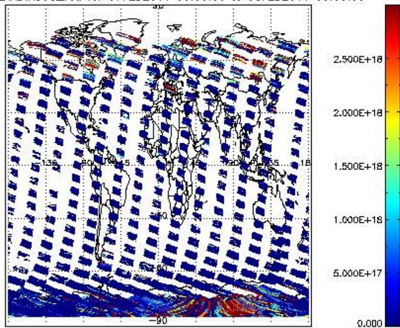
SCIDL2P_NADIR3CO_vcd for 07FEB2011 00:00:00 to 08FEB2011 00:00:00
