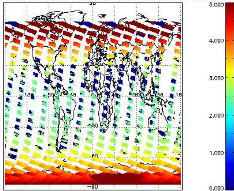
SCIOL2P_NADUV3BRO_amf_cl for 07FEB2011 00:00:00 to 08FEB2011 00:00:00
