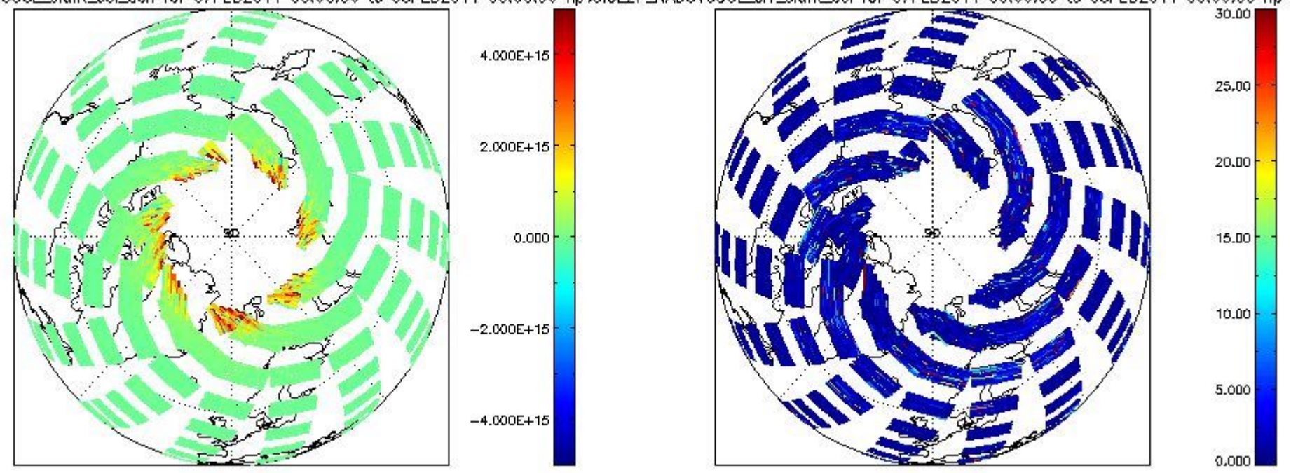
CIOL2P_NADUV6OCL_slant_col_den for 07FEB2011 00:00:00 to 08FEB2011 00:00:00 np; CIOL2P_NADUV6OCL_err_slant_col for 07FEB2011 00:00:00 to 08FEB2011 00:00:00 np
