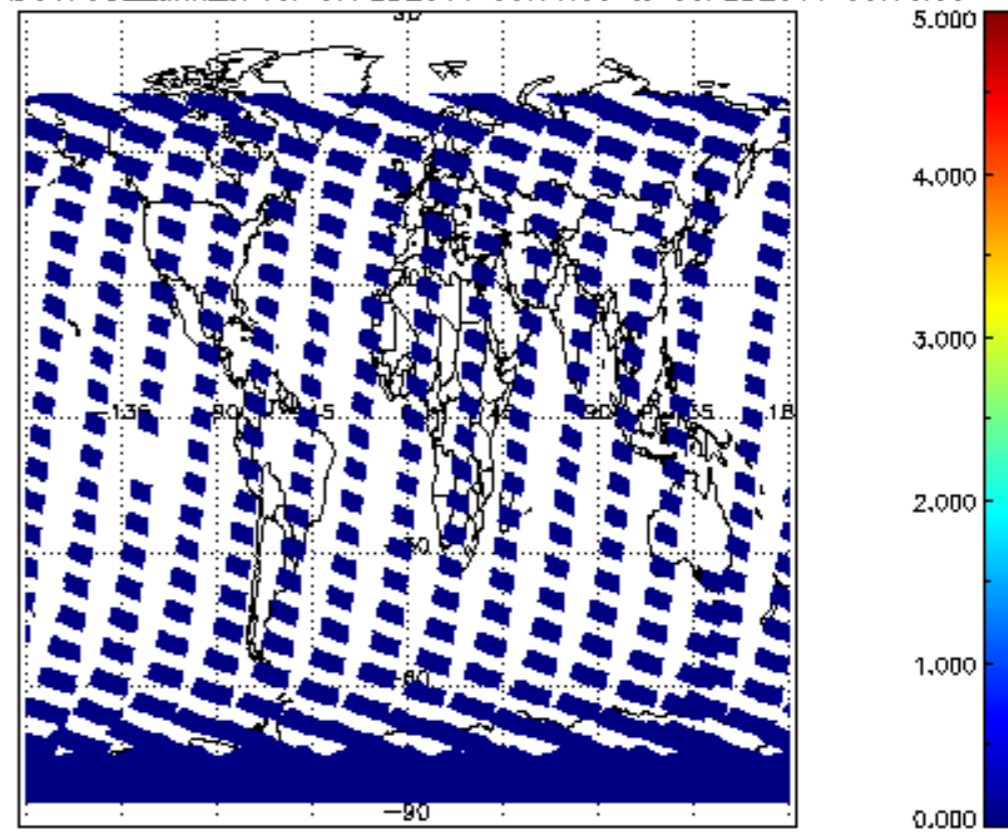
SCIOL2P_NADUV7S02_amf_cl for 07FEB2011 00:00:00 to 08FEB2011 00:00:00
