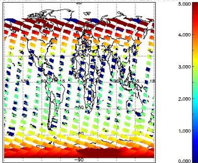
SCIOL2P_NADUV003_amf_cl for 07FEB2011 00:00:00 to 08FEB2011 00:00:00
