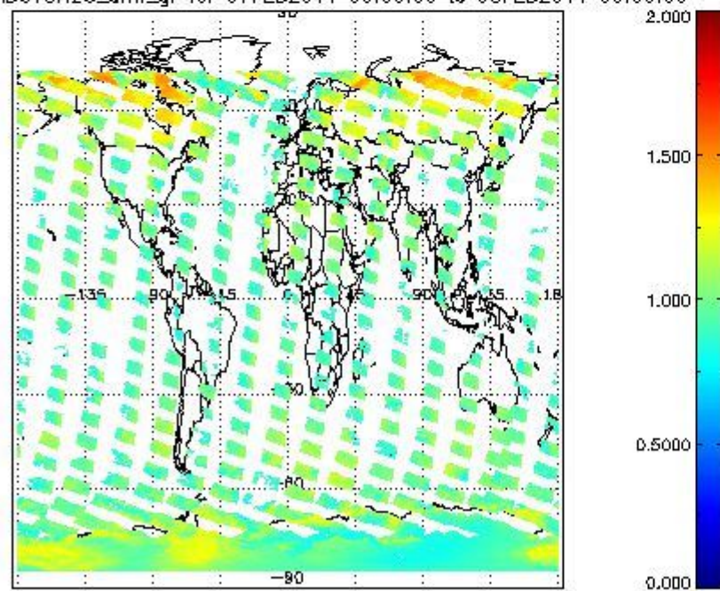
SCIOL2P_NADUV8H2O_amf_gr for 07FEB2011 00:00:00 to 08FEB2011 00:00:00
