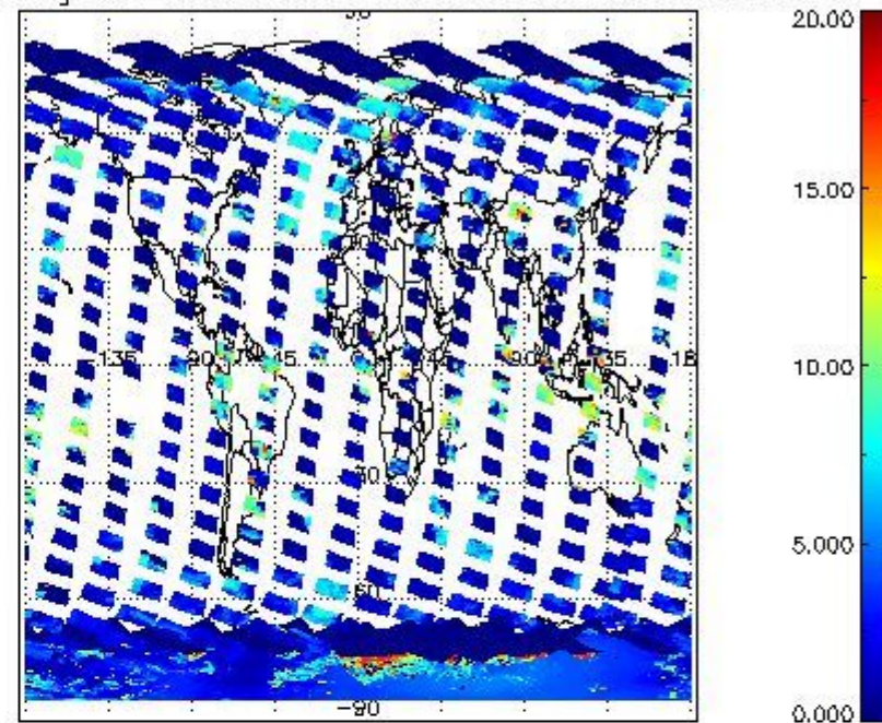
cL_top_height for 07FEB2011 00:00:00 to 08FEB2011 00:00:00
