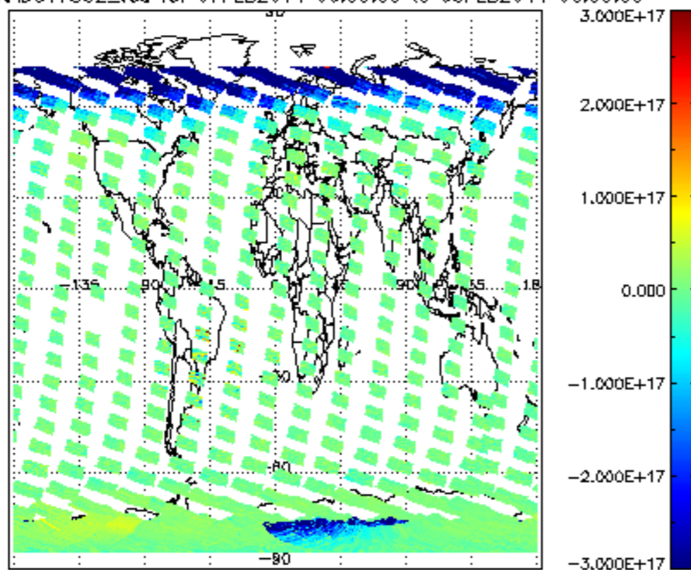
SCIOL2P_NADUV7S02_vcd for 07FEB2011 00:00:00 to 08FEB2011 00:00:00
