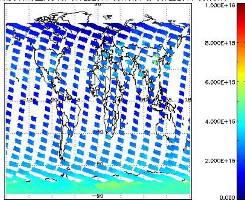
SCIOL2P_NADUV1N02_vcd for 07FEB2011 00:00:00 to 08FEB2011 00:00:00
