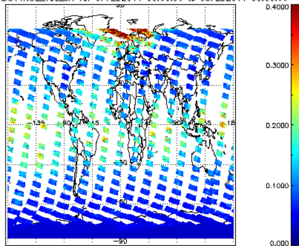
SCIOL2P_NADUV1N02_vcd_err for 07FEB2011 00:00:00 to 08FEB2011 00:00:00
