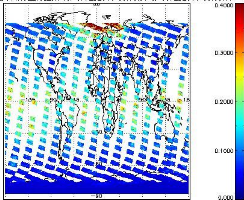
SCIOL2P_NADUV1N02_vcd_err for 07FEB2011 00:00:00 to 08FEB2011 00:00:00
