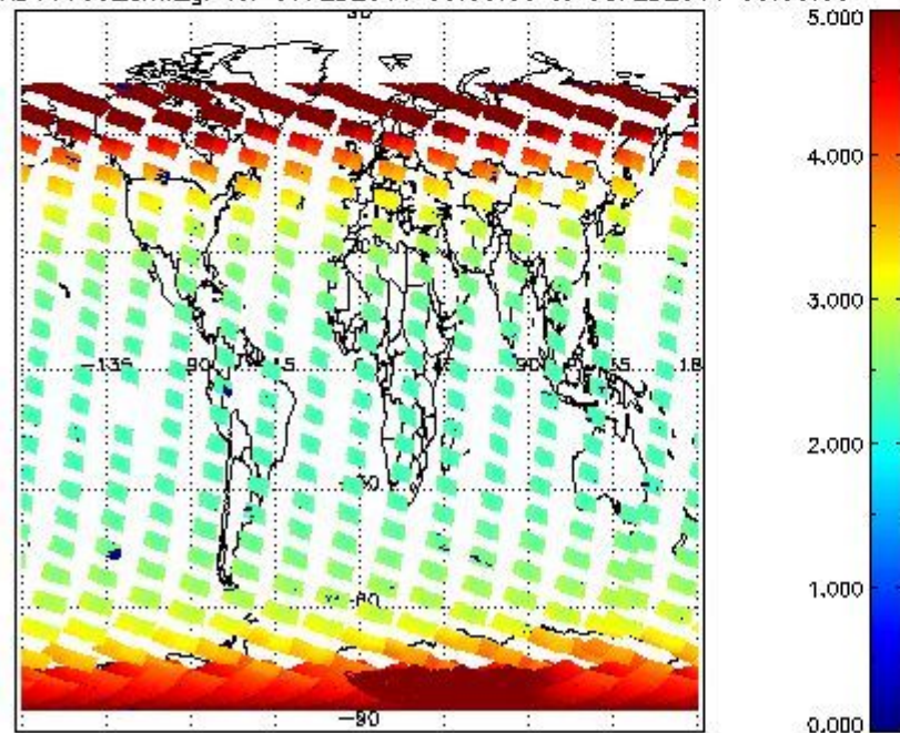
SCIOL2P_NADUV003_amf_gr for 07FEB2011 00:00:00 to 08FEB2011 00:00:00
