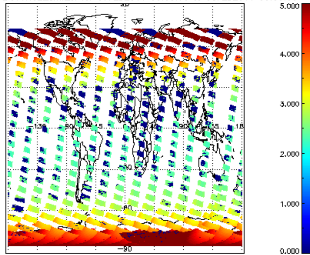
SCIOL2P_NADUV1N02_amf_cl for 07FEB2011 00:00:00 to 08FEB2011 00:00:00
