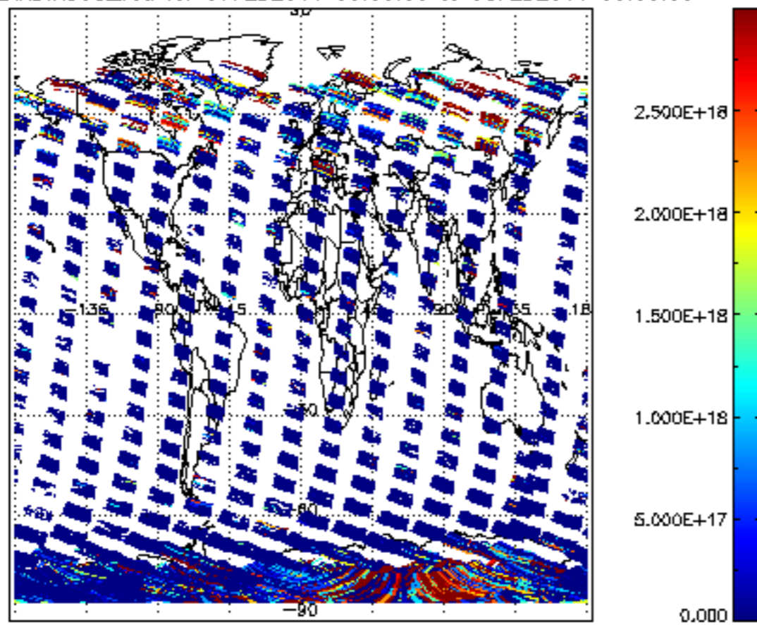
SCIOL2P_NADIR3CO_vcd for 07FEB2011 00:00:00 to 08FEB2011 00:00:00
