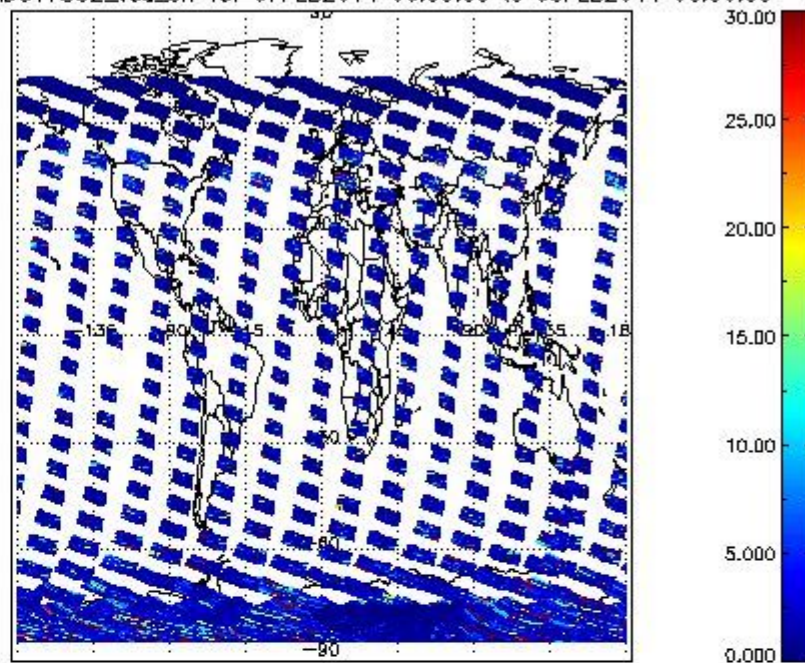
SCIOL2P_NADUV7S02_vcd_err for 07FEB2011 00:00:00 to 08FEB2011 00:00:00
