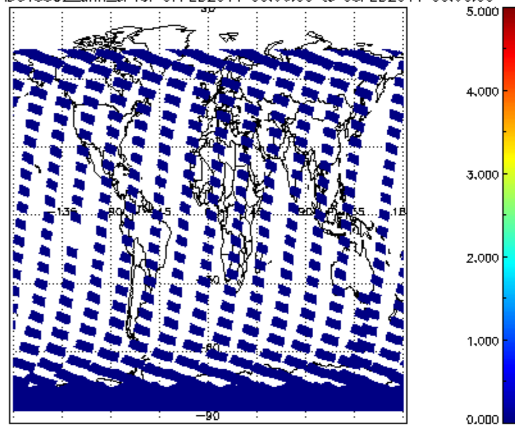
SCIOL2P_NADUV5S02_amf_cl for 07FEB2011 00:00:00 to 08FEB2011 00:00:00
