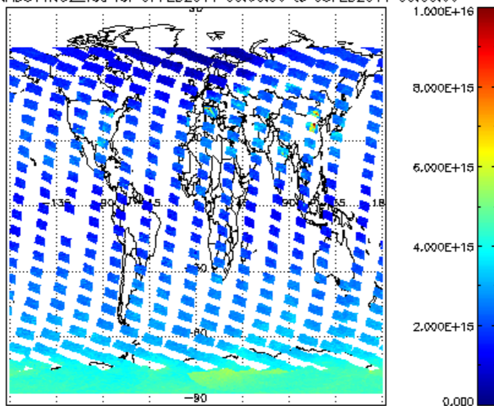
SCIOL2P_NADUV1N02_vcd for 07FEB2011 00:00:00 to 08FEB2011 00:00:00
