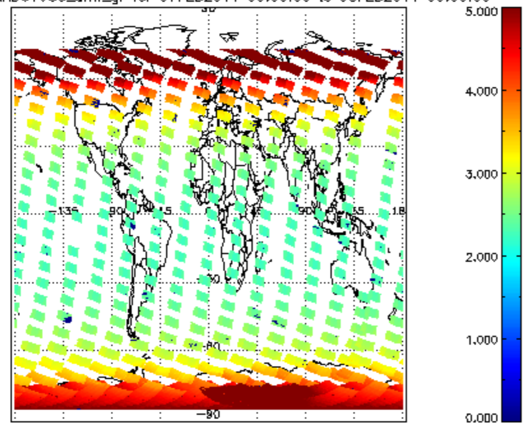
SCIOL2P_NADUV003_amf_gr for 07FEB2011 00:00:00 to 08FEB2011 00:00:00
