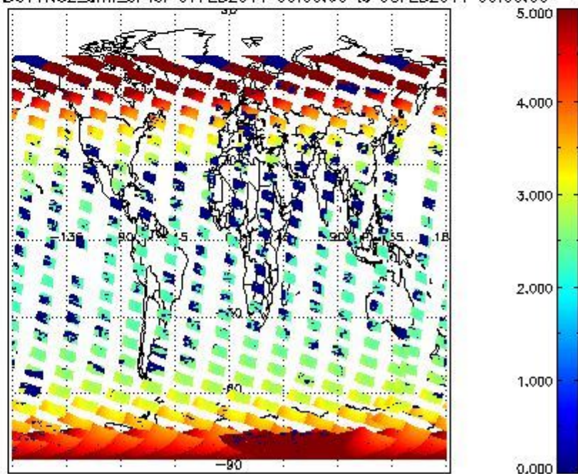
SCIOL2P_NADUV1N02_amf_cl for 07FEB2011 00:00:00 to 08FEB2011 00:00:00
