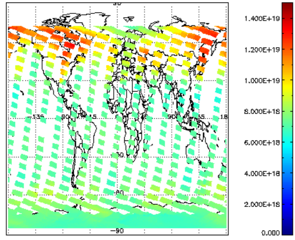
SCIOL2P_NADUV003_vcd for 07FEB2011 00:00:00 to 08FEB2011 00:00:00
