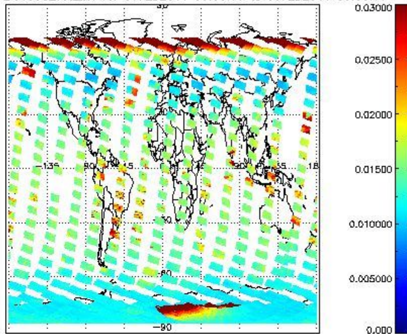
SCIOL2P_NADUV003_vcd_err for 07FEB2011 00:00:00 to 08FEB2011 00:00:00
