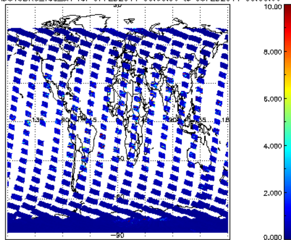
SCIOL2P_NADUV3BRO_vcd_err for 07FEB2011 00:00:00 to 08FEB2011 00:00:00
