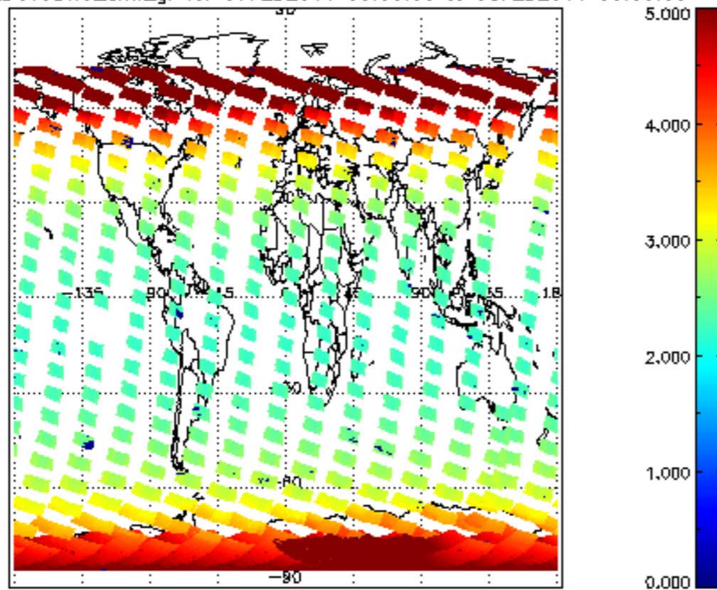
SCIOL2P_NADUV3BRO_amf_gr for 07FEB2011 00:00:00 to 08FEB2011 00:00:00
