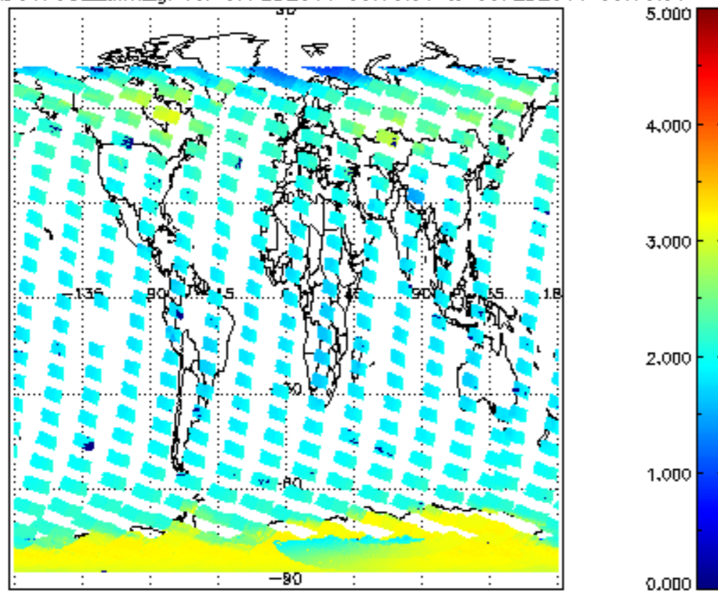
SCIOL2P_NADUV7S02_amf_gr for 07FEB2011 00:00:00 to 08FEB2011 00:00:00
