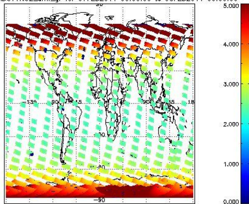
SCIOL2P_NADUV1N02_amf_gr for 07FEB2011 00:00:00 to 08FEB2011 00:00:00
