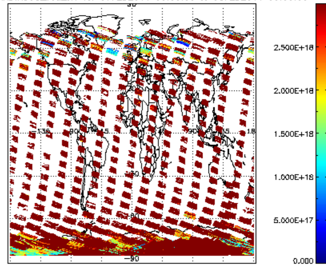
SCIOL2P_NADIR3CO_vcd_err for 07FEB2011 00:00:00 to 08FEB2011 00:00:00
