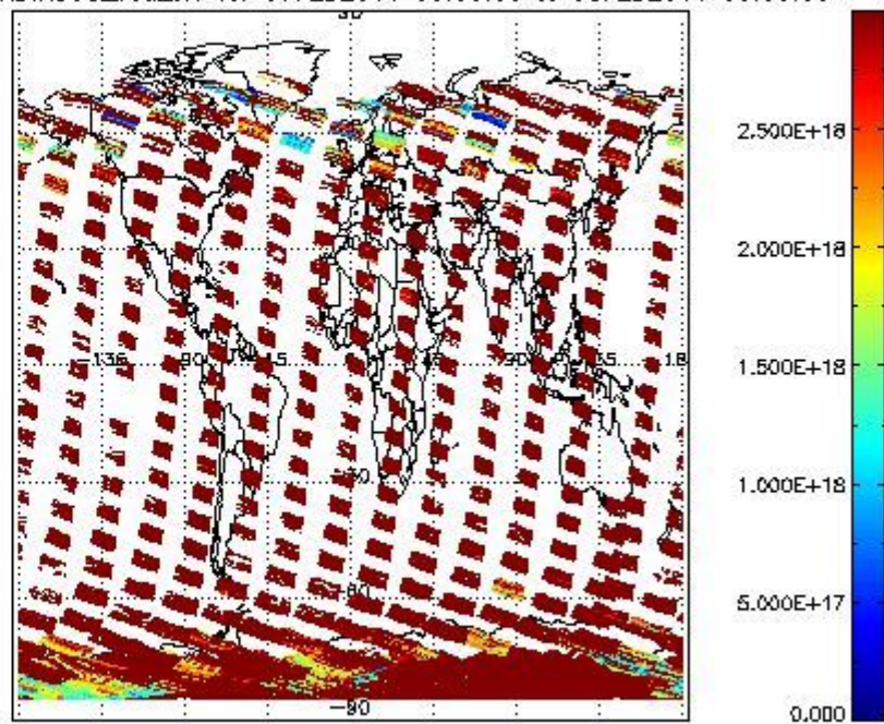
SCIDL2P_NADIR3CO_vcd_err for 07FEB2011 00:00:00 to 08FEB2011 00:00:00
