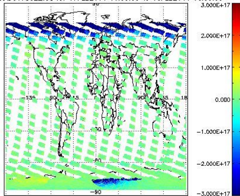
SCIOL2P_NADUV7S02_vcd for 07FEB2011 00:00:00 to 08FEB2011 00:00:00
