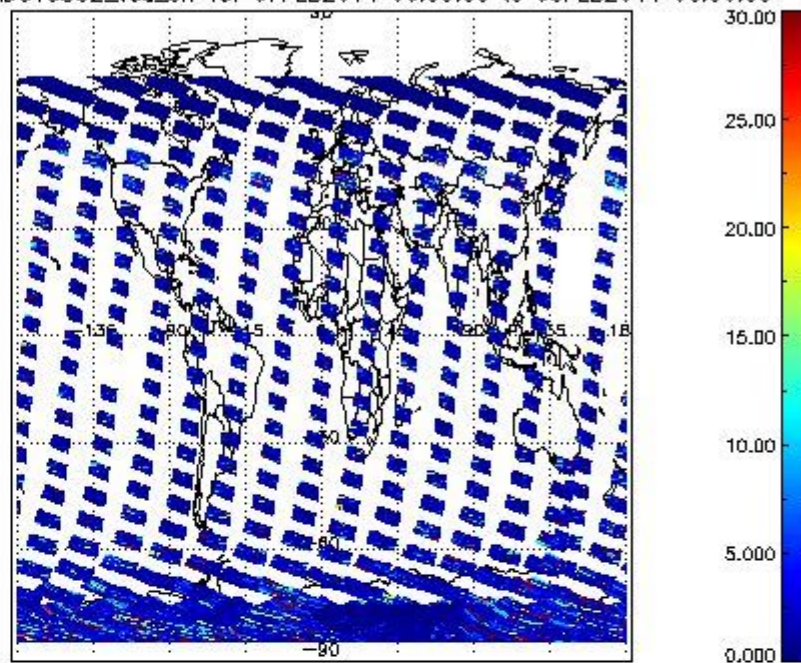
SCIOL2P_NADUV5S02_vcd_err for 07FEB2011 00:00:00 to 08FEB2011 00:00:00
