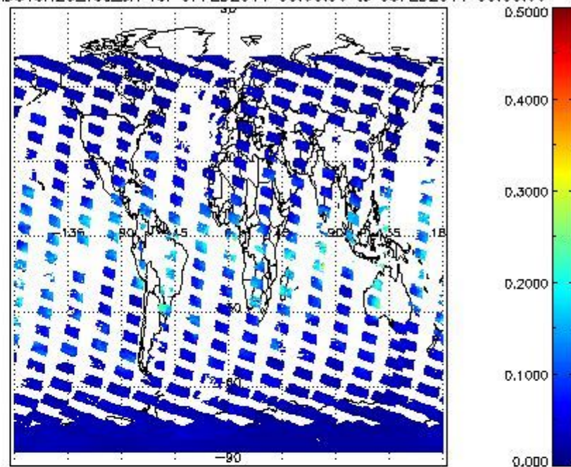
SCIOL2P_NADUV8H2O_vcd_err for 07FEB2011 00:00:00 to 08FEB2011 00:00:00
