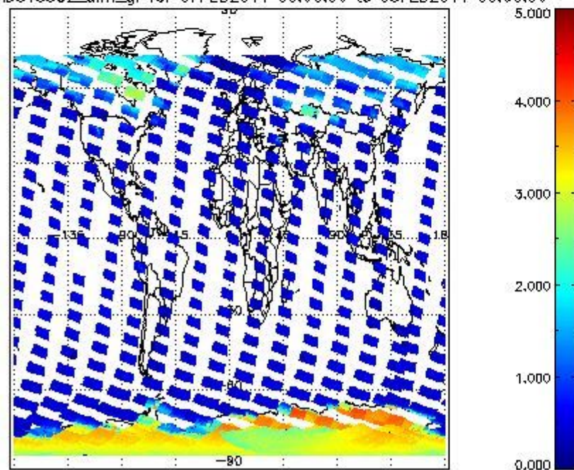
SCIOL2P_NADUV5S02_amf_gr for 07FEB2011 00:00:00 to 08FEB2011 00:00:00
