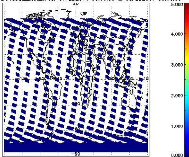
SCIOL2P_NADUV5S02_amf_cl for 07FEB2011 00:00:00 to 08FEB2011 00:00:00
