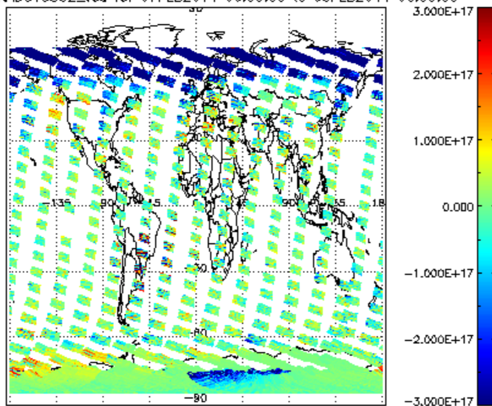
SCIOL2P_NADUV5S02_vcd for 07FEB2011 00:00:00 to 08FEB2011 00:00:00
