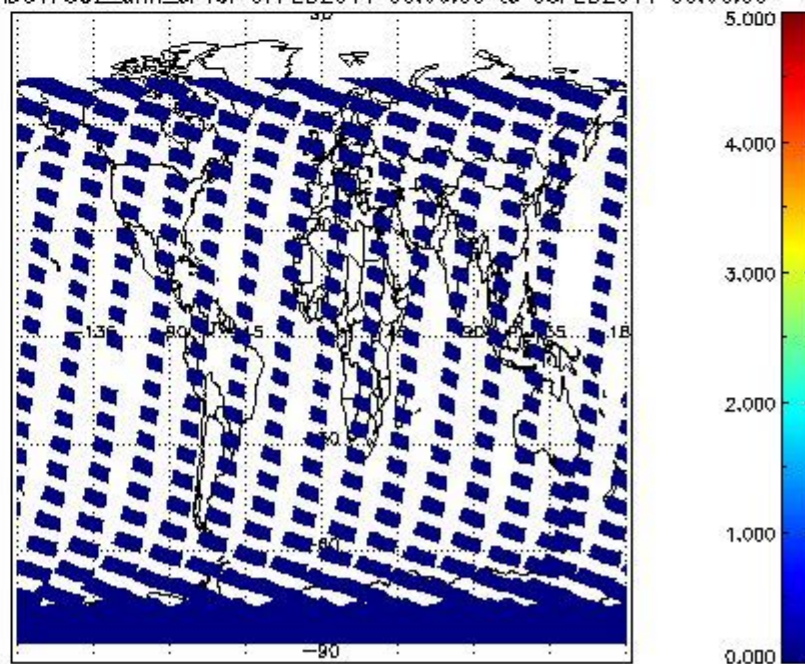
SCIOL2P_NADUV7S02_amf_cl for 07FEB2011 00:00:00 to 08FEB2011 00:00:00
