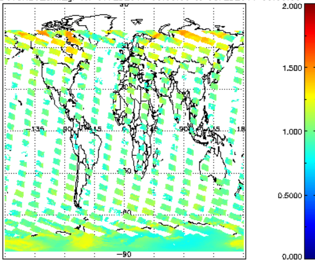
SCIOL2P_NADUV8H20_amf_gr for 07FEB2011 00:00:00 to 08FEB2011 00:00:00
