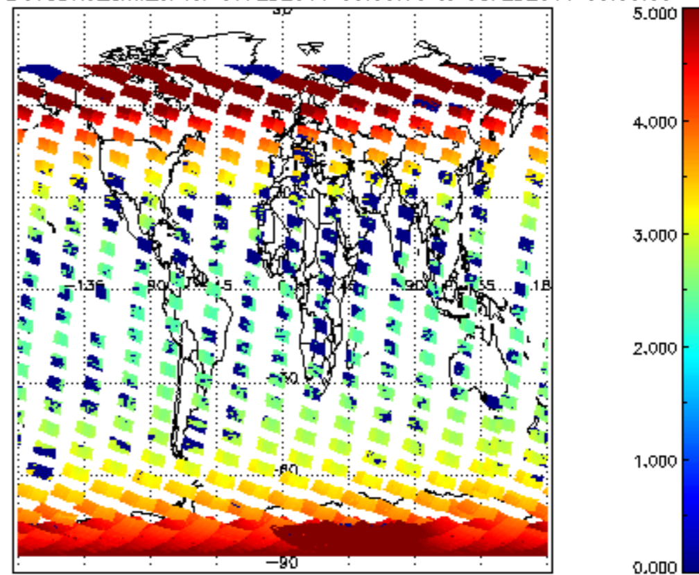
SCIOL2P_NADUV3BRO_amf_cl for 07FEB2011 00:00:00 to 08FEB2011 00:00:00
