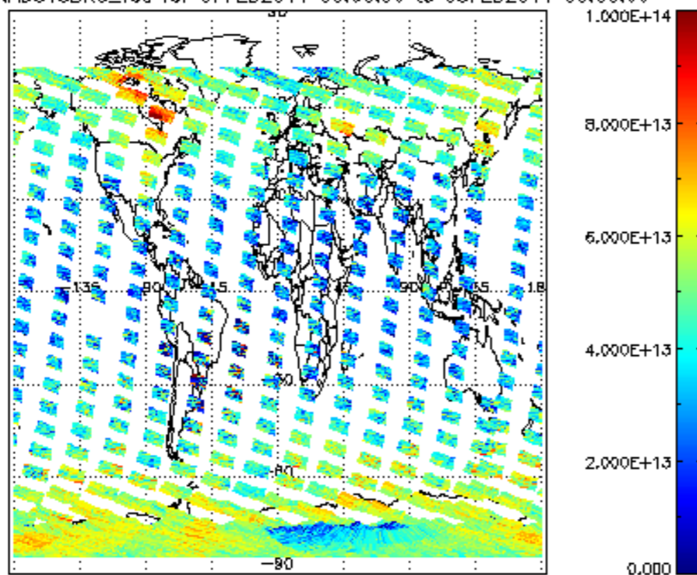
SCIOL2P_NADUV3BRO_vcd for 07FEB2011 00:00:00 to 08FEB2011 00:00:00
