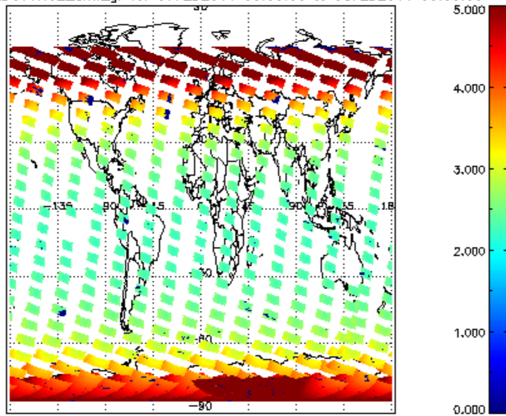
SCIOL2P_NADUV1N02_amf_gr for 07FEB2011 00:00:00 to 08FEB2011 00:00:00
