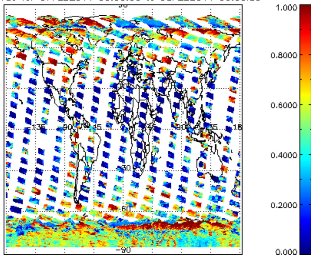
cI_frac for 07FEB2011 00:00:00 to 08FEB2011 00:00:00
