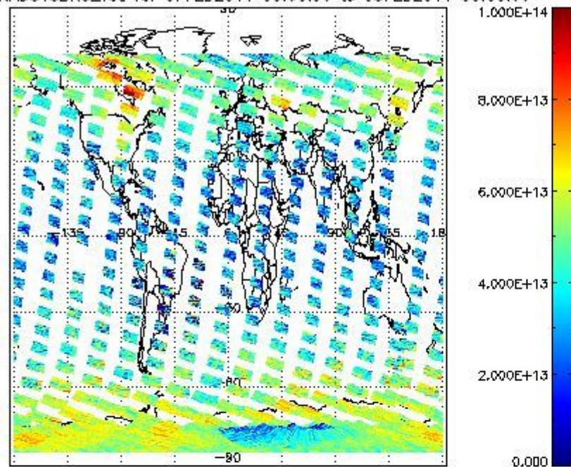
SCIOL2P_NADUV3BRO_vcd for 07FEB2011 00:00:00 to 08FEB2011 00:00:00
