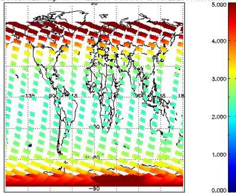
SCIOL2P_NADUV3BRO_amf_gr for 07FEB2011 00:00:00 to 08FEB2011 00:00:00
