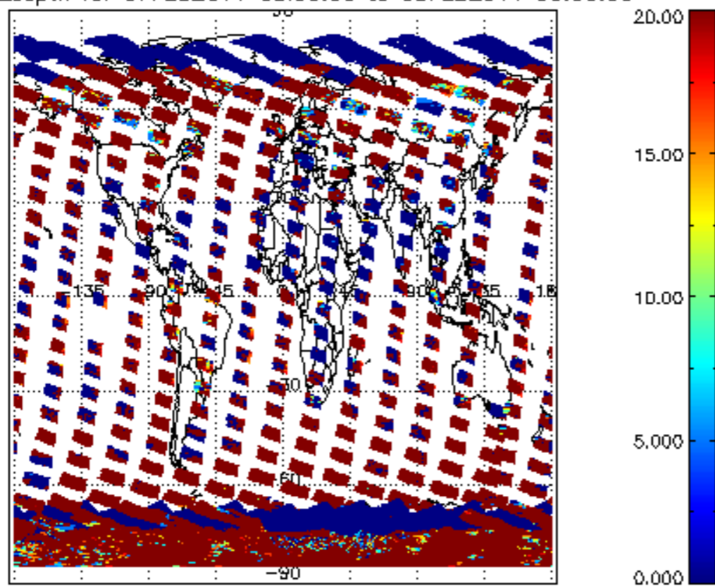
cI_opt_depth for 07FEB2011 00:00:00 to 08FEB2011 00:00:00
