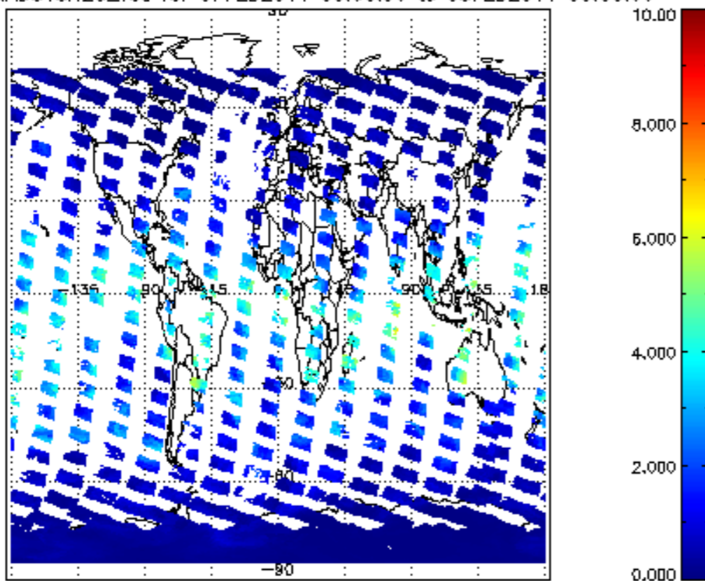
SCIOL2P_NADUV8H20_vcd for 07FEB2011 00:00:00 to 08FEB2011 00:00:00
