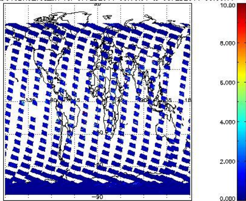
SCIOL2P_NADUV3BRO_vcd_err for 07FEB2011 00:00:00 to 08FEB2011 00:00:00
