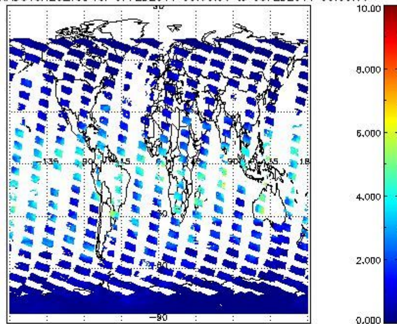
SCIOL2P_NADUV8H2O_vcd for 07FEB2011 00:00:00 to 08FEB2011 00:00:00
