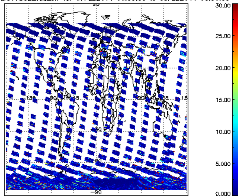
SCIOL2P_NADUV7S02_vcd_err for 07FEB2011 00:00:00 to 08FEB2011 00:00:00
