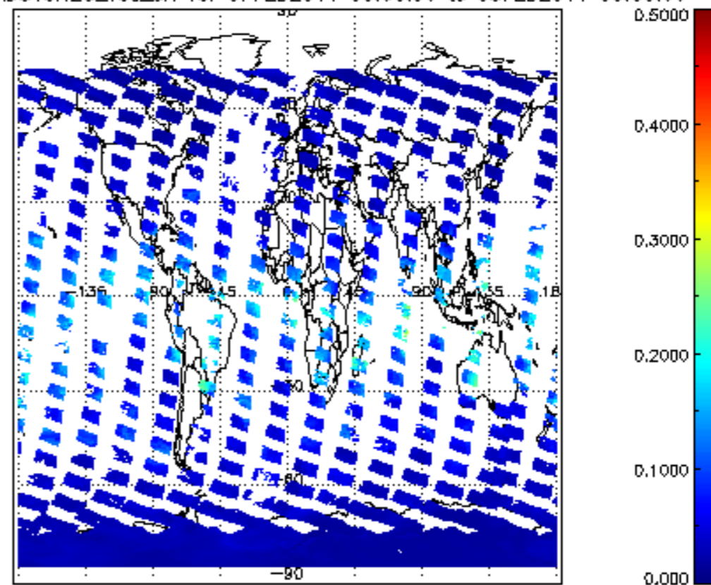
SCIOL2P_NADUV8H20_vcd_err for 07FEB2011 00:00:00 to 08FEB2011 00:00:00
