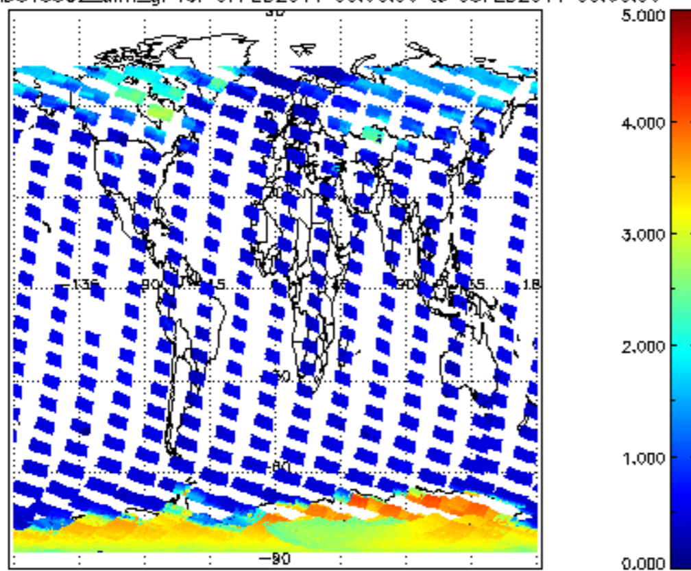
SCIOL2P_NADUV5S02_amf_gr for 07FEB2011 00:00:00 to 08FEB2011 00:00:00
