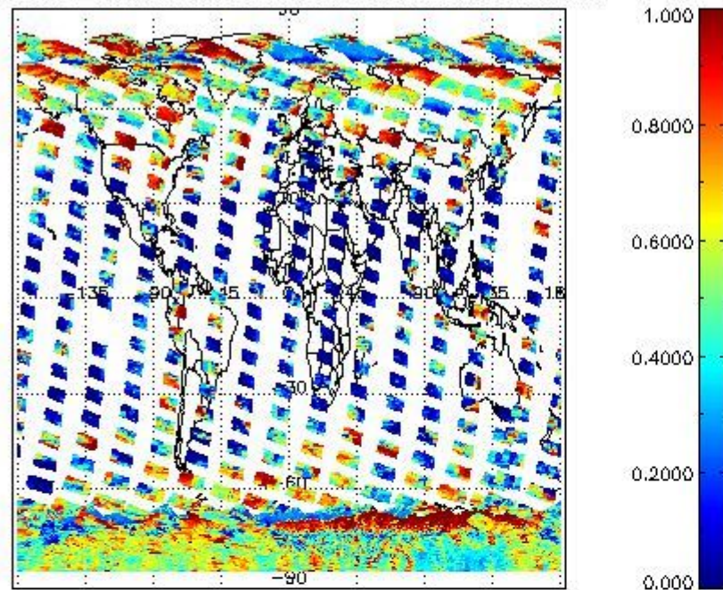
cL_frac for 07FEB2011 00:00:00 to 08FEB2011 00:00:00
