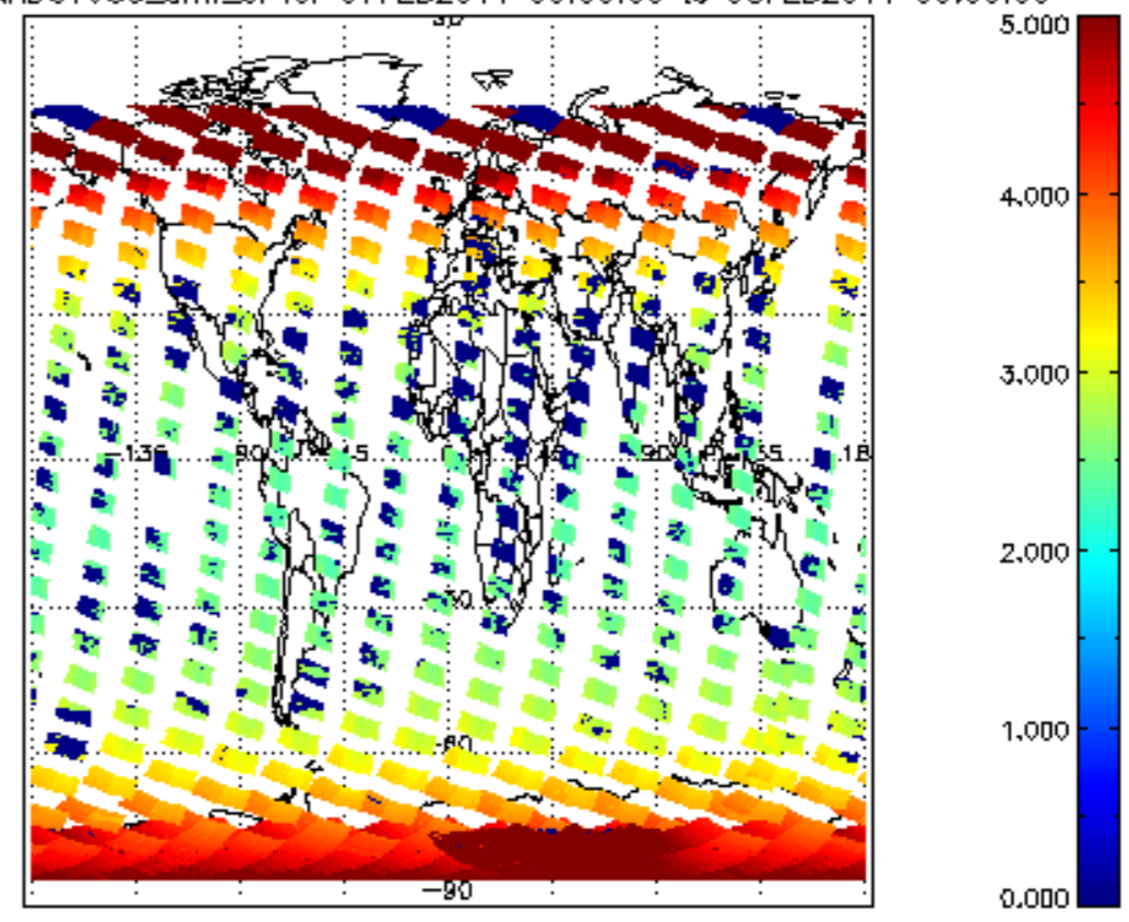
SCIOL2P_NADUV003_amf_cl for 07FEB2011 00:00:00 to 08FEB2011 00:00:00
