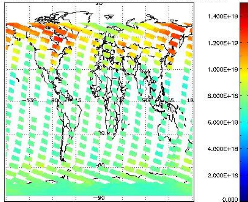
SCIOL2P_NADUV003_vcd for 07FEB2011 00:00:00 to 08FEB2011 00:00:00
