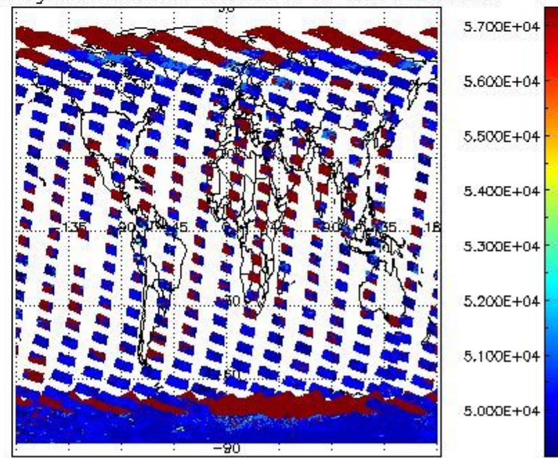
cloud_flags for 07FEB2011 00:00:00 to 08FEB2011 00:00:00
