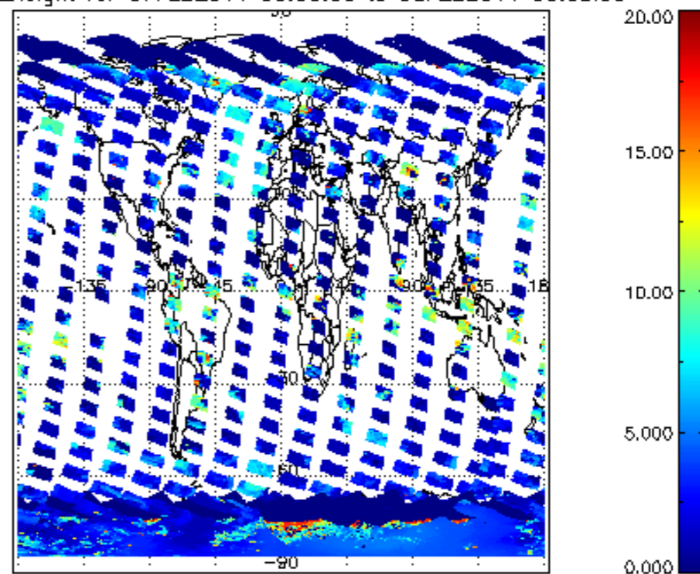
cI_top_height for 07FEB2011 00:00:00 to 08FEB2011 00:00:00
