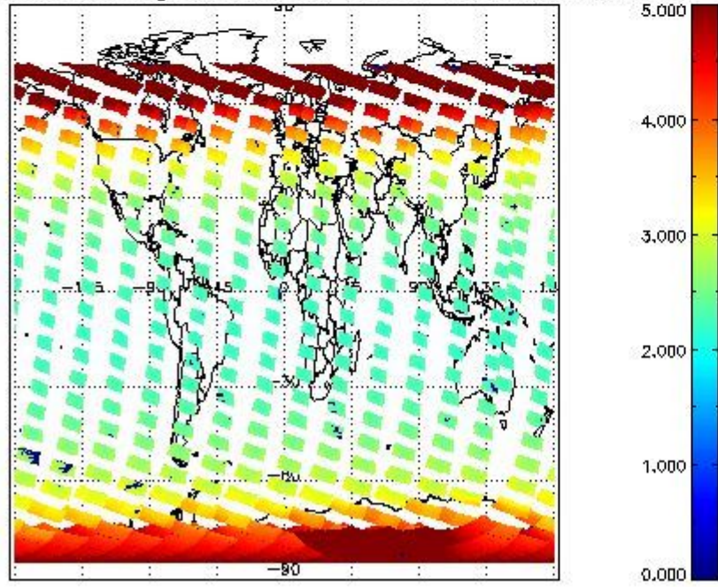
SCIOL2P_NADUV3BRO_amf_gr for 06FEB2011 00:00:00 to 07FEB2011 00:00:00
