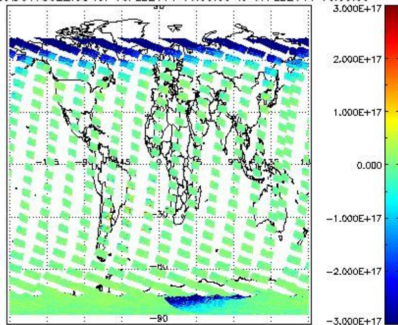
SCIOL2P_NADUV7S02_vcd for 06FEB2011 00:00:00 to 07FEB2011 00:00:00
