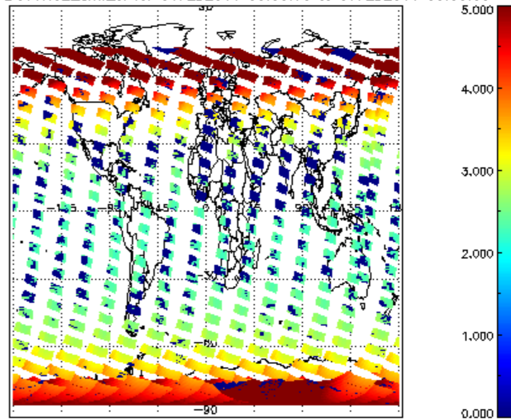
SCIOL2P_NADUV1N02_amf_cl for 06FEB2011 00:00:00 to 07FEB2011 00:00:00
