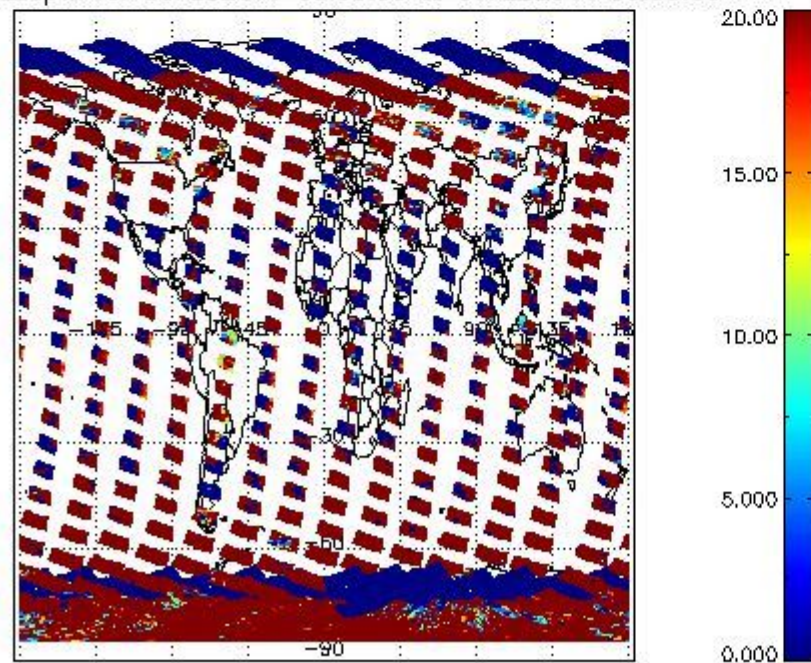
cL_opt_depth for 06FEB2011 00:00:00 to 07FEB2011 00:00:00
