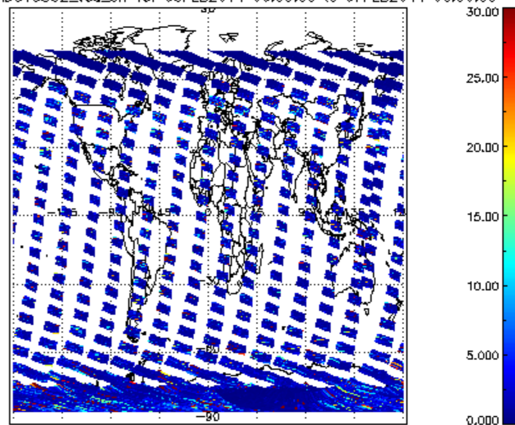
SCIOL2P_NADUV5S02_vcd_err for 06FEB2011 00:00:00 to 07FEB2011 00:00:00
