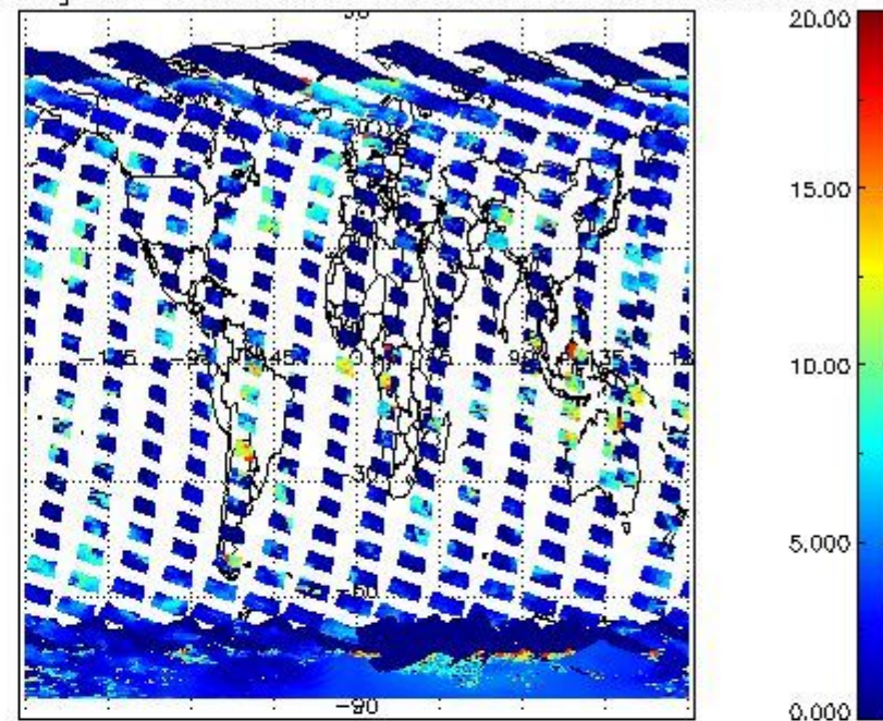
cL_top_height for 06FEB2011 00:00:00 to 07FEB2011 00:00:00
