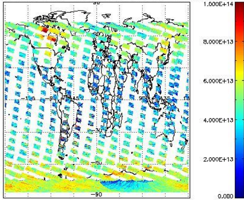
SCIOL2P_NADUV3BRO_vcd for 06FEB2011 00:00:00 to 07FEB2011 00:00:00
