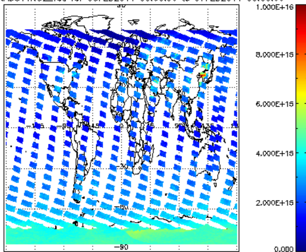
SCIOL2P_NADUV1N02_vcd for 06FEB2011 00:00:00 to 07FEB2011 00:00:00
