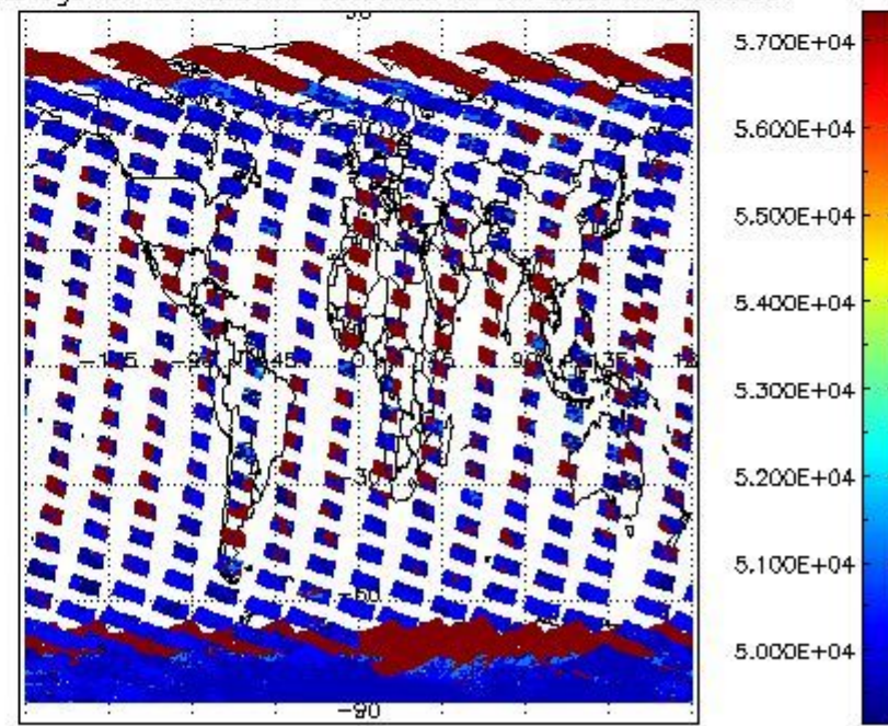
cloud_flags for 06FEB2011 00:00:00 to 07FEB2011 00:00:00
