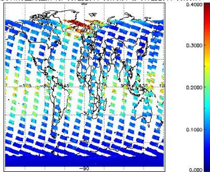
SCIOL2P_NADUV1N02_vcd_err for 06FEB2011 00:00:00 to 07FEB2011 00:00:00
