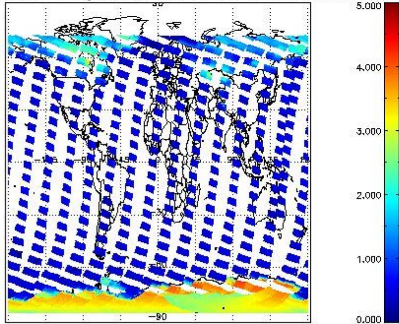
SCIOL2P_NADUV5S02_amf_gr for 06FEB2011 00:00:00 to 07FEB2011 00:00:00
