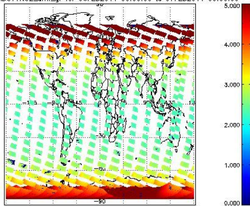
SCIOL2P_NADUV1N02_amf_gr for 06FEB2011 00:00:00 to 07FEB2011 00:00:00
