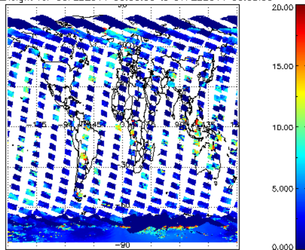
cl_top_height for 06FEB2011 00:00:00 to 07FEB2011 00:00:00
