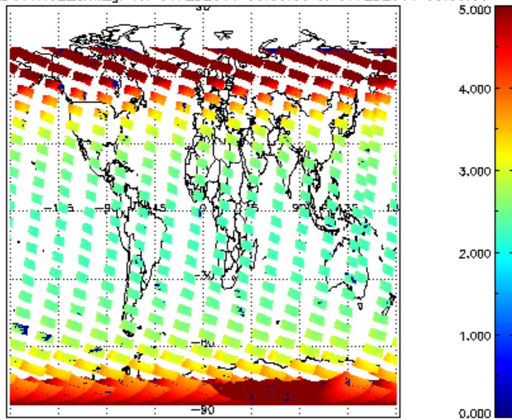
SCIOL2P_NADUV1N02_amf_gr for 06FEB2011 00:00:00 to 07FEB2011 00:00:00
