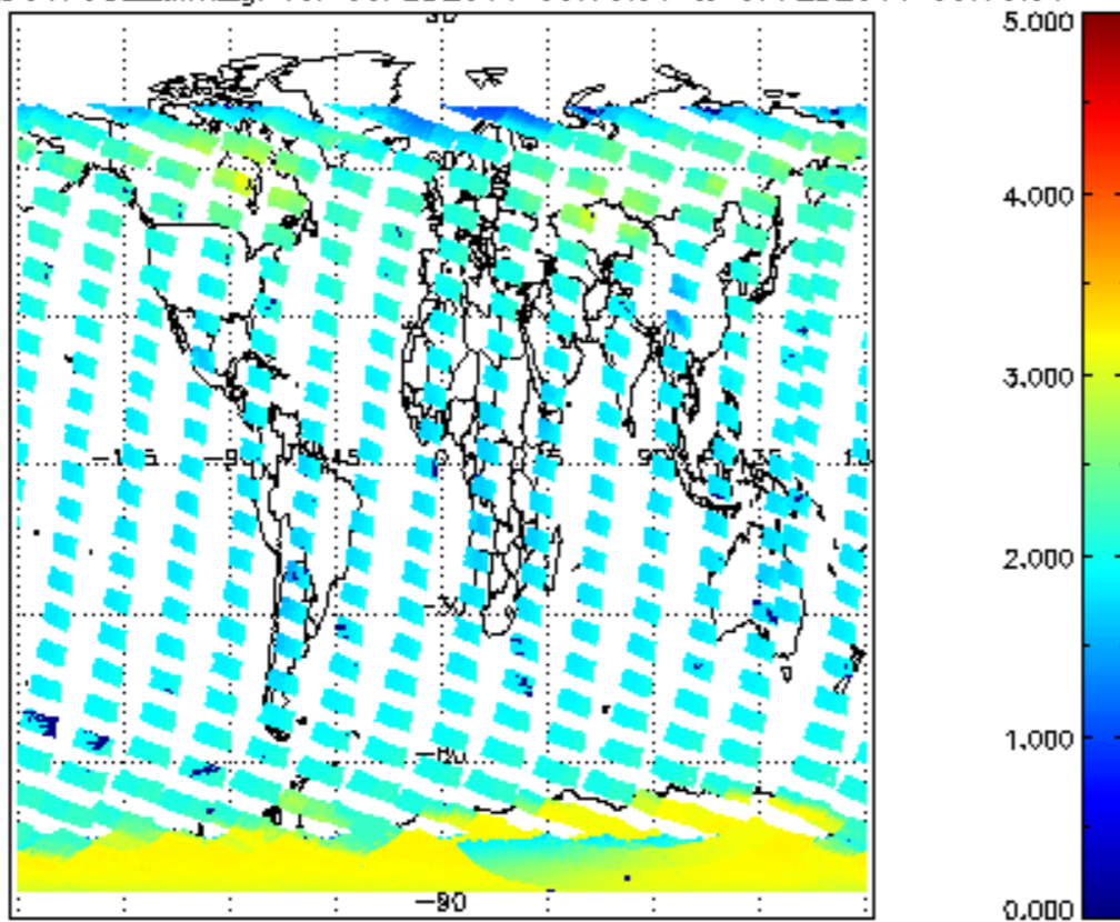
SCIOL2P_NADUV7S02_amf_gr for 06FEB2011 00:00:00 to 07FEB2011 00:00:00
