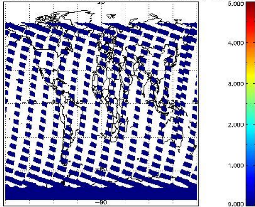
SCIOL2P_NADUV5S02_amf_cl for 06FEB2011 00:00:00 to 07FEB2011 00:00:00
