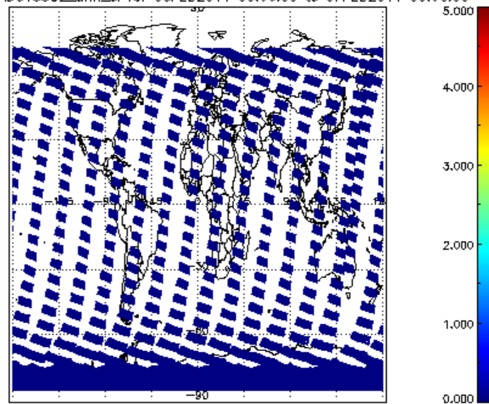
SCIOL2P_NADUV5S02_amf_cl for 06FEB2011 00:00:00 to 07FEB2011 00:00:00
