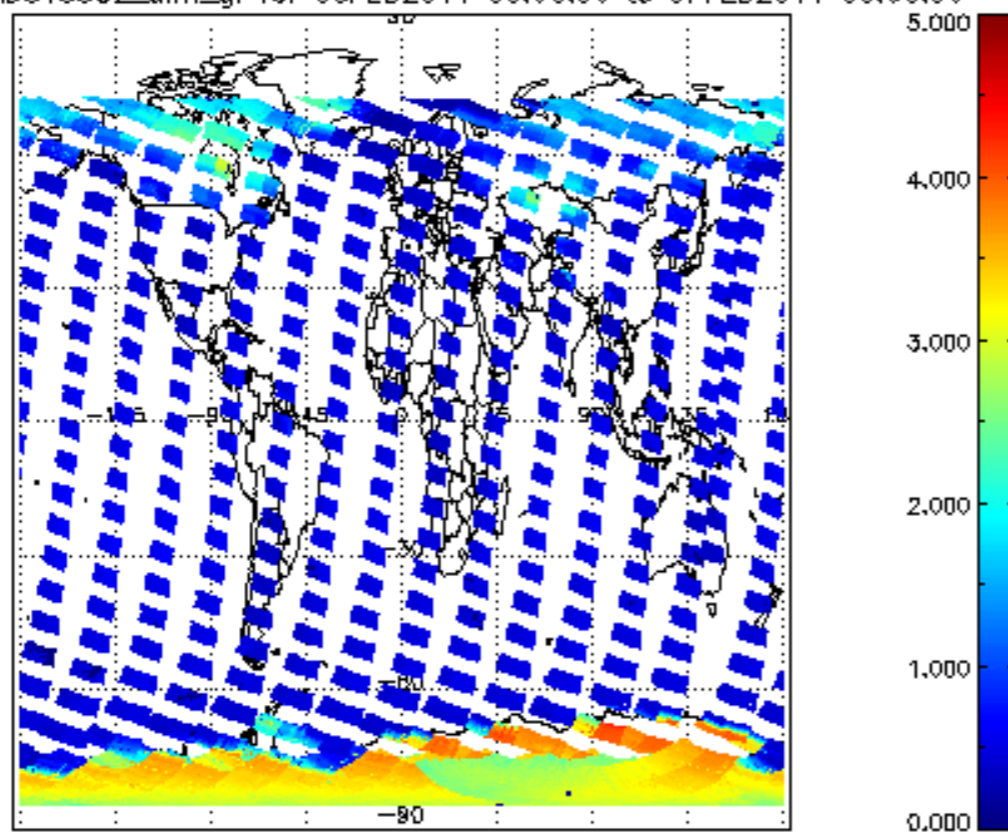
SCIOL2P_NADUV5S02_amf_gr for 06FEB2011 00:00:00 to 07FEB2011 00:00:00
