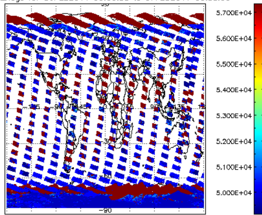
cloud_flags for 06FEB2011 00:00:00 to 07FEB2011 00:00:00
