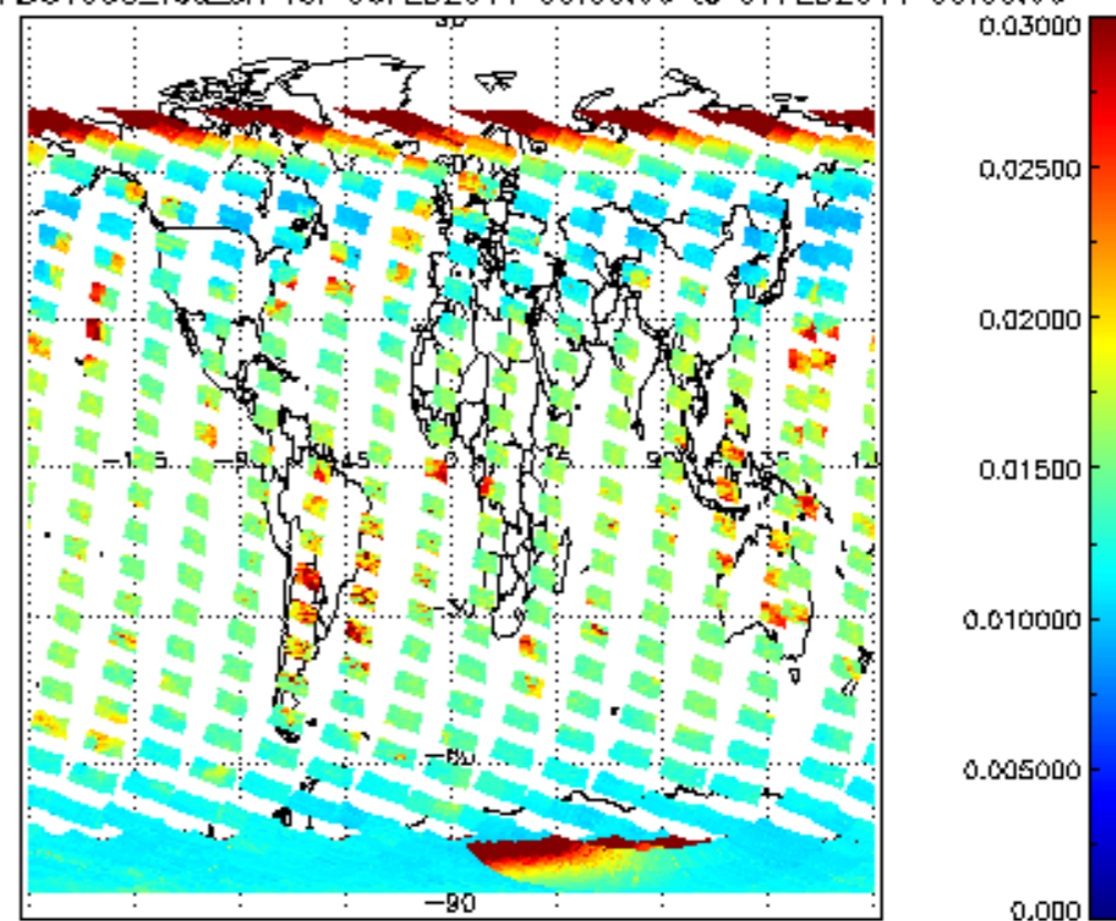
SCIOL2P_NADUV003_vcd_err for 06FEB2011 00:00:00 to 07FEB2011 00:00:00
