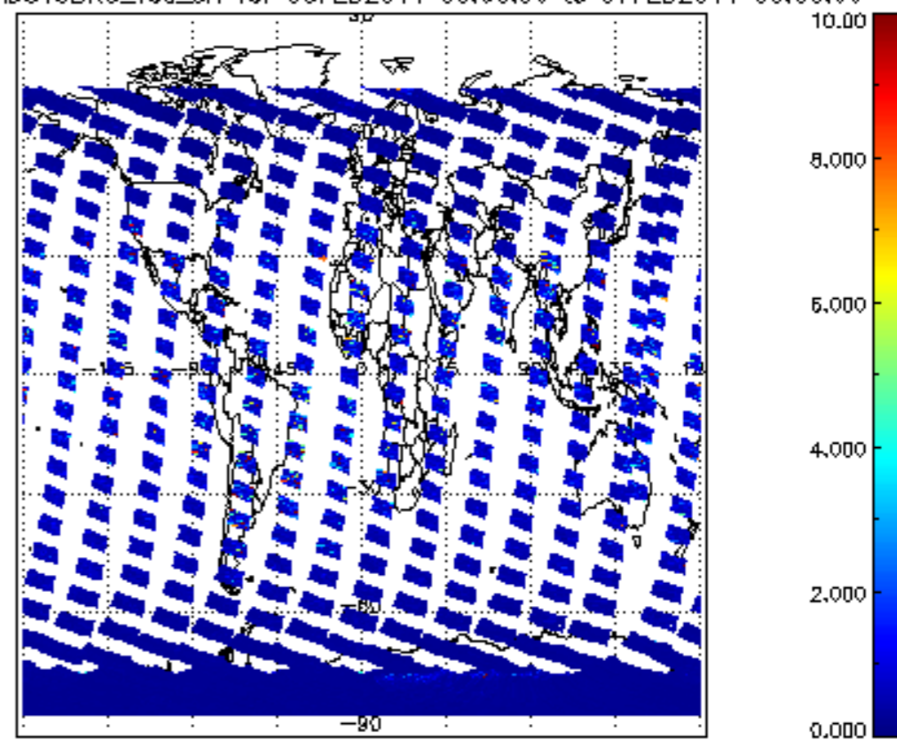
SCIOL2P_NADUV3BRO_vcd_err for 06FEB2011 00:00:00 to 07FEB2011 00:00:00
