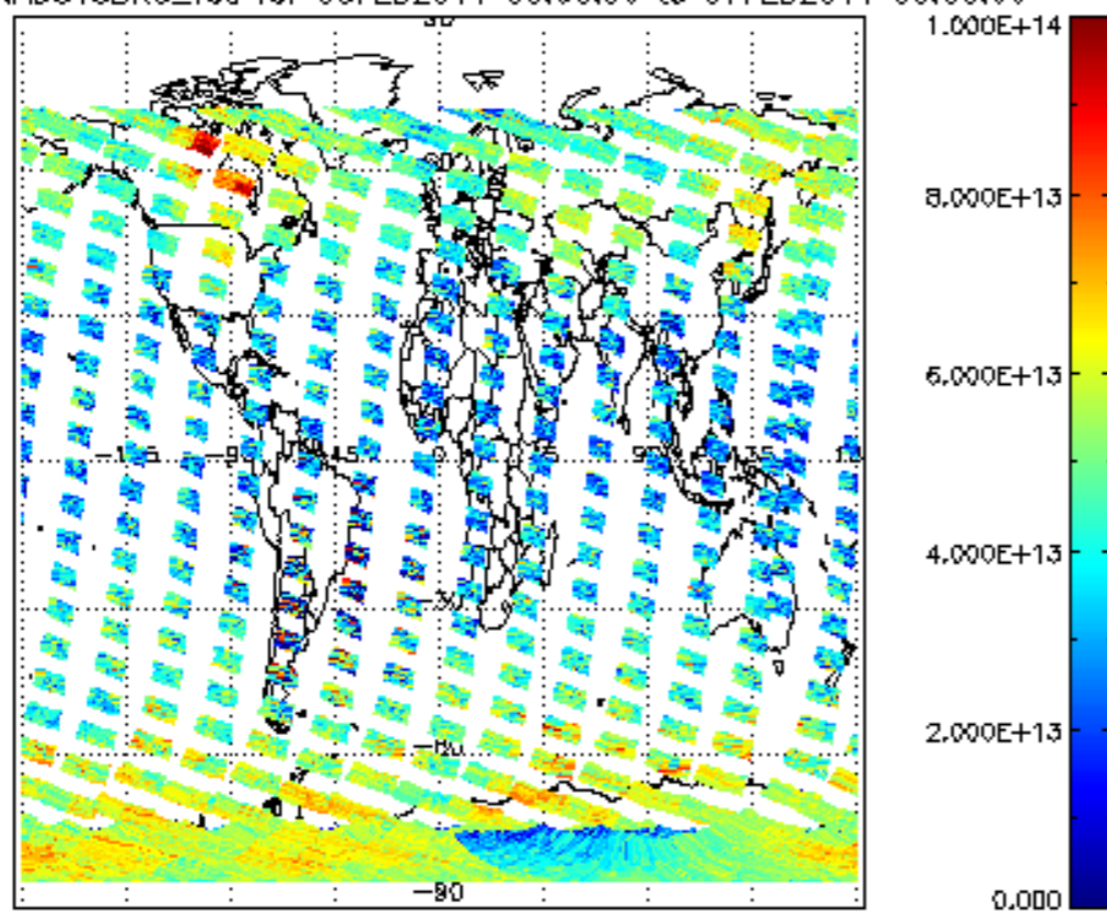
SCIOL2P_NADUV3BRO_vcd for 06FEB2011 00:00:00 to 07FEB2011 00:00:00
