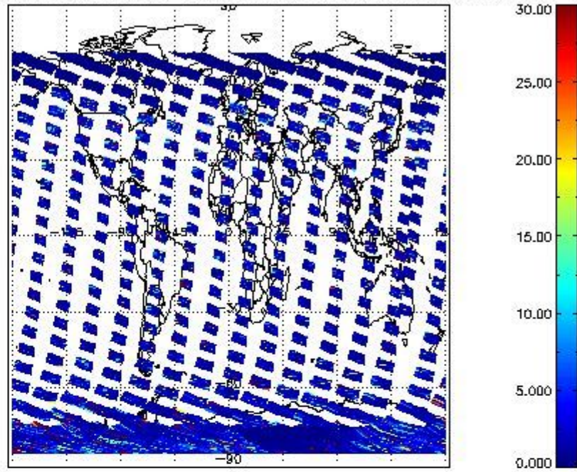
SCIOL2P_NADUV5S02_vcd_err for 06FEB2011 00:00:00 to 07FEB2011 00:00:00
