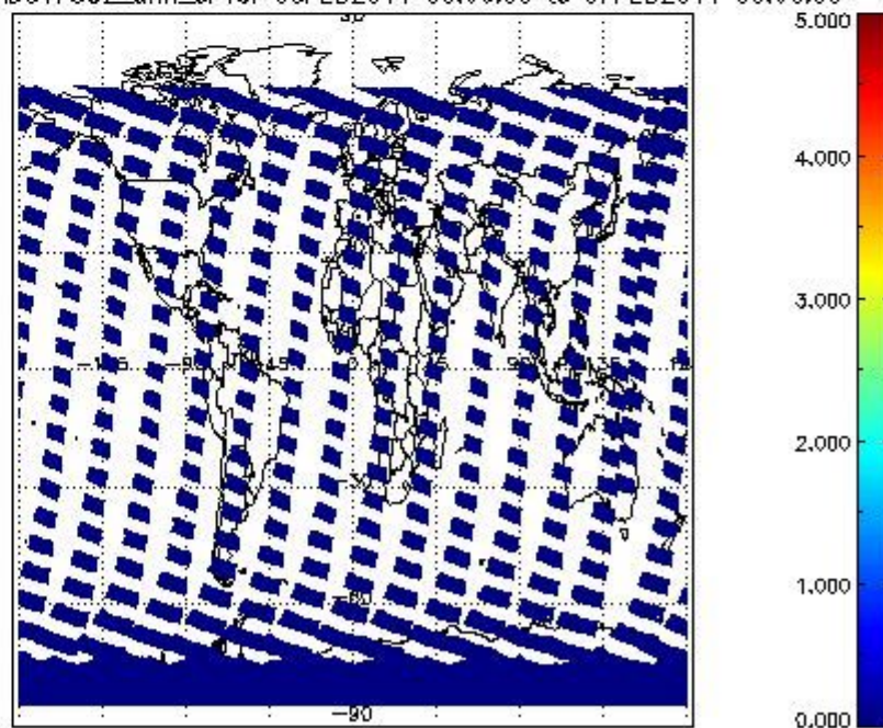
SCIOL2P_NADUV7S02_amf_cl for 06FEB2011 00:00:00 to 07FEB2011 00:00:00
