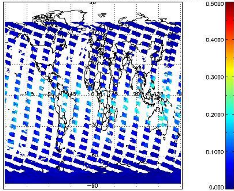
SCIOL2P_NADUV8H2O_vcd_err for 06FEB2011 00:00:00 to 07FEB2011 00:00:00
