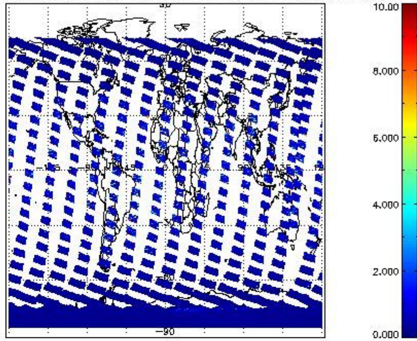
SCIOL2P_NADUV3BRO_vcd_err for 06FEB2011 00:00:00 to 07FEB2011 00:00:00
