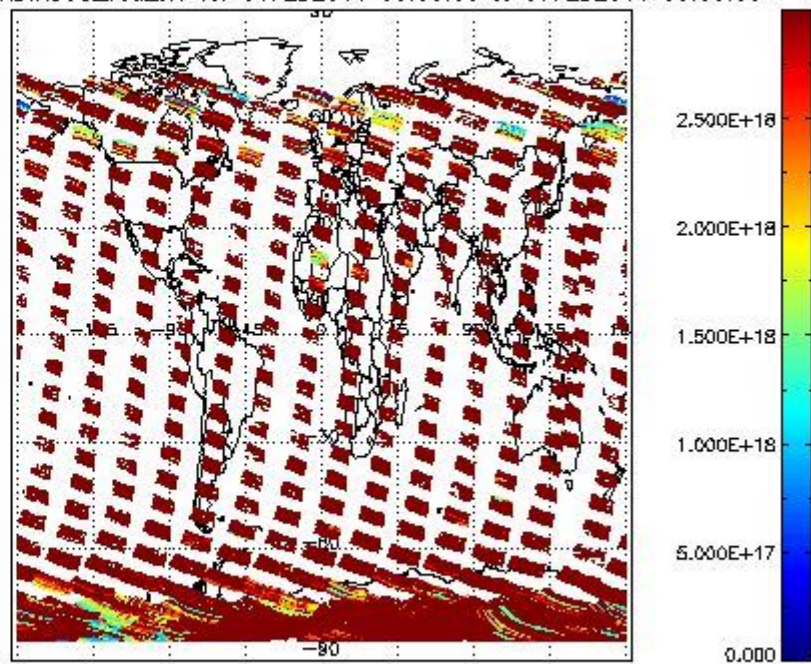
SCIDL2P_NADIR3CO_vcd_err for 06FEB2011 00:00:00 to 07FEB2011 00:00:00
