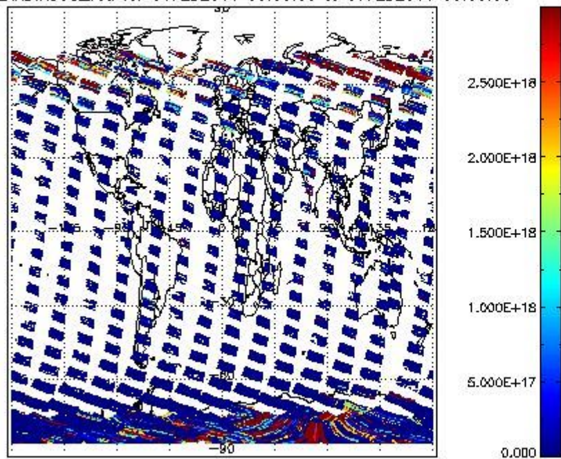
SCIDL2P_NADIR3CO_vcd for 06FEB2011 00:00:00 to 07FEB2011 00:00:00
