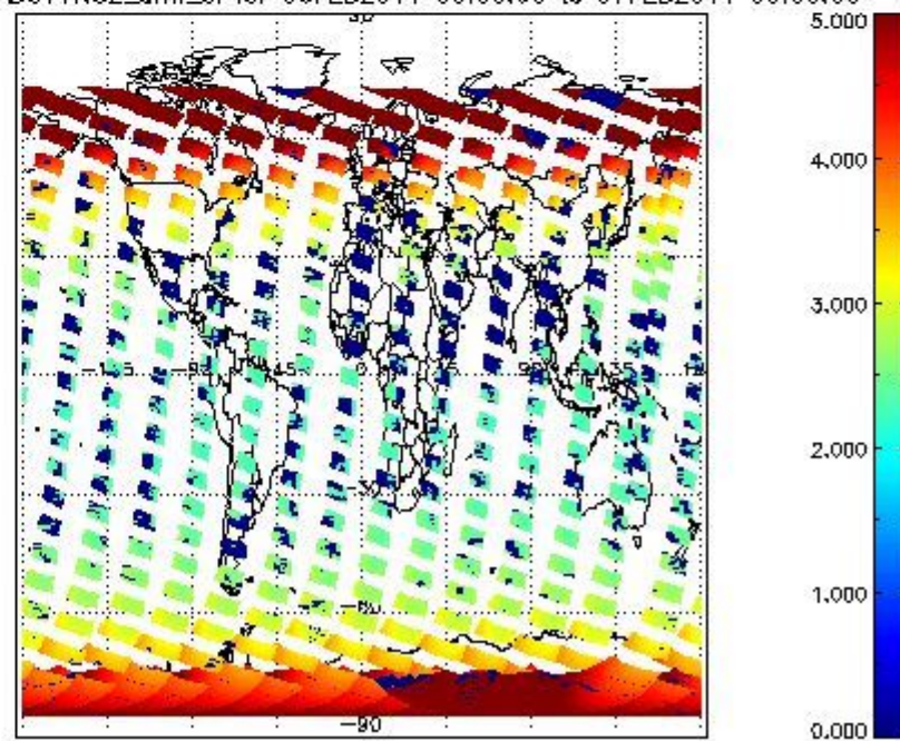
SCIOL2P_NADUV1N02_amf_cl for 06FEB2011 00:00:00 to 07FEB2011 00:00:00
