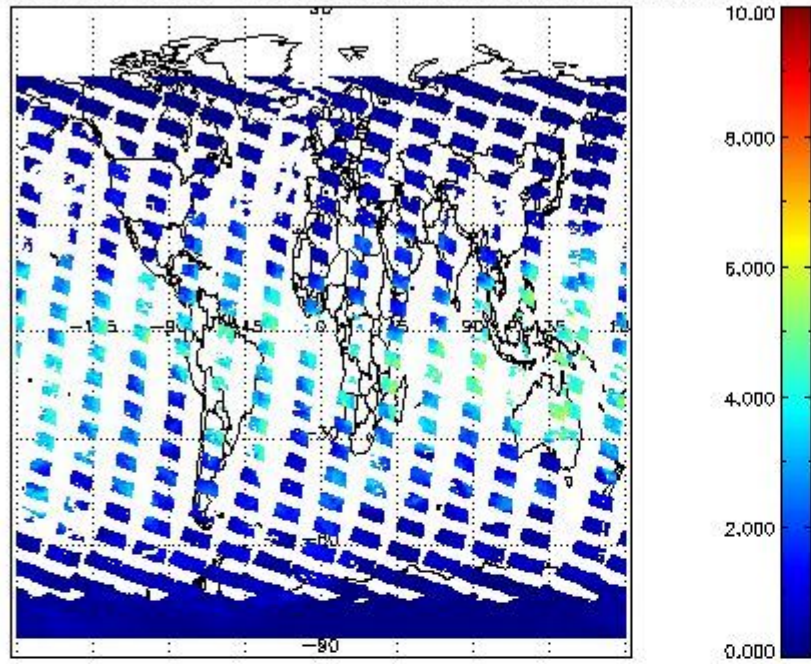
SCIOL2P_NADUV8H2O_vcd for 06FEB2011 00:00:00 to 07FEB2011 00:00:00
