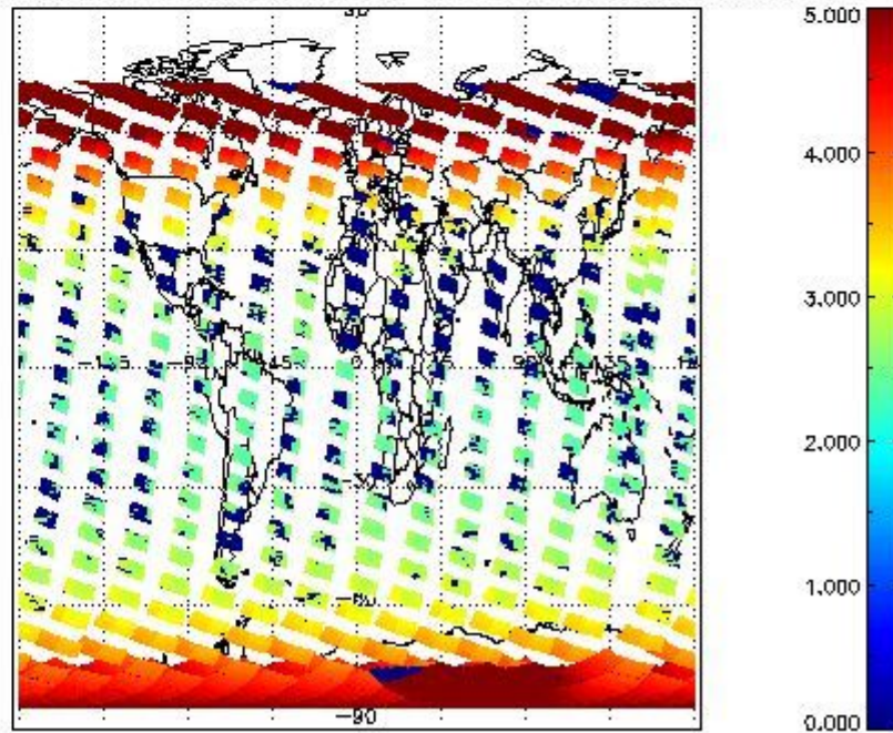
SCIOL2P_NADUV003_amf_cl for 06FEB2011 00:00:00 to 07FEB2011 00:00:00
