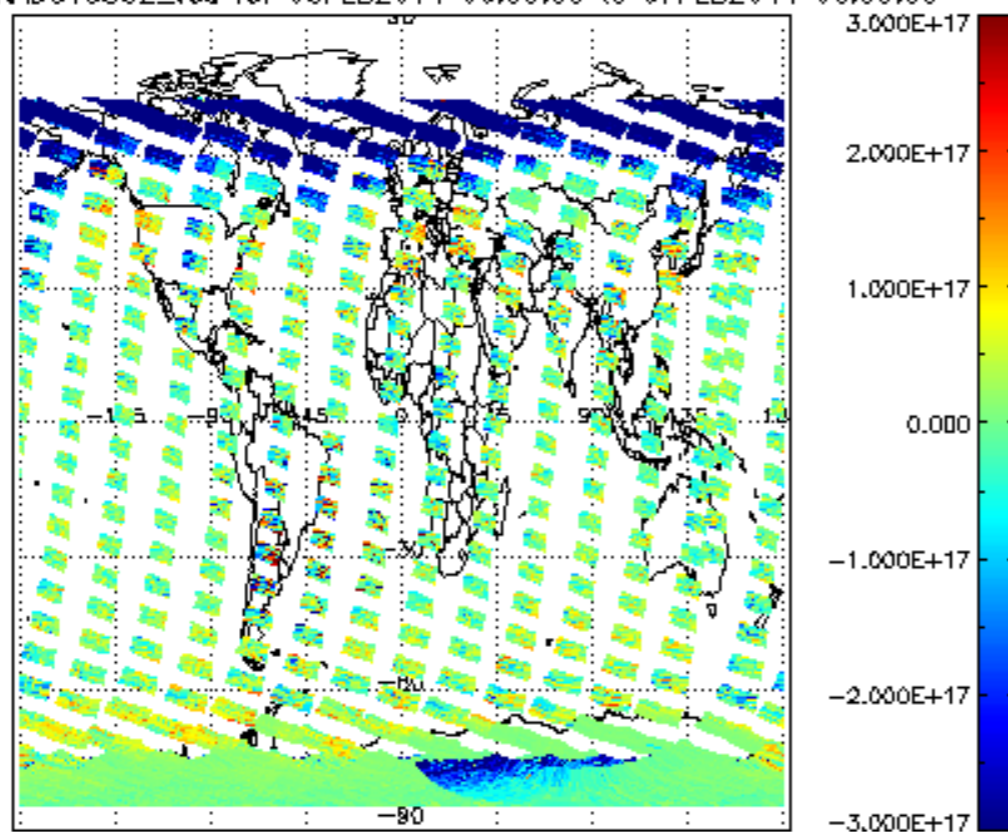
SCIOL2P_NADUV5S02_vcd for 06FEB2011 00:00:00 to 07FEB2011 00:00:00
