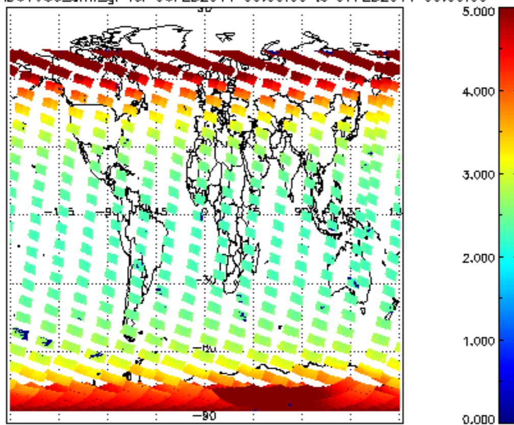
SCIOL2P_NADUV003_amf_gr for 06FEB2011 00:00:00 to 07FEB2011 00:00:00
