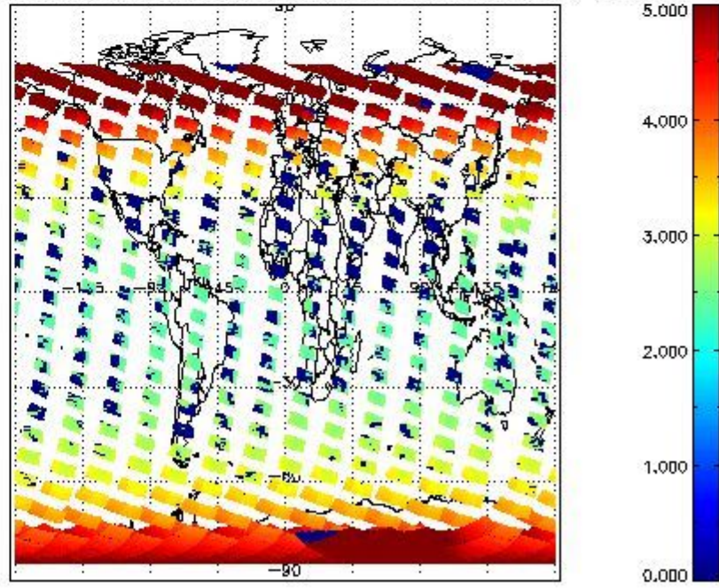
SCIOL2P_NADUV3BRO_amf_cl for 06FEB2011 00:00:00 to 07FEB2011 00:00:00
