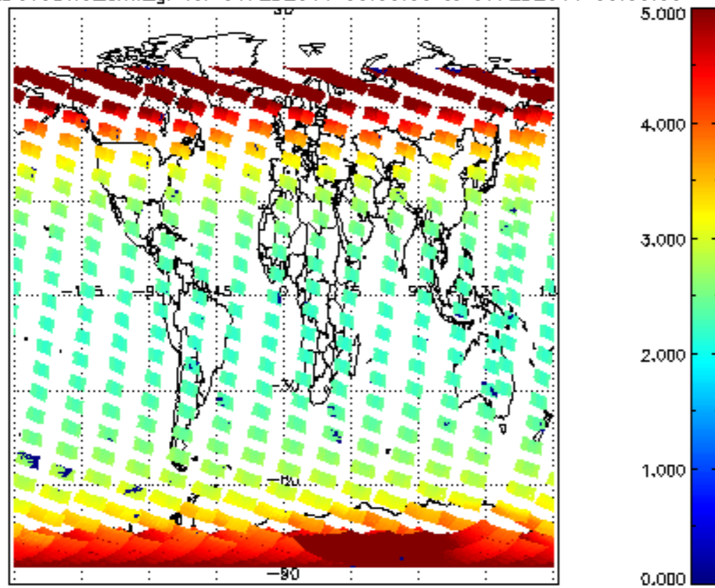
SCIOL2P_NADUV3BRO_amf_gr for 06FEB2011 00:00:00 to 07FEB2011 00:00:00
