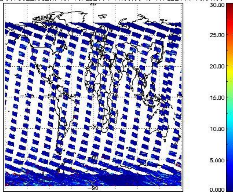
SCIOL2P_NADUV7S02_vcd_err for 06FEB2011 00:00:00 to 07FEB2011 00:00:00
