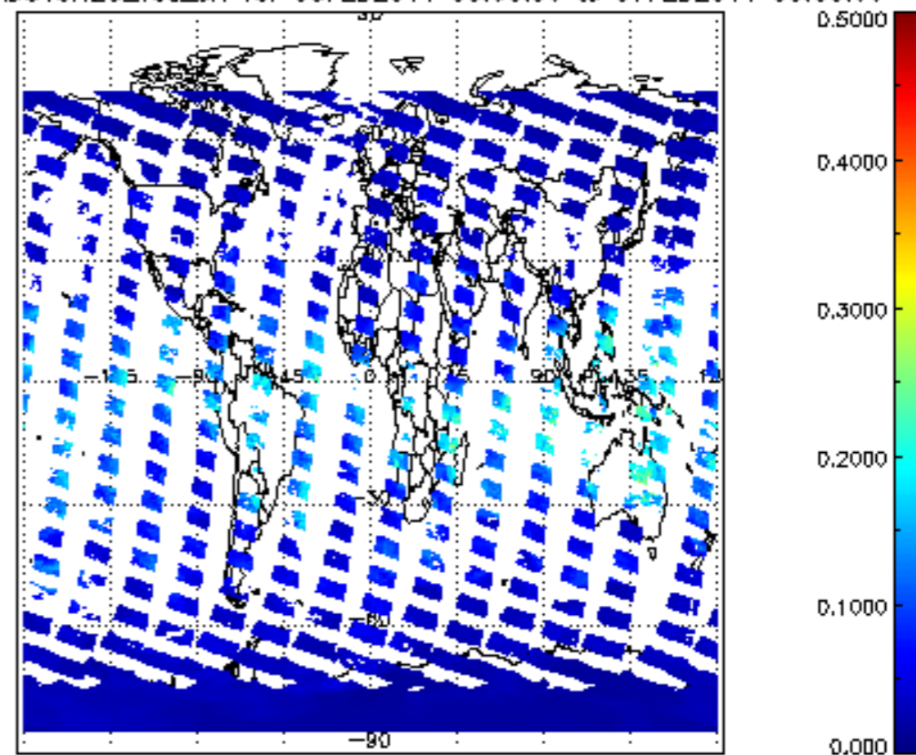
SCIOL2P_NADUV8H2O_vcd_err for 06FEB2011 00:00:00 to 07FEB2011 00:00:00
