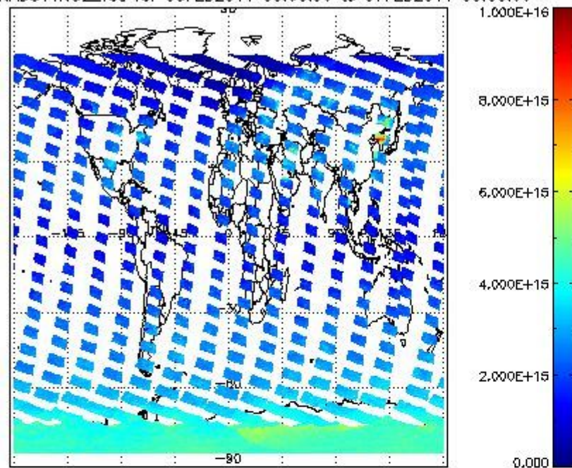
SCIOL2P_NADUV1N02_vcd for 06FEB2011 00:00:00 to 07FEB2011 00:00:00
