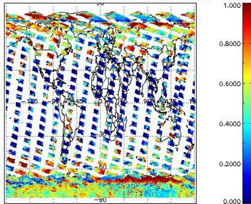
cL_frac for 06FEB2011 00:00:00 to 07FEB2011 00:00:00
