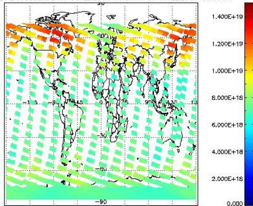
SCIOL2P_NADUV003_vcd for 06FEB2011 00:00:00 to 07FEB2011 00:00:00
