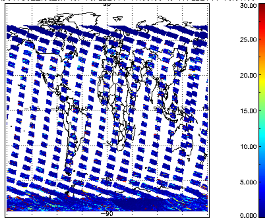
SCIOL2P_NADUV7S02_vcd_err for 06FEB2011 00:00:00 to 07FEB2011 00:00:00
