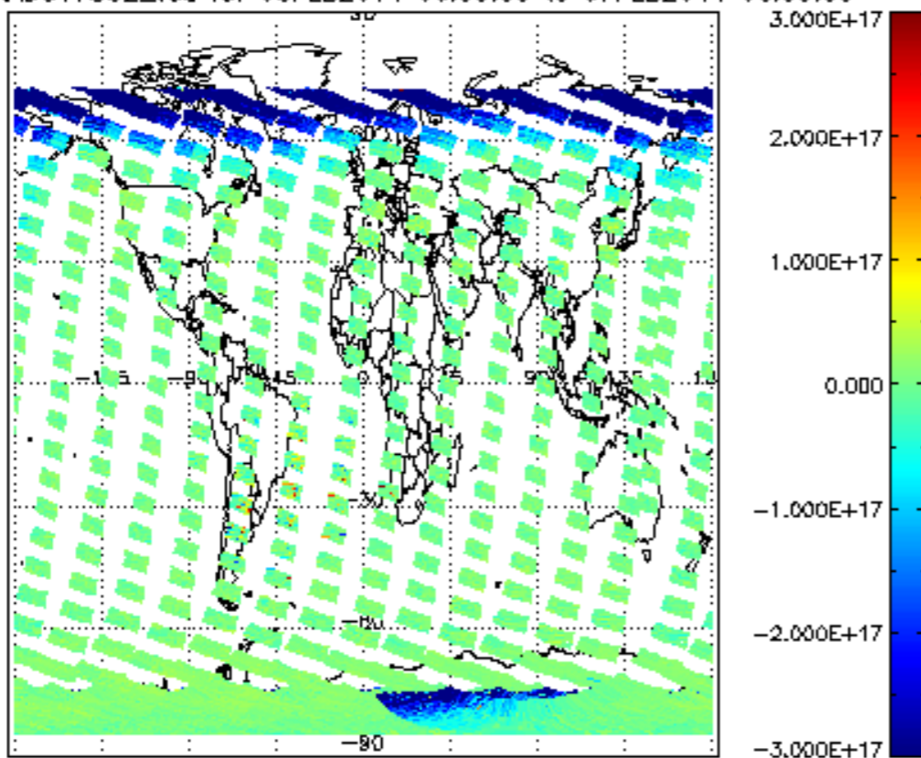
SCIOL2P_NADUV7S02_vcd for 06FEB2011 00:00:00 to 07FEB2011 00:00:00
