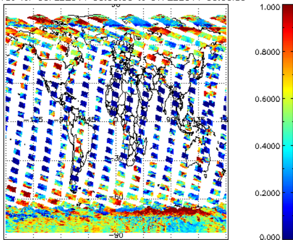
cl_frac for 06FEB2011 00:00:00 to 07FEB2011 00:00:00
