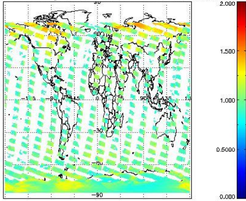
SCIOL2P_NADUV8H2O_amf_gr for 06FEB2011 00:00:00 to 07FEB2011 00:00:00
