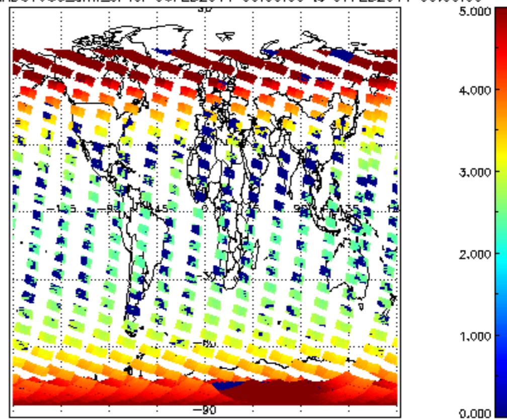
SCIOL2P_NADUV003_amf_cl for 06FEB2011 00:00:00 to 07FEB2011 00:00:00
