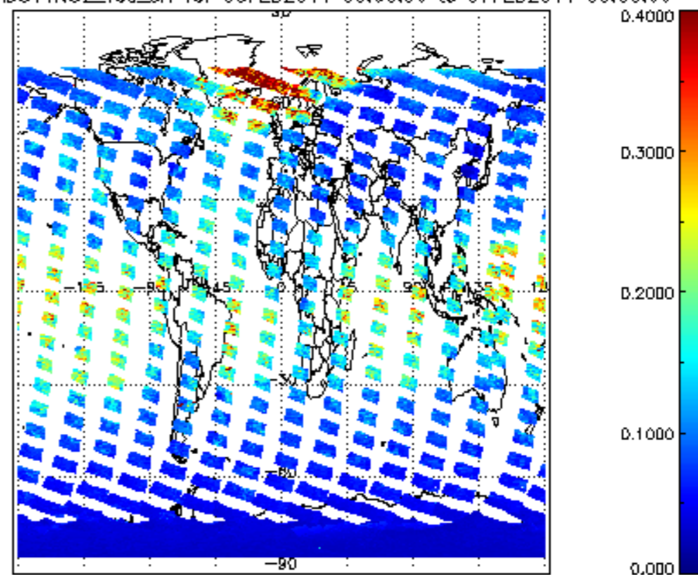
SCIOL2P_NADUV1N02_vcd_err for 06FEB2011 00:00:00 to 07FEB2011 00:00:00
