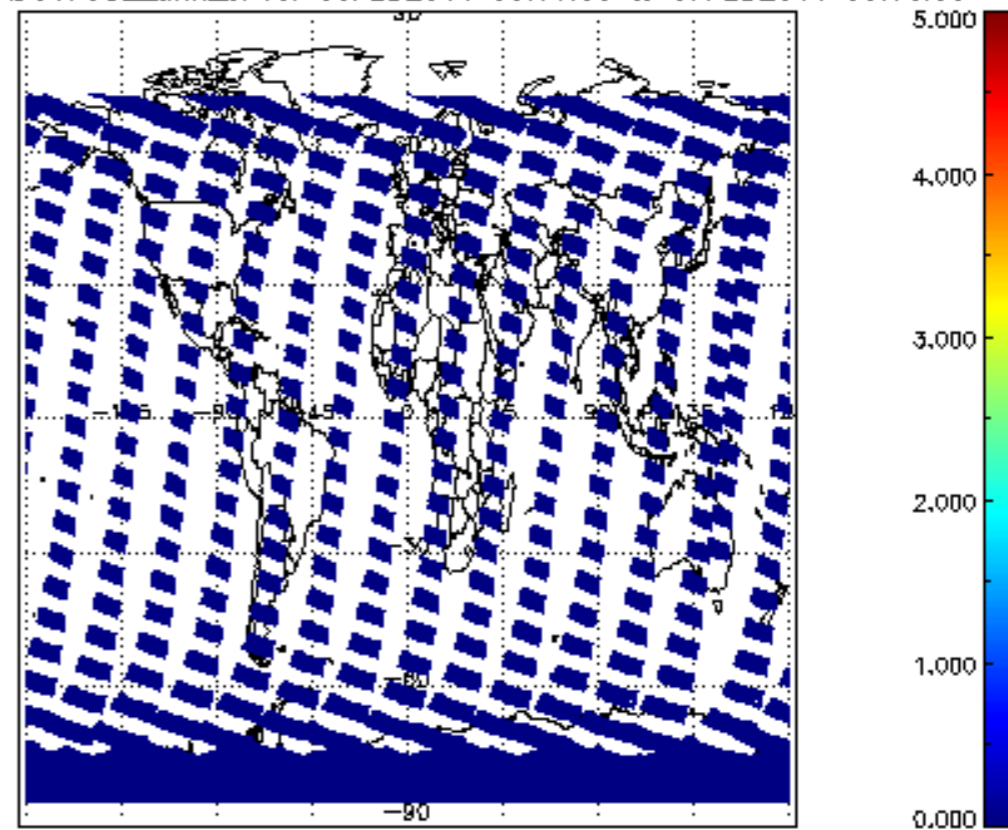
SCIOL2P_NADUV7S02_amf_cl for 06FEB2011 00:00:00 to 07FEB2011 00:00:00
