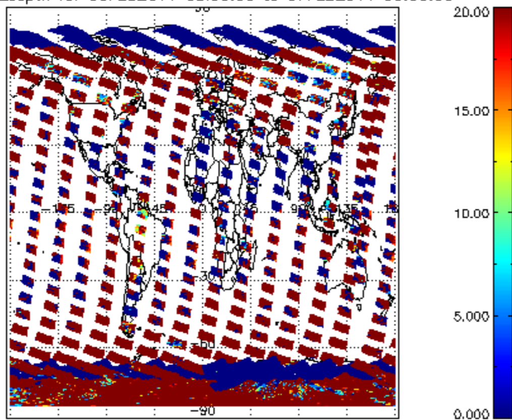
cl_opt_depth for 06FEB2011 00:00:00 to 07FEB2011 00:00:00
