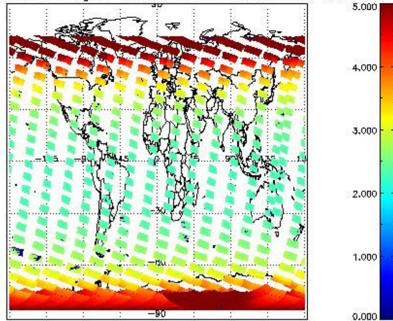
SCIOL2P_NADUV003_amf_gr for 06FEB2011 00:00:00 to 07FEB2011 00:00:00
