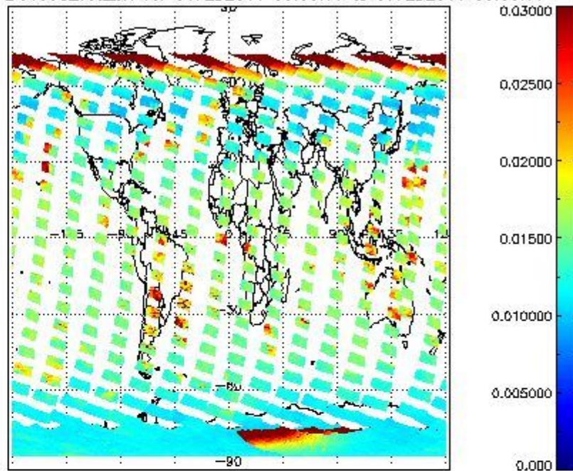
SCIOL2P_NADUV003_vcd_err for 06FEB2011 00:00:00 to 07FEB2011 00:00:00
