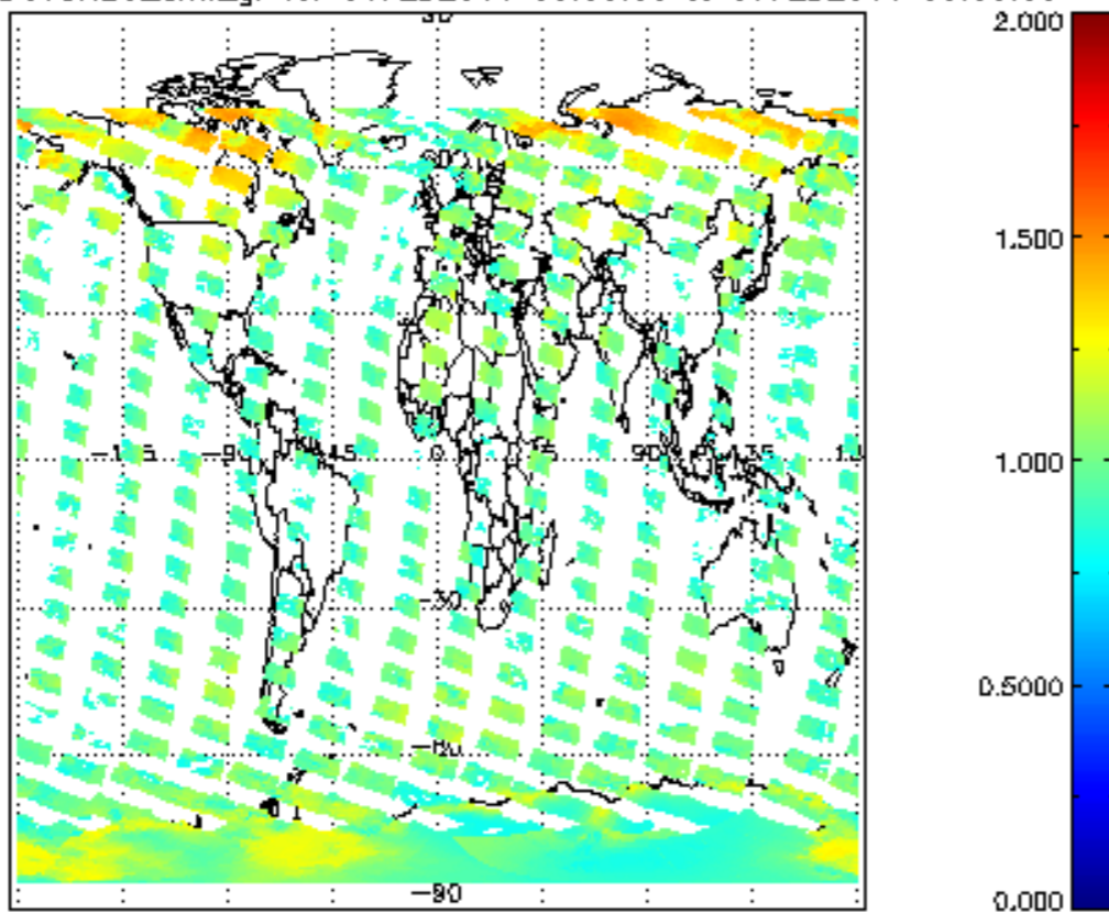
SCIOL2P_NADUV8H2O_amf_gr for 06FEB2011 00:00:00 to 07FEB2011 00:00:00
