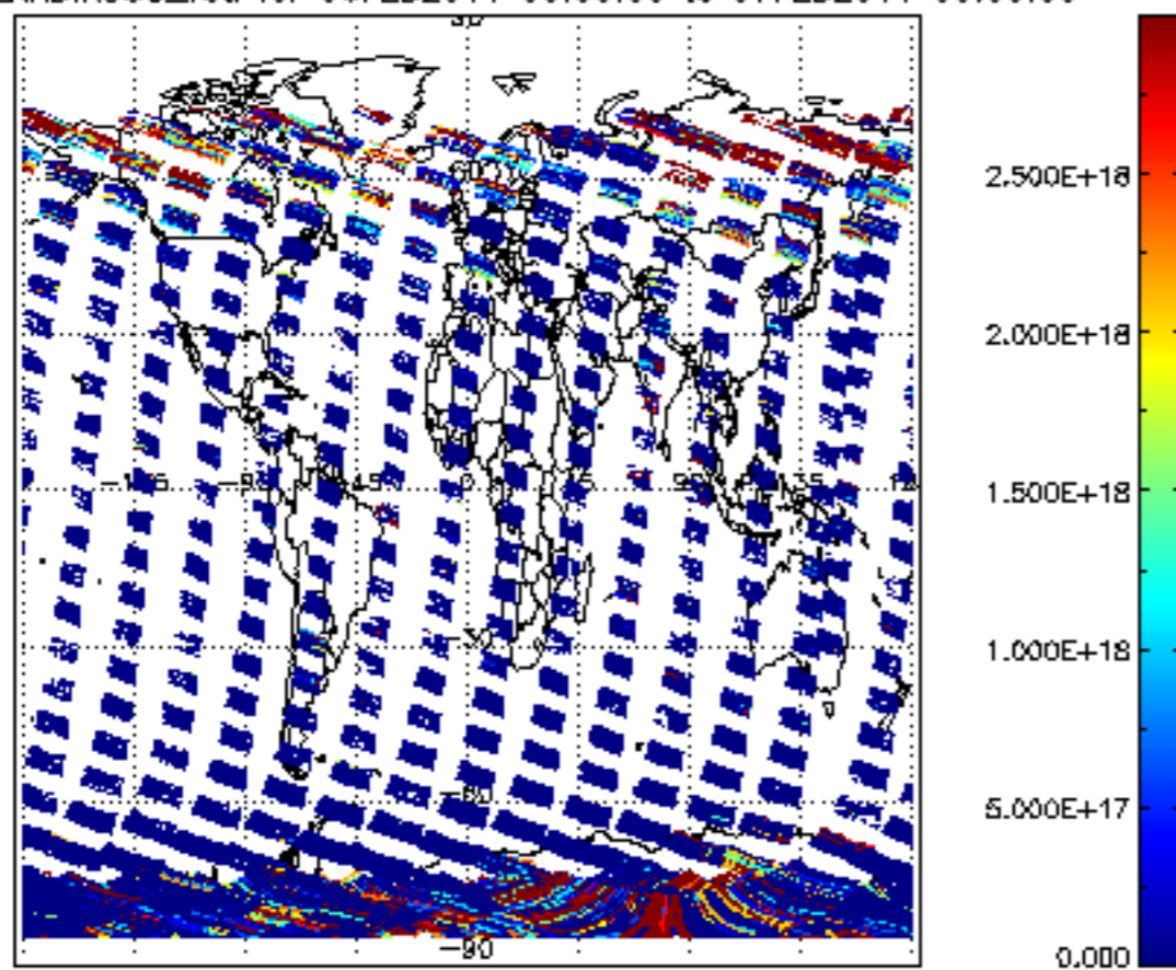
SCIOL2P_NADIR3CO_vcd for 06FEB2011 00:00:00 to 07FEB2011 00:00:00
