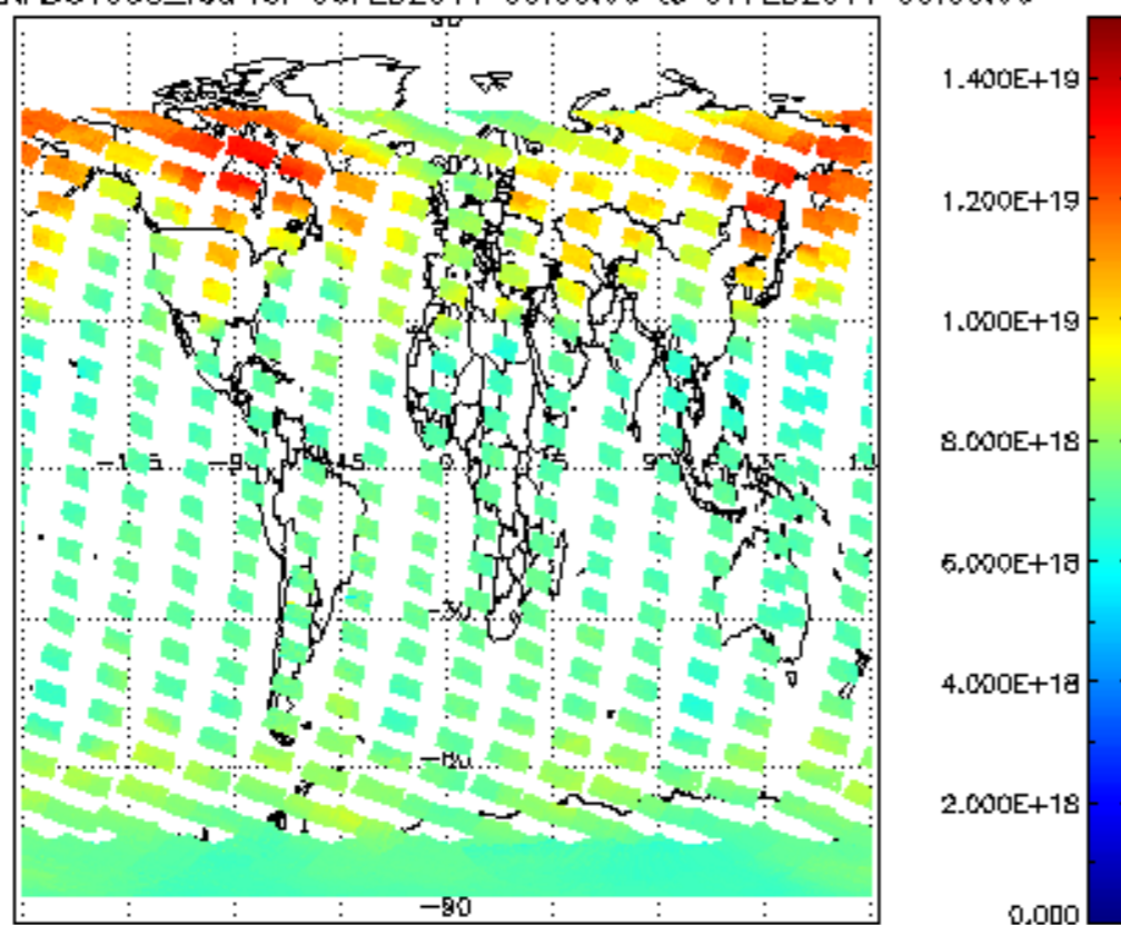
SCIOL2P_NADUV003_vcd for 06FEB2011 00:00:00 to 07FEB2011 00:00:00
