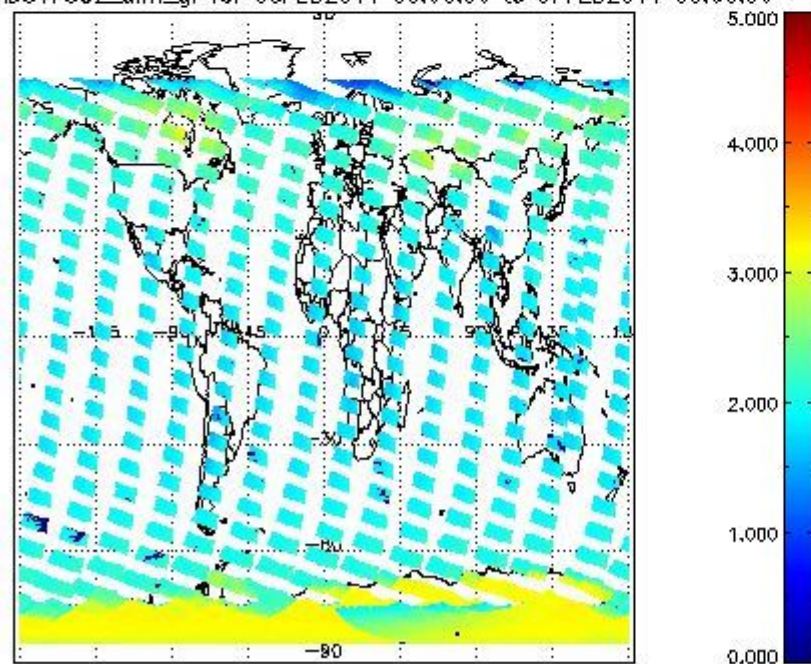
SCIOL2P_NADUV7S02_amf_gr for 06FEB2011 00:00:00 to 07FEB2011 00:00:00
