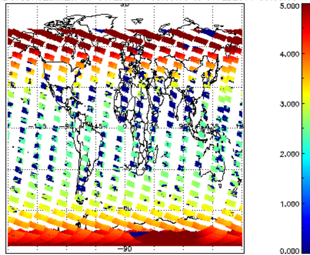
SCIOL2P_NADUV3BRO_amf_cl for 06FEB2011 00:00:00 to 07FEB2011 00:00:00
