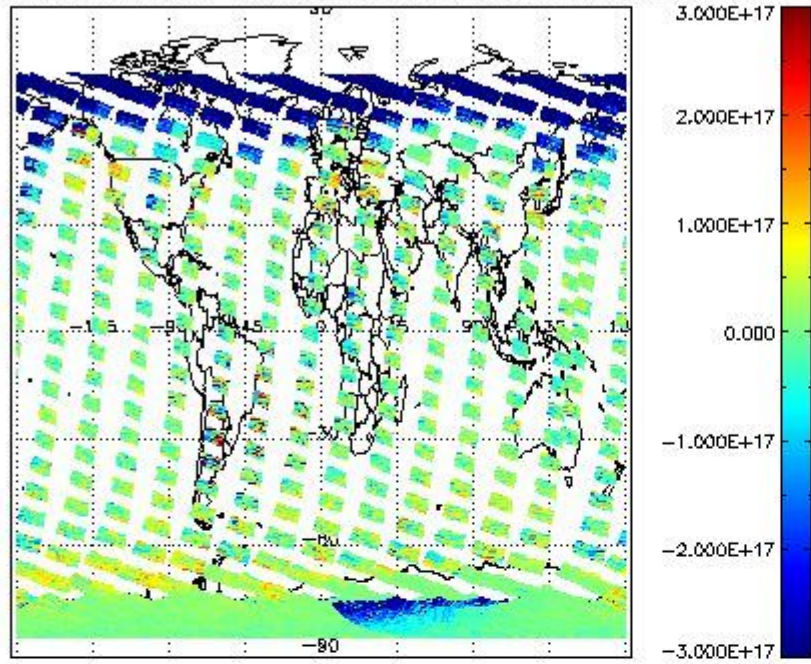
SCIOL2P_NADUV5S02_vcd for 06FEB2011 00:00:00 to 07FEB2011 00:00:00
