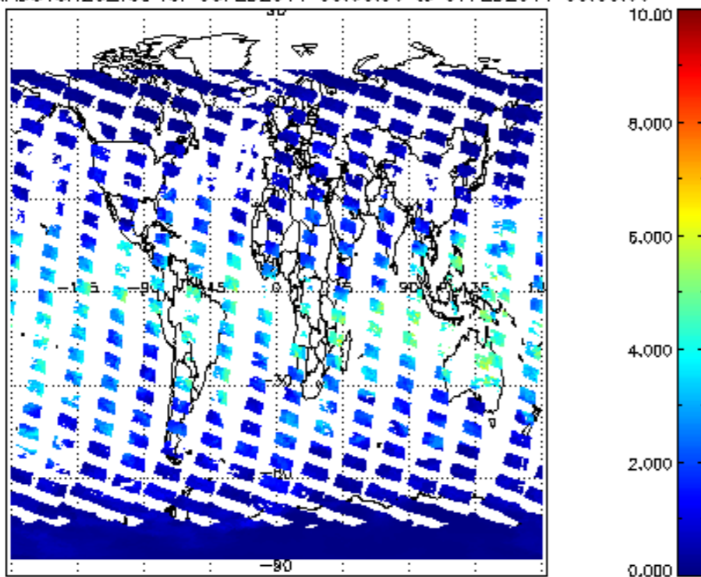
SCIOL2P_NADUV8H2O_vcd for 06FEB2011 00:00:00 to 07FEB2011 00:00:00
