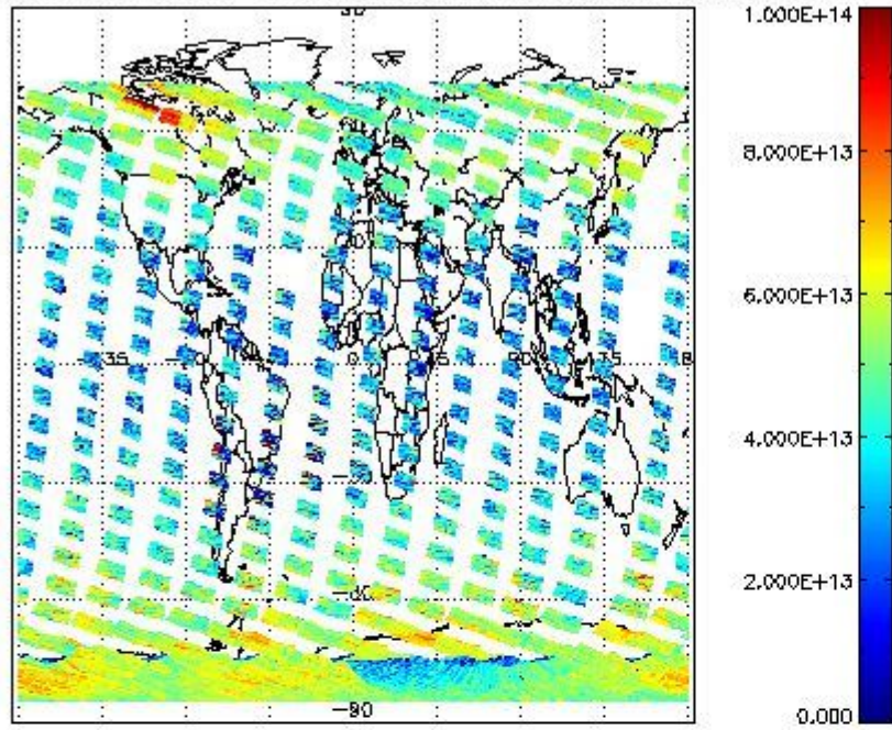
SCIOL2P_NADUV3BRO_vcd for 05FEB2011 00:00:00 to 06FEB2011 00:00:00
