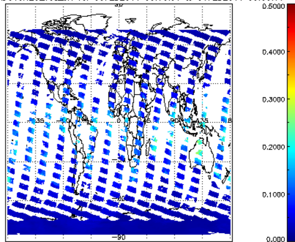
SCIOL2P_NADUV8H20_vcd_err for 05FEB2011 00:00:00 to 06FEB2011 00:00:00
