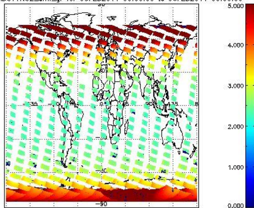
SCIOL2P_NADUV1N02_amf_gr for 05FEB2011 00:00:00 to 06FEB2011 00:00:00
