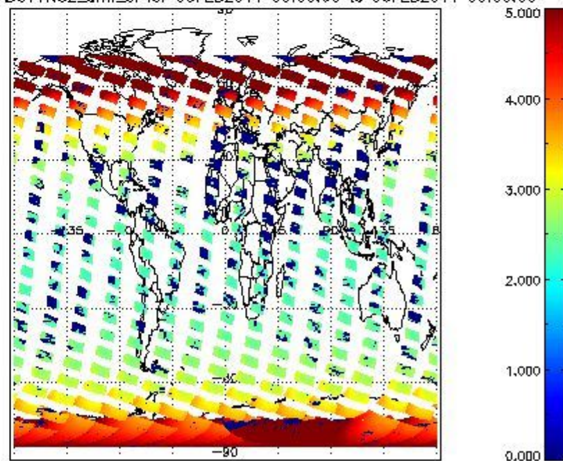
SCIOL2P_NADUV1N02_amf_cl for 05FEB2011 00:00:00 to 06FEB2011 00:00:00
