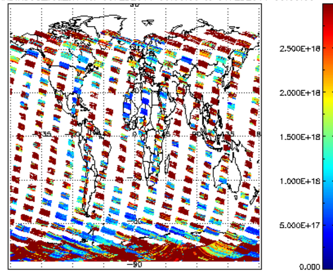
SCIOL2P_NADIR3CO_vcd_err for 05FEB2011 00:00:00 to 06FEB2011 00:00:00
