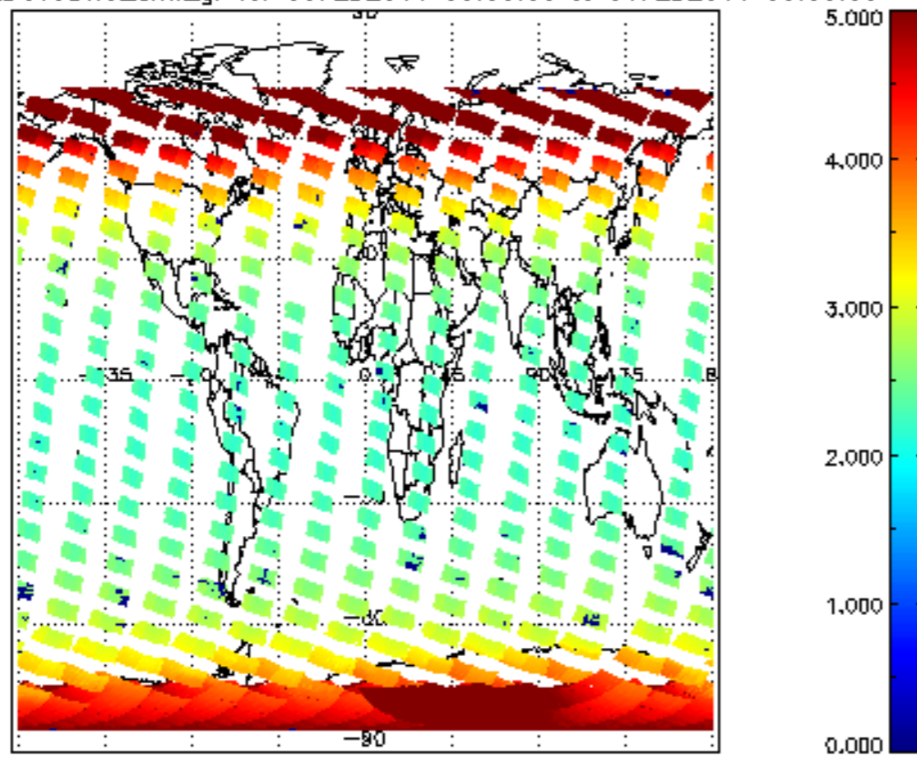
SCIOL2P_NADUV3BRO_amf_gr for 05FEB2011 00:00:00 to 06FEB2011 00:00:00
