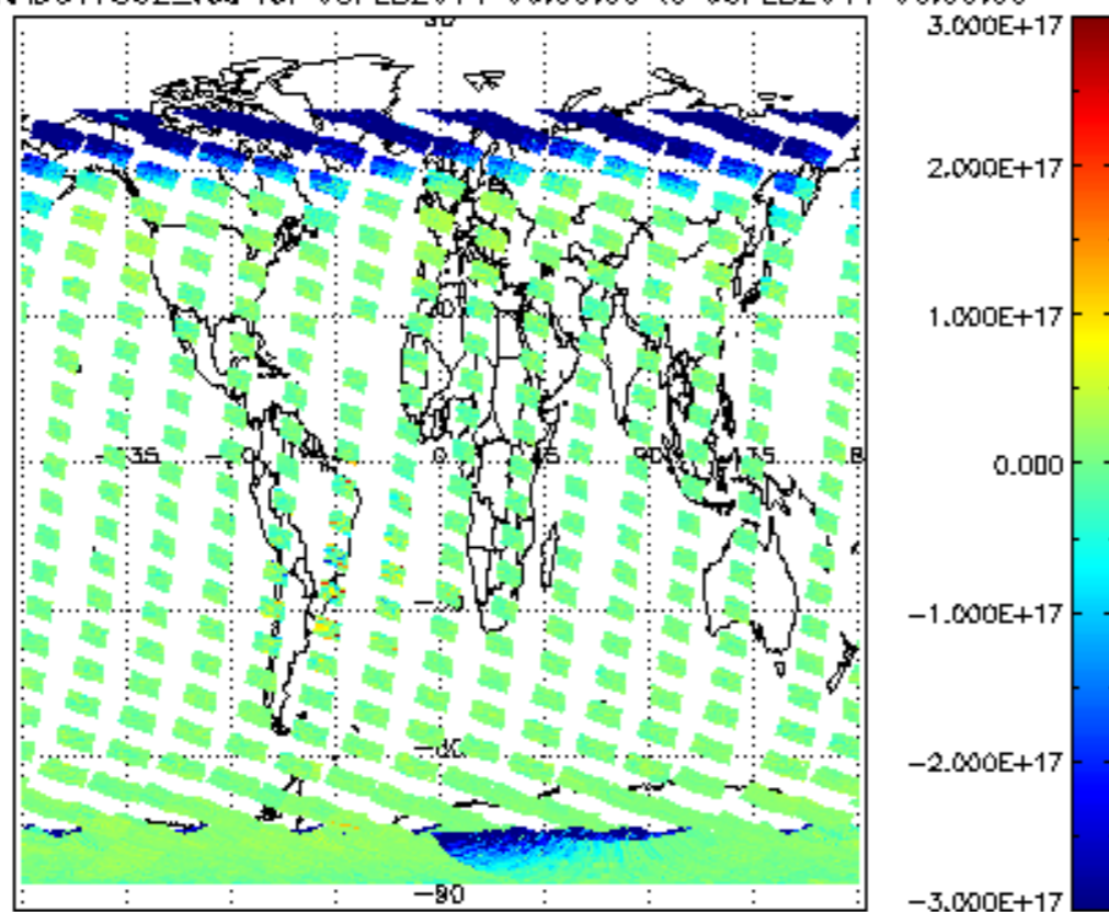
SCIOL2P_NADUV7S02_vcd for 05FEB2011 00:00:00 to 06FEB2011 00:00:00
