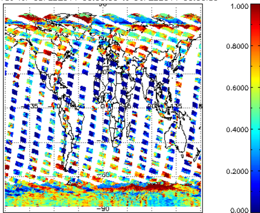
cL_frac for 05FEB2011 00:00:00 to 06FEB2011 00:00:00
