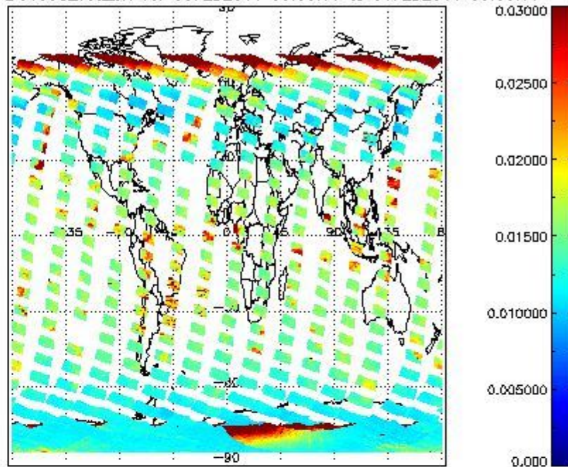
SCIOL2P_NADUV003_vcd_err for 05FEB2011 00:00:00 to 06FEB2011 00:00:00
