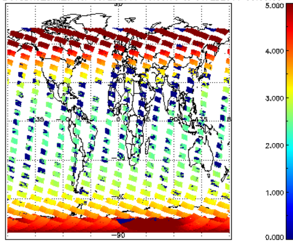
SCIOL2P_NADUV3BRO_amf_cl for 05FEB2011 00:00:00 to 06FEB2011 00:00:00
