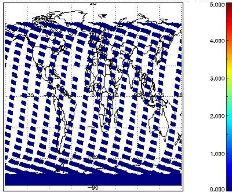
SCIOL2P_NADUV5S02_amf_cl for 05FEB2011 00:00:00 to 06FEB2011 00:00:00
