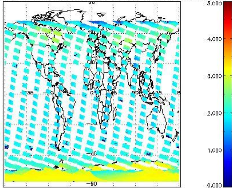
SCIOL2P_NADUV7S02_amf_gr for 05FEB2011 00:00:00 to 06FEB2011 00:00:00
