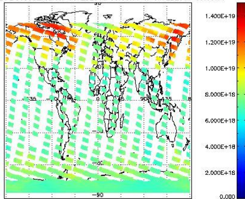
SCIOL2P_NADUV003_vcd for 05FEB2011 00:00:00 to 06FEB2011 00:00:00
