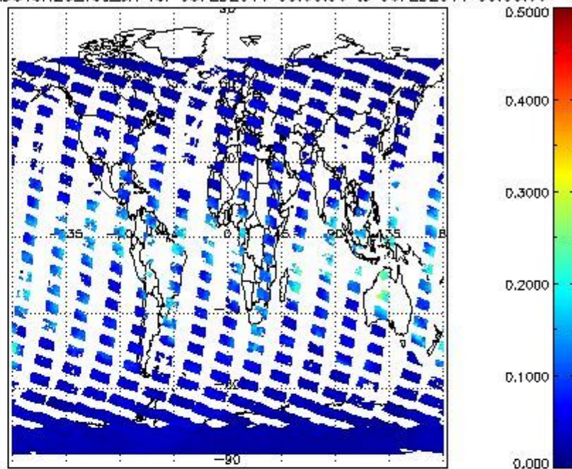
SCIOL2P_NADUV8H2O_vcd_err for 05FEB2011 00:00:00 to 06FEB2011 00:00:00
