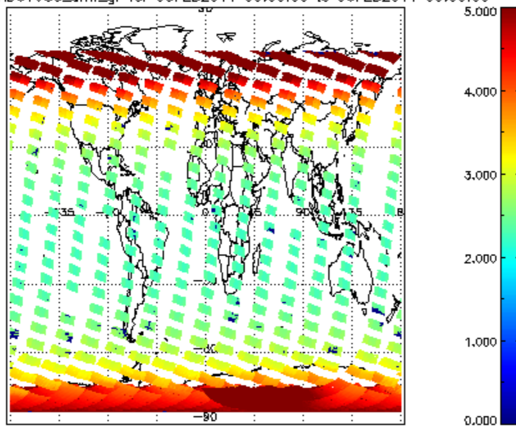
SCIOL2P_NADUV003_amf_gr for 05FEB2011 00:00:00 to 06FEB2011 00:00:00
