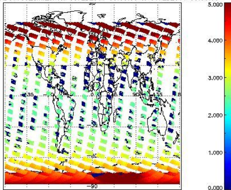
SCIOL2P_NADUV003_amf_cl for 05FEB2011 00:00:00 to 06FEB2011 00:00:00
