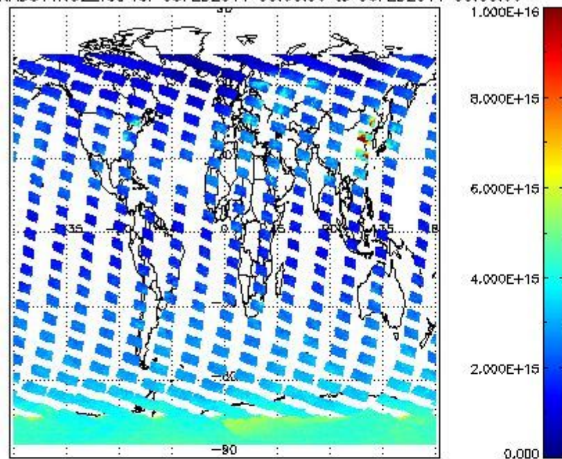
SCIOL2P_NADUV1N02_vcd for 05FEB2011 00:00:00 to 06FEB2011 00:00:00
