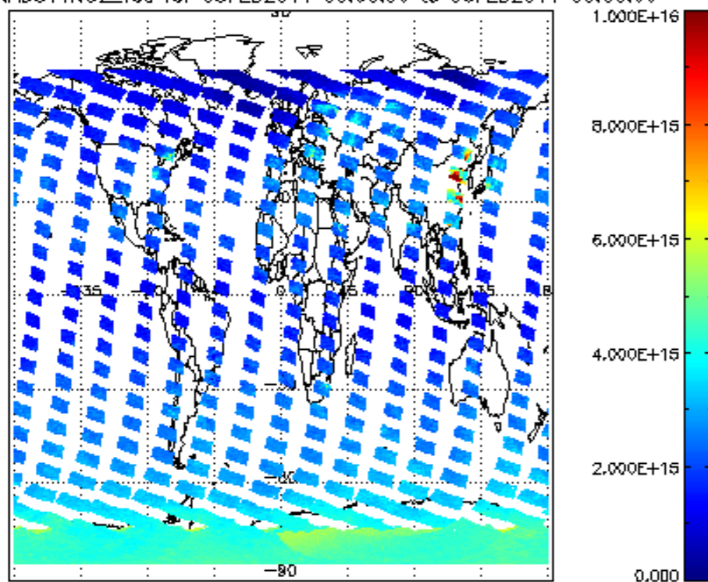
SCIOL2P_NADUV1N02_vcd for 05FEB2011 00:00:00 to 06FEB2011 00:00:00
