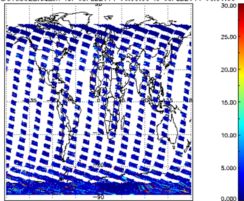
SCIOL2P_NADUV5S02_vcd_err for 05FEB2011 00:00:00 to 06FEB2011 00:00:00
