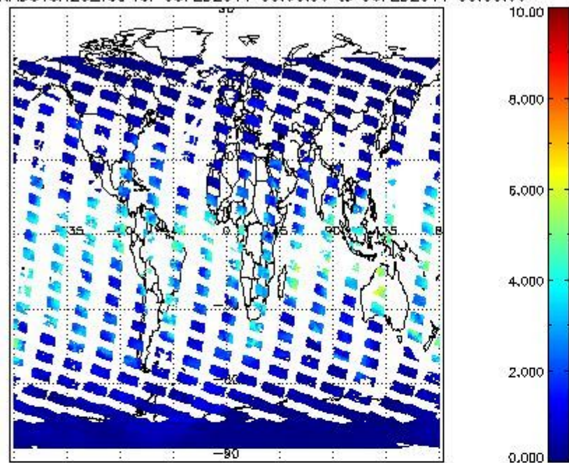
SCIOL2P_NADUV8H2O_vcd for 05FEB2011 00:00:00 to 06FEB2011 00:00:00
