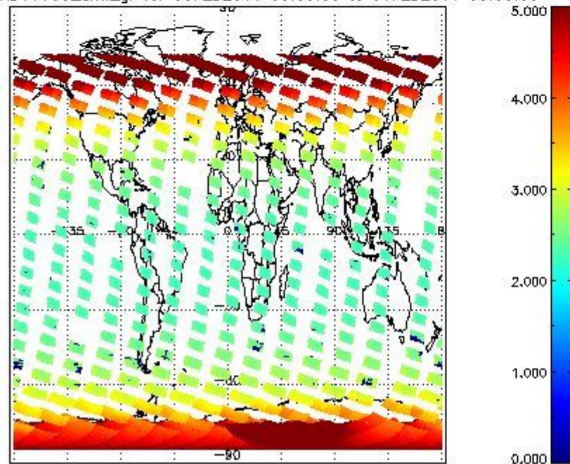
SCIOL2P_NADUV003_amf_gr for 05FEB2011 00:00:00 to 06FEB2011 00:00:00
