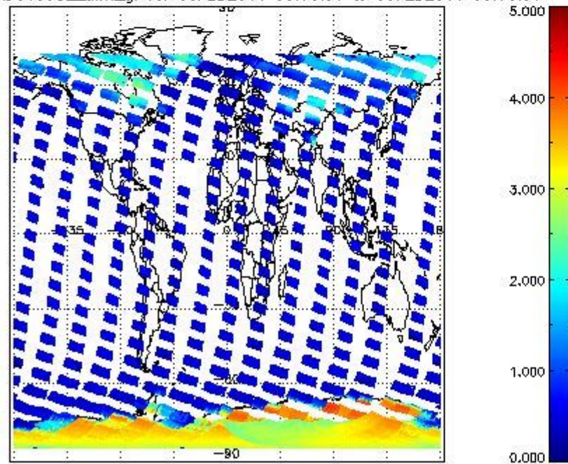
SCIOL2P_NADUV5S02_amf_gr for 05FEB2011 00:00:00 to 06FEB2011 00:00:00
