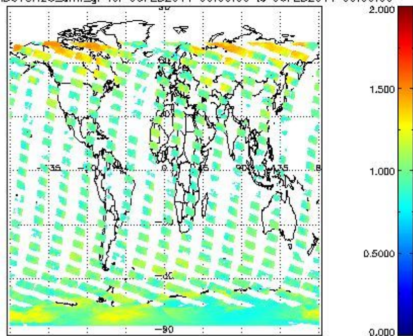
SCIOL2P_NADUV8H2O_amf_gr for 05FEB2011 00:00:00 to 06FEB2011 00:00:00
