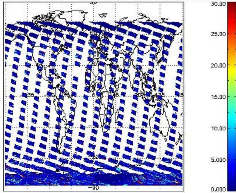
SCIOL2P_NADUV7S02_vcd_err for 05FEB2011 00:00:00 to 06FEB2011 00:00:00
