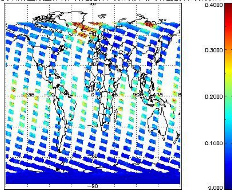
SCIOL2P_NADUV1N02_vcd_err for 05FEB2011 00:00:00 to 06FEB2011 00:00:00
