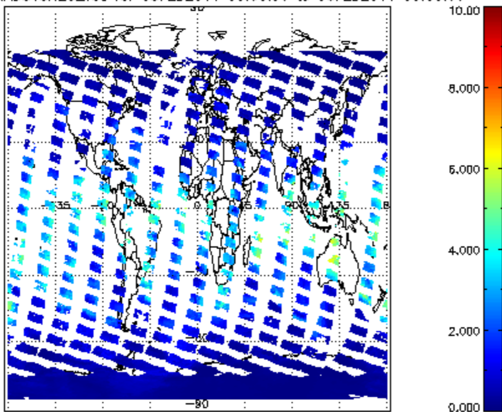
SCIOL2P_NADUV8H20_vcd for 05FEB2011 00:00:00 to 06FEB2011 00:00:00
