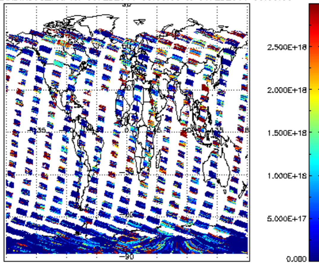
SCIOL2P_NADIR3CO_vcd for 05FEB2011 00:00:00 to 06FEB2011 00:00:00
