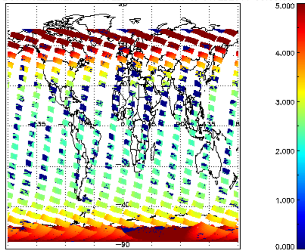
SCIOL2P_NADUV1N02_amf_cl for 05FEB2011 00:00:00 to 06FEB2011 00:00:00
