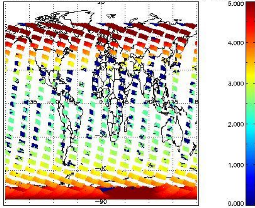
SCIOL2P_NADUV3BRO_amf_cl for 05FEB2011 00:00:00 to 06FEB2011 00:00:00
