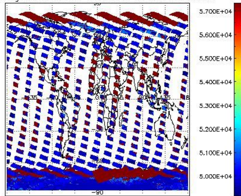
cloud_flags for 05FEB2011 00:00:00 to 06FEB2011 00:00:00
