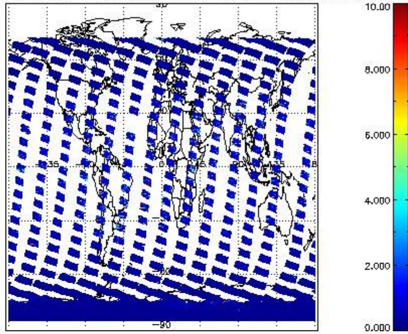
SCIOL2P_NADUV3BRO_vcd_err for 05FEB2011 00:00:00 to 06FEB2011 00:00:00
