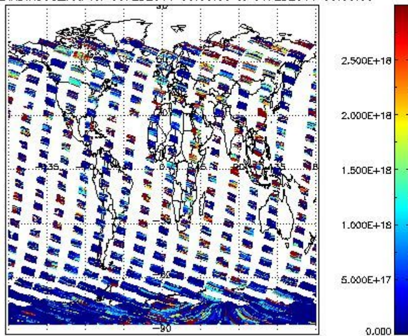
SCIDL2P_NADIR3CO_vcd for 05FEB2011 00:00:00 to 06FEB2011 00:00:00
