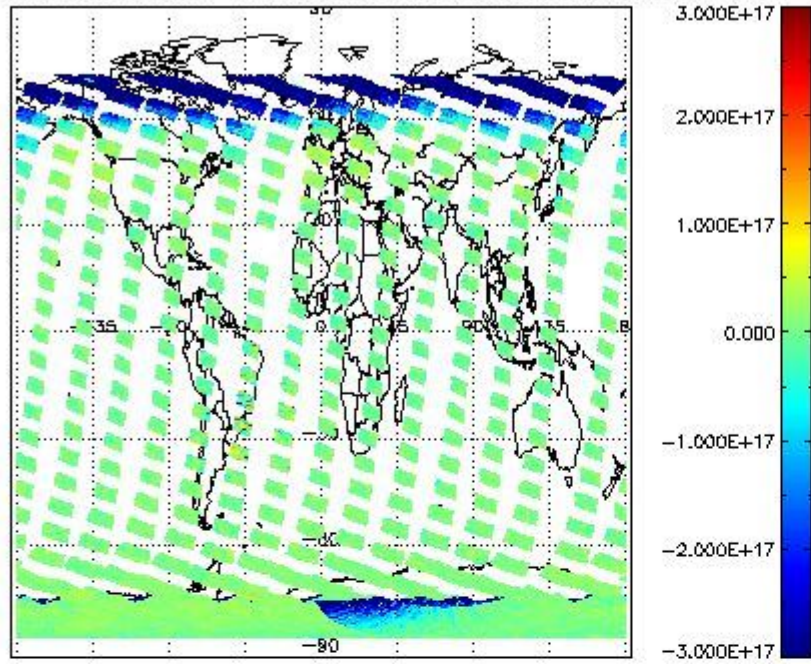
SCIOL2P_NADUV7S02_vcd for 05FEB2011 00:00:00 to 06FEB2011 00:00:00
