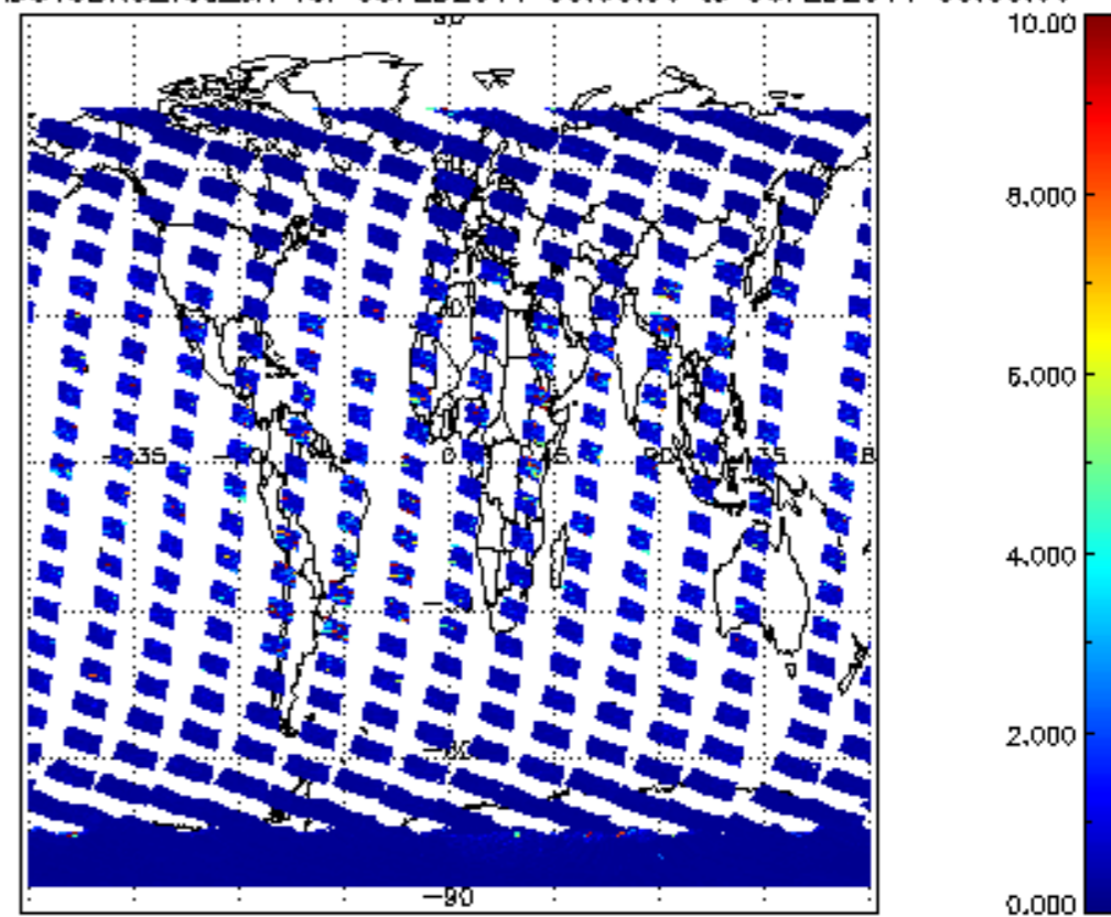
SCIOL2P_NADUV3BRO_vcd_err for 05FEB2011 00:00:00 to 06FEB2011 00:00:00
