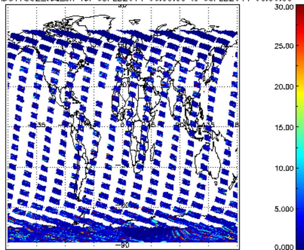
SCIOL2P_NADUV7S02_vcd_err for 05FEB2011 00:00:00 to 06FEB2011 00:00:00
