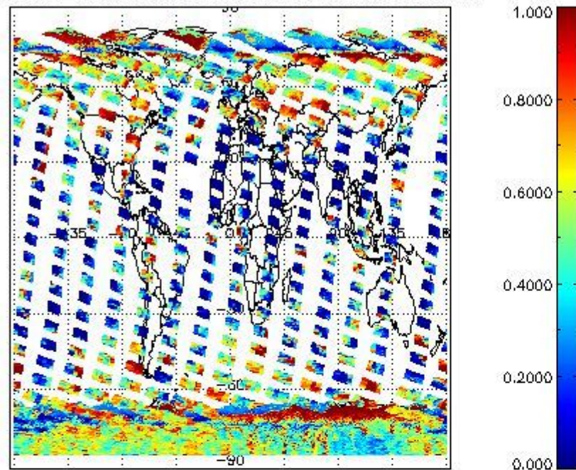
cL_frac for 05FEB2011 00:00:00 to 06FEB2011 00:00:00
