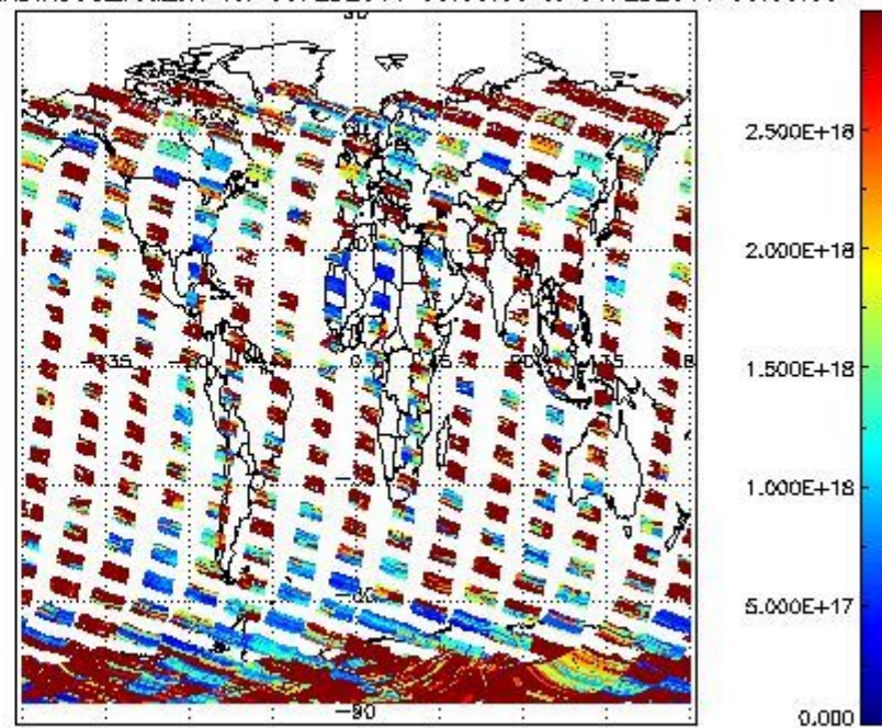
SCIDL2P_NADIR3CO_vcd_err for 05FEB2011 00:00:00 to 06FEB2011 00:00:00
