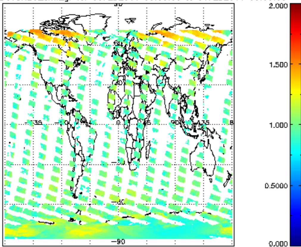
SCIOL2P_NADUV8H20_amf_gr for 05FEB2011 00:00:00 to 06FEB2011 00:00:00
