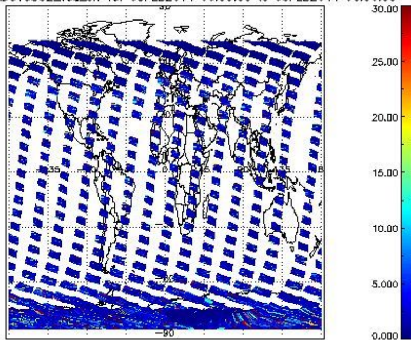
SCIOL2P_NADUV5S02_vcd_err for 05FEB2011 00:00:00 to 06FEB2011 00:00:00
