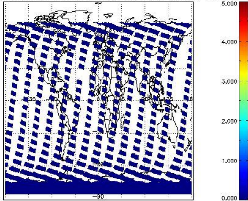
SCIOL2P_NADUV7S02_amf_cl for 05FEB2011 00:00:00 to 06FEB2011 00:00:00
