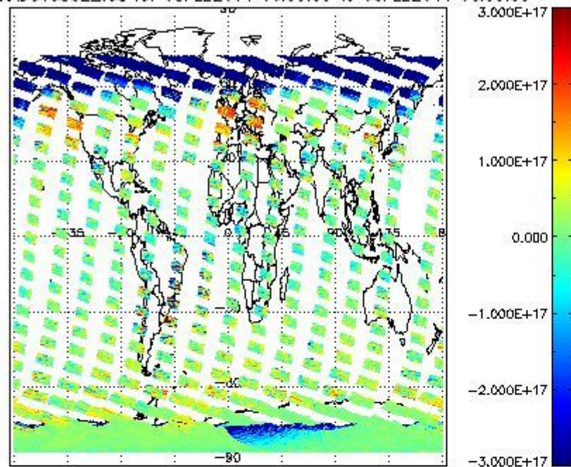
SCIOL2P_NADUV5S02_vcd for 05FEB2011 00:00:00 to 06FEB2011 00:00:00
