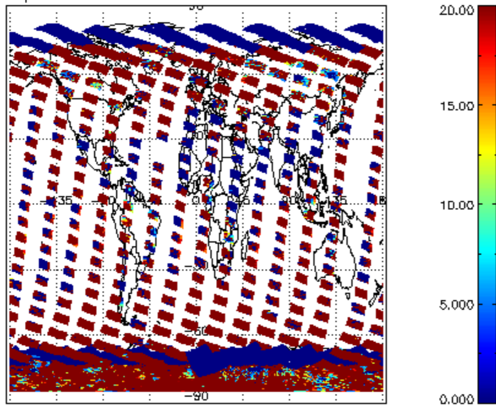
cL_opt_depth for 05FEB2011 00:00:00 to 06FEB2011 00:00:00
