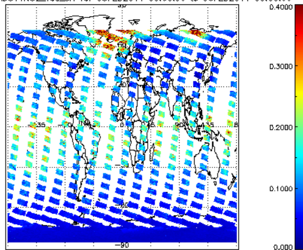
SCIOL2P_NADUV1N02_vcd_err for 05FEB2011 00:00:00 to 06FEB2011 00:00:00
