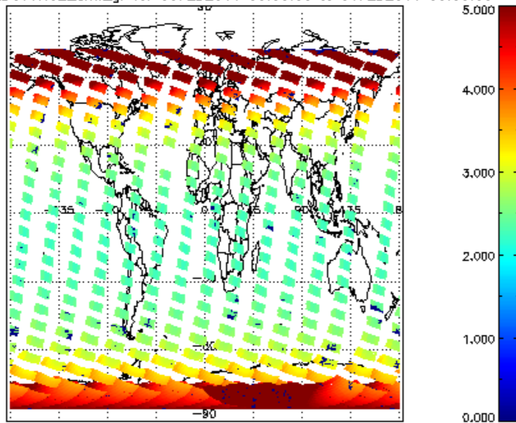
SCIOL2P_NADUV1N02_amf_gr for 05FEB2011 00:00:00 to 06FEB2011 00:00:00
