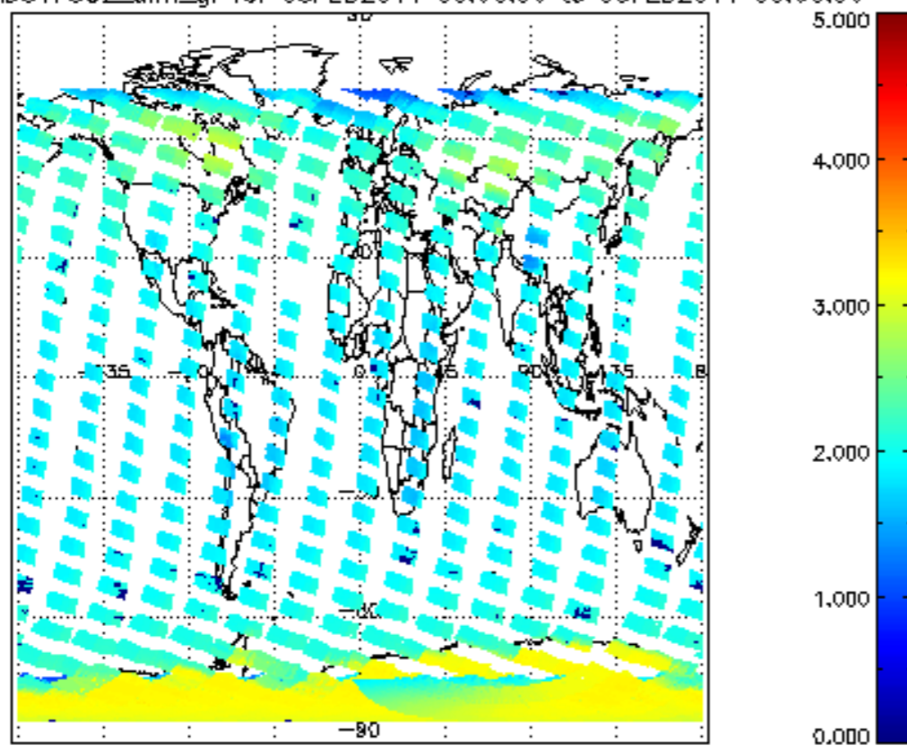
SCIOL2P_NADUV7S02_amf_gr for 05FEB2011 00:00:00 to 06FEB2011 00:00:00
