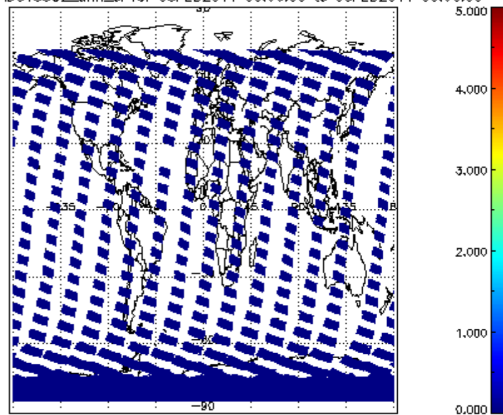
SCIOL2P_NADUV5S02_amf_cl for 05FEB2011 00:00:00 to 06FEB2011 00:00:00
