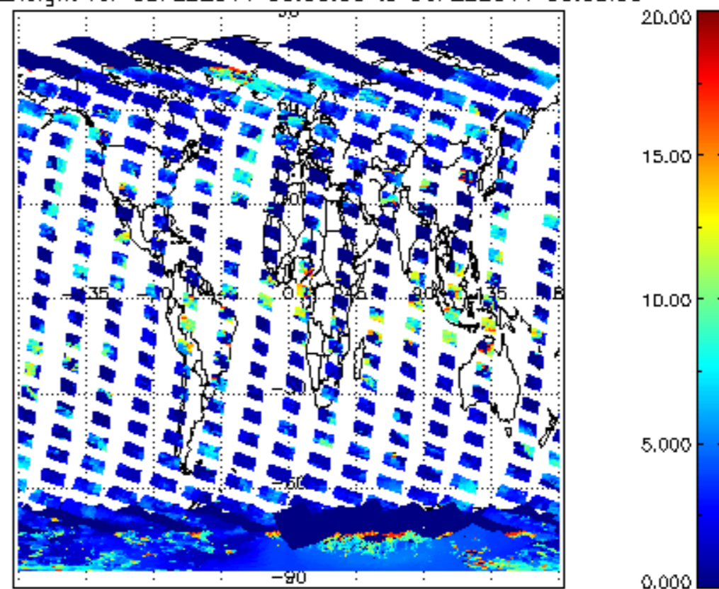
cL_top_height for 05FEB2011 00:00:00 to 06FEB2011 00:00:00
