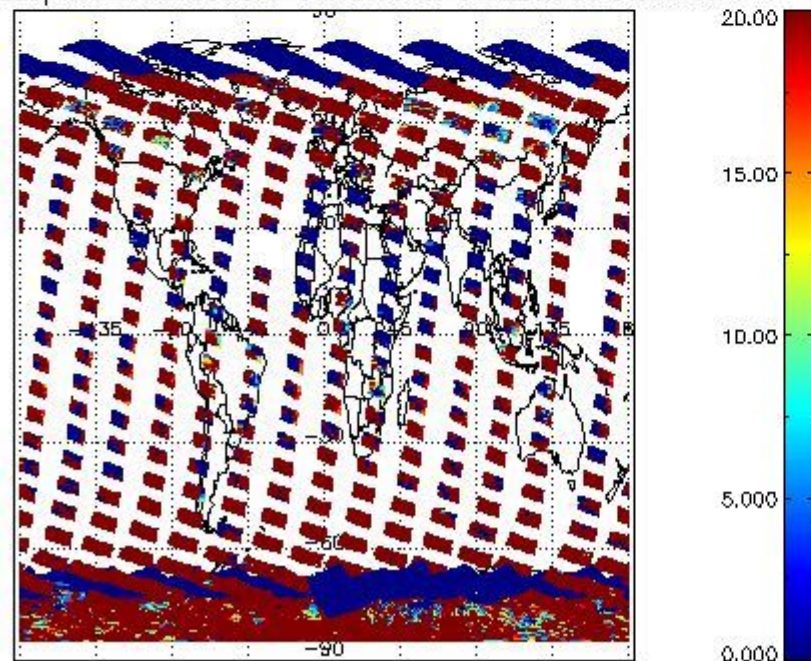
cL_opt_depth for 05FEB2011 00:00:00 to 06FEB2011 00:00:00
