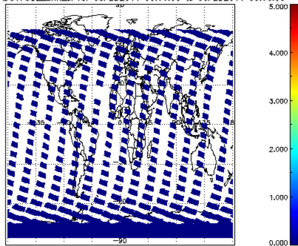
SCIOL2P_NADUV7S02_amf_cl for 05FEB2011 00:00:00 to 06FEB2011 00:00:00
