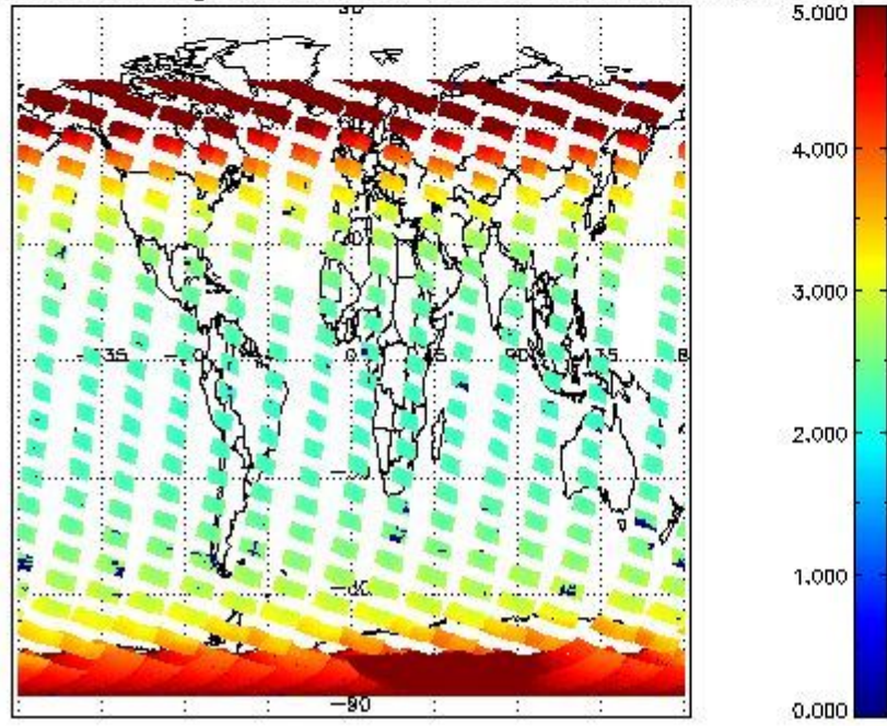
SCIOL2P_NADUV3BRO_amf_gr for 05FEB2011 00:00:00 to 06FEB2011 00:00:00
