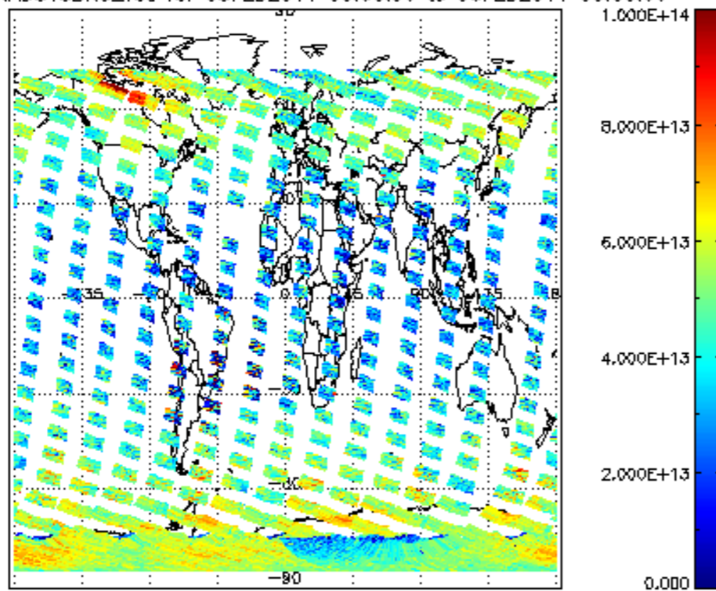
SCIOL2P_NADUV3BRO_vcd for 05FEB2011 00:00:00 to 06FEB2011 00:00:00
