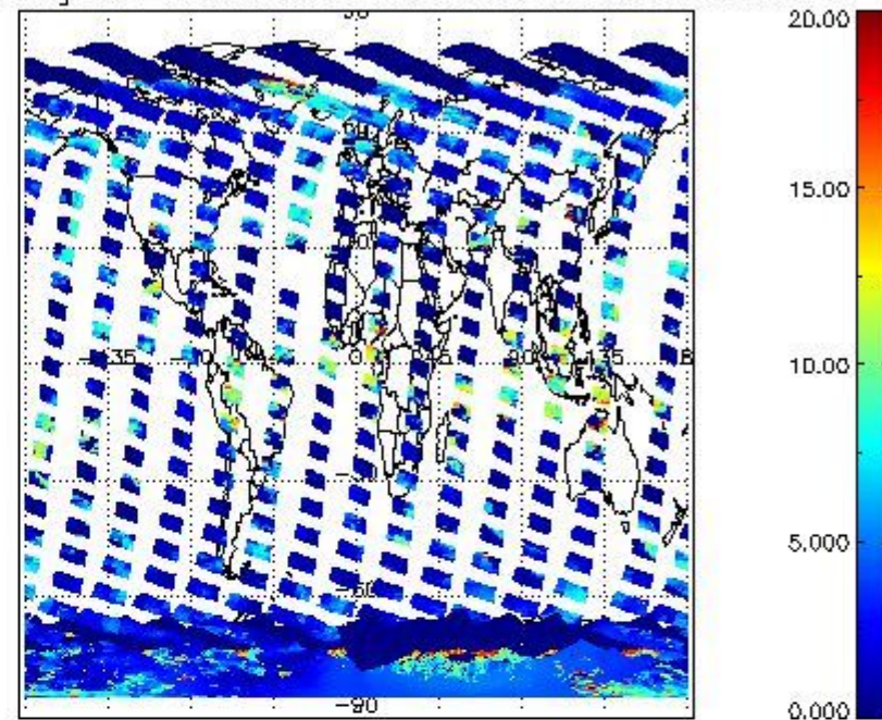
cL_top_height for 05FEB2011 00:00:00 to 06FEB2011 00:00:00
