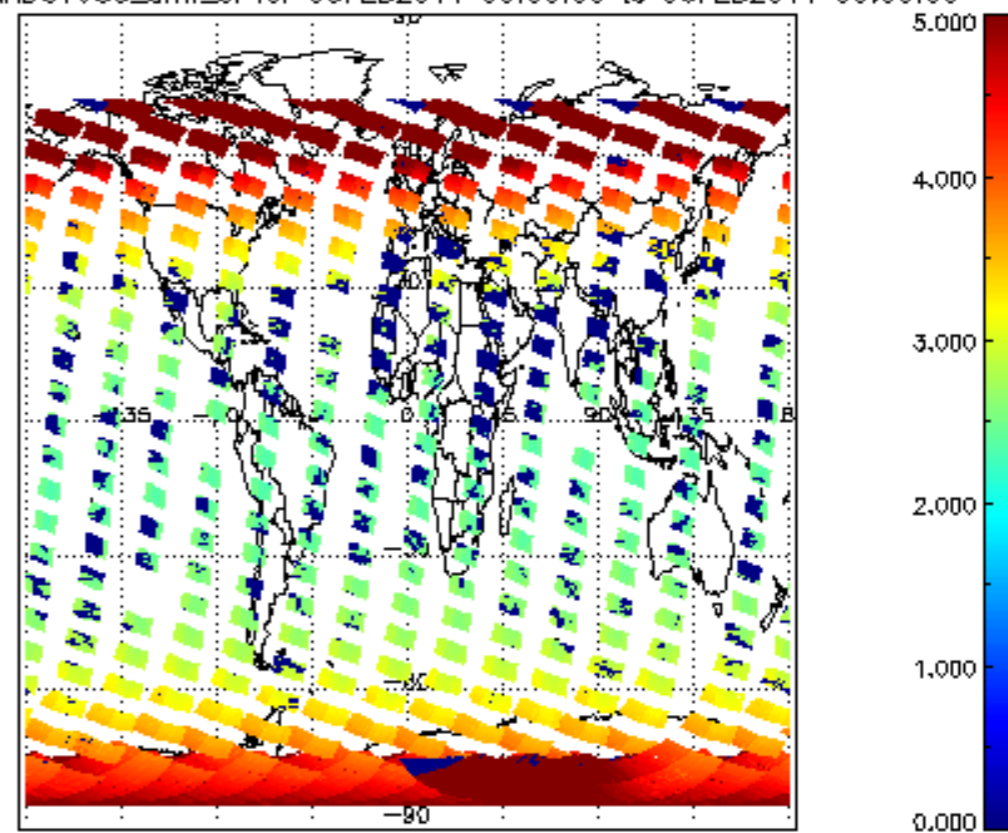
SCIOL2P_NADUV003_amf_cl for 05FEB2011 00:00:00 to 06FEB2011 00:00:00
