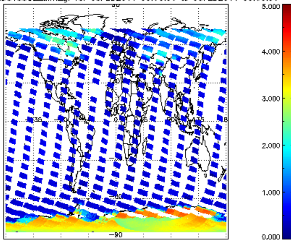
SCIOL2P_NADUV5S02_amf_gr for 05FEB2011 00:00:00 to 06FEB2011 00:00:00
