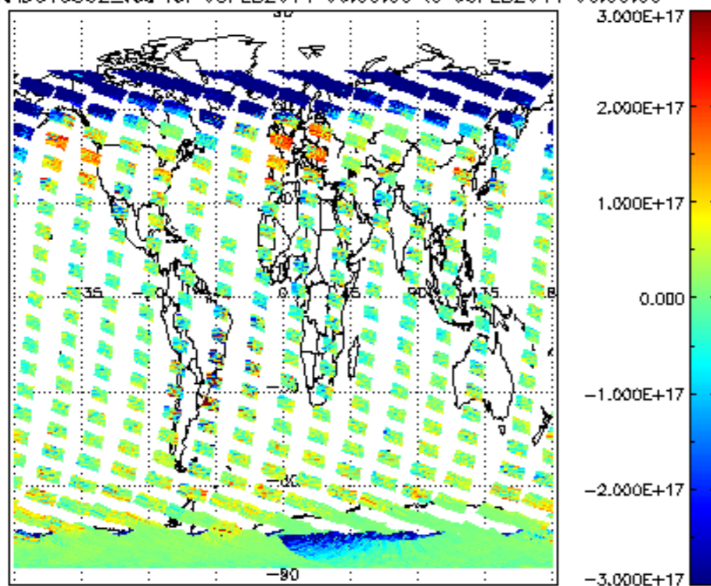
SCIOL2P_NADUV5S02_vcd for 05FEB2011 00:00:00 to 06FEB2011 00:00:00
