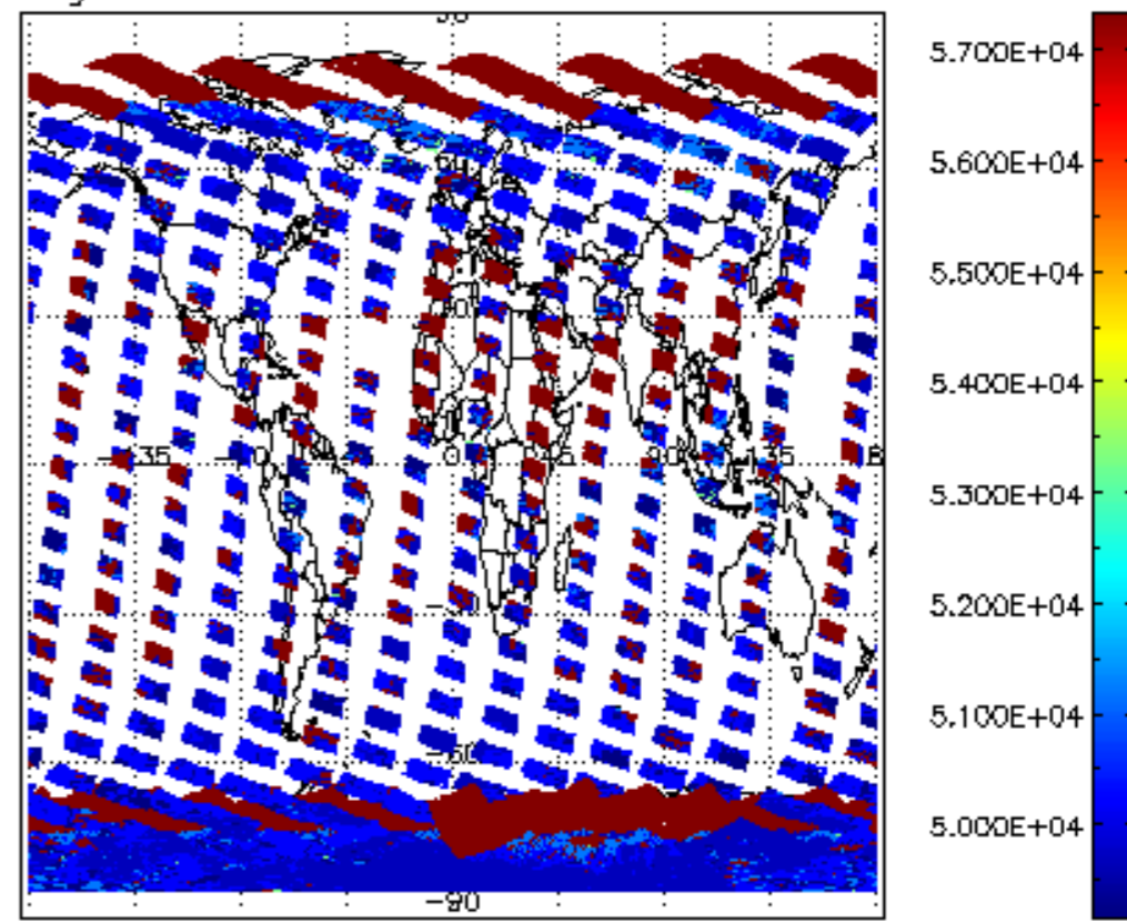
cloud_flags for 05FEB2011 00:00:00 to 06FEB2011 00:00:00
