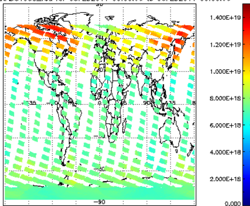
SCIOL2P_NADUV003_vcd for 05FEB2011 00:00:00 to 06FEB2011 00:00:00
