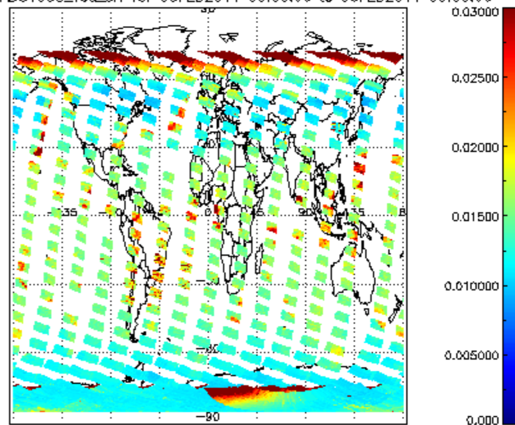
SCIOL2P_NADUV003_vcd_err for 05FEB2011 00:00:00 to 06FEB2011 00:00:00
