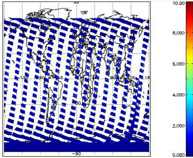
SCIOL2P_NADUV3BRO_vcd_err for 04FEB2011 00:00:00 to 05FEB2011 00:00:00
