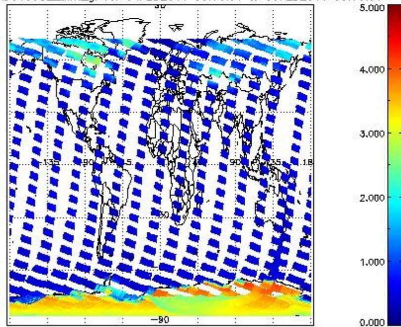
SCIOL2P_NADUV5S02_amf_gr for 04FEB2011 00:00:00 to 05FEB2011 00:00:00
