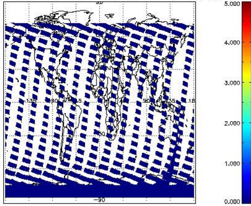
SCIOL2P_NADUV7S02_amf_cl for 04FEB2011 00:00:00 to 05FEB2011 00:00:00
