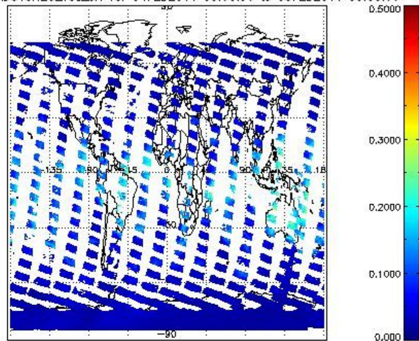
SCIOL2P_NADUV8H2O_vcd_err for 04FEB2011 00:00:00 to 05FEB2011 00:00:00
