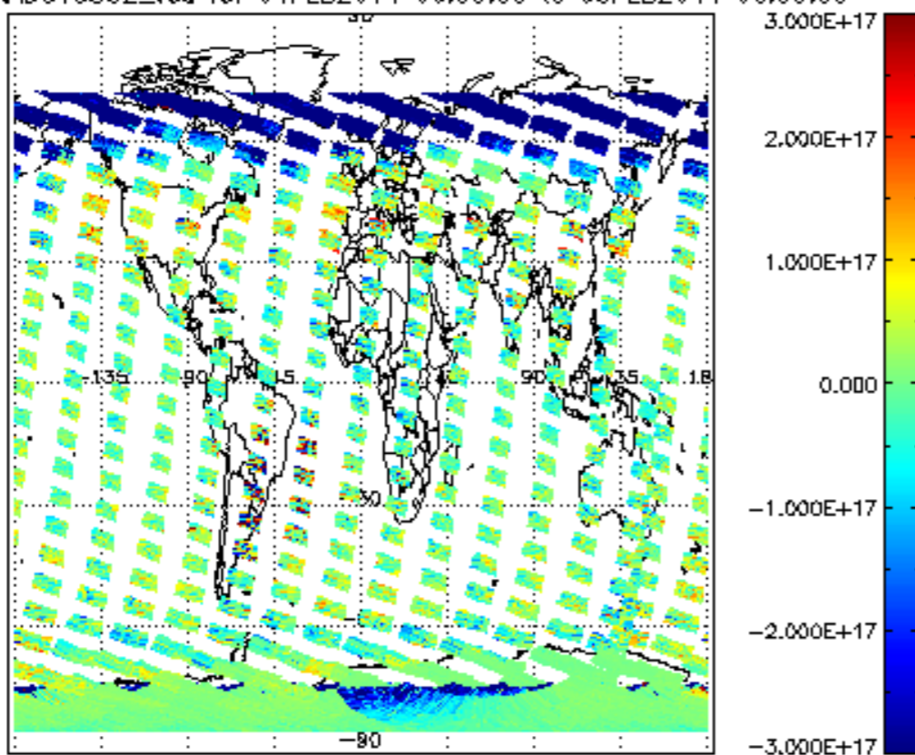
SCIOL2P_NADUV5S02_vcd for 04FEB2011 00:00:00 to 05FEB2011 00:00:00
