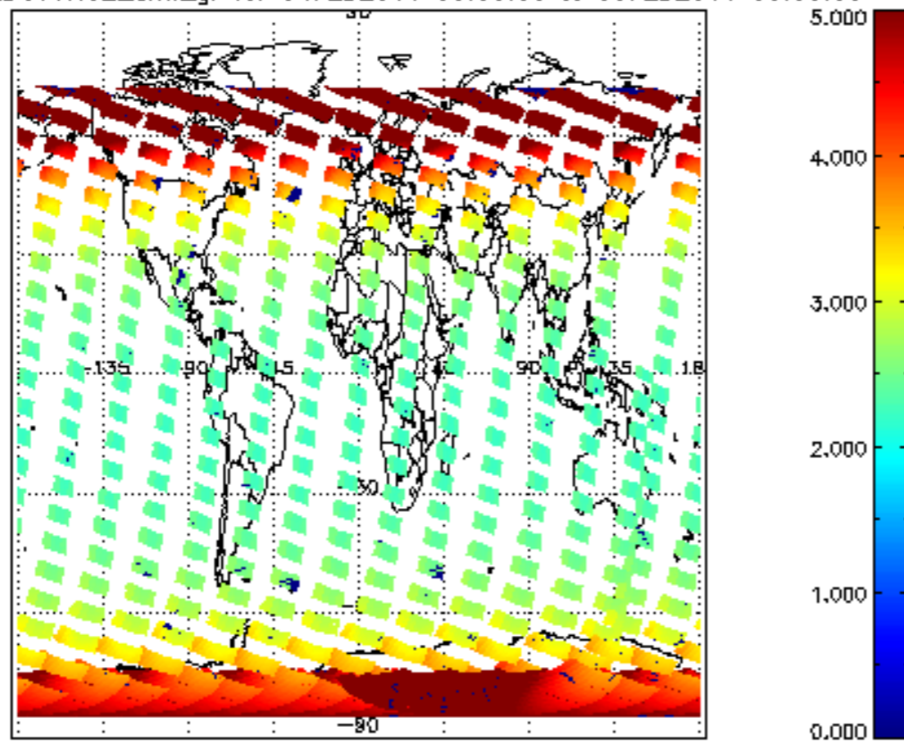
SCIOL2P_NADUV1N02_amf_gr for 04FEB2011 00:00:00 to 05FEB2011 00:00:00
