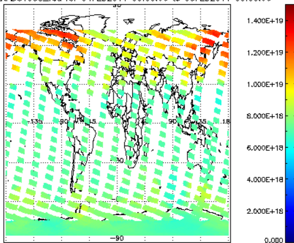
SCIOL2P_NADUV003_vcd for 04FEB2011 00:00:00 to 05FEB2011 00:00:00
