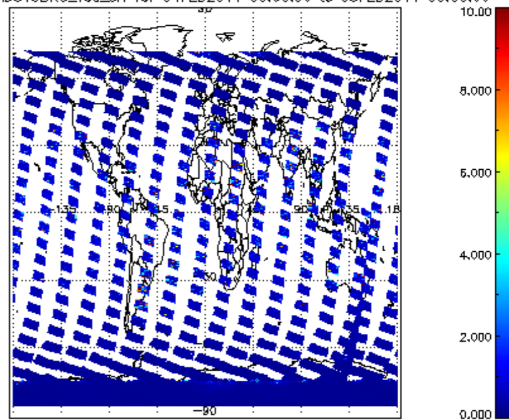
SCIOL2P_NADUV3BRO_vcd_err for 04FEB2011 00:00:00 to 05FEB2011 00:00:00
