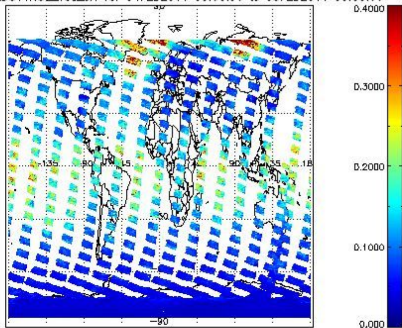
SCIOL2P_NADUV1N02_vcd_err for 04FEB2011 00:00:00 to 05FEB2011 00:00:00
