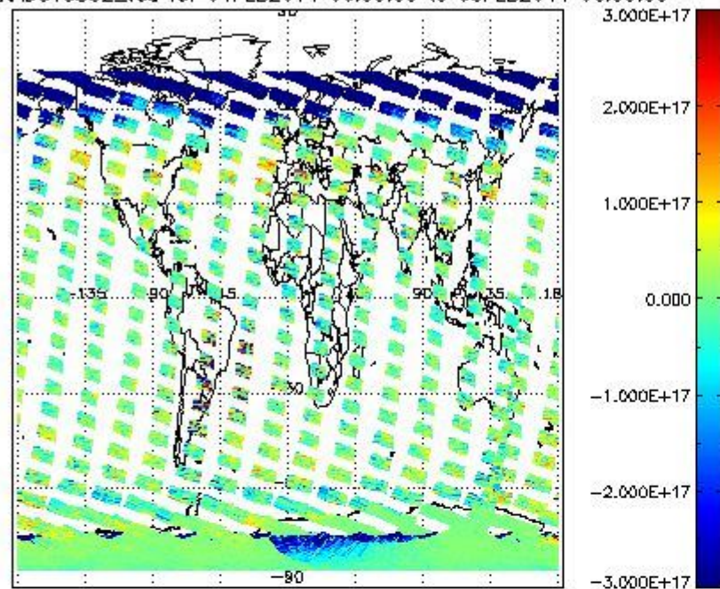
SCIOL2P_NADUV5S02_vcd for 04FEB2011 00:00:00 to 05FEB2011 00:00:00
