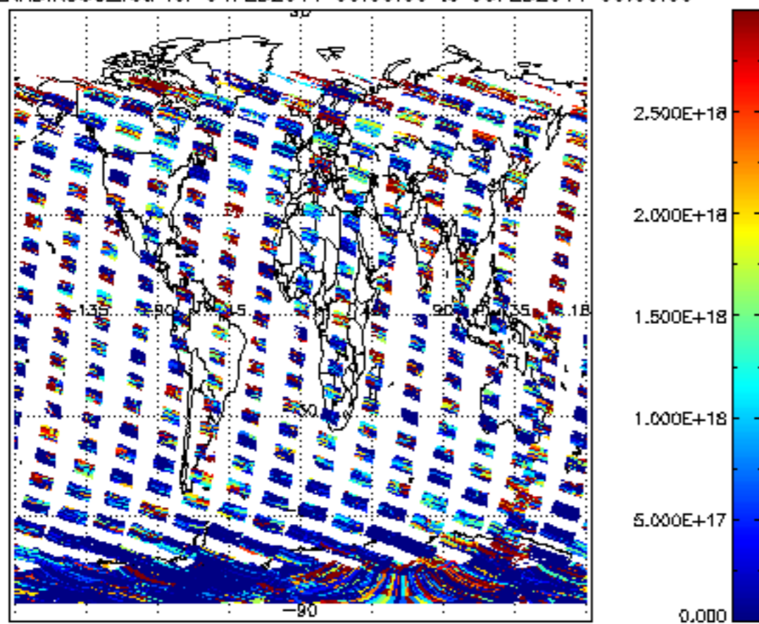
SCIOL2P_NADIR3CO_vcd for 04FEB2011 00:00:00 to 05FEB2011 00:00:00
