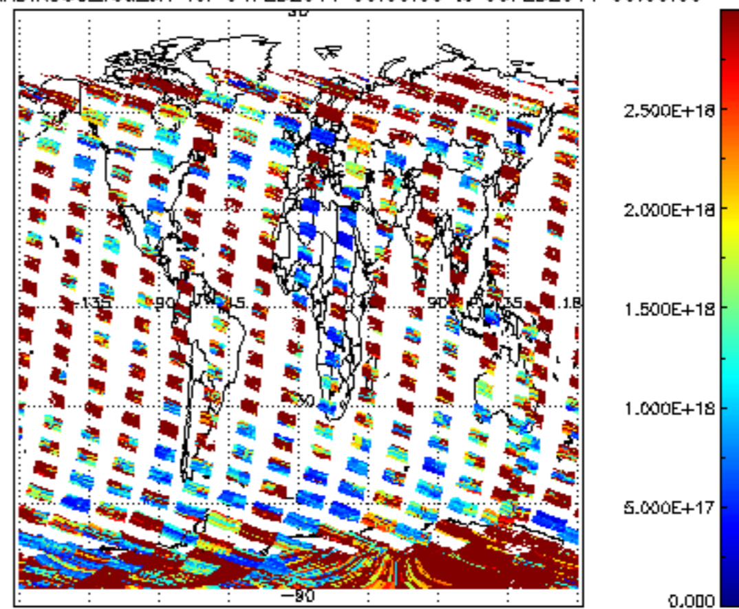
SCIOL2P_NADIR3CO_vcd_err for 04FEB2011 00:00:00 to 05FEB2011 00:00:00
