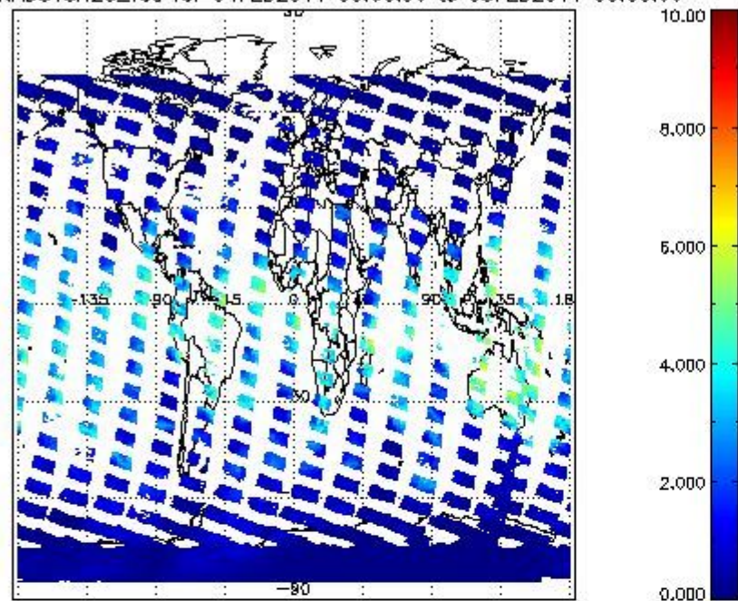
SCIOL2P_NADUV8H2O_vcd for 04FEB2011 00:00:00 to 05FEB2011 00:00:00
