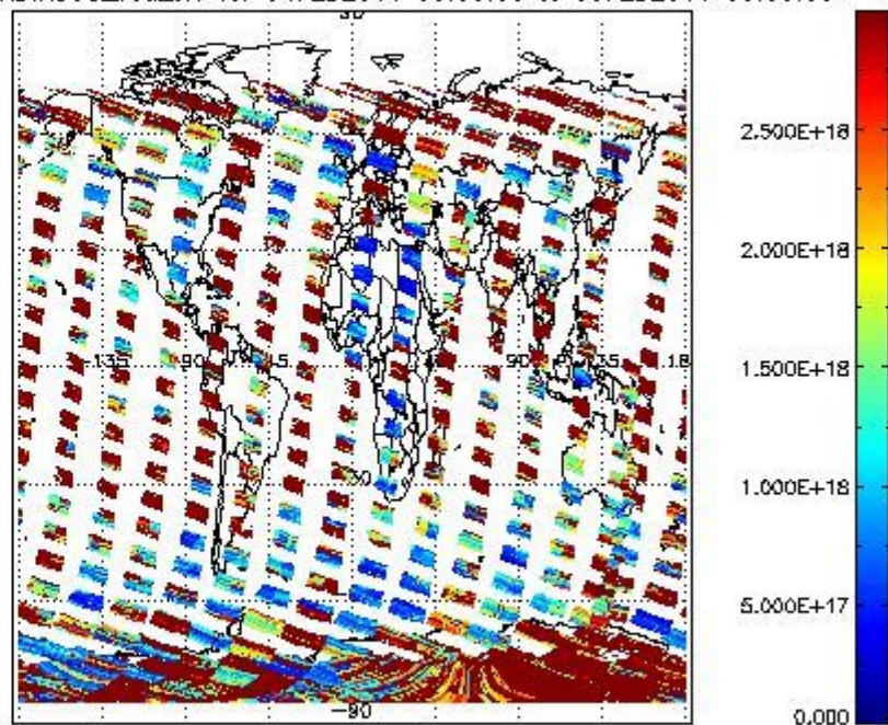
SCIDL2P_NADIR3CO_vcd_err for 04FEB2011 00:00:00 to 05FEB2011 00:00:00
