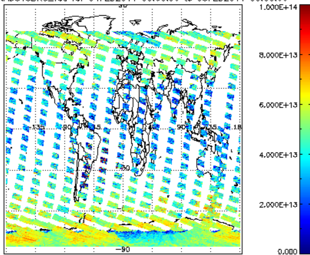
SCIOL2P_NADUV3BRO_vcd for 04FEB2011 00:00:00 to 05FEB2011 00:00:00
