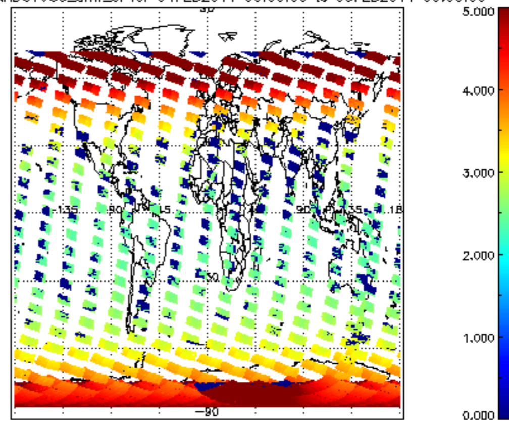
SCIOL2P_NADUV003_amf_cl for 04FEB2011 00:00:00 to 05FEB2011 00:00:00
