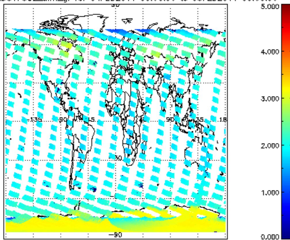
SCIOL2P_NADUV7S02_amf_gr for 04FEB2011 00:00:00 to 05FEB2011 00:00:00
