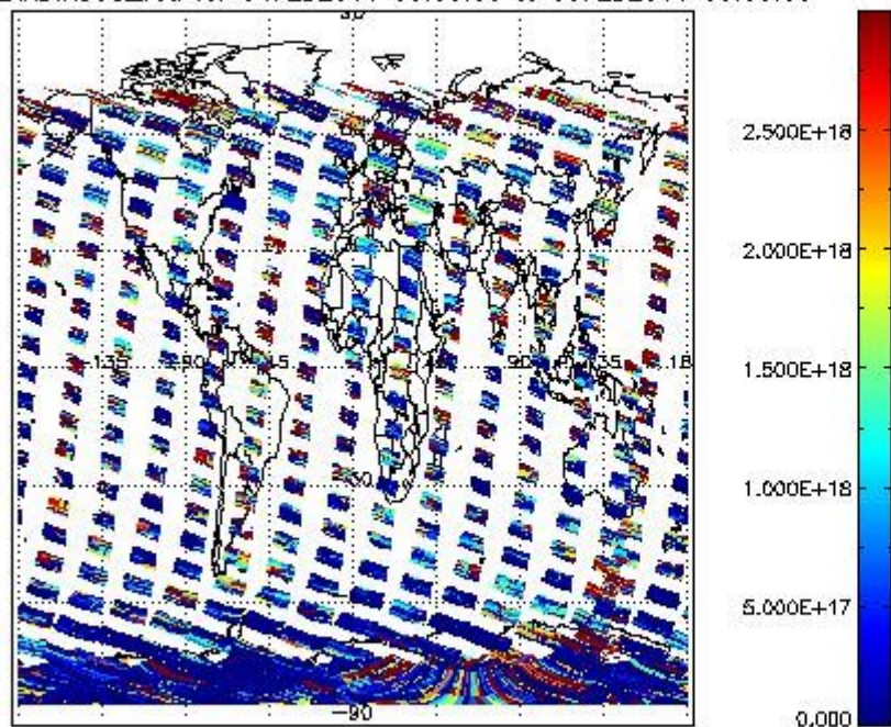
SCIDL2P_NADIR3CO_vcd for 04FEB2011 00:00:00 to 05FEB2011 00:00:00
