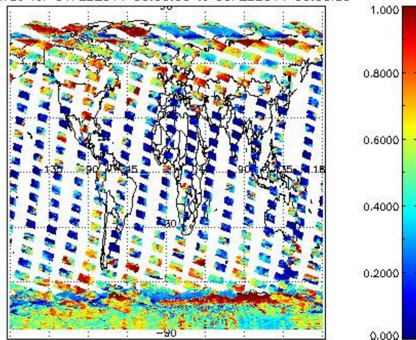
cL_frac for 04FEB2011 00:00:00 to 05FEB2011 00:00:00
