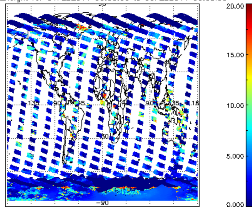
cI_top_height for 04FEB2011 00:00:00 to 05FEB2011 00:00:00
