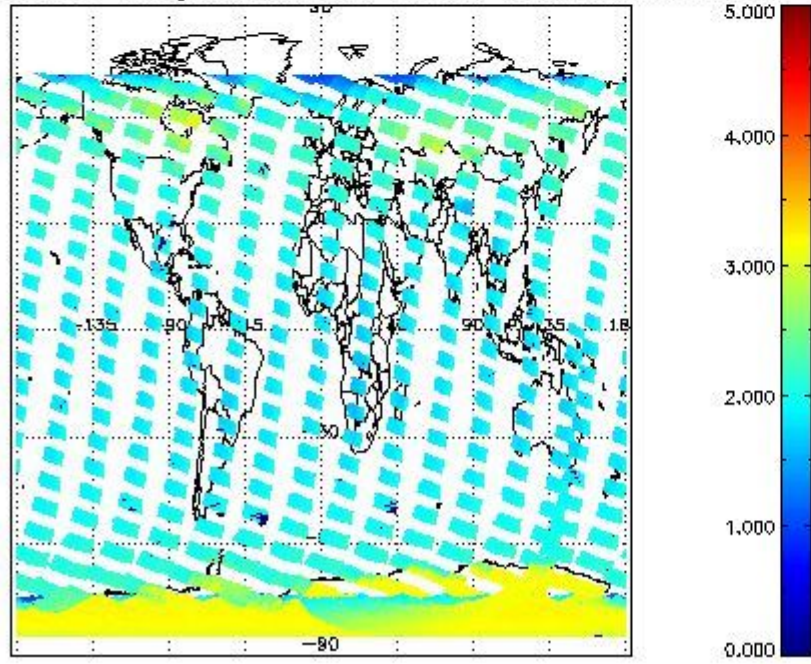
SCIOL2P_NADUV7S02_amf_gr for 04FEB2011 00:00:00 to 05FEB2011 00:00:00
