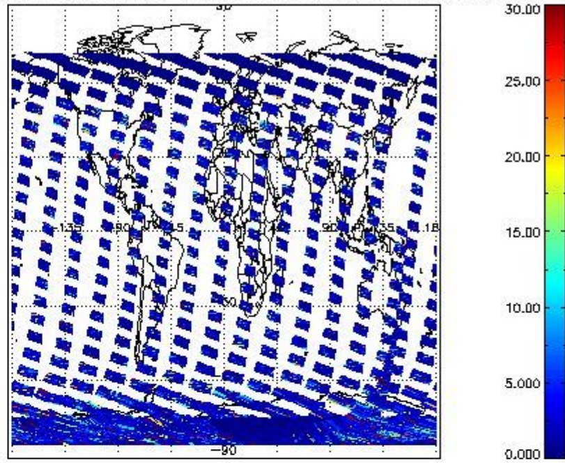
SCIOL2P_NADUV7S02_vcd_err for 04FEB2011 00:00:00 to 05FEB2011 00:00:00
