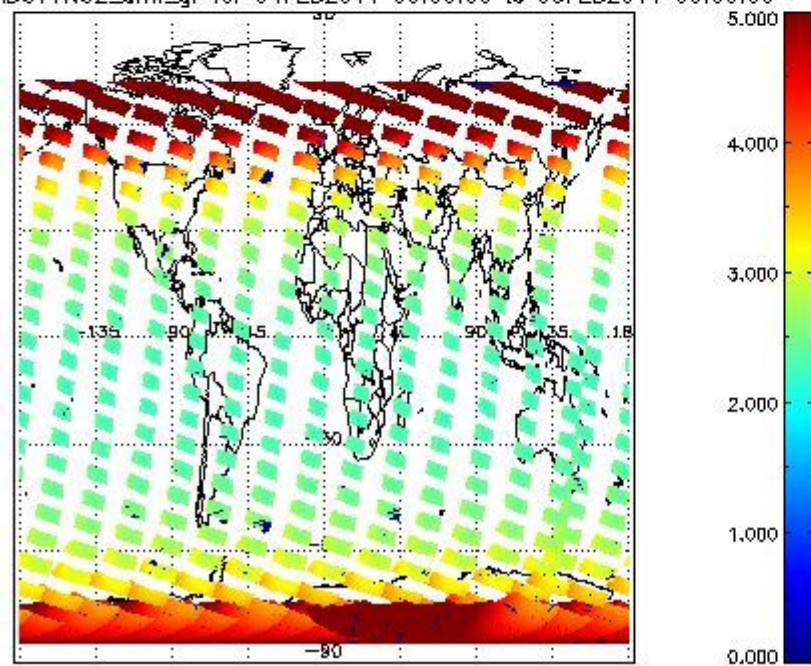
SCIOL2P_NADUV1N02_amf_gr for 04FEB2011 00:00:00 to 05FEB2011 00:00:00
