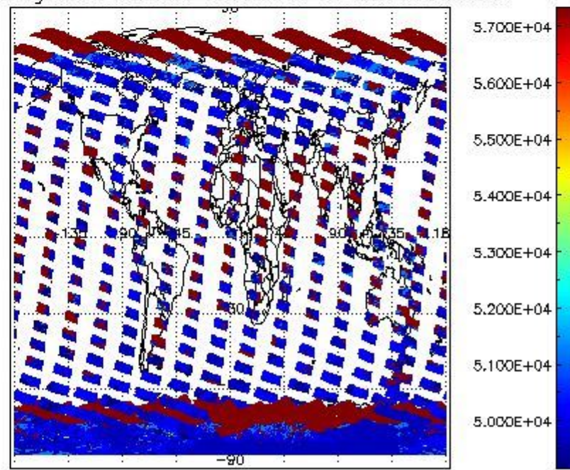
cloud_flags for 04FEB2011 00:00:00 to 05FEB2011 00:00:00
