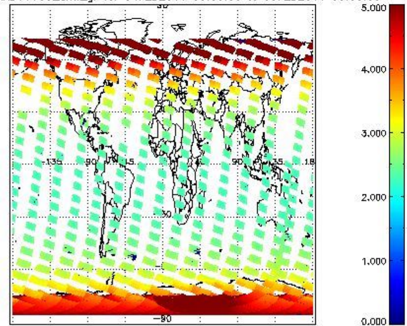
SCIOL2P_NADUV003_amf_gr for 04FEB2011 00:00:00 to 05FEB2011 00:00:00
