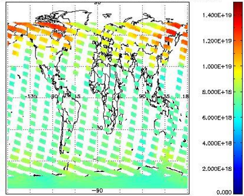
SCIOL2P_NADUV003_vcd for 04FEB2011 00:00:00 to 05FEB2011 00:00:00
