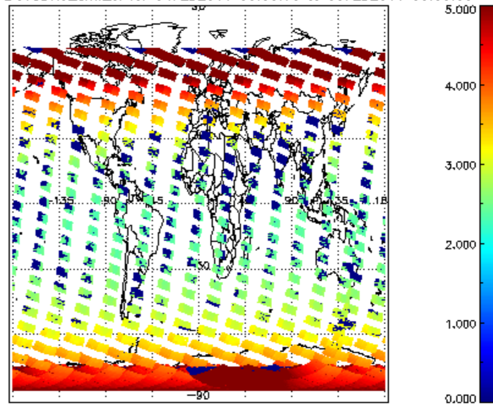
SCIOL2P_NADUV3BRO_amf_cl for 04FEB2011 00:00:00 to 05FEB2011 00:00:00
