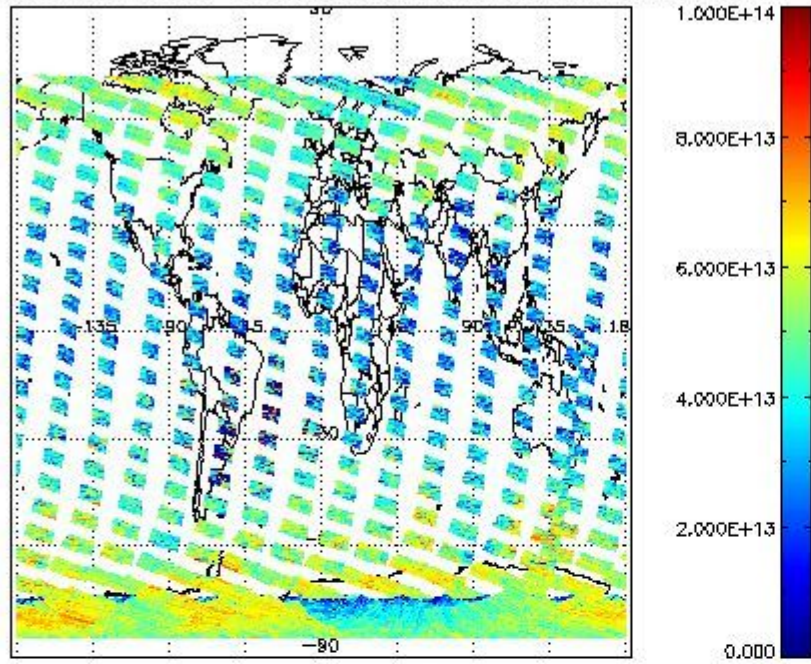
SCIOL2P_NADUV3BRO_vcd for 04FEB2011 00:00:00 to 05FEB2011 00:00:00
