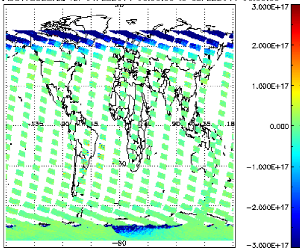
SCIOL2P_NADUV7S02_vcd for 04FEB2011 00:00:00 to 05FEB2011 00:00:00
