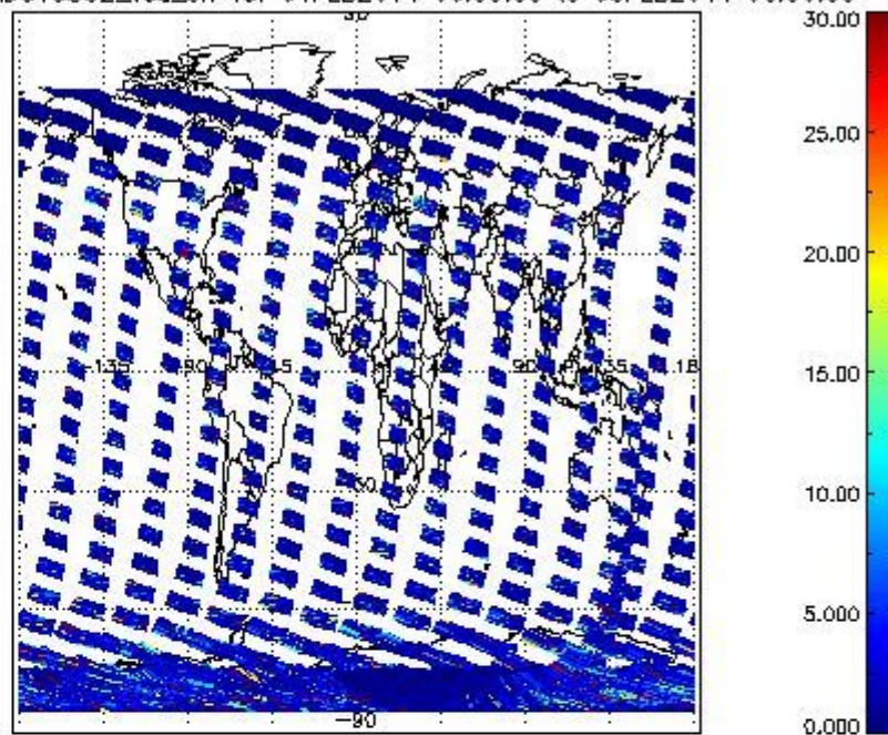
SCIOL2P_NADUV5S02_vcd_err for 04FEB2011 00:00:00 to 05FEB2011 00:00:00
