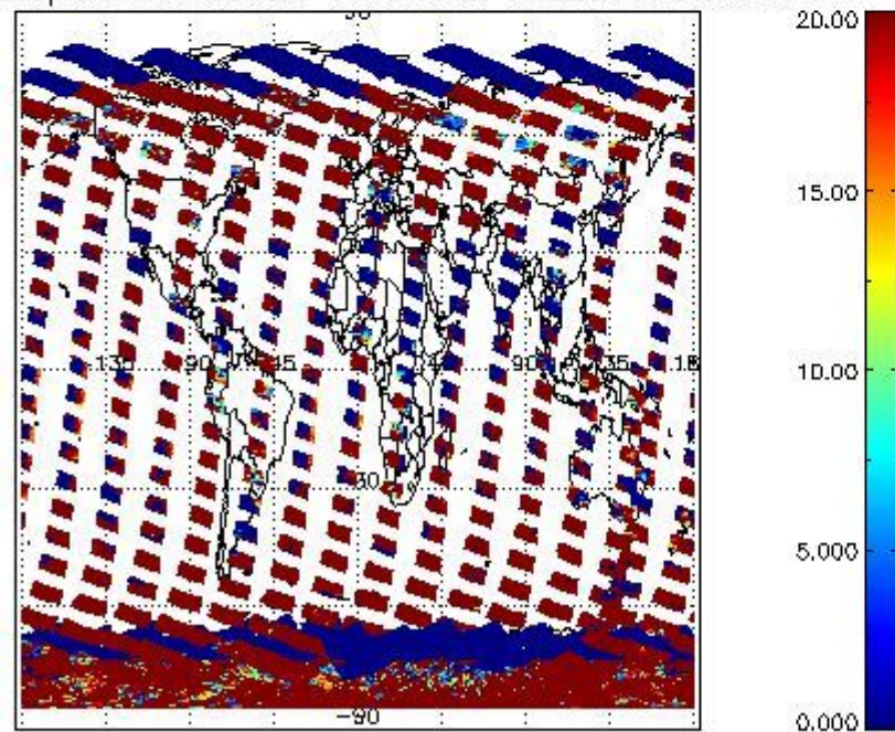
cL_opt_depth for 04FEB2011 00:00:00 to 05FEB2011 00:00:00
