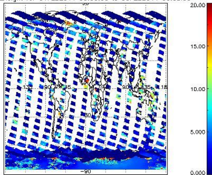
cL_top_height for 04FEB2011 00:00:00 to 05FEB2011 00:00:00
