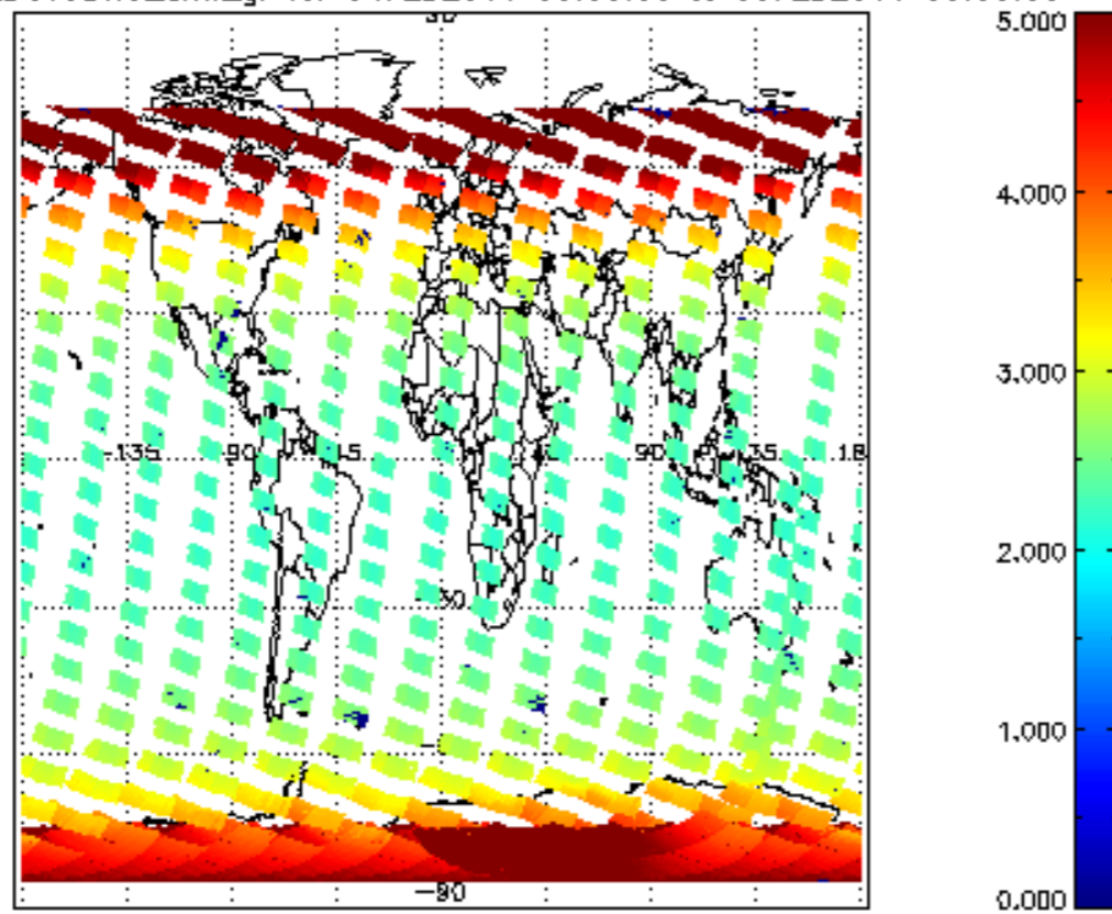
SCIOL2P_NADUV3BRO_amf_gr for 04FEB2011 00:00:00 to 05FEB2011 00:00:00
