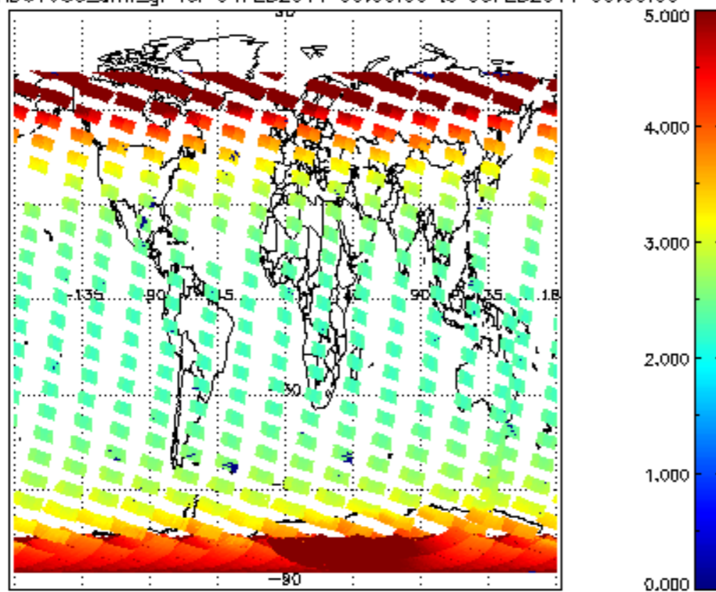
SCIOL2P_NADUV003_amf_gr for 04FEB2011 00:00:00 to 05FEB2011 00:00:00
