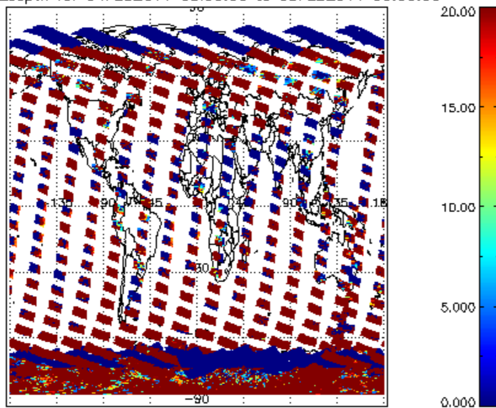
cI_opt_depth for 04FEB2011 00:00:00 to 05FEB2011 00:00:00
