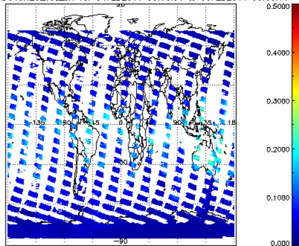
SCIOL2P_NADUV8H2O_vcd_err for 04FEB2011 00:00:00 to 05FEB2011 00:00:00
