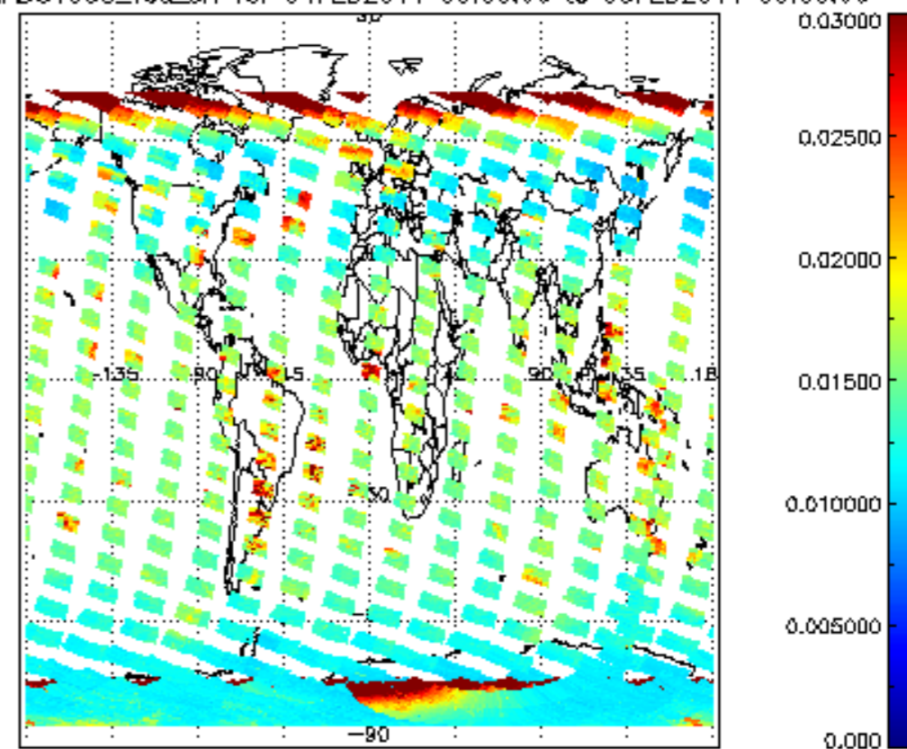
SCIOL2P_NADUV003_vcd_err for 04FEB2011 00:00:00 to 05FEB2011 00:00:00
