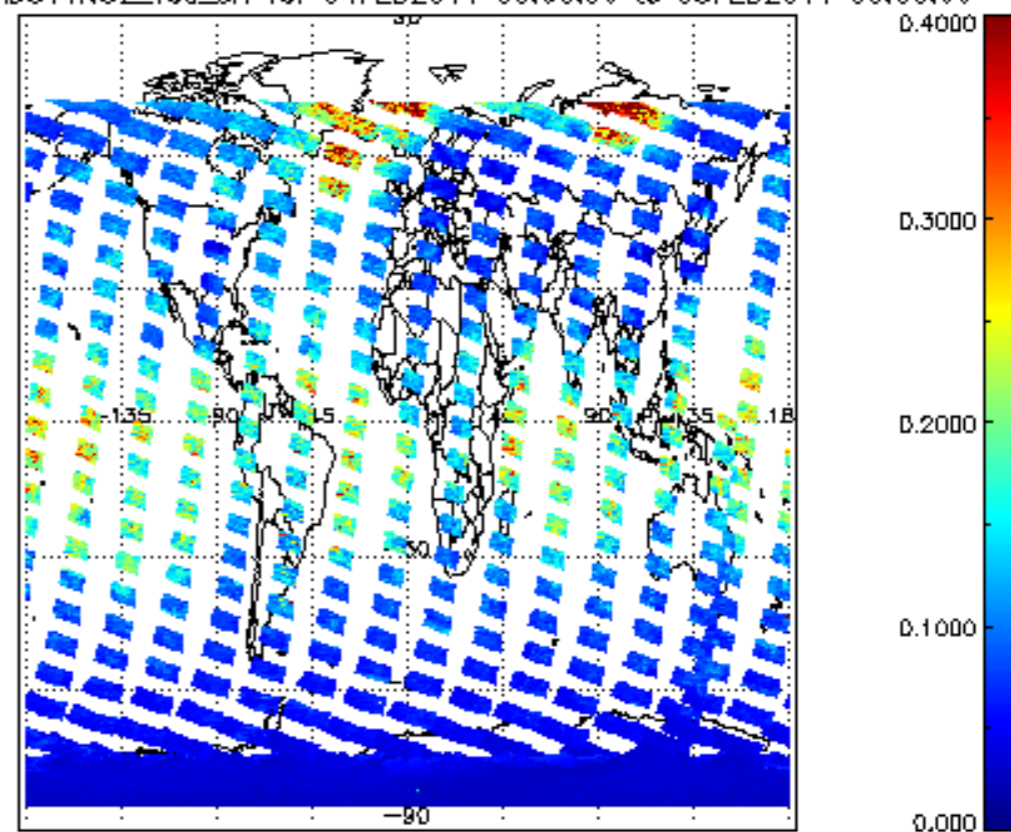
SCIOL2P_NADUV1N02_vcd_err for 04FEB2011 00:00:00 to 05FEB2011 00:00:00
