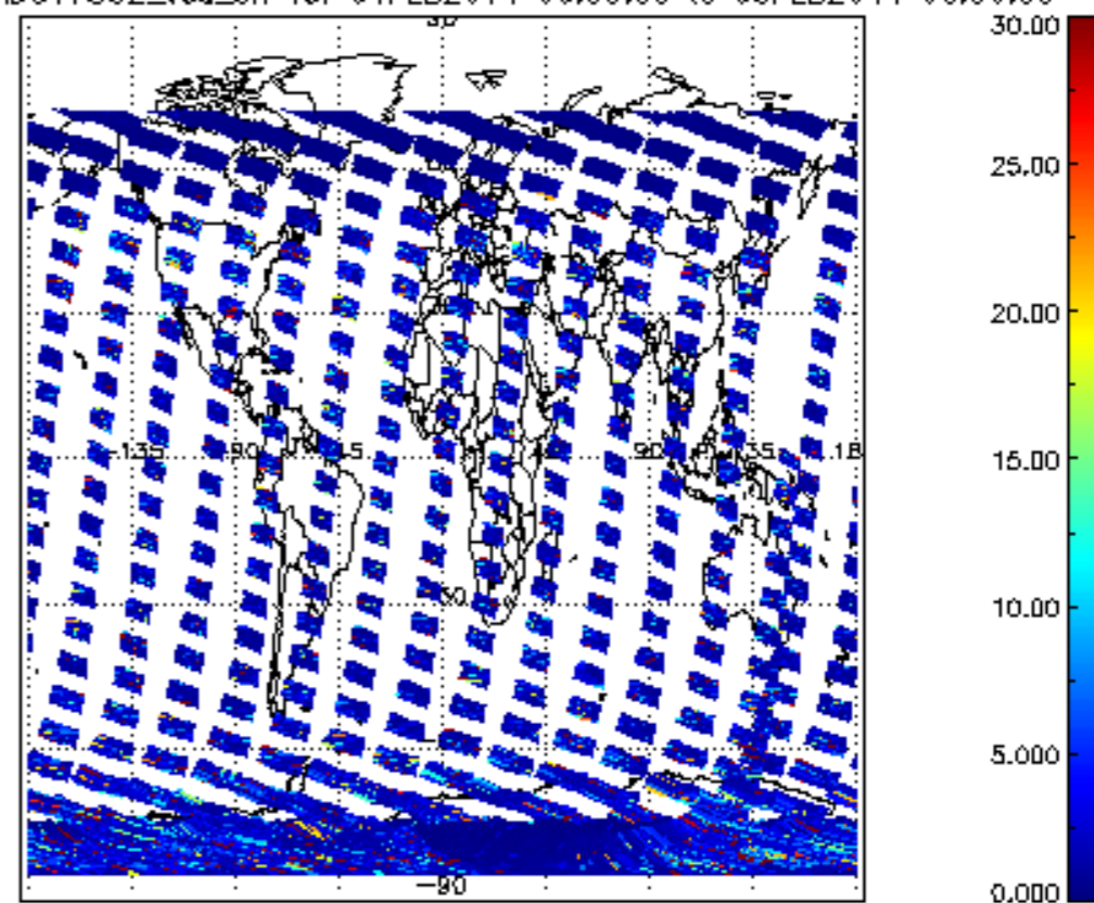
SCIOL2P_NADUV7S02_vcd_err for 04FEB2011 00:00:00 to 05FEB2011 00:00:00
