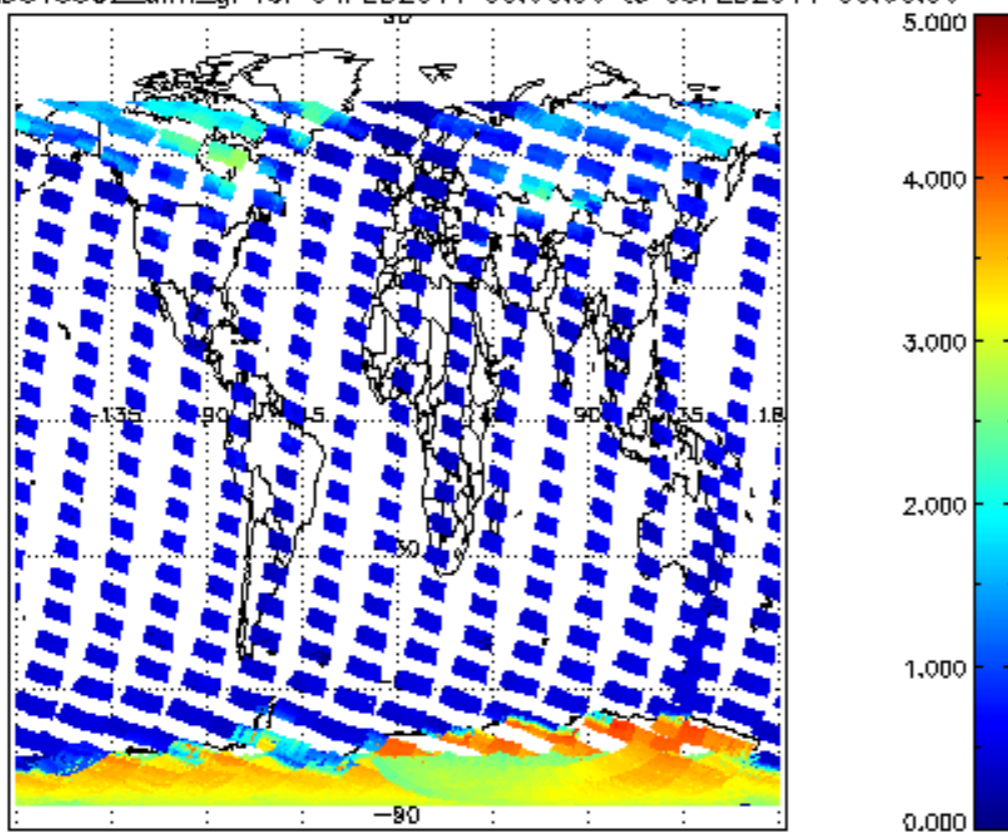
SCIOL2P_NADUV5S02_amf_gr for 04FEB2011 00:00:00 to 05FEB2011 00:00:00
