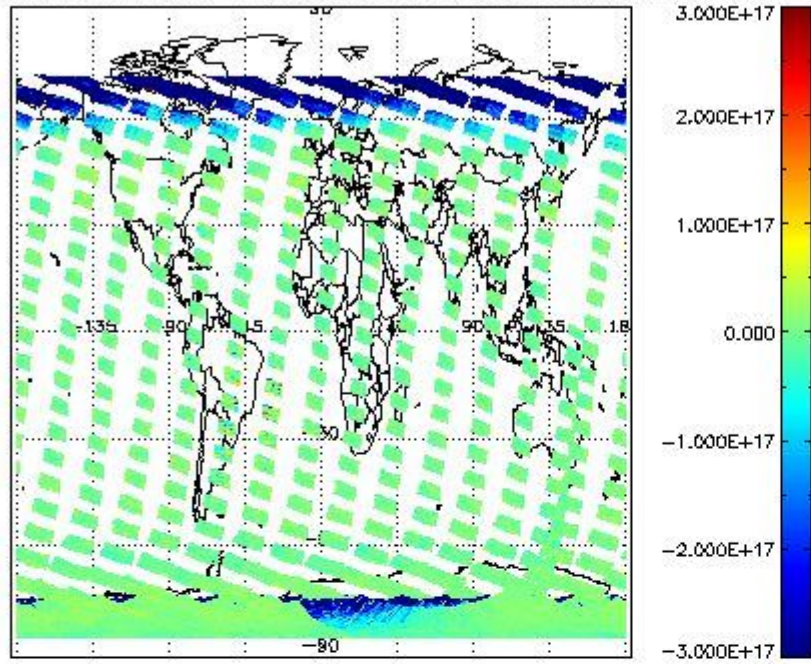
SCIOL2P_NADUV7S02_vcd for 04FEB2011 00:00:00 to 05FEB2011 00:00:00
