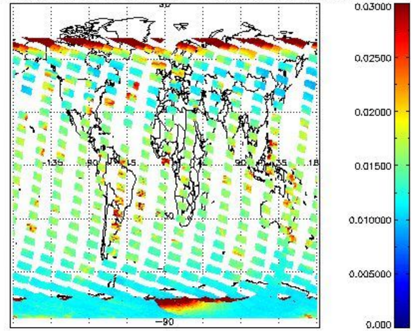
SCIOL2P_NADUV003_vcd_err for 04FEB2011 00:00:00 to 05FEB2011 00:00:00
