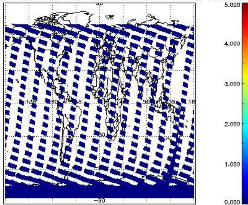
SCIOL2P_NADUV5S02_amf_cl for 04FEB2011 00:00:00 to 05FEB2011 00:00:00
