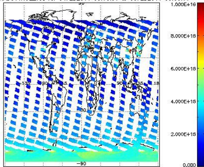
SCIOL2P_NADUV1N02_vcd for 04FEB2011 00:00:00 to 05FEB2011 00:00:00
