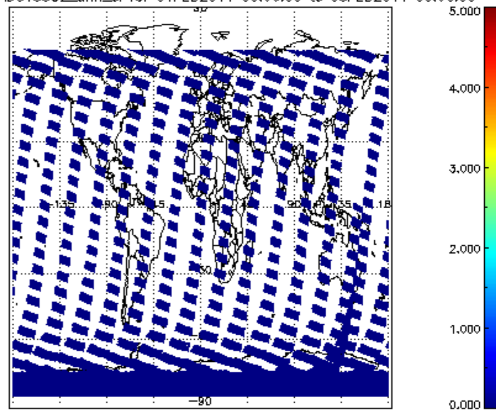
SCIOL2P_NADUV5S02_amf_cl for 04FEB2011 00:00:00 to 05FEB2011 00:00:00
