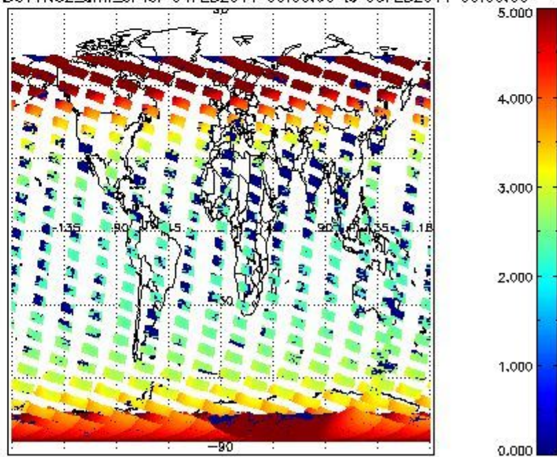
SCIOL2P_NADUV1N02_amf_cl for 04FEB2011 00:00:00 to 05FEB2011 00:00:00
