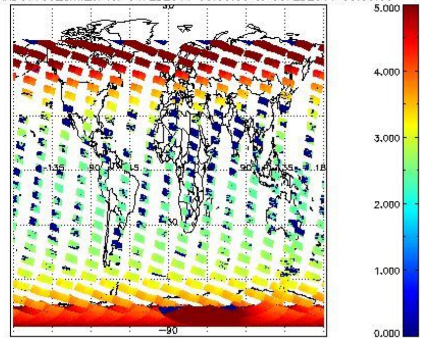
SCIOL2P_NADUV003_amf_cl for 04FEB2011 00:00:00 to 05FEB2011 00:00:00
