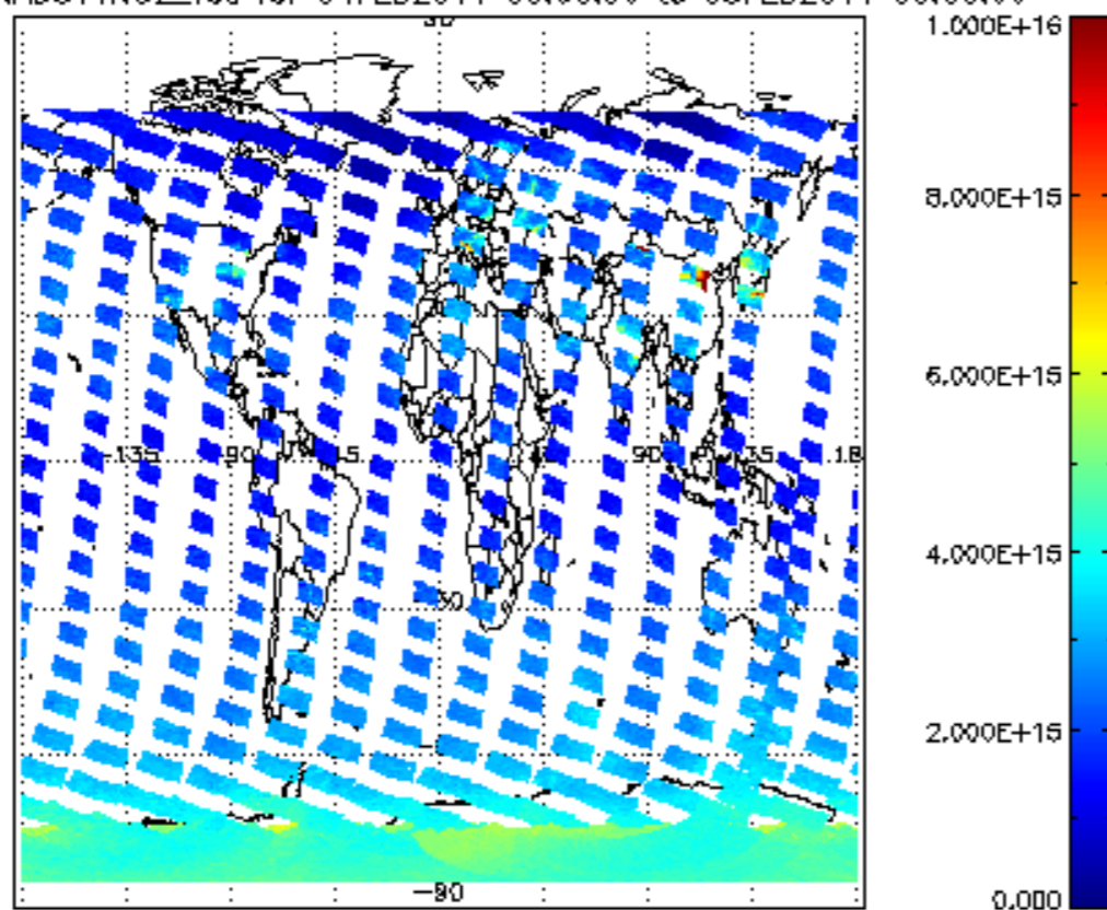
SCIOL2P_NADUV1N02_vcd for 04FEB2011 00:00:00 to 05FEB2011 00:00:00
