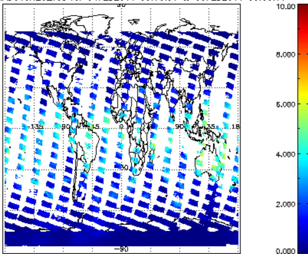
SCIOL2P_NADUV8H2O_vcd for 04FEB2011 00:00:00 to 05FEB2011 00:00:00
