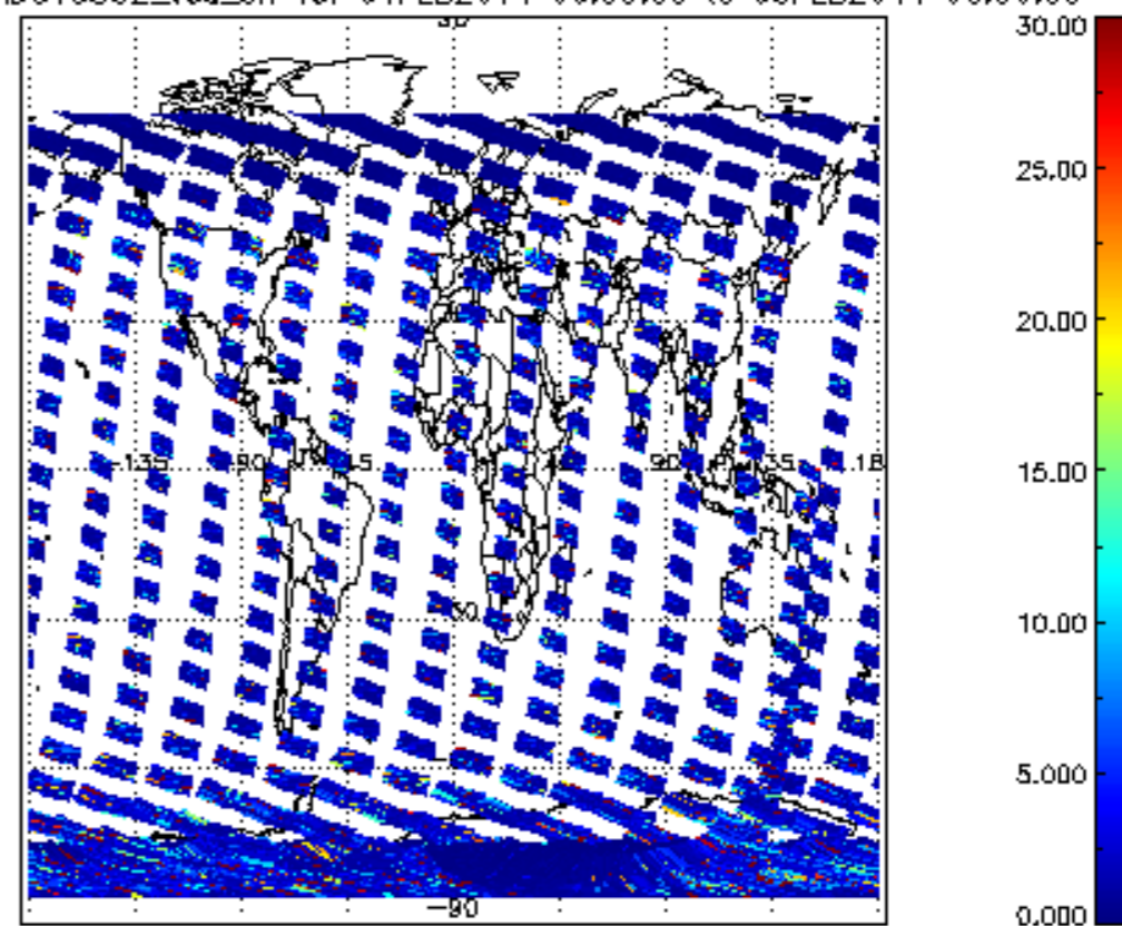
SCIOL2P_NADUV5S02_vcd_err for 04FEB2011 00:00:00 to 05FEB2011 00:00:00
