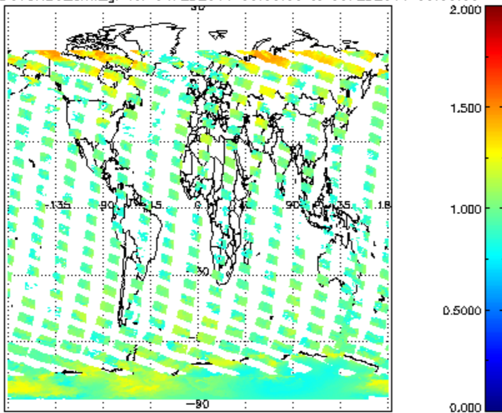
SCIOL2P_NADUV8H2O_amf_gr for 04FEB2011 00:00:00 to 05FEB2011 00:00:00
