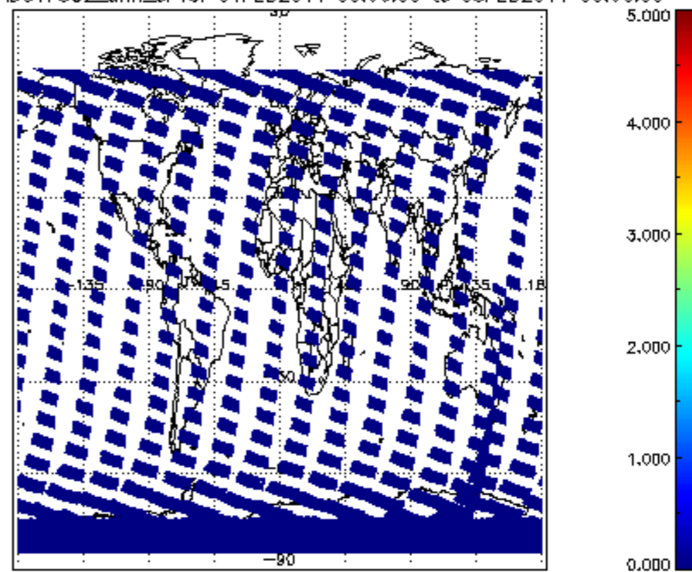
SCIOL2P_NADUV7S02_amf_cl for 04FEB2011 00:00:00 to 05FEB2011 00:00:00
