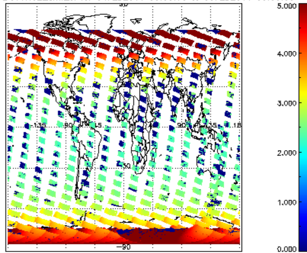
SCIOL2P_NADUV1N02_amf_cl for 04FEB2011 00:00:00 to 05FEB2011 00:00:00
