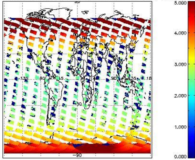
SCIOL2P_NADUV3BRO_amf_cl for 04FEB2011 00:00:00 to 05FEB2011 00:00:00
