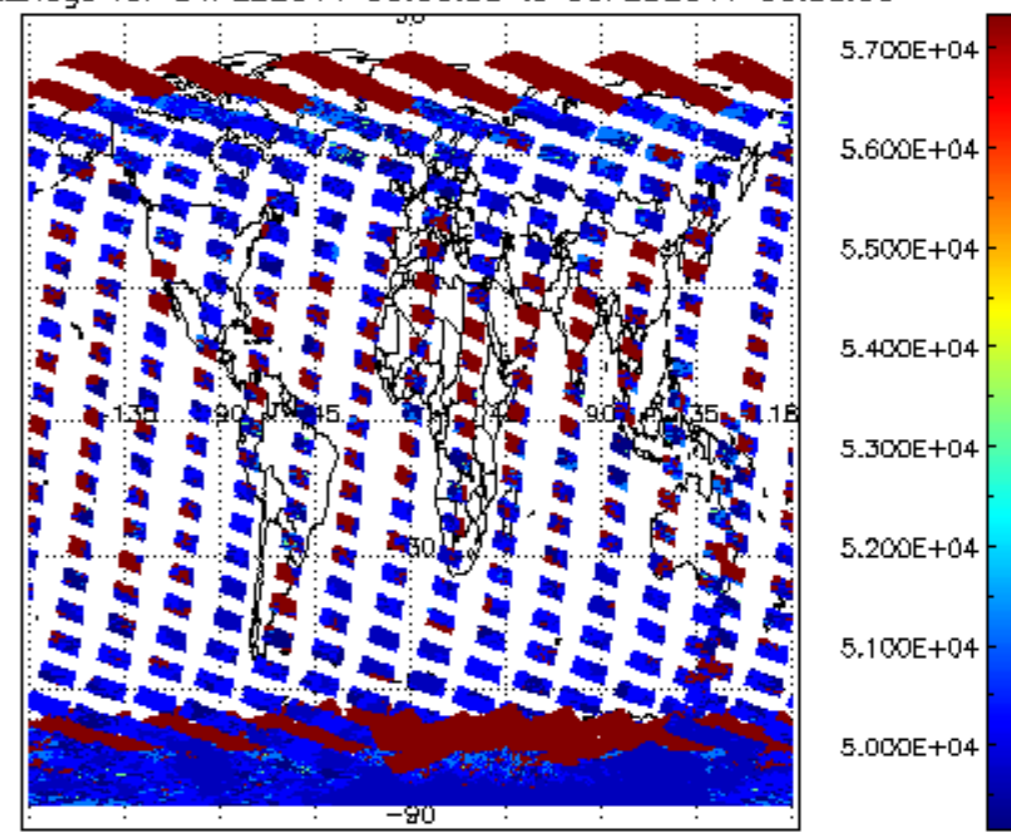
cloud_flags for 04FEB2011 00:00:00 to 05FEB2011 00:00:00
