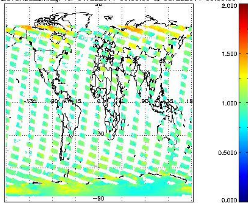
SCIOL2P_NADUV8H2O_amf_gr for 04FEB2011 00:00:00 to 05FEB2011 00:00:00
