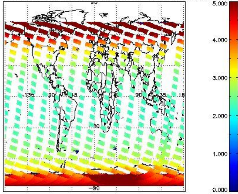
SCIOL2P_NADUV3BRO_amf_gr for 04FEB2011 00:00:00 to 05FEB2011 00:00:00
