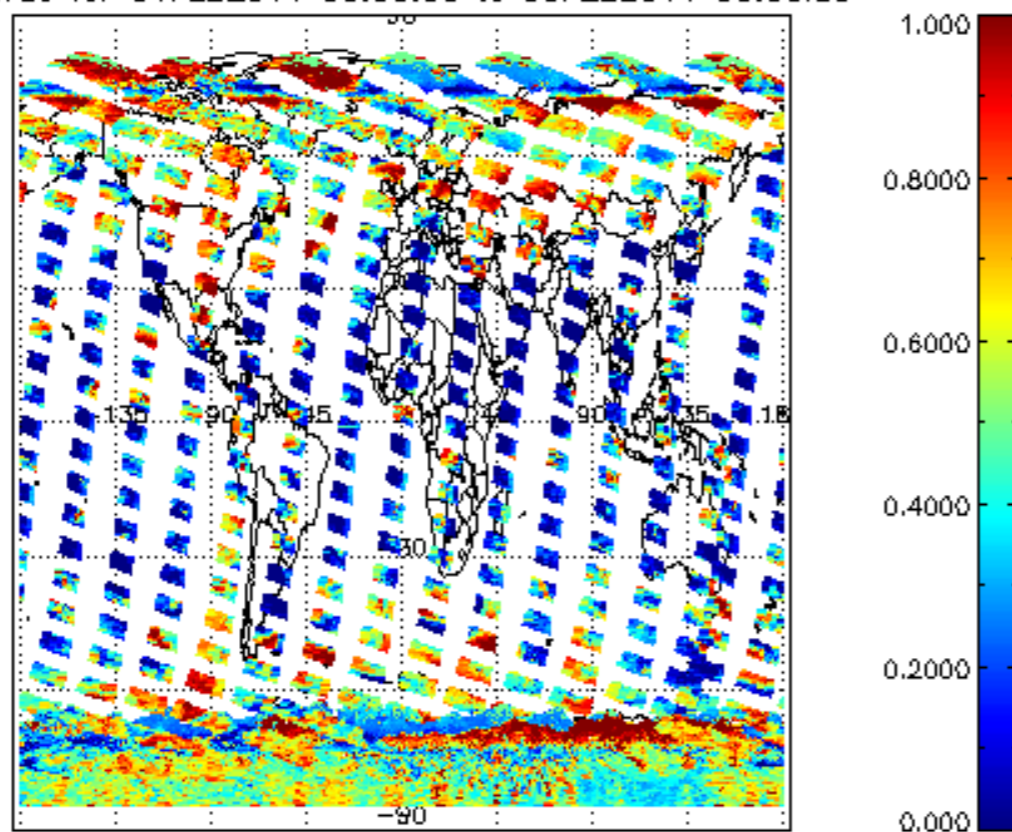
cI_frac for 04FEB2011 00:00:00 to 05FEB2011 00:00:00
