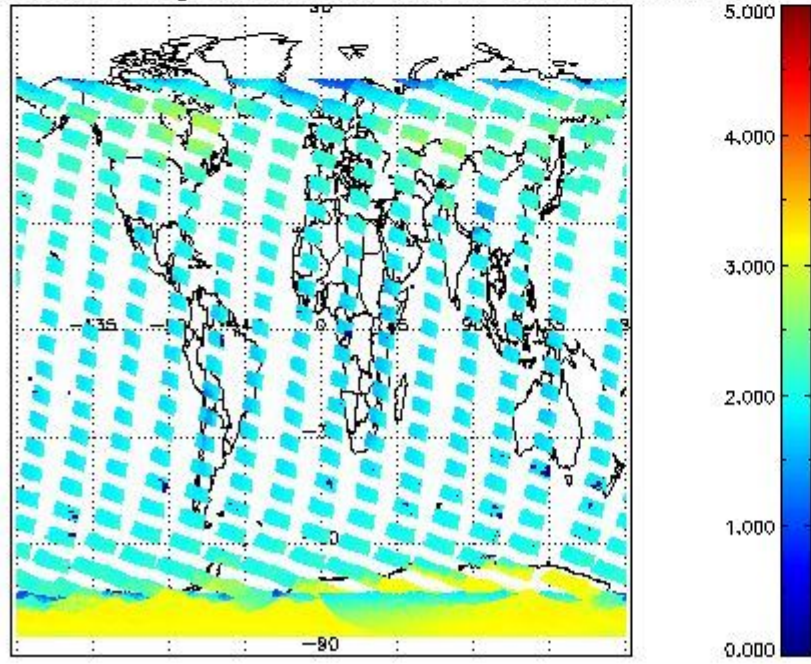
SCIOL2P_NADUV7S02_amf_gr for 31JAN2011 00:00:00 to 01FEB2011 00:00:00
