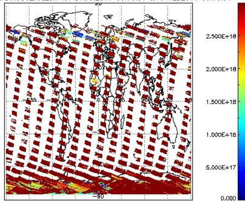
SCIOL2P_NADIR3CO_vcd_err for 31JAN2011 00:00:00 to 01FEB2011 00:00:00
