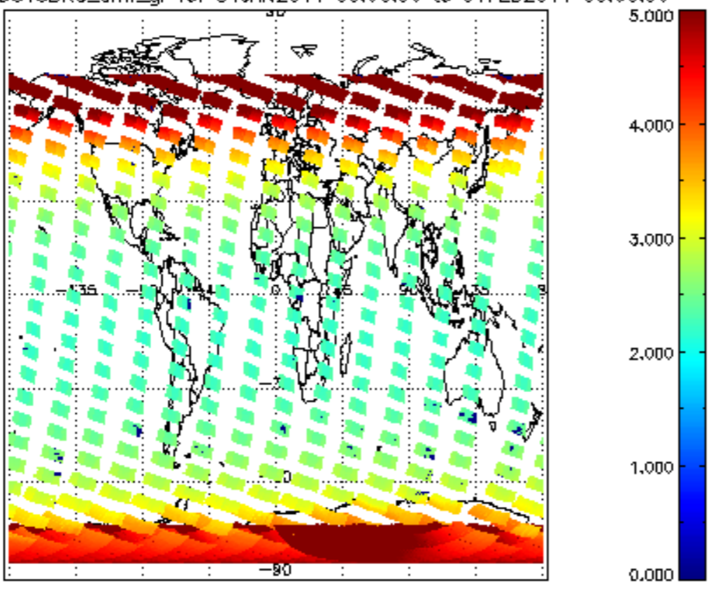
SCIOL2P_NADUV3BRO_amf_gr for 31JAN2011 00:00:00 to 01FEB2011 00:00:00
