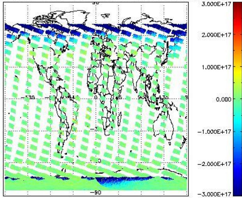
SCIOL2P_NADUV7S02_vcd for 31JAN2011 00:00:00 to 01FEB2011 00:00:00
