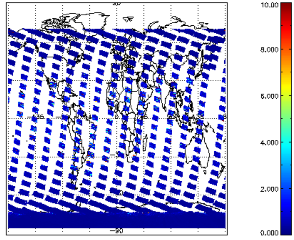
SCIOL2P_NADUV3BRO_vcd_err for 31JAN2011 00:00:00 to 01FEB2011 00:00:00
