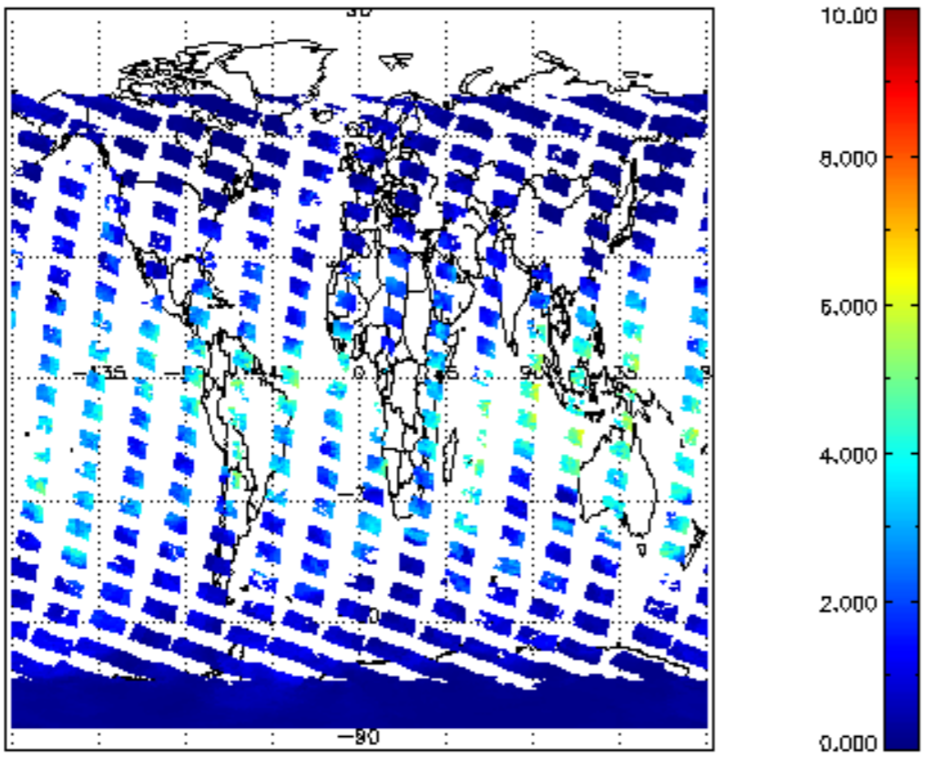
SCIOL2P_NADUV8H20_vcd for 31JAN2011 00:00:00 to 01FEB2011 00:00:00
