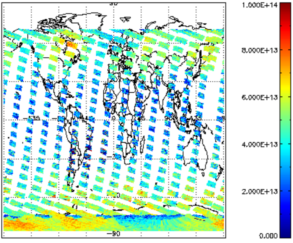
SCIOL2P_NADUV3BRO_vcd for 31JAN2011 00:00:00 to 01FEB2011 00:00:00
