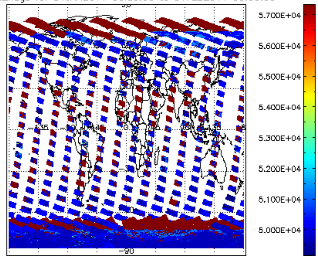
cloud_flags for 31JAN2011 00:00:00 to 01FEB2011 00:00:00
