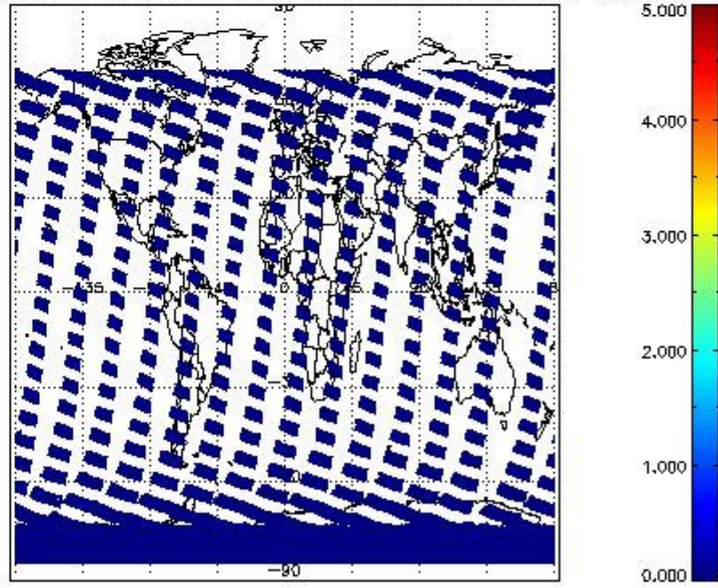
SCIOL2P_NADUV7S02_amf_cl for 31JAN2011 00:00:00 to 01FEB2011 00:00:00
