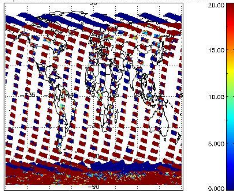
cL_top_depth for 31JAN2011 00:00:00 to 01FEB2011 00:00:00
