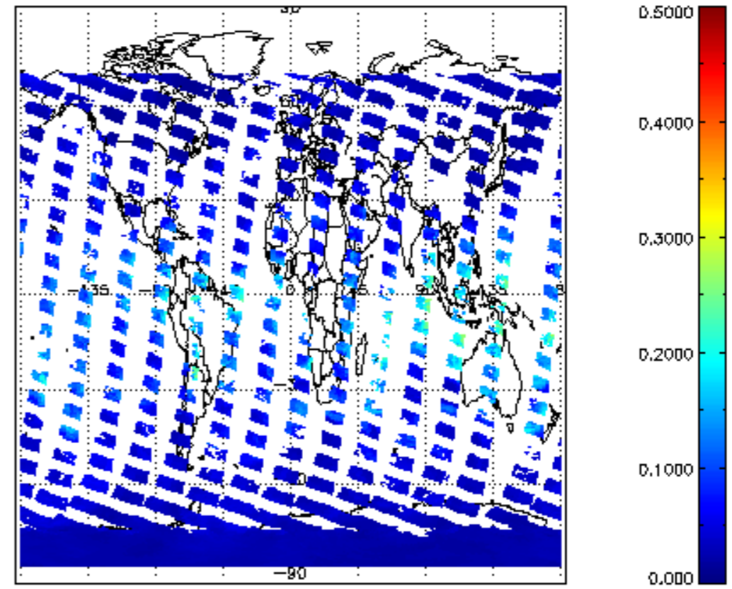
SCIOL2P_NADUV8H20_vcd_err for 31JAN2011 00:00:00 to 01FEB2011 00:00:00
