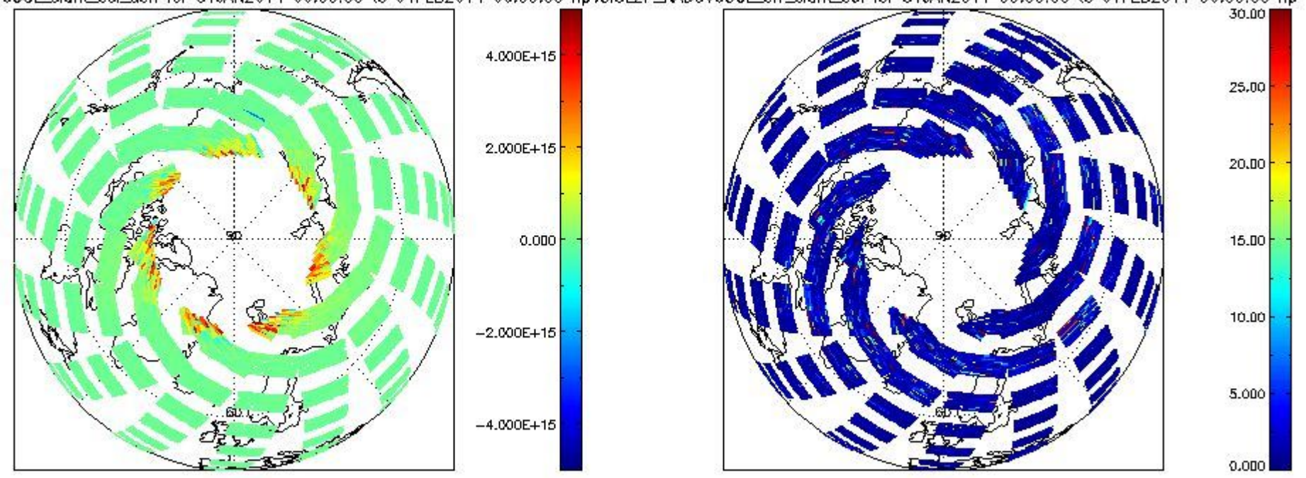
CIOL2P_NADUV6OCLslant_col_den for 31JAN2011 00:00:00 to 01FEB2011 00:00:00 np;CIOL2P_NADUV6OCLarr_slant_col for 31JAN2011 00:00:00 to 01FEB2011 00:00:00 np
