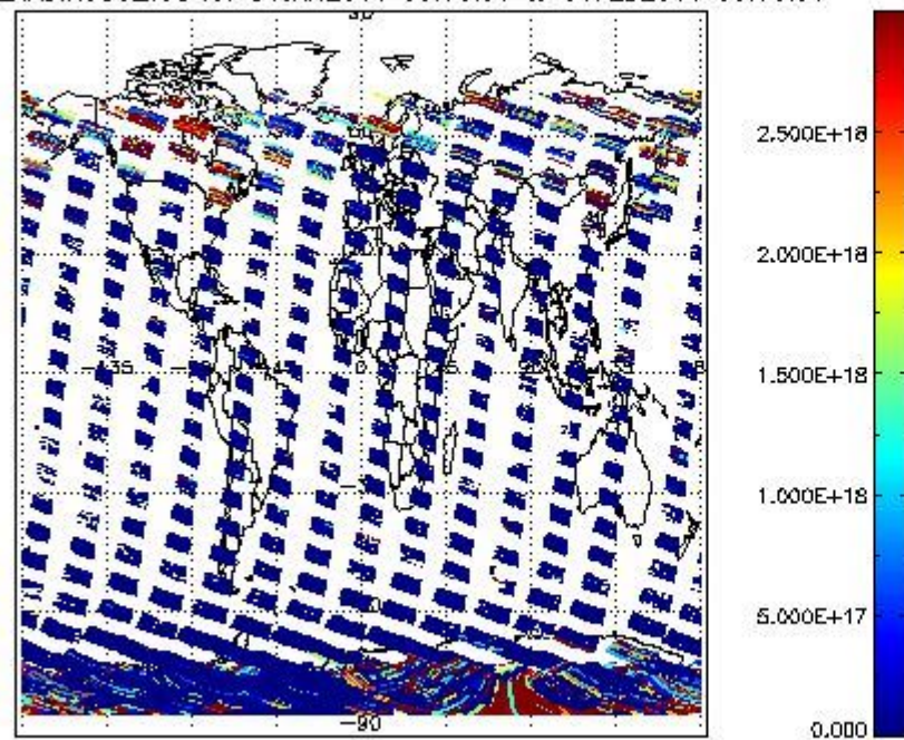
SCIOL2P_NADIR3CO_vcd for 31JAN2011 00:00:00 to 01FEB2011 00:00:00
