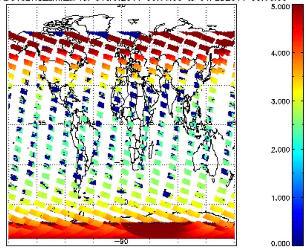
SCIOL2P_NADUV3BRO_amf_sl for 31JAN2011 00:00:00 to 01FEB2011 00:00:00
