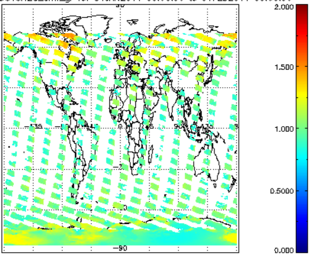
SCIOL2P_NADUV8H20_amf_gr for 31JAN2011 00:00:00 to 01FEB2011 00:00:00
