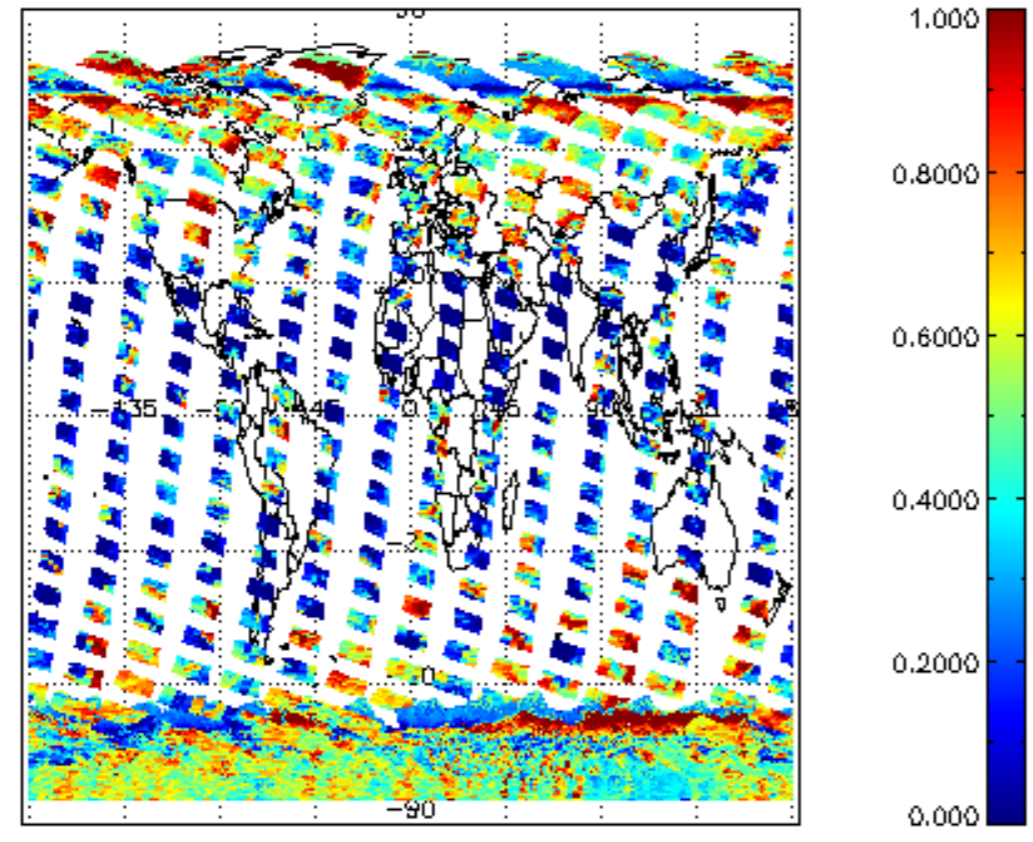
cl_frac for 31JAN2011 00:00:00 to 01FEB2011 00:00:00
