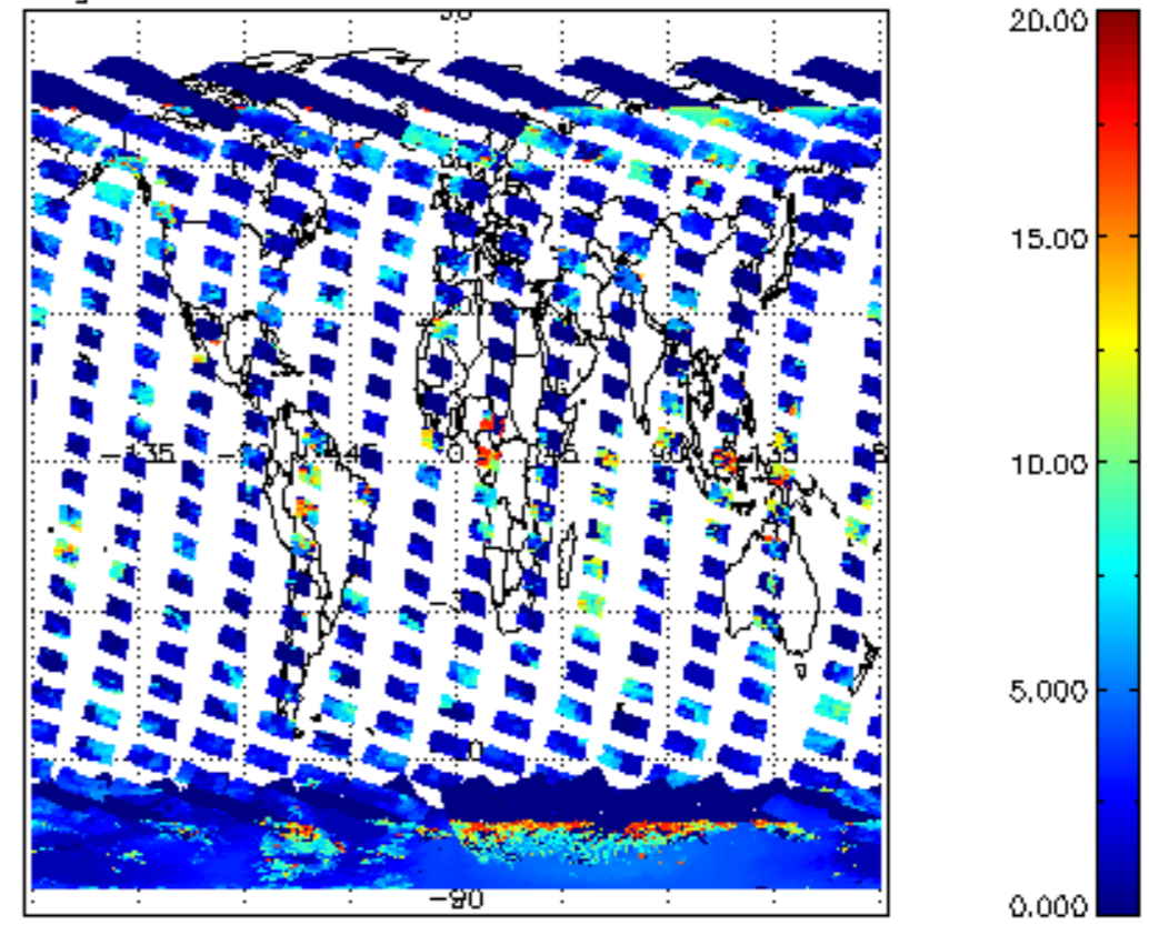
cl_top_height for 31JAN2011 00:00:00 to 01FEB2011 00:00:00
