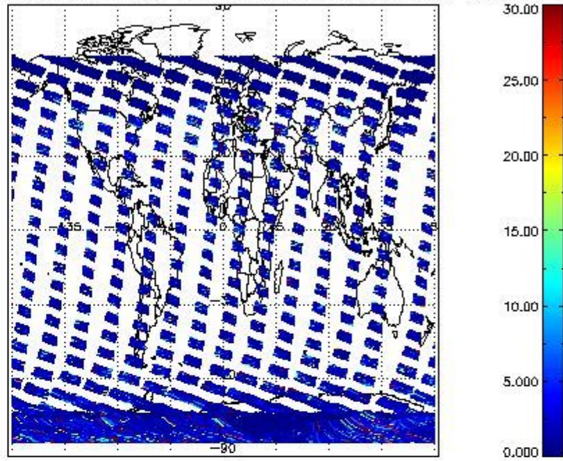
SCIOL2P_NADUV7S02_vcd_err for 31JAN2011 00:00:00 to 01FEB2011 00:00:00
