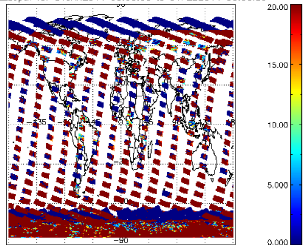
cl_opt_depth for 31JAN2011 00:00:00 to 01FEB2011 00:00:00
