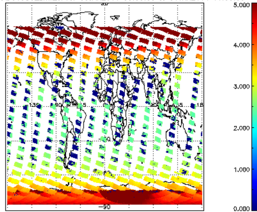
SCIOL2P_NADUV003_amf_cl for 30JAN2011 00:00:00 to 31JAN2011 00:00:00
