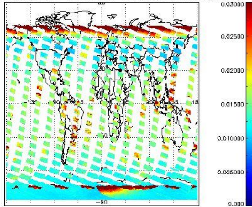
SCIOL2P_NADUV003_vcd_err for 30JAN2011 00:00:00 to 31JAN2011 00:00:00
