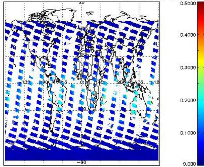
SCIOL2P_NADUV8H20_vcd_err for 30JAN2011 00:00:00 to 31JAN2011 00:00:00
