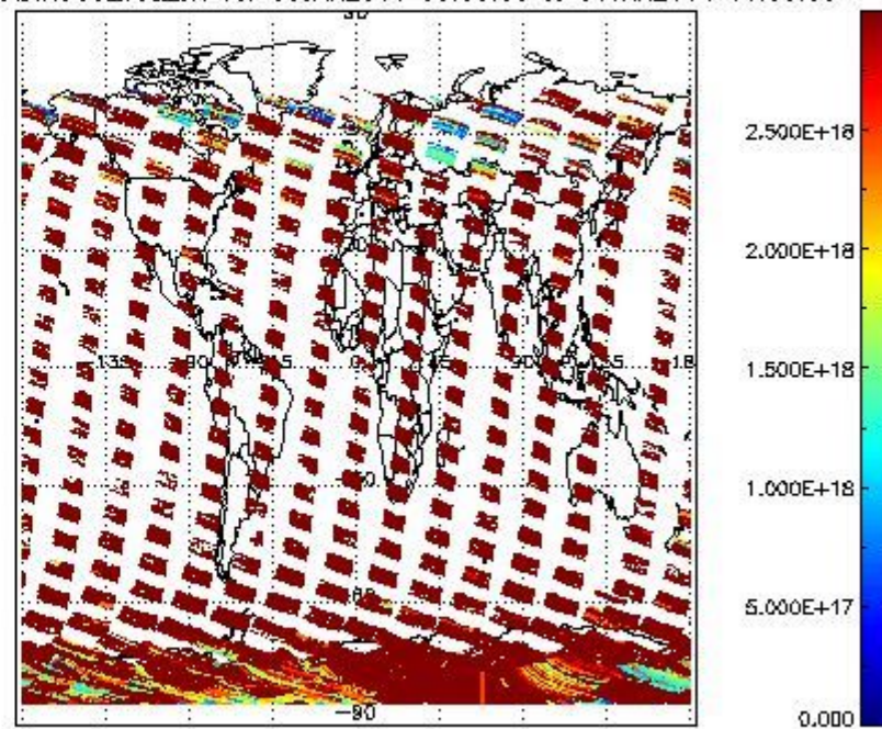
SCIDL2P_NADIR3CO_vcd_err for 30JAN2011 00:00:00 to 31JAN2011 00:00:00
