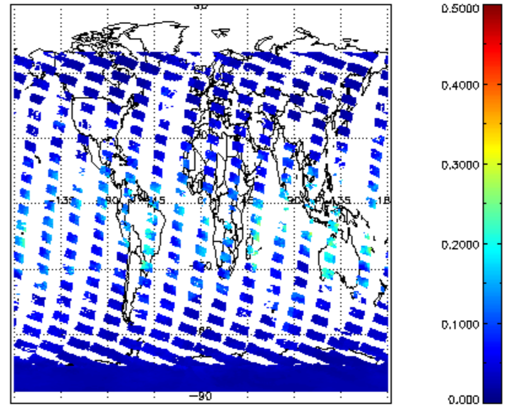
SCIOL2P_NADUVBH20_vcd_err for 30JAN2011 00:00:00 to 31JAN2011 00:00:00
