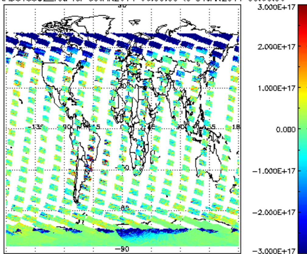
SCIOL2P_NADUV5S02_vcd for 30JAN2011 00:00:00 to 31JAN2011 00:00:00
