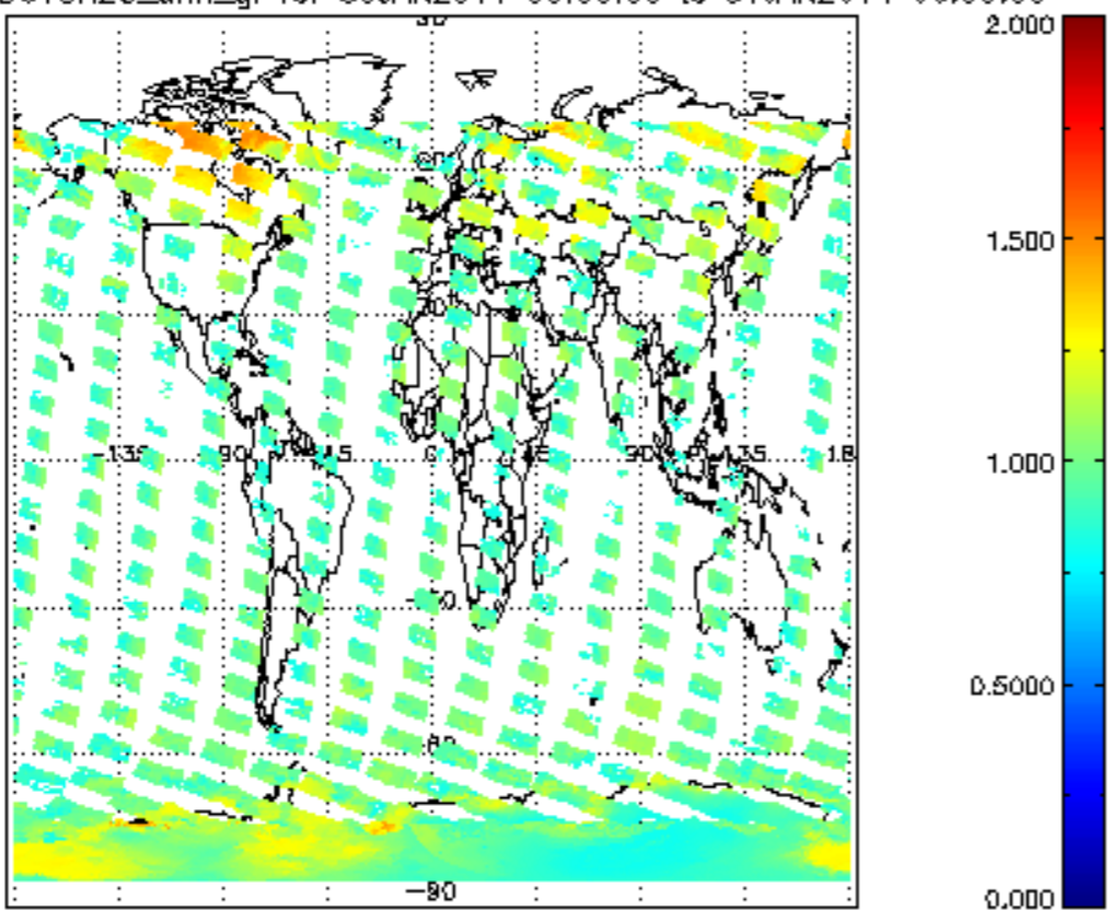
SCIOL2P_NADUVBH20_amf_gr for 30JAN2011 00:00:00 to 31JAN2011 00:00:00
