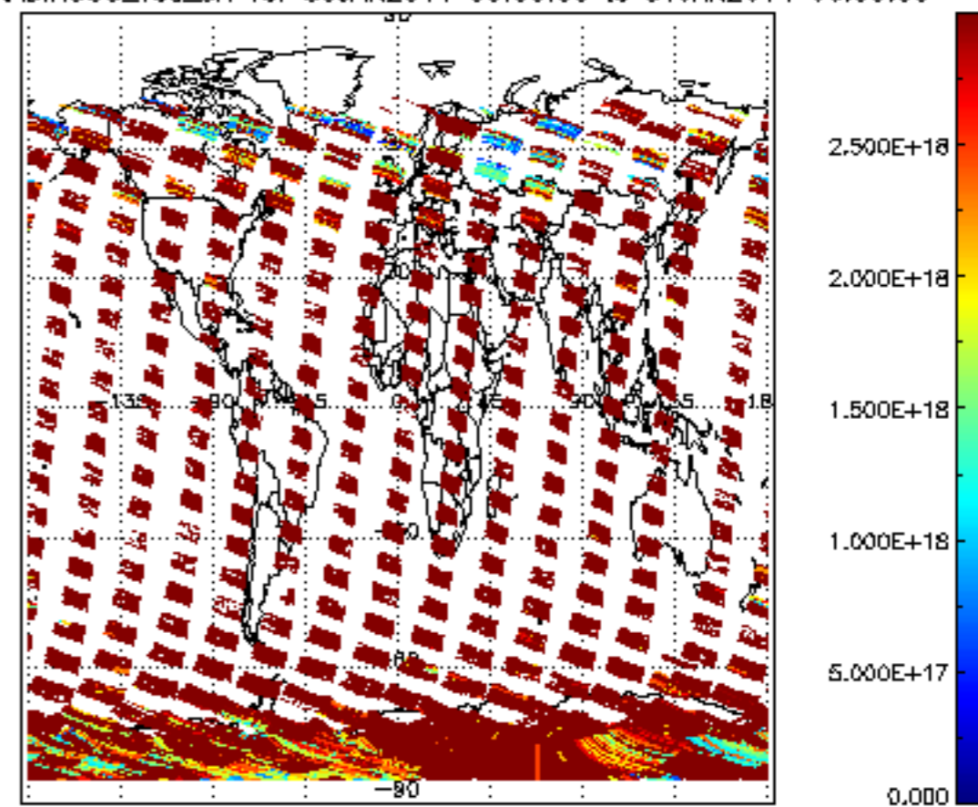
SCIOL2P_NADIR3CO_vcd_err for 30JAN2011 00:00:00 to 31JAN2011 00:00:00
