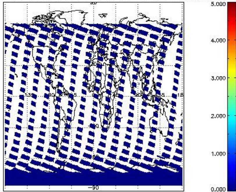
SCIOL2P_NADUV7S02_amf_cl for 30JAN2011 00:00:00 to 31JAN2011 00:00:00
