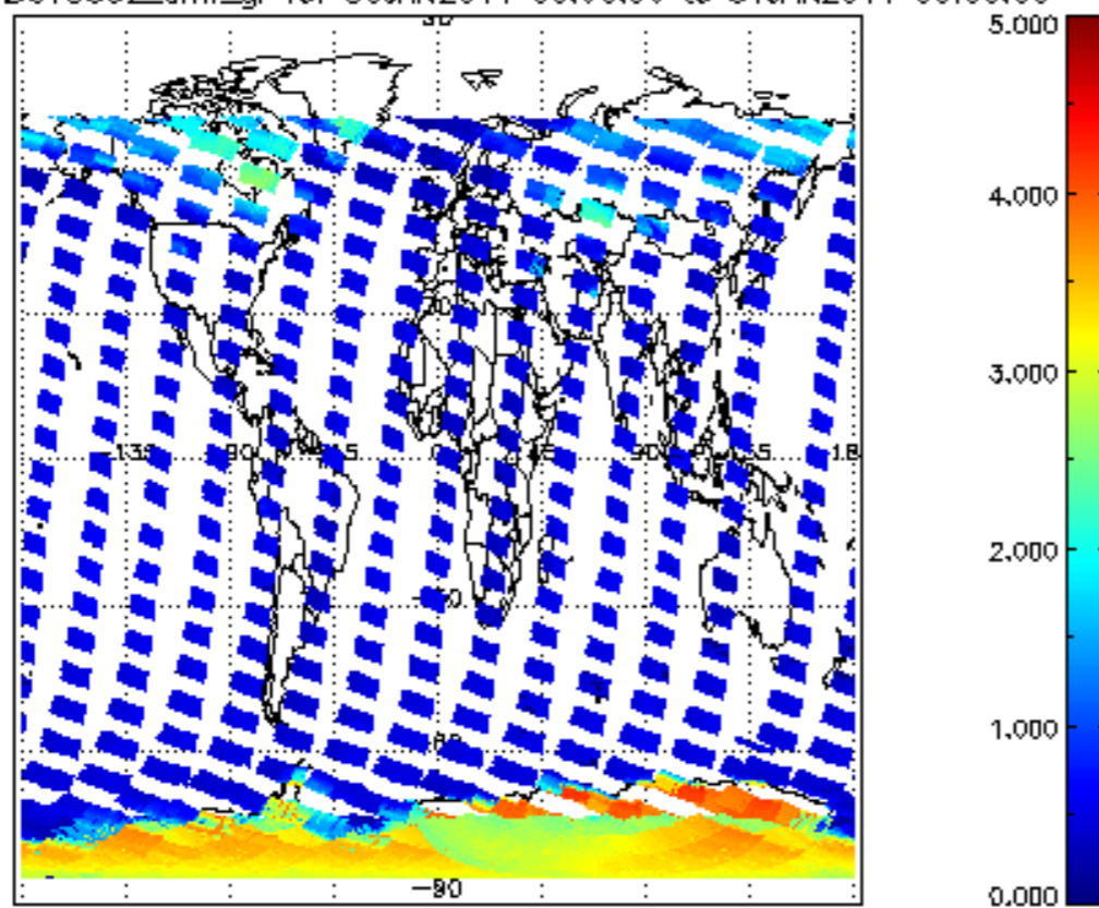
SCIOL2P_NADUV5S02_amf_gr for 30JAN2011 00:00:00 to 31JAN2011 00:00:00
