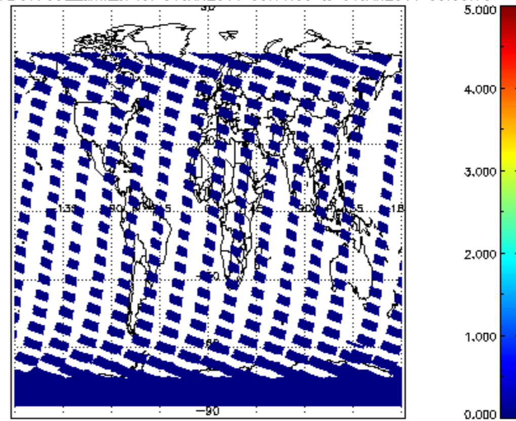
SCIOL2P_NADUV7S02_amf_sl for 30JAN2011 00:00:00 to 31JAN2011 00:00:00
