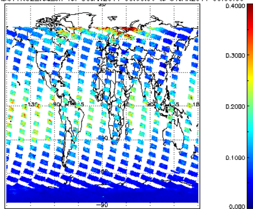
SCIOL2P_NADUV1NO2_vcd_err for 30JAN2011 00:00:00 to 31JAN2011 00:00:00
