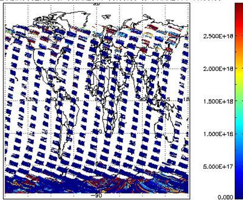
SCIDL2P_NADIR3CO_vcd for 30JAN2011 00:00:00 to 31JAN2011 00:00:00
