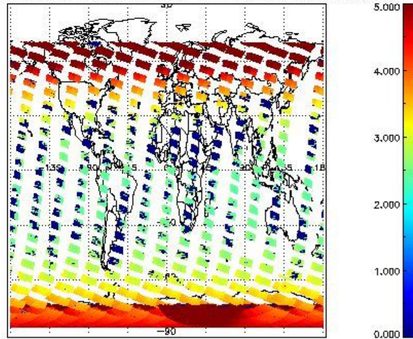
SCIOL2P_NADUV003_amf_cl for 30JAN2011 00:00:00 to 31JAN2011 00:00:00
