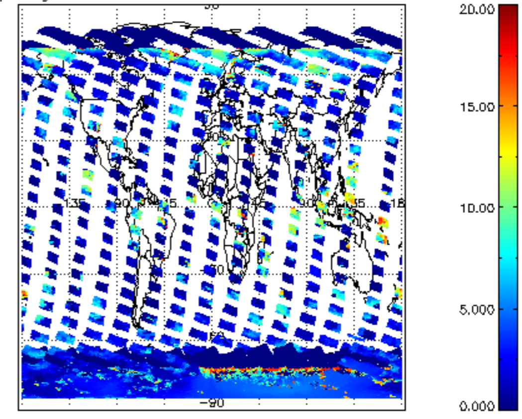
cL_top_height for 30JAN2011 00:00:00 to 31JAN2011 00:00:00
