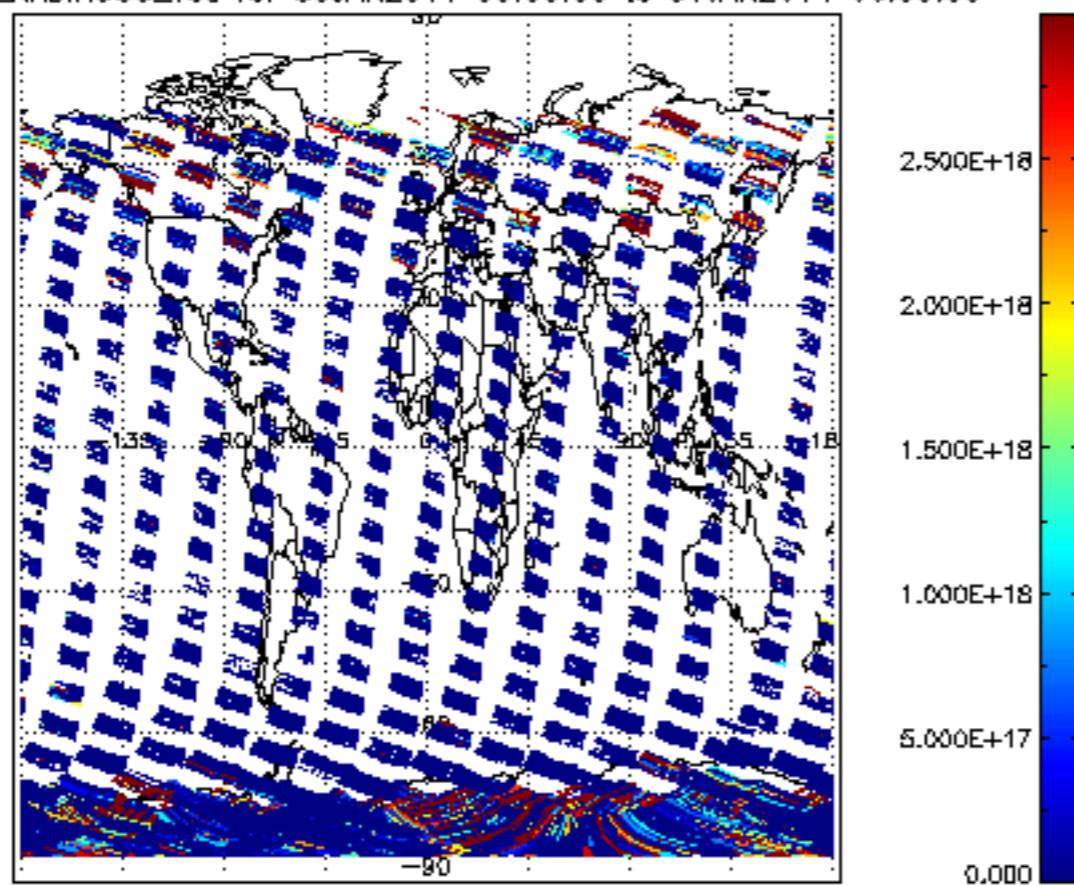
SCIOL2P_NADIR3CO_vcd for 30JAN2011 00:00:00 to 31JAN2011 00:00:00
