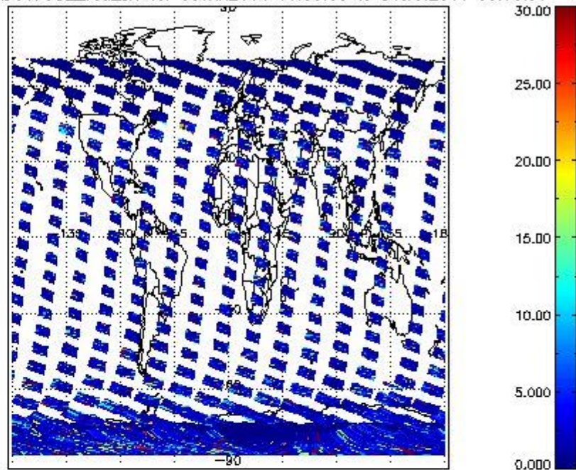
SCIOL2P_NADUV7S02_vcd_err for 30JAN2011 00:00:00 to 31JAN2011 00:00:00
