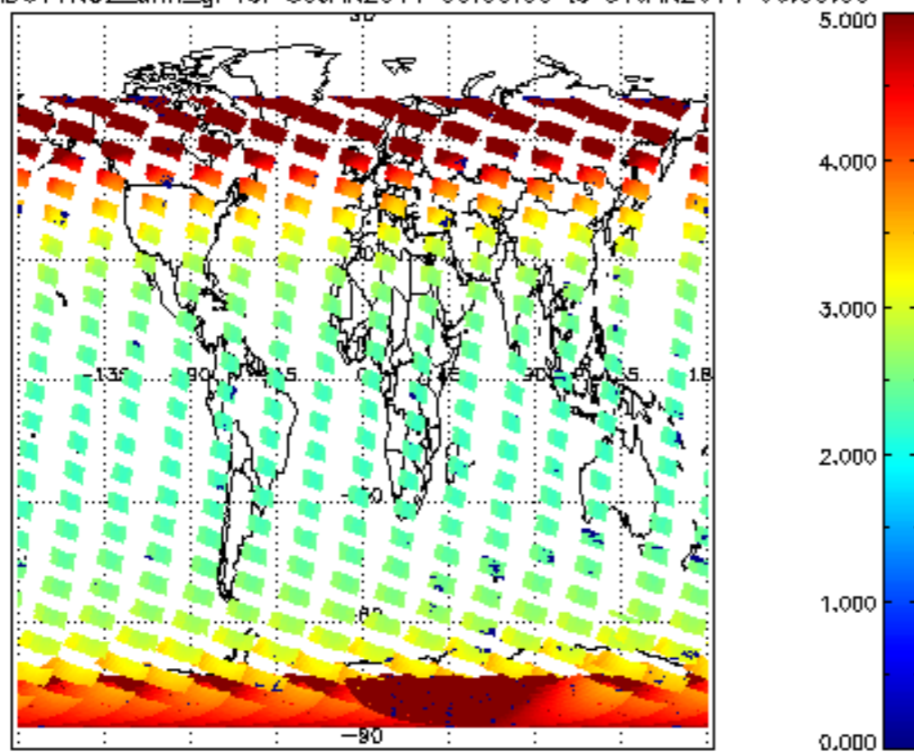
SCIOL2P_NADUV1NO2_amf_gr for 30JAN2011 00:00:00 to 31JAN2011 00:00:00
