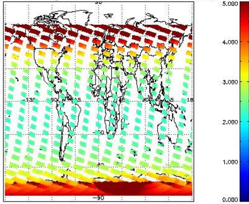
SCIOL2P_NADUV3BRO_amf_gr for 30JAN2011 00:00:00 to 31JAN2011 00:00:00
