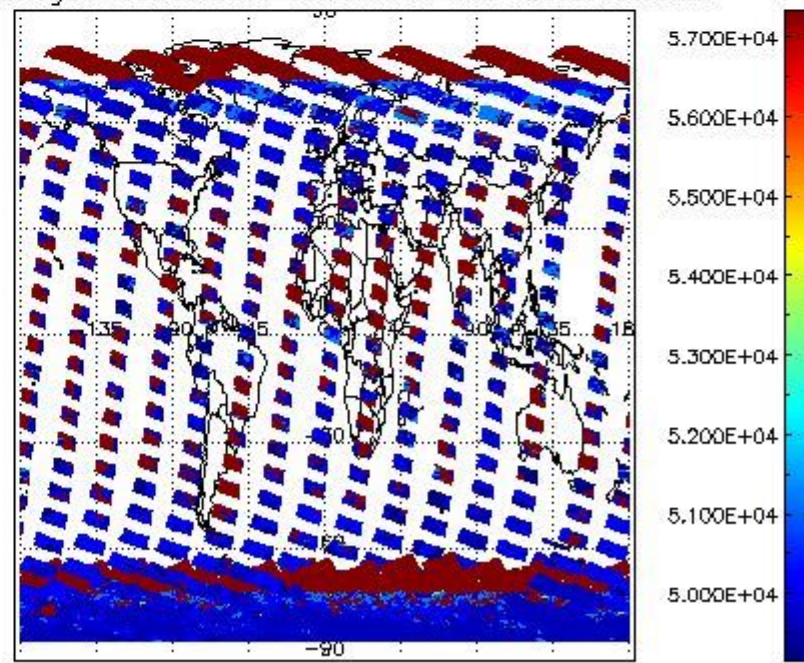
cloud_flags for 30JAN2011 00:00:00 to 31JAN2011 00:00:00
