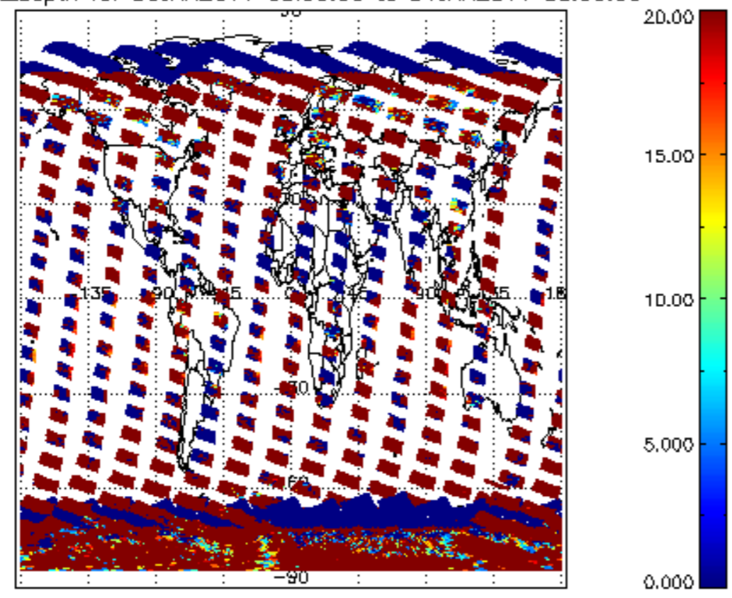
cL_opt_depth for 30JAN2011 00:00:00 to 31JAN2011 00:00:00
