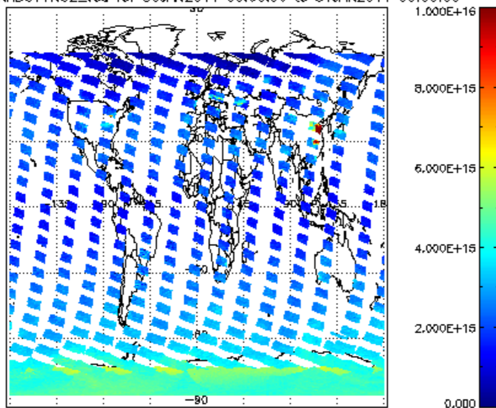
SCIOL2P_NADUV1NO2_vcd for 30JAN2011 00:00:00 to 31JAN2011 00:00:00
