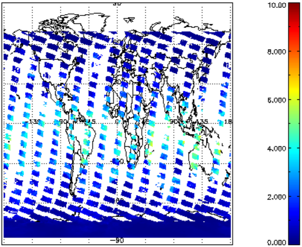
SCIOL2P_NADUVBH20_vcd for 30JAN2011 00:00:00 to 31JAN2011 00:00:00
