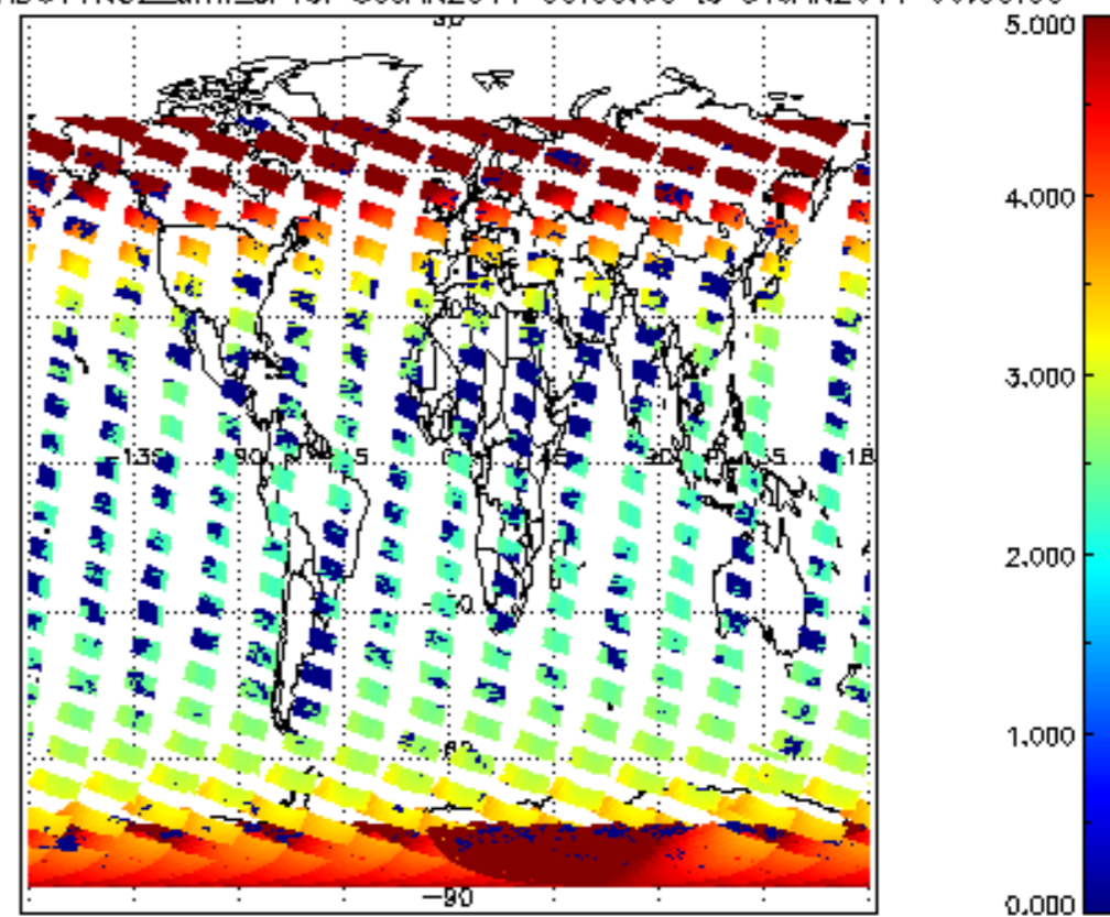
SCIOL2P_NADUV1NO2_amf_cl for 30JAN2011 00:00:00 to 31JAN2011 00:00:00
