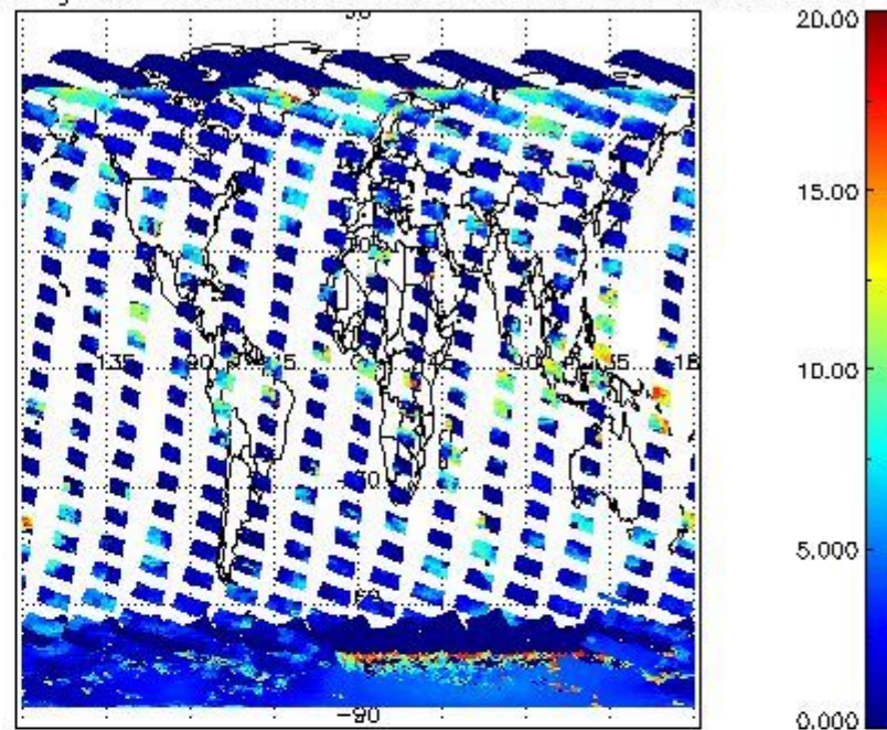
cL_top_height for 30JAN2011 00:00:00 to 31JAN2011 00:00:00
