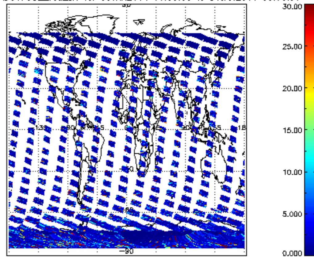
SCIOL2P_NADUV7S02_vcd_err for 30JAN2011 00:00:00 to 31JAN2011 00:00:00
