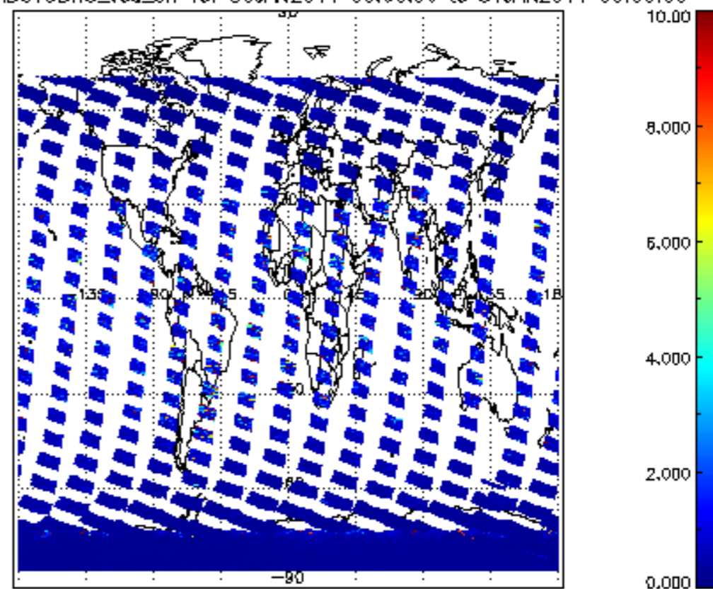
SCIOL2P_NADUV3BRO_vcd_err for 30JAN2011 00:00:00 to 31JAN2011 00:00:00
