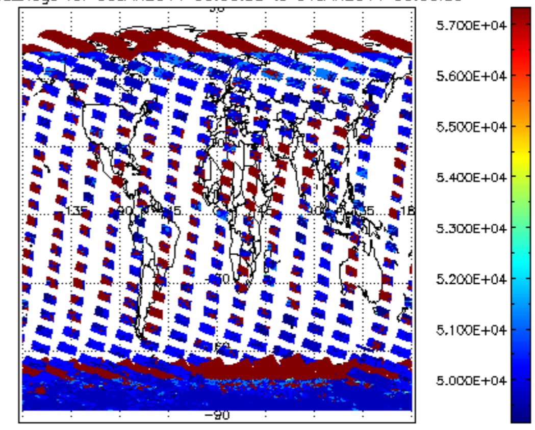
cloud_flags for 30JAN2011 00:00:00 to 31JAN2011 00:00:00
