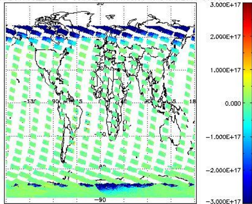
SCIOL2P_NADUV7S02_vcd for 30JAN2011 00:00:00 to 31JAN2011 00:00:00
