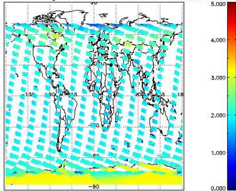
SCIOL2P_NADUV7S02_amf_gr for 30JAN2011 00:00:00 to 31JAN2011 00:00:00
