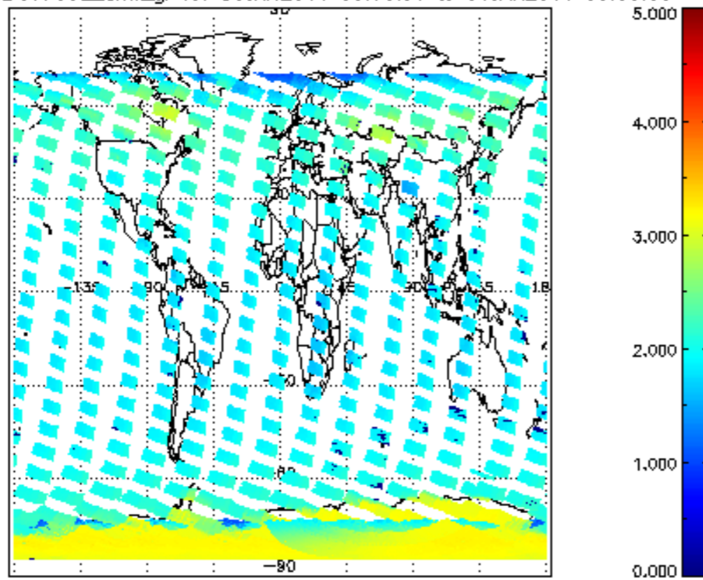
SCIOL2P_NADUV7S02_amf_gr for 30JAN2011 00:00:00 to 31JAN2011 00:00:00
