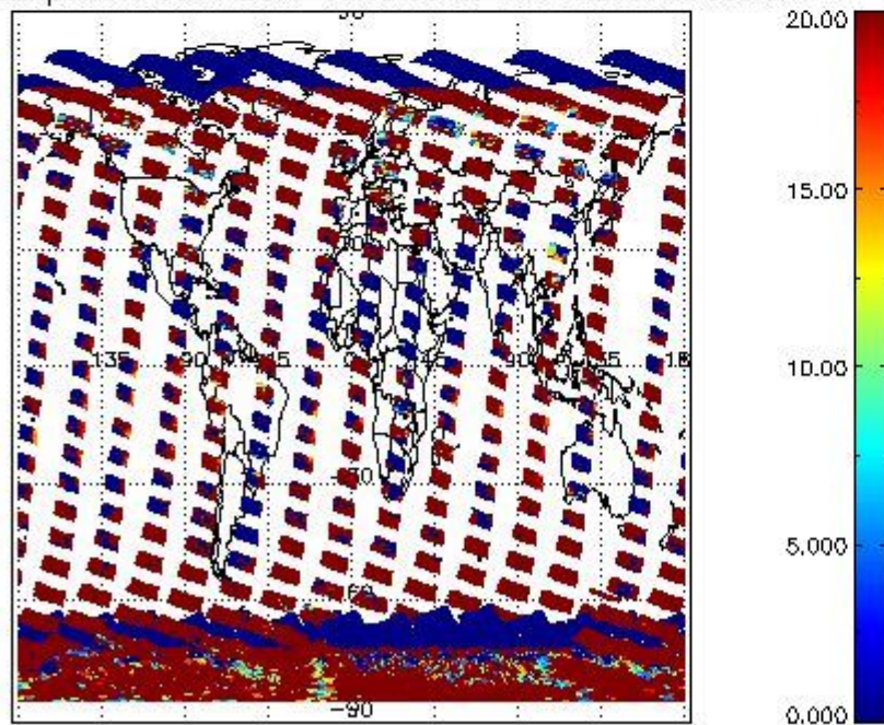
cLopt_depth for 30JAN2011 00:00:00 to 31JAN2011 00:00:00
