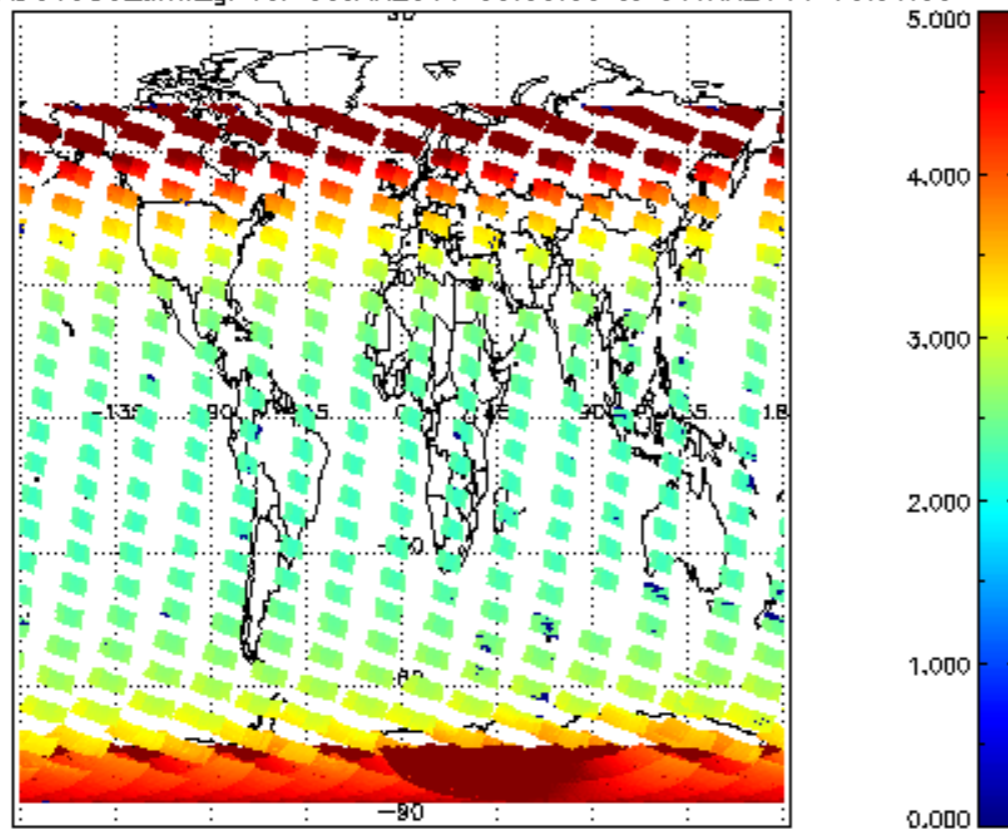
SCIOL2P_NADUV003_amf_gr for 30JAN2011 00:00:00 to 31JAN2011 00:00:00
