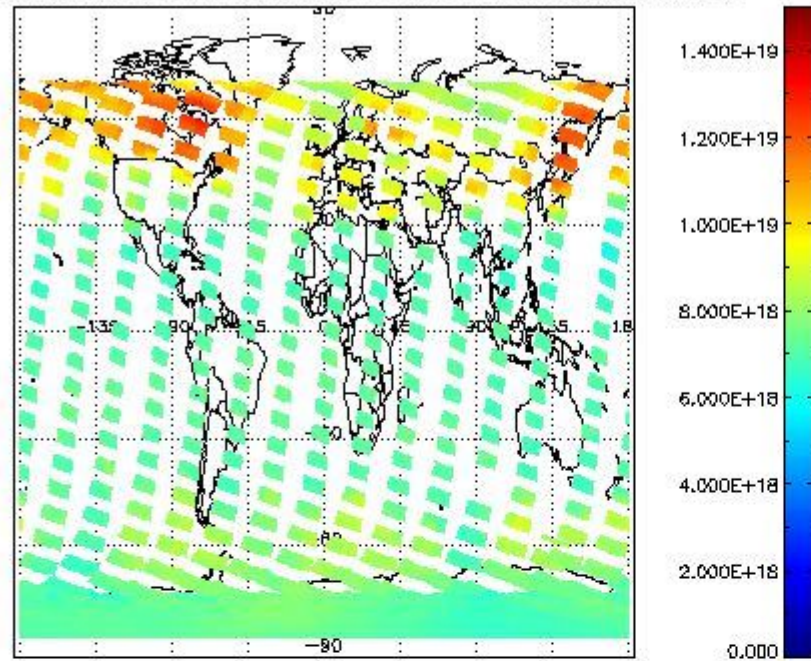
SCIOL2P_NADUV003_vcd for 30JAN2011 00:00:00 to 31JAN2011 00:00:00
