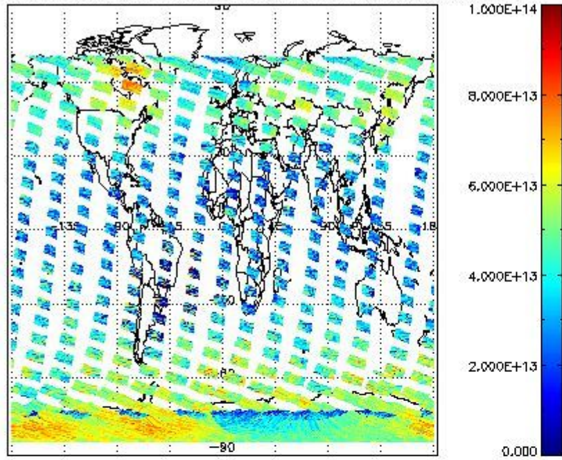
SCIOL2P_NADUV3BRO_vcd for 30JAN2011 00:00:00 to 31JAN2011 00:00:00
