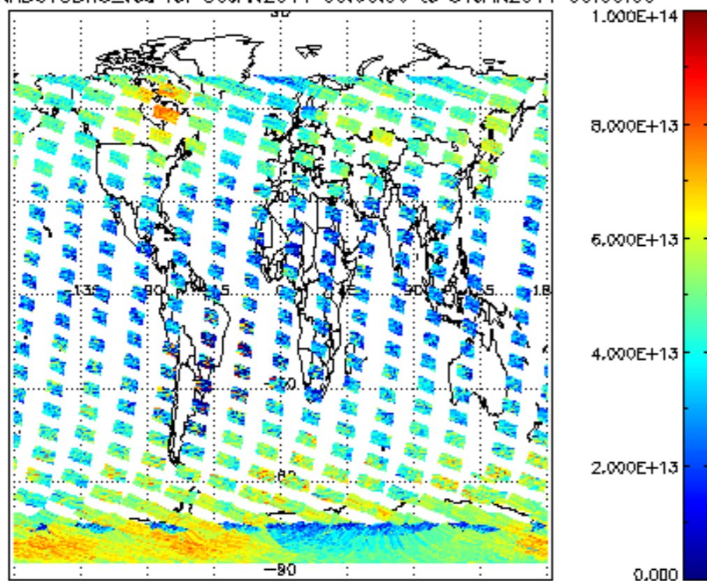
SCIOL2P_NADUV3BRO_vcd for 30JAN2011 00:00:00 to 31JAN2011 00:00:00
