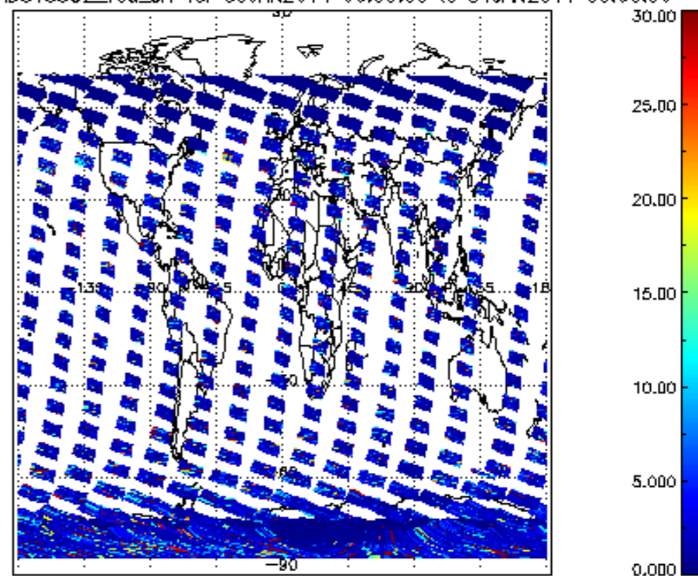
SCIOL2P_NADUV5S02_vcd_err for 30JAN2011 00:00:00 to 31JAN2011 00:00:00
