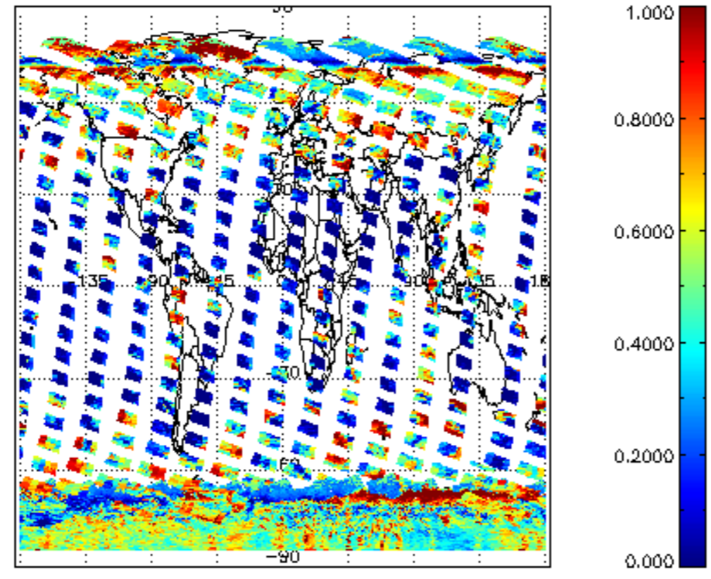
cL_frac for 30JAN2011 00:00:00 to 31JAN2011 00:00:00
