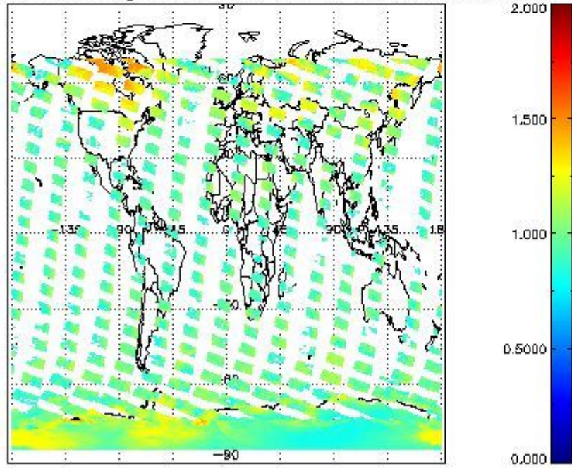
SCIOL2P_NADUV8H20_amf_gr for 30JAN2011 00:00:00 to 31JAN2011 00:00:00
