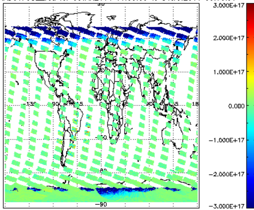
SCIOL2P_NADUV7S02_vcd for 30JAN2011 00:00:00 to 31JAN2011 00:00:00
