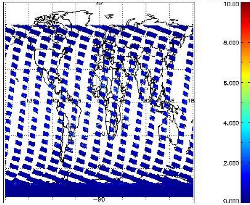
SCIOL2P_NADUV3BRO_vcd_err for 30JAN2011 00:00:00 to 31JAN2011 00:00:00
