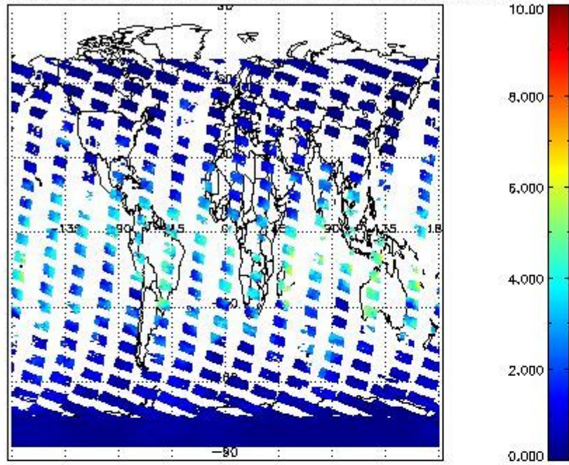
SCIOL2P_NADUV8H20_vcd for 30JAN2011 00:00:00 to 31JAN2011 00:00:00
