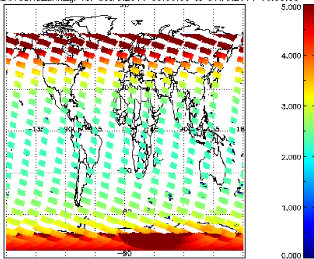
SCIOL2P_NADUV3BRO_amf_gr for 30JAN2011 00:00:00 to 31JAN2011 00:00:00
