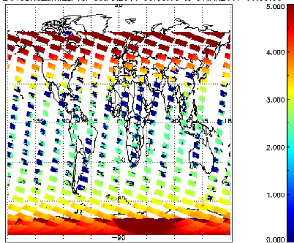
SCIOL2P_NADUV3BRO_amf_cl for 30JAN2011 00:00:00 to 31JAN2011 00:00:00
