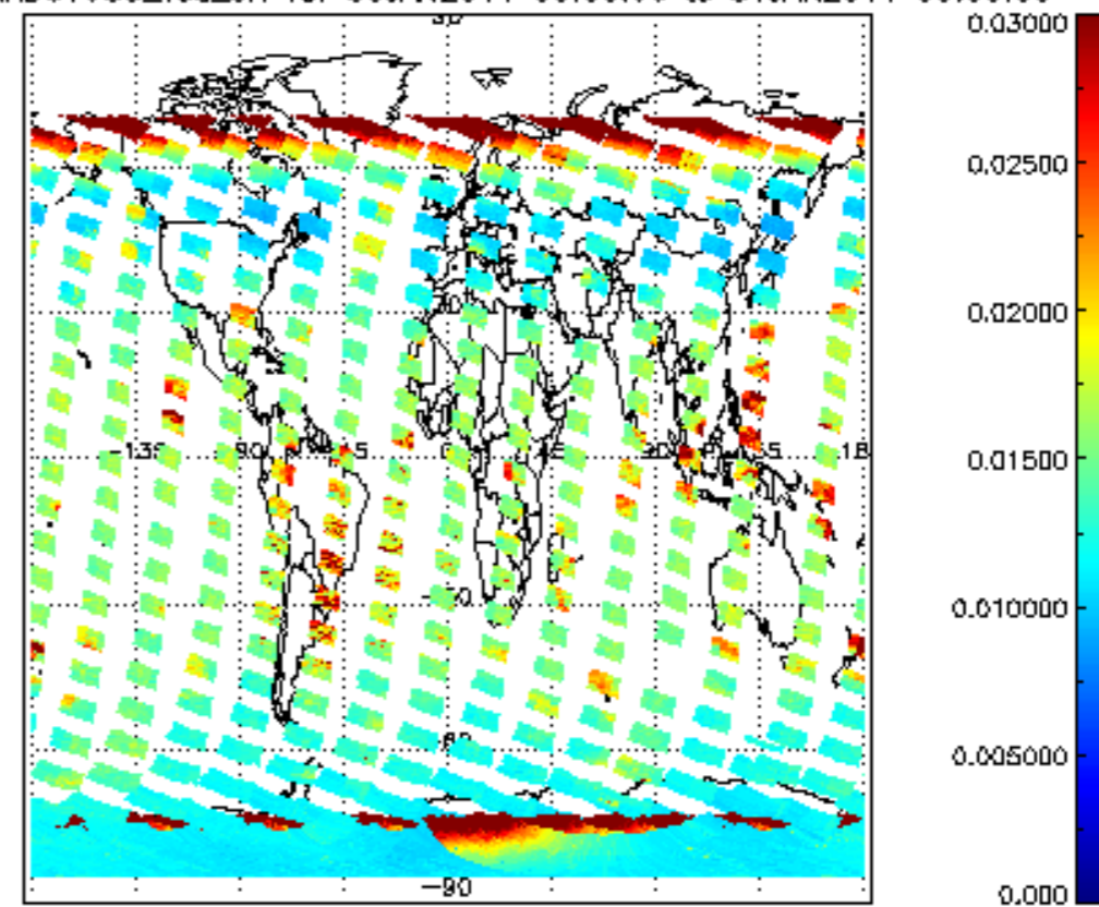
SCIOL2P_NADUV003_vcd_err for 30JAN2011 00:00:00 to 31JAN2011 00:00:00
