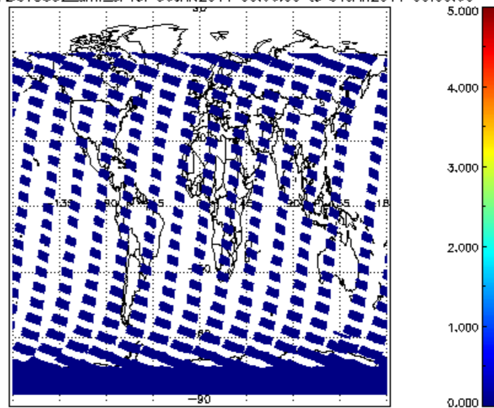
SCIOL2P_NADUV5S02_amf_sl for 30JAN2011 00:00:00 to 31JAN2011 00:00:00
