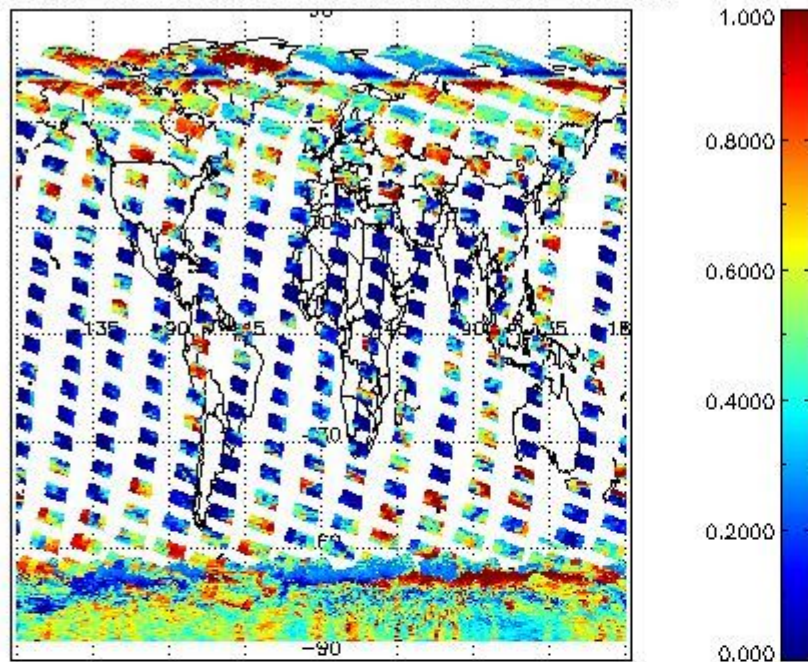
cL_frac for 30JAN2011 00:00:00 to 31JAN2011 00:00:00
