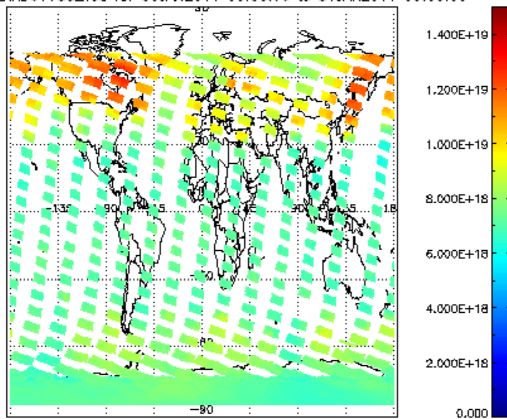
SCIOL2P_NADUV003_vcd for 30JAN2011 00:00:00 to 31JAN2011 00:00:00
