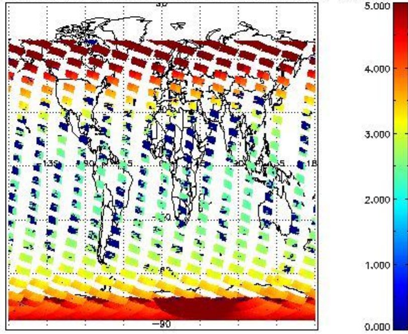
SCIOL2P_NADUV3BRO_amf_cl for 30JAN2011 00:00:00 to 31JAN2011 00:00:00
