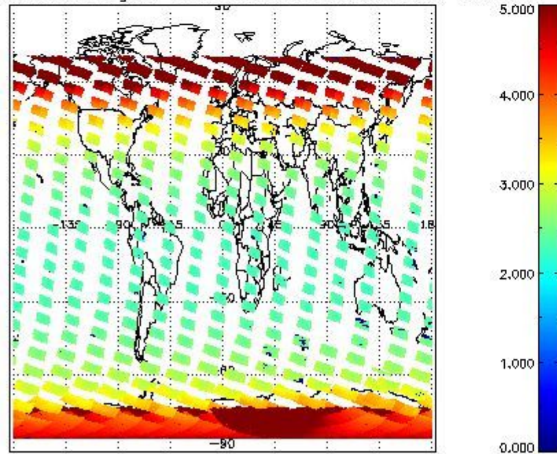
SCIOL2P_NADUV003_amf_gr for 30JAN2011 00:00:00 to 31JAN2011 00:00:00
