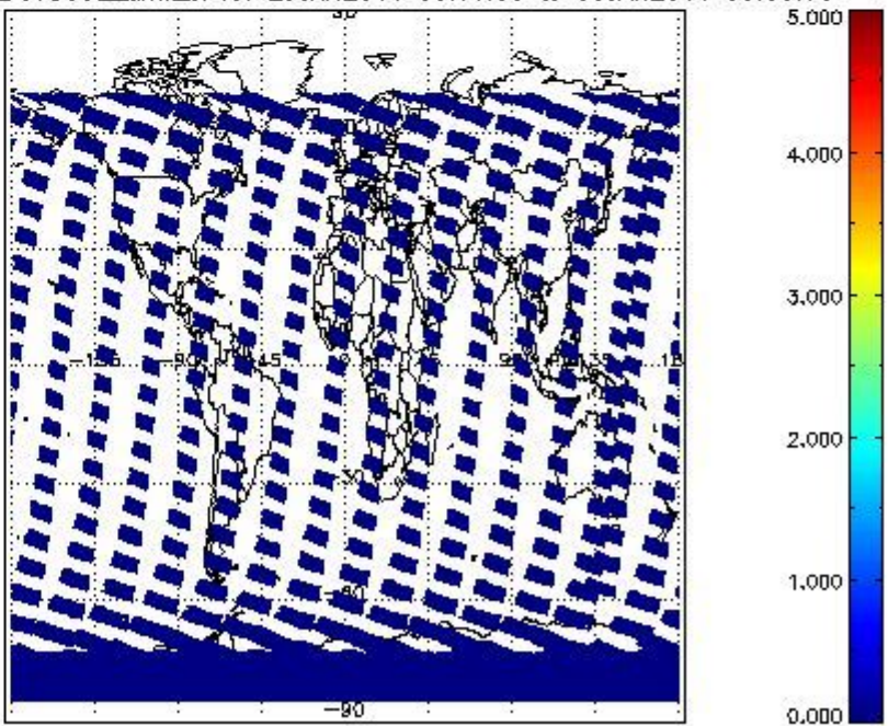
SCIOL2P_NADUV5SO2_amf_cl for 29JAN2011 00:00:00 to 30JAN2011 00:00:00
