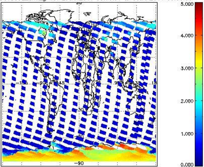
SCIOL2P_NADUV5SO2_amf_gr for 29JAN2011 00:00:00 to 30JAN2011 00:00:00
