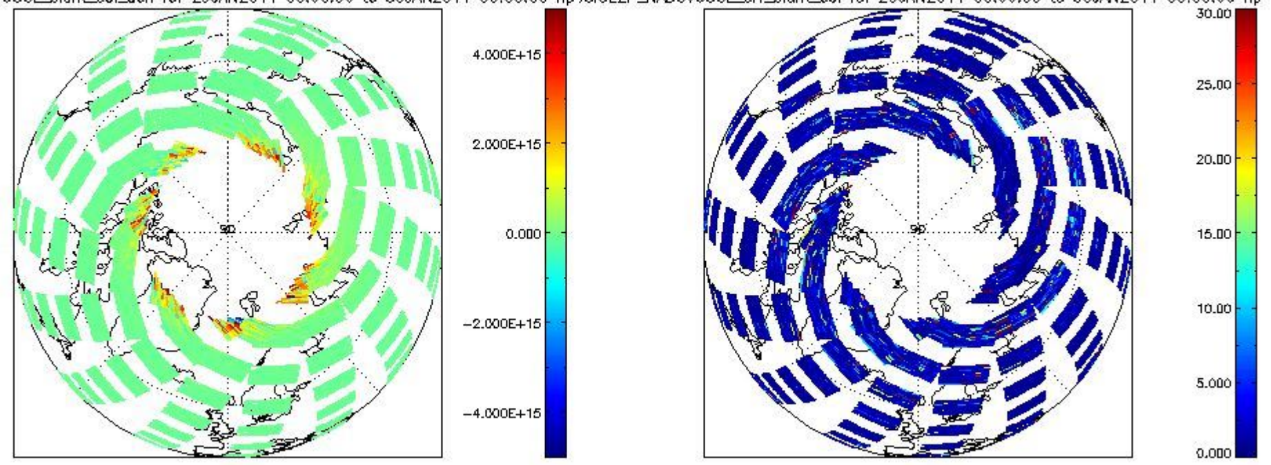
SCIOI2P_NADUV60CL_slant_col_den for 29JAN2011 00:00:00 to 30JAN2011 00:00:00 np; SCIOI2P_NADUV60CL_err_slant_col for 29JAN2011 00:00:00 to 30JAN2011 00:00:00 np
