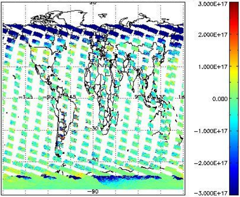
SCIOL2P_NADUV5SO2_vcd for 29JAN2011 00:00:00 to 30JAN2011 00:00:00
