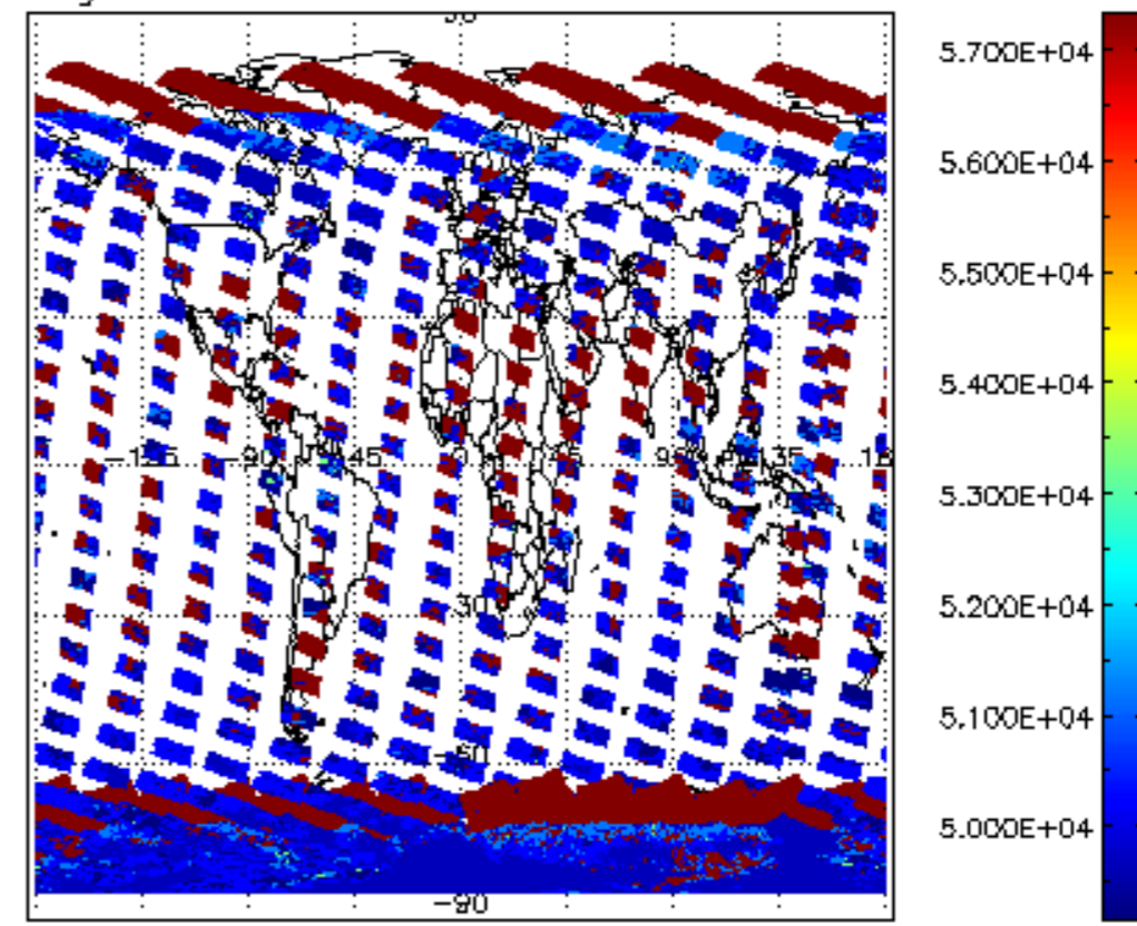
cloud_flags for 29JAN2011 00:00:00 to 30JAN2011 00:00:00
