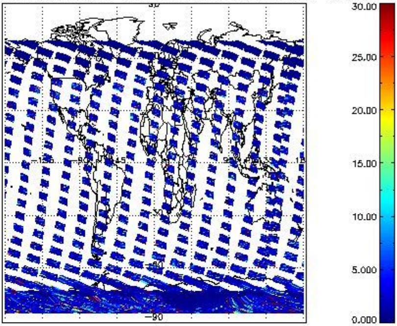
SCIOL2P_NADUV5SO2_vcd_err for 29JAN2011 00:00:00 to 30JAN2011 00:00:00
