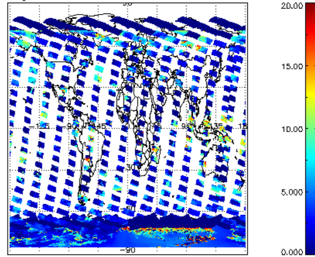
cL_top_height for 29JAN2011 00:00:00 to 30JAN2011 00:00:00
