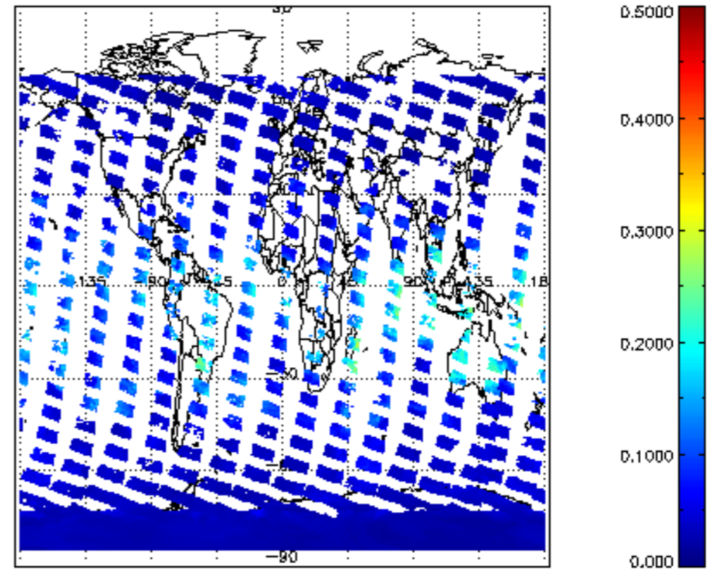
SCIOL2P_NADUV8H20_vcd_err for 27JAN2011 00:00:00 to 28JAN2011 00:00:00
