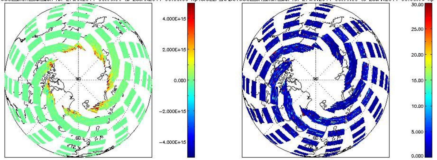
SCIOI2P_NADUV60CL_slant_col_den for 27JAN2011 00:00:00 to 28JAN2011 00:00:00 np; SCIOI2P_NADUV60CL_err_slant_col for 27JAN2011 00:00:00 to 28JAN2011 00:00:00 np
