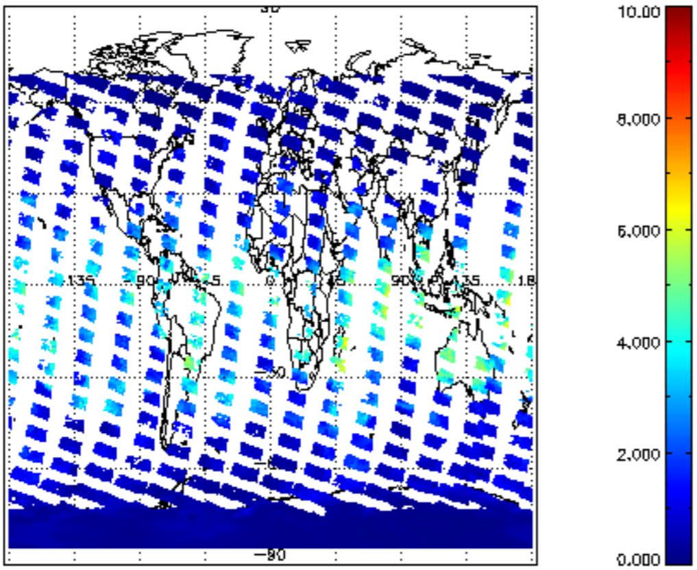
SCIOL2P_NADUV8H20_vcd for 27JAN2011 00:00:00 to 28JAN2011 00:00:00
