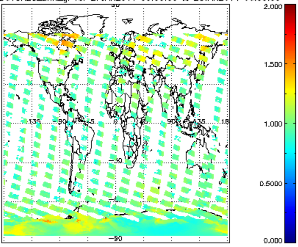
SCIOL2P_NADUV8H20_amf_gr for 27JAN2011 00:00:00 to 28JAN2011 00:00:00
