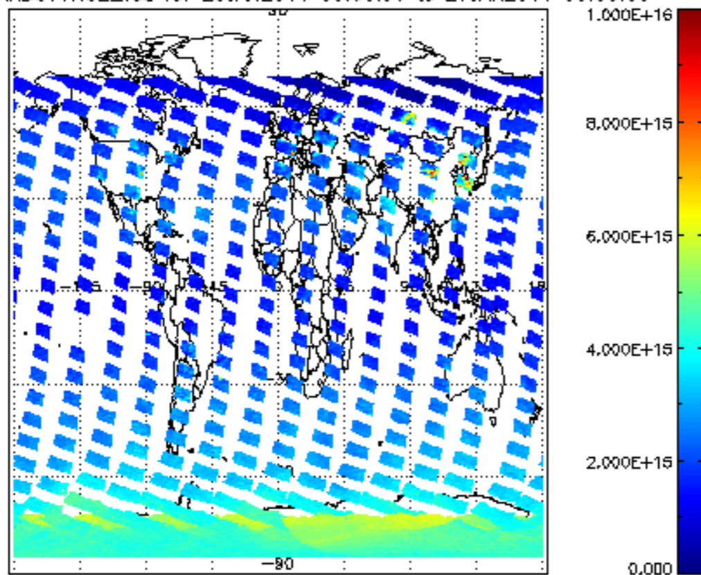
SCIOL2P_NADUV1NO2_vcd for 26JAN2011 00:00:00 to 27JAN2011 00:00:00
