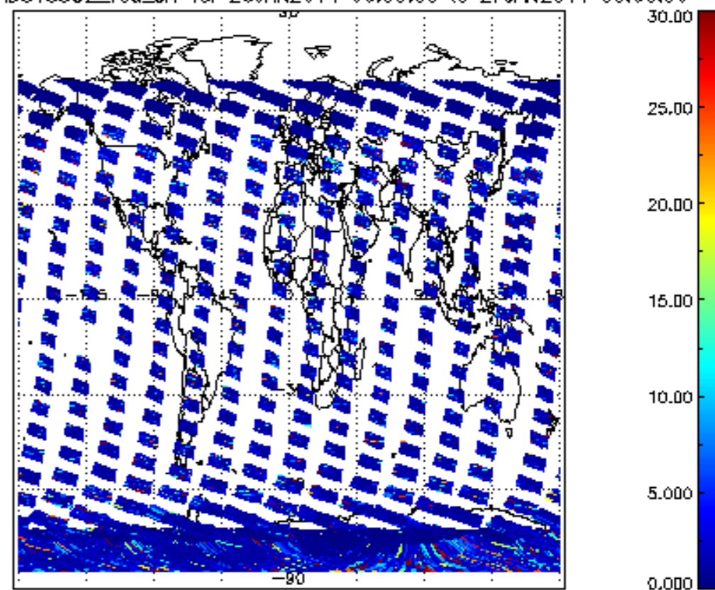
SCIOL2P_NADUV5S02_vcd_err for 26JAN2011 00:00:00 to 27JAN2011 00:00:00
