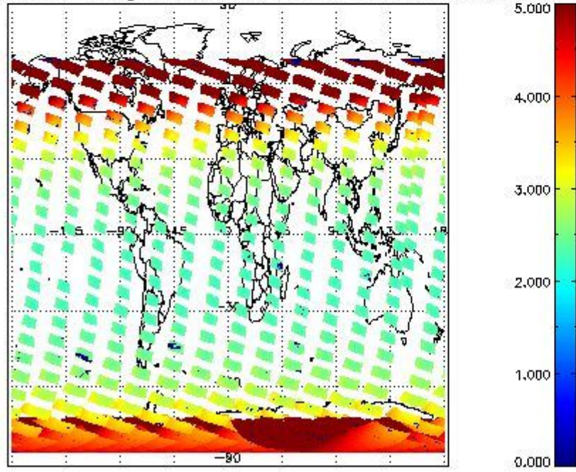
SCIOL2P_NADUV1NO2_amf_gr for 26JAN2011 00:00:00 to 27JAN2011 00:00:00
