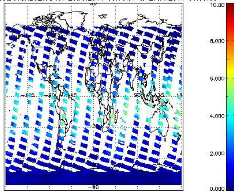
SCIOL2P_NADUV8H20_vcd for 26JAN2011 00:00:00 to 27JAN2011 00:00:00
