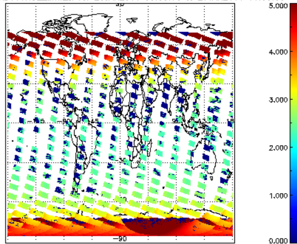
SCIOL2P_NADUV1NO2_amf_cl for 26JAN2011 00:00:00 to 27JAN2011 00:00:00
