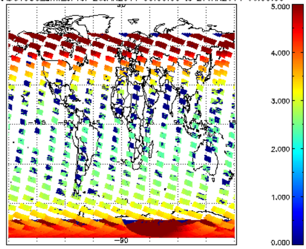
SCIOL2P_NADUV003_amf_cl for 26JAN2011 00:00:00 to 27JAN2011 00:00:00
