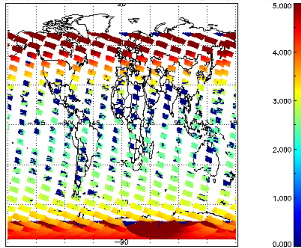
SCIOL2P_NADUV3BRO_amf_cl for 26JAN2011 00:00:00 to 27JAN2011 00:00:00
