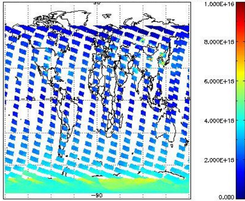
SCIOL2P_NADUV1NO2_vcd for 26JAN2011 00:00:00 to 27JAN2011 00:00:00
