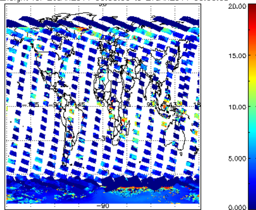
cL_top_height for 26JAN2011 00:00:00 to 27JAN2011 00:00:00
