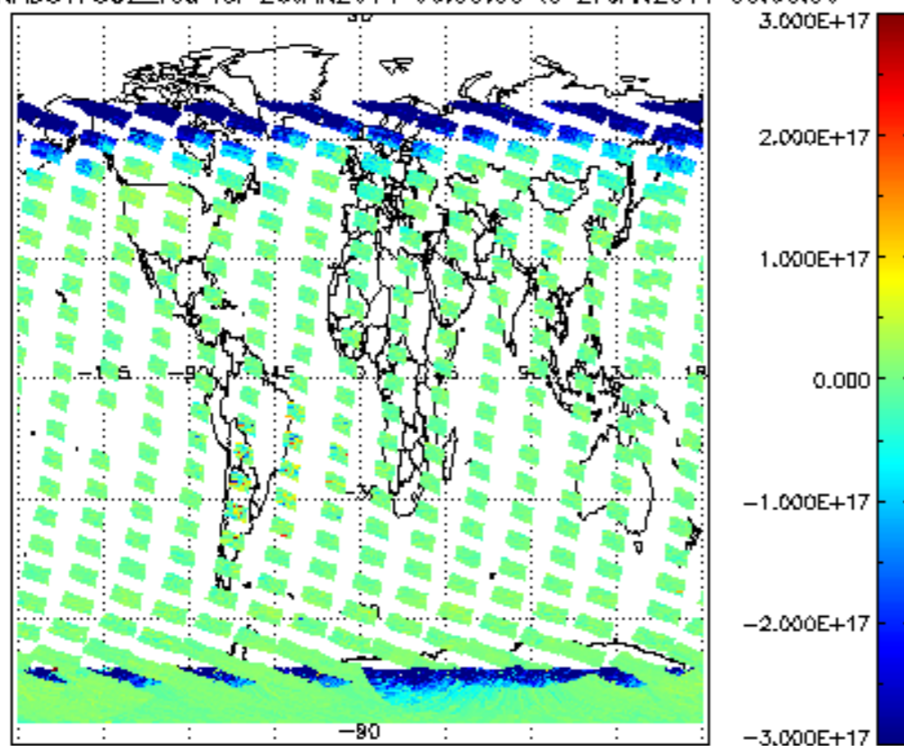
SCIOL2P_NADUV7S02_vcd for 26JAN2011 00:00:00 to 27JAN2011 00:00:00
