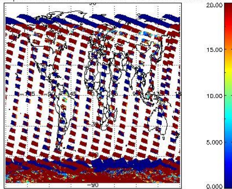
cLopt_depth for 26JAN2011 00:00:00 to 27JAN2011 00:00:00
