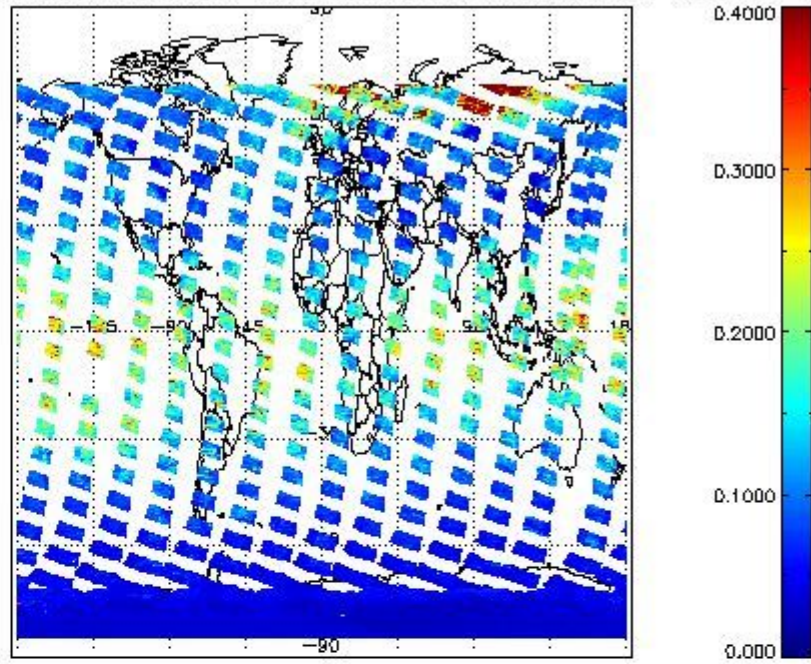
SCIOL2P_NADUV1NO2_vcd_err for 26JAN2011 00:00:00 to 27JAN2011 00:00:00
