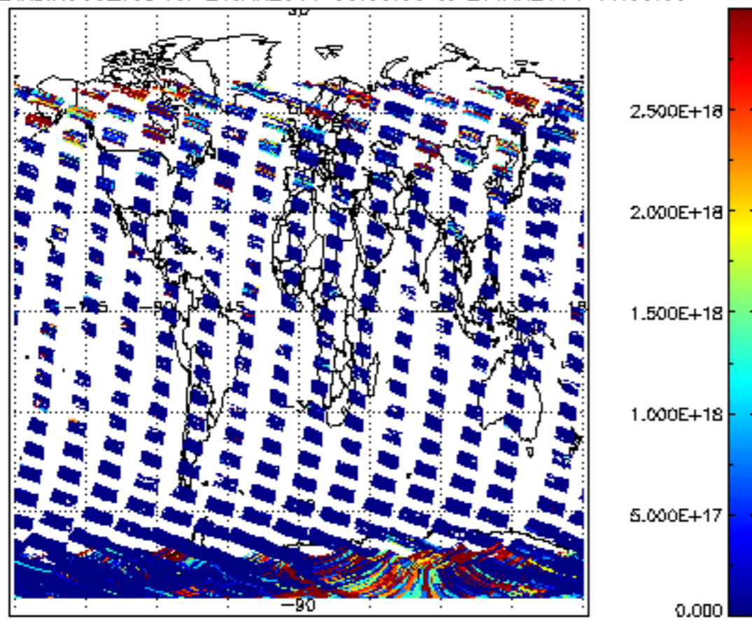
SCIOL2P_NADIR3CO_vcd for 26JAN2011 00:00:00 to 27JAN2011 00:00:00
