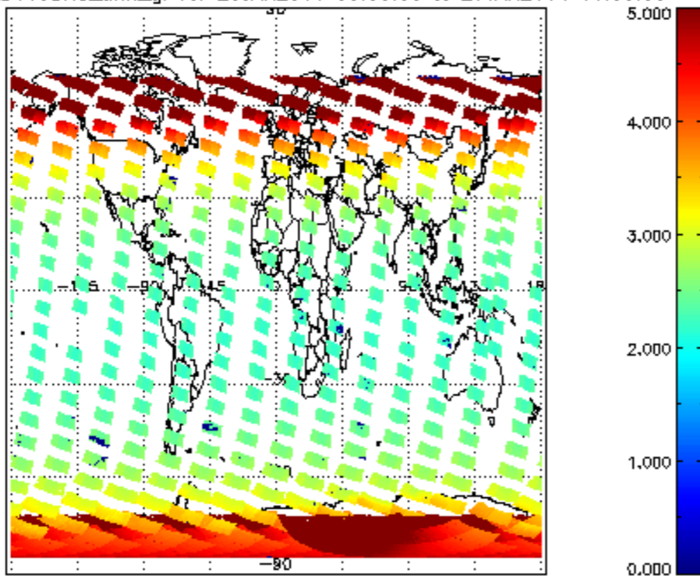
SCIOL2P_NADUV3BRO_amf_gr for 26JAN2011 00:00:00 to 27JAN2011 00:00:00
