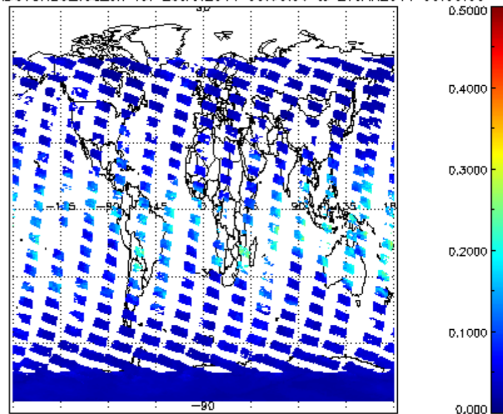
SCIOL2P_NADUV8H20_vcd_err for 26JAN2011 00:00:00 to 27JAN2011 00:00:00
