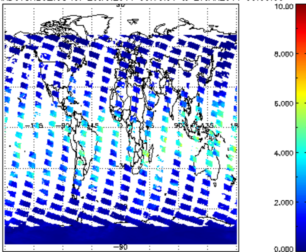
SCIOL2P_NADUV8H20_vcd for 26JAN2011 00:00:00 to 27JAN2011 00:00:00
