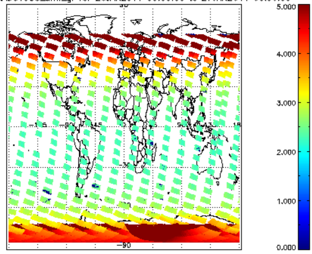
SCIOL2P_NADUV003_amf_gr for 26JAN2011 00:00:00 to 27JAN2011 00:00:00
