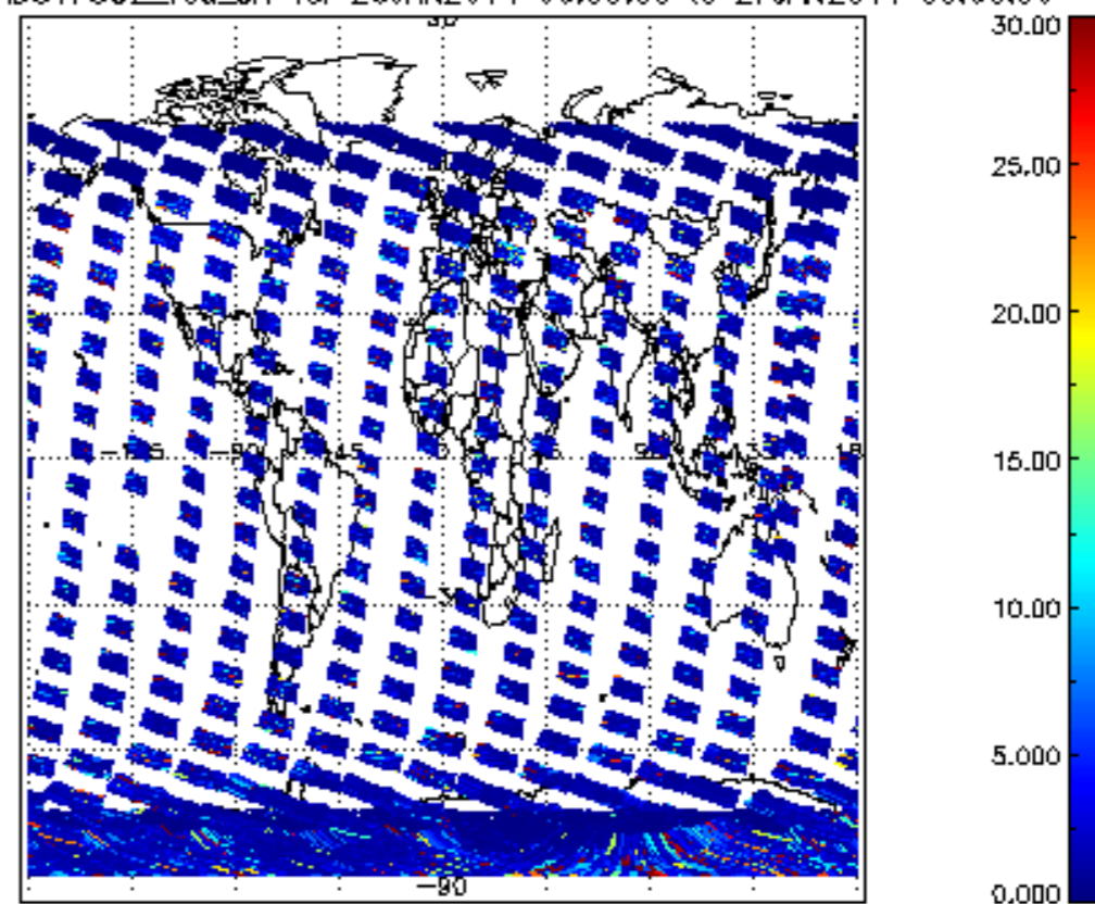
SCIOL2P_NADUV7S02_vcd_err for 26JAN2011 00:00:00 to 27JAN2011 00:00:00
