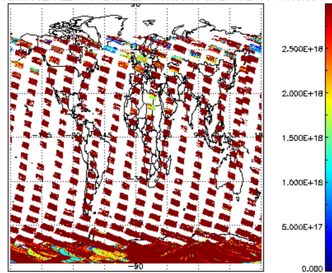
SCIOL2P_NADIR3CO_vcd_err for 26JAN2011 00:00:00 to 27JAN2011 00:00:00
