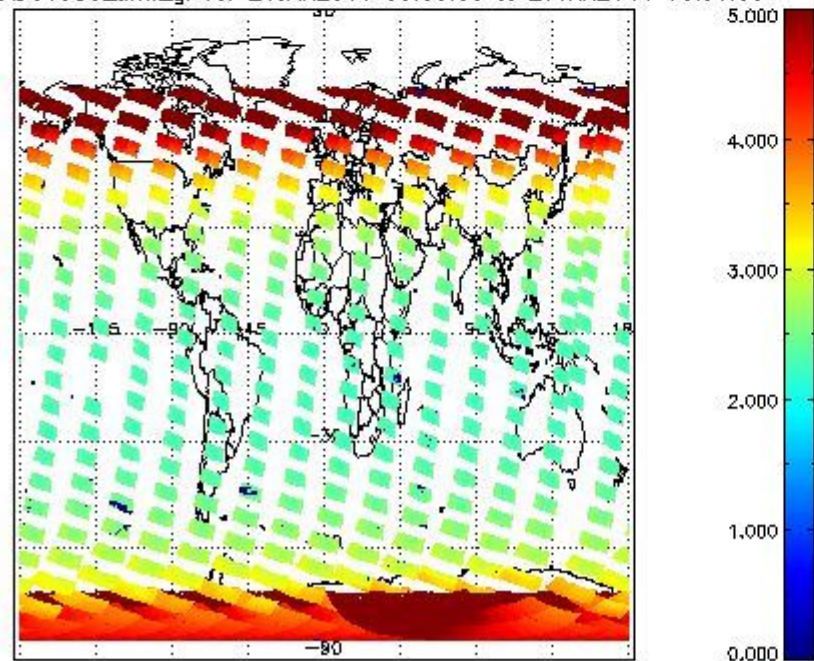
SCIOL2P_NADUV003_amf_gr for 26JAN2011 00:00:00 to 27JAN2011 00:00:00
