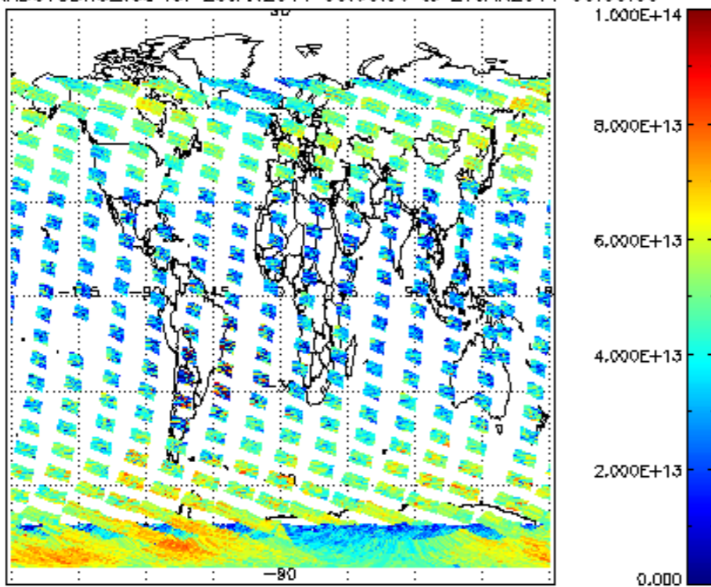
SCIOL2P_NADUV3BRO_vcd for 26JAN2011 00:00:00 to 27JAN2011 00:00:00
