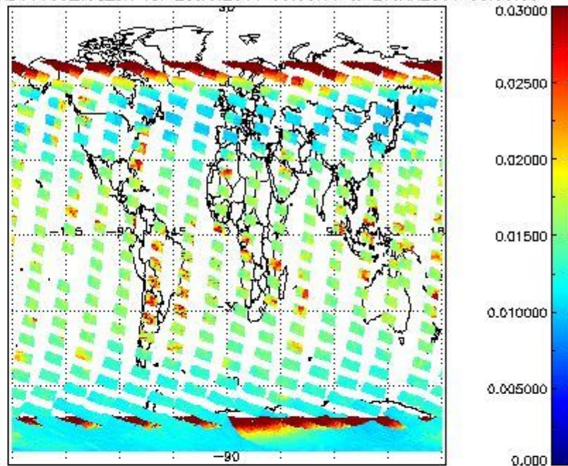
SCIOL2P_NADUV003_vcd_err for 26JAN2011 00:00:00 to 27JAN2011 00:00:00
