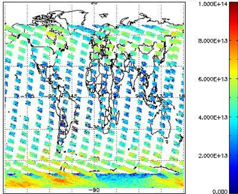
SCIOL2P_NADUV3BRO_vcd for 26JAN2011 00:00:00 to 27JAN2011 00:00:00
