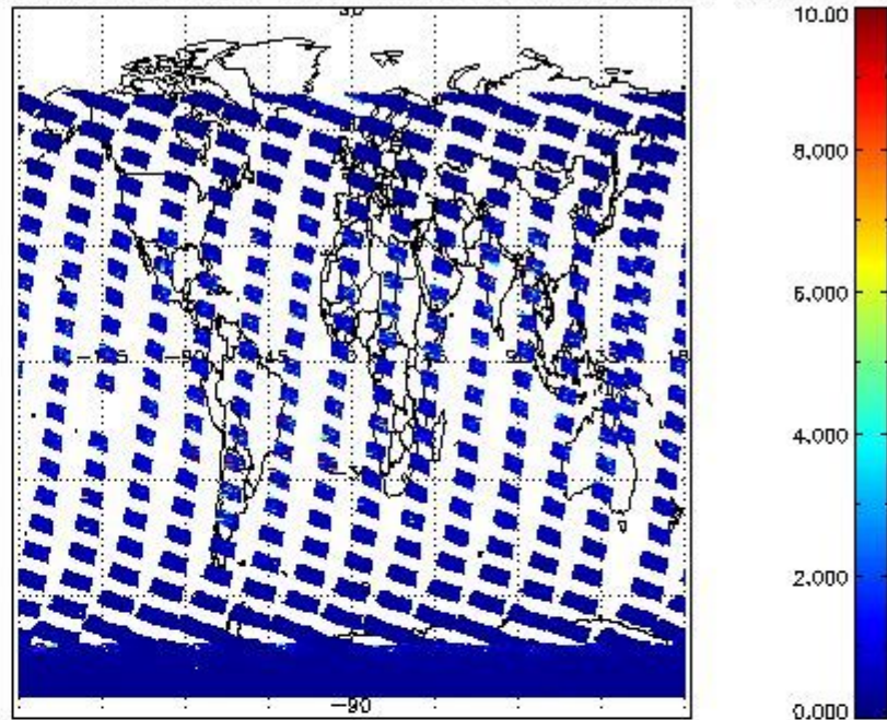
SCIOL2P_NADUV3BRO_vcd_err for 26JAN2011 00:00:00 to 27JAN2011 00:00:00
