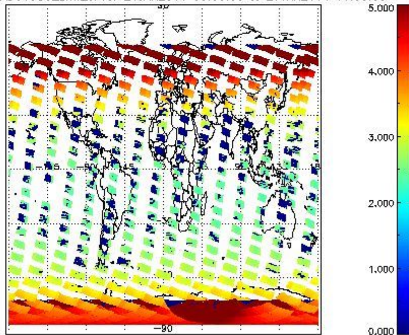
SCIOL2P_NADUV003_amf_cl for 26JAN2011 00:00:00 to 27JAN2011 00:00:00
