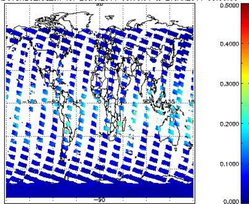
SCIOL2P_NADUV8H20_vcd_err for 26JAN2011 00:00:00 to 27JAN2011 00:00:00
