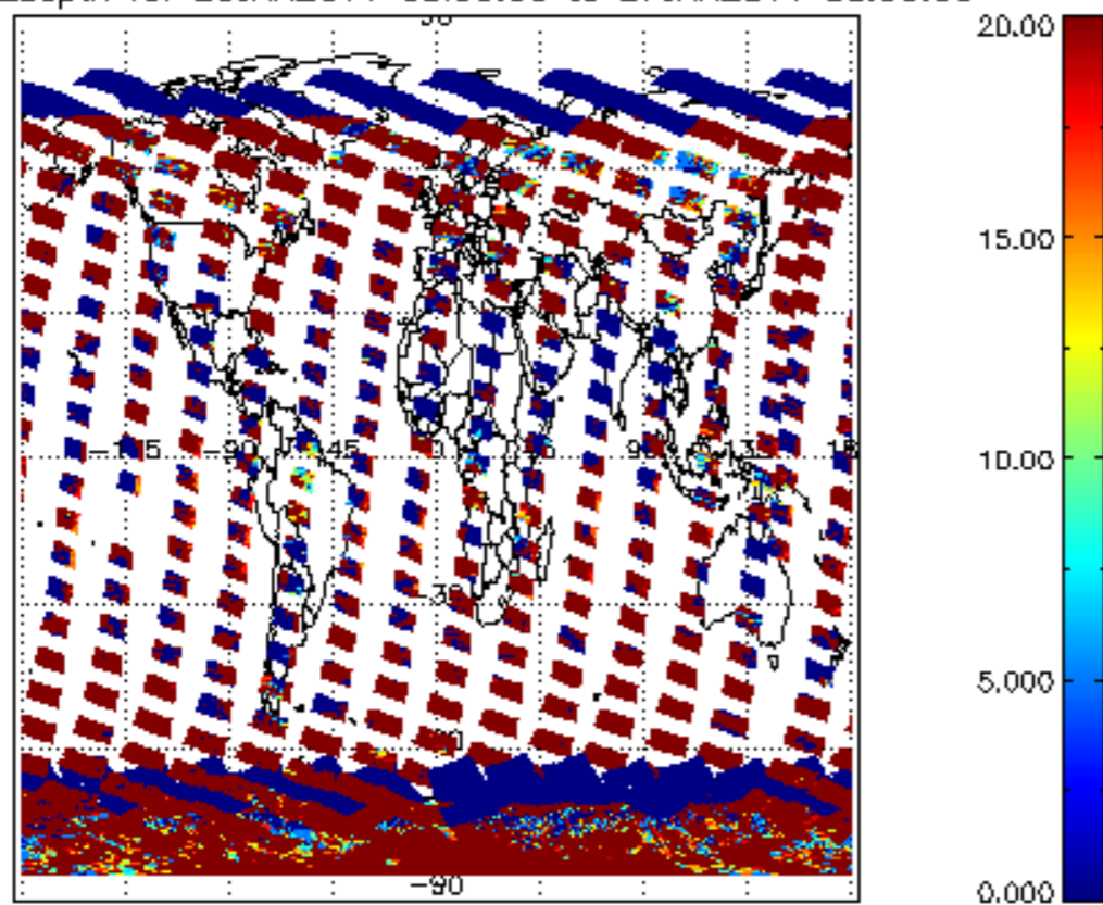
cLopt_depth for 26JAN2011 00:00:00 to 27JAN2011 00:00:00
