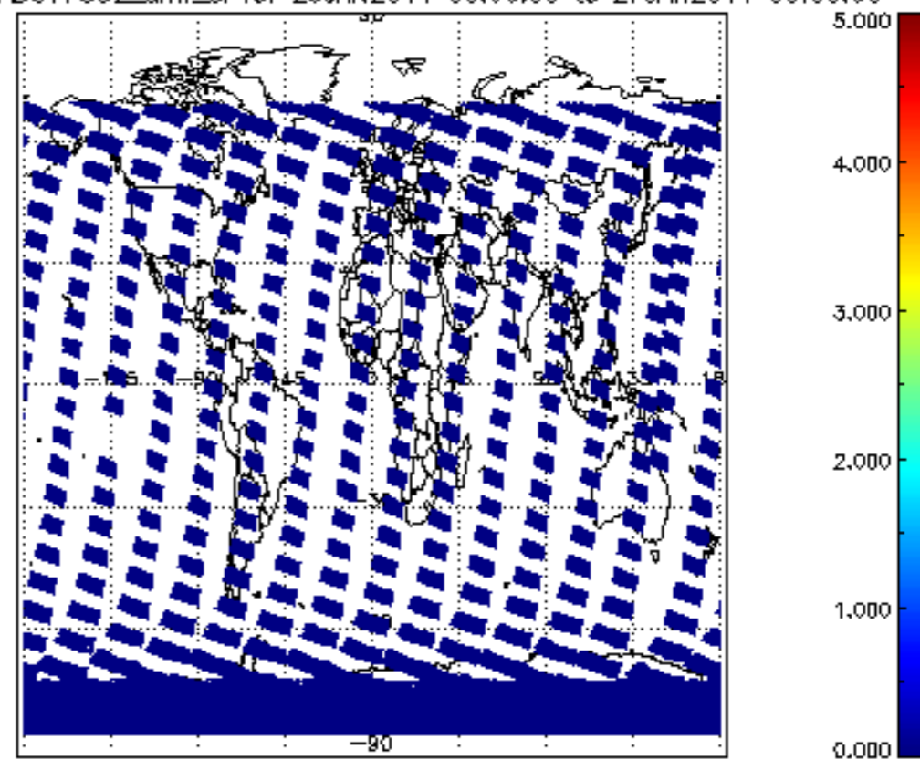
SCIOL2P_NADUV7S02_amf_cl for 26JAN2011 00:00:00 to 27JAN2011 00:00:00
