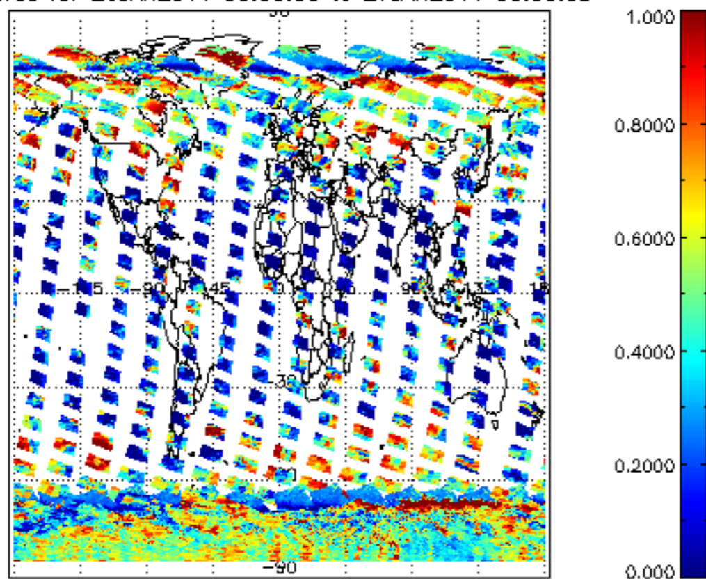
cL_frac for 26JAN2011 00:00:00 to 27JAN2011 00:00:00
