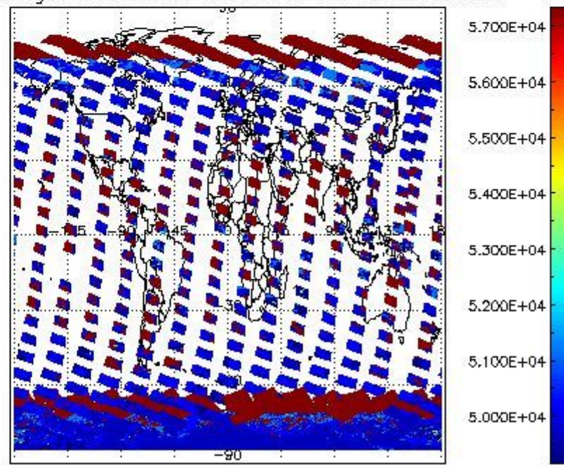
cloud_flags for 26JAN2011 00:00:00 to 27JAN2011 00:00:00
