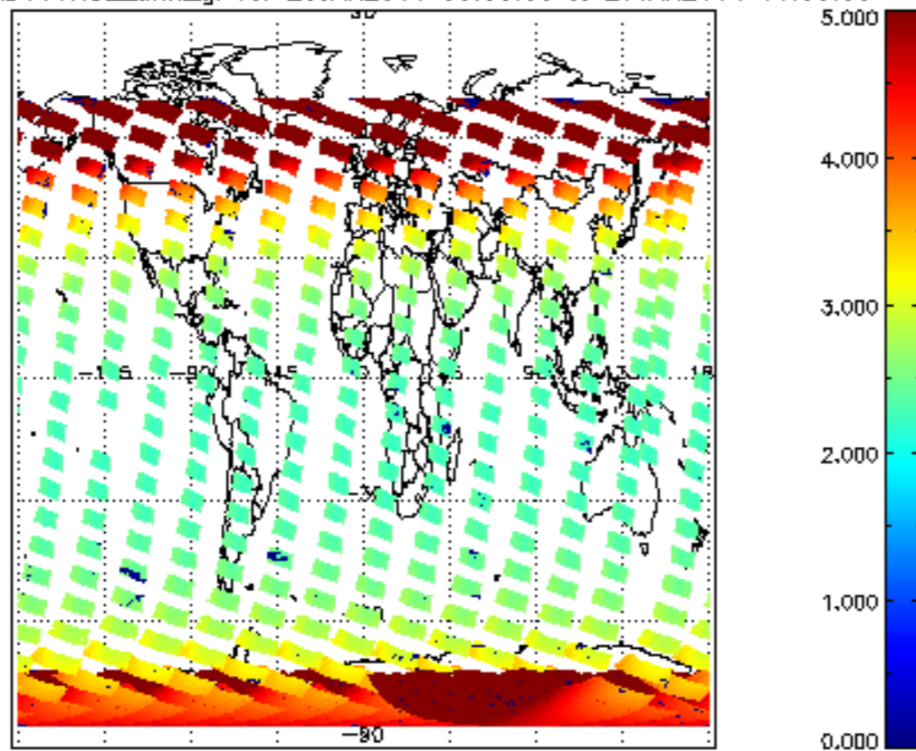
SCIOL2P_NADUV1NO2_amf_gr for 26JAN2011 00:00:00 to 27JAN2011 00:00:00
