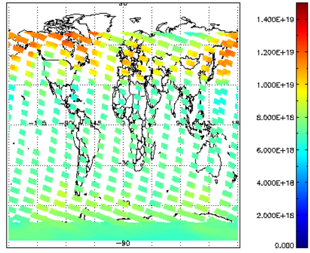
SCIOL2P_NADUV003_vcd for 26JAN2011 00:00:00 to 27JAN2011 00:00:00
