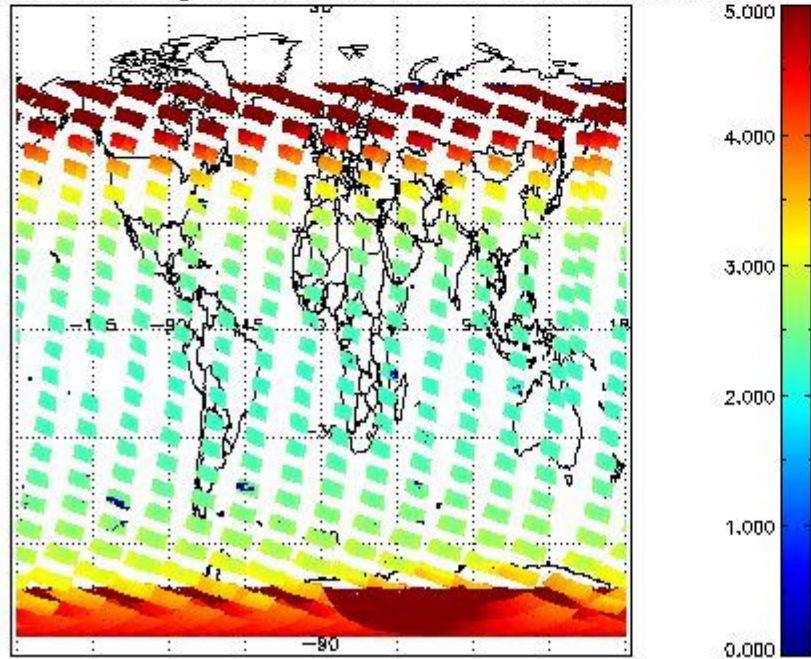
SCIOL2P_NADUV3BRO_amf_gr for 26JAN2011 00:00:00 to 27JAN2011 00:00:00
