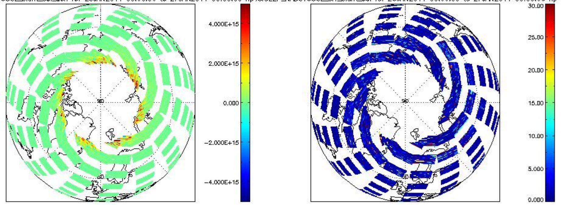
SCIOI2P_NADUV60CL_slant_col_den for 26JAN2011 00:00:00 to 27JAN2011 00:00:00 np; SCIOI2P_NADUV60CL_err_slant_col for 26JAN2011 00:00:00 to 27JAN2011 00:00:00 np
