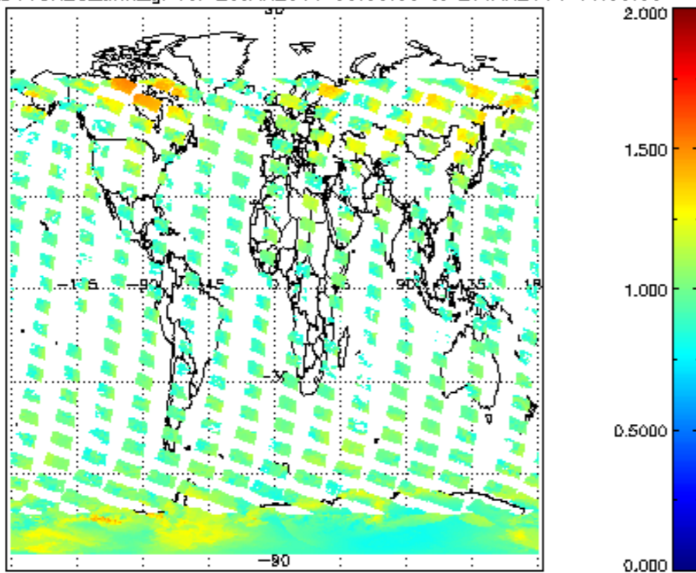
SCIOL2P_NADUV8H20_amf_gr for 26JAN2011 00:00:00 to 27JAN2011 00:00:00
