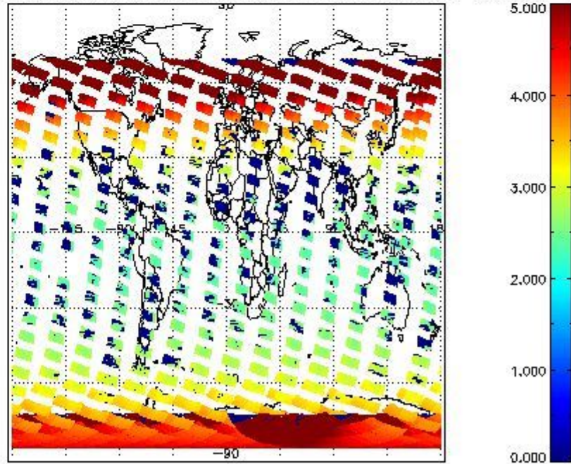
SCIOL2P_NADUV3BRO_amf_cl for 26JAN2011 00:00:00 to 27JAN2011 00:00:00
