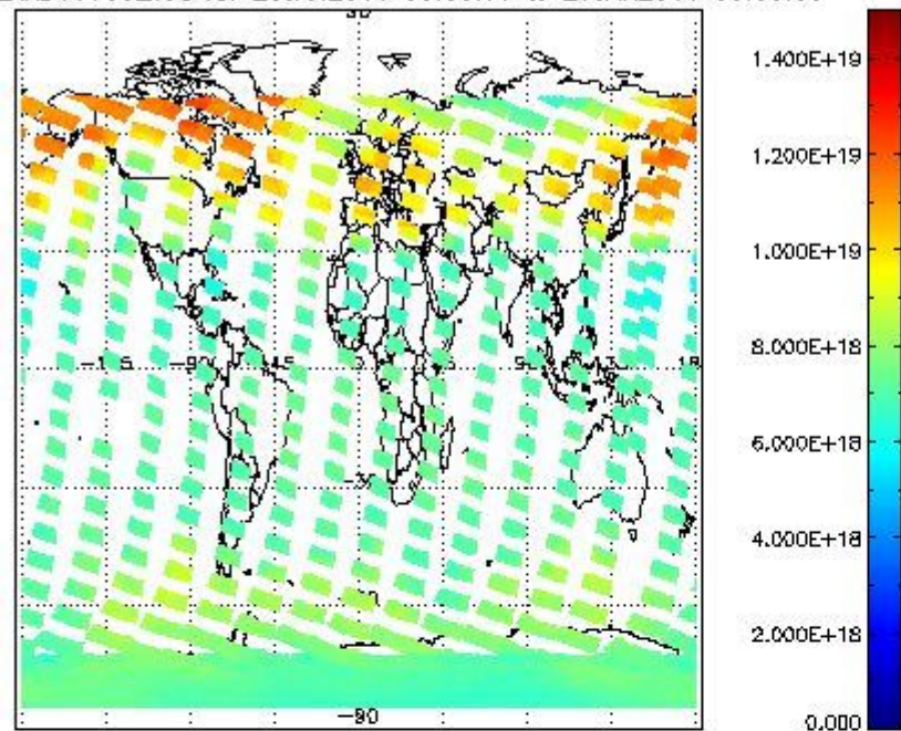
SCIOL2P_NADUV003_vcd for 26JAN2011 00:00:00 to 27JAN2011 00:00:00
