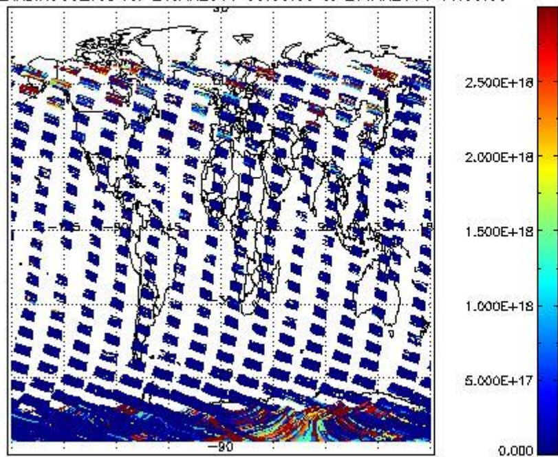
SCIDL2P_NADIR3CO_vcd for 26JAN2011 00:00:00 to 27JAN2011 00:00:00
