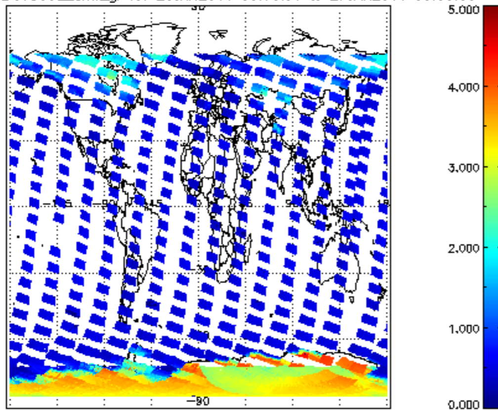
SCIOL2P_NADUV5S02_amf_gr for 26JAN2011 00:00:00 to 27JAN2011 00:00:00
