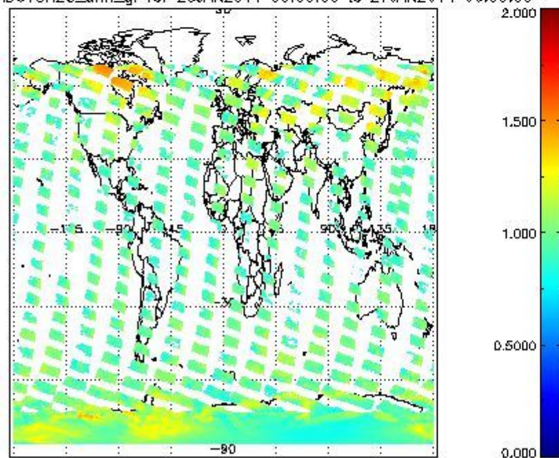
SCIOL2P_NADUV8H20_amf_gr for 26JAN2011 00:00:00 to 27JAN2011 00:00:00
