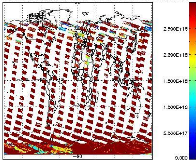
SCIDL2P_NADIR3CO_vcd_err for 26JAN2011 00:00:00 to 27JAN2011 00:00:00
