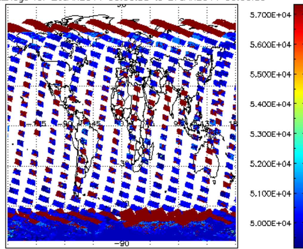
cloud_flags for 26JAN2011 00:00:00 to 27JAN2011 00:00:00
