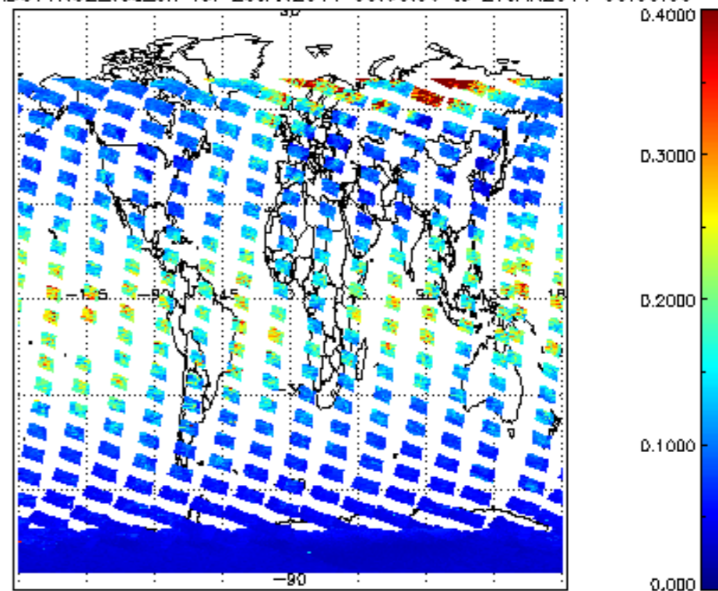
SCIOL2P_NADUV1NO2_vcd_err for 26JAN2011 00:00:00 to 27JAN2011 00:00:00
