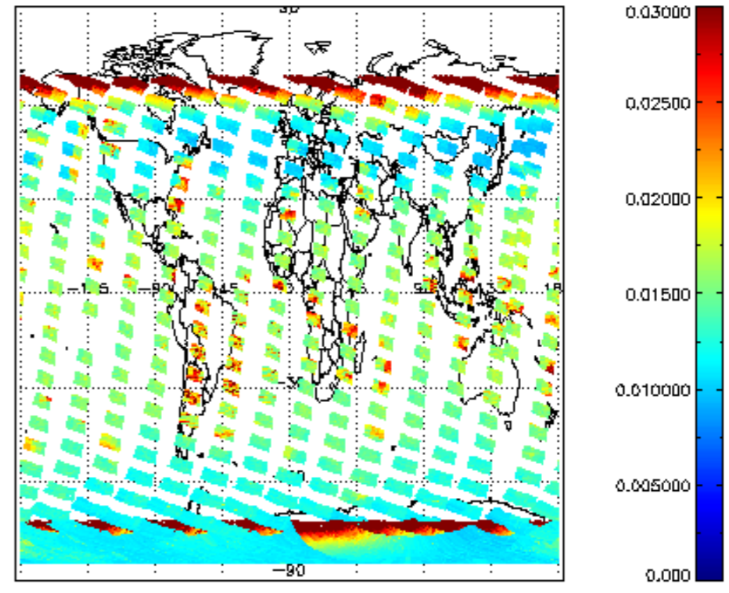
SCIOL2P_NADUV003_vcd_err for 26JAN2011 00:00:00 to 27JAN2011 00:00:00
