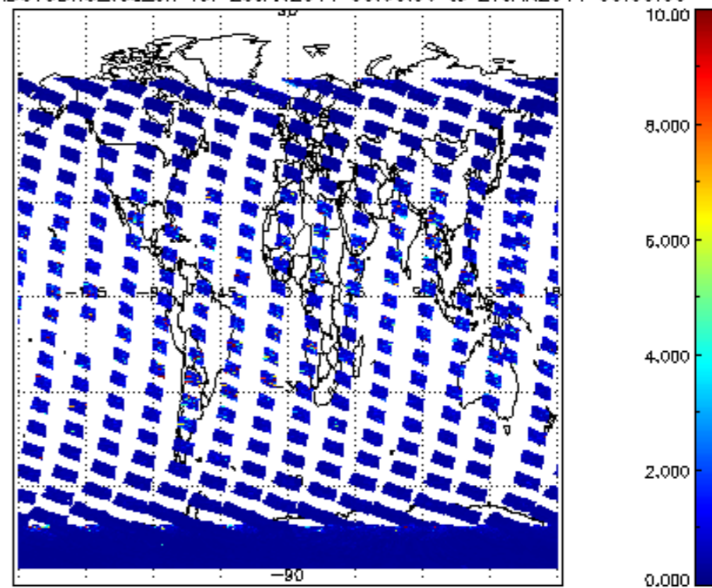
SCIOL2P_NADUV3BRO_vcd_err for 26JAN2011 00:00:00 to 27JAN2011 00:00:00
