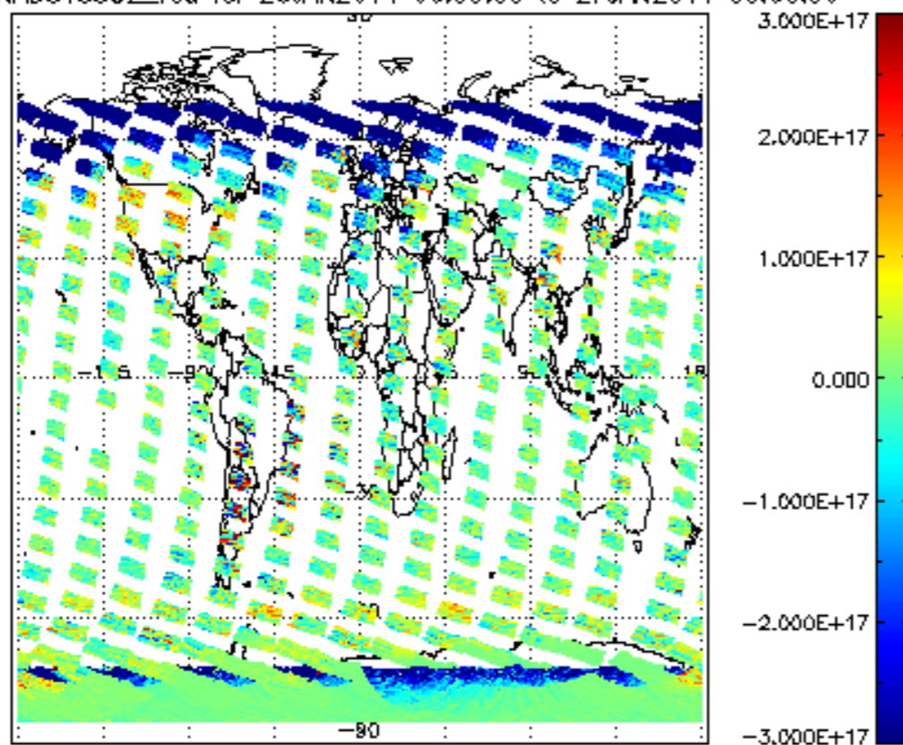
SCIOL2P_NADUV5S02_vcd for 26JAN2011 00:00:00 to 27JAN2011 00:00:00
