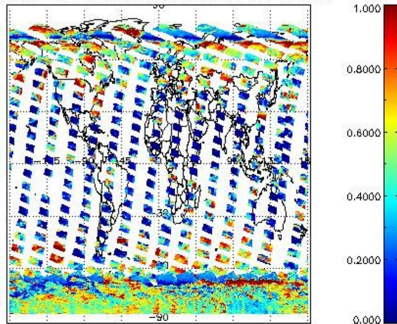
cL_frac for 26JAN2011 00:00:00 to 27JAN2011 00:00:00
