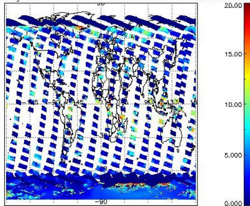
cL_top_height for 26JAN2011 00:00:00 to 27JAN2011 00:00:00
