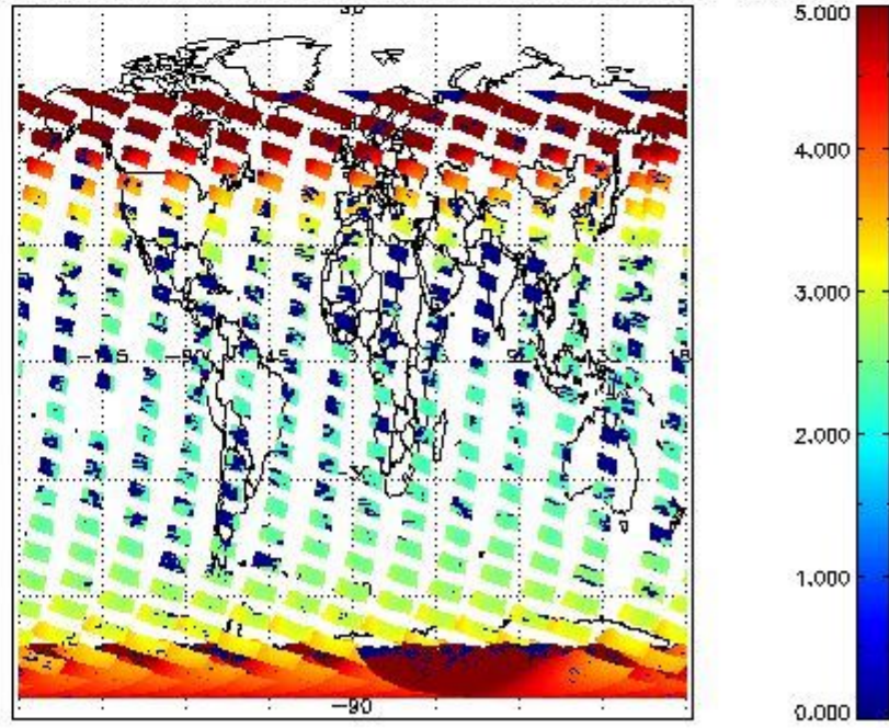
SCIOL2P_NADUV1NO2_amf_cl for 26JAN2011 00:00:00 to 27JAN2011 00:00:00
