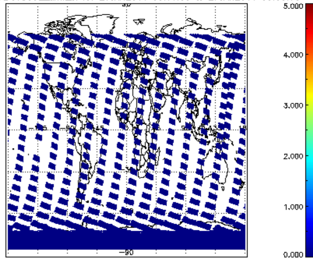
SCIOL2P_NADUV5S02_amf_cl for 26JAN2011 00:00:00 to 27JAN2011 00:00:00
