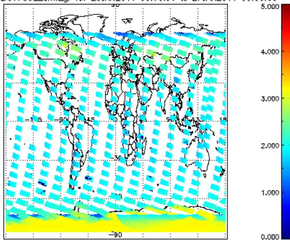
SCIOL2P_NADUV7S02_amf_gr for 26JAN2011 00:00:00 to 27JAN2011 00:00:00
