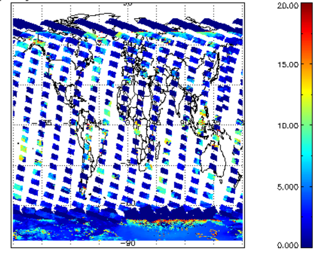
cL_top_height for 23JAN2011 00:00:00 to 24JAN2011 00:00:00
