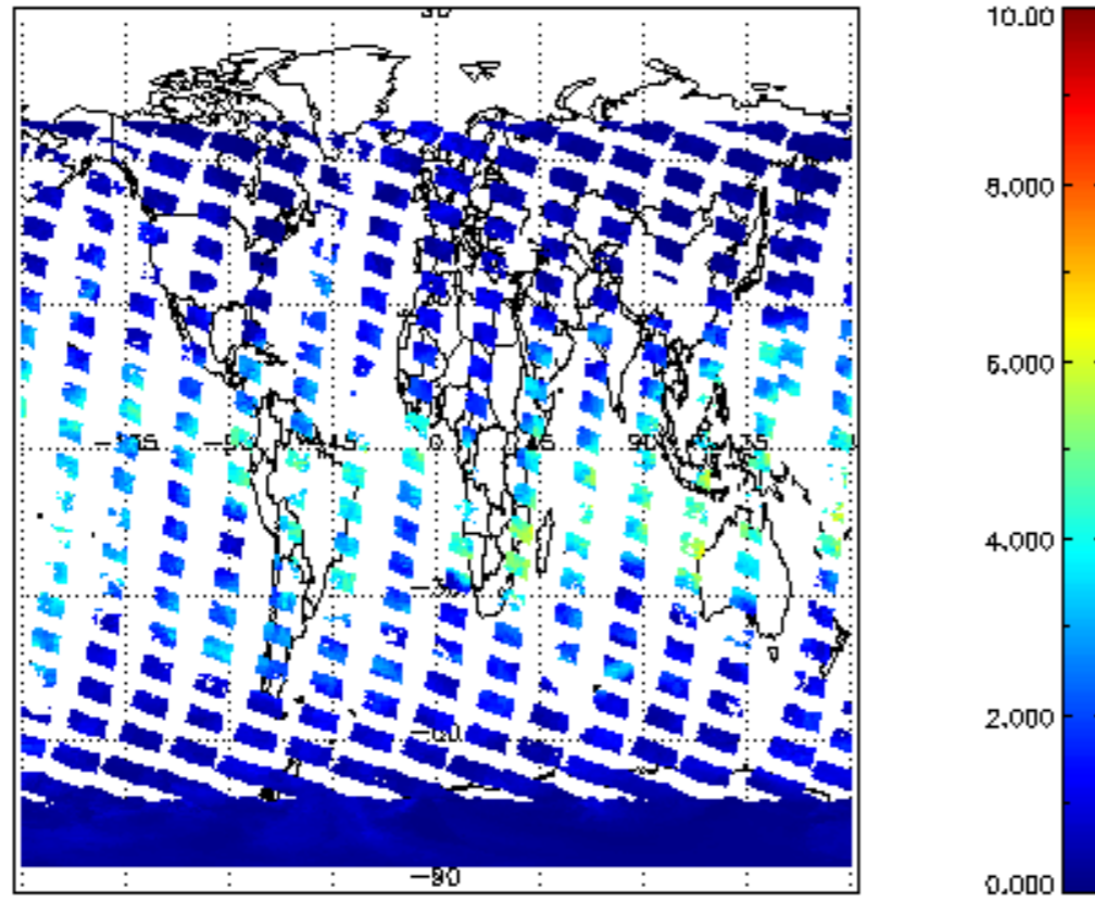
SCIOL2P_NADUV8H20_vcd for 23JAN2011 00:00:00 to 24JAN2011 00:00:00
