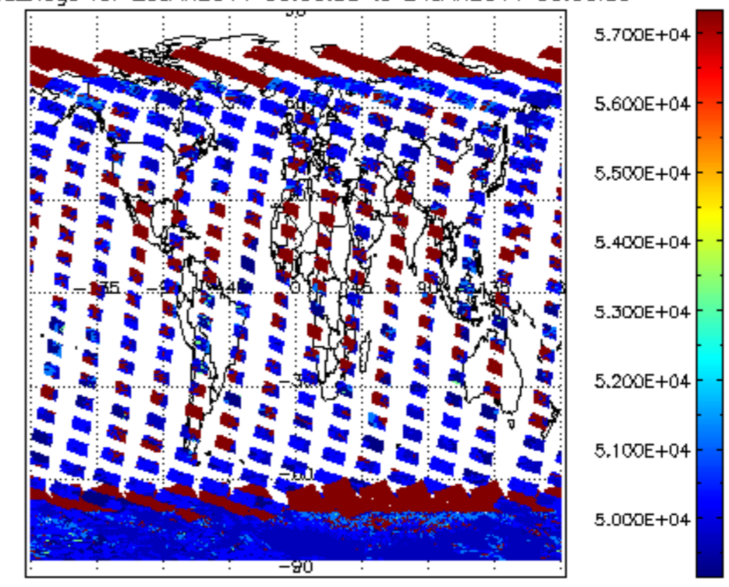
cloud_flags for 23JAN2011 00:00:00 to 24JAN2011 00:00:00
