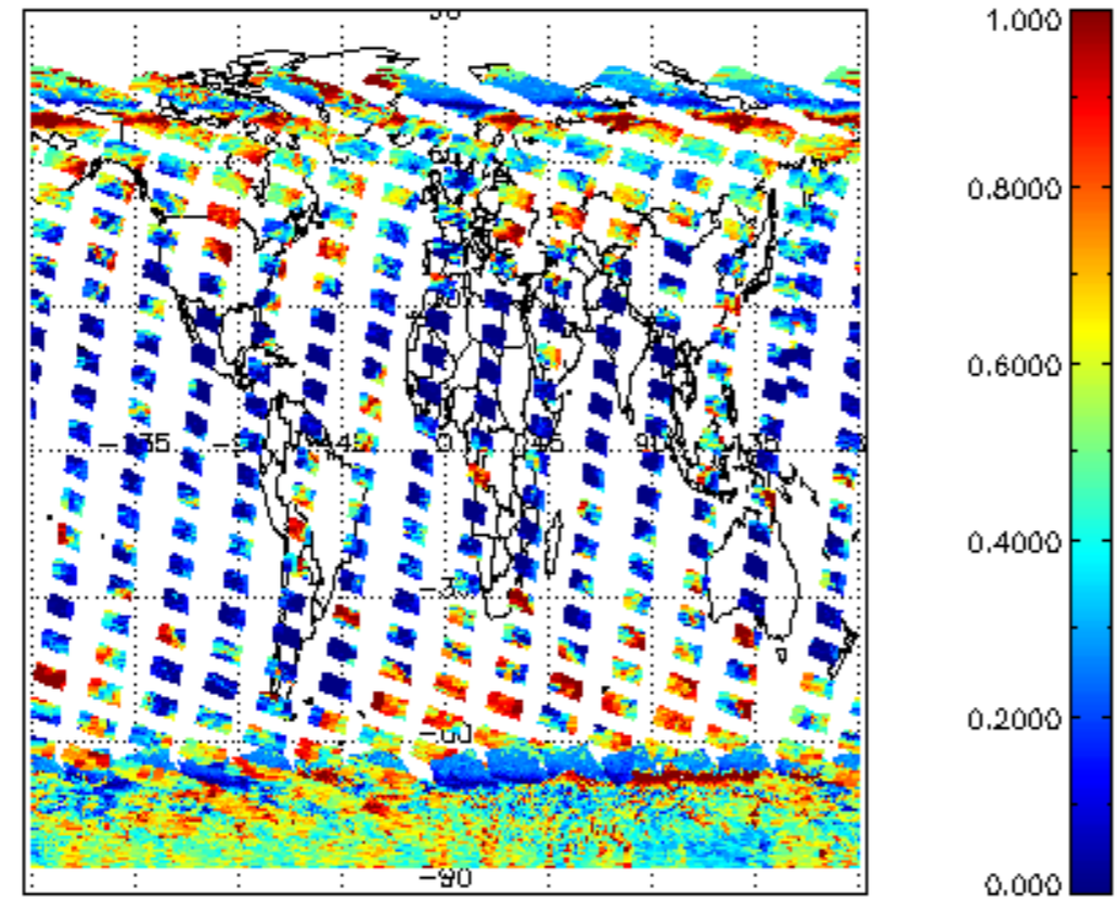
cL_frac for 23JAN2011 00:00:00 to 24JAN2011 00:00:00
