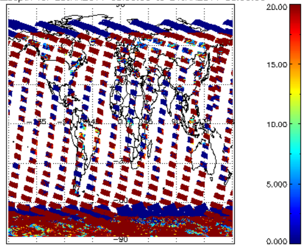
cLopt_depth for 23JAN2011 00:00:00 to 24JAN2011 00:00:00
