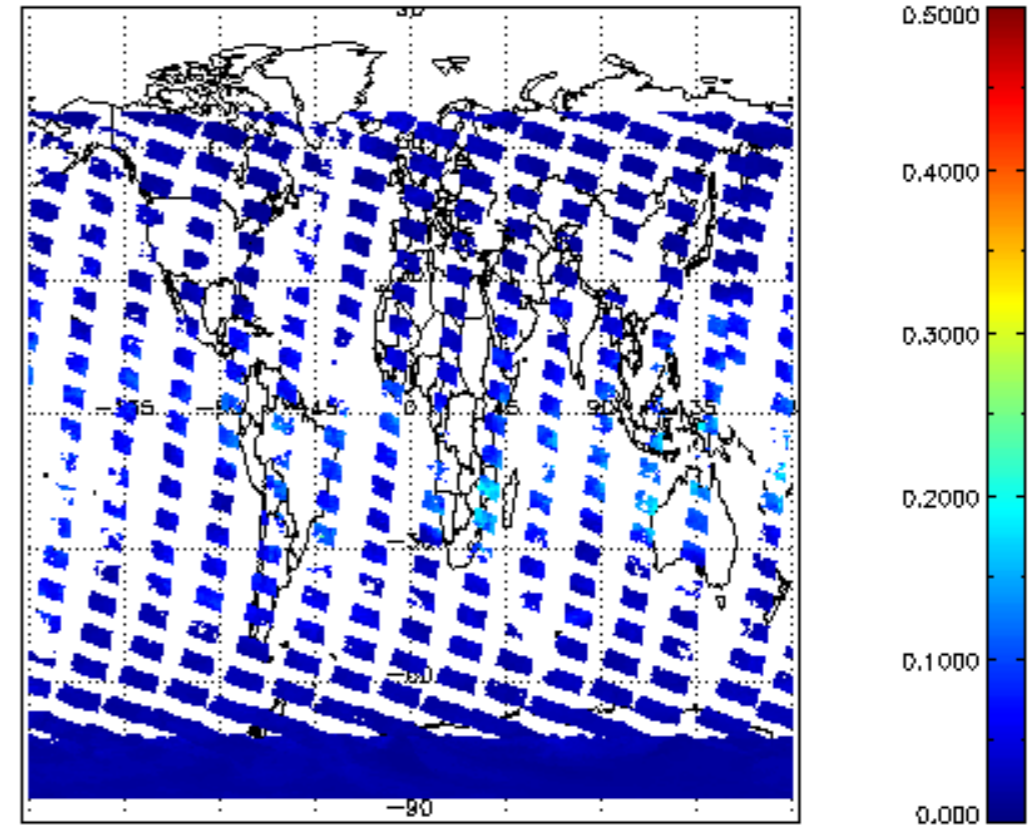
SCIOL2P_NADUV8H20_vcd_err for 23JAN2011 00:00:00 to 24JAN2011 00:00:00
