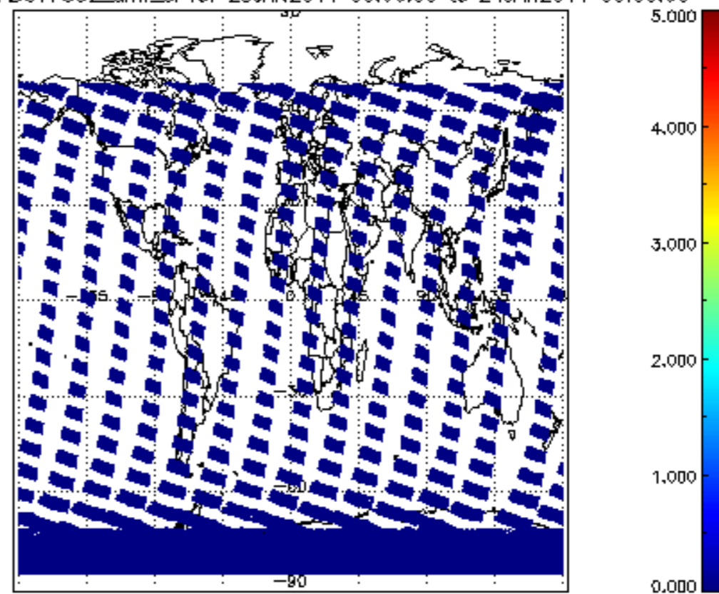
SCIOL2P_NADUV7S02_amf_cl for 23JAN2011 00:00:00 to 24JAN2011 00:00:00
