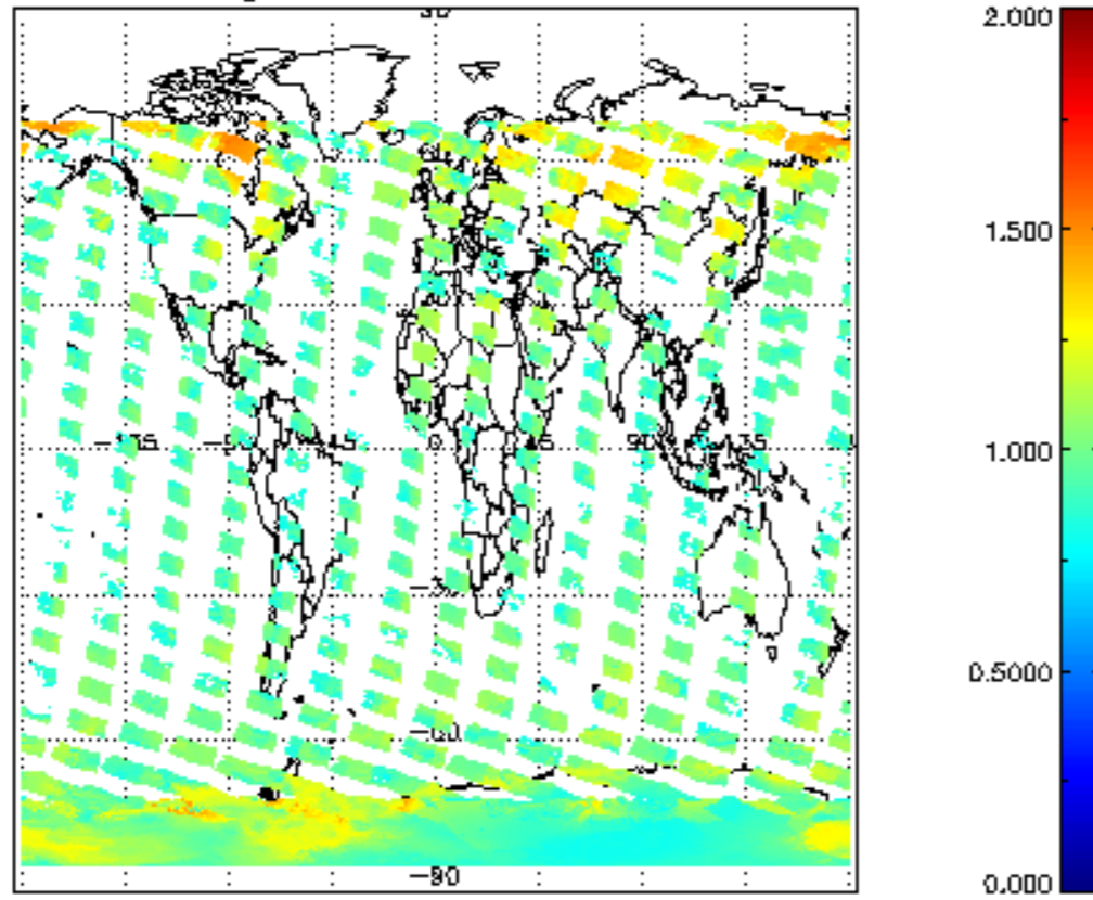
SCIOL2P_NADUV8H20_amf_gr for 23JAN2011 00:00:00 to 24JAN2011 00:00:00
