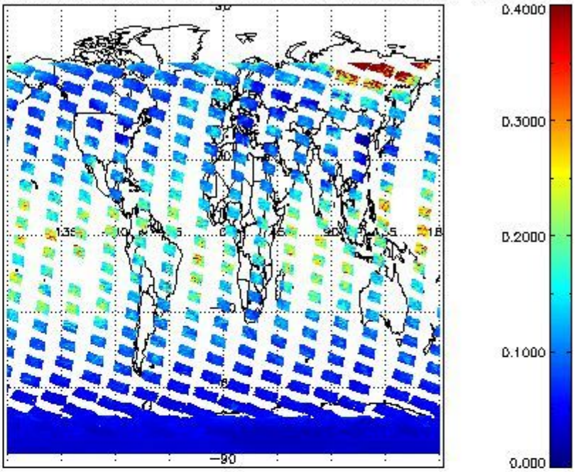
SCIOL2P_NADUV1NO2_vcd_err for 22JAN2011 00:00:00 to 23JAN2011 00:00:00
