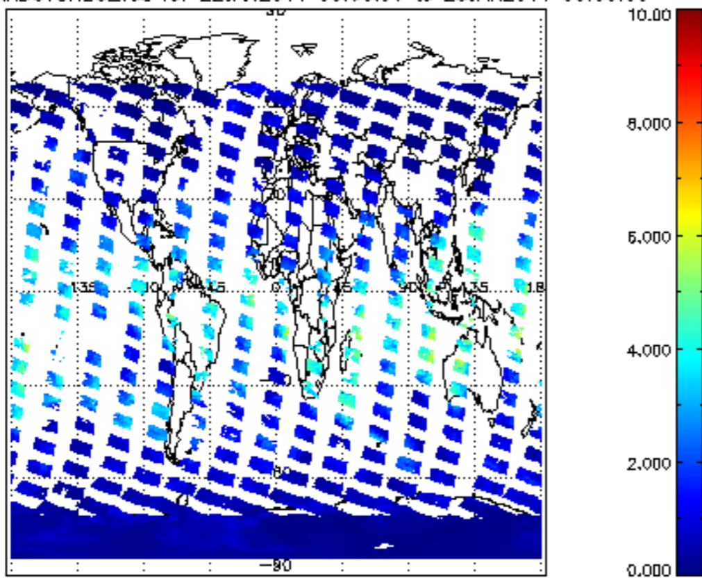
SCIOL2P_NADUV8H20_vcd for 22JAN2011 00:00:00 to 23JAN2011 00:00:00
