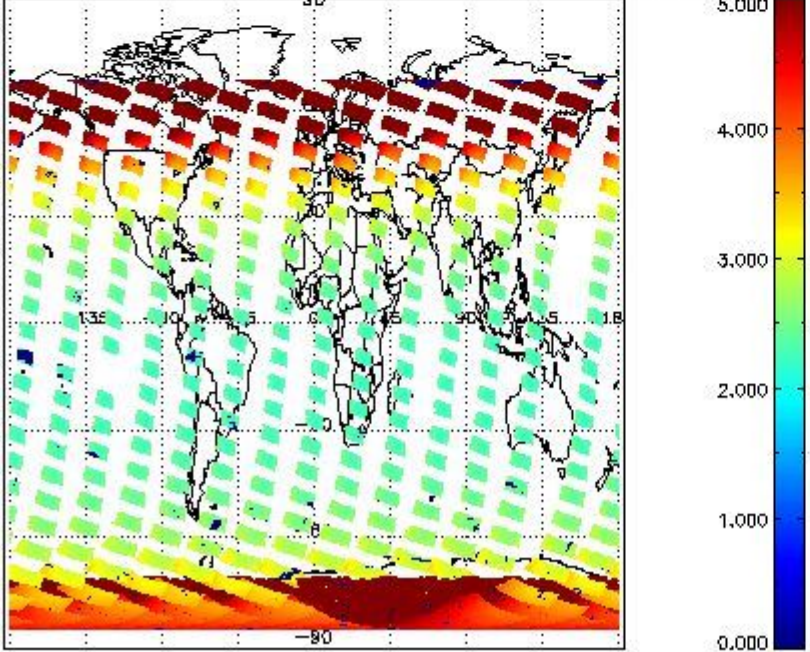
SCIOL2P_NADUV1NO2_amf_gr for 22JAN2011 00:00:00 to 23JAN2011 00:00:00
