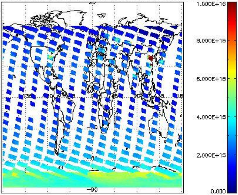
SCIOL2P_NADUV1NO2_vcd for 22JAN2011 00:00:00 to 23JAN2011 00:00:00
