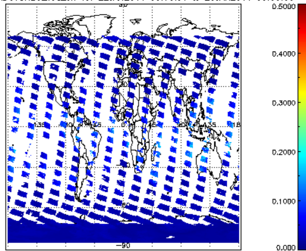
SCIOL2P_NADUV8H20_vcd_err for 22JAN2011 00:00:00 to 23JAN2011 00:00:00
