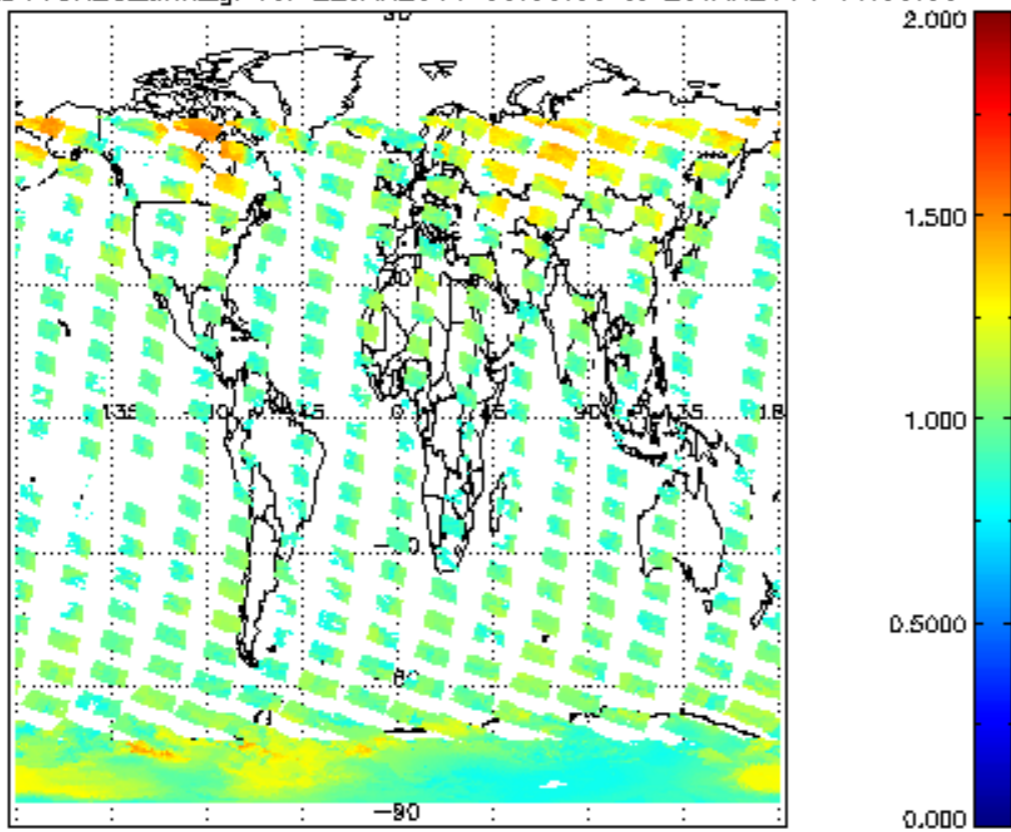
SCIOL2P_NADUV8H20_amf_gr for 22JAN2011 00:00:00 to 23JAN2011 00:00:00
