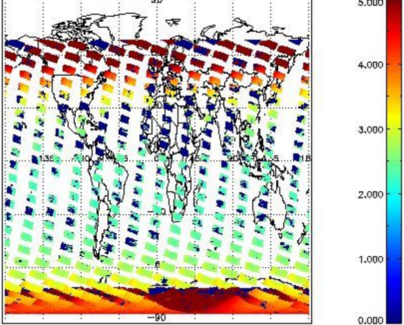
SCIOL2P_NADUV1NO2_amf_cl for 22JAN2011 00:00:00 to 23JAN2011 00:00:00
