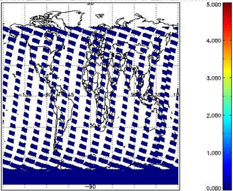
SCIOL2P_NADUV5SO2_amf_cl for 21JAN2011 00:00:00 to 22JAN2011 00:00:00
