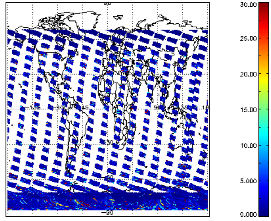
SCIOL2P_NADUV7S02_vcd_err for 21JAN2011 00:00:00 to 22JAN2011 00:00:00
