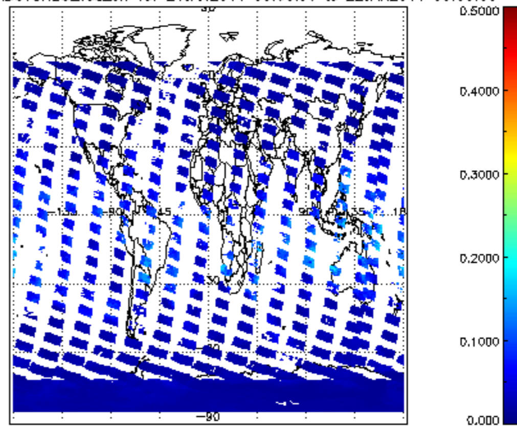
SCIOL2P_NADUV8H20_vcd_err for 21JAN2011 00:00:00 to 22JAN2011 00:00:00
