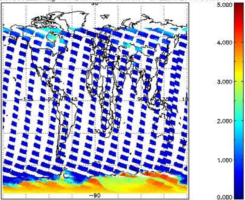
SCIOL2P_NADUV5SO2_amf_gr for 21JAN2011 00:00:00 to 22JAN2011 00:00:00
