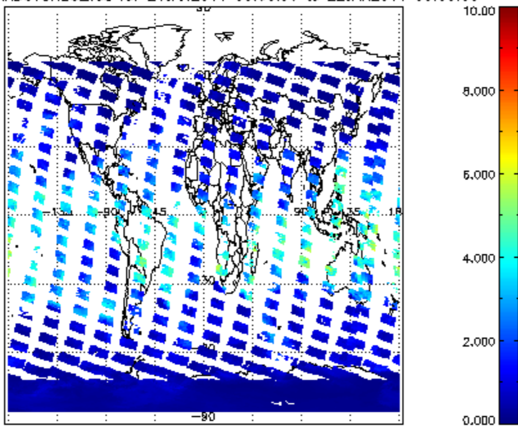
SCIOL2P_NADUV8H20_vcd for 21JAN2011 00:00:00 to 22JAN2011 00:00:00
