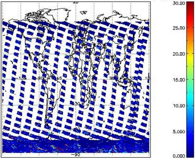
SCIOL2P_NADUV5SO2_vcd_err for 21JAN2011 00:00:00 to 22JAN2011 00:00:00
