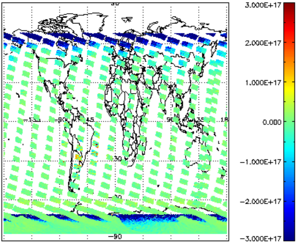
SCIOL2P_NADUV7S02_vcd for 21JAN2011 00:00:00 to 22JAN2011 00:00:00
