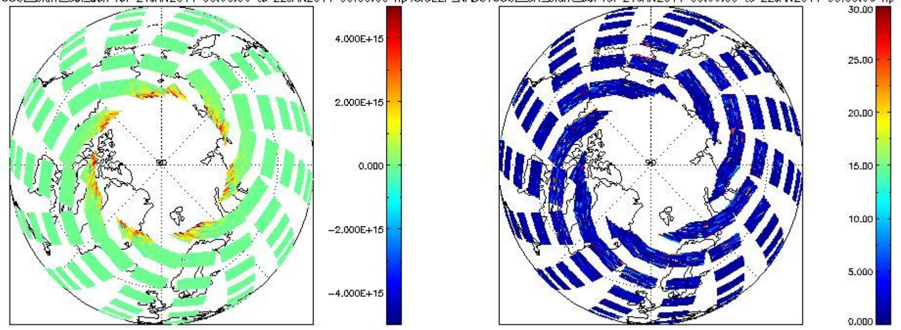
SCIOI2P_NADUV6OCL_slant_col_den for 21JAN2011 00:00:00 to 22JAN2011 00:00:00 np; SCIOI2P_NADUV6OCL_err_slant_col for 21JAN2011 00:00:00 to 22JAN2011 00:00:00 np
