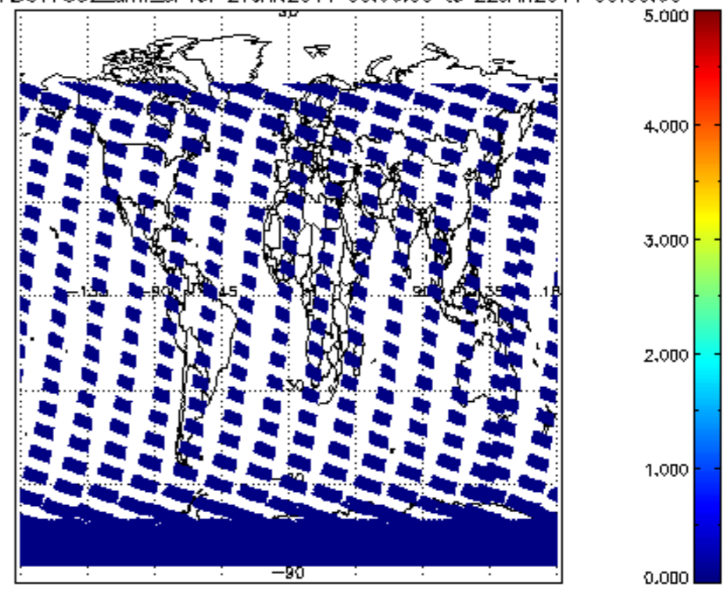
SCIOL2P_NADUV7S02_amf_sl for 21JAN2011 00:00:00 to 22JAN2011 00:00:00
