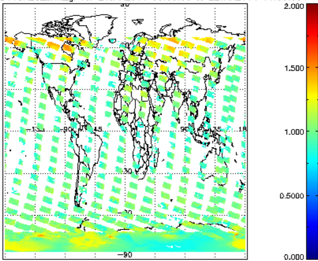
SCIOL2P_NADUV8H20_amf_gr for 21JAN2011 00:00:00 to 22JAN2011 00:00:00
