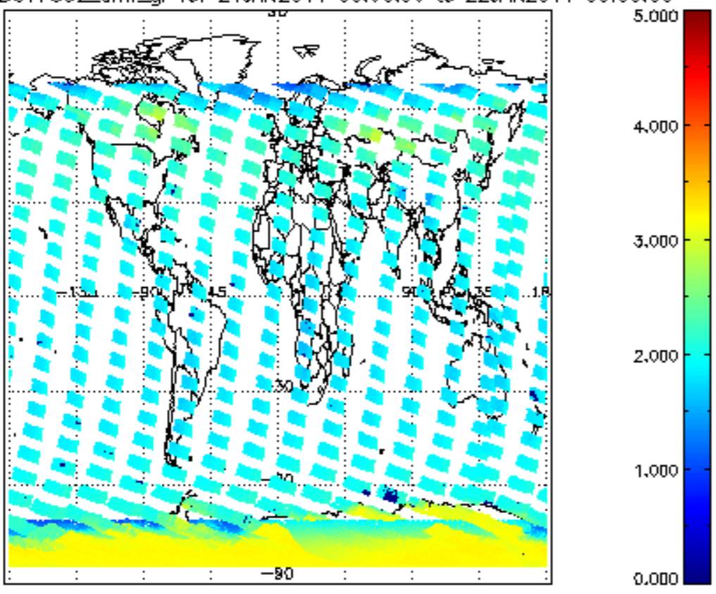
SCIOL2P_NADUV7S02_amf_gr for 21JAN2011 00:00:00 to 22JAN2011 00:00:00
