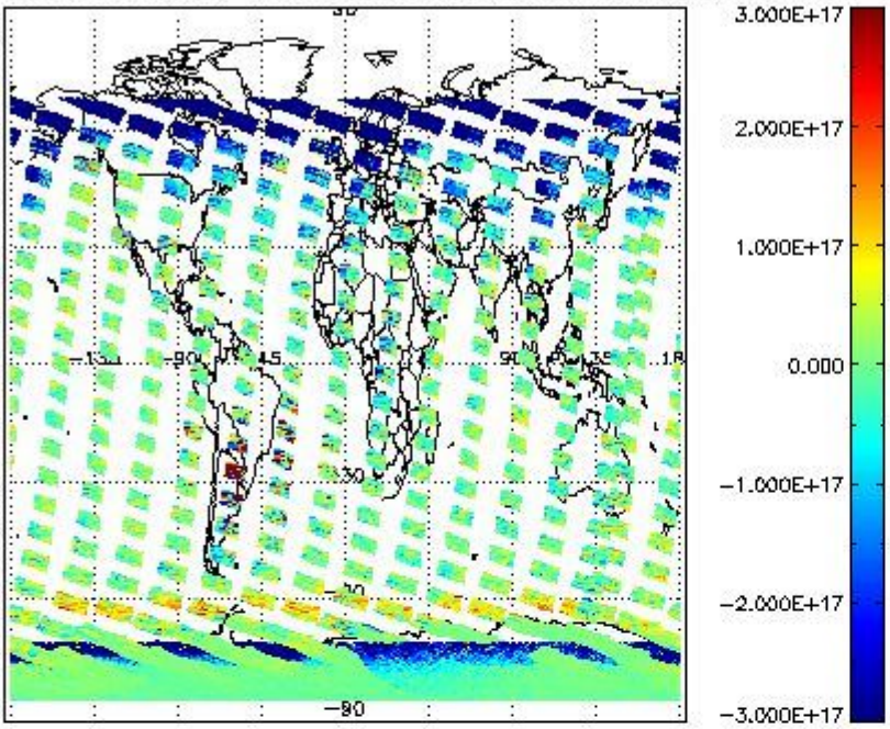
SCIOL2P_NADUV5SO2_vcd for 21JAN2011 00:00:00 to 22JAN2011 00:00:00
