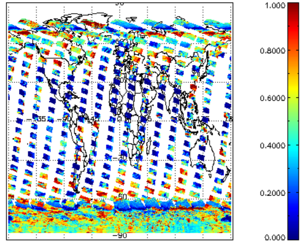
cL_frac for 20JAN2011 00:00:00 to 21JAN2011 00:00:00
