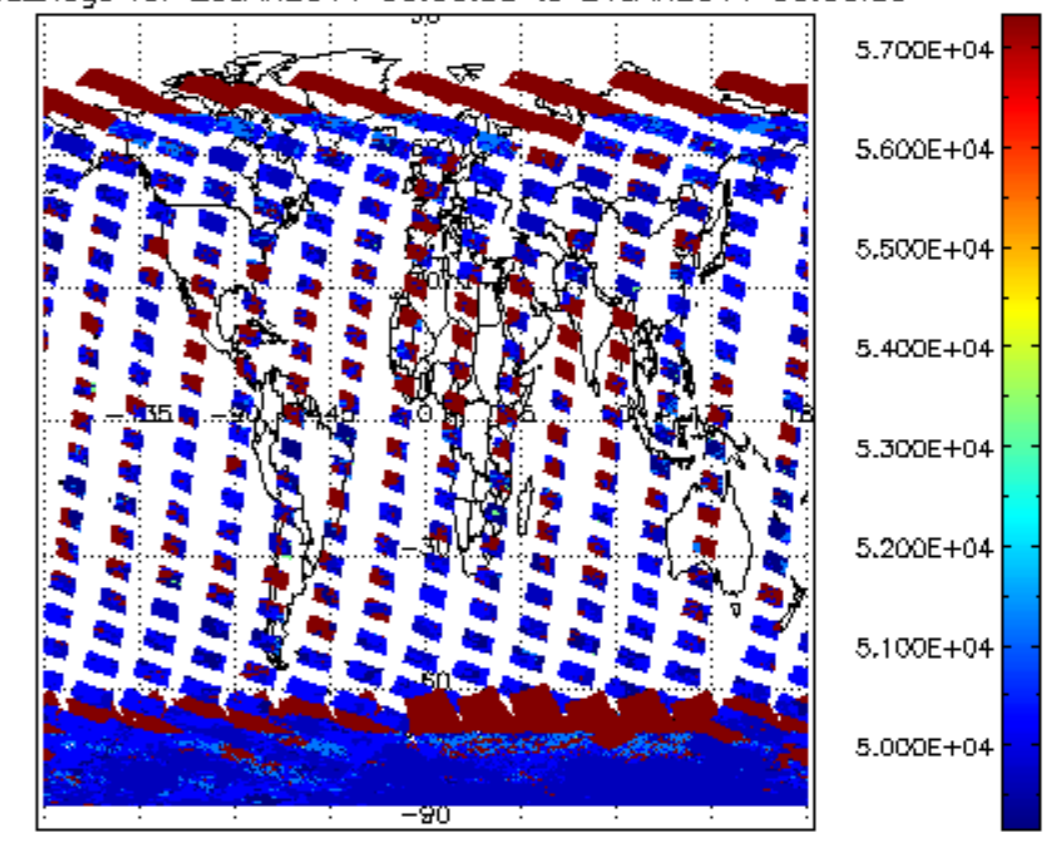
cloud_flags for 20JAN2011 00:00:00 to 21JAN2011 00:00:00
