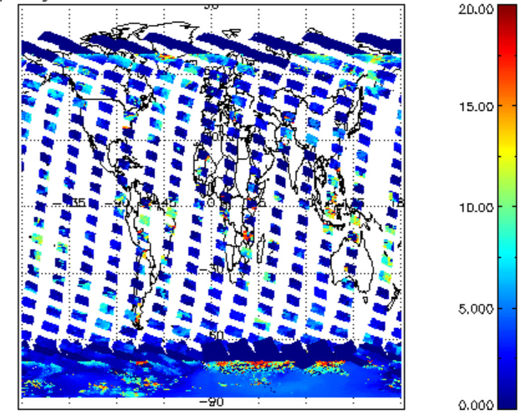
cL_top_height for 20JAN2011 00:00:00 to 21JAN2011 00:00:00
