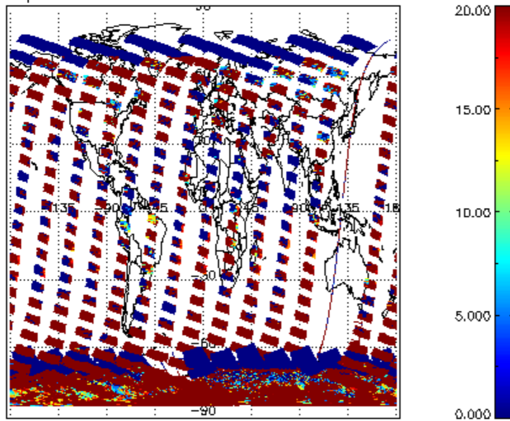
cLopt_depth for 19JAN2011 00:00:00 to 20JAN2011 00:00:00
