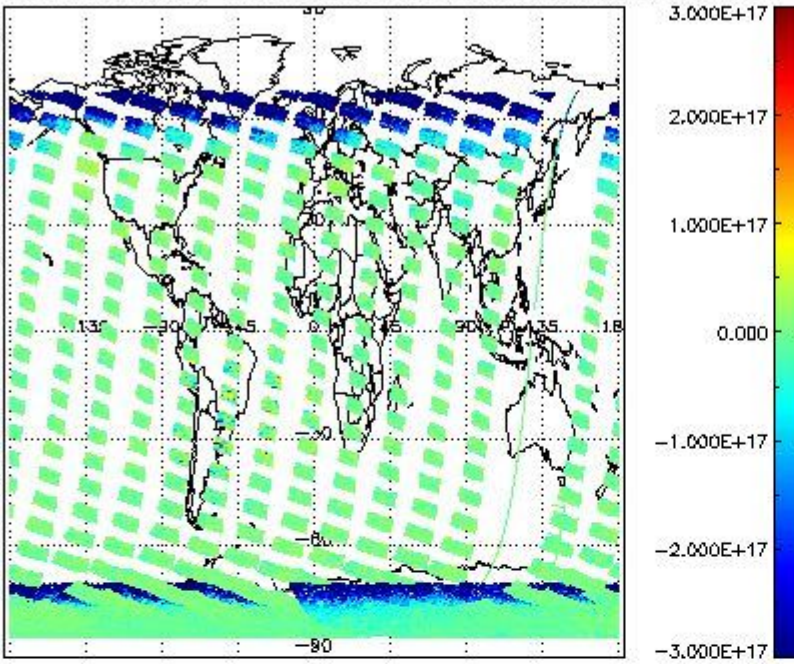
SCIOL2P_NADUV7S02_vcd for 19JAN2011 00:00:00 to 20JAN2011 00:00:00
