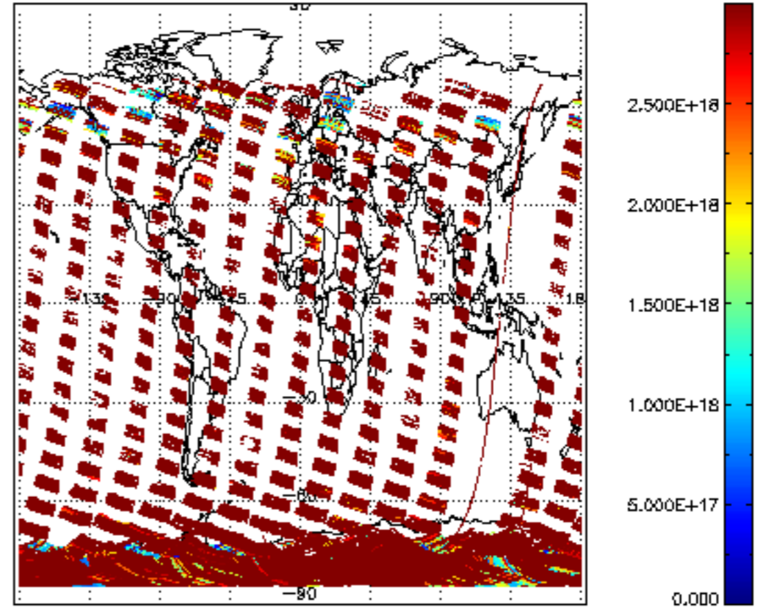
SCIOL2P_NADIR3CO_vcd_err for 19JAN2011 00:00:00 to 20JAN2011 00:00:00
