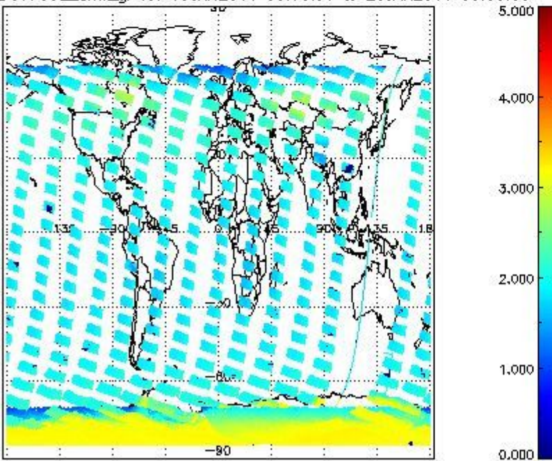
SCIOL2P_NADUV7S02_amf_gr for 19JAN2011 00:00:00 to 20JAN2011 00:00:00
