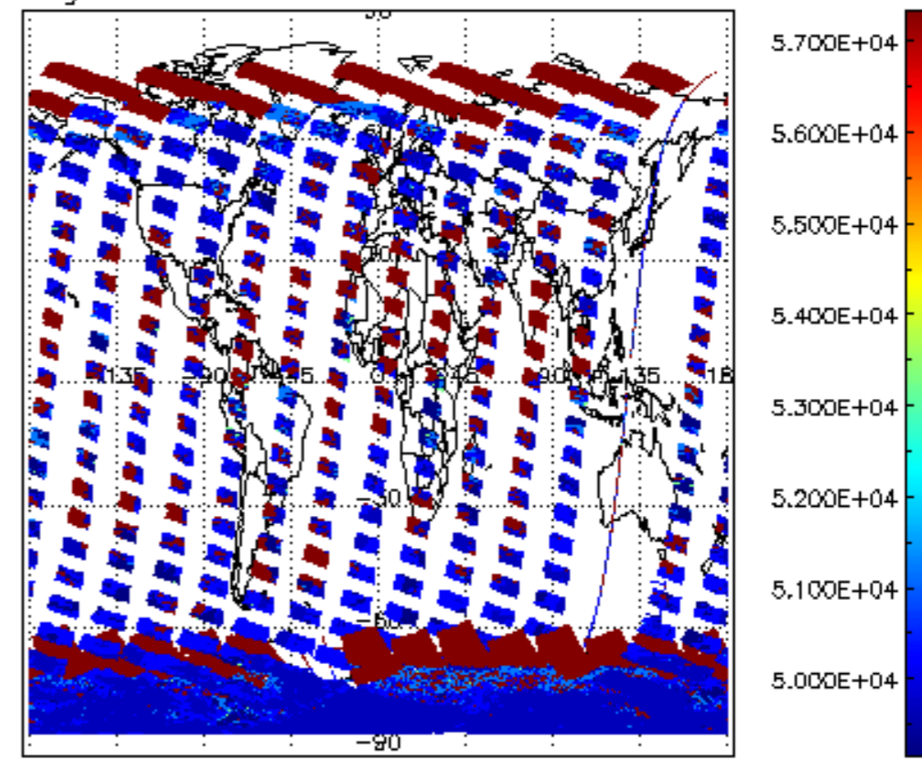
cloud_flags for 19JAN2011 00:00:00 to 20JAN2011 00:00:00
