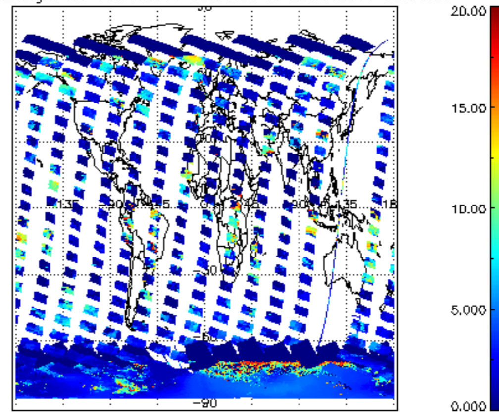
cL_top_height for 19JAN2011 00:00:00 to 20JAN2011 00:00:00
