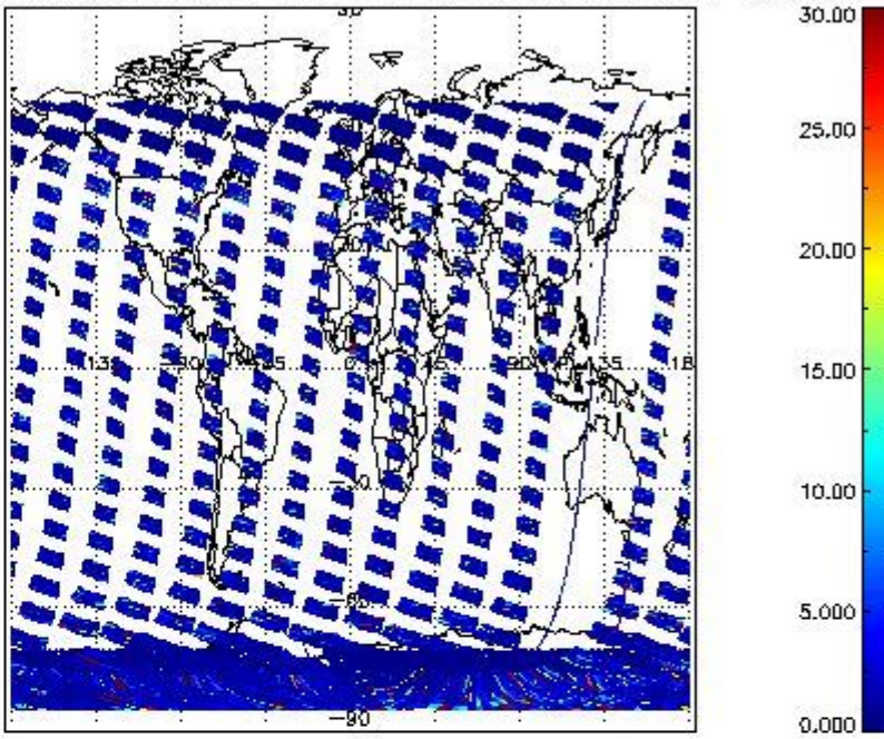
SCIOL2P_NADUV7S02_vcd_err for 19JAN2011 00:00:00 to 20JAN2011 00:00:00
