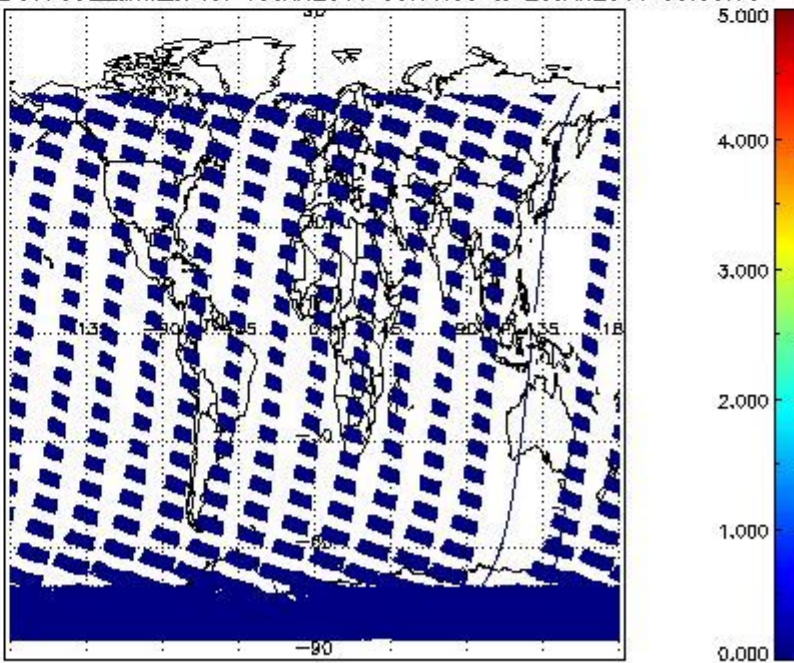
SCIOL2P_NADUV7S02_amf_cl for 19JAN2011 00:00:00 to 20JAN2011 00:00:00
