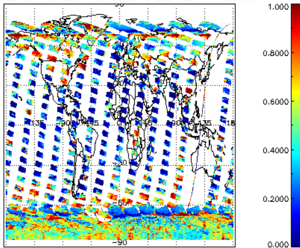
cL_frac for 19JAN2011 00:00:00 to 20JAN2011 00:00:00
