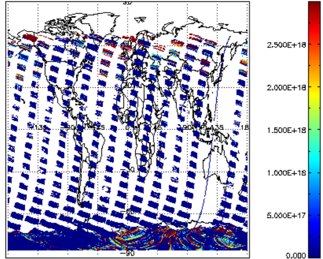
SCIOL2P_NADIR3CO_vcd for 19JAN2011 00:00:00 to 20JAN2011 00:00:00
