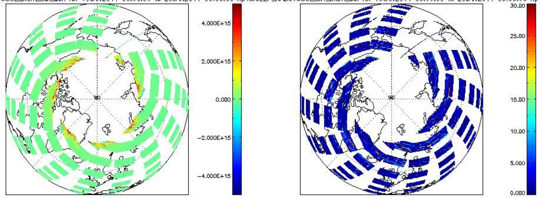
SCIOI2P_NADUV60CL_slant_col_den for 19JAN2011 00:00:00 to 20JAN2011 00:00:00 np; SCIOI2P_NADUV60CL_err_slant_col for 19JAN2011 00:00:00 to 20JAN2011 00:00:00 np
