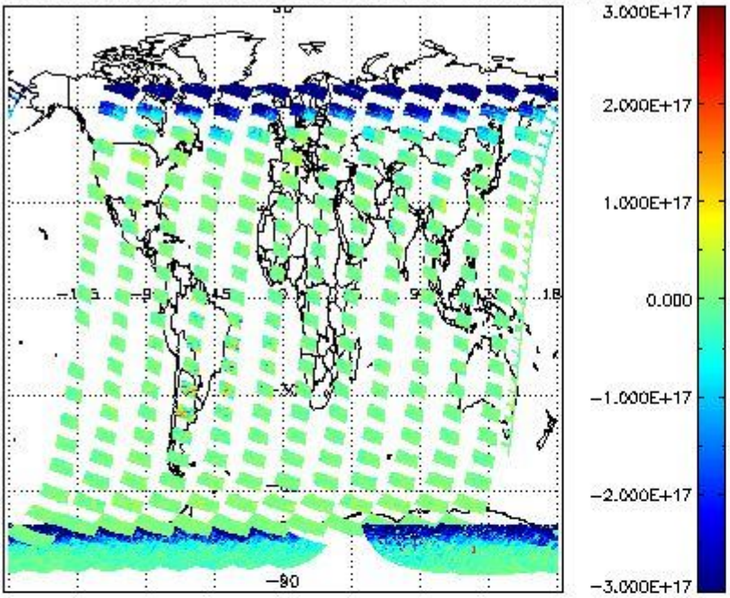
SCIOL2P_NADUV7S02_vcd for 18JAN2011 00:00:00 to 19JAN2011 00:00:00
