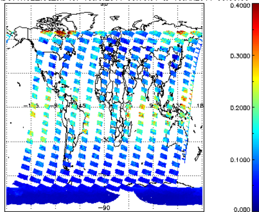
SCIOL2P_NADUV1NO2_vcd_err for 18JAN2011 00:00:00 to 19JAN2011 00:00:00
