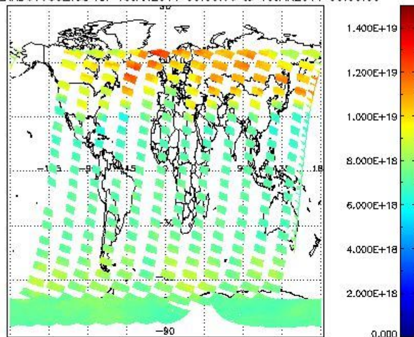
SCIOL2P_NADUV003_vcd for 18JAN2011 00:00:00 to 19JAN2011 00:00:00
