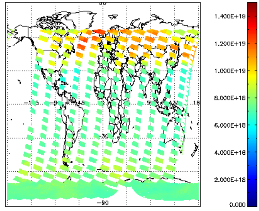
SCIOL2P_NADUV003_vcd for 18JAN2011 00:00:00 to 19JAN2011 00:00:00
