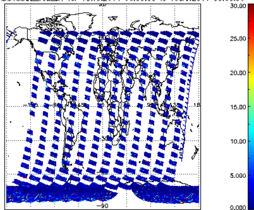
SCIOL2P_NADUV5S02_vcd_err for 18JAN2011 00:00:00 to 19JAN2011 00:00:00
