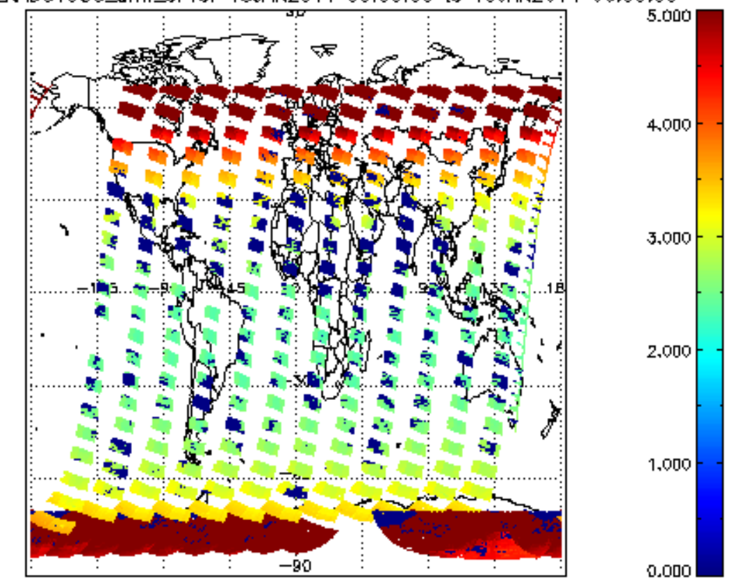
SCIOL2P_NADUV003_amf_cl for 18JAN2011 00:00:00 to 19JAN2011 00:00:00
