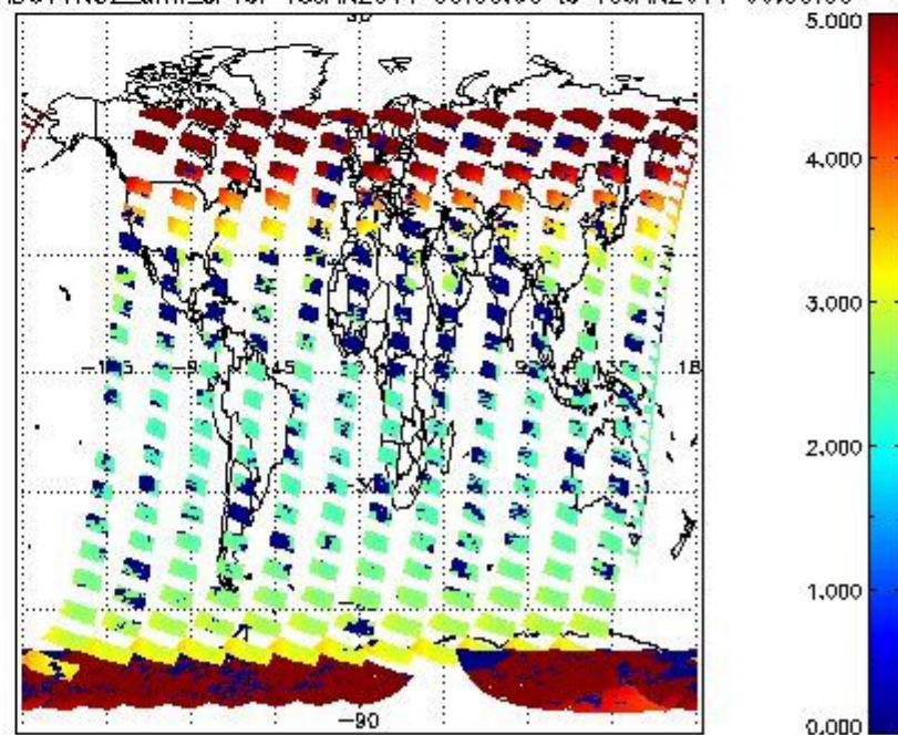
SCIOL2P_NADUV1NO2_amf_cl for 18JAN2011 00:00:00 to 19JAN2011 00:00:00
