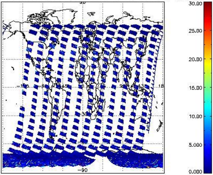
SCIOL2P_NADUV7S02_vcd_err for 18JAN2011 00:00:00 to 19JAN2011 00:00:00
