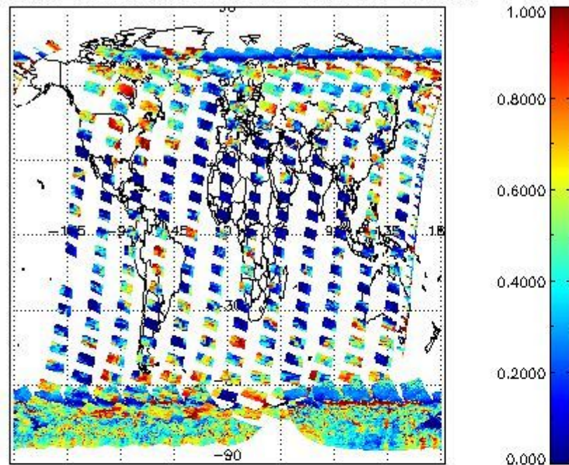
cL_frac for 18JAN2011 00:00:00 to 19JAN2011 00:00:00
