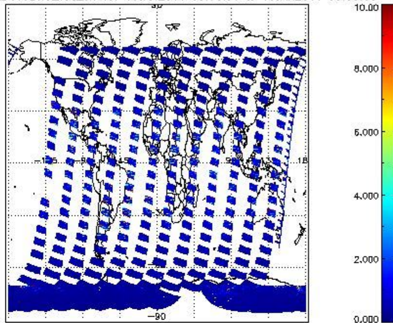
SCIOL2P_NADUV3BRO_vcd_err for 18JAN2011 00:00:00 to 19JAN2011 00:00:00
