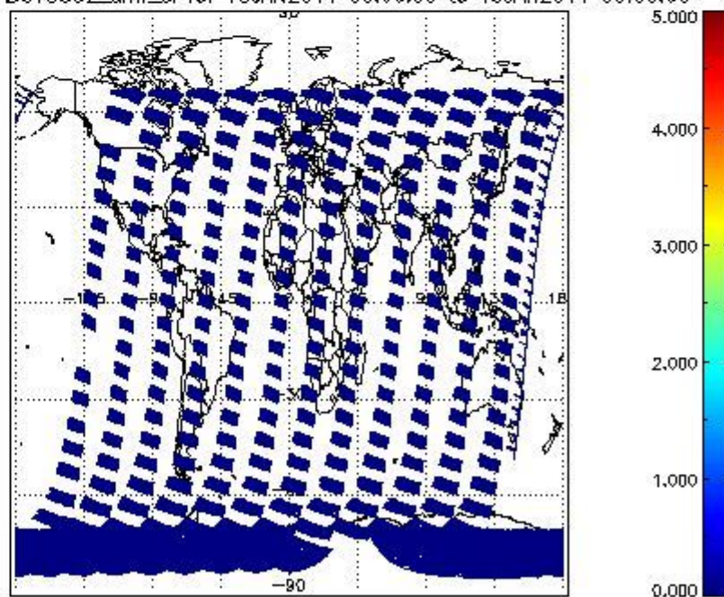
SCIOL2P_NADUV5SO2_amf_cl for 18JAN2011 00:00:00 to 19JAN2011 00:00:00
