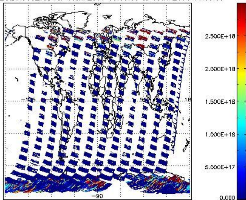
SCIDL2P_NADIR3CO_vcd for 16JAN2011 00:00:00 to 19JAN2011 00:00:00
