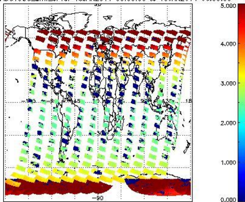
SCIOL2P_NADUV003_amf_cl for 18JAN2011 00:00:00 to 19JAN2011 00:00:00
