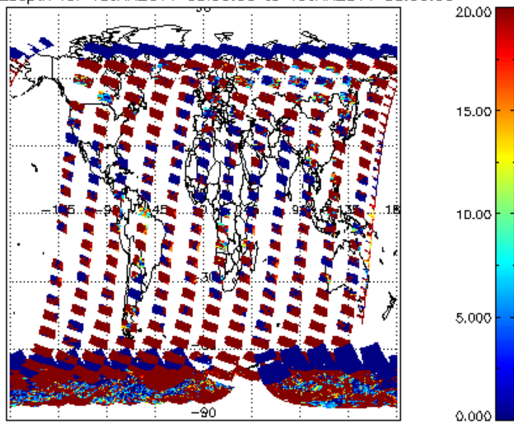
cLopt_depth for 18JAN2011 00:00:00 to 19JAN2011 00:00:00
