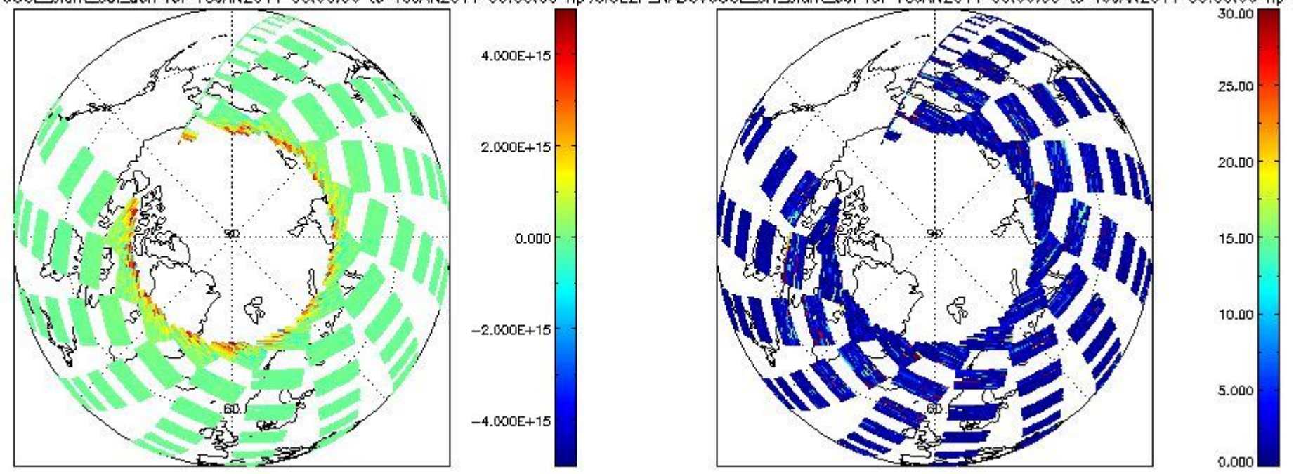
SCIOI2P_NADUV60CL_slant_col_den for 18JAN2011 00:00:00 to 19JAN2011 00:00:00 np; SCIOI2P_NADUV60CL_err_slant_col for 18JAN2011 00:00:00 to 19JAN2011 00:00:00 np
