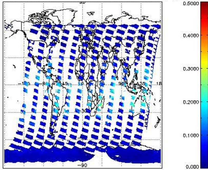
SCIOL2P_NADUV8H20_vcd_err for 18JAN2011 00:00:00 to 19JAN2011 00:00:00
