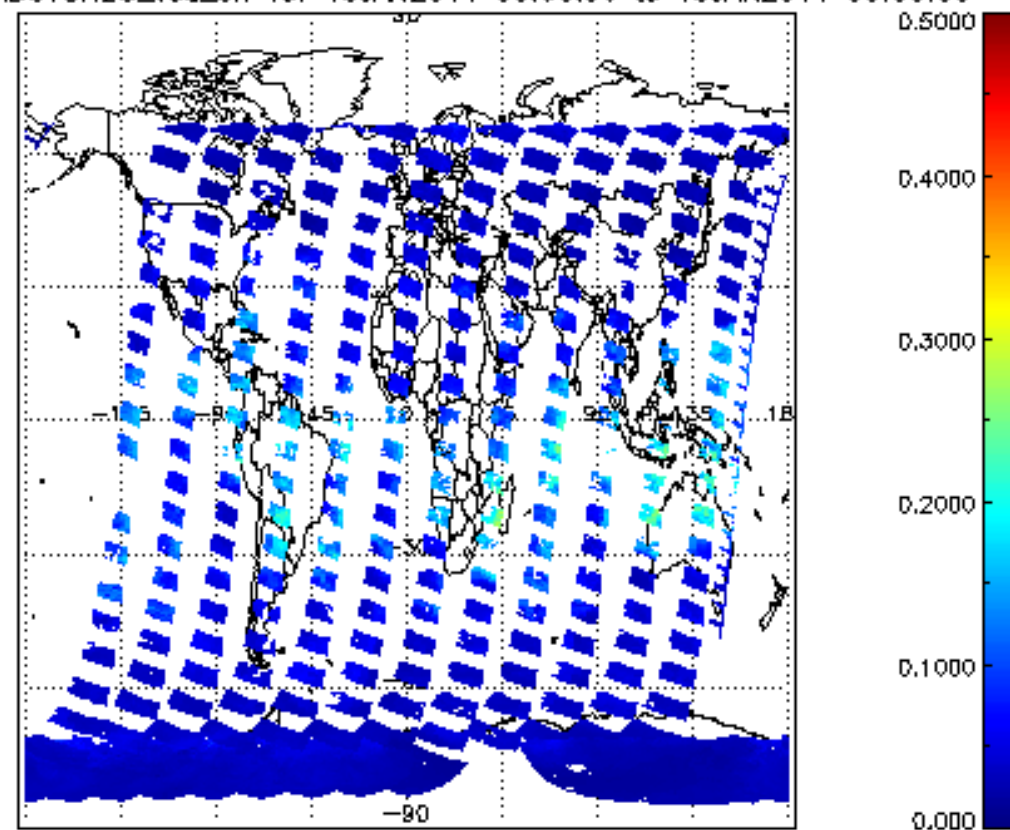
SCIOL2P_NADUV8H20_vcd_err for 18JAN2011 00:00:00 to 19JAN2011 00:00:00
