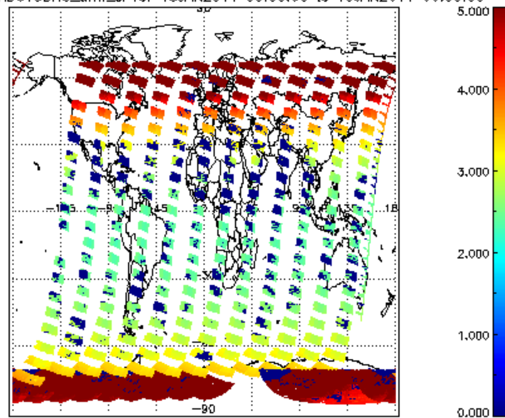
SCIOL2P_NADUV3BRO_amf_cl for 18JAN2011 00:00:00 to 19JAN2011 00:00:00
