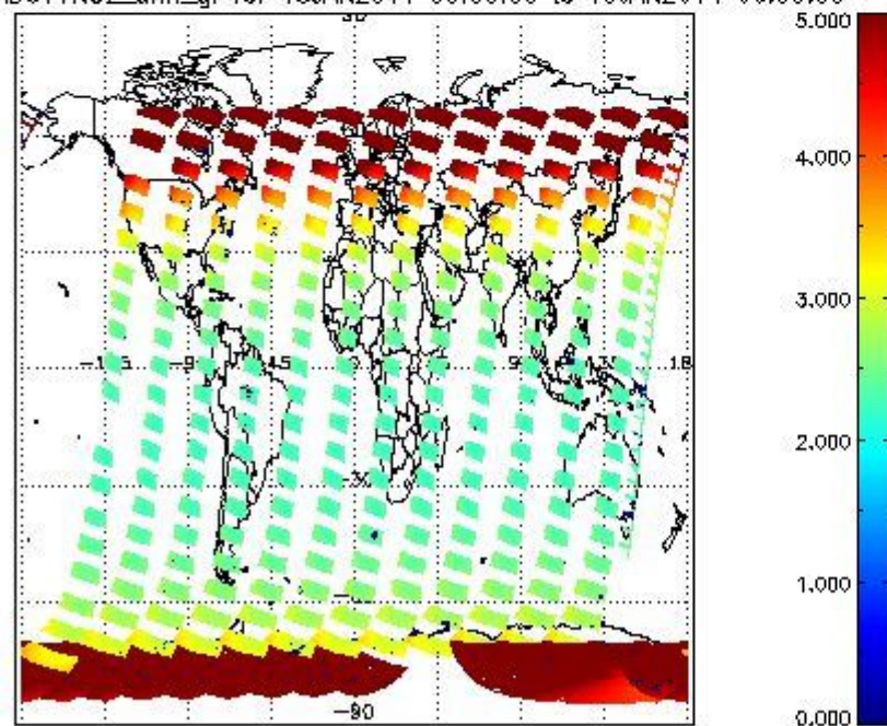
SCIOL2P_NADUV1NO2_amf_gr for 18JAN2011 00:00:00 to 19JAN2011 00:00:00
