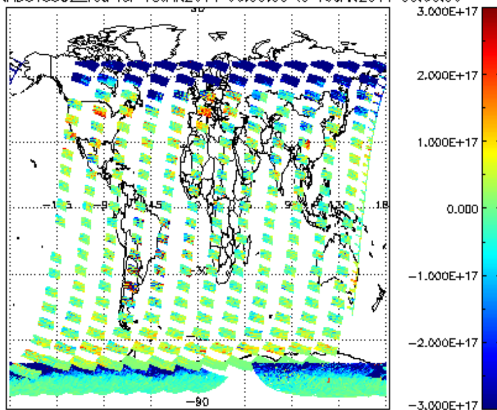
SCIOL2P_NADUV5S02_vcd for 18JAN2011 00:00:00 to 19JAN2011 00:00:00
