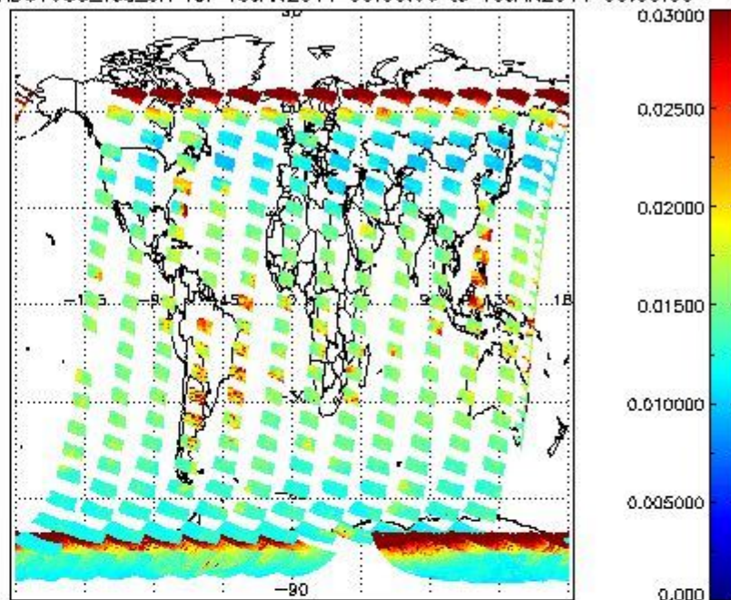
SCIOL2P_NADUV003_vcd_err for 18JAN2011 00:00:00 to 19JAN2011 00:00:00
