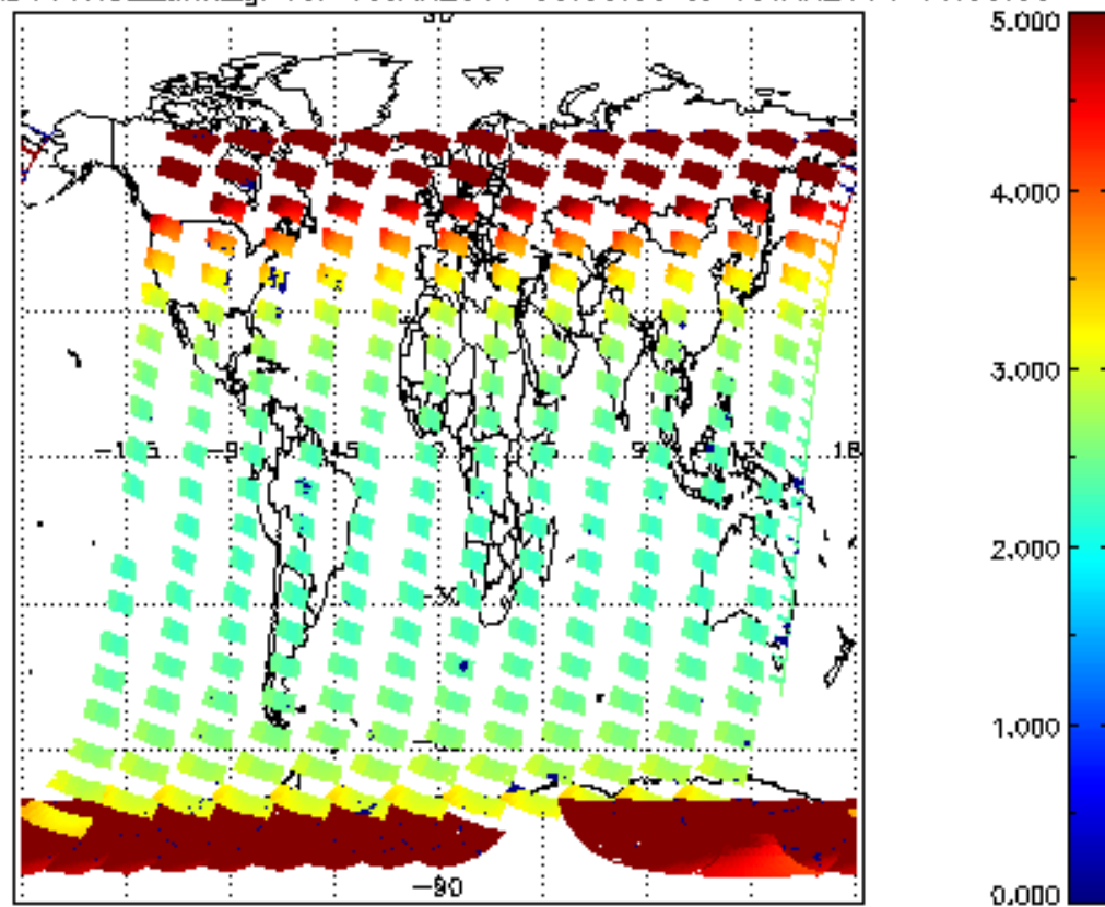
SCIOL2P_NADUV1NO2_amf_gr for 18JAN2011 00:00:00 to 19JAN2011 00:00:00
