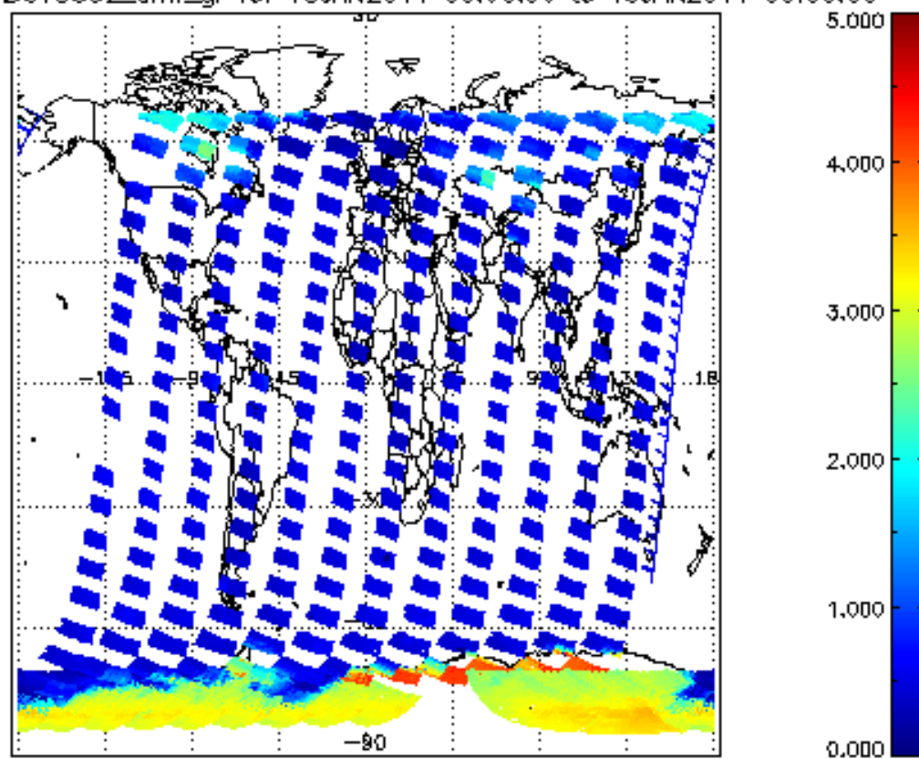
SCIOL2P_NADUV5S02_amf_gr for 18JAN2011 00:00:00 to 19JAN2011 00:00:00
