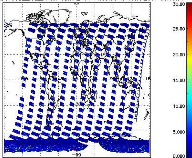
SCIOL2P_NADUV5SO2_vcd_err for 18JAN2011 00:00:00 to 19JAN2011 00:00:00
