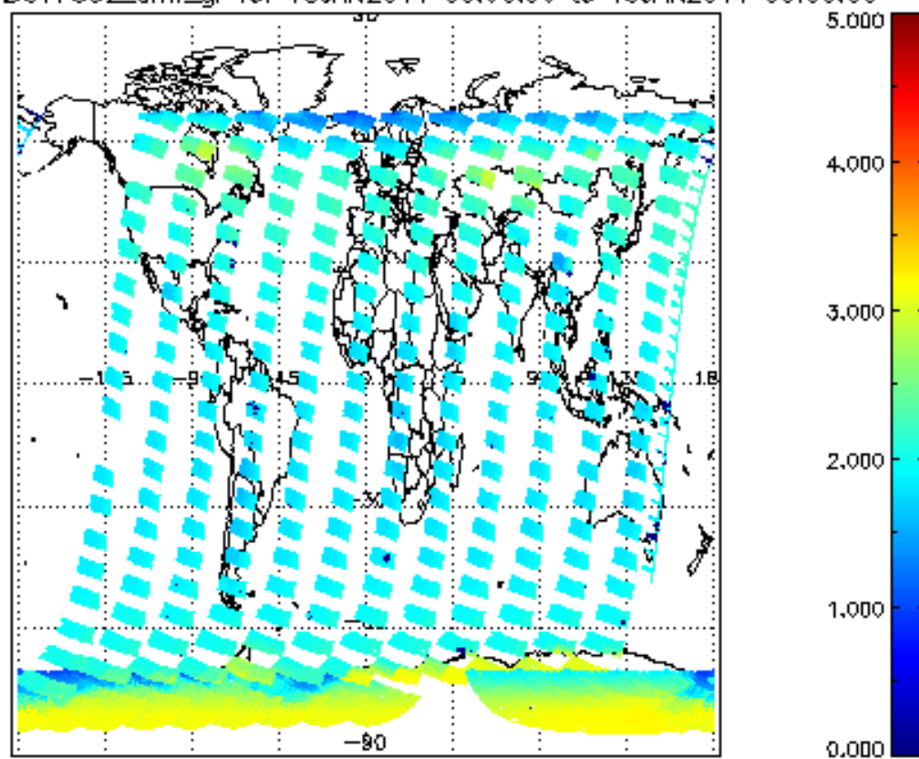
SCIOL2P_NADUV7S02_amf_gr for 18JAN2011 00:00:00 to 19JAN2011 00:00:00
