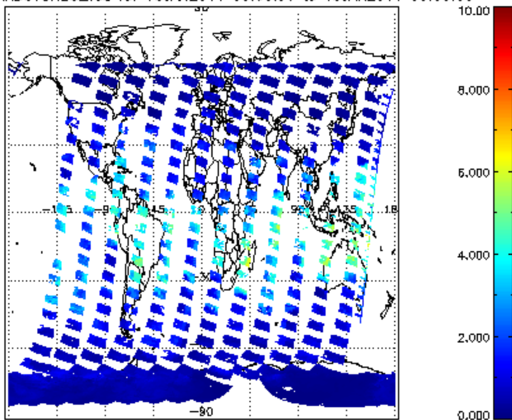
SCIOL2P_NADUV8H20_vcd for 18JAN2011 00:00:00 to 19JAN2011 00:00:00
