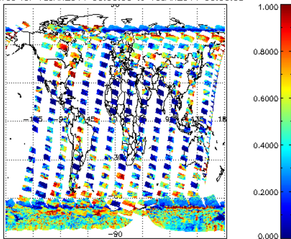
cL_frac for 18JAN2011 00:00:00 to 19JAN2011 00:00:00
