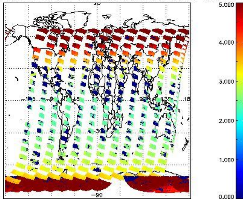
SCIOL2P_NADUV3BRO_amf_cl for 18JAN2011 00:00:00 to 19JAN2011 00:00:00
