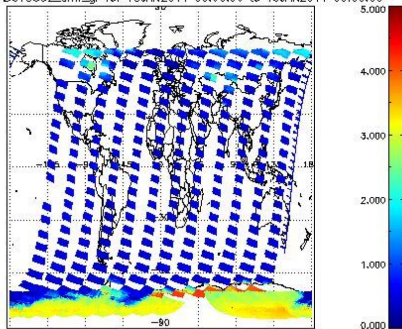
SCIOL2P_NADUV5SO2_amf_gr for 18JAN2011 00:00:00 to 19JAN2011 00:00:00
