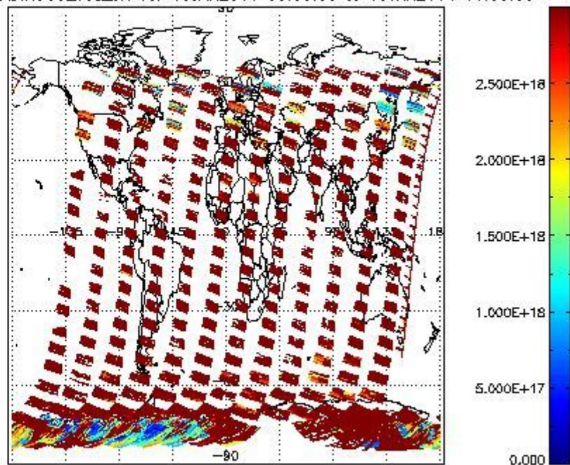
SCIDL2P_NADIR3CO_vcd_err for 16JAN2011 00:00:00 to 19JAN2011 00:00:00
