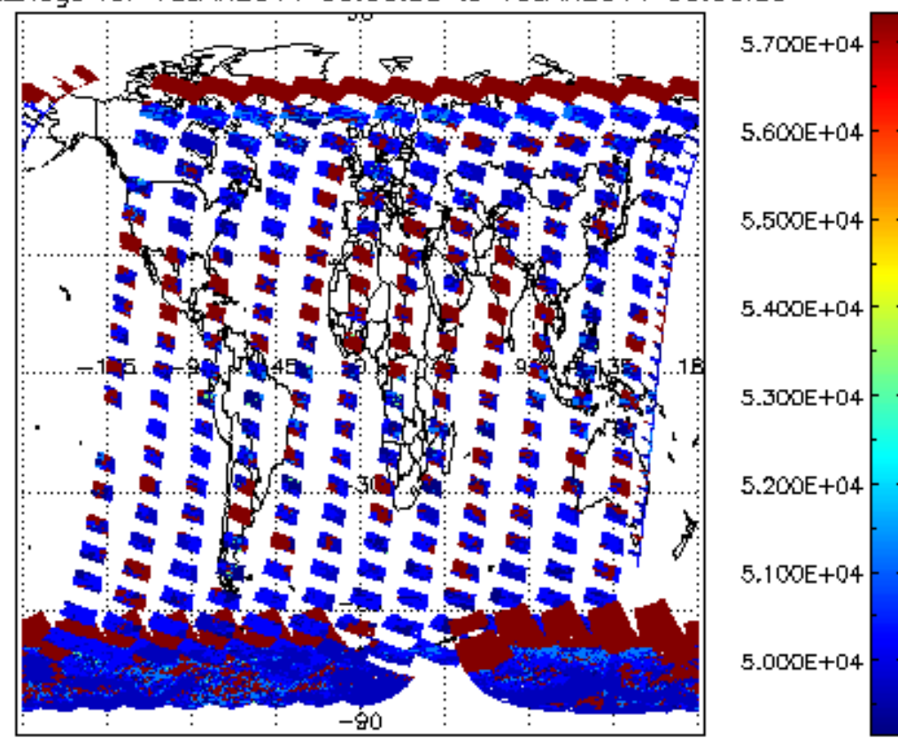
cloud_flags for 18JAN2011 00:00:00 to 19JAN2011 00:00:00
