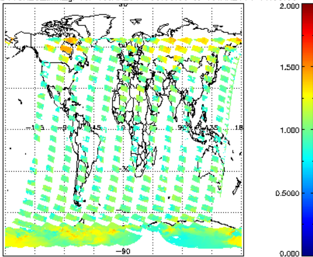
SCIOL2P_NADUV8H20_amf_gr for 18JAN2011 00:00:00 to 19JAN2011 00:00:00
