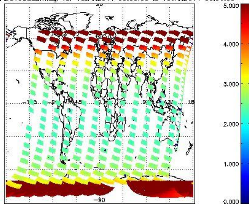
SCIOL2P_NADUV003_amf_gr for 18JAN2011 00:00:00 to 19JAN2011 00:00:00
