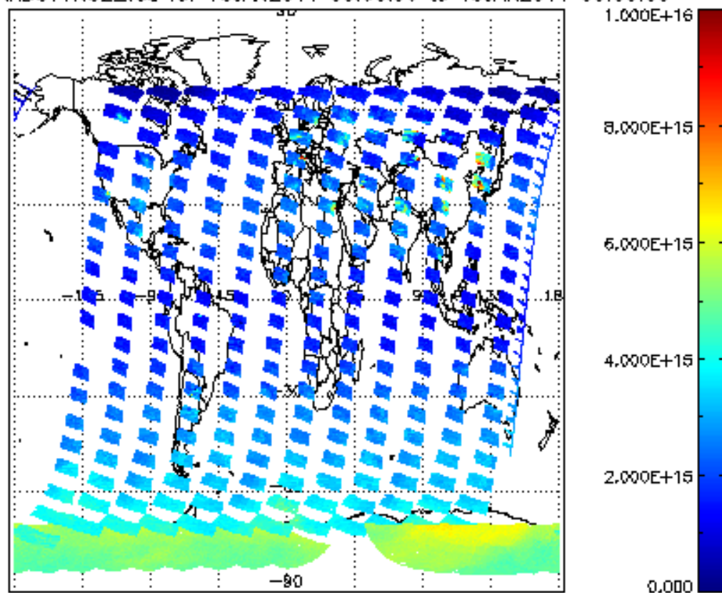
SCIOL2P_NADUV1NO2_vcd for 18JAN2011 00:00:00 to 19JAN2011 00:00:00
