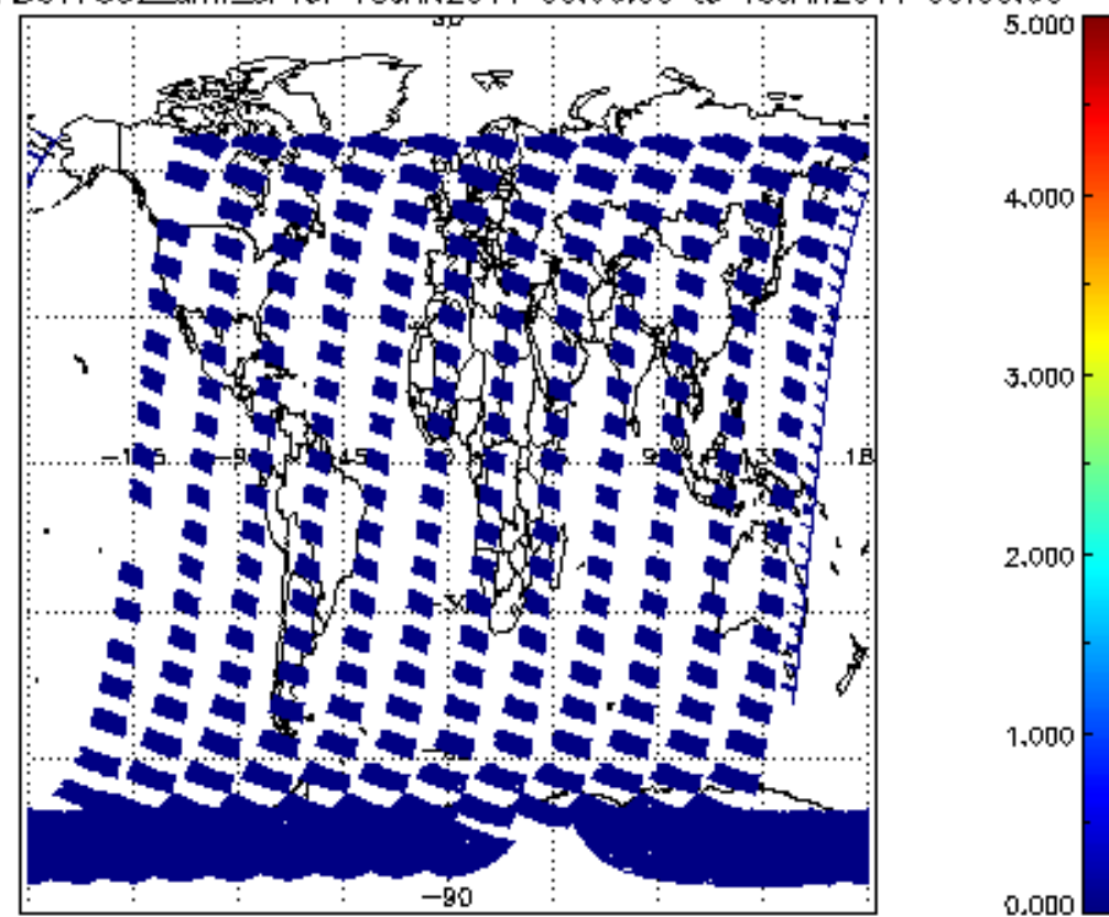
SCIOL2P_NADUV7S02_amf_cl for 18JAN2011 00:00:00 to 19JAN2011 00:00:00
