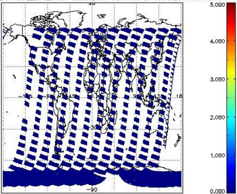
SCIOL2P_NADUV7S02_amf_cl for 18JAN2011 00:00:00 to 19JAN2011 00:00:00
