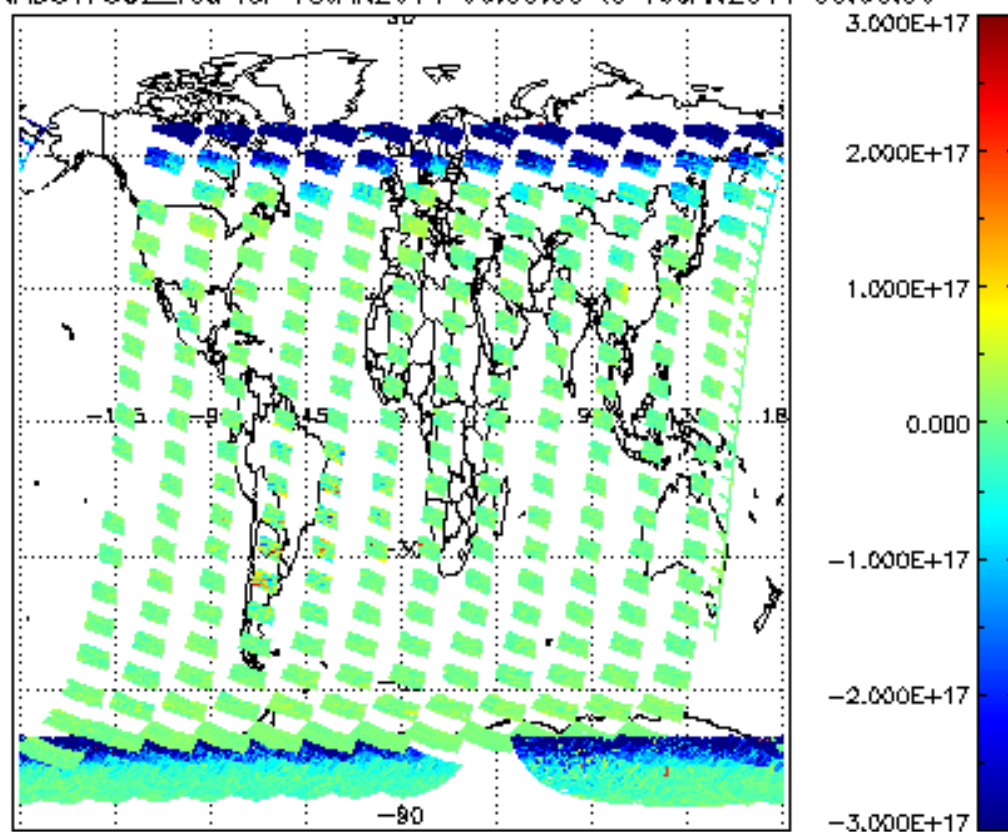
SCIOL2P_NADUV7S02_vcd for 18JAN2011 00:00:00 to 19JAN2011 00:00:00
