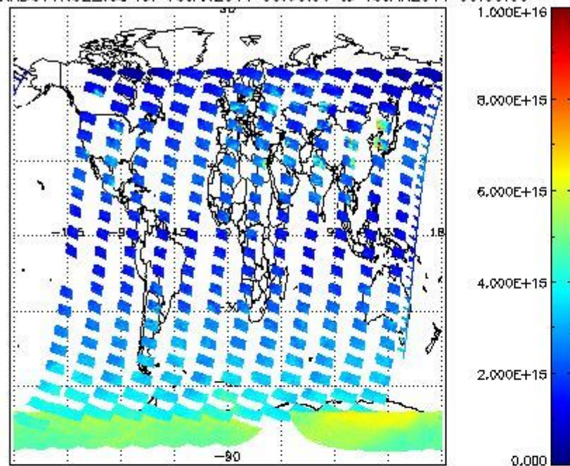
SCIOL2P_NADUV1NO2_vcd for 18JAN2011 00:00:00 to 19JAN2011 00:00:00
