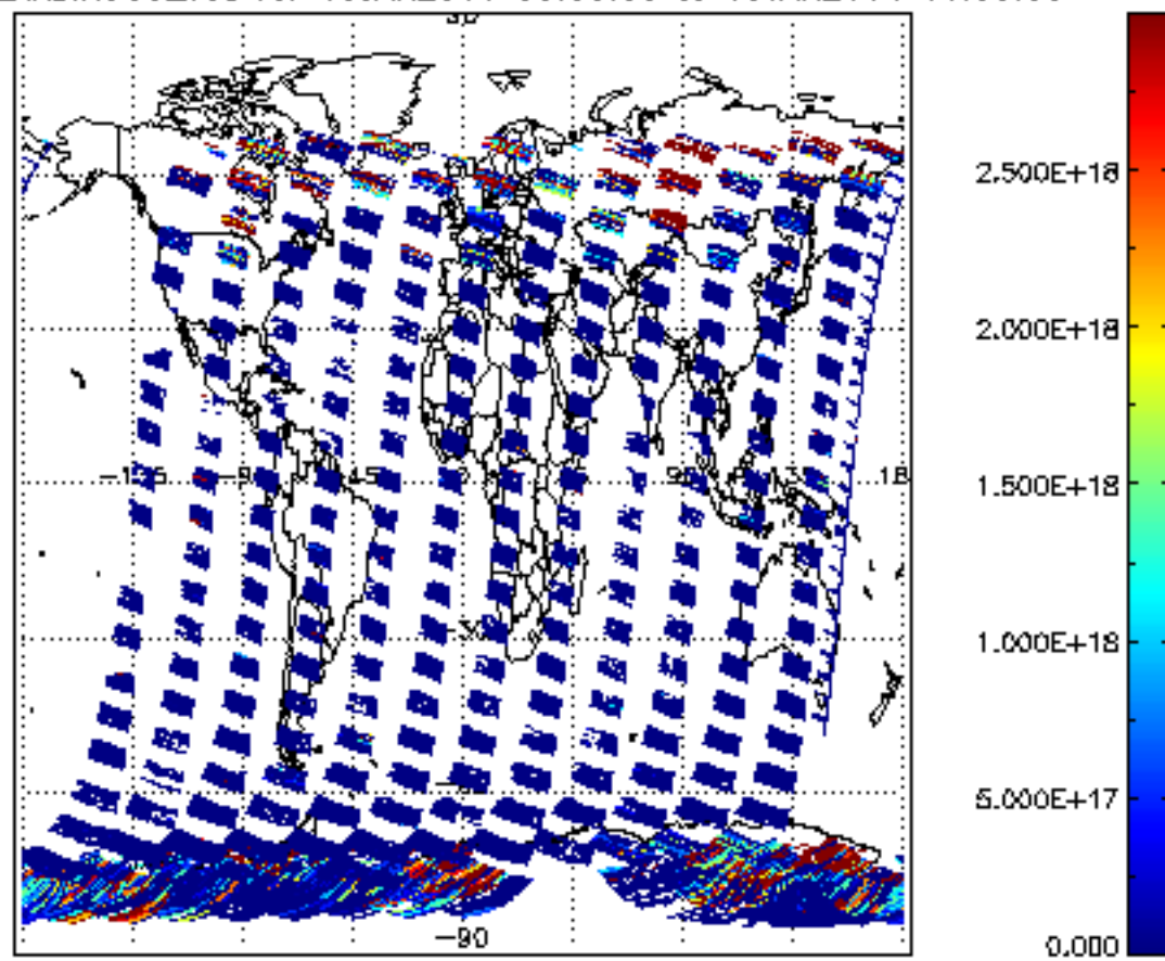
SCIOL2P_NADIR3CO_vcd for 18JAN2011 00:00:00 to 19JAN2011 00:00:00
