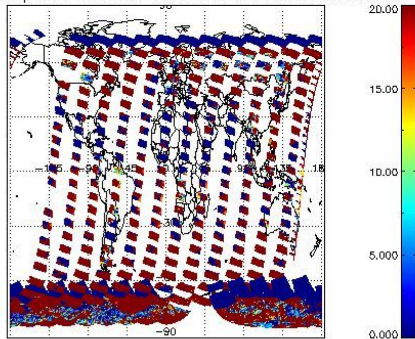
cLopt_depth for 18JAN2011 00:00:00 to 19JAN2011 00:00:00
