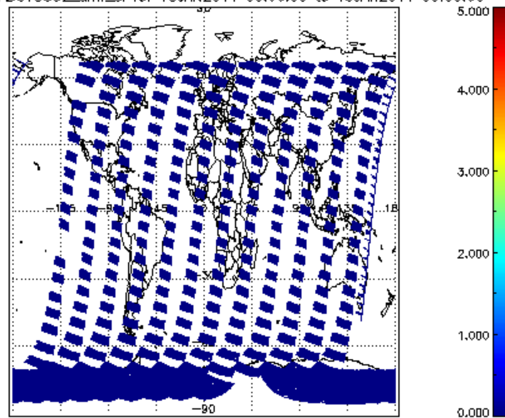
SCIOL2P_NADUV5S02_amf_sl for 18JAN2011 00:00:00 to 19JAN2011 00:00:00
