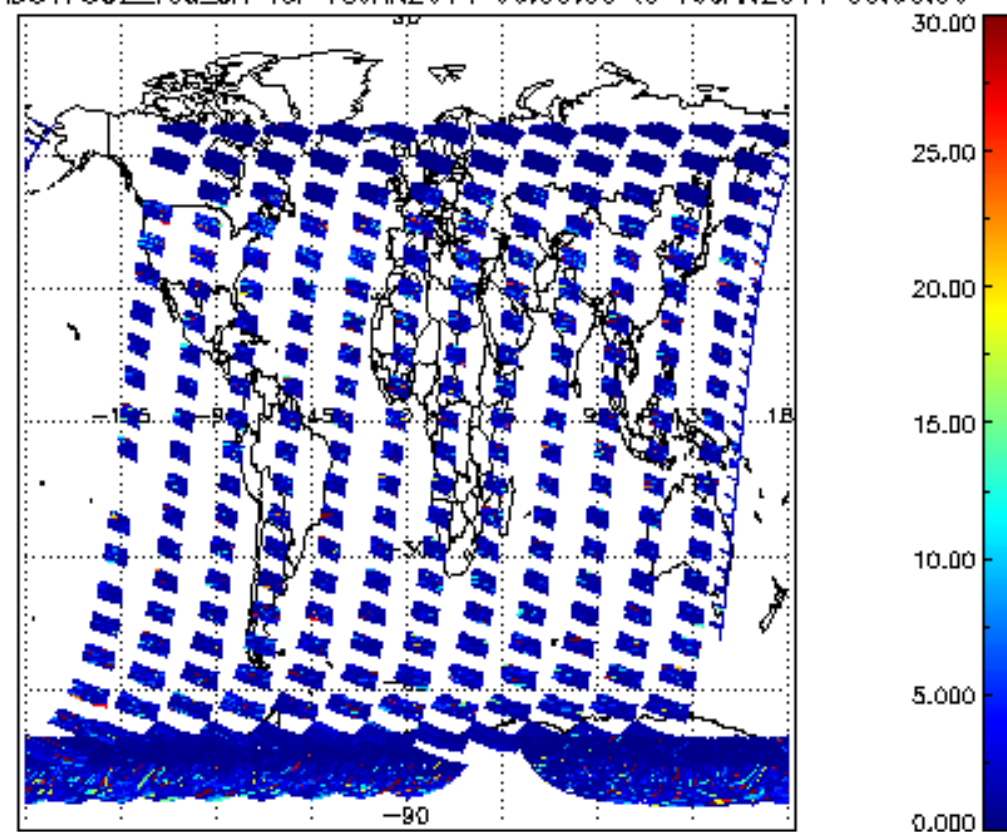
SCIOL2P_NADUV7S02_vcd_err for 18JAN2011 00:00:00 to 19JAN2011 00:00:00
