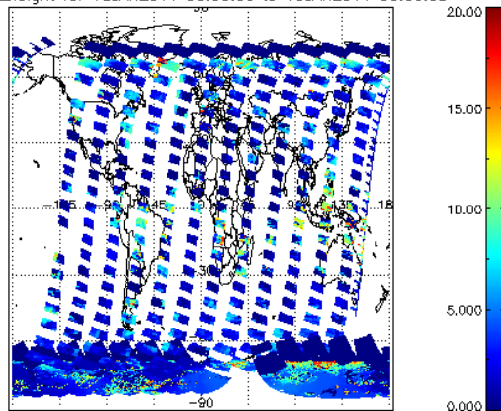
cL_top_height for 18JAN2011 00:00:00 to 19JAN2011 00:00:00
