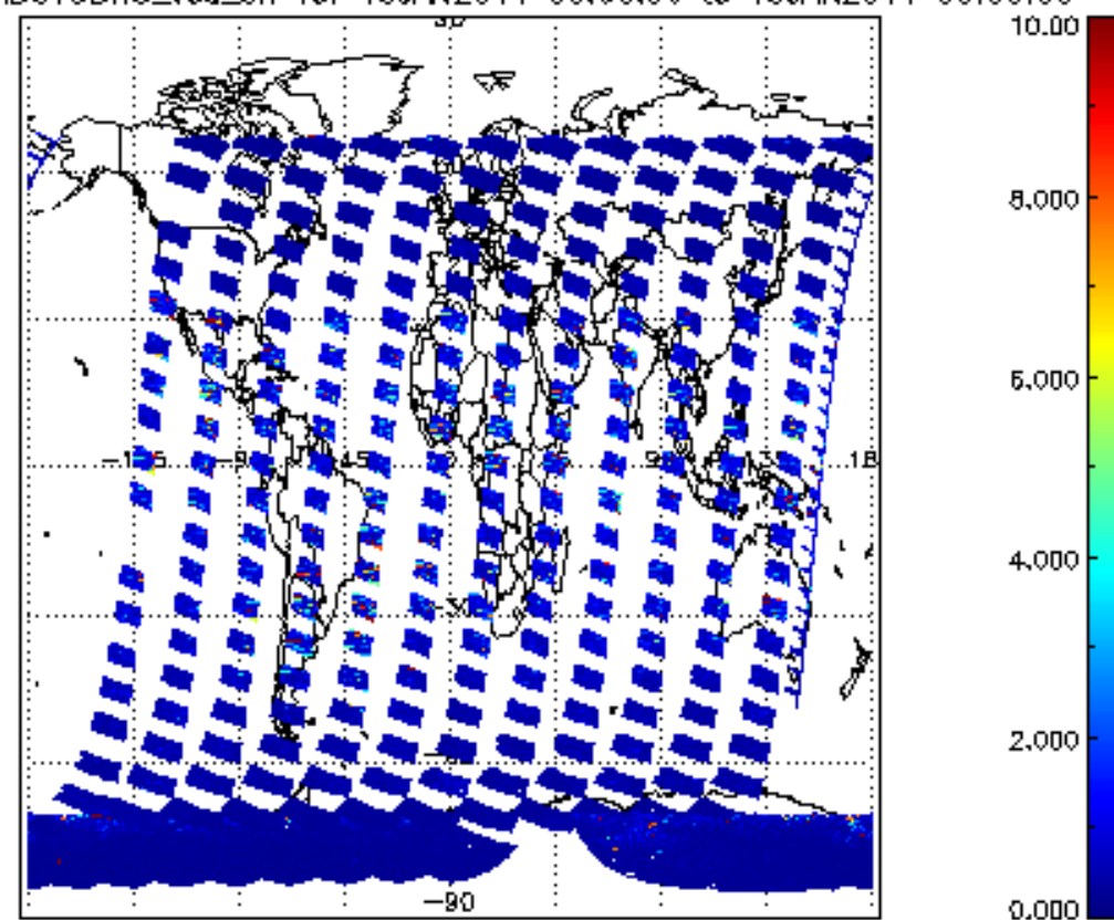
SCIOL2P_NADUV3BRO_vcd_err for 18JAN2011 00:00:00 to 19JAN2011 00:00:00
