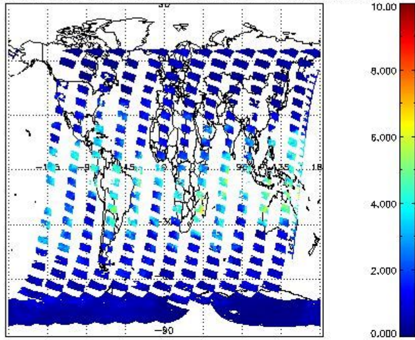
SCIOL2P_NADUV8H20_vcd for 18JAN2011 00:00:00 to 19JAN2011 00:00:00
