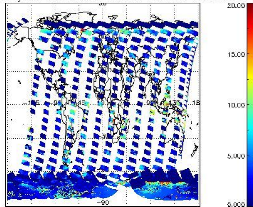
cL_top_height for 18JAN2011 00:00:00 to 19JAN2011 00:00:00
