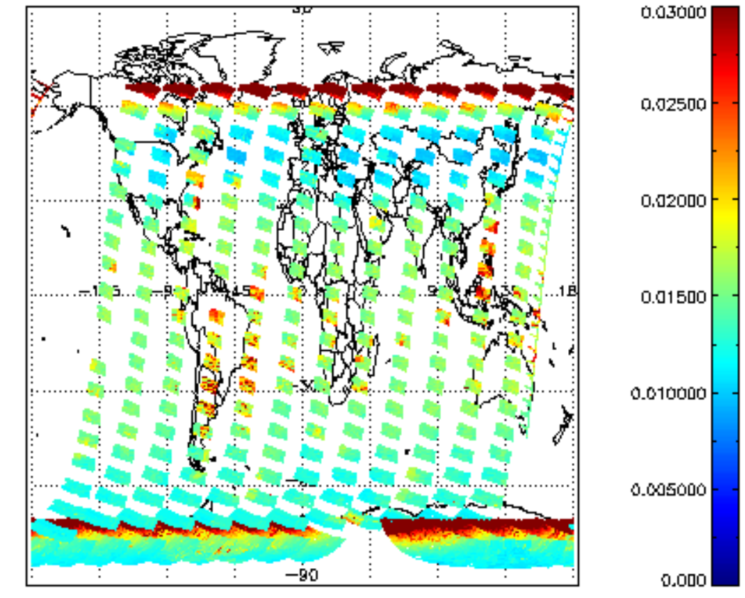
SCIOL2P_NADUV003_vcd_err for 18JAN2011 00:00:00 to 19JAN2011 00:00:00
