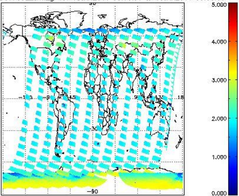
SCIOL2P_NADUV7S02_amf_gr for 18JAN2011 00:00:00 to 19JAN2011 00:00:00
