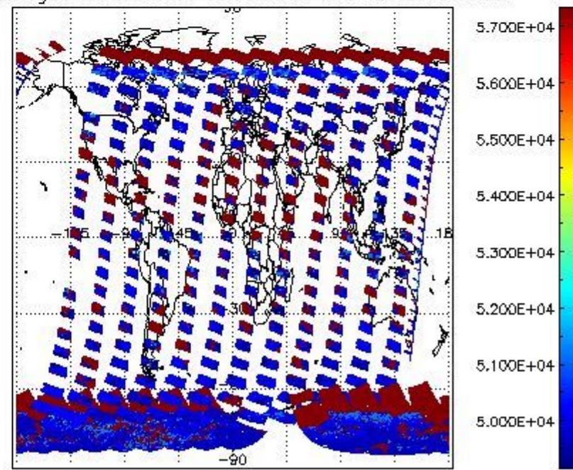
cloud_flags for 18JAN2011 00:00:00 to 19JAN2011 00:00:00
