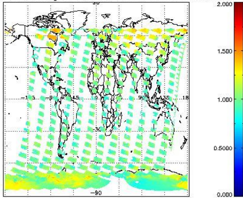
SCIOL2P_NADUV8H20_amf_gr for 18JAN2011 00:00:00 to 19JAN2011 00:00:00
