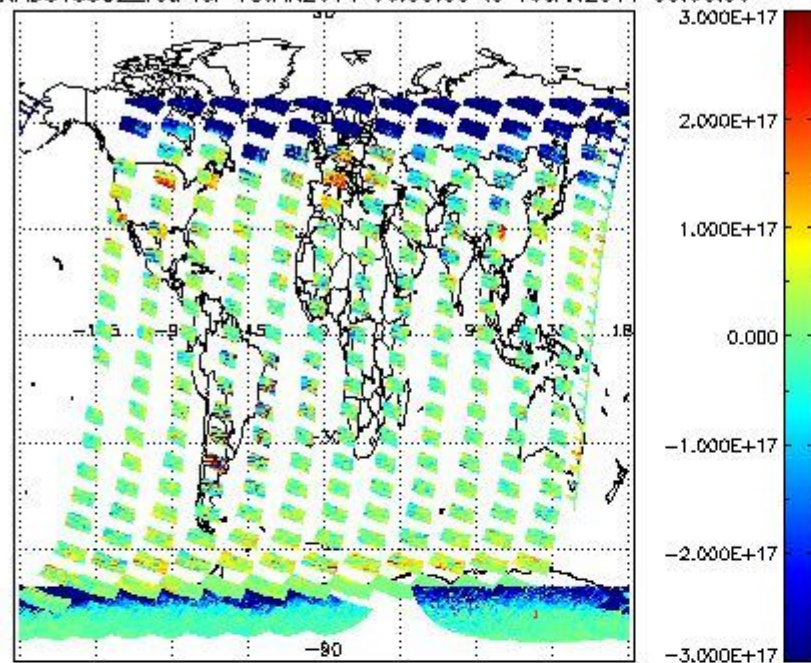
SCIOL2P_NADUV5SO2_vcd for 18JAN2011 00:00:00 to 19JAN2011 00:00:00
