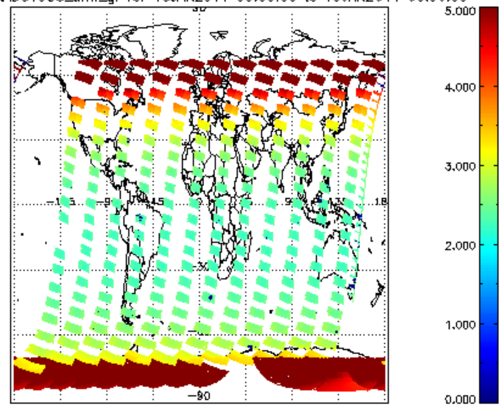
SCIOL2P_NADUV003_amf_gr for 18JAN2011 00:00:00 to 19JAN2011 00:00:00
