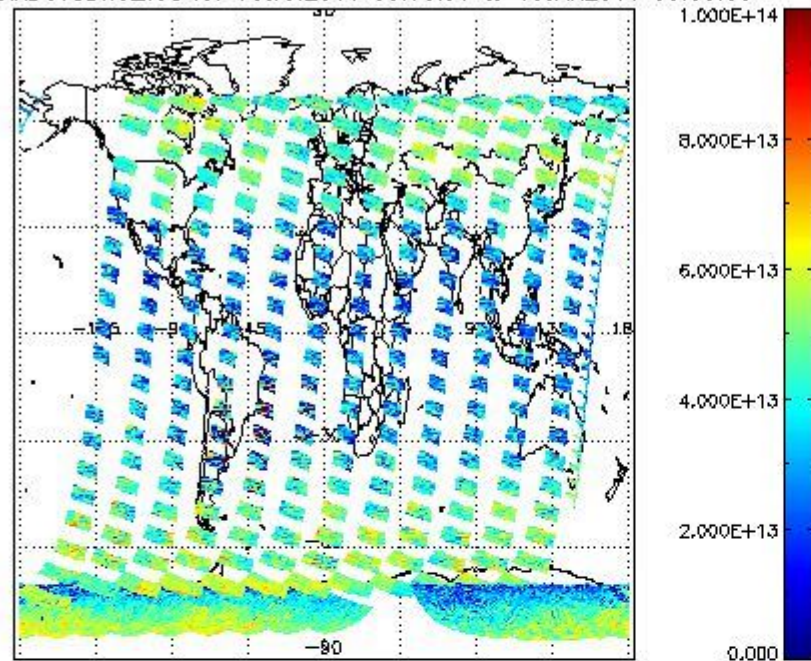
SCIOL2P_NADUV3BRO_vcd for 18JAN2011 00:00:00 to 19JAN2011 00:00:00
