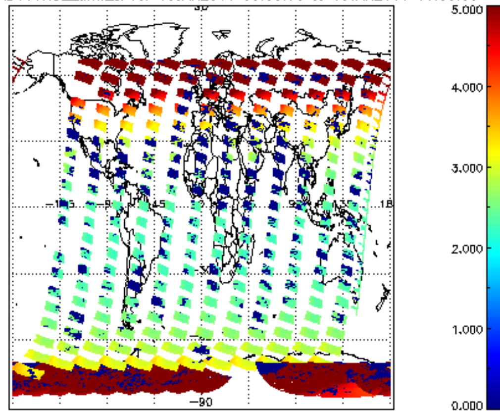
SCIOL2P_NADUV1NO2_amf_cl for 18JAN2011 00:00:00 to 19JAN2011 00:00:00
