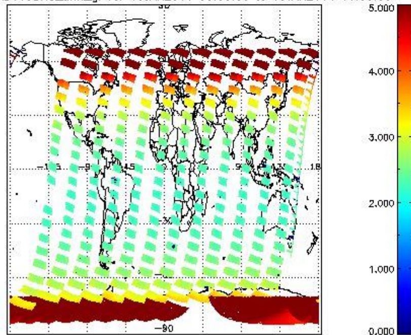
SCIOL2P_NADUV3BRO_amf_gr for 18JAN2011 00:00:00 to 19JAN2011 00:00:00
