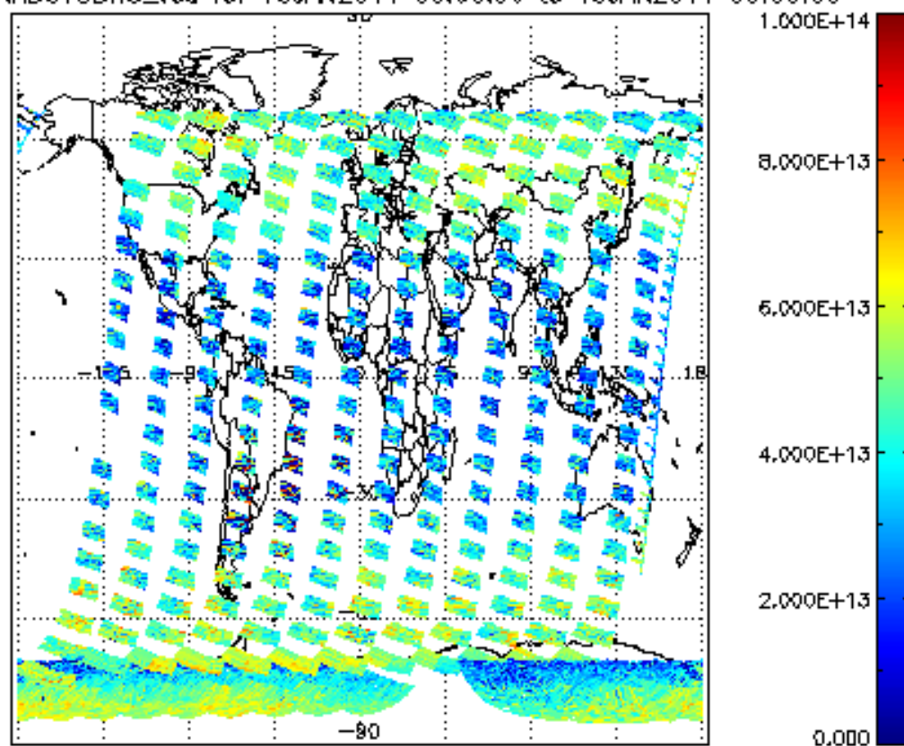
SCIOL2P_NADUV3BRO_vcd for 18JAN2011 00:00:00 to 19JAN2011 00:00:00
