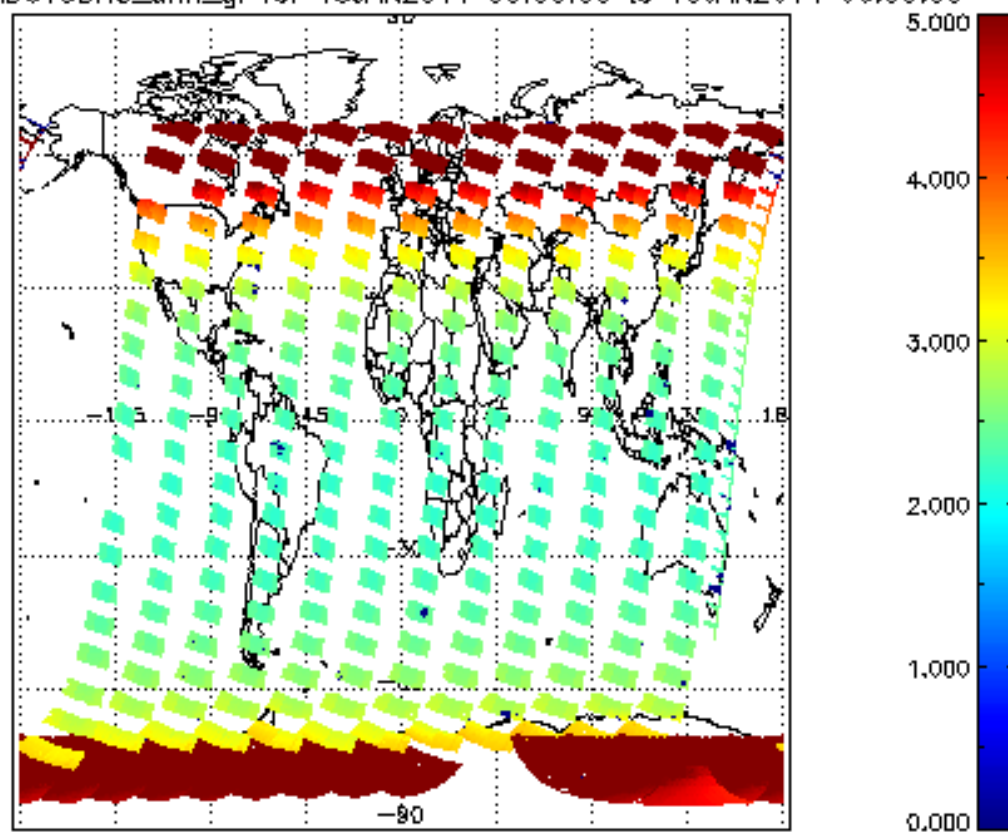
SCIOL2P_NADUV3BRO_amf_gr for 18JAN2011 00:00:00 to 19JAN2011 00:00:00
