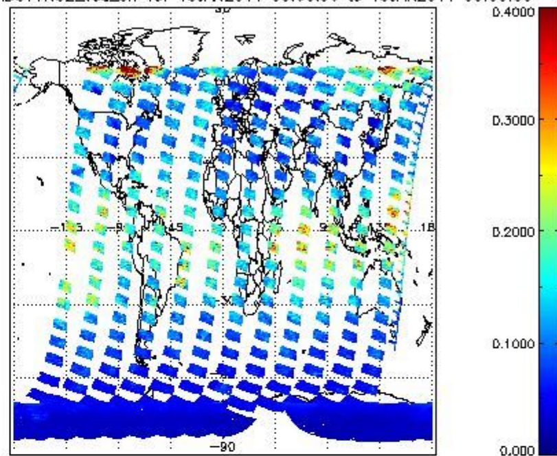
SCIOL2P_NADUV1NO2_vcd_err for 18JAN2011 00:00:00 to 19JAN2011 00:00:00
