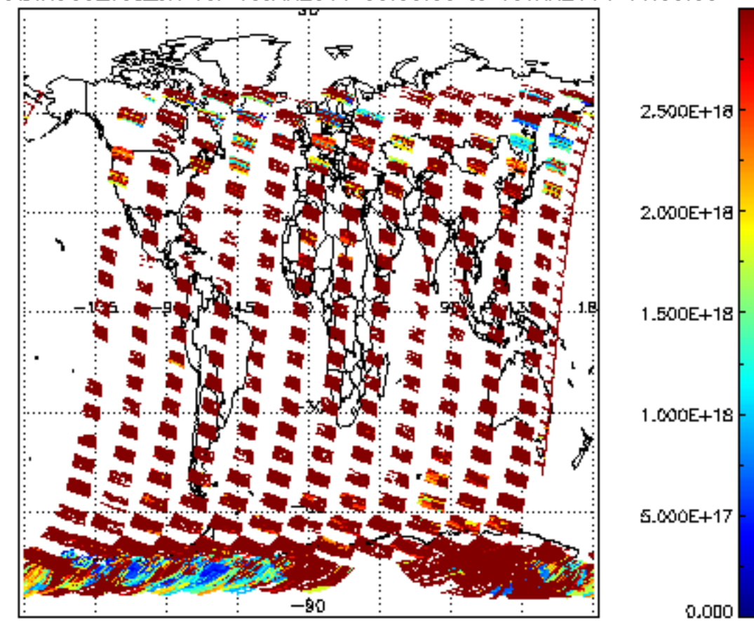
SCIOL2P_NADIR3CO_vcd_err for 18JAN2011 00:00:00 to 19JAN2011 00:00:00
