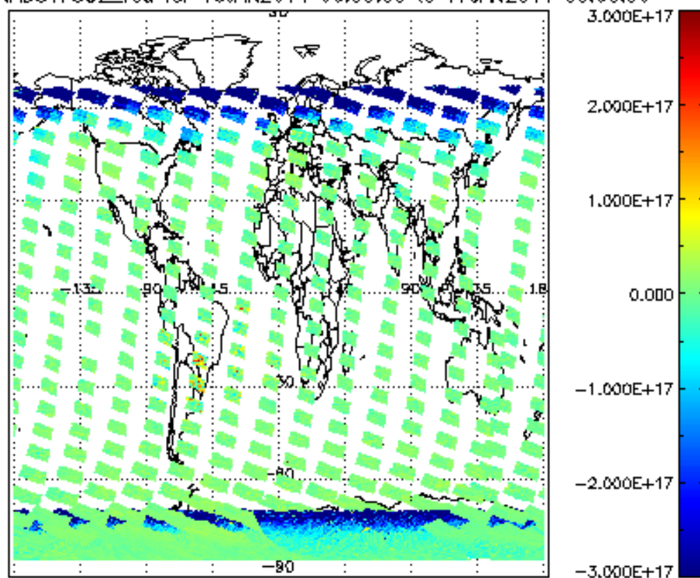
SCIOL2P_NADUV7S02_vcd for 16JAN2011 00:00:00 to 17JAN2011 00:00:00
