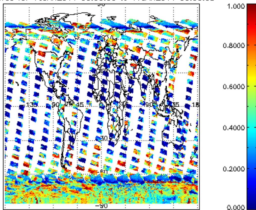
cL_frac for 16JAN2011 00:00:00 to 17JAN2011 00:00:00
