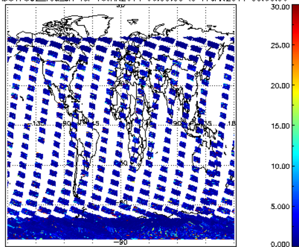
SCIOL2P_NADUV7S02_vcd_err for 16JAN2011 00:00:00 to 17JAN2011 00:00:00
