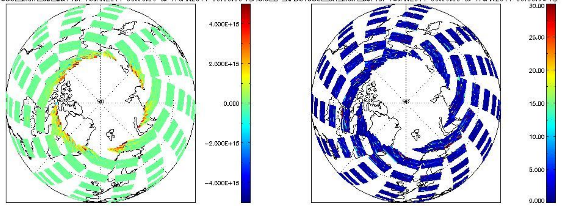
SCIOI2P_NADUV60CL_slant_col_den for 16JAN2011 00:00:00 to 17JAN2011 00:00:00 np; SCIOI2P_NADUV60CL_err_slant_col for 16JAN2011 00:00:00 to 17JAN2011 00:00:00 np
