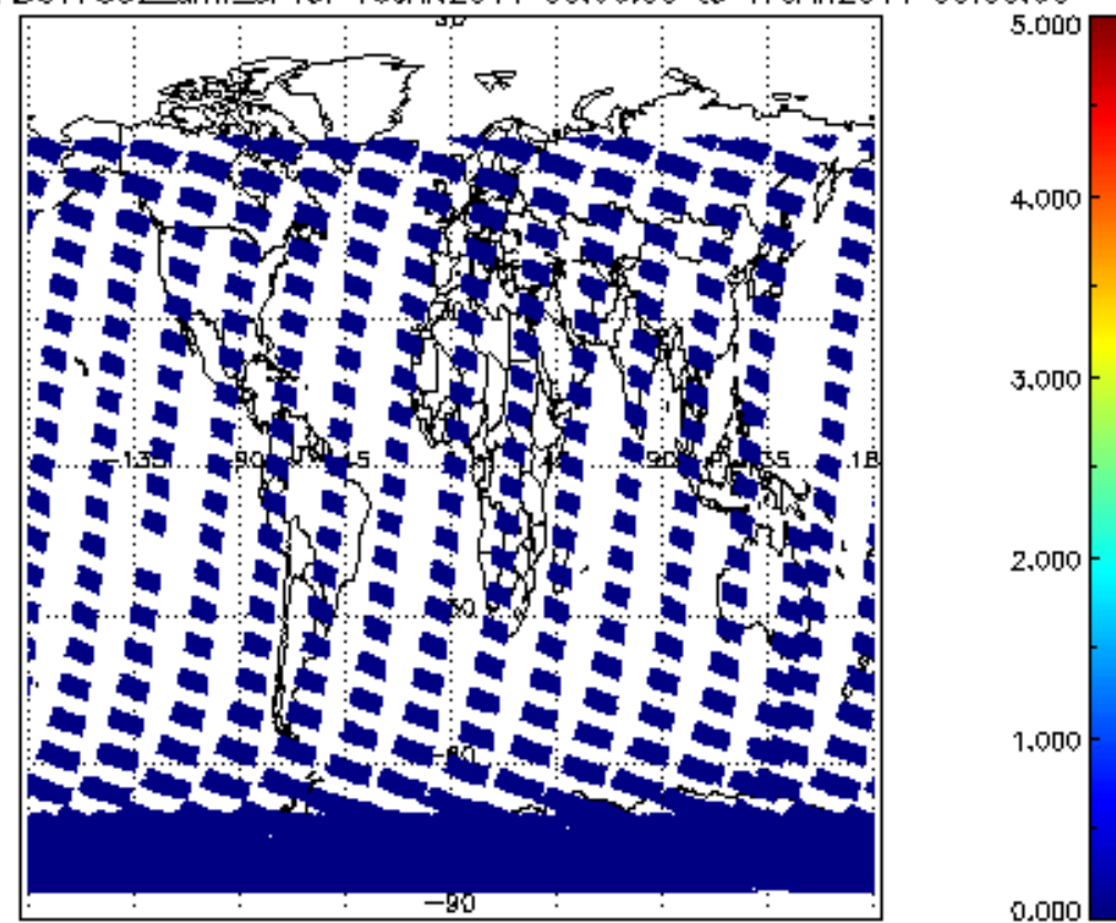
SCIOL2P_NADUV7S02_amf_cl for 16JAN2011 00:00:00 to 17JAN2011 00:00:00
