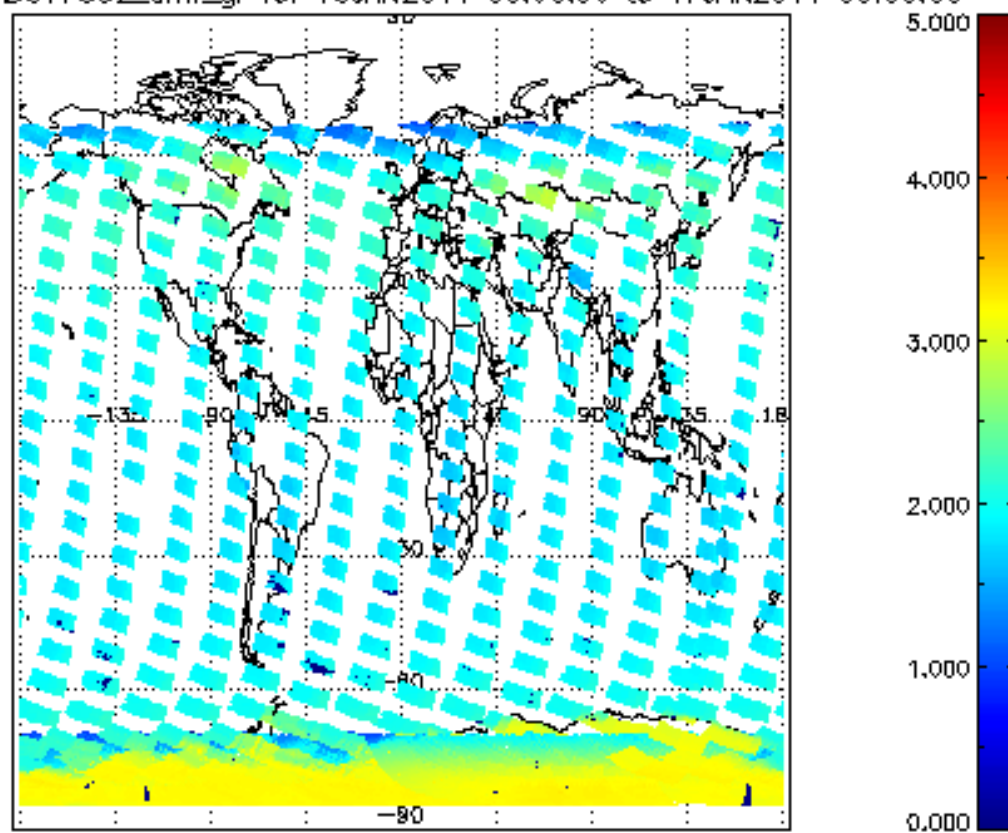
SCIOL2P_NADUV7S02_amf_gr for 16JAN2011 00:00:00 to 17JAN2011 00:00:00
