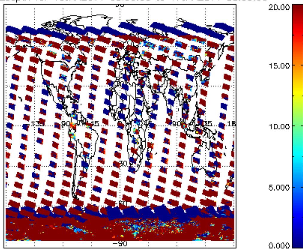
cLopt_depth for 16JAN2011 00:00:00 to 17JAN2011 00:00:00
