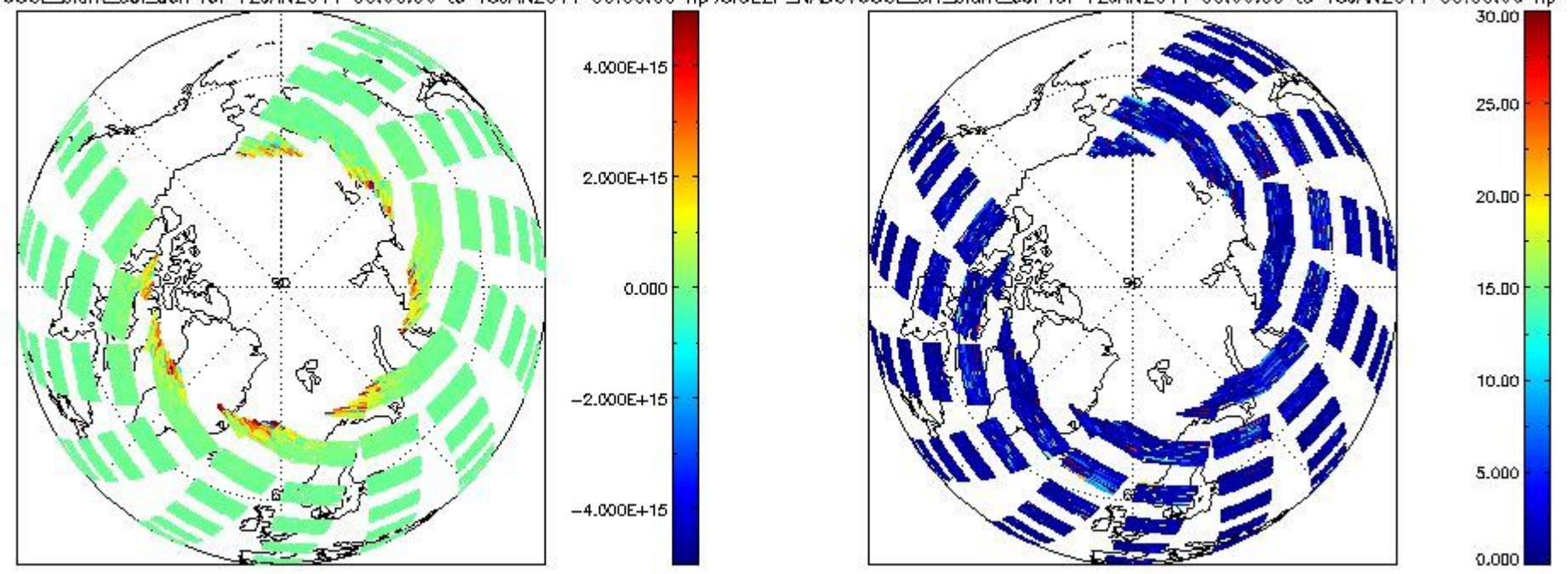
SCIOI2P_NADUV60CL_slant_col_den for 12JAN2011 00:00:00 to 13JAN2011 00:00:00 np; SCIOI2P_NADUV60CL_err_slant_col for 12JAN2011 00:00:00 to 13JAN2011 00:00:00 np
