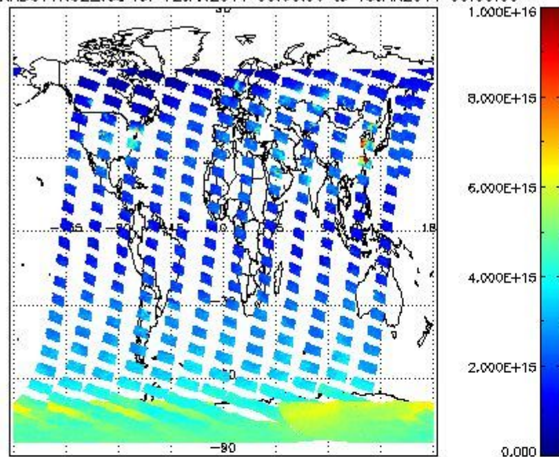
SCIOL2P_NADUV1NO2_vcd for 12JAN2011 00:00:00 to 13JAN2011 00:00:00
