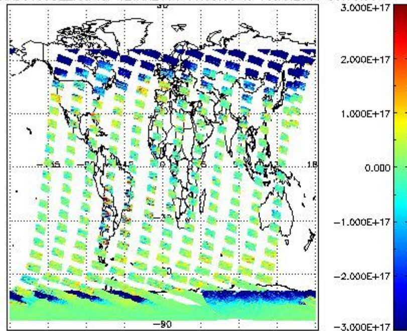
SCIOL2P_NADUV5S02_vcd for 12JAN2011 00:00:00 to 13JAN2011 00:00:00
