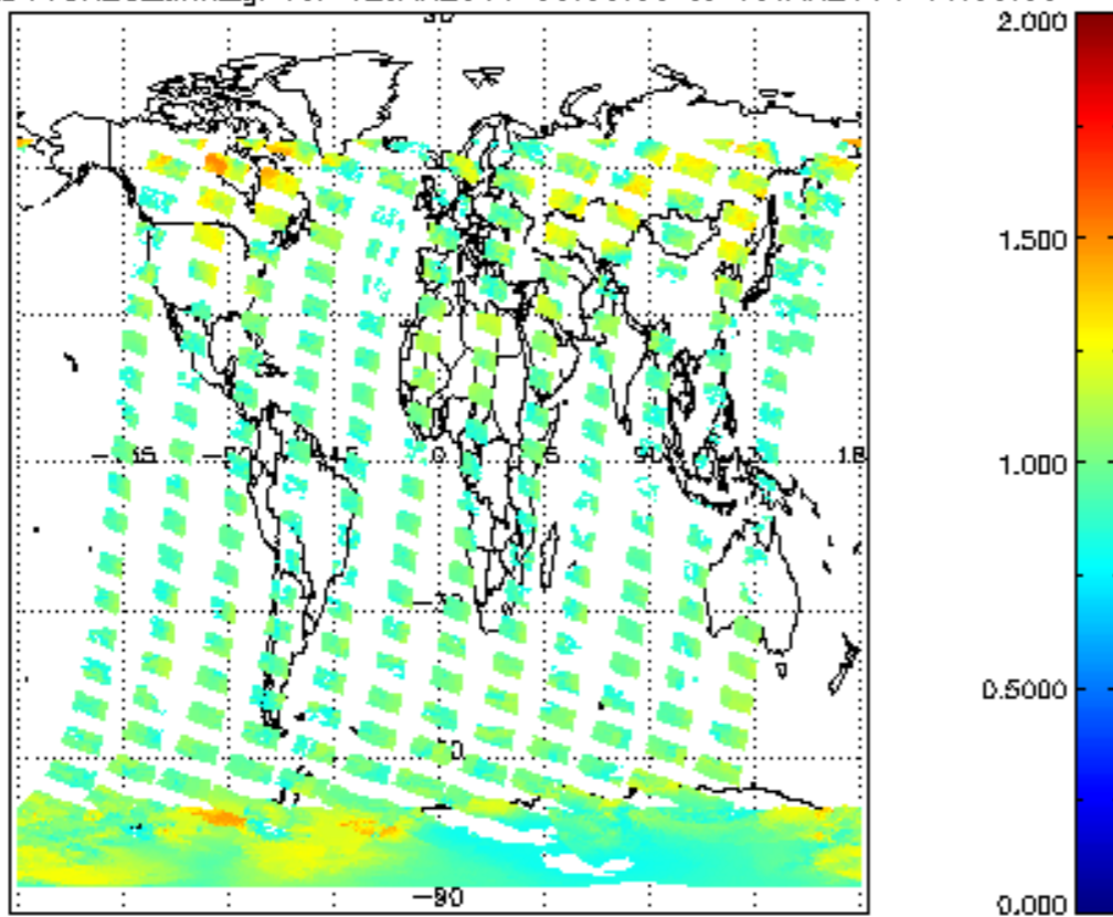
SCIOL2P_NADUV8H20_amf_gr for 12JAN2011 00:00:00 to 13JAN2011 00:00:00
