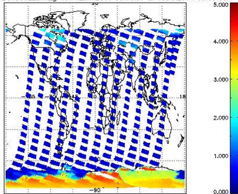
SCIOL2P_NADUV5S02_amf_gr for 12JAN2011 00:00:00 to 13JAN2011 00:00:00
