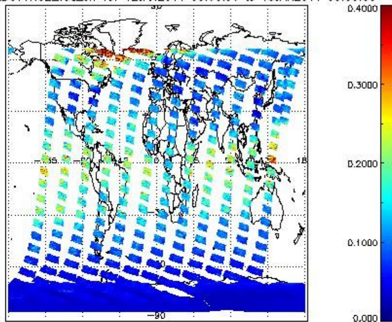
SCIOL2P_NADUV1NO2_vcd_err for 12JAN2011 00:00:00 to 13JAN2011 00:00:00
