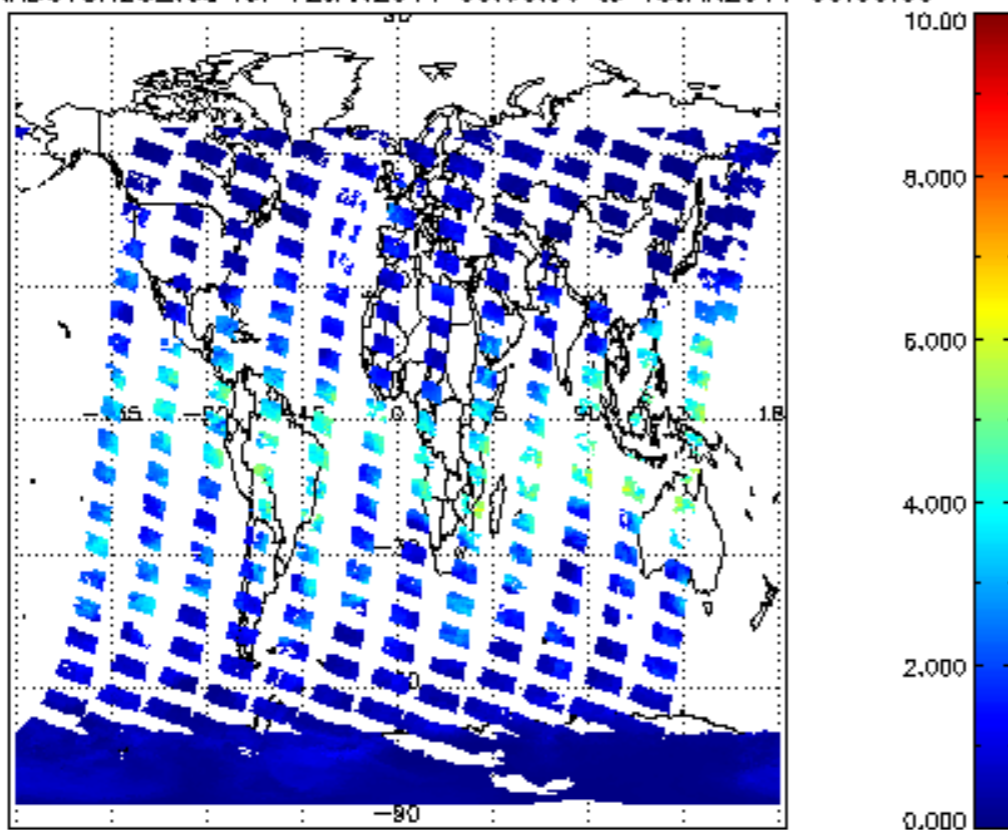
SCIOL2P_NADUV8H20_vcd for 12JAN2011 00:00:00 to 13JAN2011 00:00:00
