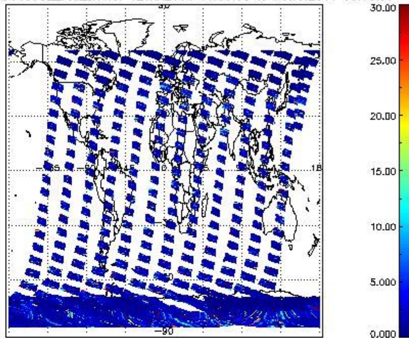
SCIOL2P_NADUV5S02_vcd_err for 12JAN2011 00:00:00 to 13JAN2011 00:00:00
