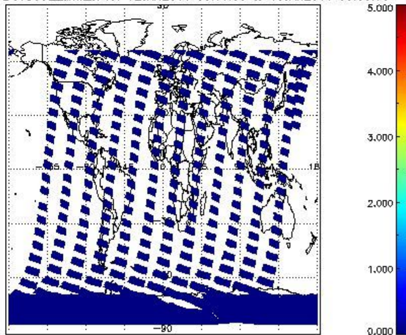
SCIOL2P_NADUV5S02_amf_cl for 12JAN2011 00:00:00 to 13JAN2011 00:00:00
