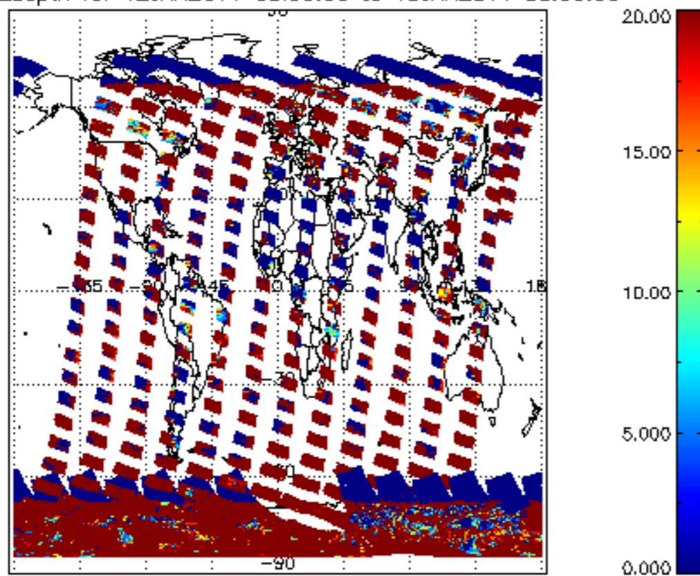
cLopt_depth for 12JAN2011 00:00:00 to 13JAN2011 00:00:00
