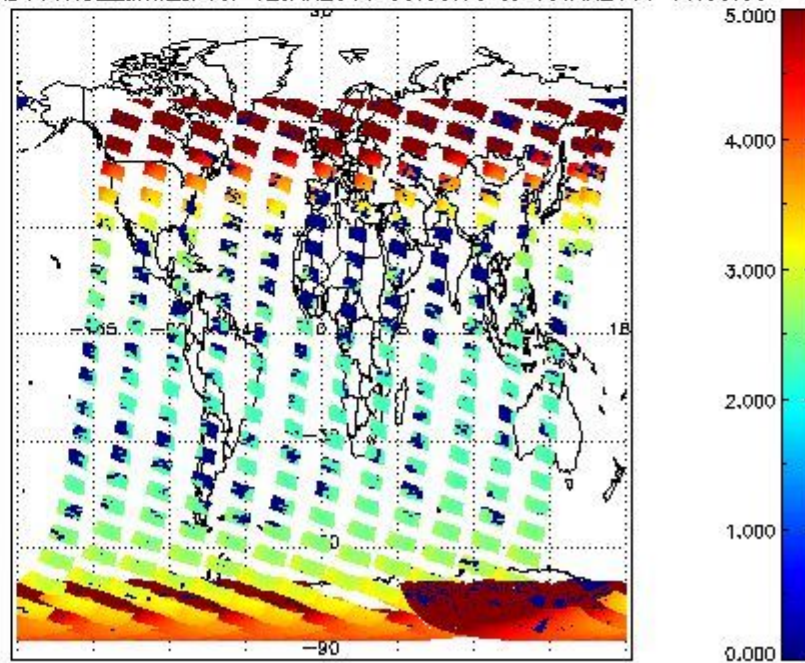
SCIOL2P_NADUV1NO2_amf_cl for 12JAN2011 00:00:00 to 13JAN2011 00:00:00
