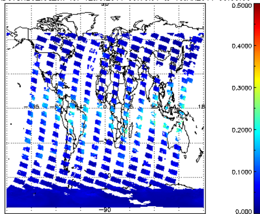
SCIOL2P_NADUV8H20_vcd_err for 12JAN2011 00:00:00 to 13JAN2011 00:00:00
