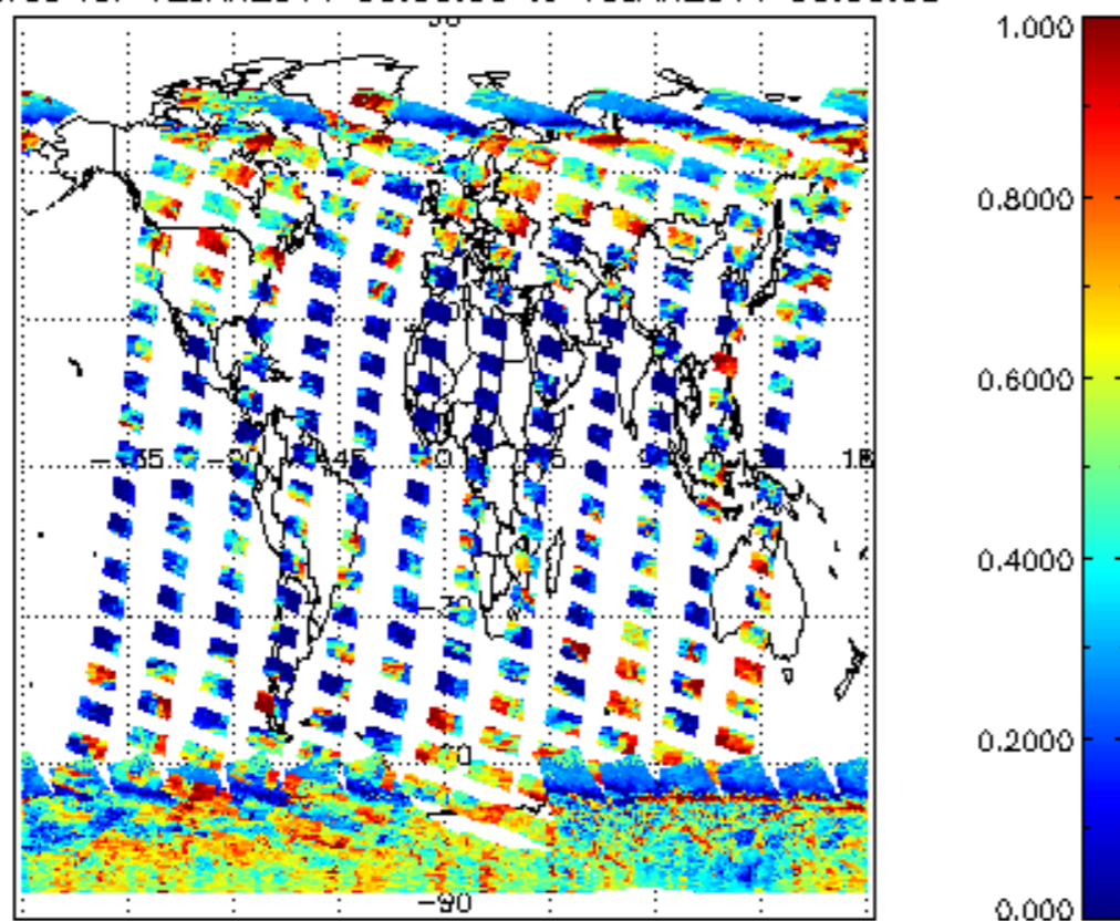
cL_frac for 12JAN2011 00:00:00 to 13JAN2011 00:00:00
