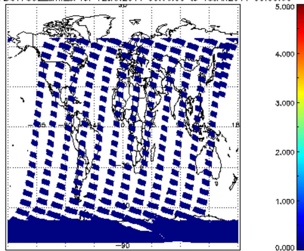
SCIOL2P_NADUV7S02_amf_cl for 12JAN2011 00:00:00 to 13JAN2011 00:00:00
