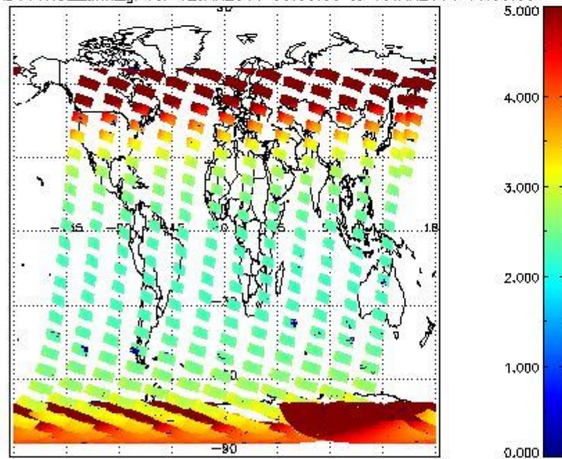
SCIOL2P_NADUV1NO2_amf_gr for 12JAN2011 00:00:00 to 13JAN2011 00:00:00
