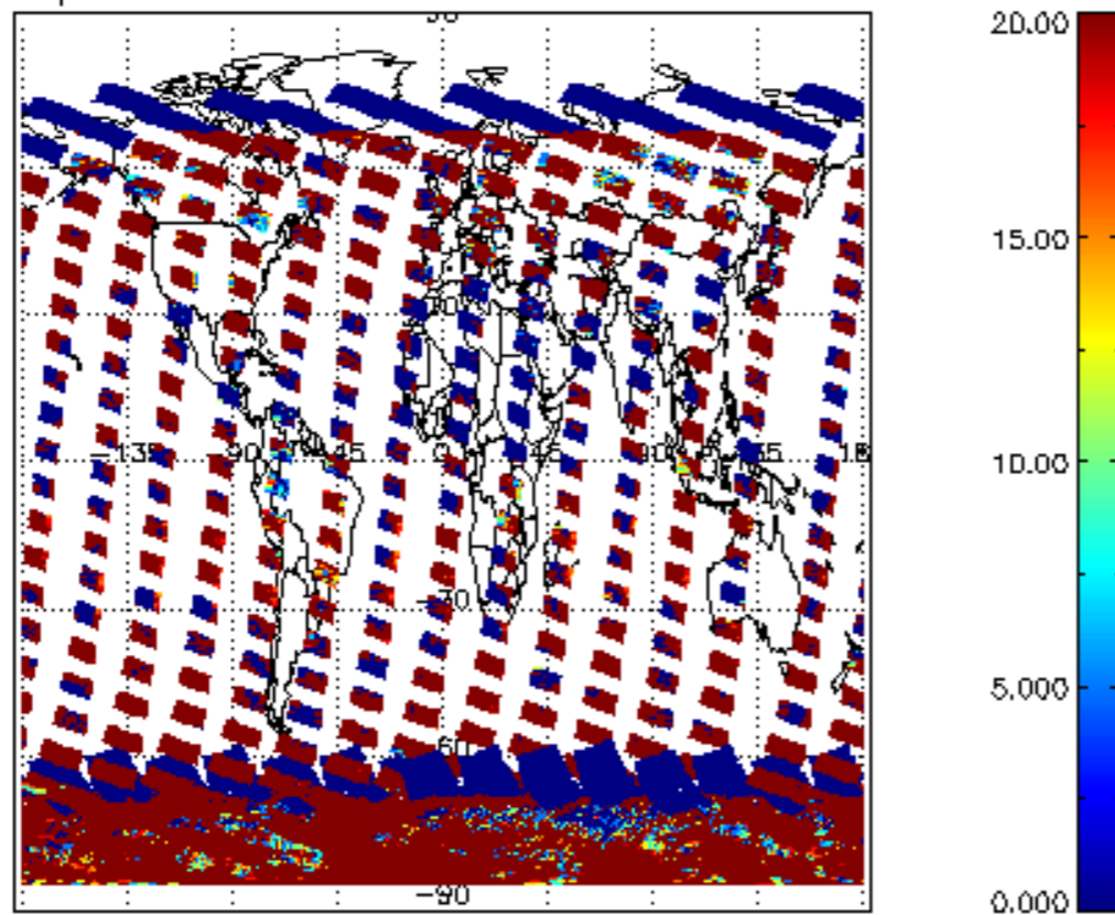
cLopt_depth for 11JAN2011 00:00:00 to 12JAN2011 00:00:00
