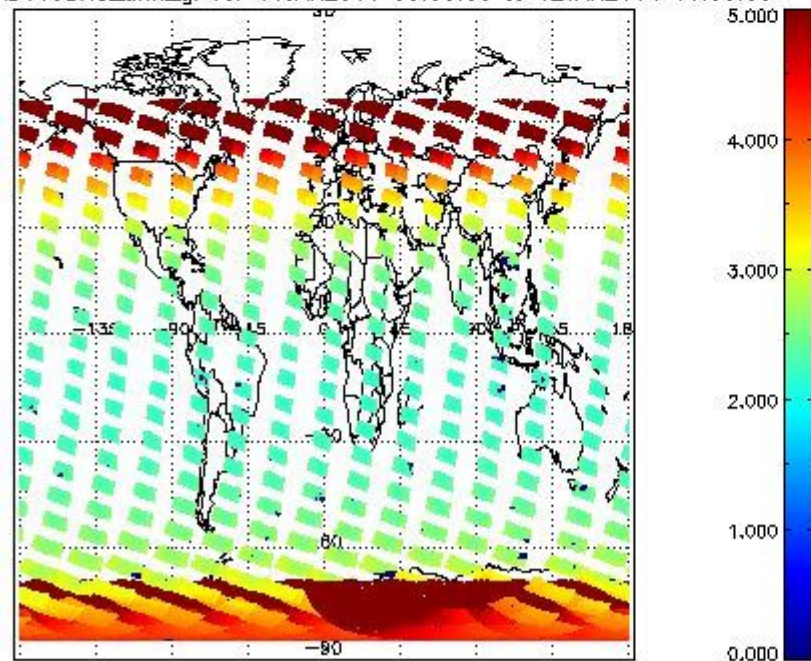
SCIOL2P_NADUV3BRO_amf_gr for 11JAN2011 00:00:00 to 12JAN2011 00:00:00
