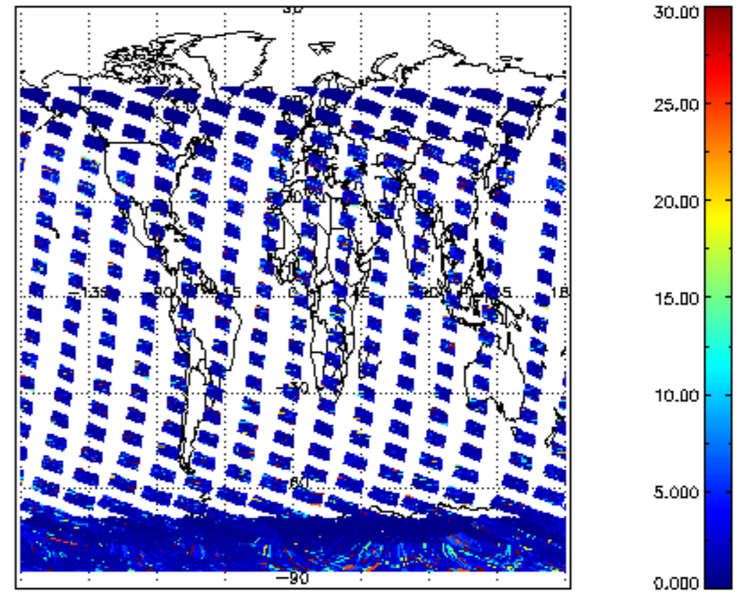
SCIOL2P_NADUV7S02_vcd_err for 11JAN2011 00:00:00 to 12JAN2011 00:00:00
