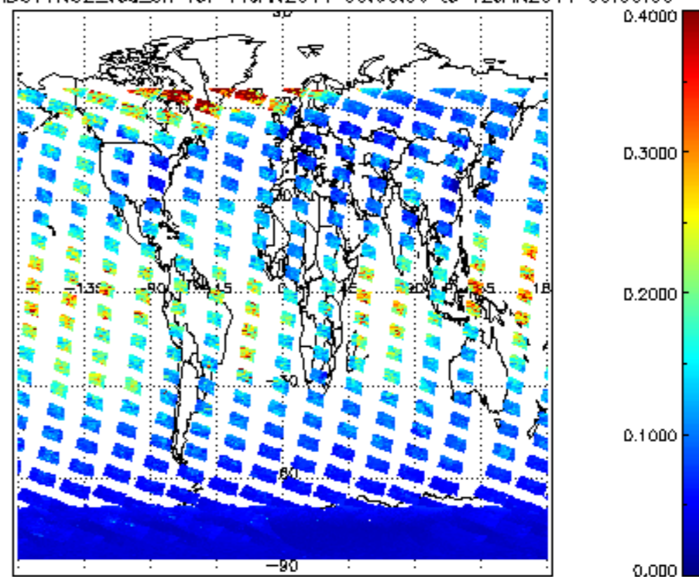
SCIOL2P_NADUV1NO2_vcd_err for 11JAN2011 00:00:00 to 12JAN2011 00:00:00
