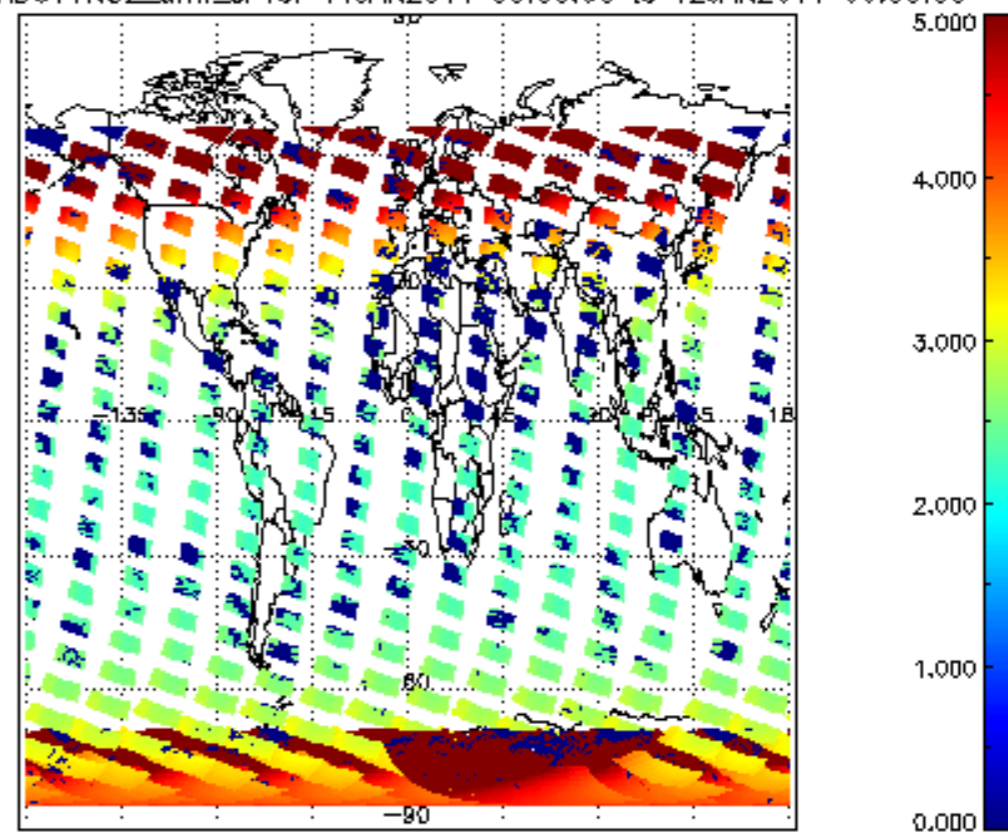
SCIOL2P_NADUV1NO2_amf_cl for 11JAN2011 00:00:00 to 12JAN2011 00:00:00
