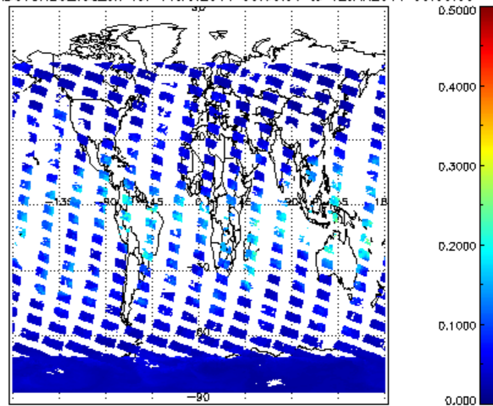
SCIOL2P_NADUV8H20_vcd_err for 11JAN2011 00:00:00 to 12JAN2011 00:00:00
