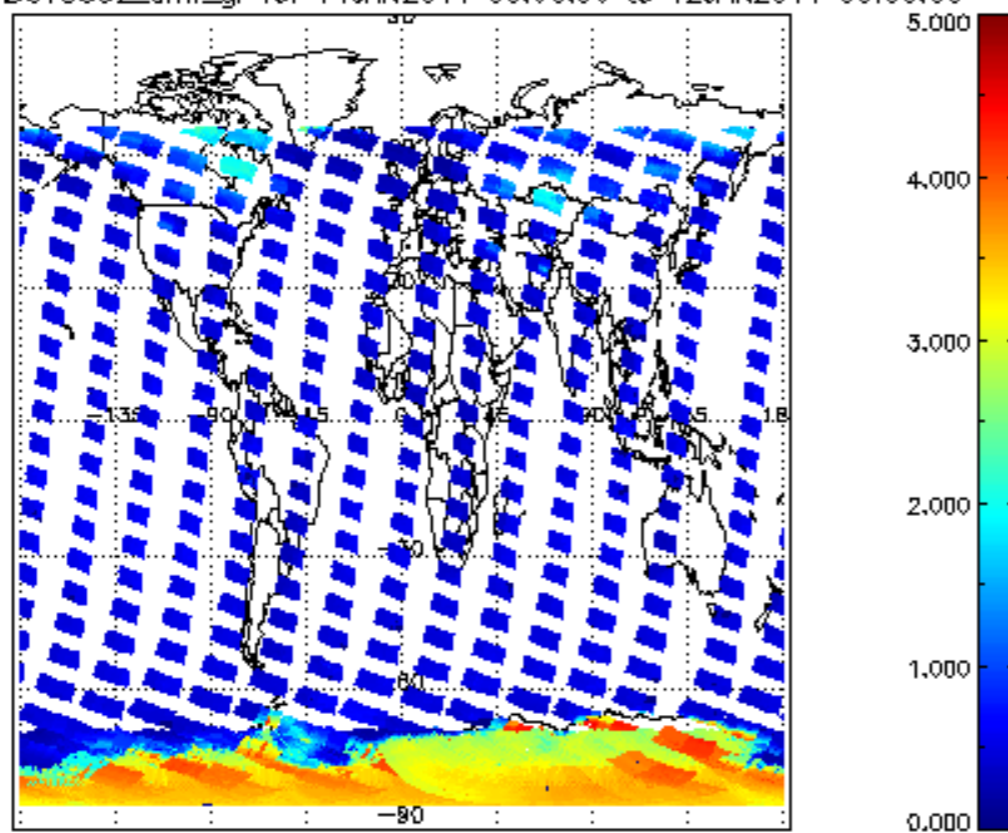
SCIOL2P_NADUV5S02_amf_gr for 11JAN2011 00:00:00 to 12JAN2011 00:00:00
