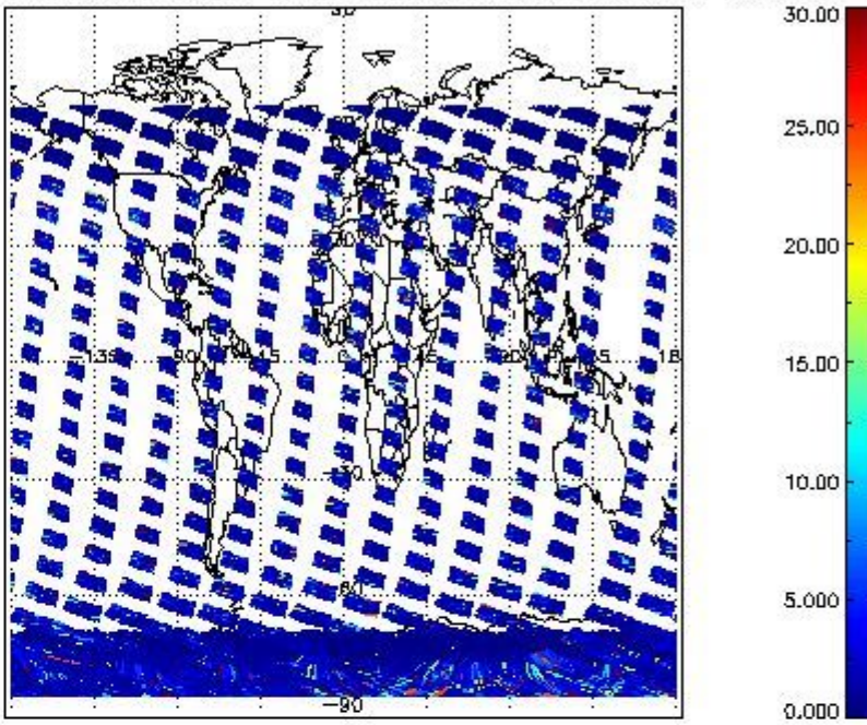
SCIOL2P_NADUV5S02_vcd_err for 11JAN2011 00:00:00 to 12JAN2011 00:00:00
