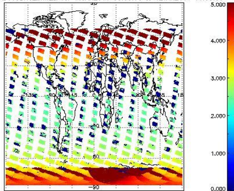
SCIOL2P_NADUV3BRO_amf_cl for 11JAN2011 00:00:00 to 12JAN2011 00:00:00
