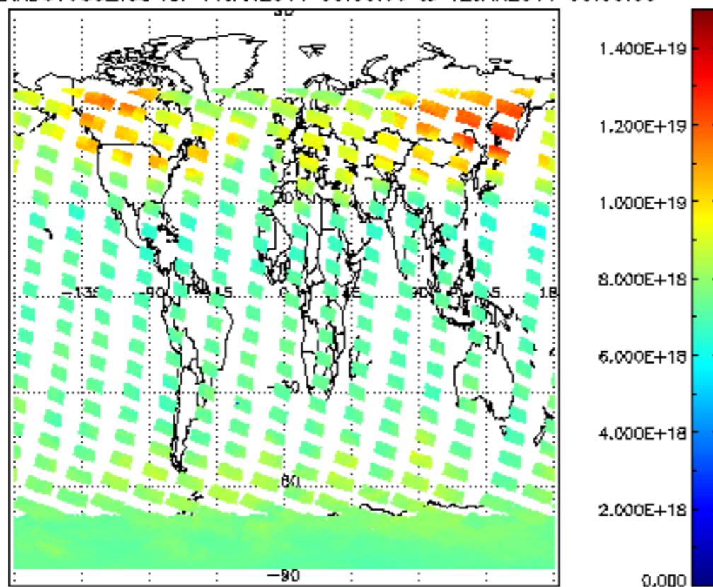
SCIOL2P_NADUV003_vcd for 11JAN2011 00:00:00 to 12JAN2011 00:00:00
