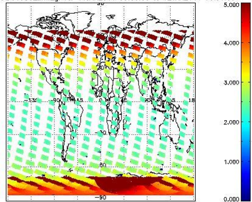
SCIOL2P_NADUV003_amf_gr for 11JAN2011 00:00:00 to 12JAN2011 00:00:00
