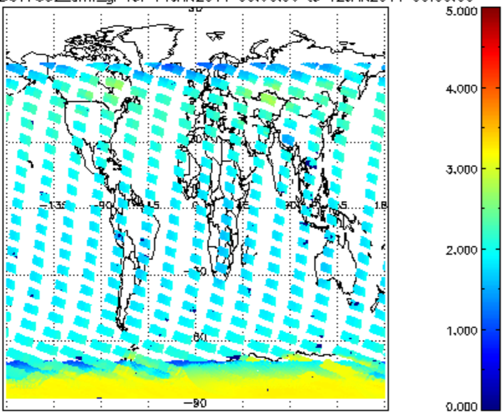
SCIOL2P_NADUV7S02_amf_gr for 11JAN2011 00:00:00 to 12JAN2011 00:00:00
