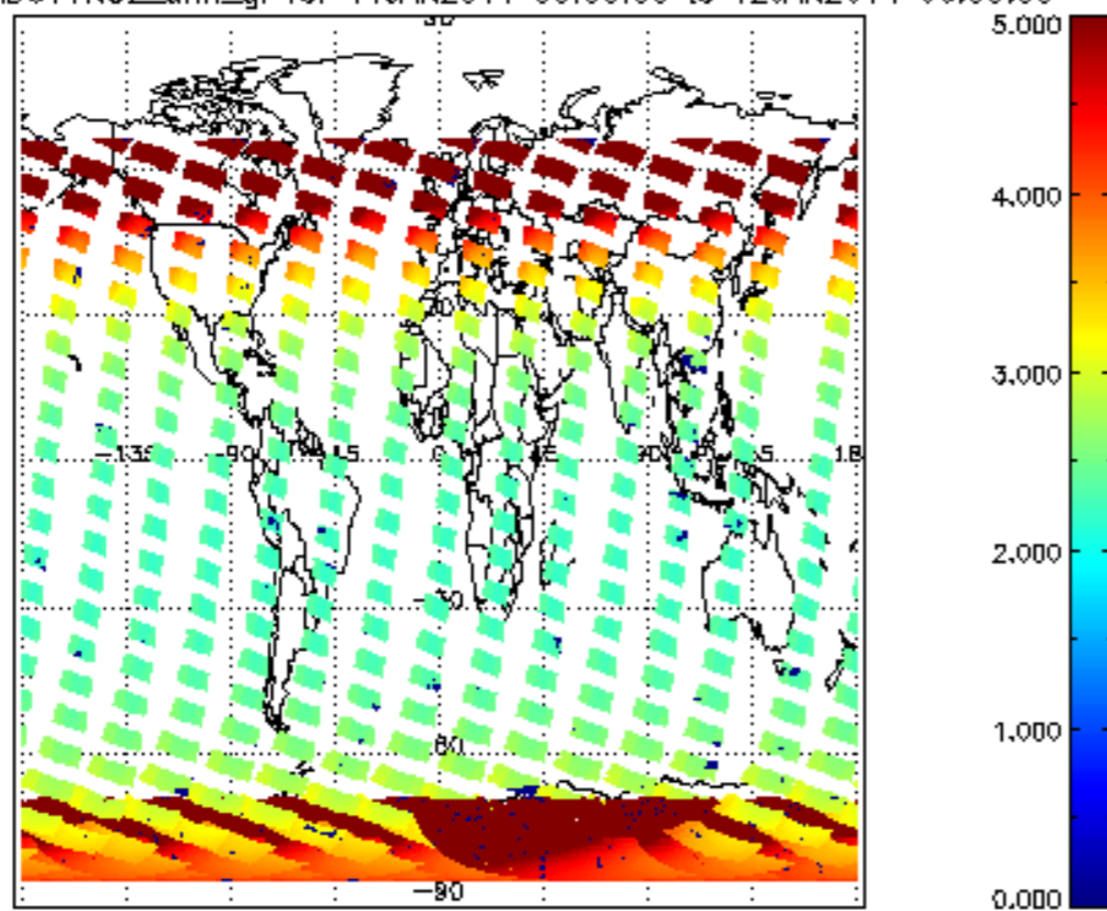
SCIOL2P_NADUV1NO2_amf_gr for 11JAN2011 00:00:00 to 12JAN2011 00:00:00
