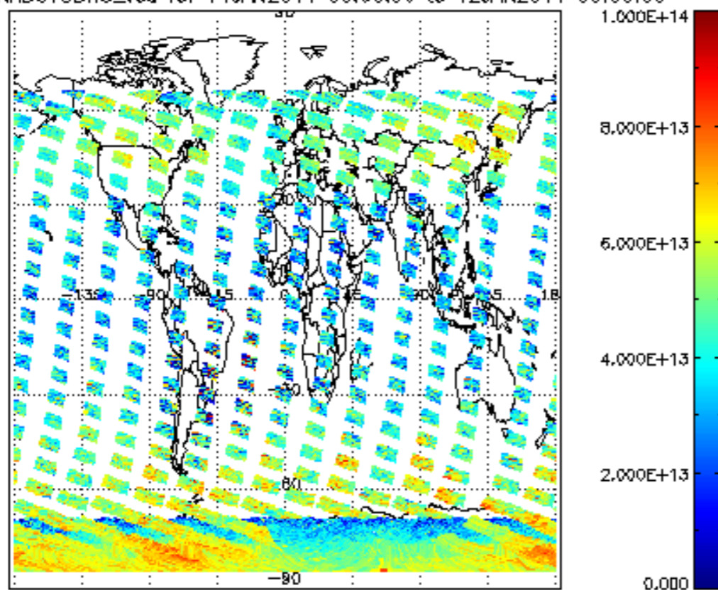
SCIOL2P_NADUV3BRO_vcd for 11JAN2011 00:00:00 to 12JAN2011 00:00:00
