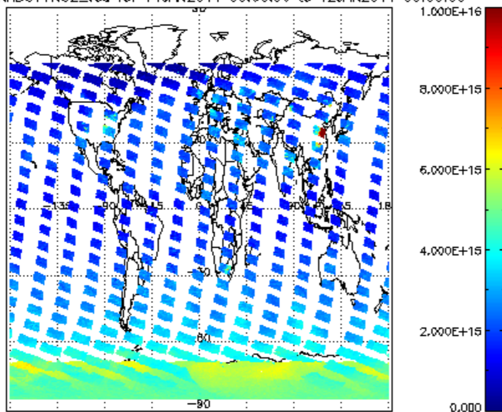
SCIOL2P_NADUV1NO2_vcd for 11JAN2011 00:00:00 to 12JAN2011 00:00:00
