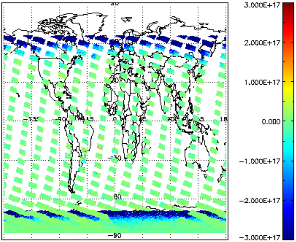
SCIOL2P_NADUV7S02_vcd for 11JAN2011 00:00:00 to 12JAN2011 00:00:00
