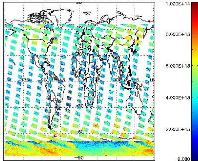
SCIOL2P_NADUV3BRO_vcd for 11JAN2011 00:00:00 to 12JAN2011 00:00:00
