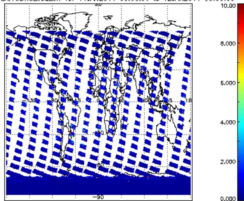
SCIOL2P_NADUV3BRO_vcd_err for 11JAN2011 00:00:00 to 12JAN2011 00:00:00
