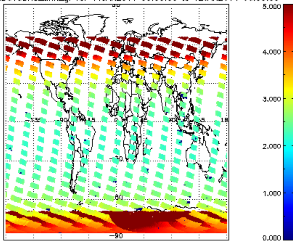
SCIOL2P_NADUV3BRO_amf_gr for 11JAN2011 00:00:00 to 12JAN2011 00:00:00
