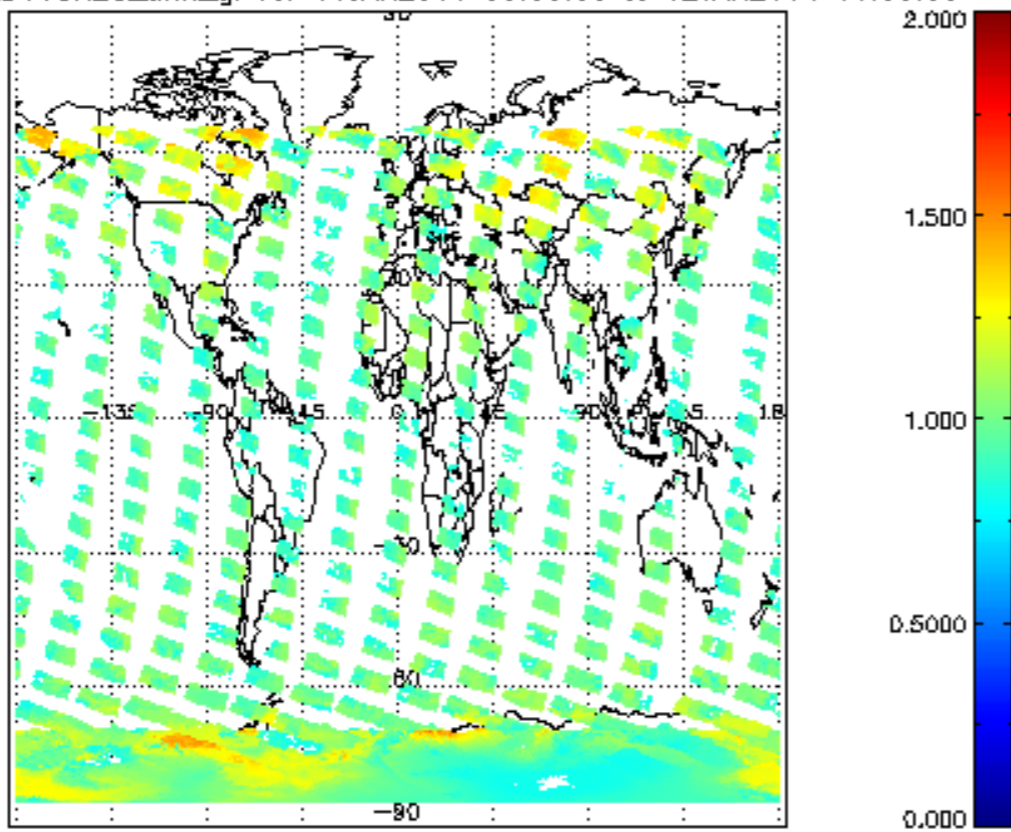
SCIOL2P_NADUV8H20_amf_gr for 11JAN2011 00:00:00 to 12JAN2011 00:00:00
