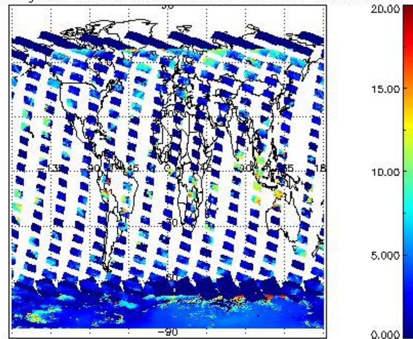
cL_top_height for 11JAN2011 00:00:00 to 12JAN2011 00:00:00
