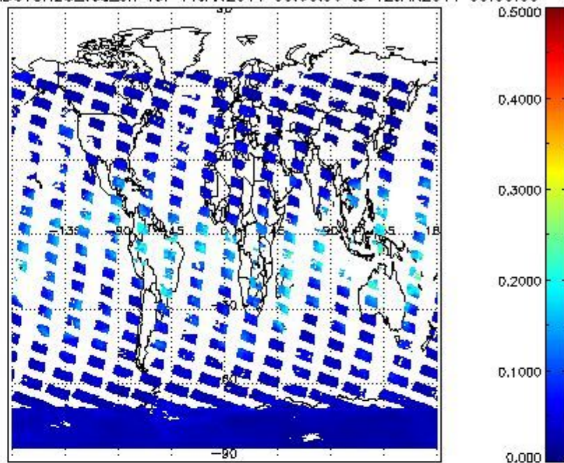
SCIOL2P_NADUV8H20_vcd_err for 11JAN2011 00:00:00 to 12JAN2011 00:00:00
