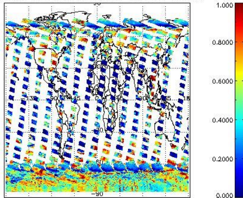
cL_frac for 11JAN2011 00:00:00 to 12JAN2011 00:00:00
