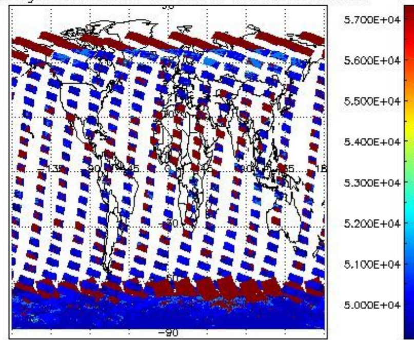
cloud_flags for 11JAN2011 00:00:00 to 12JAN2011 00:00:00
