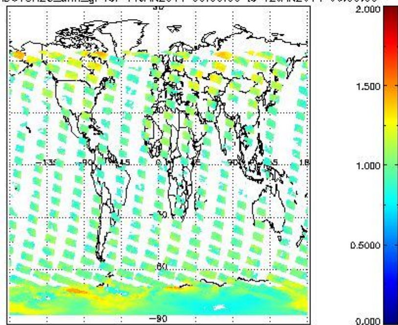
SCIOL2P_NADUV8H20_amf_gr for 11JAN2011 00:00:00 to 12JAN2011 00:00:00
