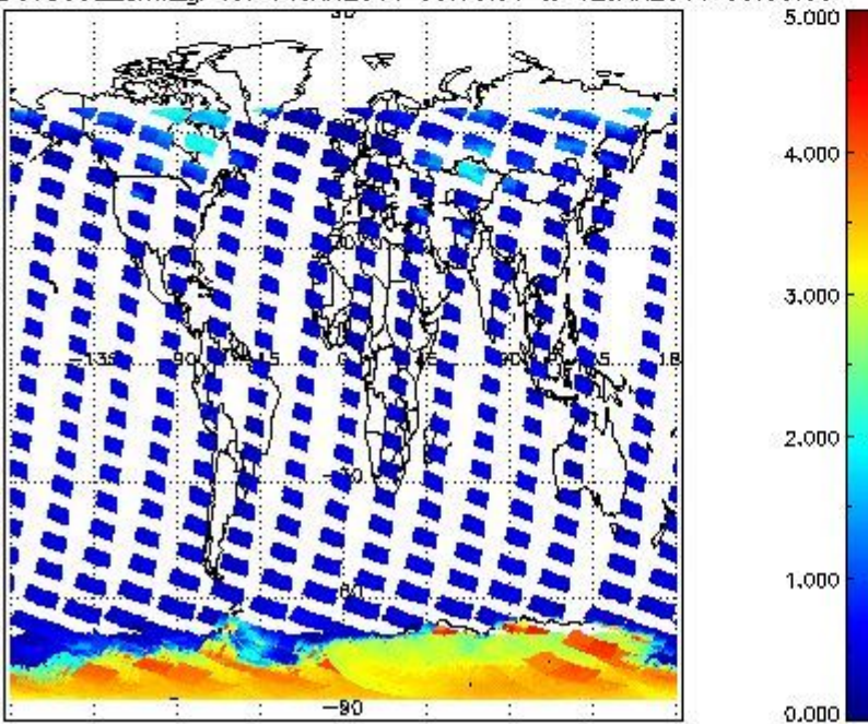
SCIOL2P_NADUV5S02_amf_gr for 11JAN2011 00:00:00 to 12JAN2011 00:00:00
