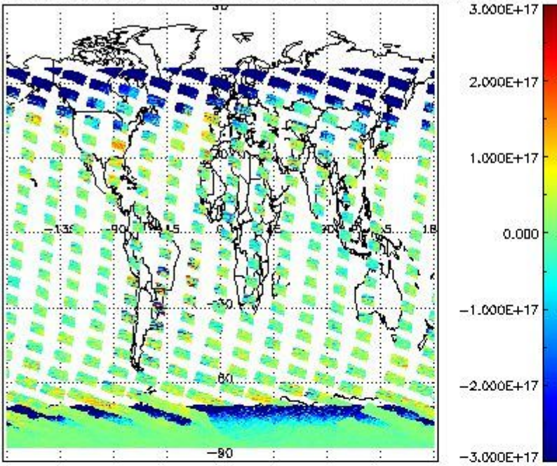
SCIOL2P_NADUV5S02_vcd for 11JAN2011 00:00:00 to 12JAN2011 00:00:00
