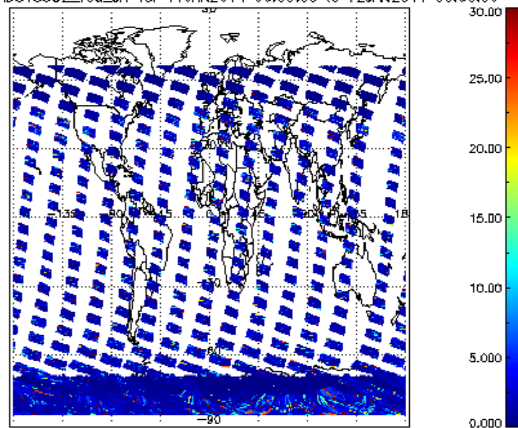
SCIOL2P_NADUV5S02_vcd_err for 11JAN2011 00:00:00 to 12JAN2011 00:00:00
