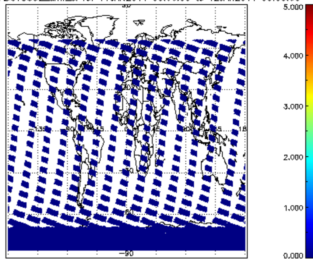
SCIOL2P_NADUV5S02_amf_sl for 11JAN2011 00:00:00 to 12JAN2011 00:00:00
