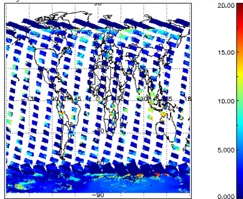
cL_top_height for 11JAN2011 00:00:00 to 12JAN2011 00:00:00
