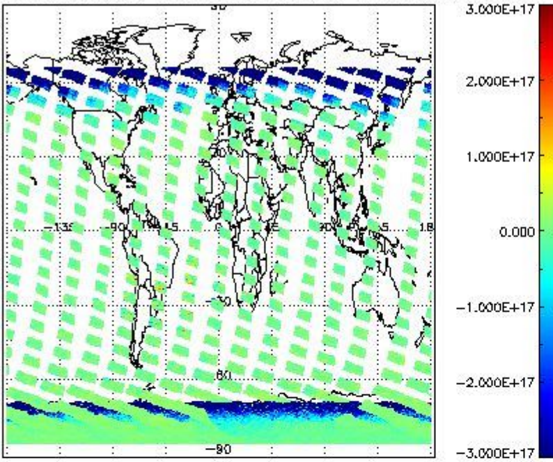
SCIOL2P_NADUV7S02_vcd for 11JAN2011 00:00:00 to 12JAN2011 00:00:00
