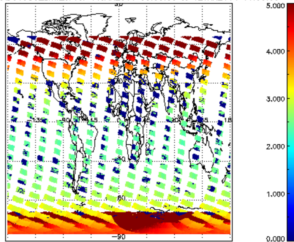
SCIOL2P_NADUV003_amf_cl for 11JAN2011 00:00:00 to 12JAN2011 00:00:00
