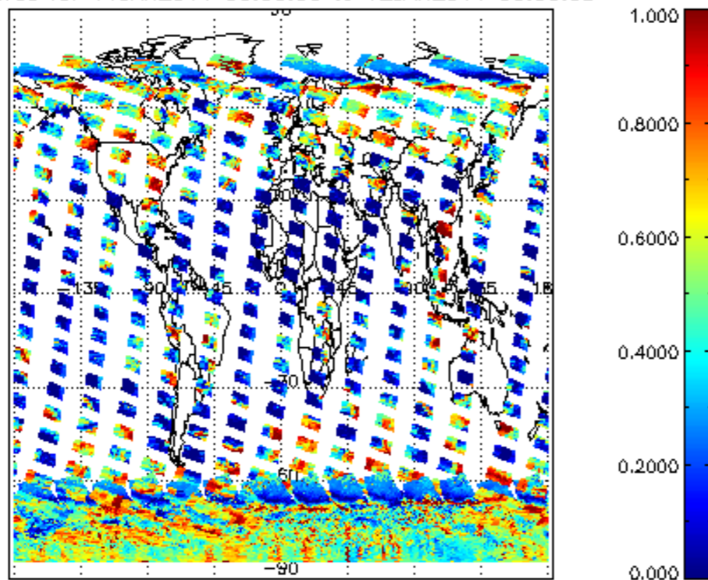
cL_frac for 11JAN2011 00:00:00 to 12JAN2011 00:00:00
