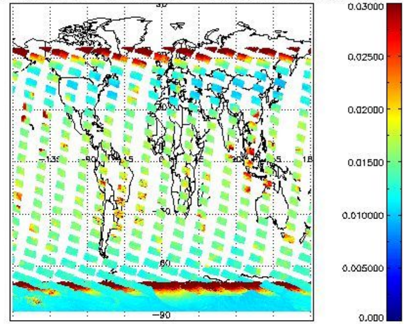
SCIOL2P_NADUV003_vcd_err for 11JAN2011 00:00:00 to 12JAN2011 00:00:00
