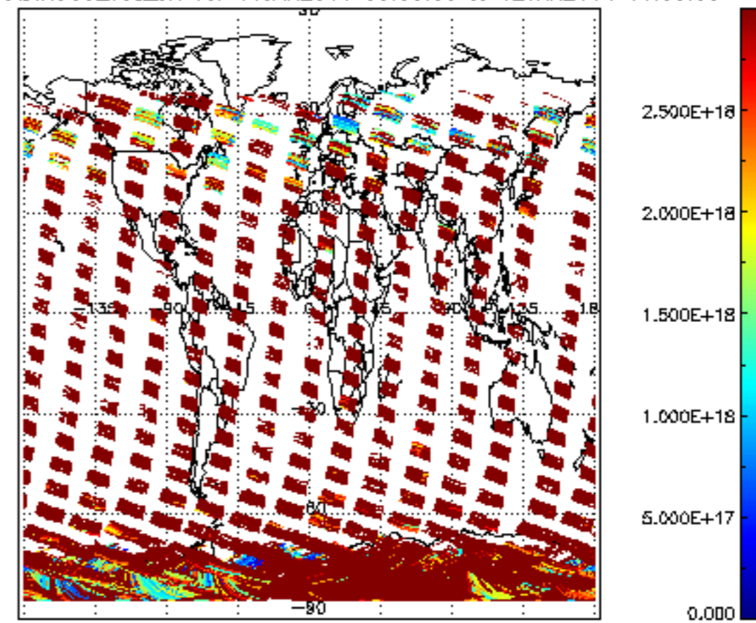
SCIOL2P_NADIR3CO_vcd_err for 11JAN2011 00:00:00 to 12JAN2011 00:00:00
