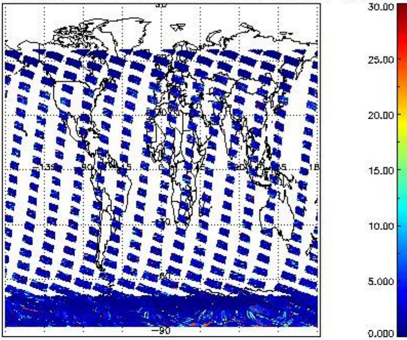
SCIOL2P_NADUV7S02_vcd_err for 11JAN2011 00:00:00 to 12JAN2011 00:00:00
