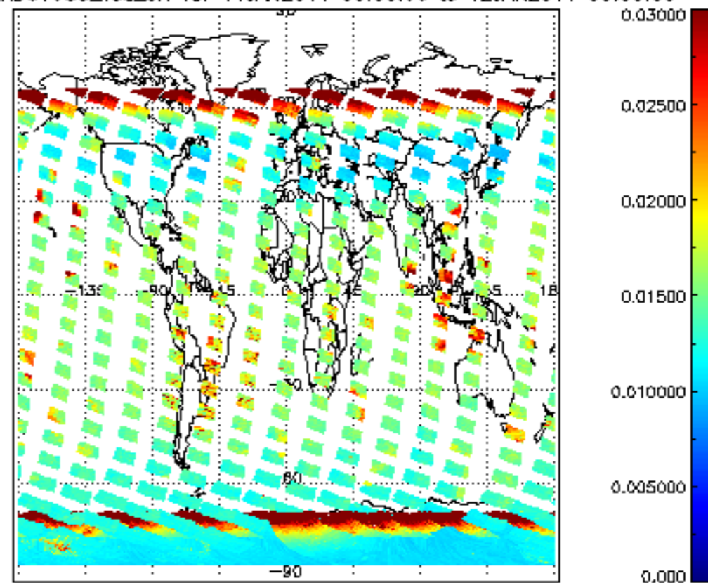
SCIOL2P_NADUV003_vcd_err for 11JAN2011 00:00:00 to 12JAN2011 00:00:00
