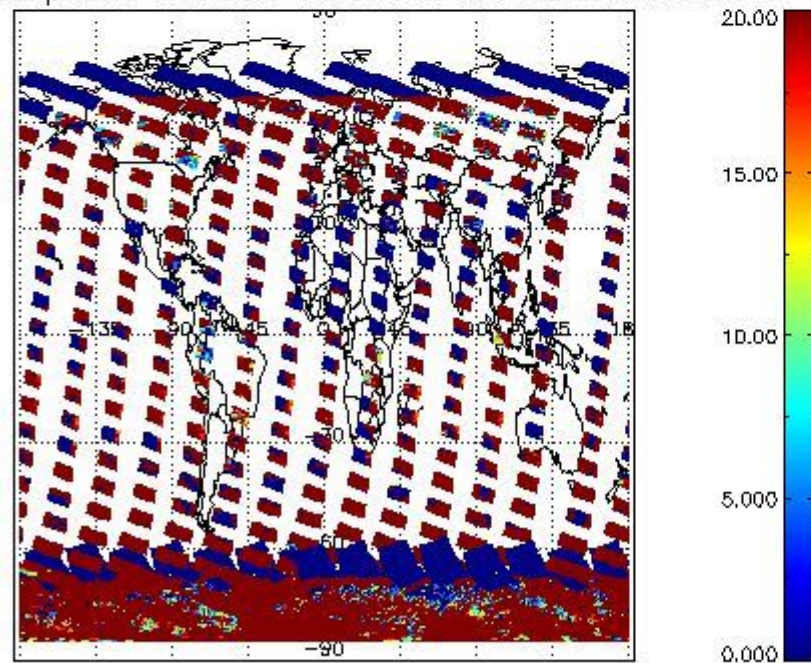
cLopt_depth for 11JAN2011 00:00:00 to 12JAN2011 00:00:00
