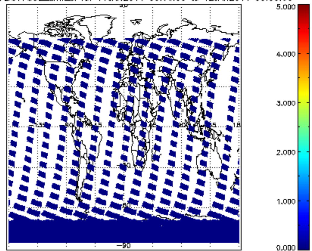
SCIOL2P_NADUV7S02_amf_cl for 11JAN2011 00:00:00 to 12JAN2011 00:00:00
