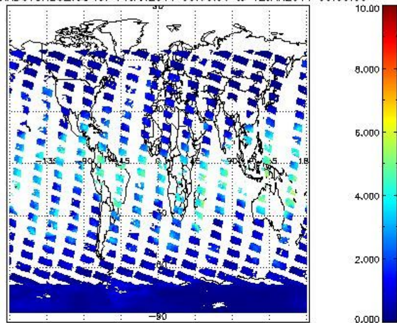
SCIOL2P_NADUV8H20_vcd for 11JAN2011 00:00:00 to 12JAN2011 00:00:00
