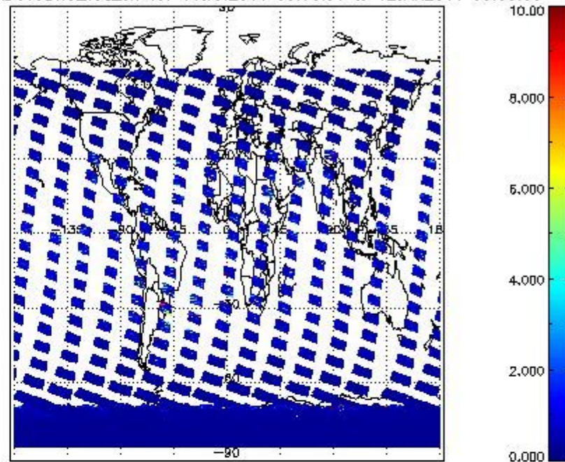
SCIOL2P_NADUV3BRO_vcd_err for 11JAN2011 00:00:00 to 12JAN2011 00:00:00
