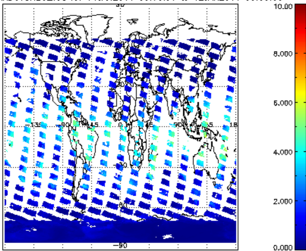
SCIOL2P_NADUV8H20_vcd for 11JAN2011 00:00:00 to 12JAN2011 00:00:00
