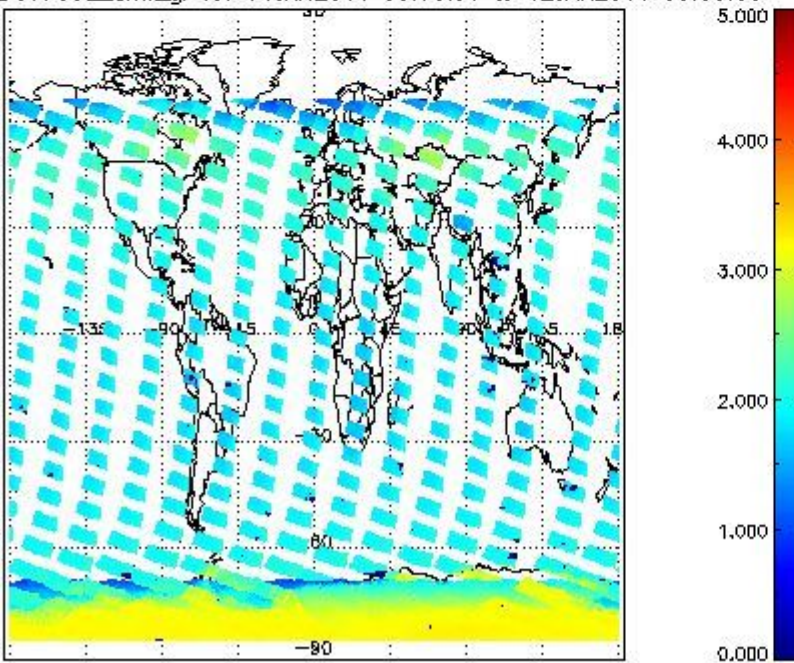
SCIOL2P_NADUV7S02_amf_gr for 11JAN2011 00:00:00 to 12JAN2011 00:00:00
