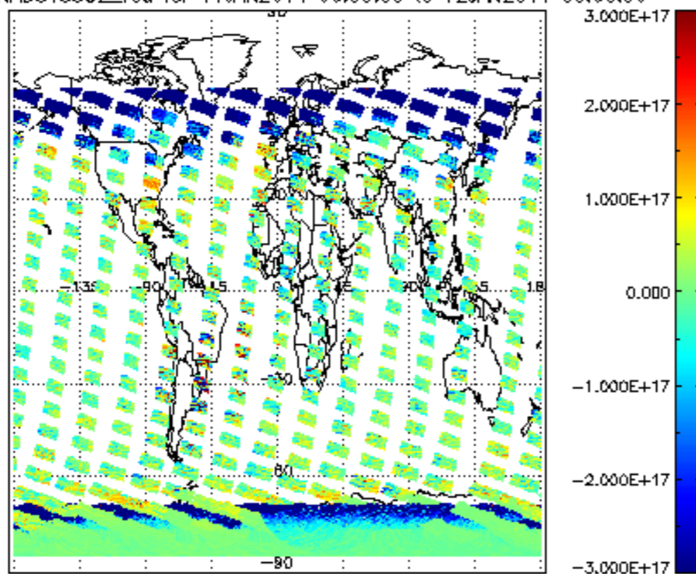
SCIOL2P_NADUV5S02_vcd for 11JAN2011 00:00:00 to 12JAN2011 00:00:00
