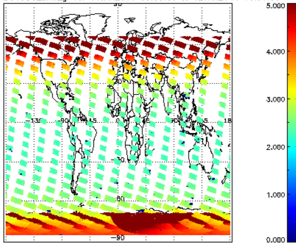
SCIOL2P_NADUV003_amf_gr for 11JAN2011 00:00:00 to 12JAN2011 00:00:00
