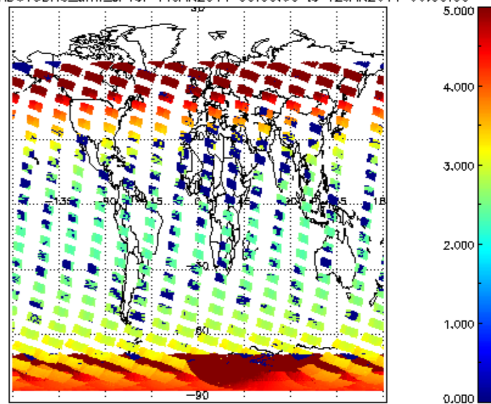
SCIOL2P_NADUV3BRO_amf_cl for 11JAN2011 00:00:00 to 12JAN2011 00:00:00
