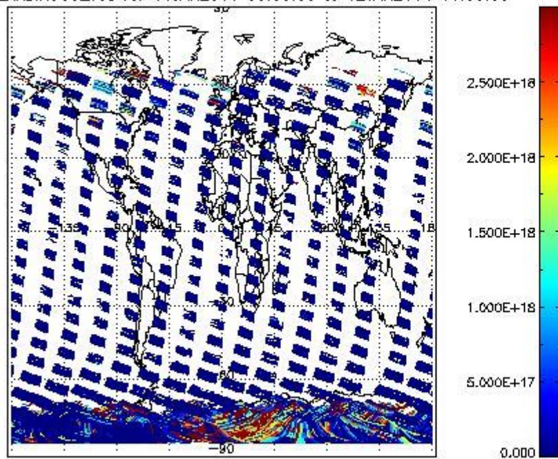
SCIDL2P_NADIR3CO_vcd for 11JAN2011 00:00:00 to 12JAN2011 00:00:00
