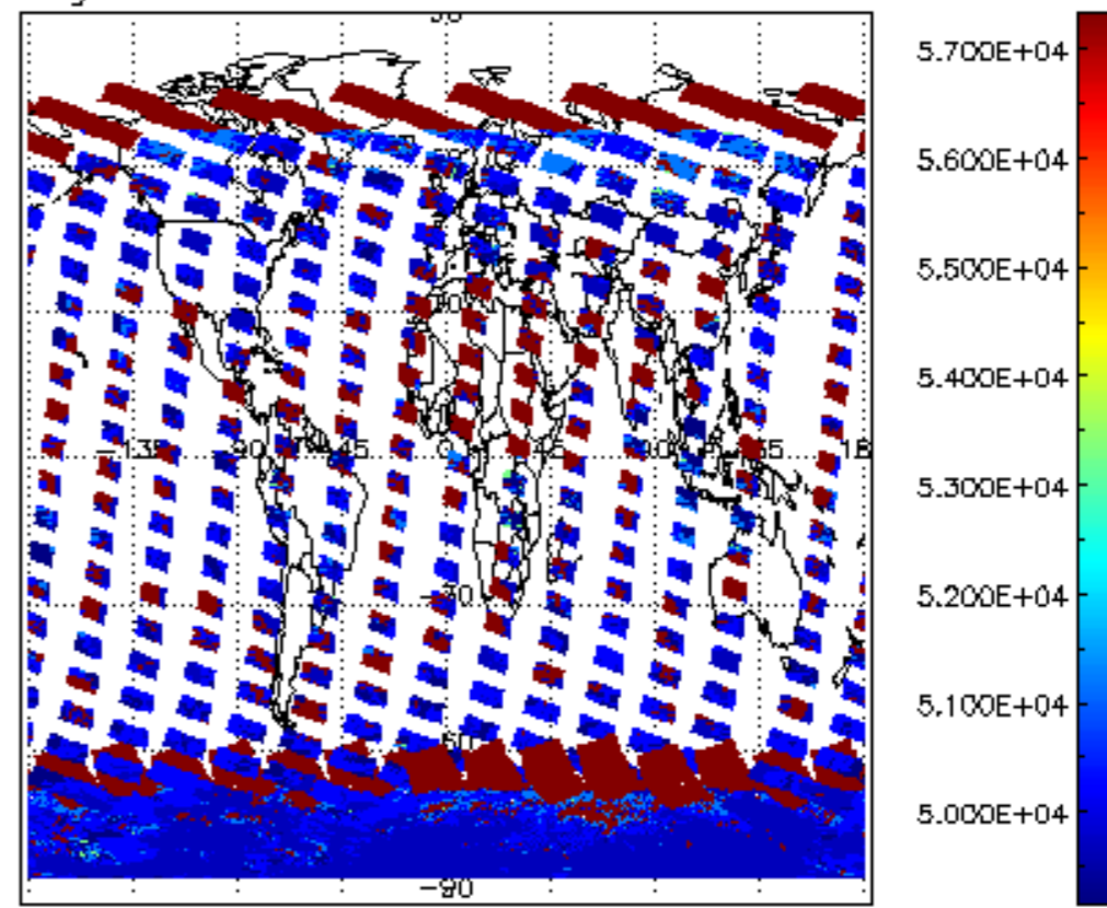
cloud_flags for 11JAN2011 00:00:00 to 12JAN2011 00:00:00
