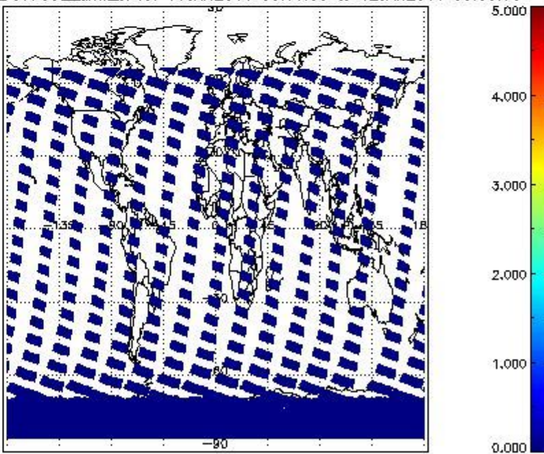
SCIOL2P_NADUV7S02_amf_cl for 11JAN2011 00:00:00 to 12JAN2011 00:00:00
