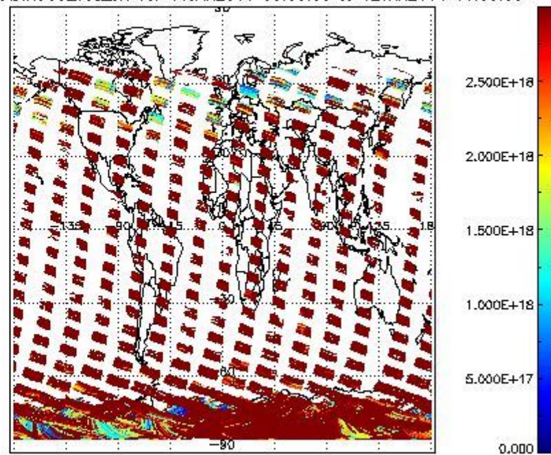
SCIDL2P_NADIR3CO_vcd_err for 11JAN2011 00:00:00 to 12JAN2011 00:00:00
