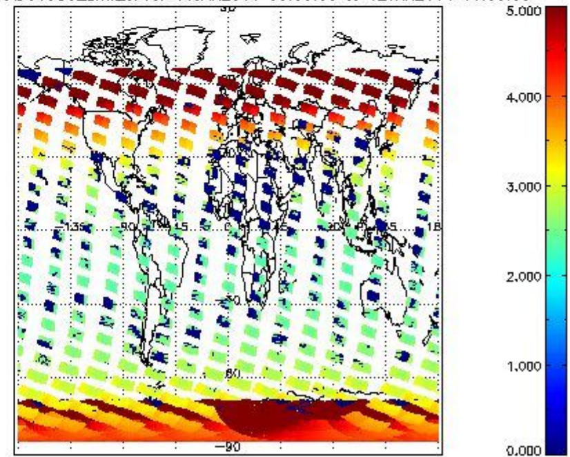
SCIOL2P_NADUV003_amf_cl for 11JAN2011 00:00:00 to 12JAN2011 00:00:00
