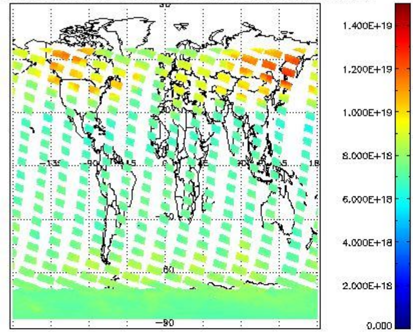
SCIOL2P_NADUV003_vcd for 11JAN2011 00:00:00 to 12JAN2011 00:00:00
