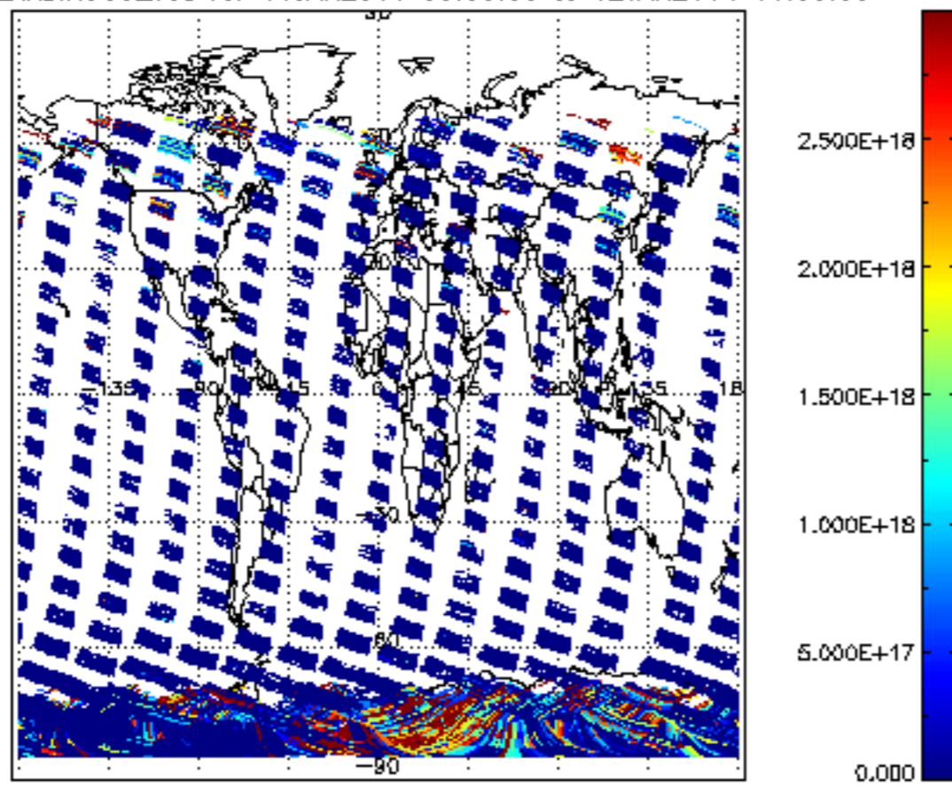
SCIOL2P_NADIR3CO_vcd for 11JAN2011 00:00:00 to 12JAN2011 00:00:00
