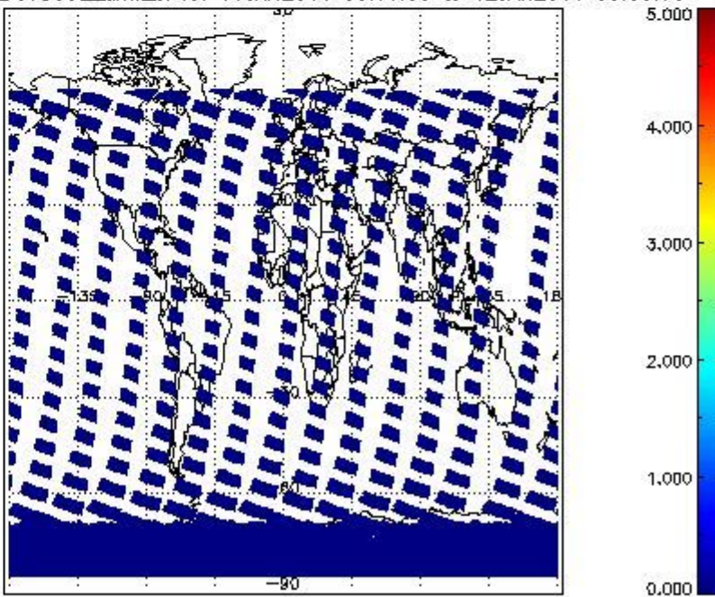
SCIOL2P_NADUV5S02_amf_cl for 11JAN2011 00:00:00 to 12JAN2011 00:00:00
