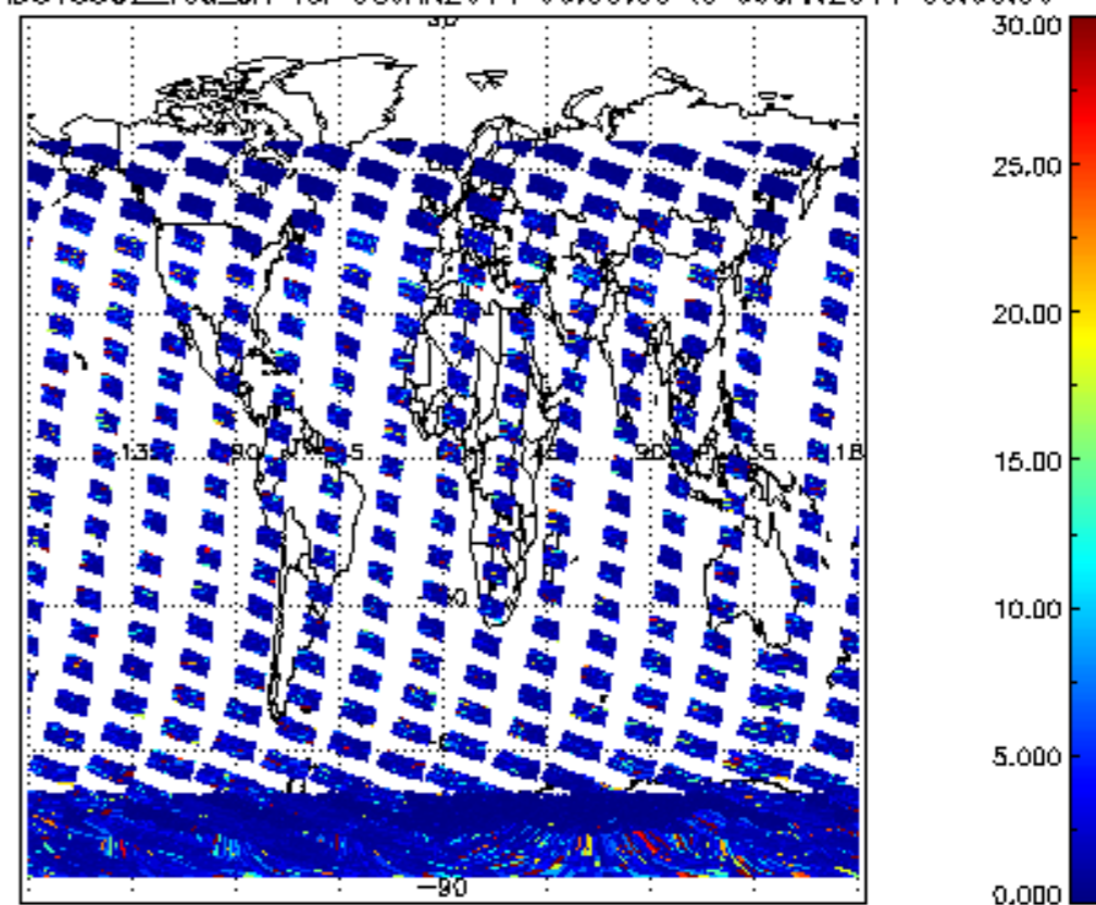
SCIOL2P_NADUV5S02_vcd_err for 08JAN2011 00:00:00 to 09JAN2011 00:00:00
