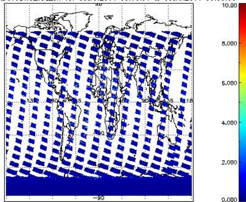
SCIOL2P_NADUV3BRO_vcd_err for 08JAN2011 00:00:00 to 09JAN2011 00:00:00
