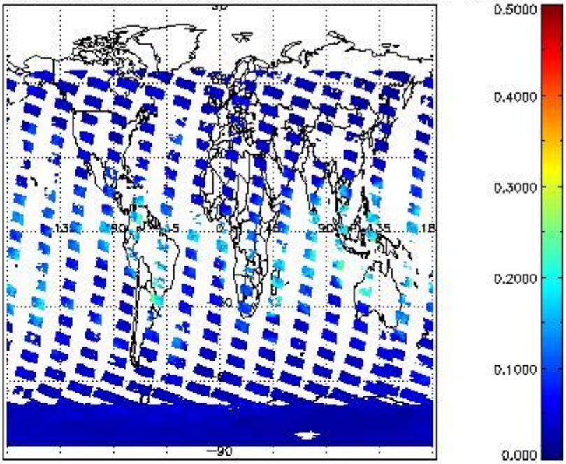
SCIOL2P_NADUV8H20_vcd_err for 08JAN2011 00:00:00 to 09JAN2011 00:00:00
