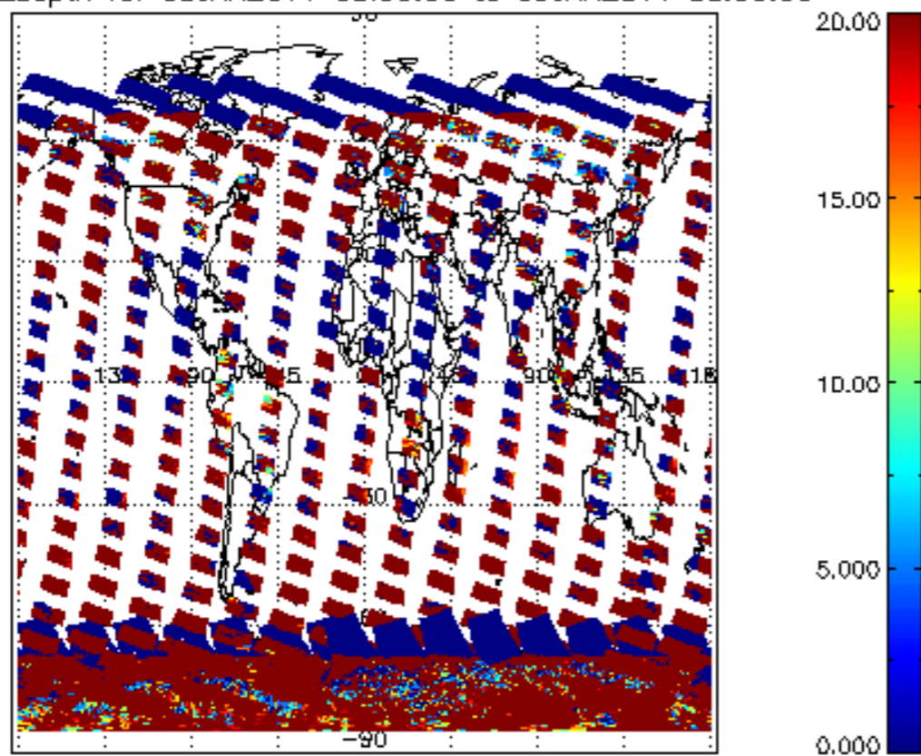
cLopt_depth for 08JAN2011 00:00:00 to 09JAN2011 00:00:00
