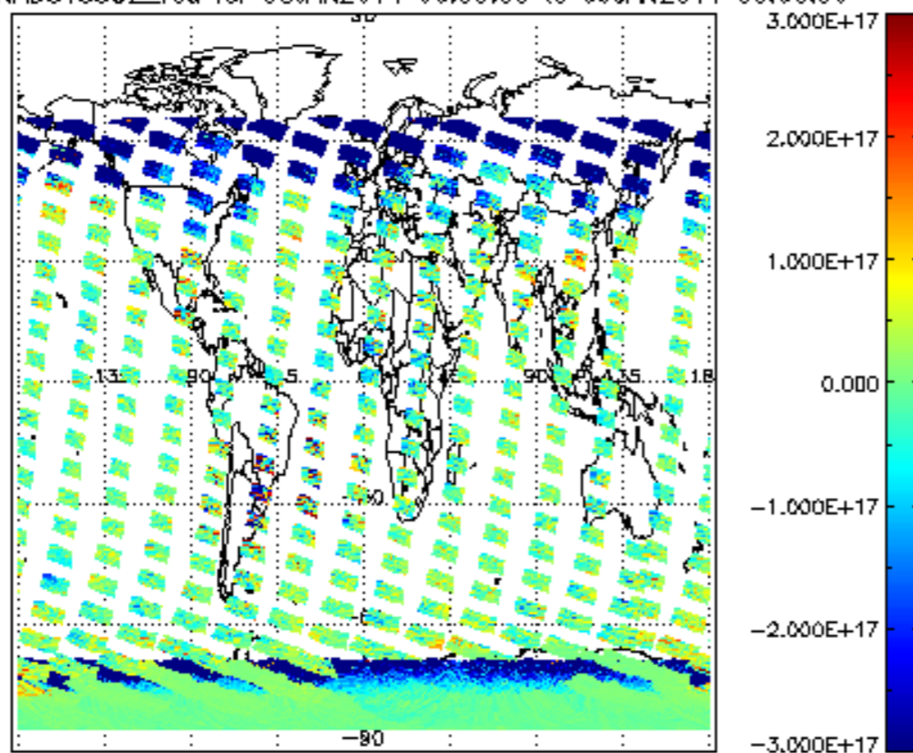
SCIOL2P_NADUV5S02_vcd for 08JAN2011 00:00:00 to 09JAN2011 00:00:00
