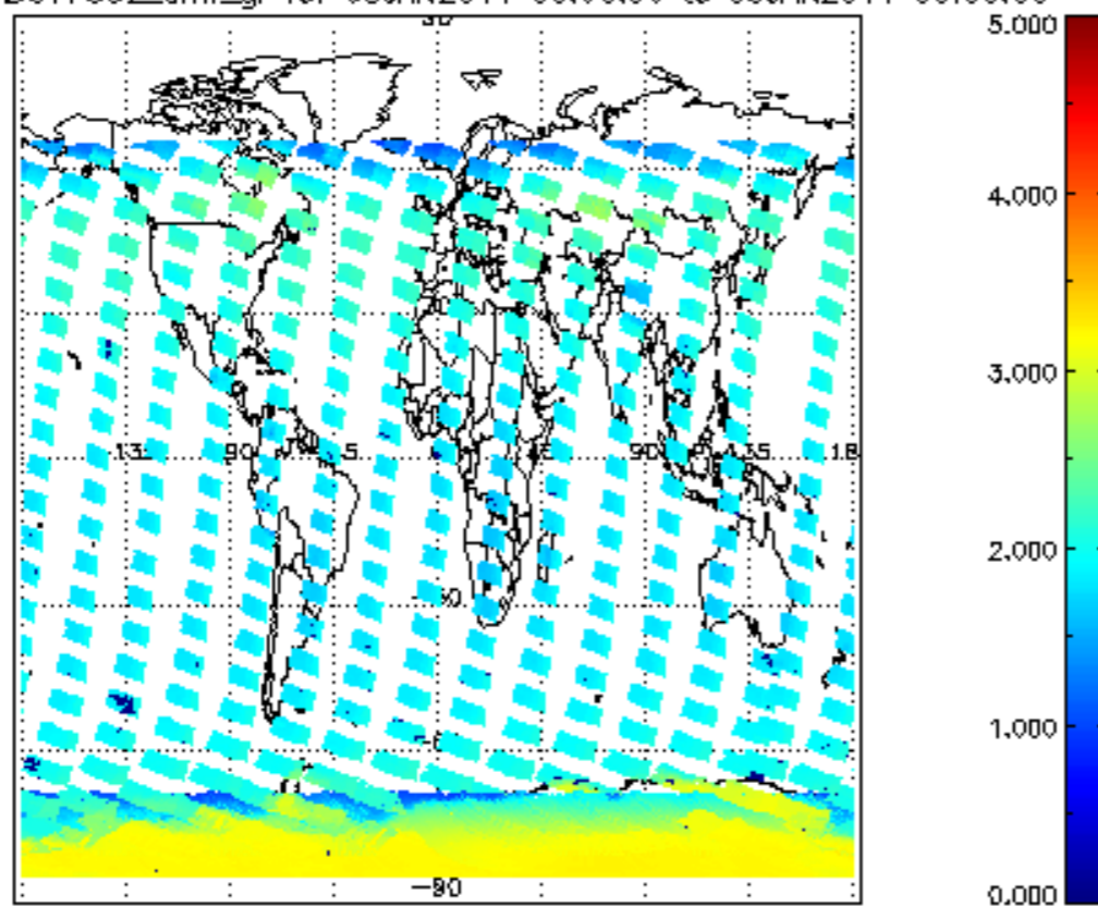
SCIOL2P_NADUV7S02_amf_gr for 08JAN2011 00:00:00 to 09JAN2011 00:00:00
