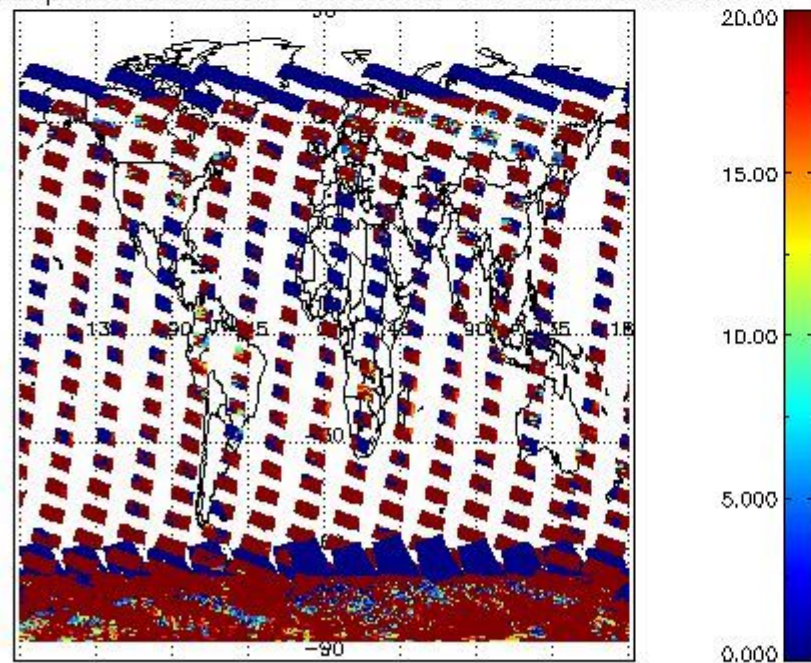
cL_opt_depth for 08JAN2011 00:00:00 to 09JAN2011 00:00:00
