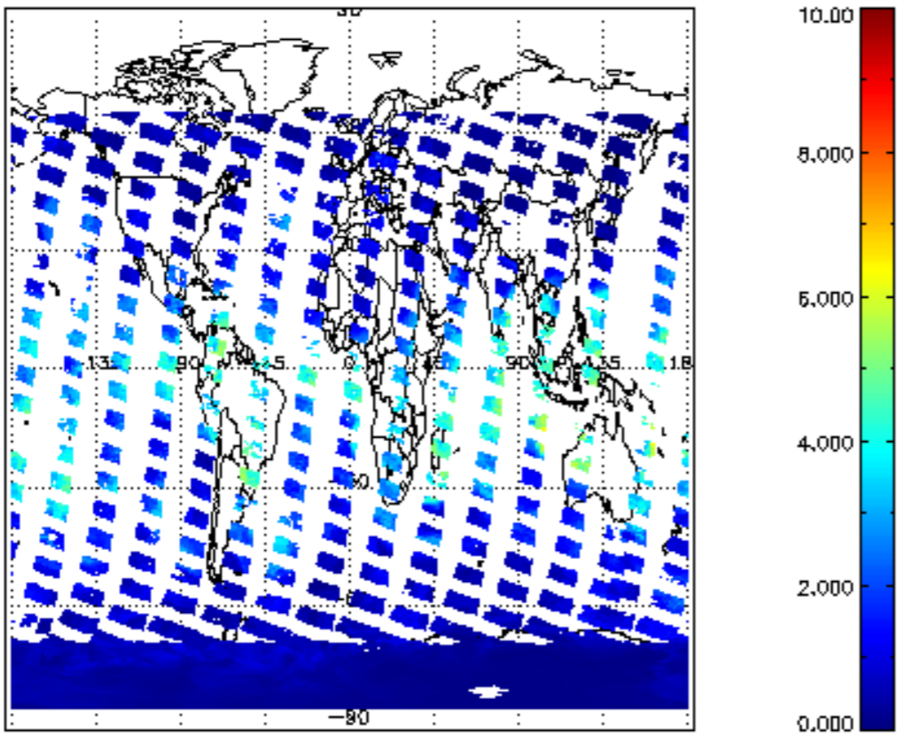
SCIOL2P_NADUV8H20_vcd for 08JAN2011 00:00:00 to 09JAN2011 00:00:00
