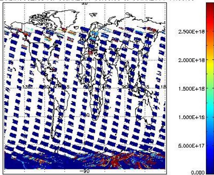
SCIDL2P_NADIR3CO_vcd for 08JAN2011 00:00:00 to 09JAN2011 00:00:00
