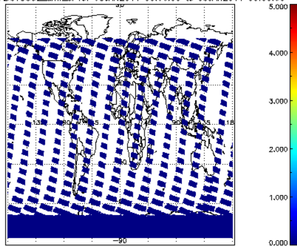
SCIOL2P_NADUV5S02_amf_cl for 08JAN2011 00:00:00 to 09JAN2011 00:00:00
