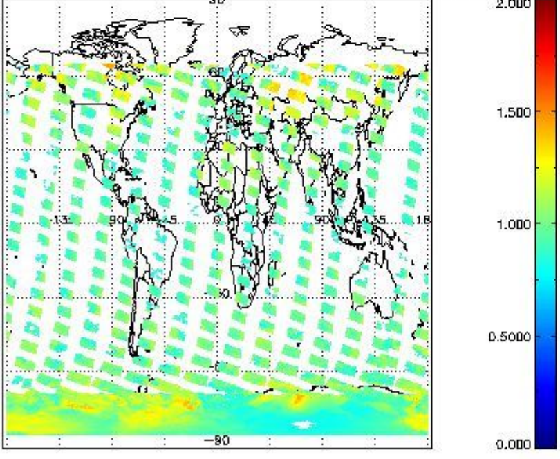
SCIOL2P_NADUV8H20_amf_gr for 08JAN2011 00:00:00 to 09JAN2011 00:00:00
