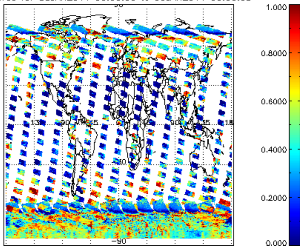
cL_frac for 08JAN2011 00:00:00 to 09JAN2011 00:00:00
