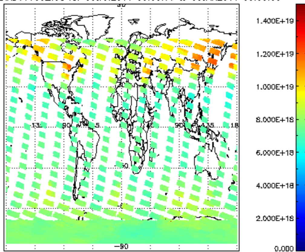
SCIOL2P_NADUV003_vcd for 08JAN2011 00:00:00 to 09JAN2011 00:00:00
