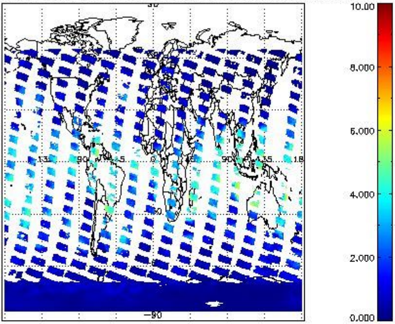
SCIOL2P_NADUV8H20_vcd for 08JAN2011 00:00:00 to 09JAN2011 00:00:00
