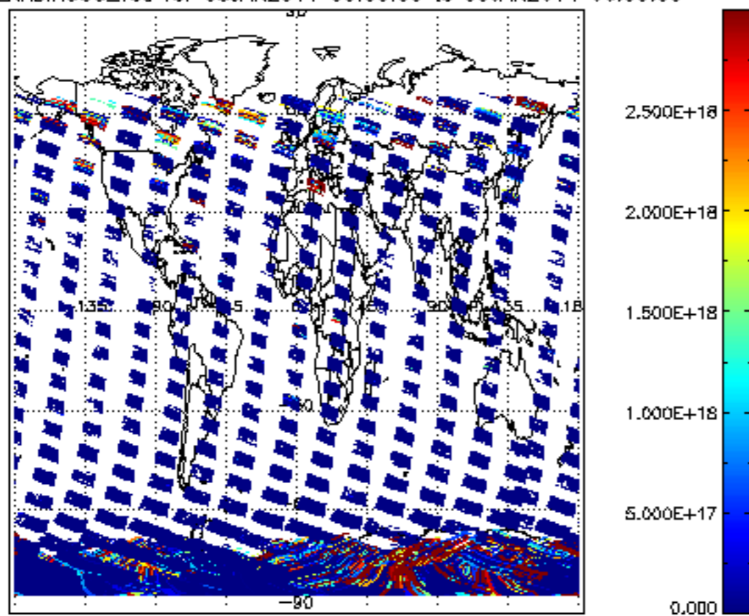
SCIOL2P_NADIR3CO_vcd for 08JAN2011 00:00:00 to 09JAN2011 00:00:00
