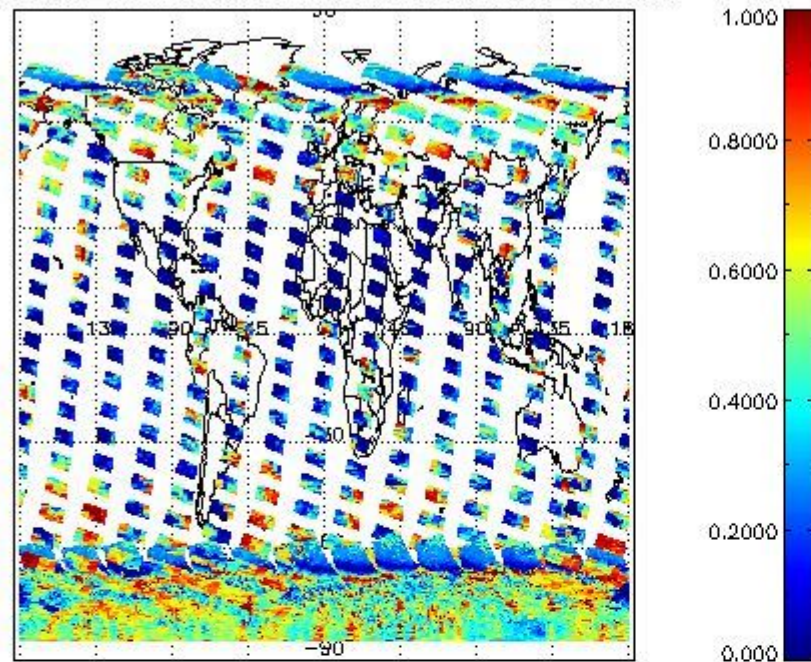
cL_frac for 08JAN2011 00:00:00 to 09JAN2011 00:00:00
