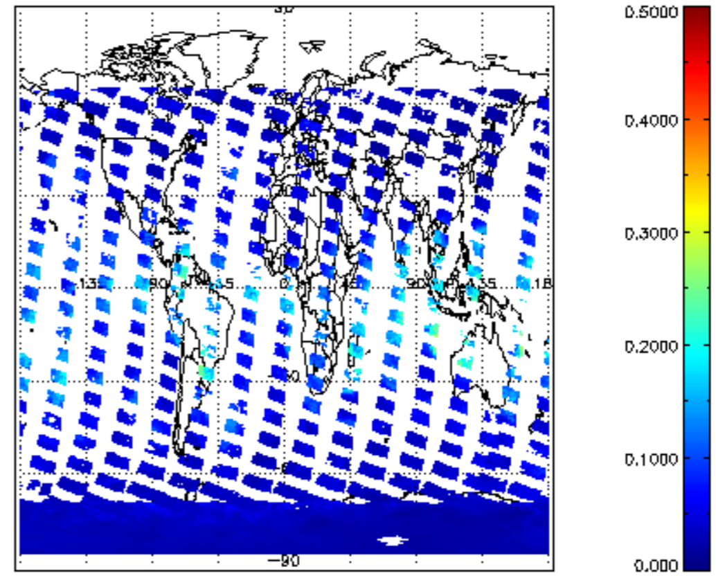
SCIOL2P_NADUV8H20_vcd_err for 08JAN2011 00:00:00 to 09JAN2011 00:00:00
