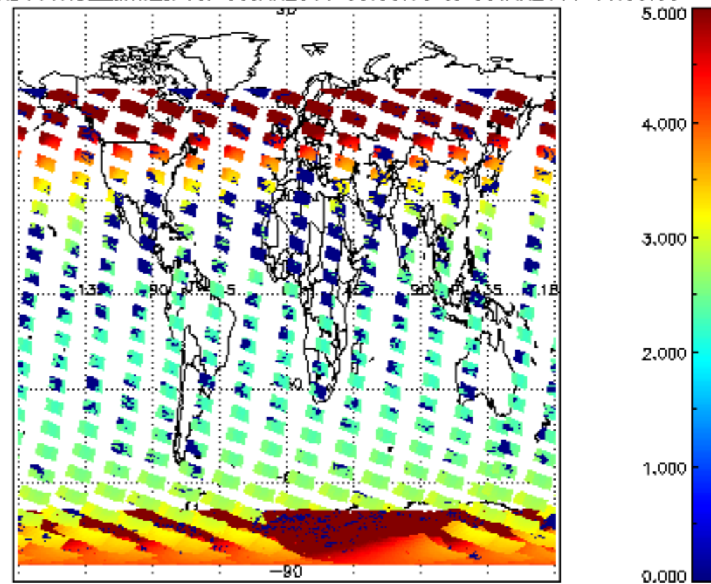
SCIOL2P_NADUV1NO2_amf_cl for 08JAN2011 00:00:00 to 09JAN2011 00:00:00
