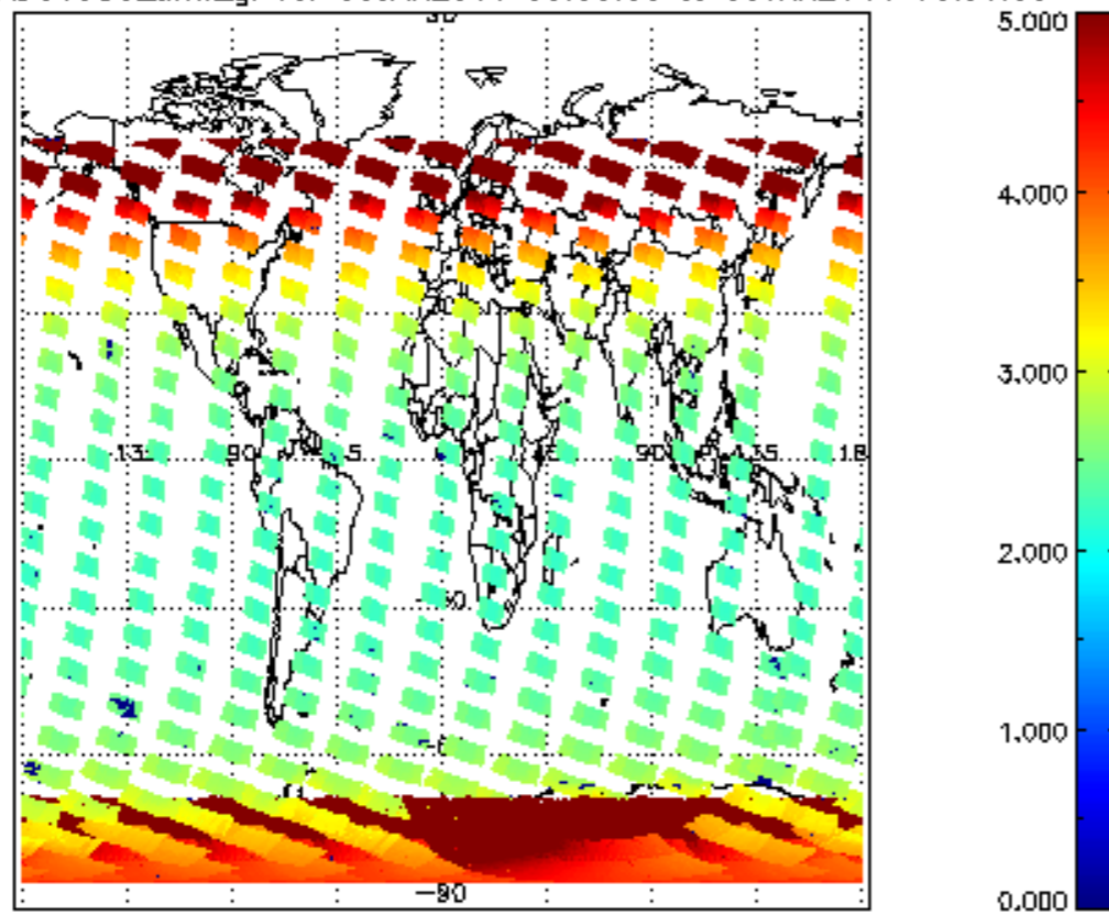
SCIOL2P_NADUV003_amf_gr for 08JAN2011 00:00:00 to 09JAN2011 00:00:00
