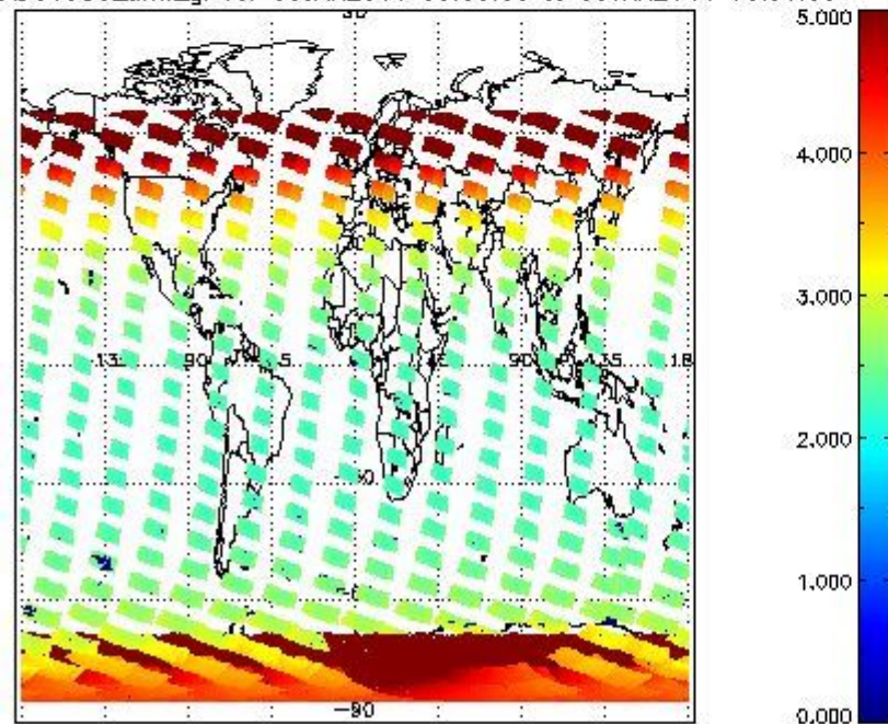
SCIOL2P_NADUV003_amf_gr for 08JAN2011 00:00:00 to 09JAN2011 00:00:00
