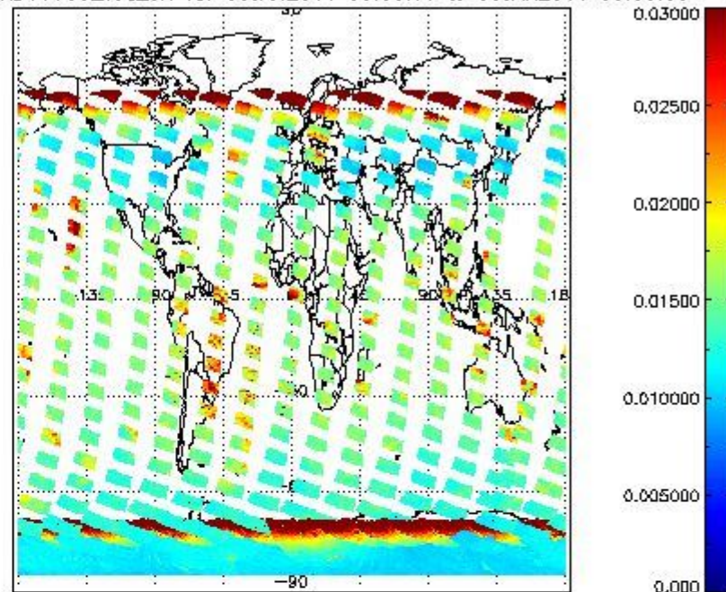
SCIOL2P_NADUV003_vcd_err for 08JAN2011 00:00:00 to 09JAN2011 00:00:00
