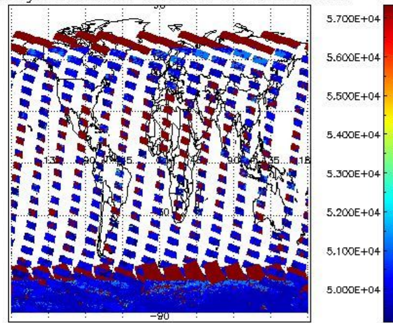
cloud_flags for 08JAN2011 00:00:00 to 09JAN2011 00:00:00
