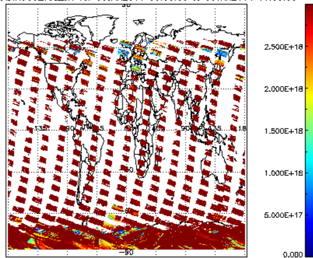
SCIOL2P_NADIR3CO_vcd_err for 08JAN2011 00:00:00 to 09JAN2011 00:00:00
