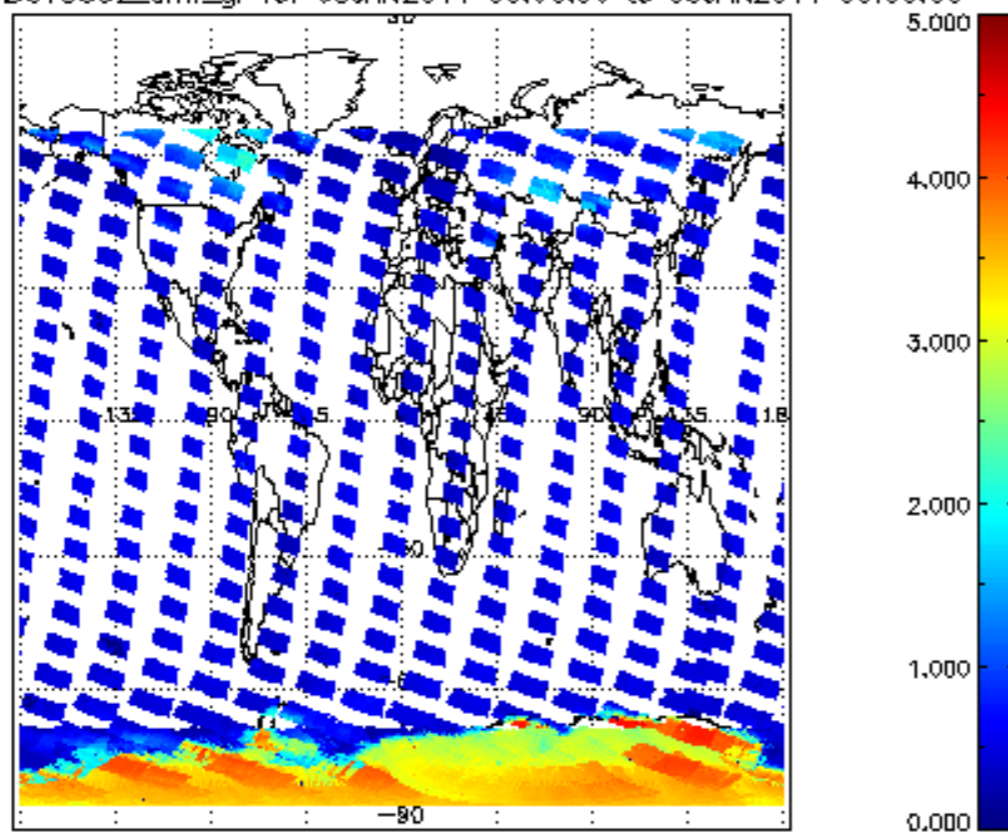
SCIOL2P_NADUV5S02_amf_gr for 08JAN2011 00:00:00 to 09JAN2011 00:00:00
