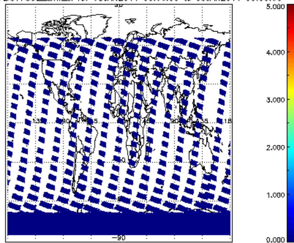
SCIOL2P_NADUV7S02_amf_cl for 08JAN2011 00:00:00 to 09JAN2011 00:00:00
