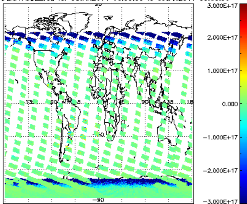
SCIOL2P_NADUV7S02_vcd for 08JAN2011 00:00:00 to 09JAN2011 00:00:00
