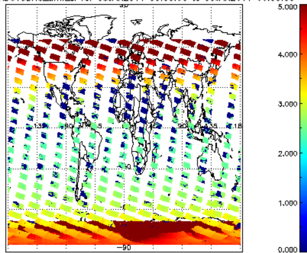
SCIOL2P_NADUV3BRO_amf_cl for 08JAN2011 00:00:00 to 09JAN2011 00:00:00
