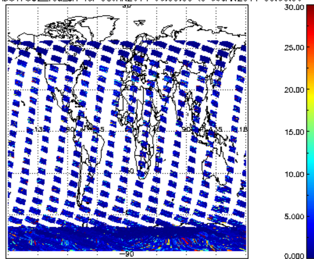
SCIOL2P_NADUV7S02_vcd_err for 08JAN2011 00:00:00 to 09JAN2011 00:00:00
