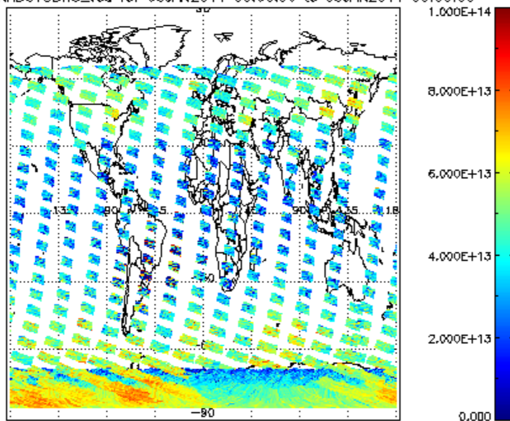
SCIOL2P_NADUV3BRO_vcd for 08JAN2011 00:00:00 to 09JAN2011 00:00:00
