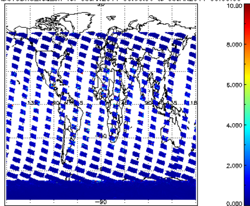
SCIOL2P_NADUV3BRO_vcd_err for 08JAN2011 00:00:00 to 09JAN2011 00:00:00
