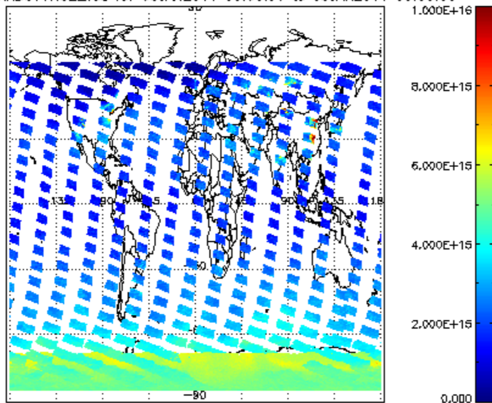
SCIOL2P_NADUV1NO2_vcd for 08JAN2011 00:00:00 to 09JAN2011 00:00:00
