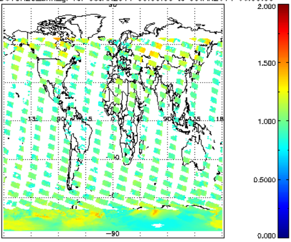
SCIOL2P_NADUV8H20_amf_gr for 08JAN2011 00:00:00 to 09JAN2011 00:00:00
