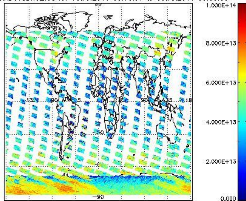
SCIOL2P_NADUV3BRO_vcd for 08JAN2011 00:00:00 to 09JAN2011 00:00:00
