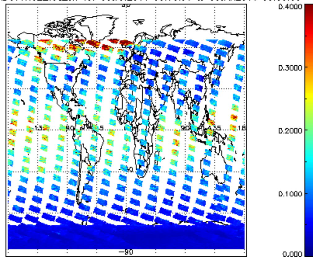
SCIOL2P_NADUV1NO2_vcd_err for 08JAN2011 00:00:00 to 09JAN2011 00:00:00
