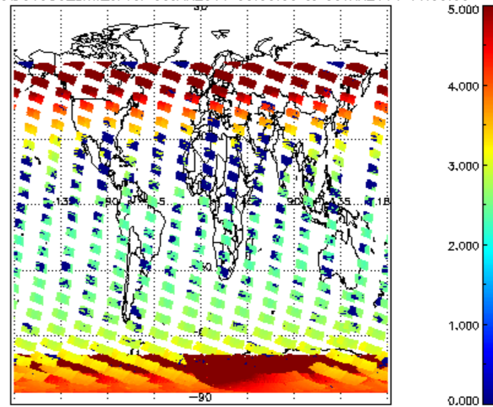
SCIOL2P_NADUV003_amf_cl for 08JAN2011 00:00:00 to 09JAN2011 00:00:00
