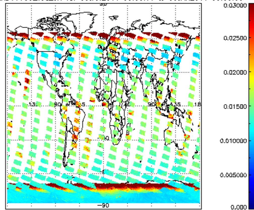
SCIOL2P_NADUV003_vcd_err for 08JAN2011 00:00:00 to 09JAN2011 00:00:00
