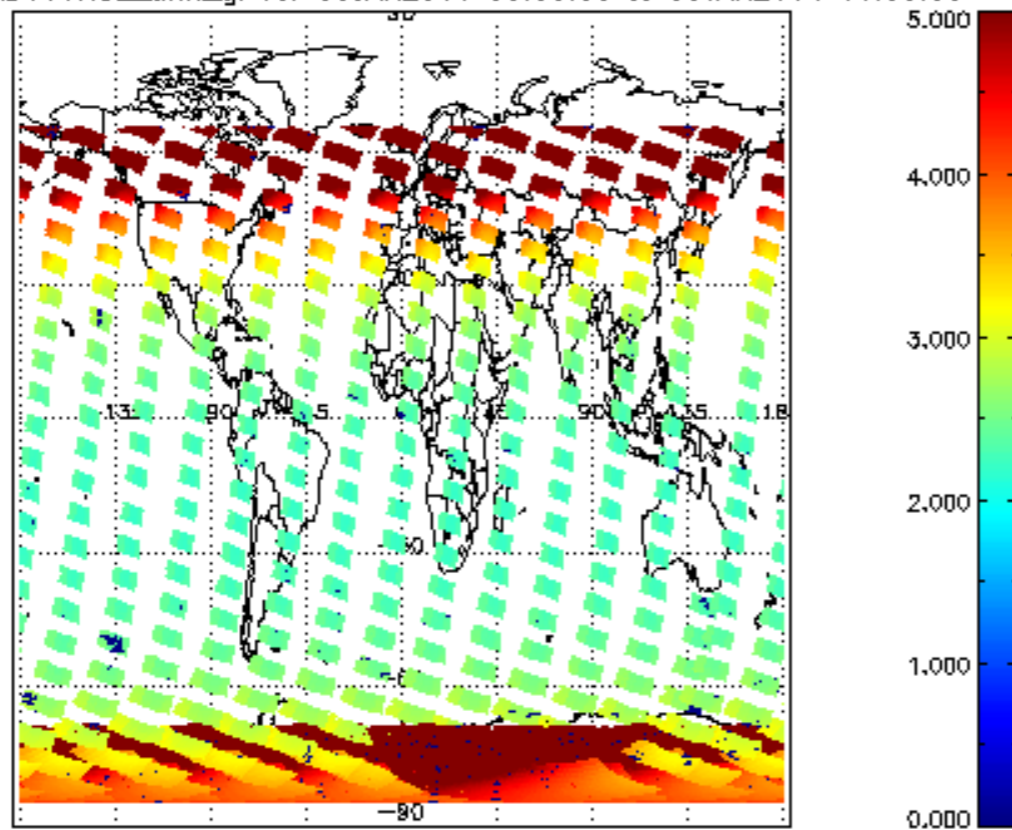
SCIOL2P_NADUV1NO2_amf_gr for 08JAN2011 00:00:00 to 09JAN2011 00:00:00
