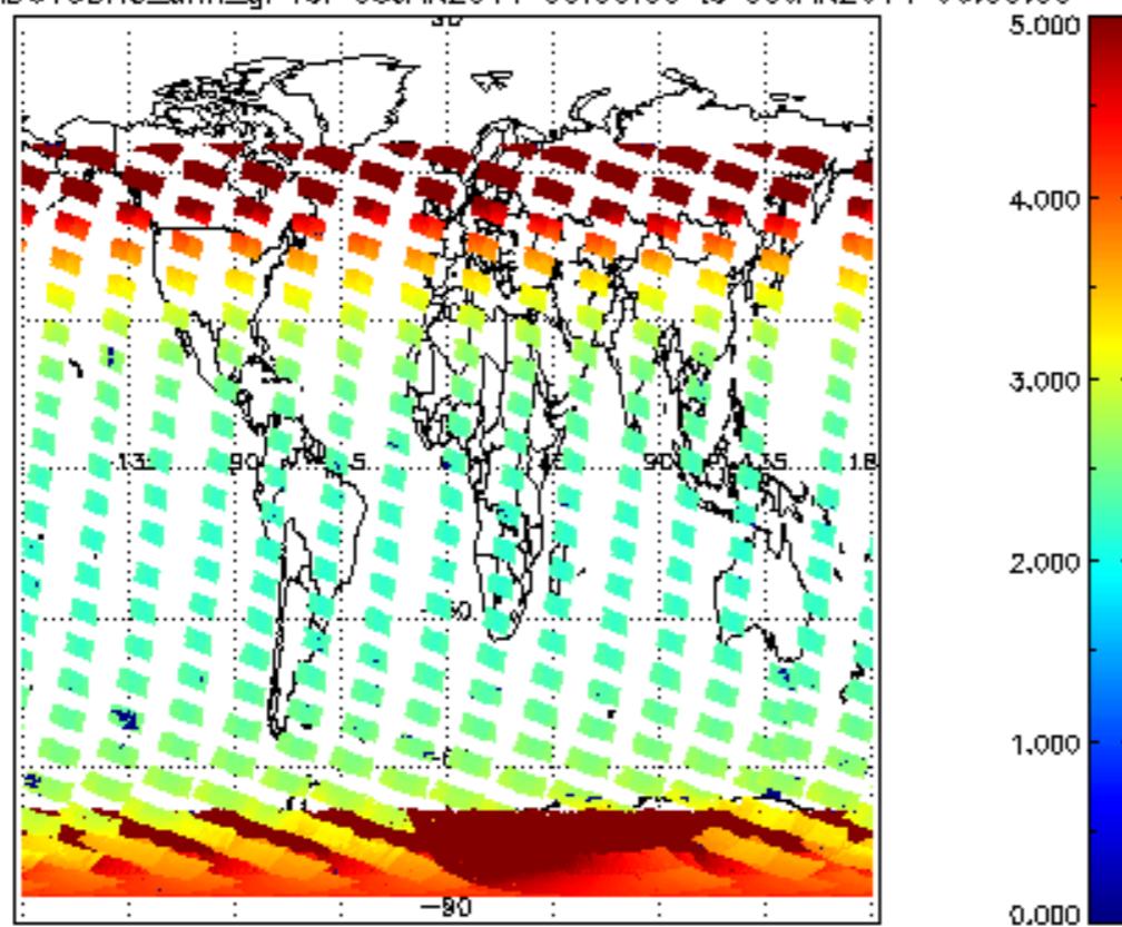
SCIOL2P_NADUV3BRO_amf_gr for 08JAN2011 00:00:00 to 09JAN2011 00:00:00
