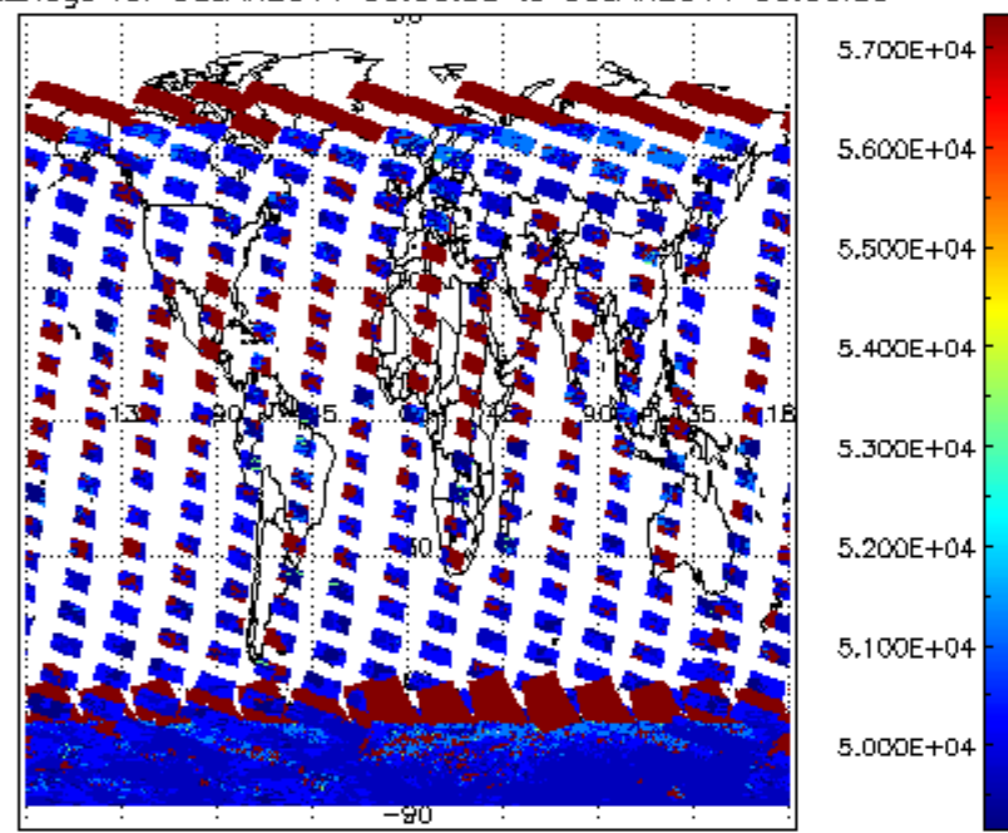
cloud_flags for 08JAN2011 00:00:00 to 09JAN2011 00:00:00
