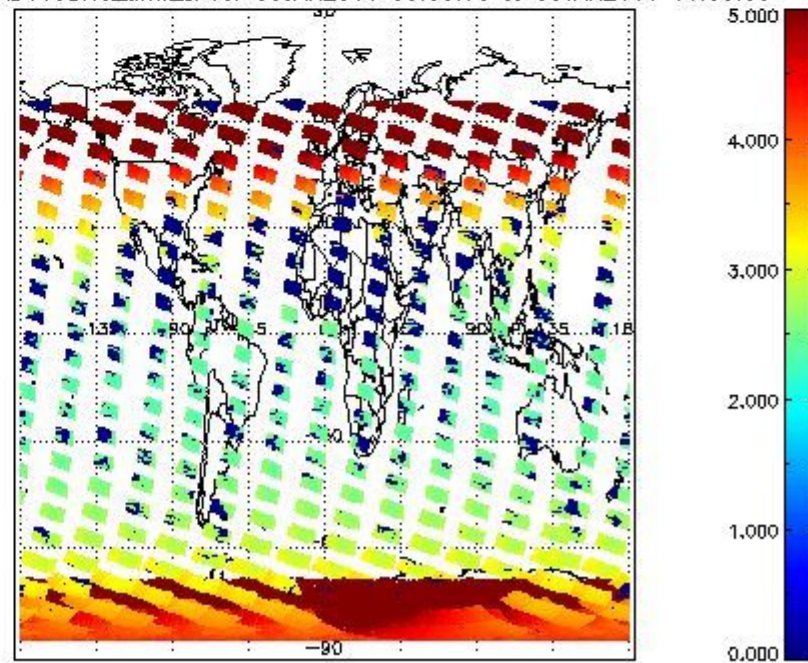
SCIOL2P_NADUV3BRO_amf_cl for 08JAN2011 00:00:00 to 09JAN2011 00:00:00
