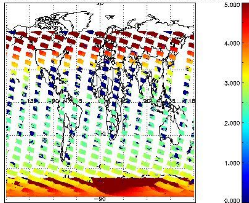
SCIOL2P_NADUV003_amf_cl for 08JAN2011 00:00:00 to 09JAN2011 00:00:00
