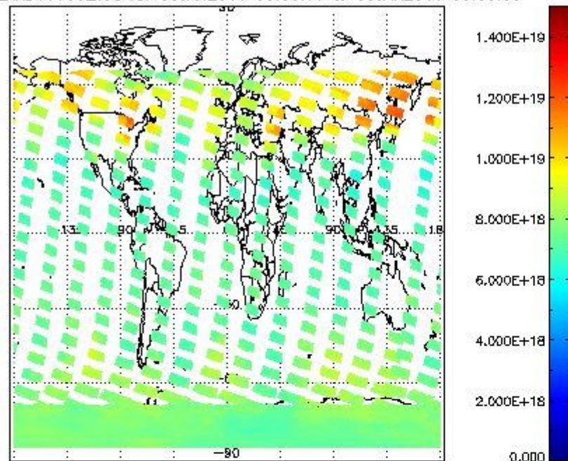
SCIOL2P_NADUV003_vcd for 08JAN2011 00:00:00 to 09JAN2011 00:00:00
