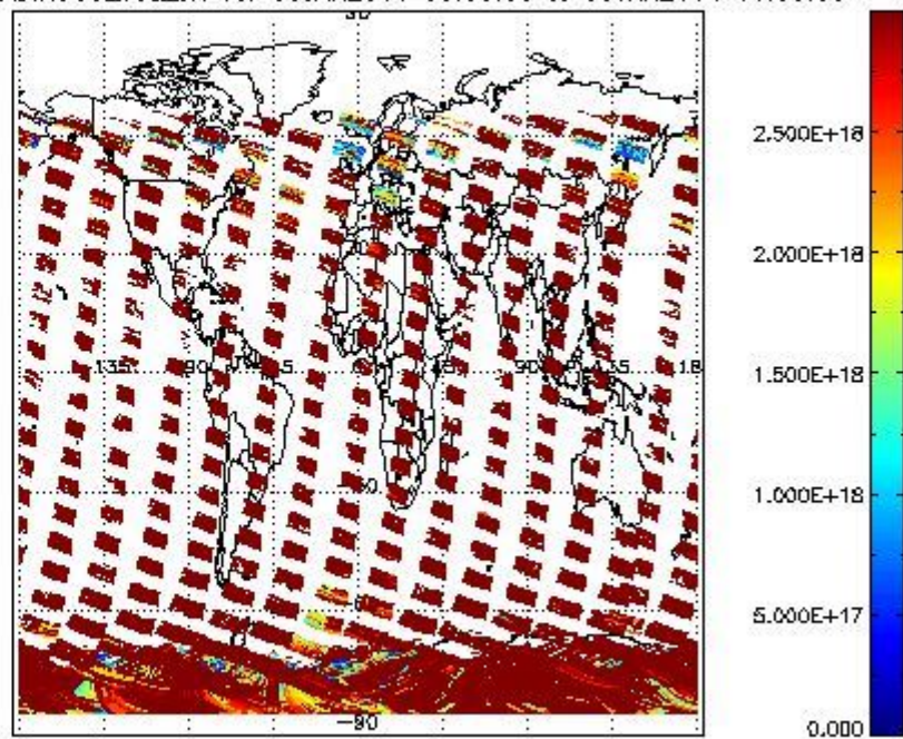
SCIDL2P_NADIR3CO_vcd_err for 08JAN2011 00:00:00 to 09JAN2011 00:00:00
