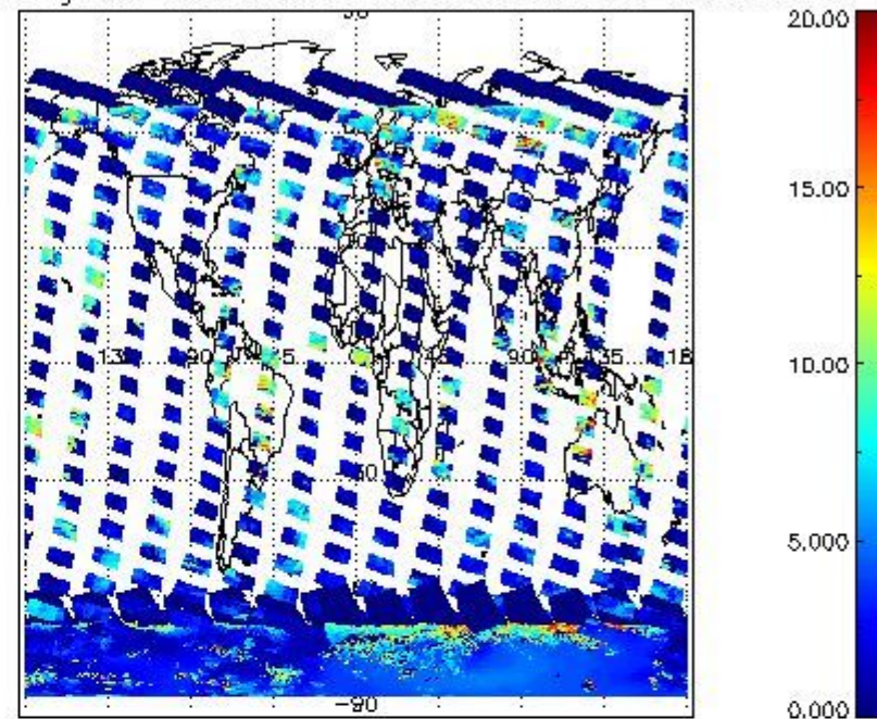
cL_top_height for 08JAN2011 00:00:00 to 09JAN2011 00:00:00
