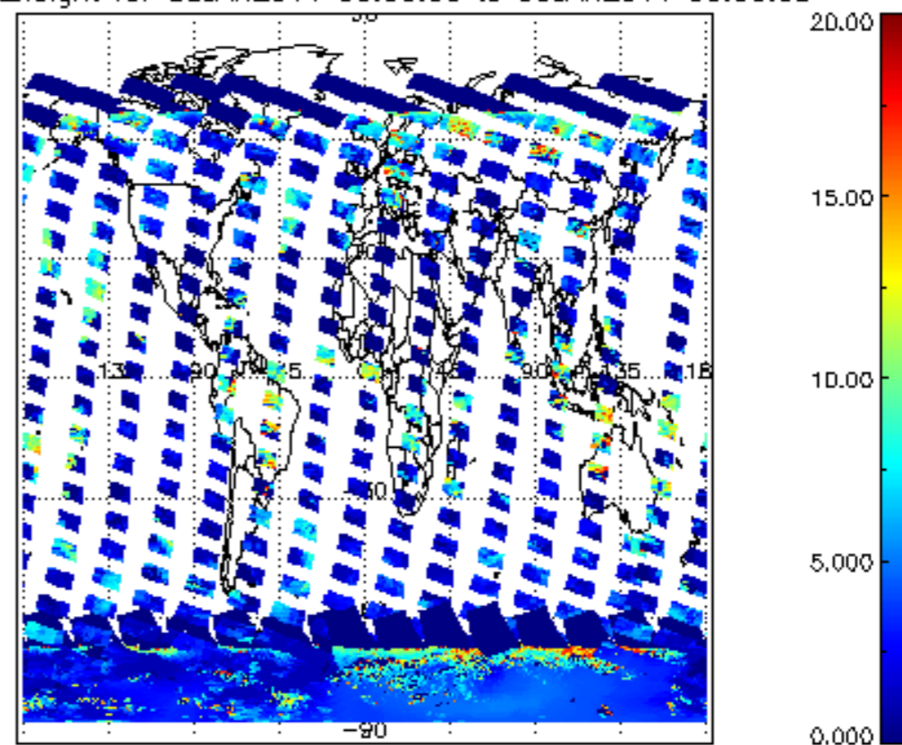
cL_top_height for 08JAN2011 00:00:00 to 09JAN2011 00:00:00
