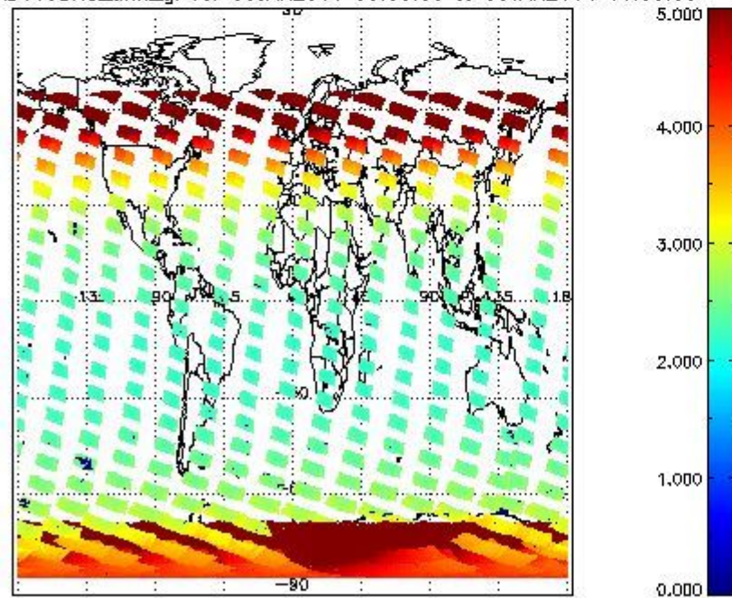
SCIOL2P_NADUV3BRO_amf_gr for 08JAN2011 00:00:00 to 09JAN2011 00:00:00
