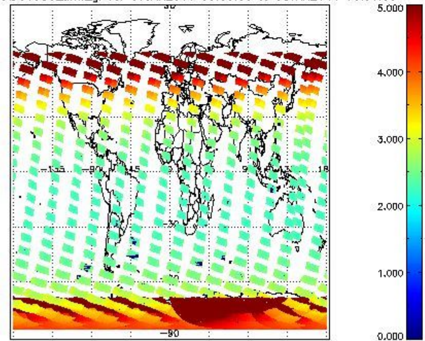
SCIOL2P_NADUV003_amf_gr for 07JAN2011 00:00:00 to 08JAN2011 00:00:00
