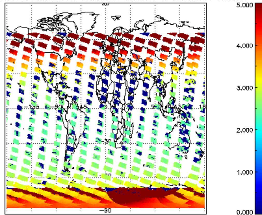
SCIOL2P_NADUV003_amf_cl for 07JAN2011 00:00:00 to 08JAN2011 00:00:00
