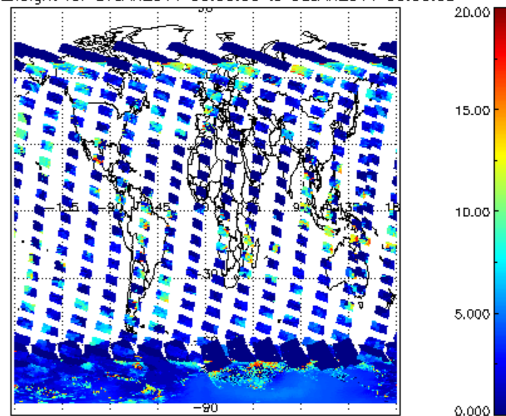
cL_top_height for 07JAN2011 00:00:00 to 08JAN2011 00:00:00
