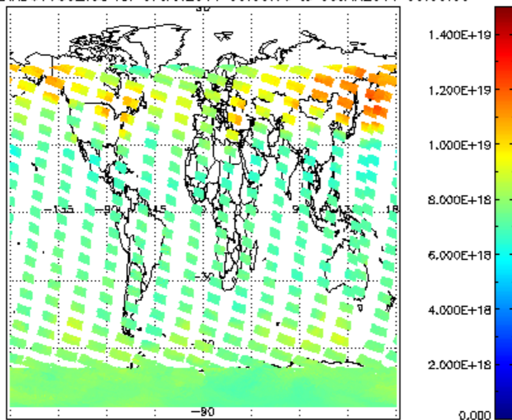
SCIOL2P_NADUV003_vcd for 07JAN2011 00:00:00 to 08JAN2011 00:00:00
