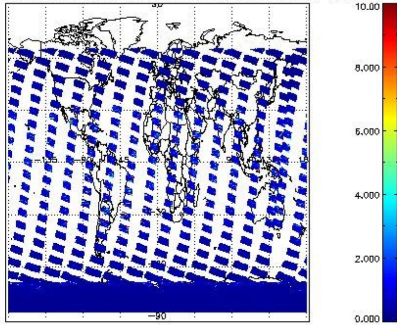
SCIOL2P_NADUV3BRO_vcd_err for 07JAN2011 00:00:00 to 08JAN2011 00:00:00
