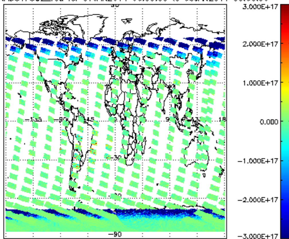
SCIOL2P_NADUV7S02_vcd for 07JAN2011 00:00:00 to 08JAN2011 00:00:00
