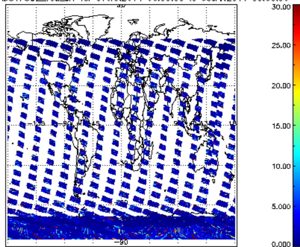
SCIOL2P_NADUV7S02_vcd_err for 07JAN2011 00:00:00 to 08JAN2011 00:00:00
