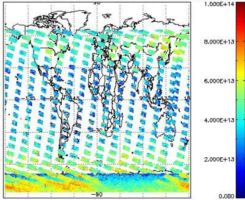
SCIOL2P_NADUV3BRO_vcd for 07JAN2011 00:00:00 to 08JAN2011 00:00:00
