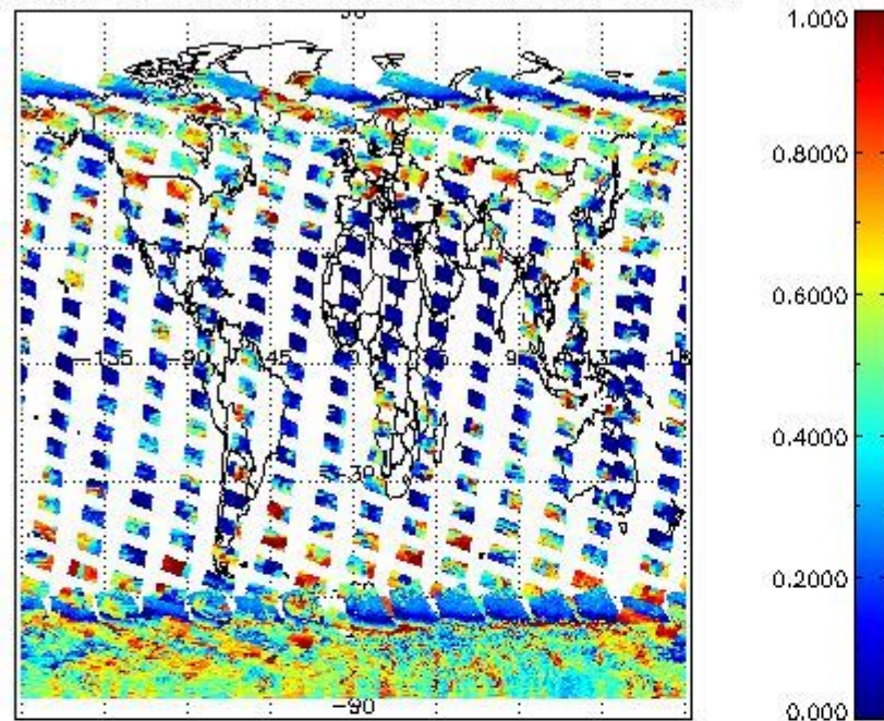
cL_frac for 07JAN2011 00:00:00 to 08JAN2011 00:00:00
