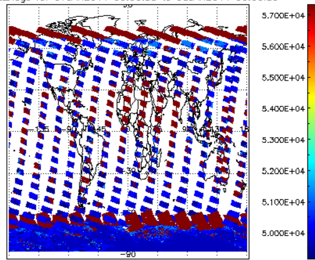
cloud_flags for 07JAN2011 00:00:00 to 08JAN2011 00:00:00
