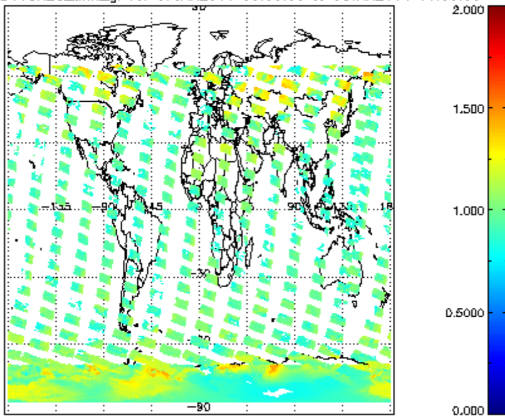
SCIOL2P_NADUV8H20_amf_gr for 07JAN2011 00:00:00 to 08JAN2011 00:00:00
