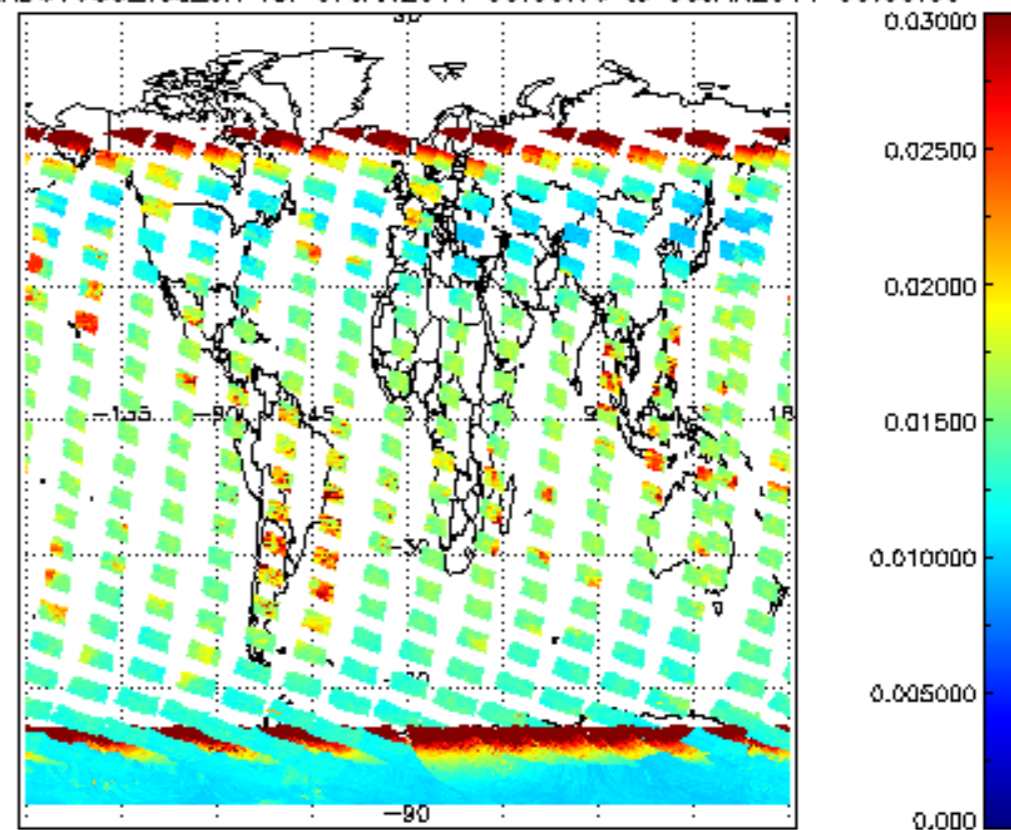
SCIOL2P_NADUV003_vcd_err for 07JAN2011 00:00:00 to 08JAN2011 00:00:00
