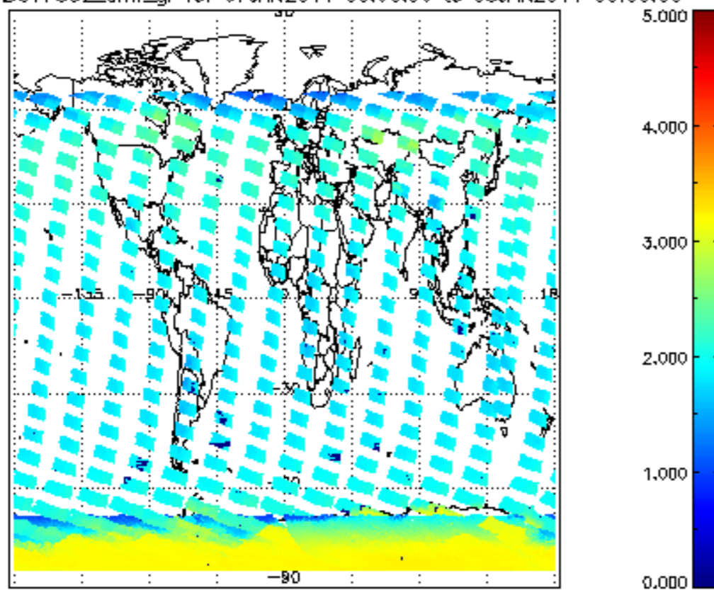
SCIOL2P_NADUV7S02_amf_gr for 07JAN2011 00:00:00 to 08JAN2011 00:00:00
