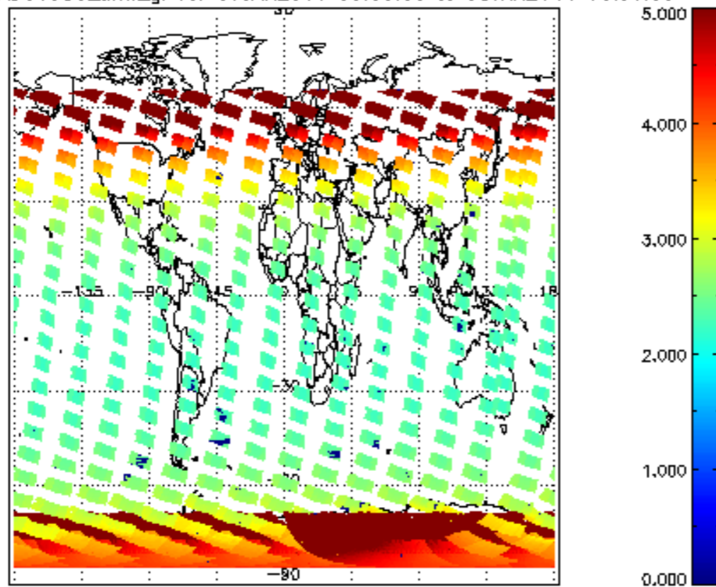
SCIOL2P_NADUV003_amf_gr for 07JAN2011 00:00:00 to 08JAN2011 00:00:00
