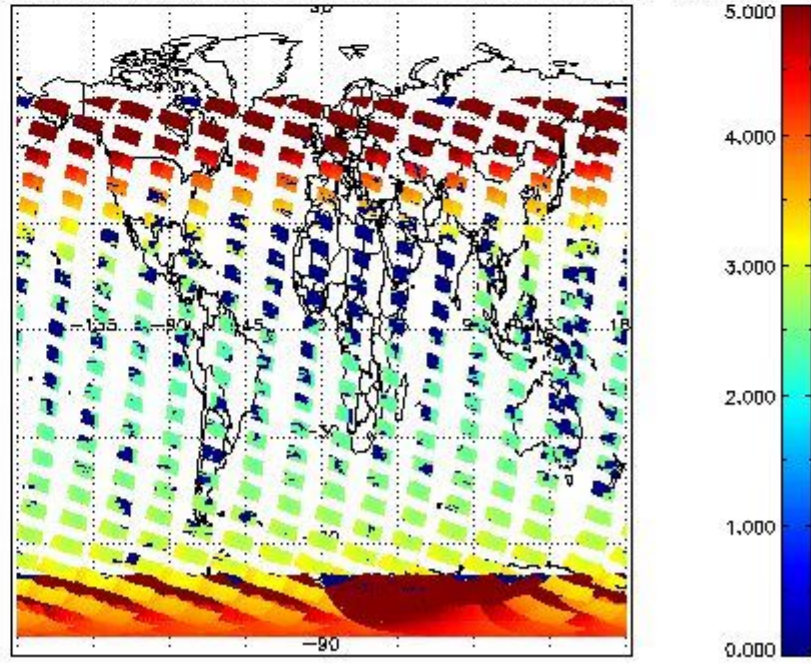
SCIOL2P_NADUV3BRO_amf_cl for 07JAN2011 00:00:00 to 08JAN2011 00:00:00
