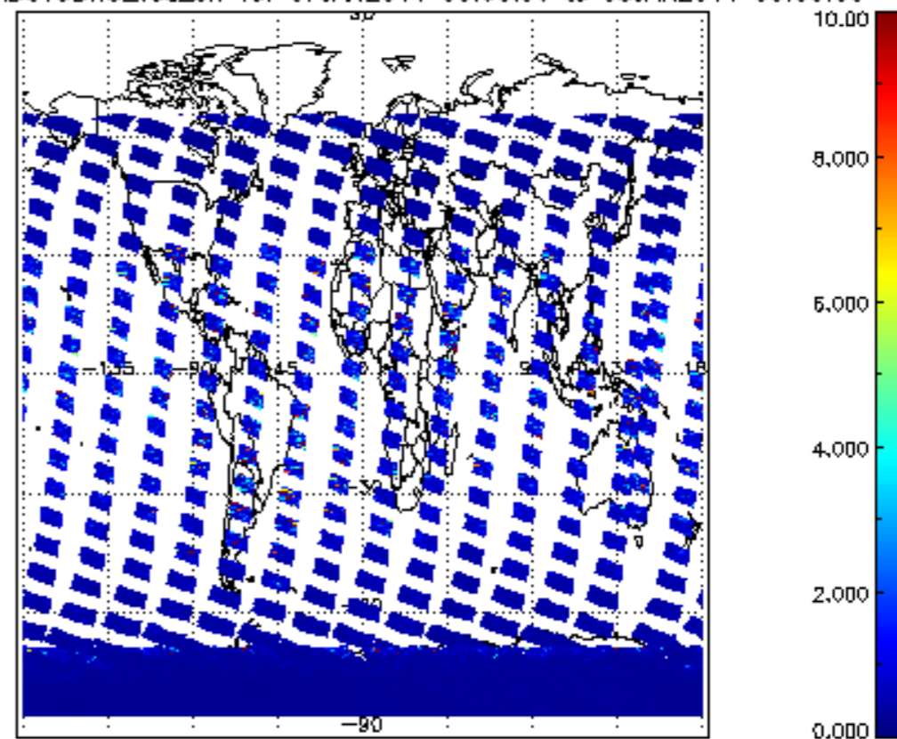
SCIOL2P_NADUV3BRO_vcd_err for 07JAN2011 00:00:00 to 08JAN2011 00:00:00
