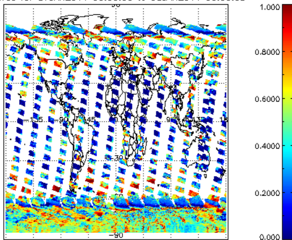
cL_frac for 07JAN2011 00:00:00 to 08JAN2011 00:00:00
