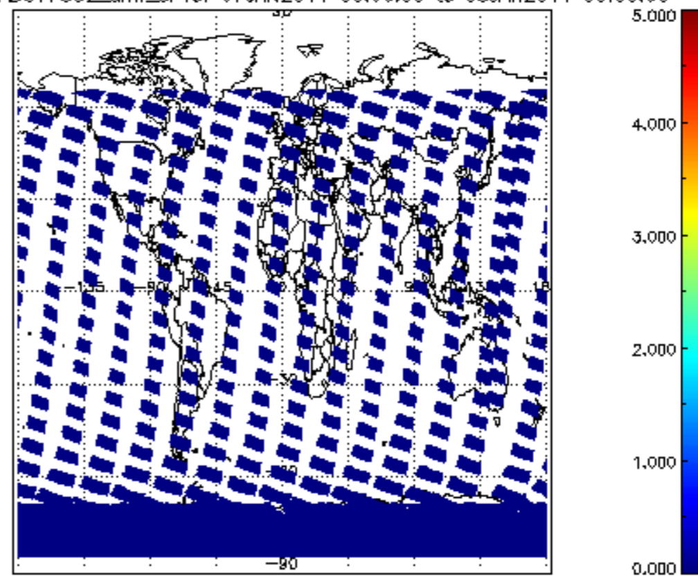
SCIOL2P_NADUV7S02_amf_cl for 07JAN2011 00:00:00 to 08JAN2011 00:00:00
