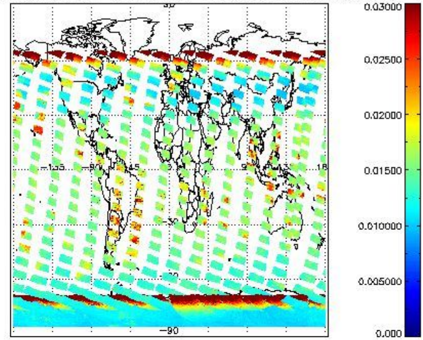
SCIOL2P_NADUV003_vcd_err for 07JAN2011 00:00:00 to 08JAN2011 00:00:00
