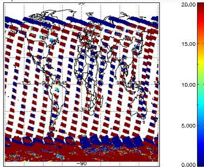
cLopt_depth for 07JAN2011 00:00:00 to 08JAN2011 00:00:00
