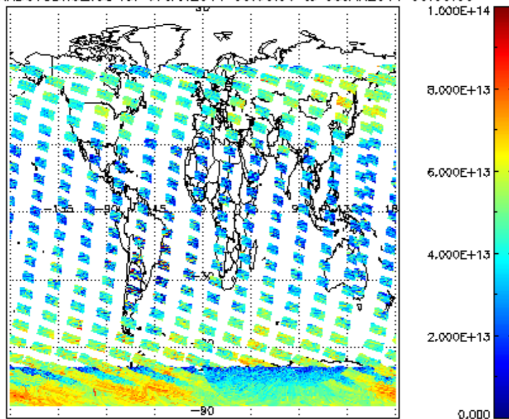
SCIOL2P_NADUV3BRO_vcd for 07JAN2011 00:00:00 to 08JAN2011 00:00:00
