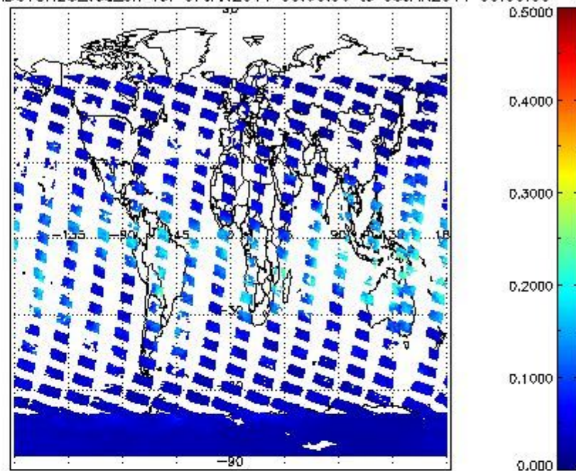
SCIOL2P_NADUV8H20_vcd_err for 07JAN2011 00:00:00 to 08JAN2011 00:00:00
