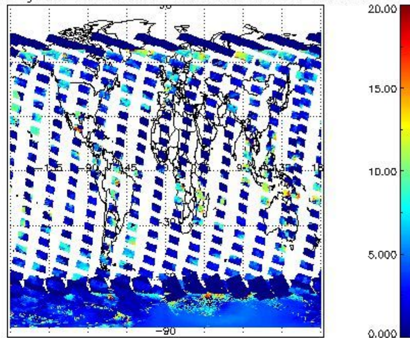
cL_top_height for 07JAN2011 00:00:00 to 08JAN2011 00:00:00
