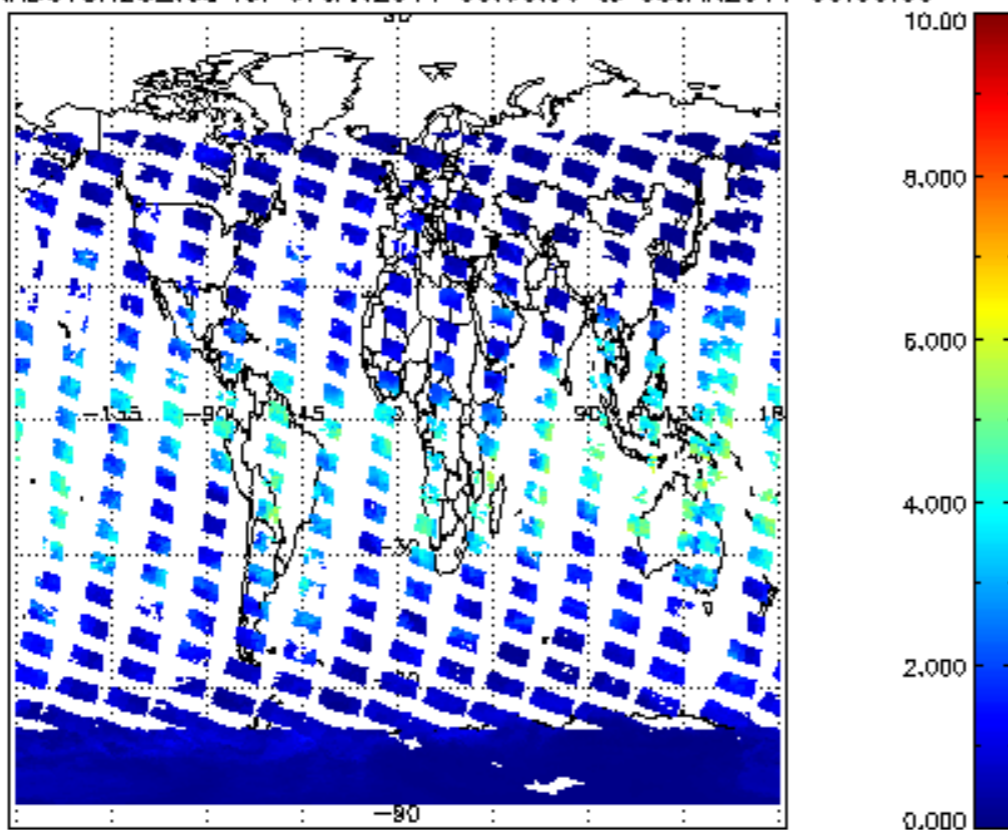
SCIOL2P_NADUV8H20_vcd for 07JAN2011 00:00:00 to 08JAN2011 00:00:00
