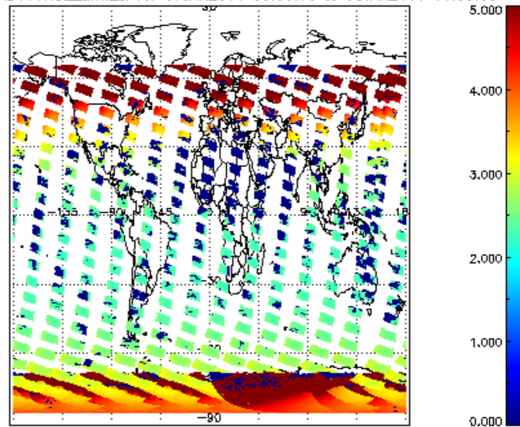
SCIOL2P_NADUV1NO2_amf_cl for 07JAN2011 00:00:00 to 08JAN2011 00:00:00
