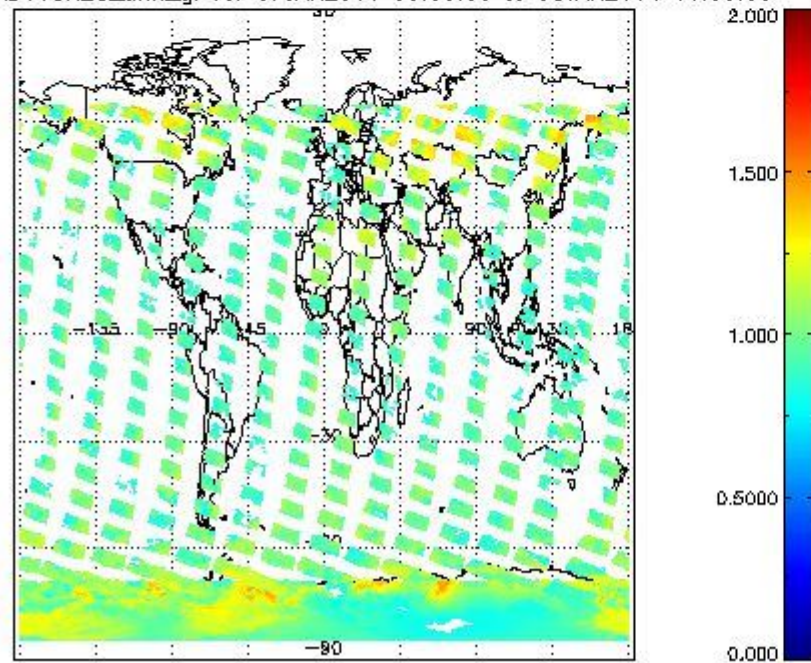
SCIOL2P_NADUV8H20_amf_gr for 07JAN2011 00:00:00 to 08JAN2011 00:00:00
