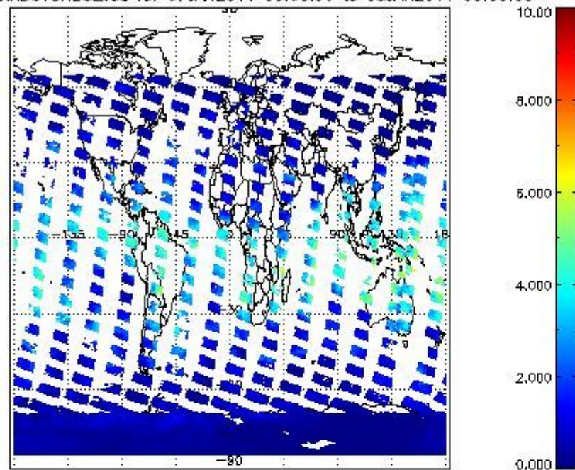
SCIOL2P_NADUV8H20_vcd for 07JAN2011 00:00:00 to 08JAN2011 00:00:00
