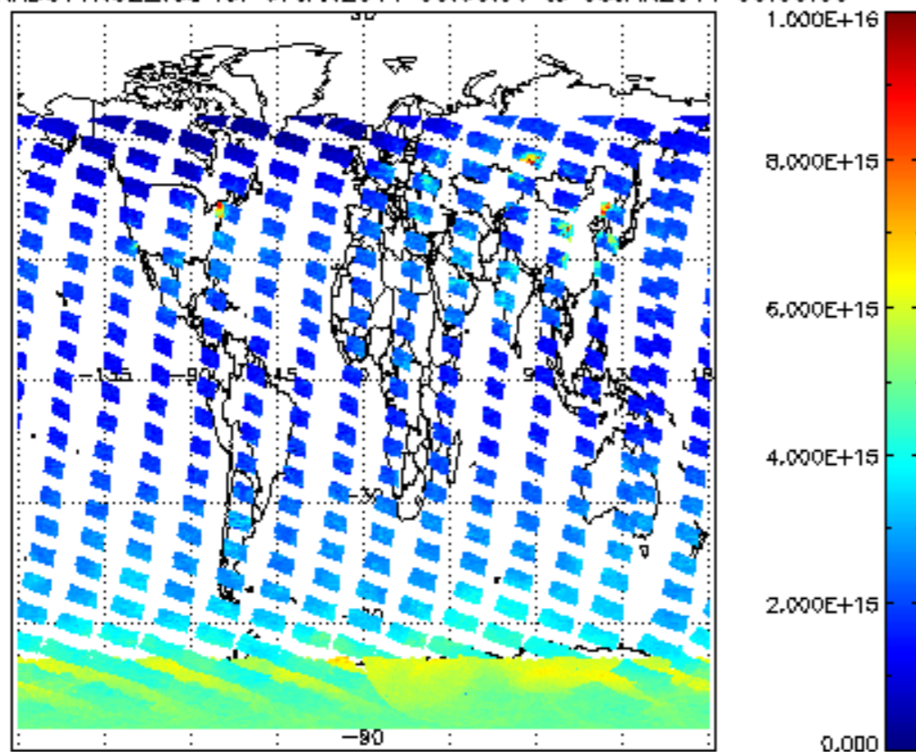
SCIOL2P_NADUV1NO2_vcd for 07JAN2011 00:00:00 to 08JAN2011 00:00:00
