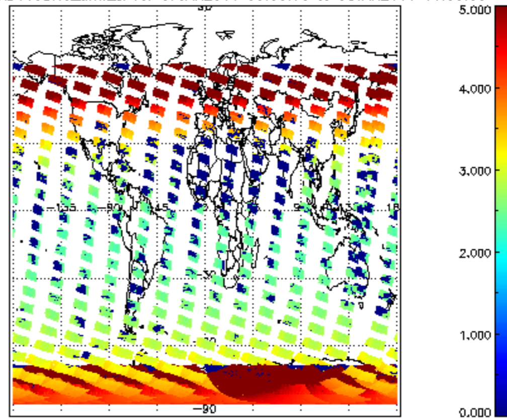
SCIOL2P_NADUV3BRO_amf_cl for 07JAN2011 00:00:00 to 08JAN2011 00:00:00
