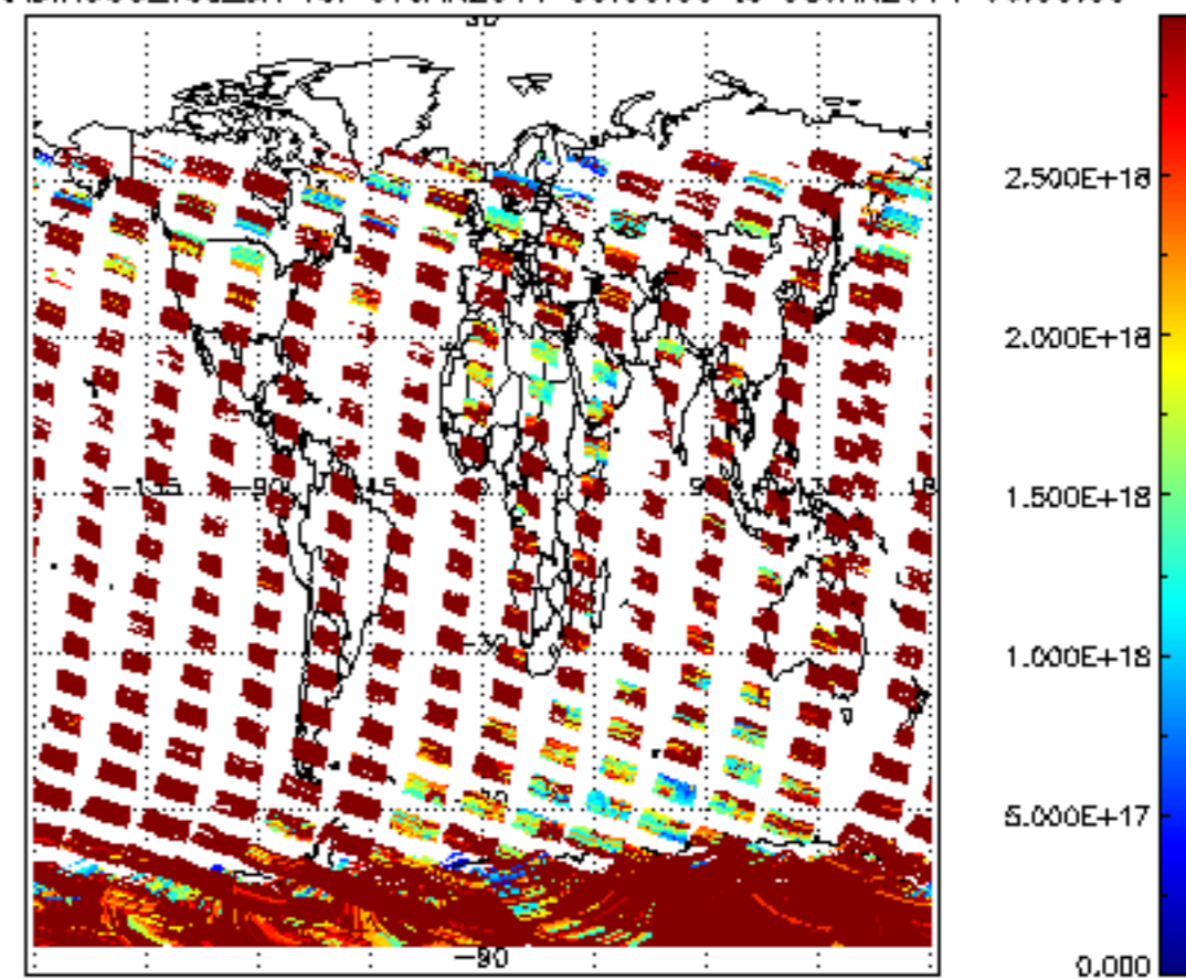
SCIOL2P_NADIR3CO_vcd_err for 07JAN2011 00:00:00 to 08JAN2011 00:00:00
