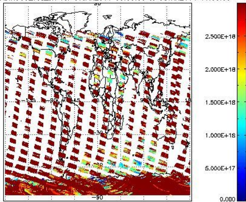
SCIDL2P_NADIR3CO_vcd_err for 07JAN2011 00:00:00 to 08JAN2011 00:00:00
