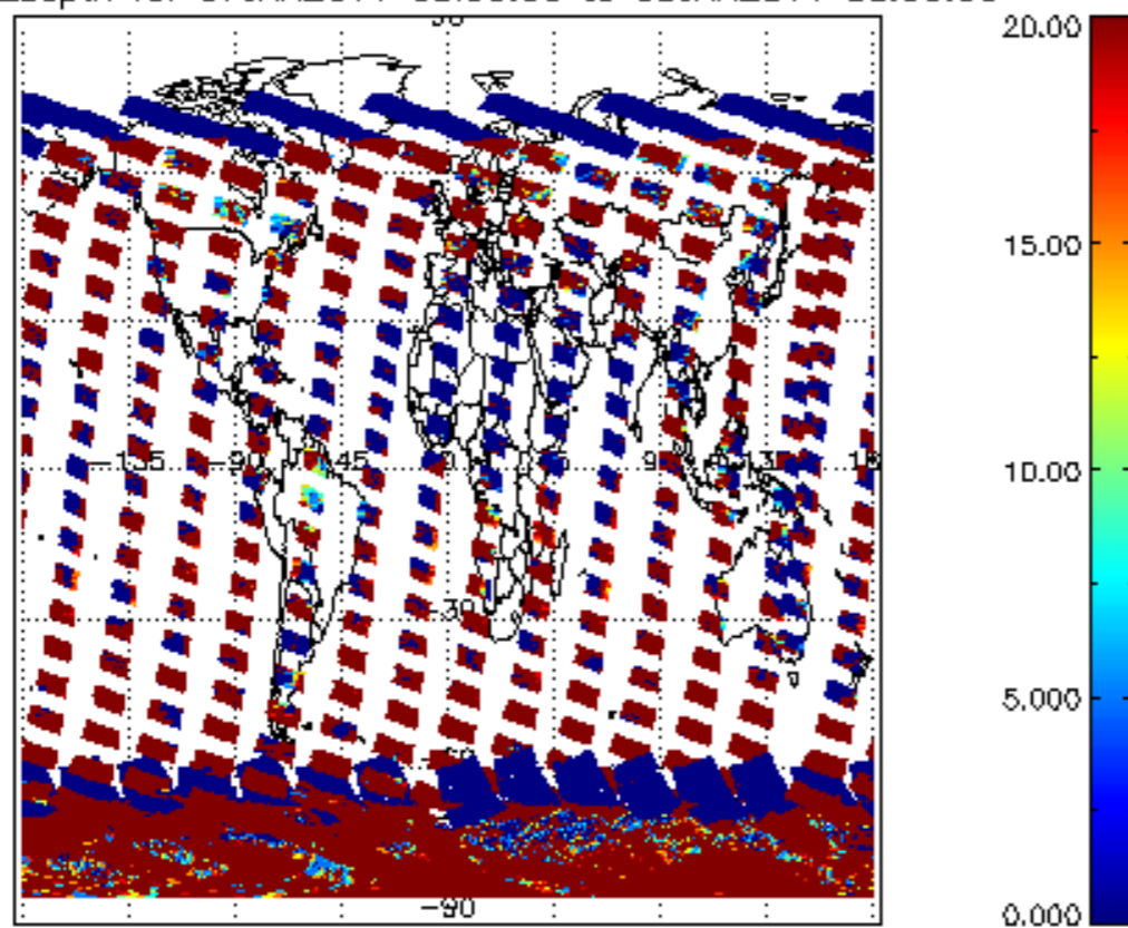
cLopt_depth for 07JAN2011 00:00:00 to 08JAN2011 00:00:00
