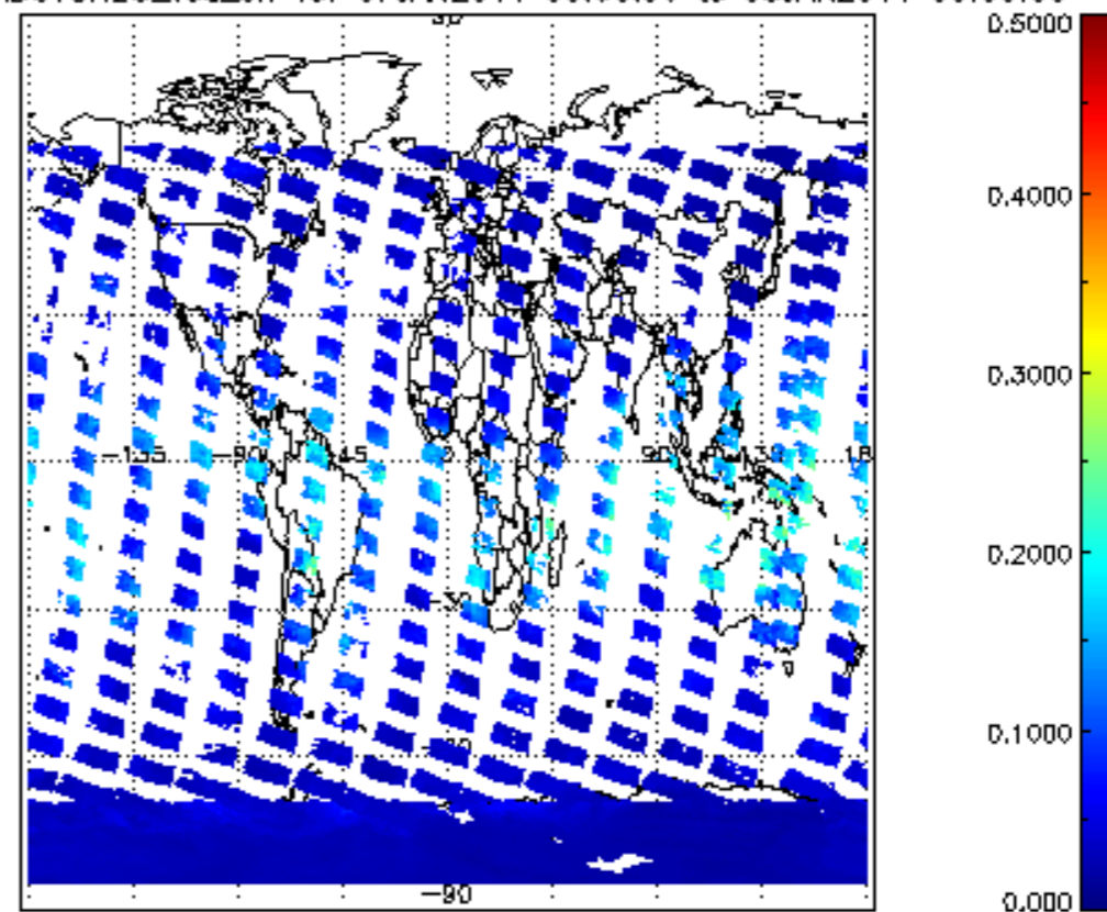
SCIOL2P_NADUV8H20_vcd_err for 07JAN2011 00:00:00 to 08JAN2011 00:00:00
