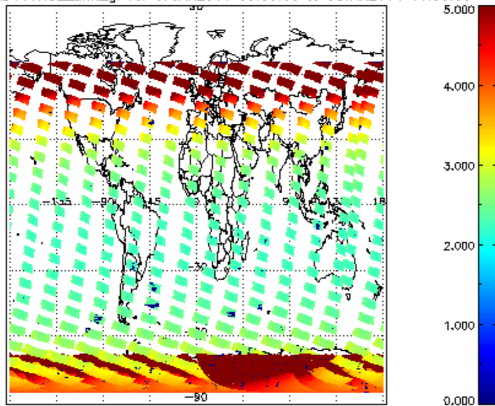
SCIOL2P_NADUV1NO2_amf_gr for 07JAN2011 00:00:00 to 08JAN2011 00:00:00
