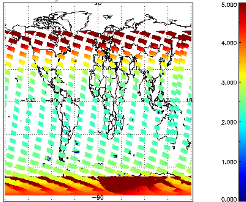
SCIOL2P_NADUV3BRO_amf_gr for 07JAN2011 00:00:00 to 08JAN2011 00:00:00
