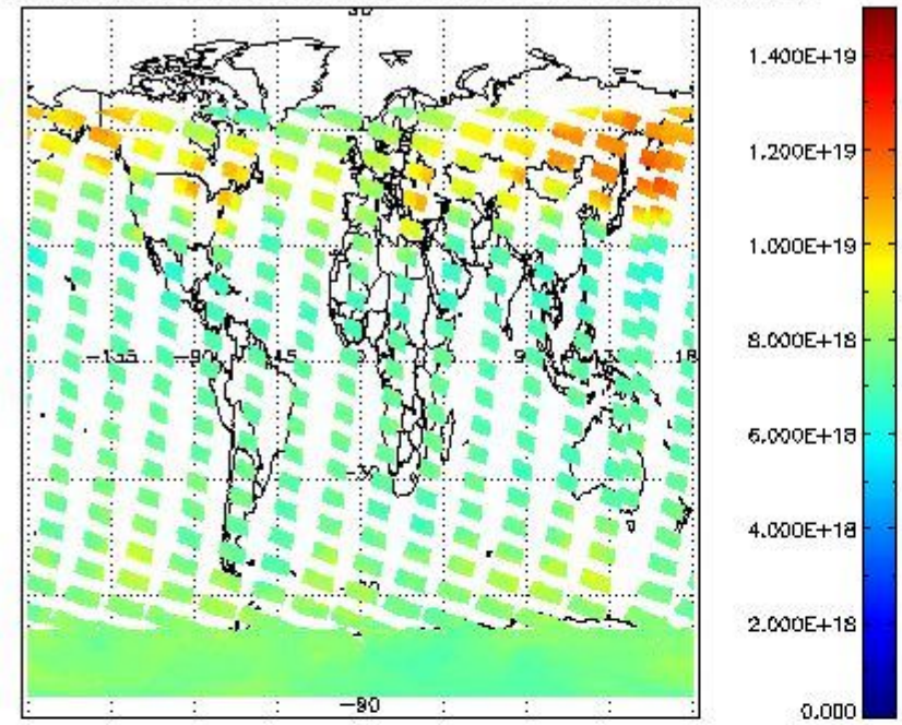
SCIOL2P_NADUV003_vcd for 07JAN2011 00:00:00 to 08JAN2011 00:00:00
