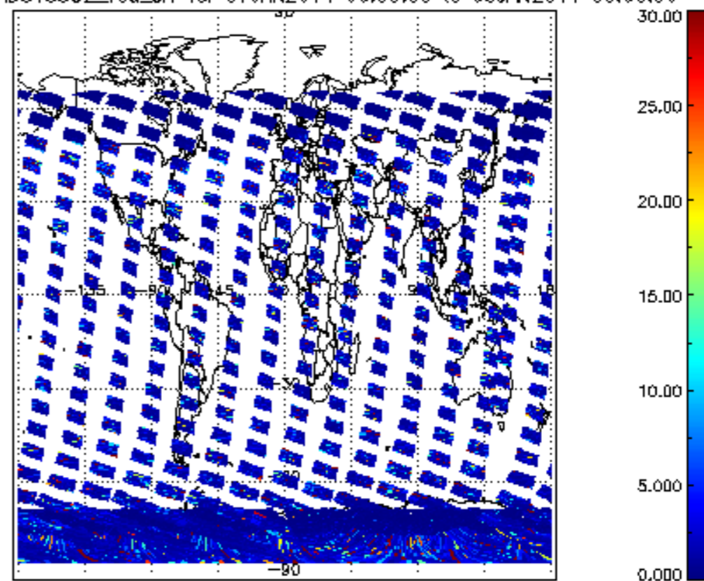
SCIOL2P_NADUV5S02_vcd_err for 07JAN2011 00:00:00 to 08JAN2011 00:00:00
