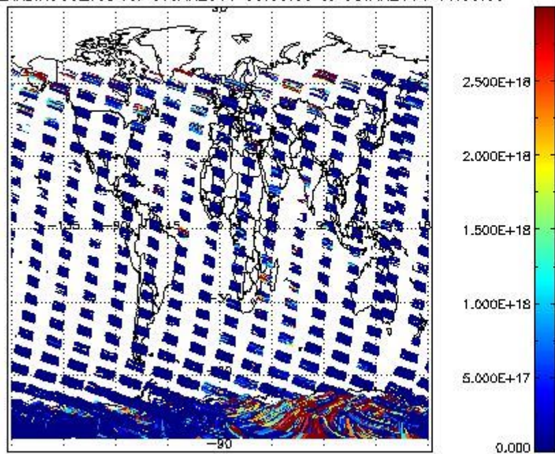
SCIDL2P_NADIR3CO_vcd for 07JAN2011 00:00:00 to 08JAN2011 00:00:00
