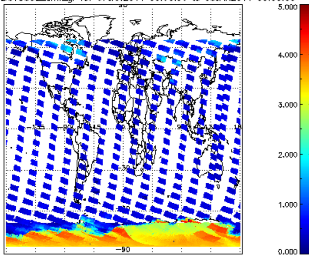
SCIOL2P_NADUV5S02_amf_gr for 07JAN2011 00:00:00 to 08JAN2011 00:00:00
