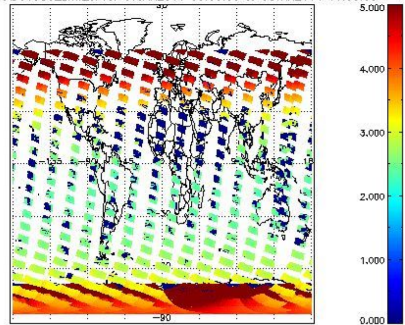
SCIOL2P_NADUV003_amf_cl for 07JAN2011 00:00:00 to 08JAN2011 00:00:00
