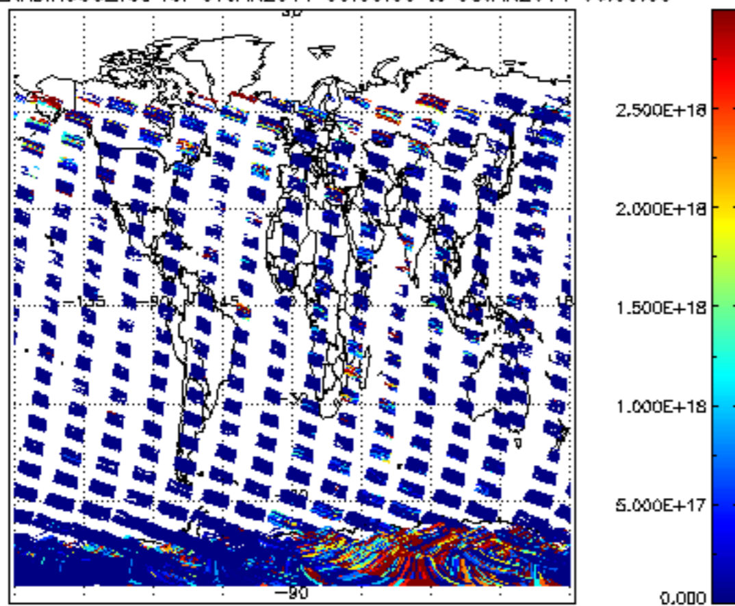
SCIOL2P_NADIR3CO_vcd for 07JAN2011 00:00:00 to 08JAN2011 00:00:00
