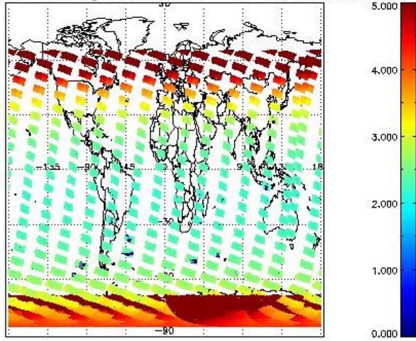
SCIOL2P_NADUV3BRO_amf_gr for 07JAN2011 00:00:00 to 08JAN2011 00:00:00
