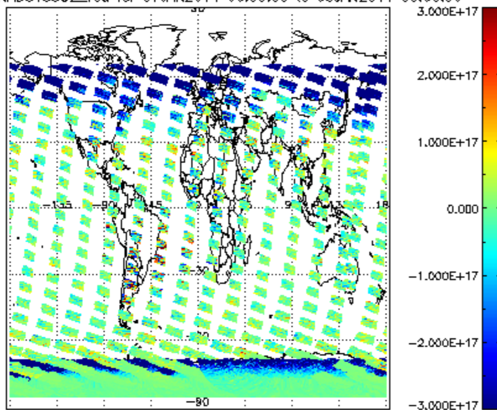
SCIOL2P_NADUV5S02_vcd for 07JAN2011 00:00:00 to 08JAN2011 00:00:00
