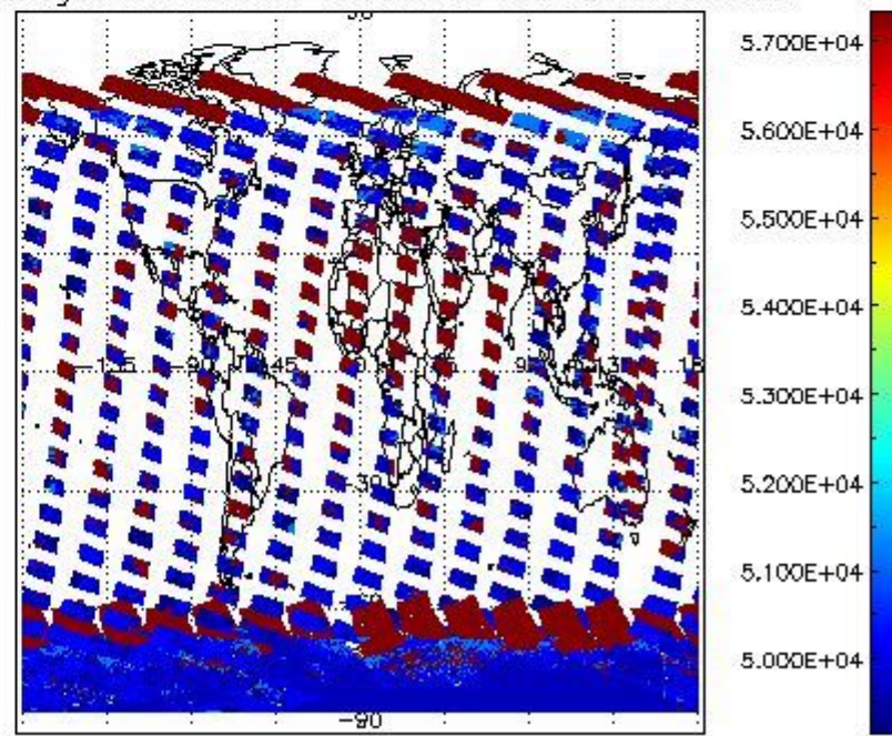
cloud_flags for 07JAN2011 00:00:00 to 08JAN2011 00:00:00
