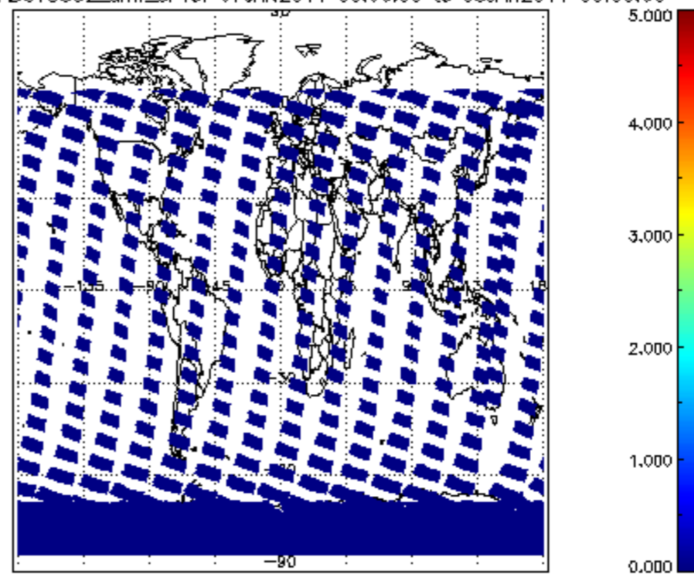
SCIOL2P_NADUV5S02_amf_cl for 07JAN2011 00:00:00 to 08JAN2011 00:00:00
