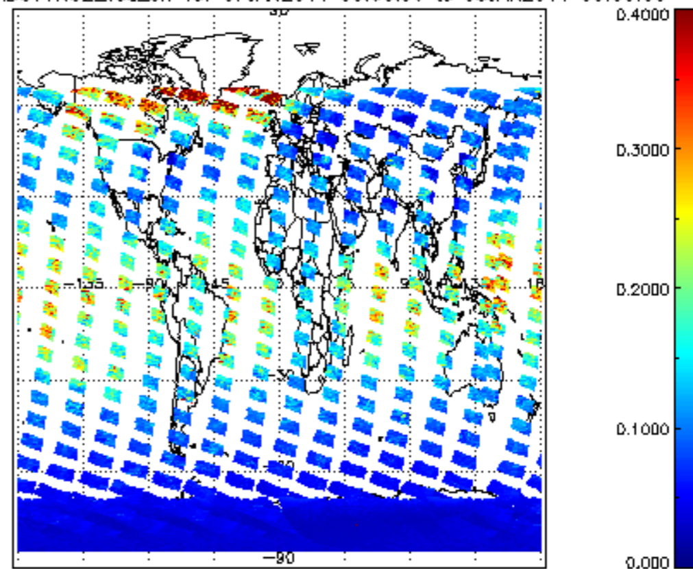
SCIOL2P_NADUV1NO2_vcd_err for 07JAN2011 00:00:00 to 08JAN2011 00:00:00
