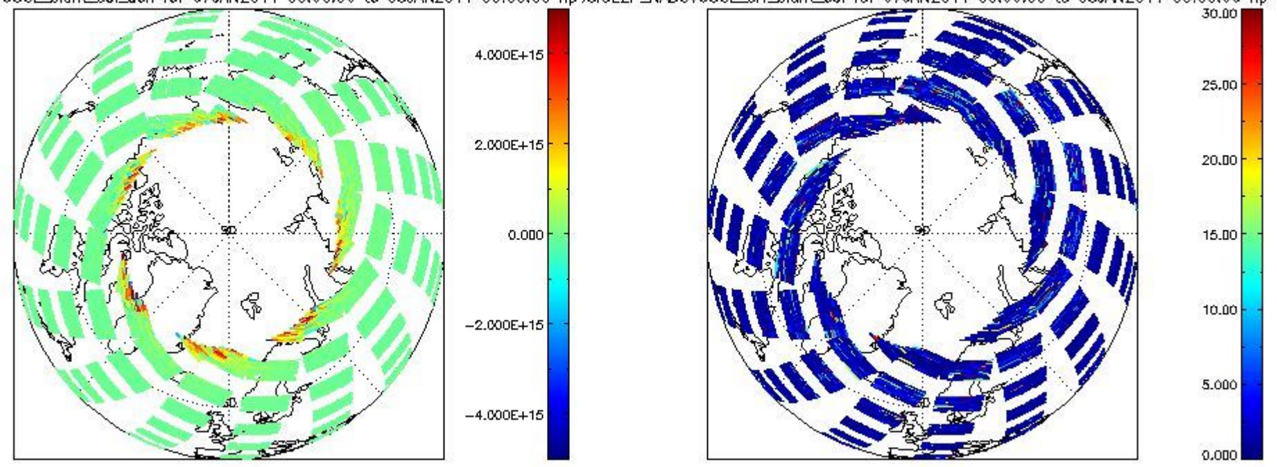
SCIOI2P_NADUV60CL_slant_col_den for 07JAN2011 00:00:00 to 08JAN2011 00:00:00 np:SCIOI2P_NADUV60CL_err_slant_col for 07JAN2011 00:00:00 to 08JAN2011 00:00:00 np
