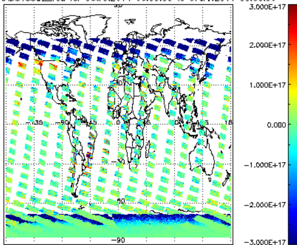
SCIOL2P_NADUV5S02_vcd for 06JAN2011 00:00:00 to 07JAN2011 00:00:00
