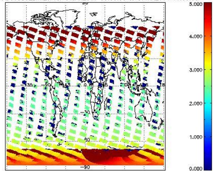
SCIOL2P_NADUV003_amf_cl for 06JAN2011 00:00:00 to 07JAN2011 00:00:00
