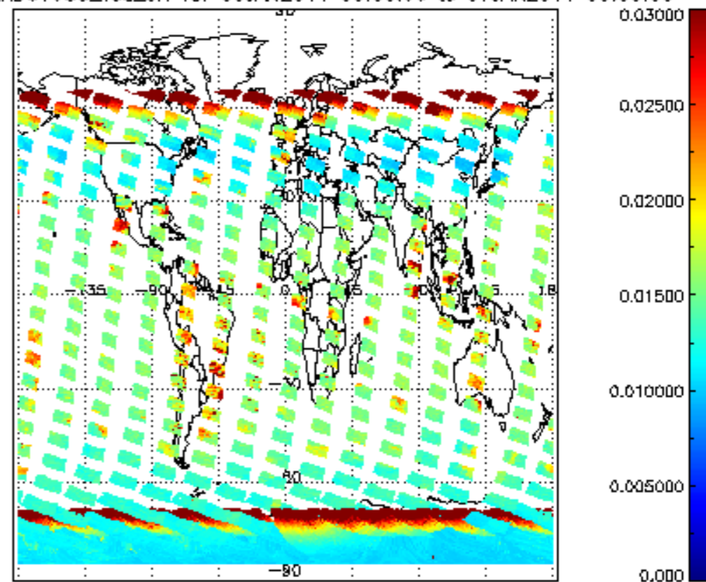
SCIOL2P_NADUV003_vcd_err for 06JAN2011 00:00:00 to 07JAN2011 00:00:00
