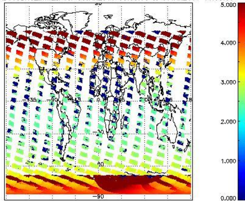
SCIOL2P_NADUV3BRO_amf_cl for 06JAN2011 00:00:00 to 07JAN2011 00:00:00
