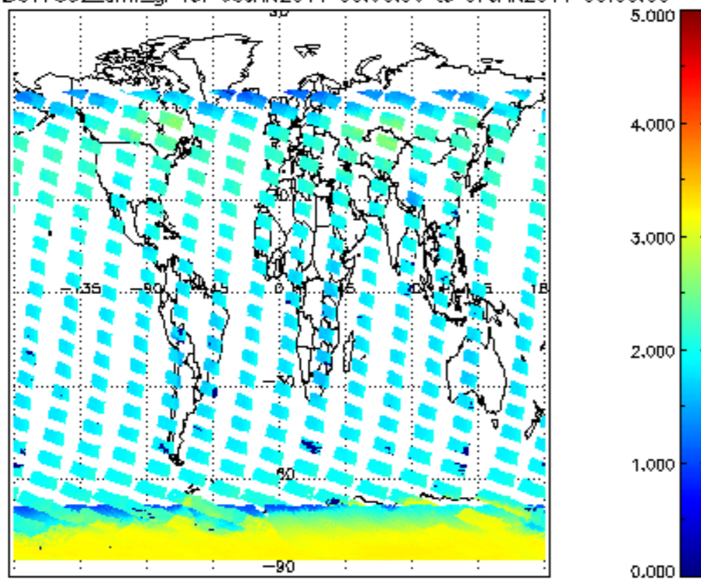
SCIOL2P_NADUV7S02_amf_gr for 06JAN2011 00:00:00 to 07JAN2011 00:00:00
