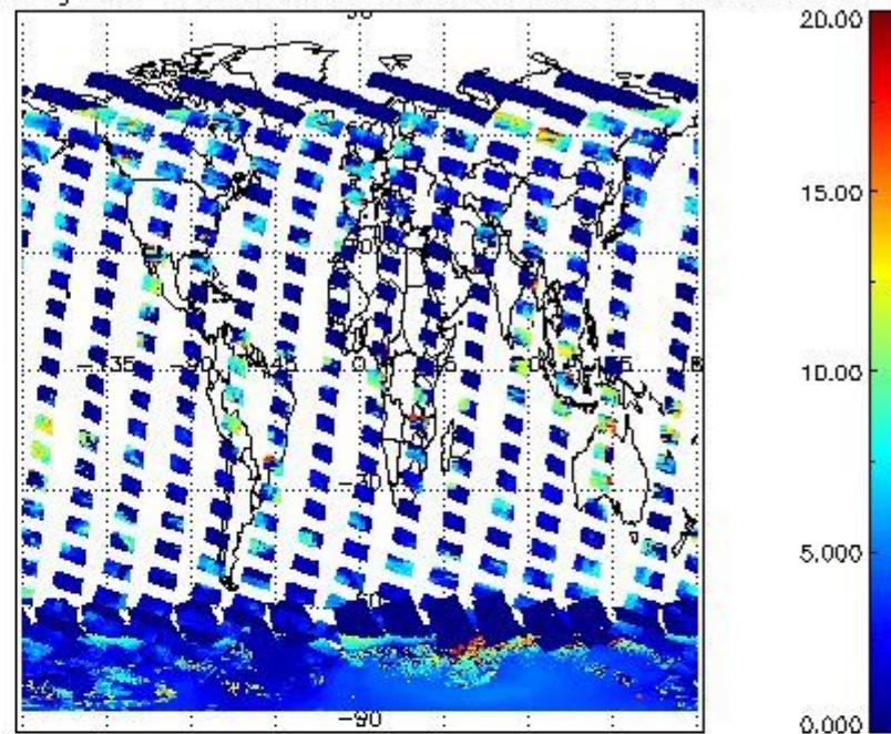
cL_top_height for 06JAN2011 00:00:00 to 07JAN2011 00:00:00
