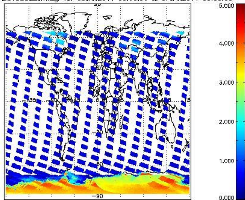
SCIOL2P_NADUV5SO2_amf_gr for 06JAN2011 00:00:00 to 07JAN2011 00:00:00
