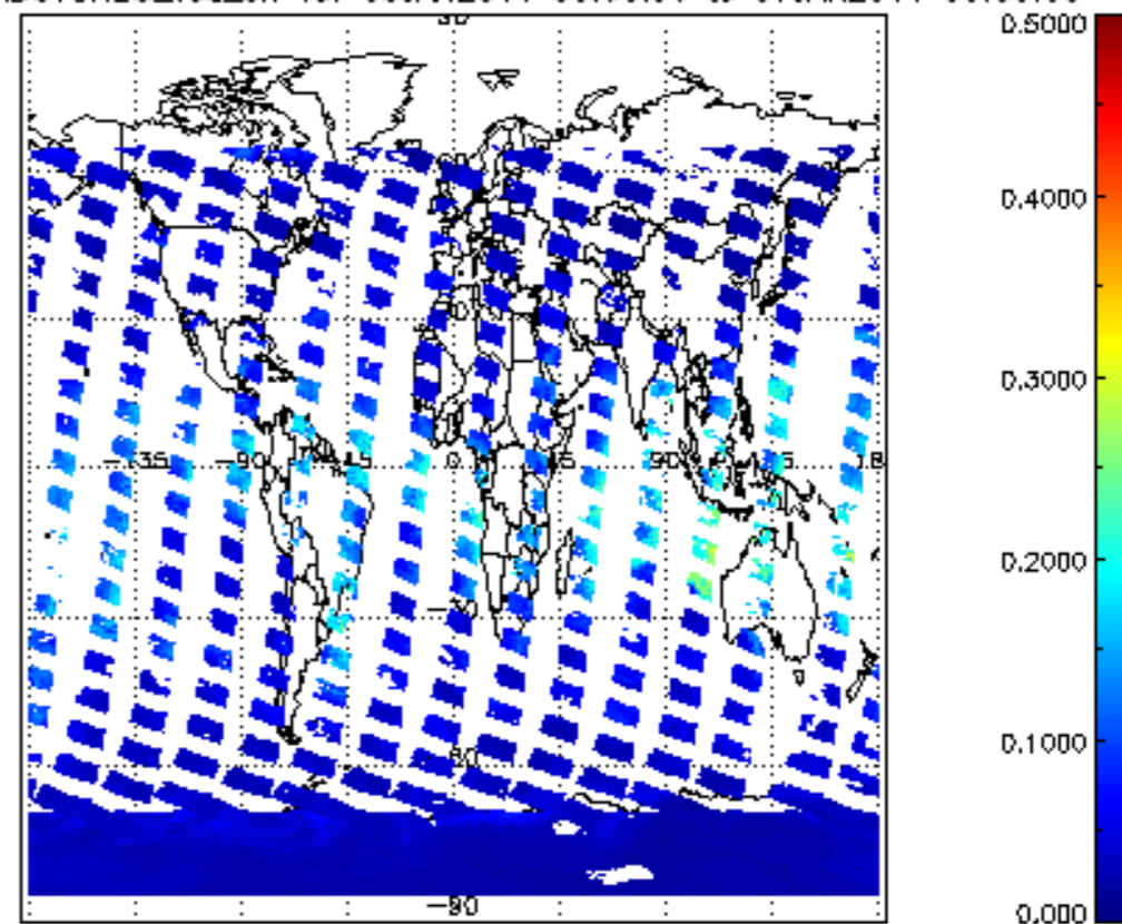
SCIOL2P_NADUV8H20_vcd_err for 06JAN2011 00:00:00 to 07JAN2011 00:00:00
