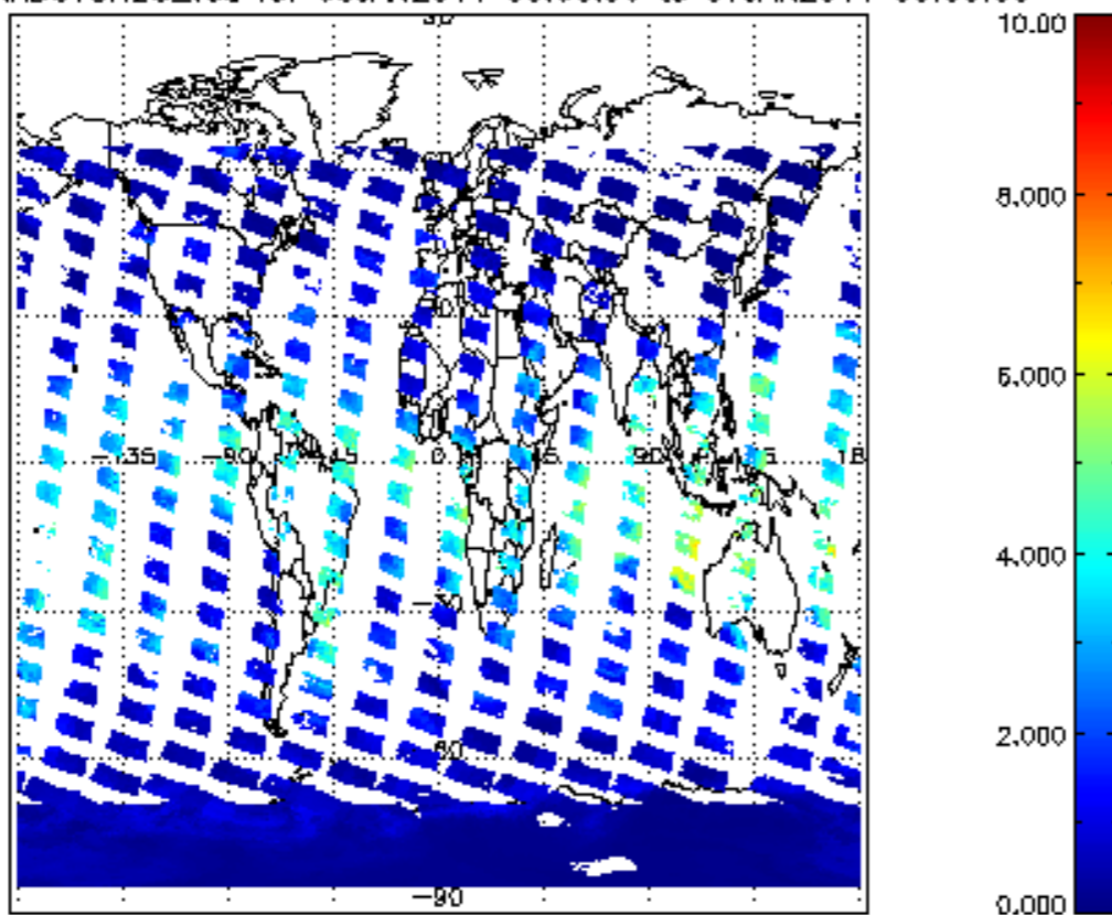
SCIOL2P_NADUV8H20_vcd for 06JAN2011 00:00:00 to 07JAN2011 00:00:00
