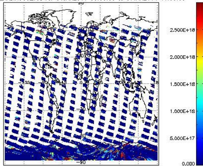
SCIDL2P_NADIR3CO_vcd for 06JAN2011 00:00:00 to 07JAN2011 00:00:00
