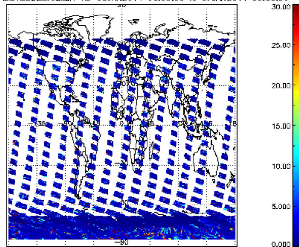
SCIOL2P_NADUV5S02_vcd_err for 06JAN2011 00:00:00 to 07JAN2011 00:00:00
