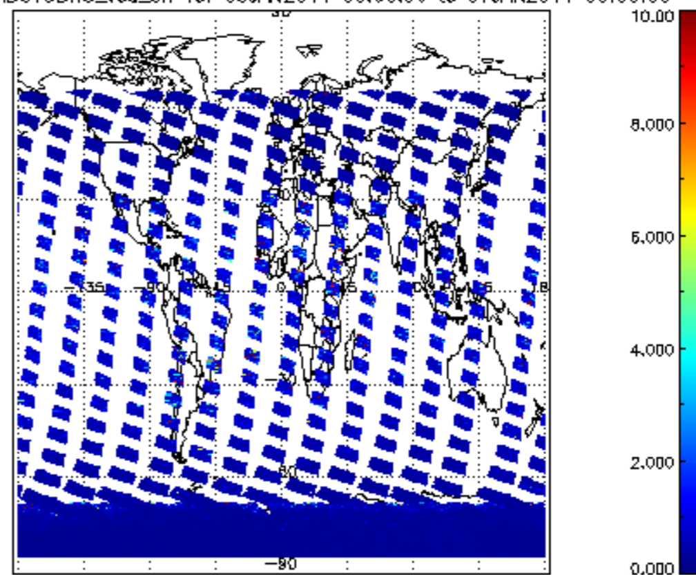
SCIOL2P_NADUV3BRO_vcd_err for 06JAN2011 00:00:00 to 07JAN2011 00:00:00
