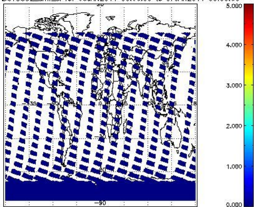
SCIOL2P_NADUV5SO2_amf_cl for 06JAN2011 00:00:00 to 07JAN2011 00:00:00
