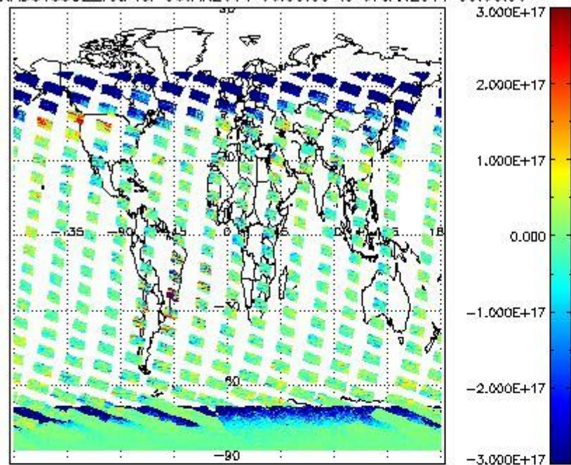
SCIOL2P_NADUV5SO2_vcd for 06JAN2011 00:00:00 to 07JAN2011 00:00:00
