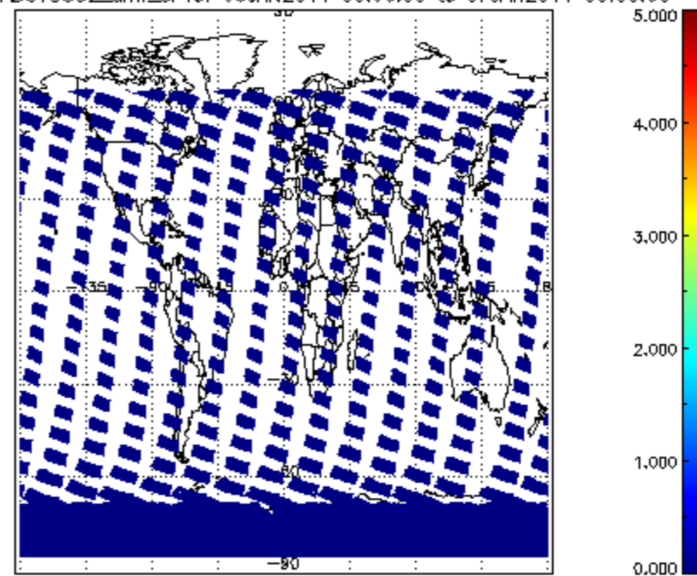
SCIOL2P_NADUV5S02_amf_cl for 06JAN2011 00:00:00 to 07JAN2011 00:00:00
