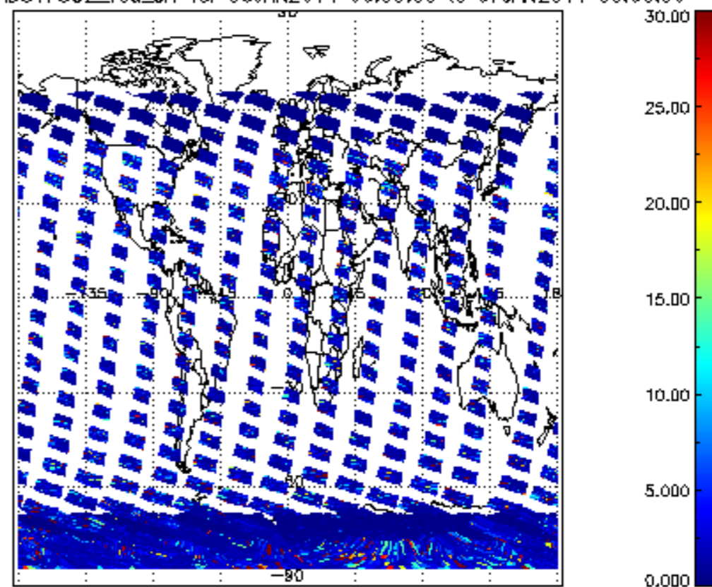
SCIOL2P_NADUV7S02_vcd_err for 06JAN2011 00:00:00 to 07JAN2011 00:00:00
