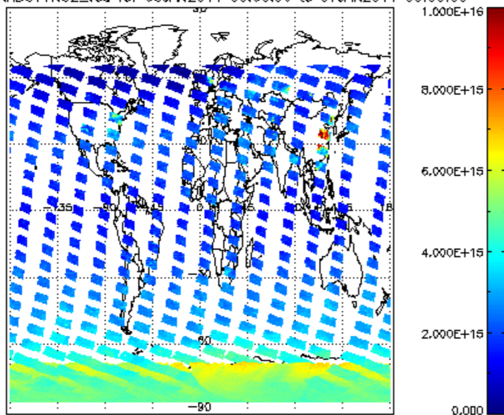
SCIOL2P_NADUV1NO2_vcd for 06JAN2011 00:00:00 to 07JAN2011 00:00:00
