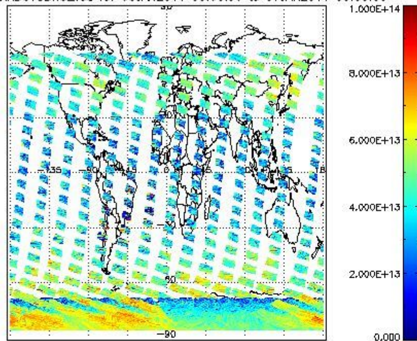
SCIOL2P_NADUV3BRO_vcd for 06JAN2011 00:00:00 to 07JAN2011 00:00:00
