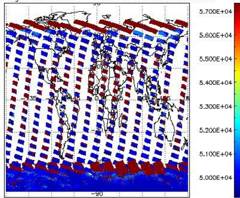
cloud_flags for 06JAN2011 00:00:00 to 07JAN2011 00:00:00
