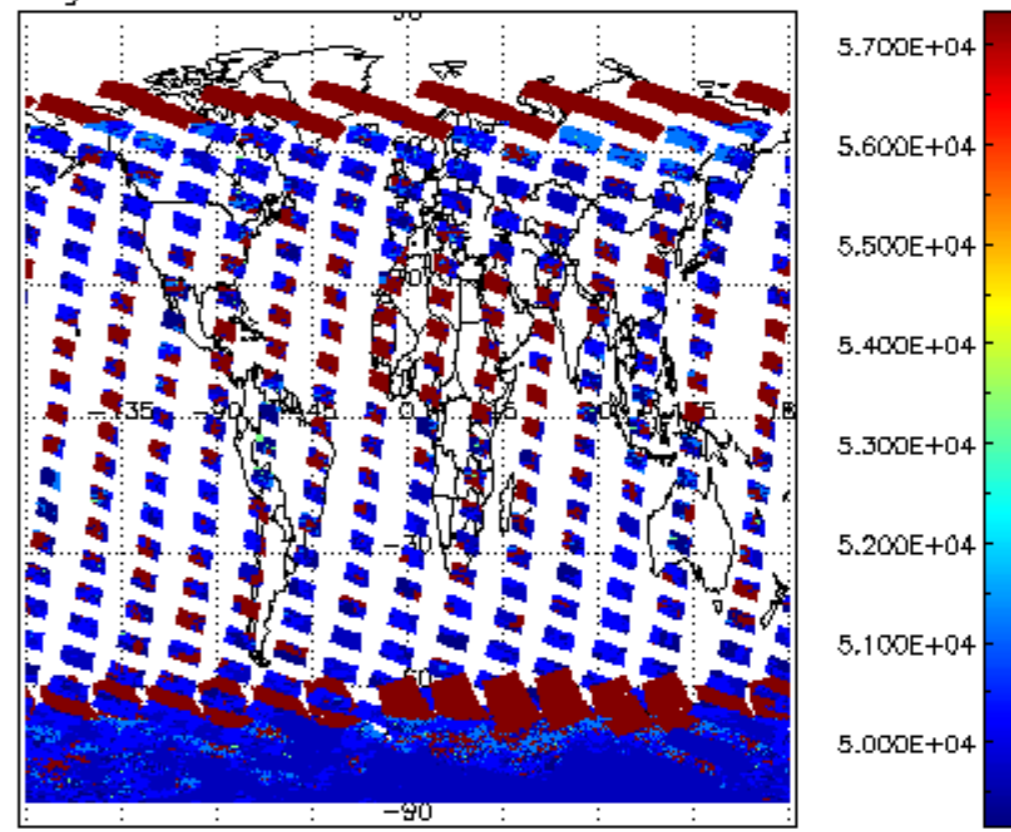
cloud_flags for 06JAN2011 00:00:00 to 07JAN2011 00:00:00
