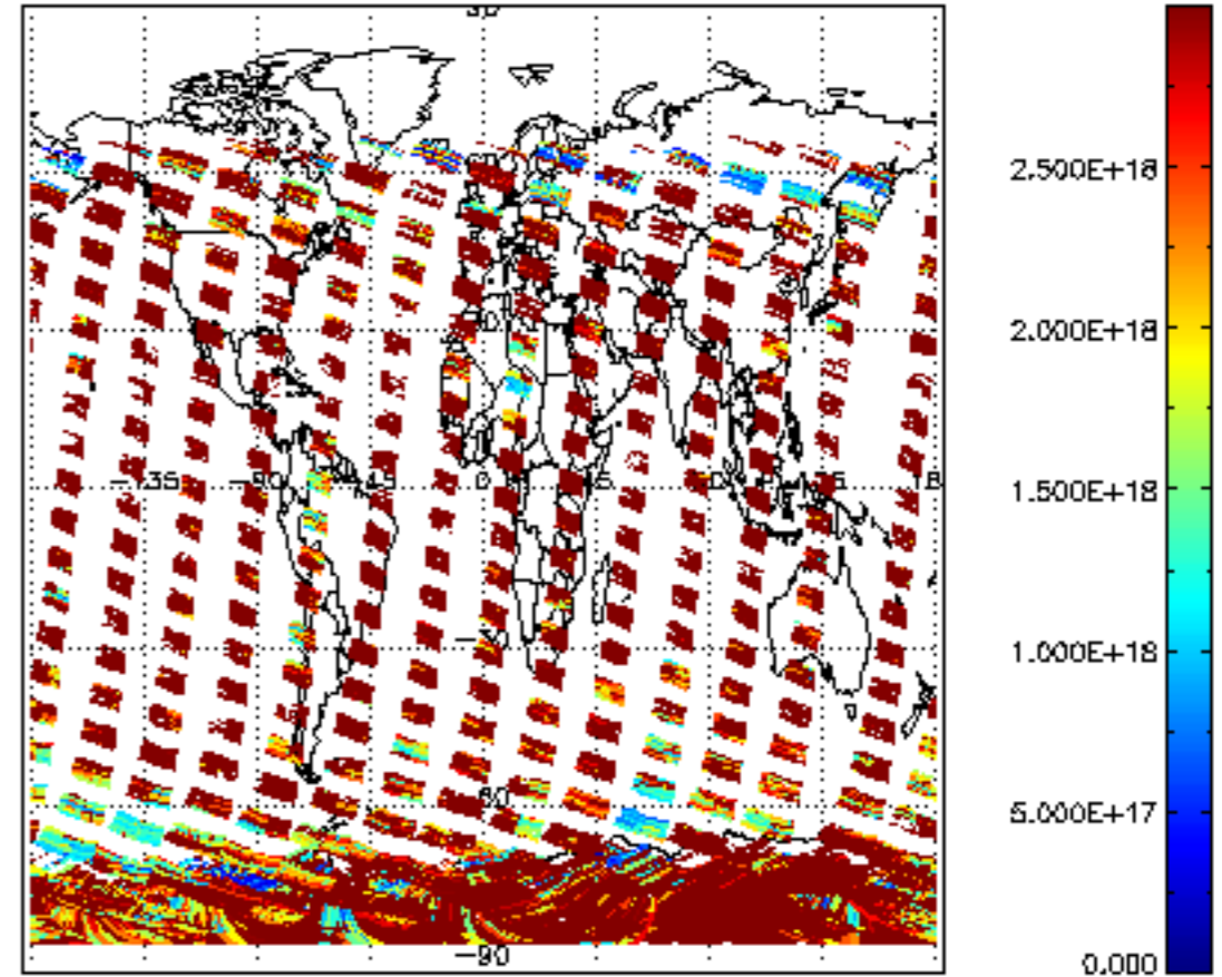
SCIOL2P_NADIR3CO_vcd_err for 06JAN2011 00:00:00 to 07JAN2011 00:00:00
