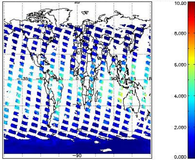
SCIOL2P_NADUV8H20_vcd for 06JAN2011 00:00:00 to 07JAN2011 00:00:00
