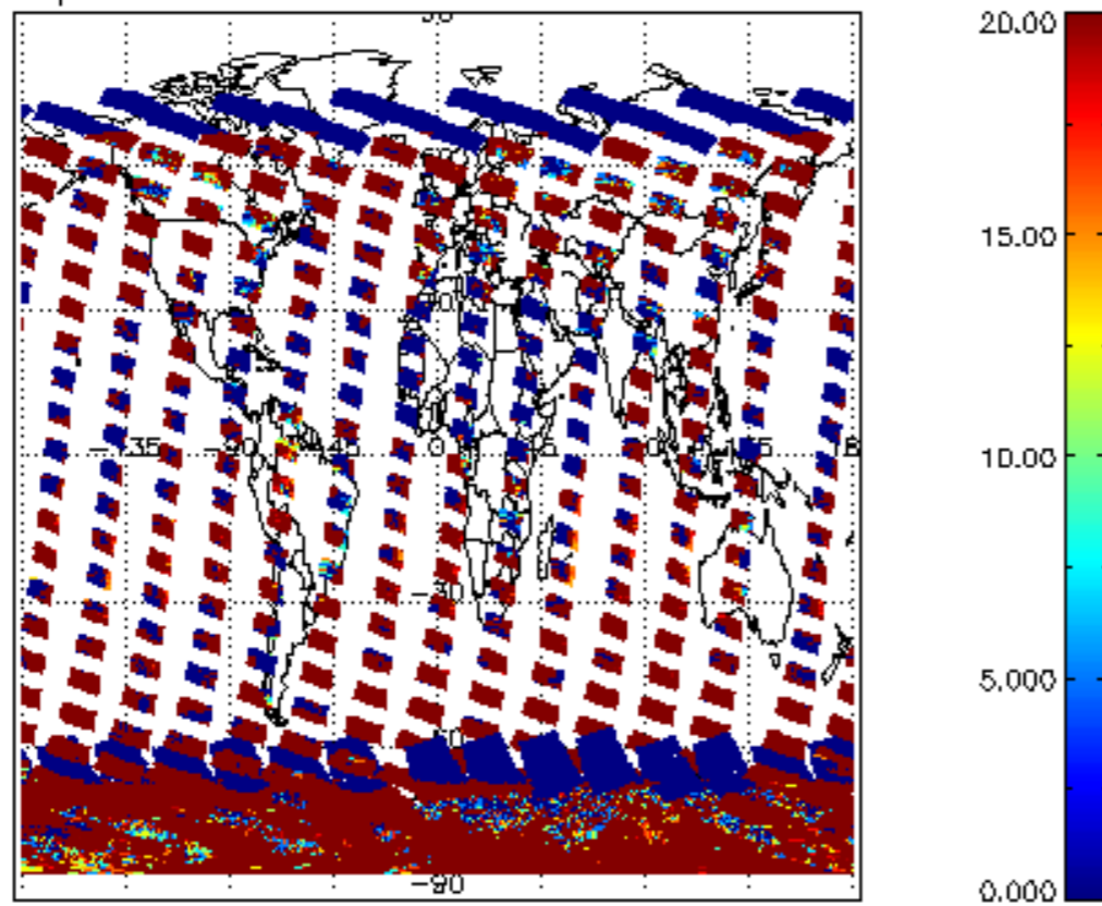
cLopt_depth for 06JAN2011 00:00:00 to 07JAN2011 00:00:00
