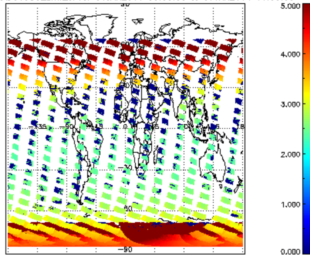
SCIOL2P_NADUV003_amf_cl for 06JAN2011 00:00:00 to 07JAN2011 00:00:00
