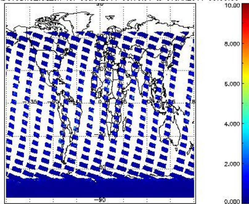
SCIOL2P_NADUV3BRO_vcd_err for 06JAN2011 00:00:00 to 07JAN2011 00:00:00
