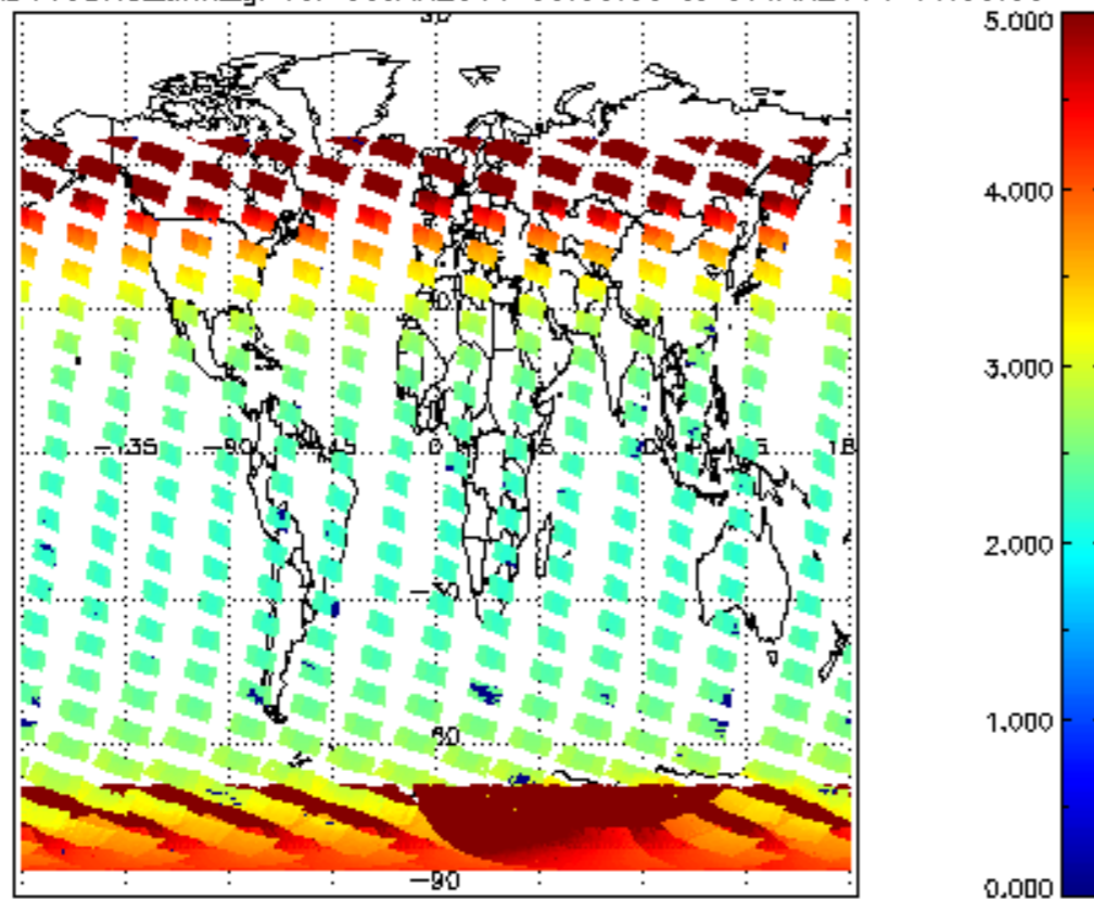
SCIOL2P_NADUV3BRO_amf_gr for 06JAN2011 00:00:00 to 07JAN2011 00:00:00
