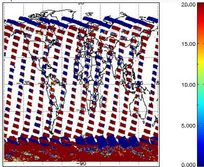
cLopt_depth for 06JAN2011 00:00:00 to 07JAN2011 00:00:00
