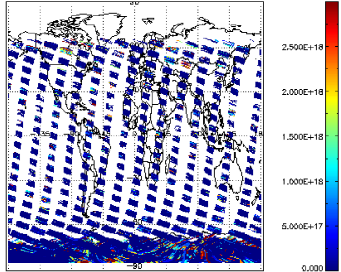
SCIOL2P_NADIR3CO_vcd for 06JAN2011 00:00:00 to 07JAN2011 00:00:00
