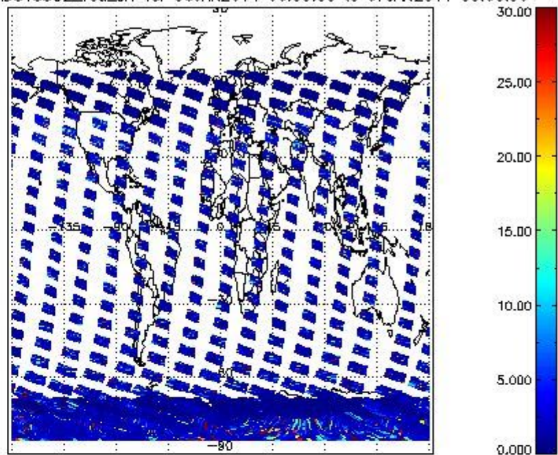
SCIOL2P_NADUV5SO2_vcd_err for 06JAN2011 00:00:00 to 07JAN2011 00:00:00
