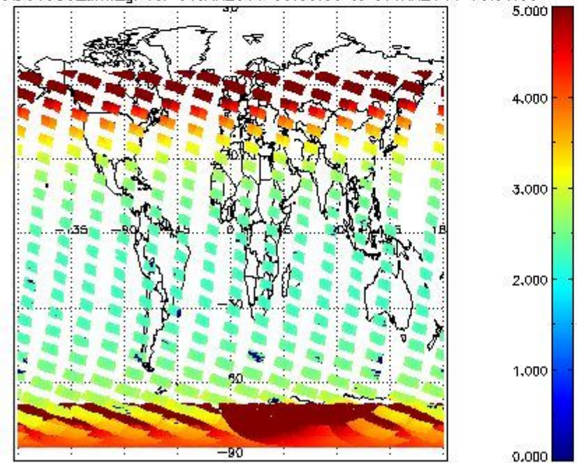
SCIOL2P_NADUV003_amf_gr for 06JAN2011 00:00:00 to 07JAN2011 00:00:00
