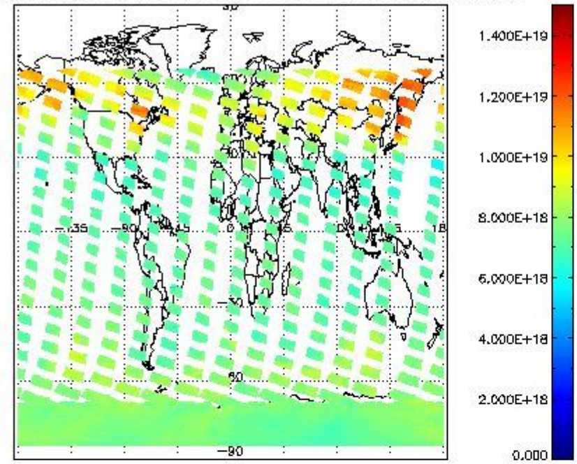
SCIOL2P_NADUV003_vcd for 06JAN2011 00:00:00 to 07JAN2011 00:00:00
