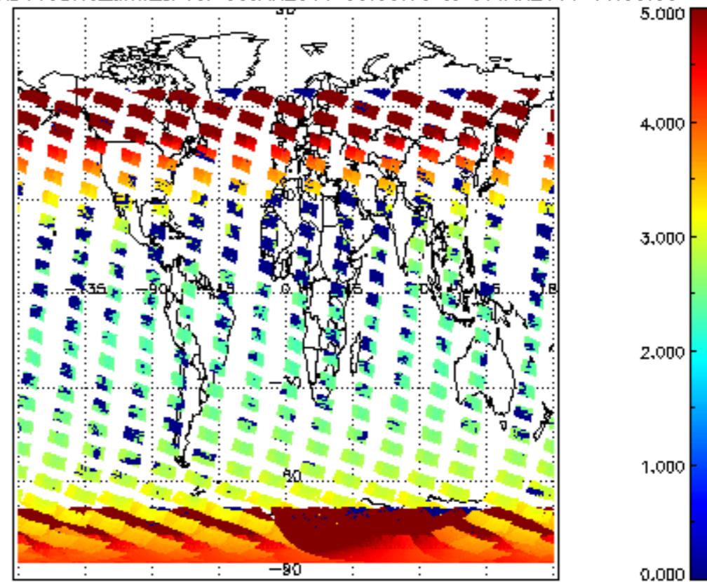
SCIOL2P_NADUV3BRO_amf_cl for 06JAN2011 00:00:00 to 07JAN2011 00:00:00
