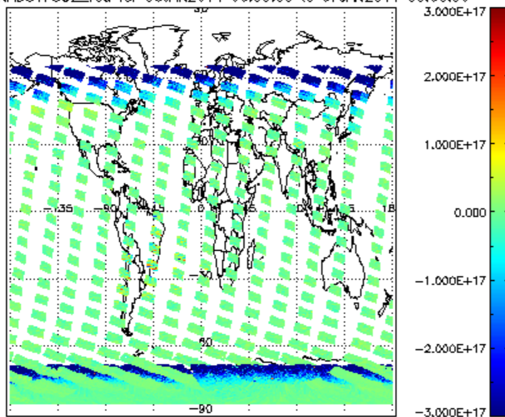
SCIOL2P_NADUV7S02_vcd for 06JAN2011 00:00:00 to 07JAN2011 00:00:00
