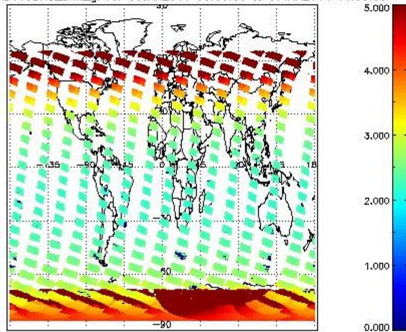
SCIOL2P_NADUV3BRO_amf_gr for 06JAN2011 00:00:00 to 07JAN2011 00:00:00
