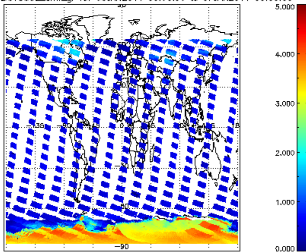
SCIOL2P_NADUV5S02_amf_gr for 06JAN2011 00:00:00 to 07JAN2011 00:00:00
