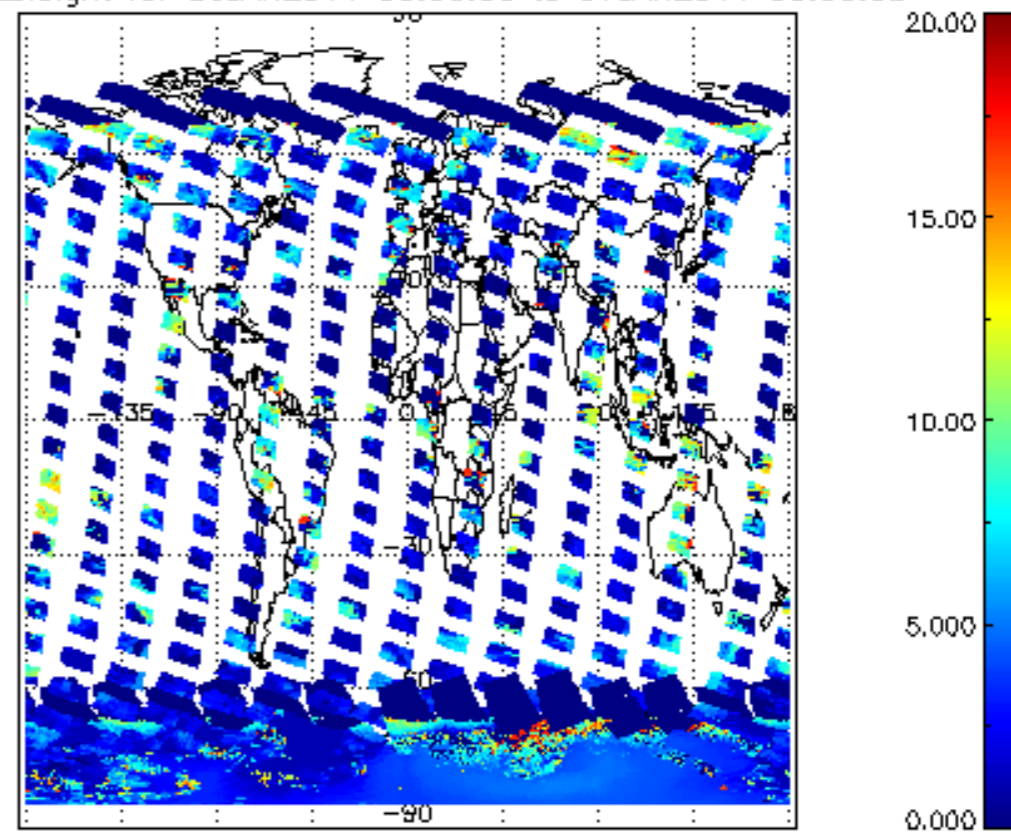
cL_top_height for 06JAN2011 00:00:00 to 07JAN2011 00:00:00
