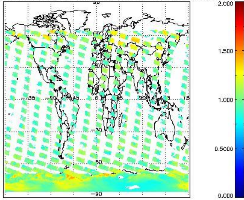
SCIOL2P_NADUV8H20_amf_gr for 06JAN2011 00:00:00 to 07JAN2011 00:00:00
