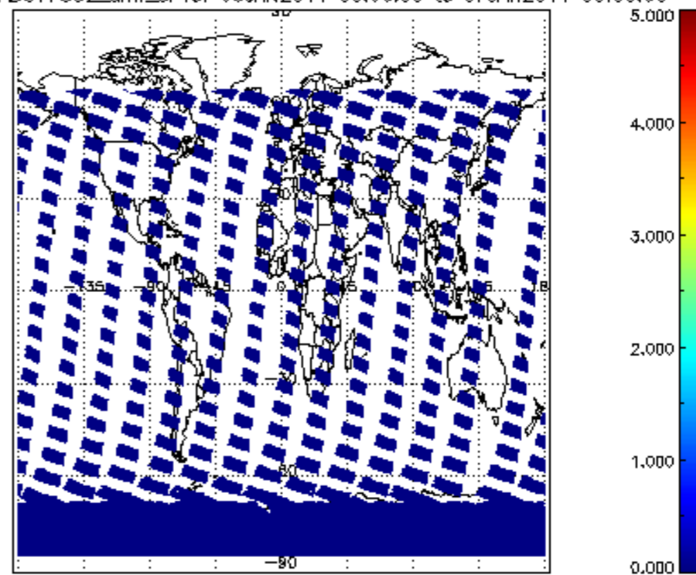
SCIOL2P_NADUV7S02_amf_cl for 06JAN2011 00:00:00 to 07JAN2011 00:00:00
