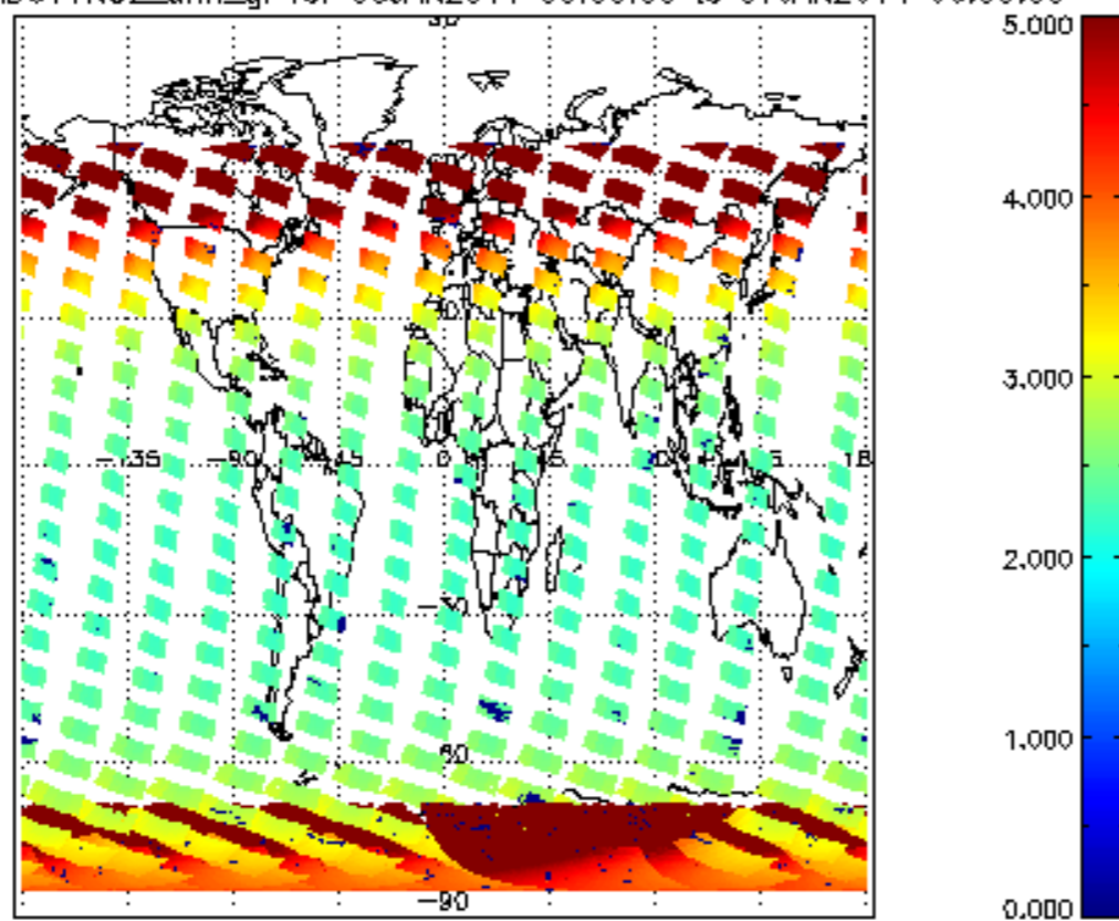
SCIOL2P_NADUV1NO2_amf_gr for 06JAN2011 00:00:00 to 07JAN2011 00:00:00
