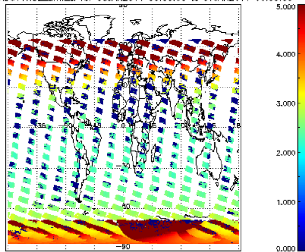
SCIOL2P_NADUV1NO2_amf_cl for 06JAN2011 00:00:00 to 07JAN2011 00:00:00
