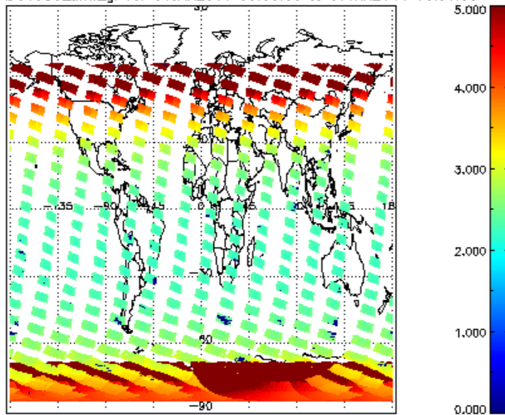
SCIOL2P_NADUV003_amf_gr for 06JAN2011 00:00:00 to 07JAN2011 00:00:00
