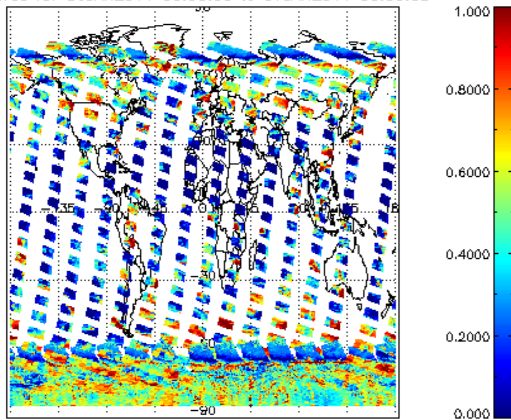
cL_frac for 06JAN2011 00:00:00 to 07JAN2011 00:00:00
