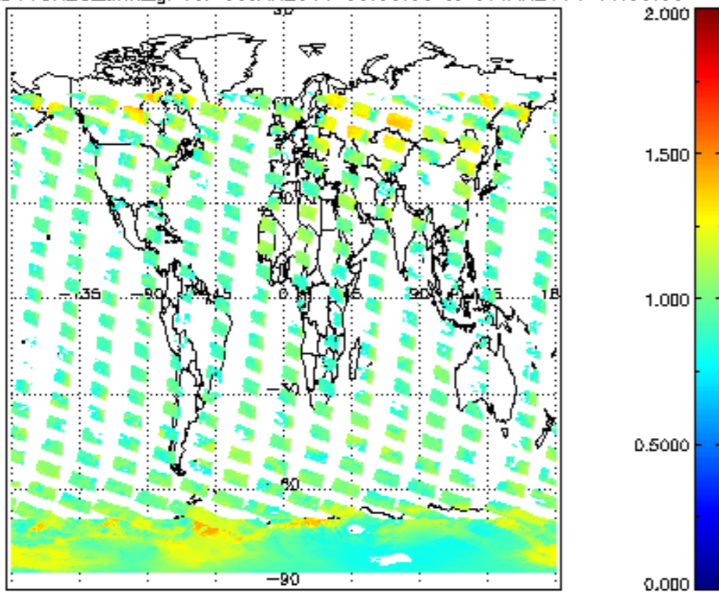
SCIOL2P_NADUV8H20_amf_gr for 06JAN2011 00:00:00 to 07JAN2011 00:00:00
