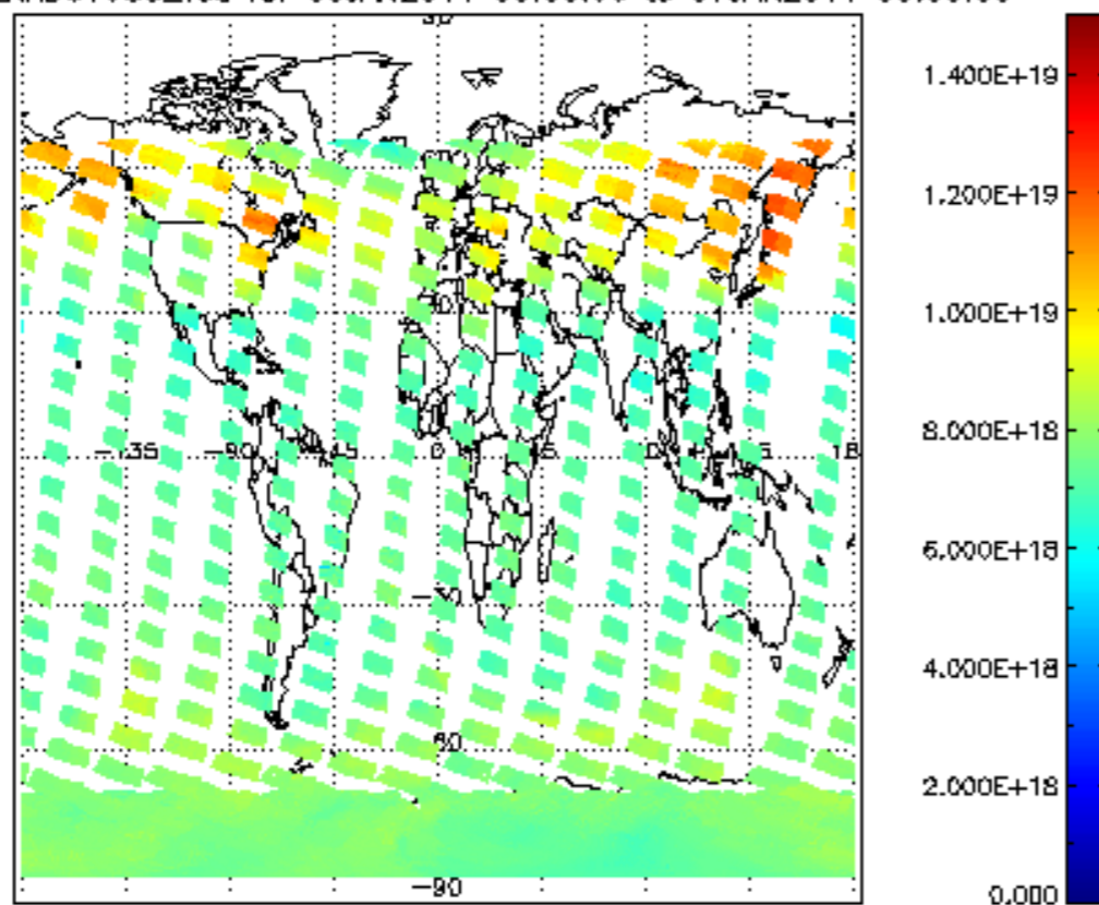
SCIOL2P_NADUV003_vcd for 06JAN2011 00:00:00 to 07JAN2011 00:00:00
