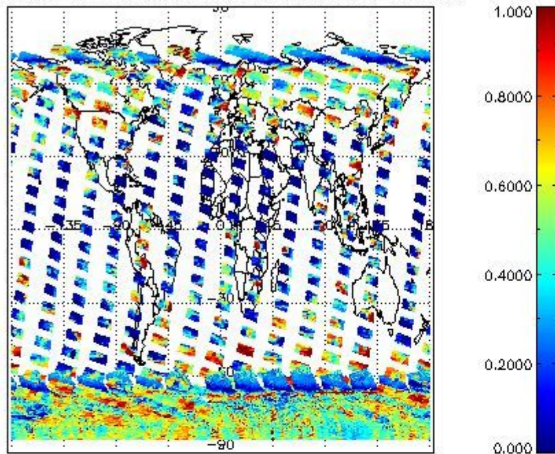
cL_frac for 06JAN2011 00:00:00 to 07JAN2011 00:00:00
