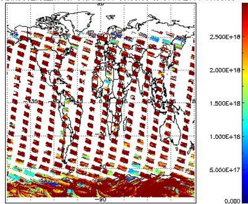
SCIDL2P_NADIR3CO_vcd_err for 06JAN2011 00:00:00 to 07JAN2011 00:00:00
