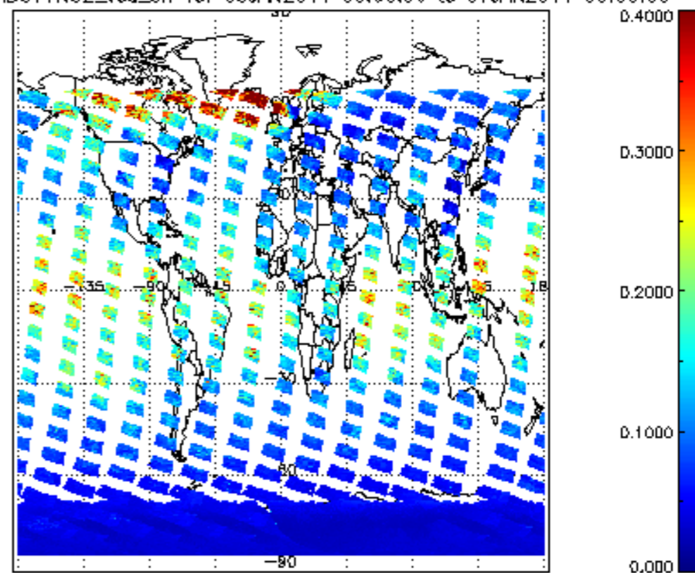
SCIOL2P_NADUV1NO2_vcd_err for 06JAN2011 00:00:00 to 07JAN2011 00:00:00
