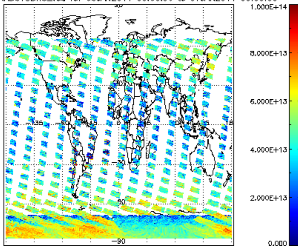
SCIOL2P_NADUV3BRO_vcd for 06JAN2011 00:00:00 to 07JAN2011 00:00:00
