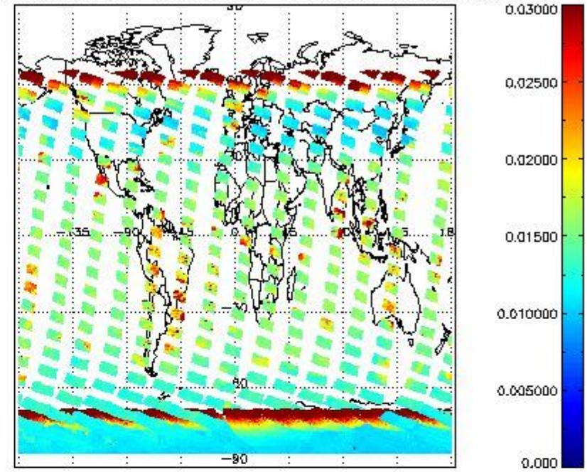
SCIOL2P_NADUV003_vcd_err for 06JAN2011 00:00:00 to 07JAN2011 00:00:00
