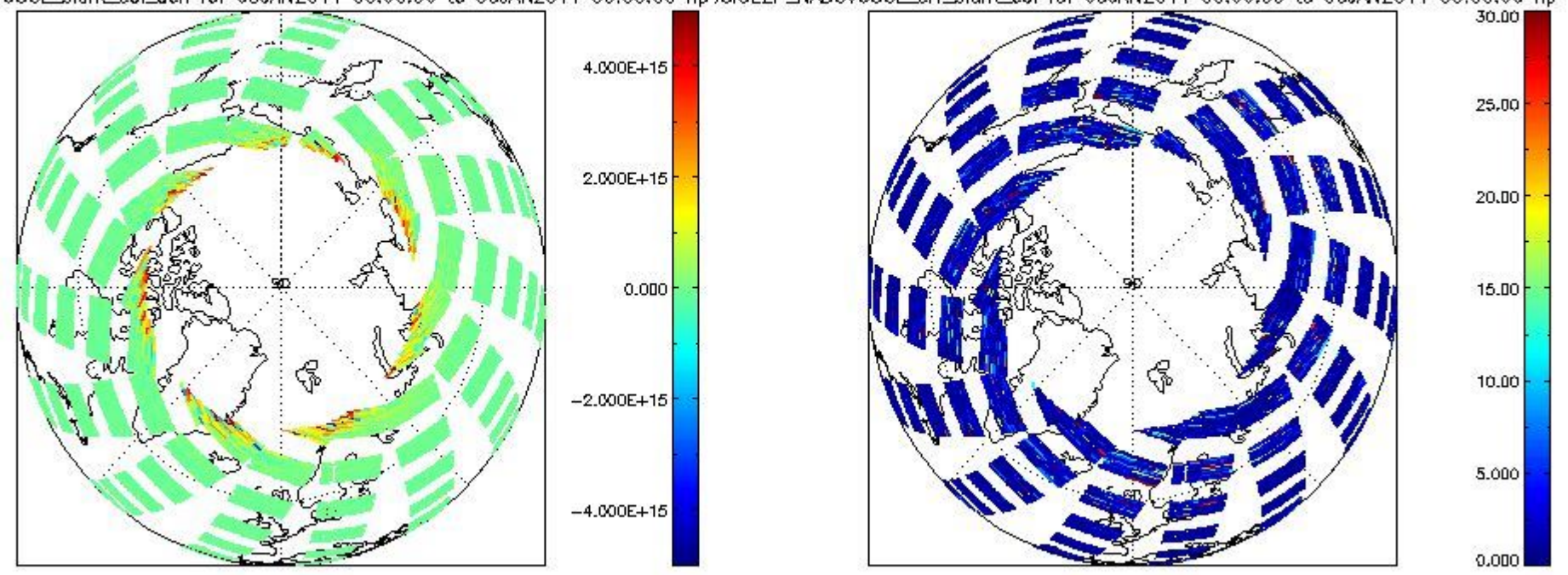
SCIOI2P_NADUV60CL_slant_col_den for 05JAN2011 00:00:00 to 06JAN2011 00:00:00 np; SCIOI2P_NADUV60CL_err_slant_col for 05JAN2011 00:00:00 to 06JAN2011 00:00:00 np
