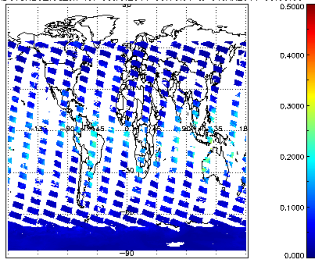
SCIOL2P_NADUVB8H20_vcd_err for 05JAN2011 00:00:00 to 06JAN2011 00:00:00
