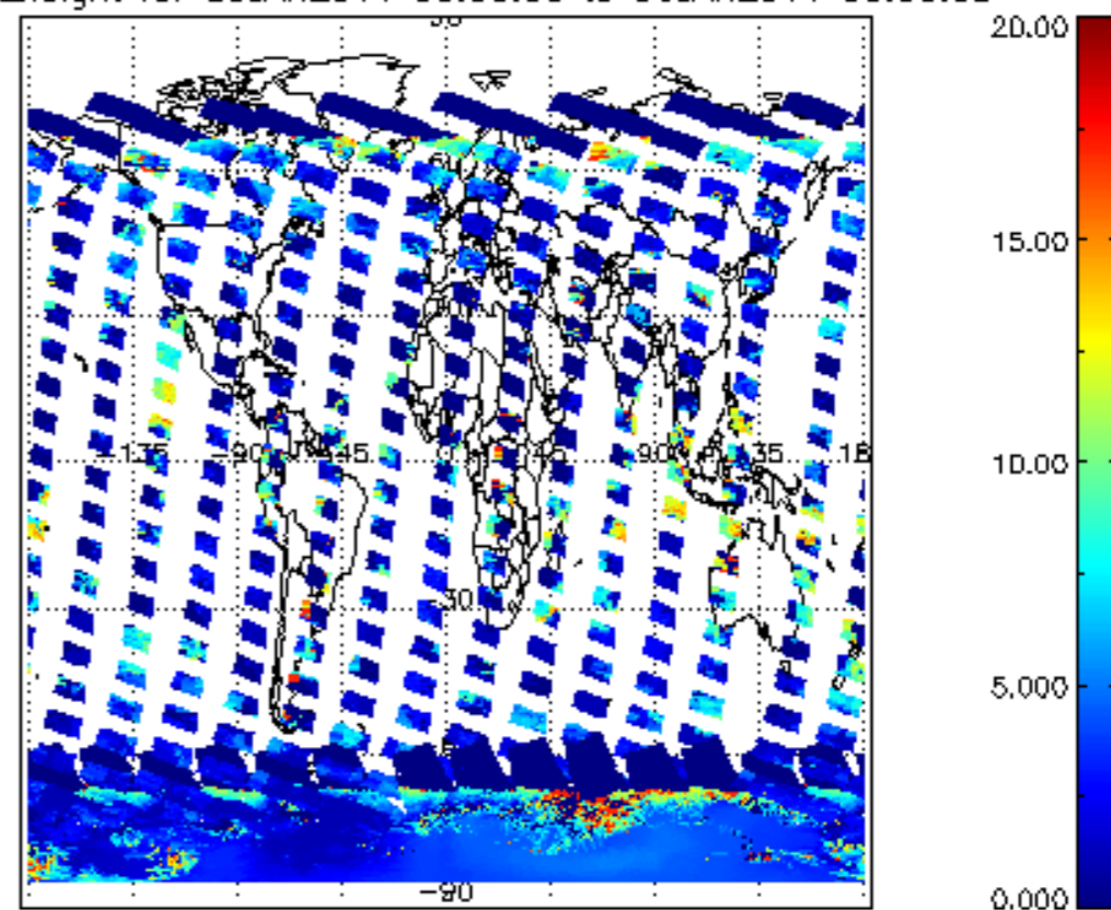
cL_top_height for 05JAN2011 00:00:00 to 06JAN2011 00:00:00
