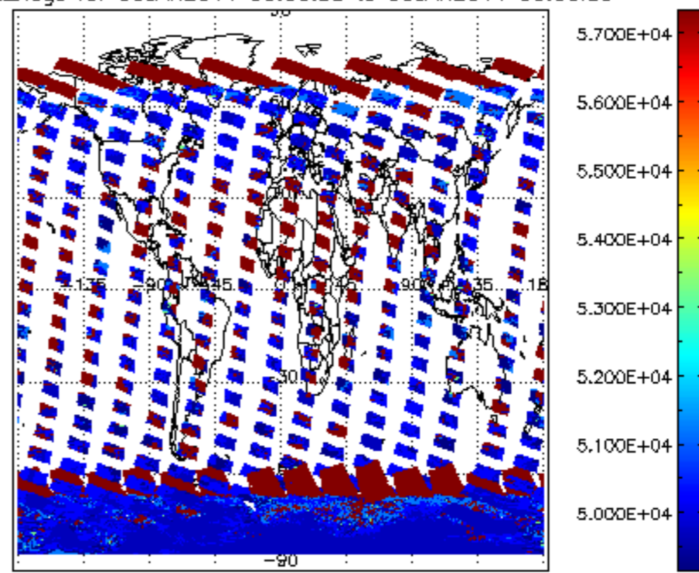
cloud_flags for 05JAN2011 00:00:00 to 06JAN2011 00:00:00
