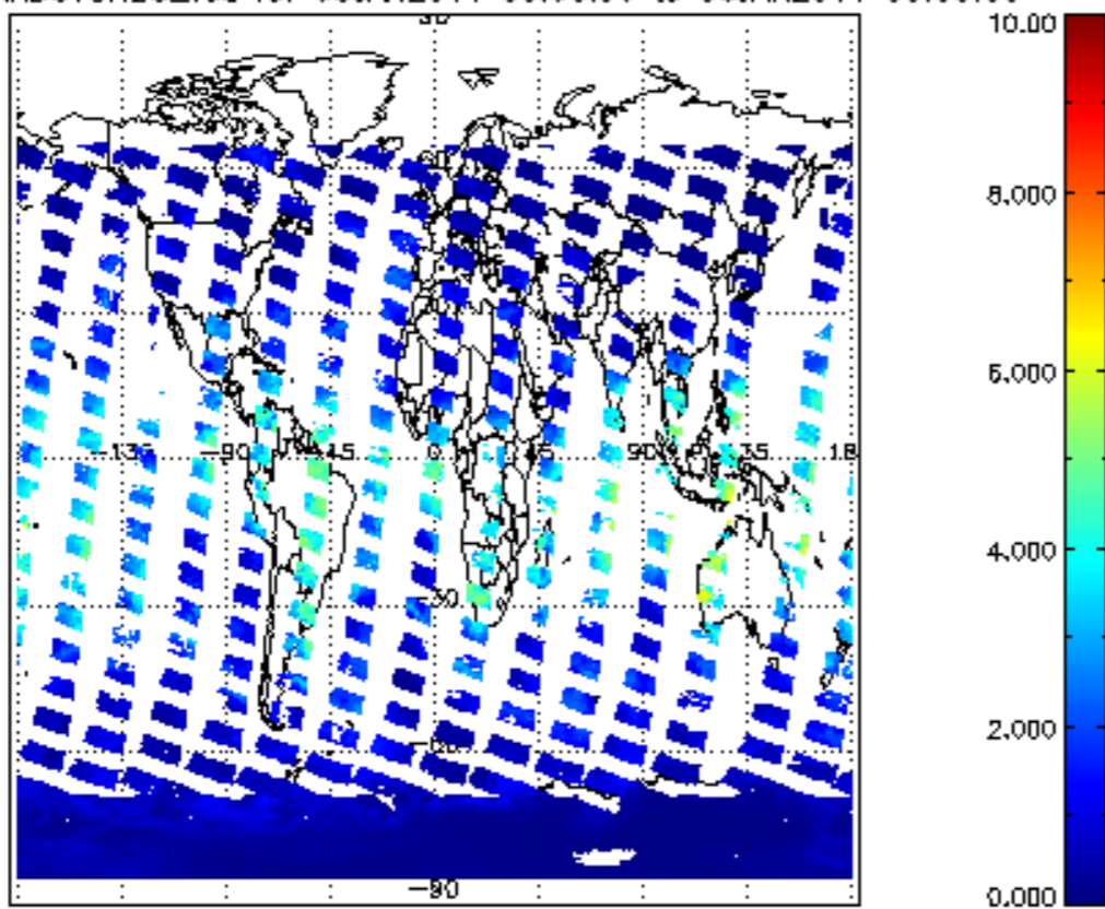
SCIOL2P_NADUVB8H20_vcd for 05JAN2011 00:00:00 to 06JAN2011 00:00:00
