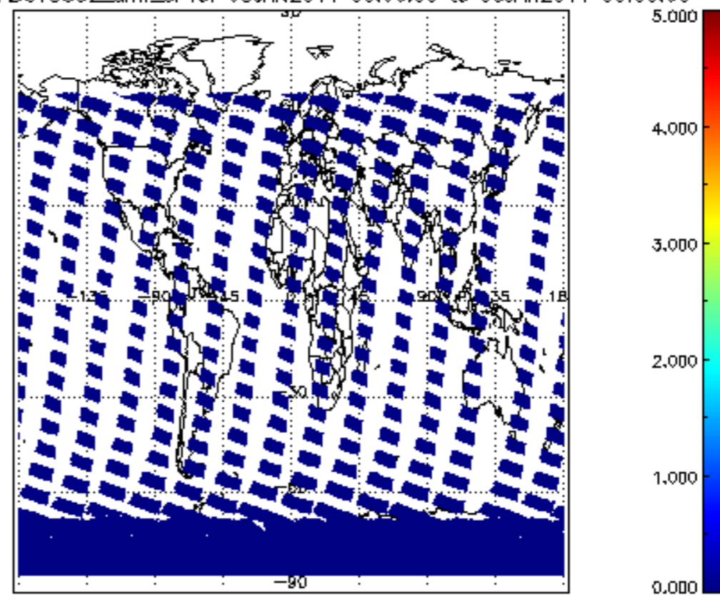
SCIOL2P_NADUV5S02_amf_cl for 05JAN2011 00:00:00 to 06JAN2011 00:00:00
