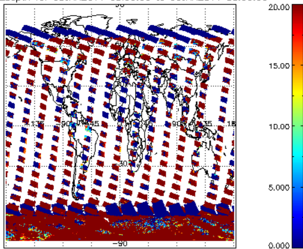
cLopt_depth for 05JAN2011 00:00:00 to 06JAN2011 00:00:00
