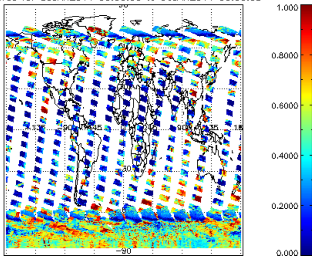
cL_frac for 05JAN2011 00:00:00 to 06JAN2011 00:00:00
