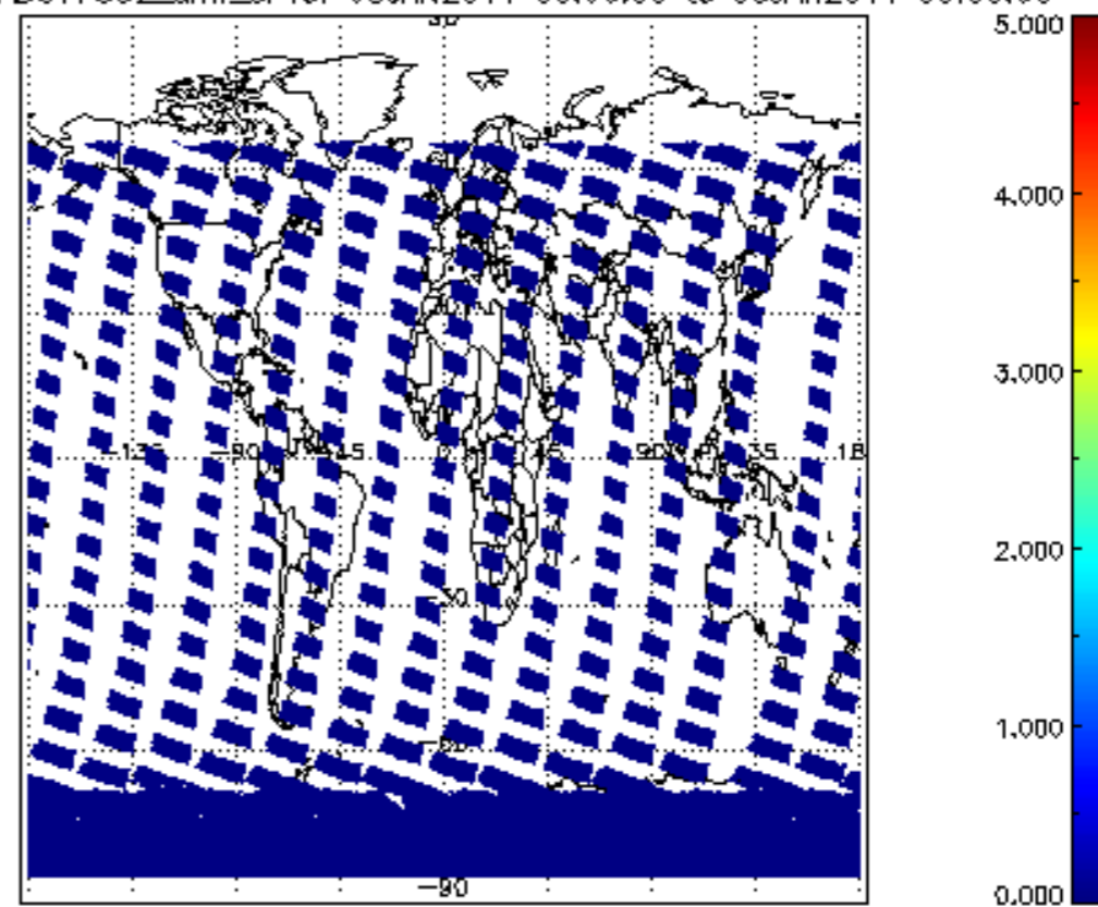
SCIOL2P_NADUV7S02_amf_cl for 05JAN2011 00:00:00 to 06JAN2011 00:00:00
