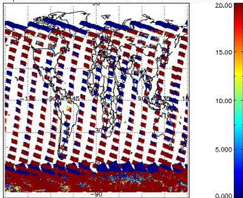
cLopt_depth for 02JAN2011 00:00:00 to 03JAN2011 00:00:00
