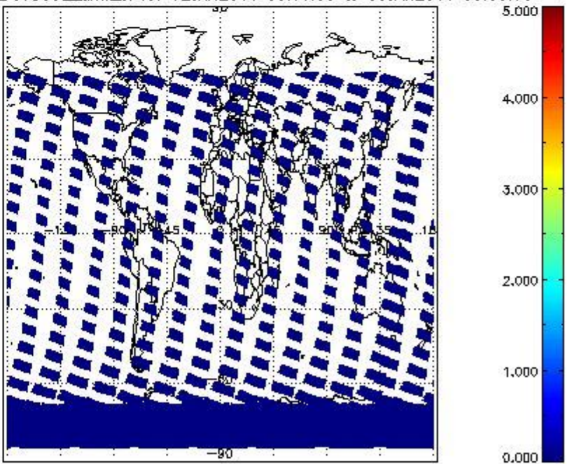
SCIOL2P_NADUV5S02_amf_cl for 02JAN2011 00:00:00 to 03JAN2011 00:00:00
