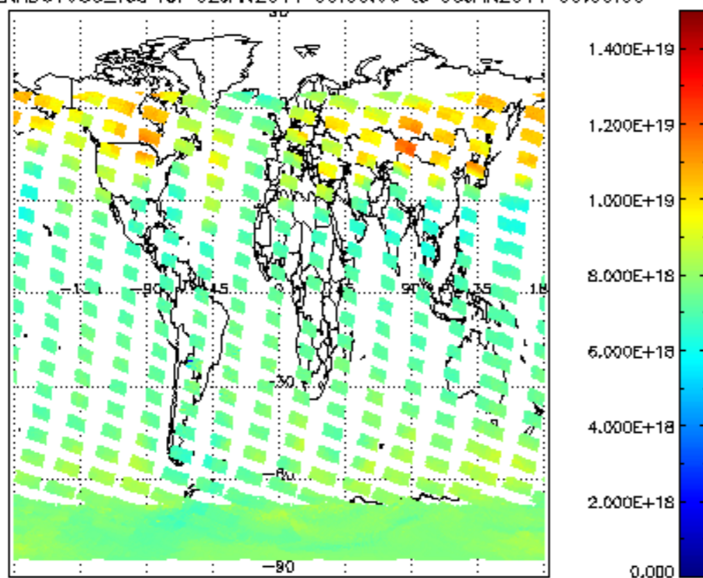
SCIOL2P_NADUV003_vcd for 02JAN2011 00:00:00 to 03JAN2011 00:00:00
