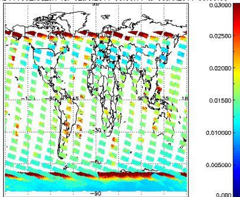
SCIOL2P_NADUV003_vcd_err for 02JAN2011 00:00:00 to 03JAN2011 00:00:00
