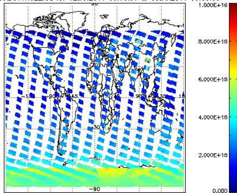
SCIOL2P_NADUV1NO2_vcd for 02JAN2011 00:00:00 to 03JAN2011 00:00:00
