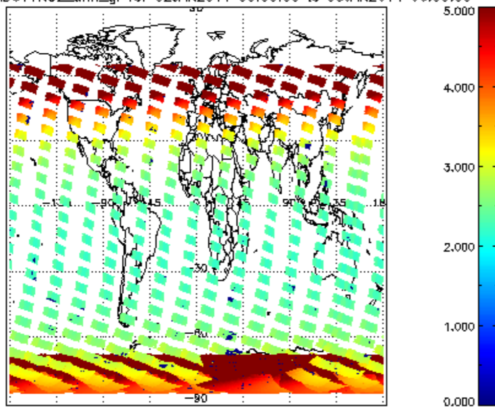
SCIOL2P_NADUV1NO2_amf_gr for 02JAN2011 00:00:00 to 03JAN2011 00:00:00
