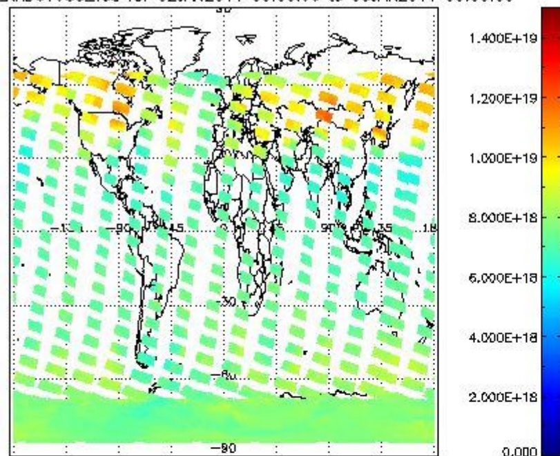
SCIOL2P_NADUV003_vcd for 02JAN2011 00:00:00 to 03JAN2011 00:00:00
