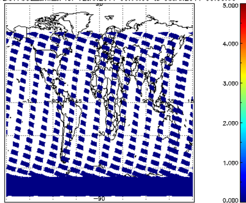
SCIOL2P_NADUV7S02_amf_sl for 02JAN2011 00:00:00 to 03JAN2011 00:00:00
