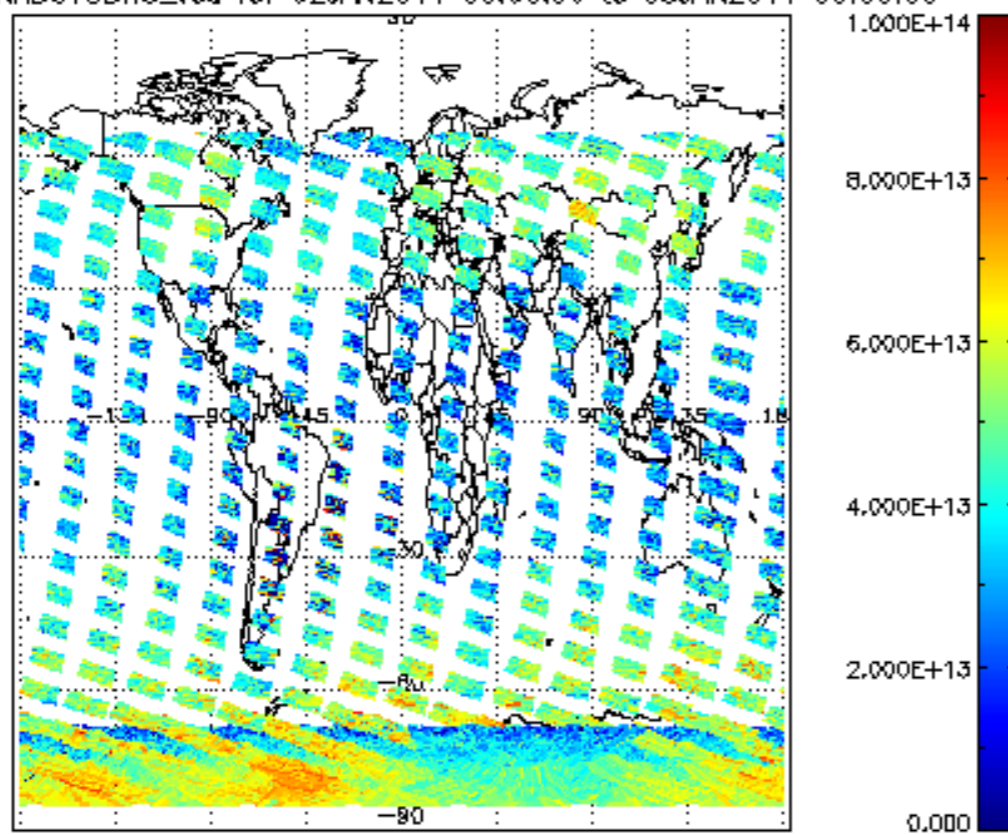
SCIOL2P_NADUV3BRO_vcd for 02JAN2011 00:00:00 to 03JAN2011 00:00:00
