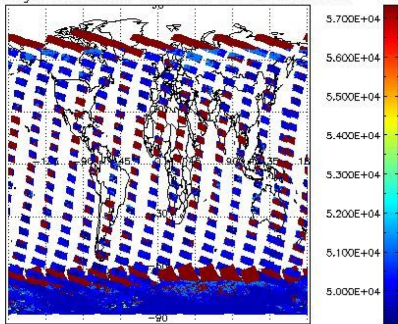
cloud_flags for 02JAN2011 00:00:00 to 03JAN2011 00:00:00
