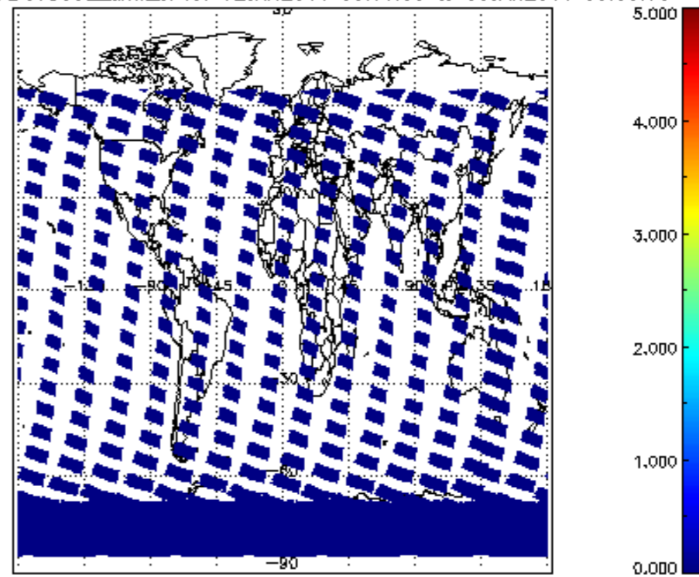
SCIOL2P_NADUV5S02_amf_sl for 02JAN2011 00:00:00 to 03JAN2011 00:00:00
