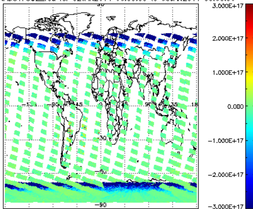
SCIOL2P_NADUV7S02_vcd for 02JAN2011 00:00:00 to 03JAN2011 00:00:00
