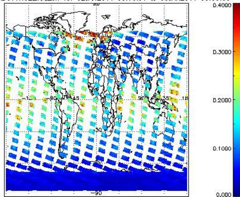
SCIOL2P_NADUV1NO2_vcd_err for 02JAN2011 00:00:00 to 03JAN2011 00:00:00
