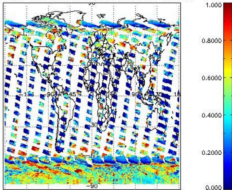
cL_frac for 02JAN2011 00:00:00 to 03JAN2011 00:00:00
