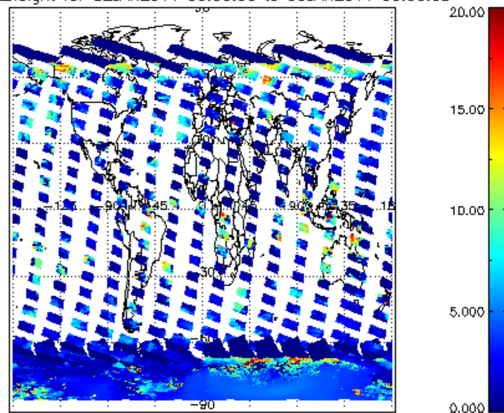
cL_top_height for 02JAN2011 00:00:00 to 03JAN2011 00:00:00
