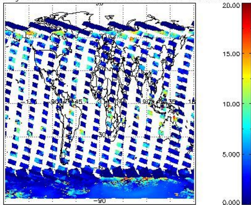
cL_top_height for 02JAN2011 00:00:00 to 03JAN2011 00:00:00
