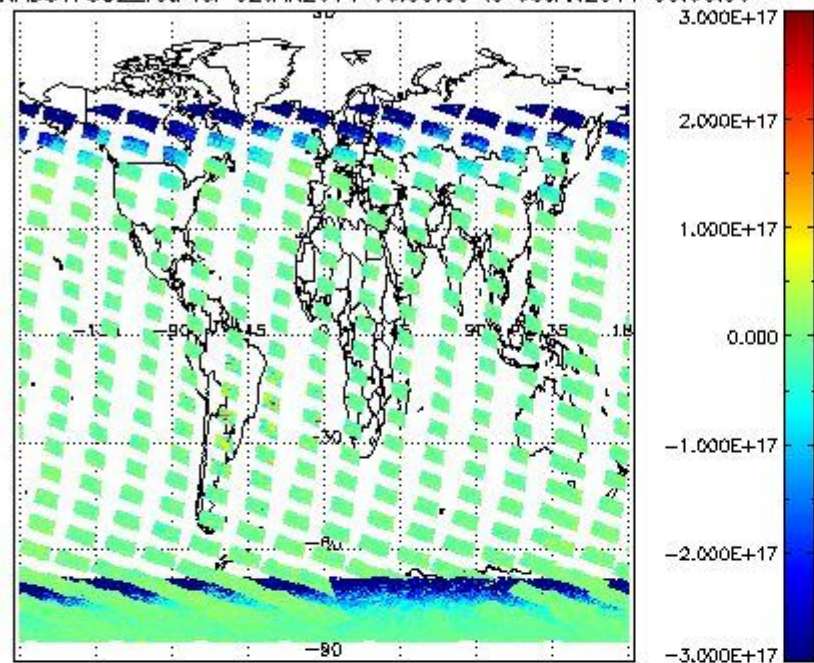
SCIOL2P_NADUV7S02_vcd for 02JAN2011 00:00:00 to 03JAN2011 00:00:00
