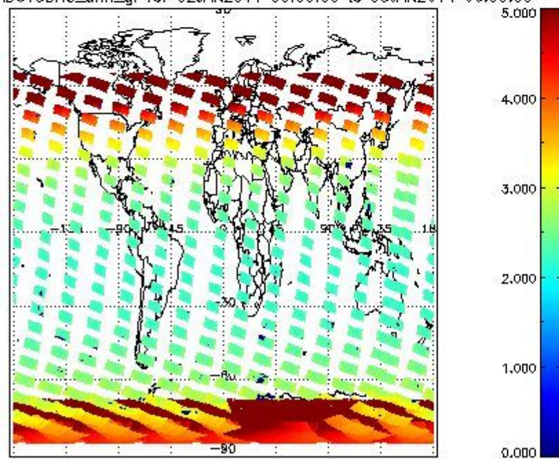
SCIOL2P_NADUV3BRO_amf_gr for 02JAN2011 00:00:00 to 03JAN2011 00:00:00
