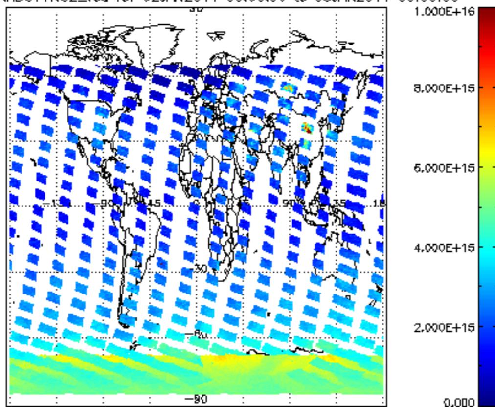
SCIOL2P_NADUV1NO2_vcd for 02JAN2011 00:00:00 to 03JAN2011 00:00:00
