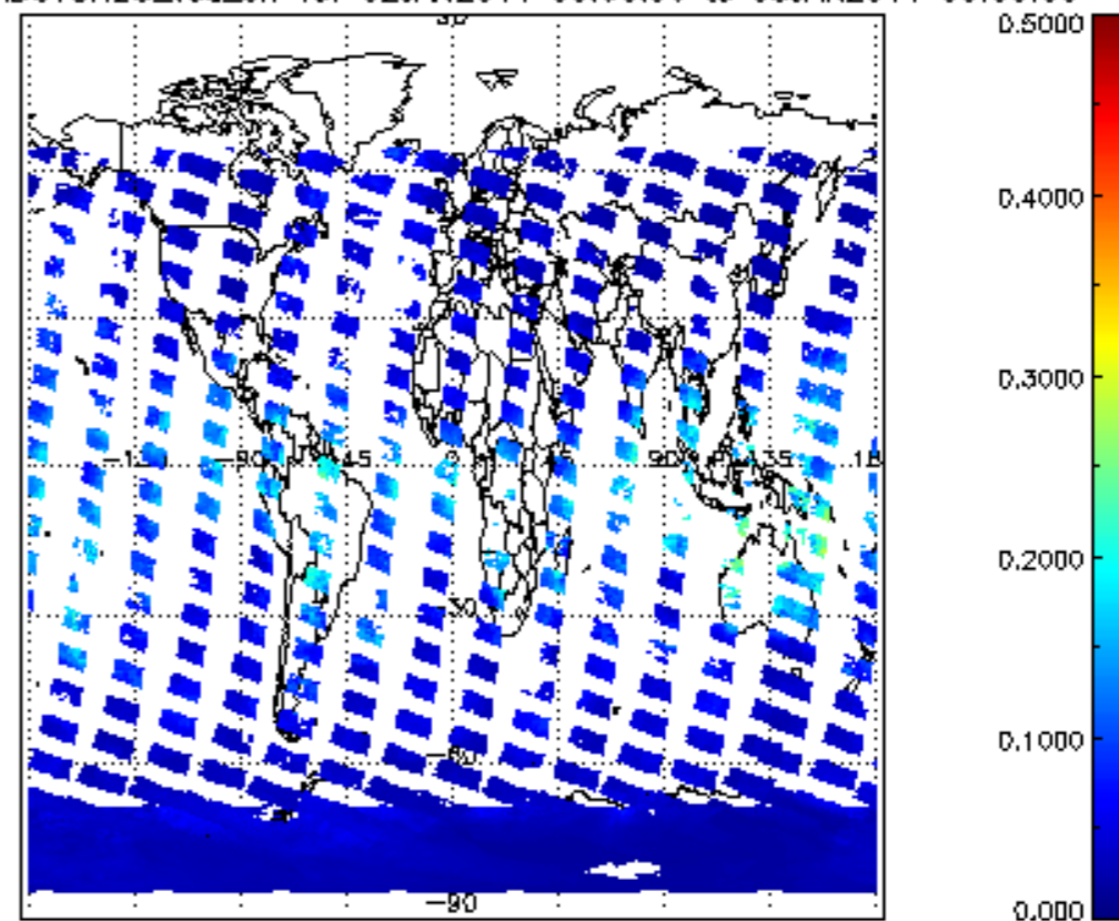
SCIOL2P_NADUV8H20_vcd_err for 02JAN2011 00:00:00 to 03JAN2011 00:00:00
