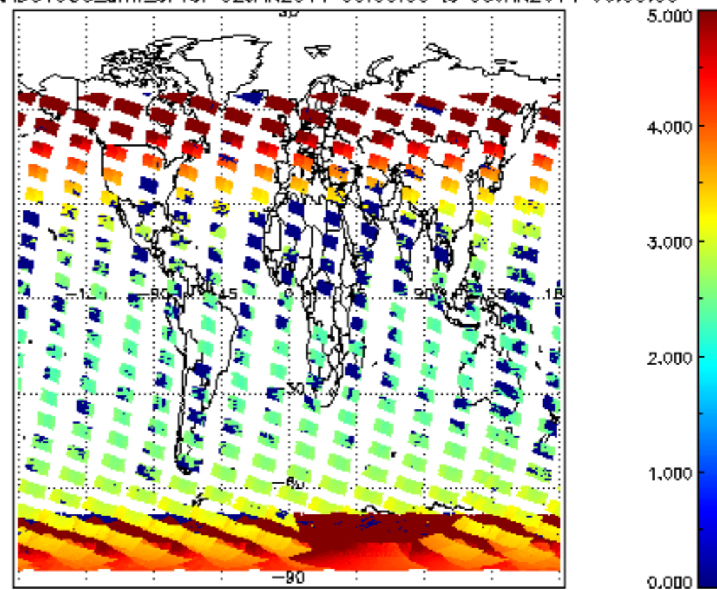
SCIOL2P_NADUV003_amf_cl for 02JAN2011 00:00:00 to 03JAN2011 00:00:00
