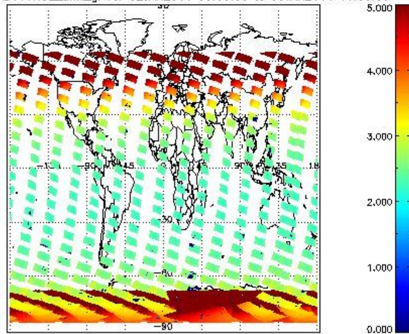
SCIOL2P_NADUV1NO2_amf_gr for 02JAN2011 00:00:00 to 03JAN2011 00:00:00
