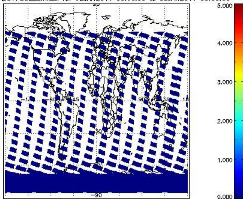
SCIOL2P_NADUV7S02_amf_cl for 02JAN2011 00:00:00 to 03JAN2011 00:00:00
