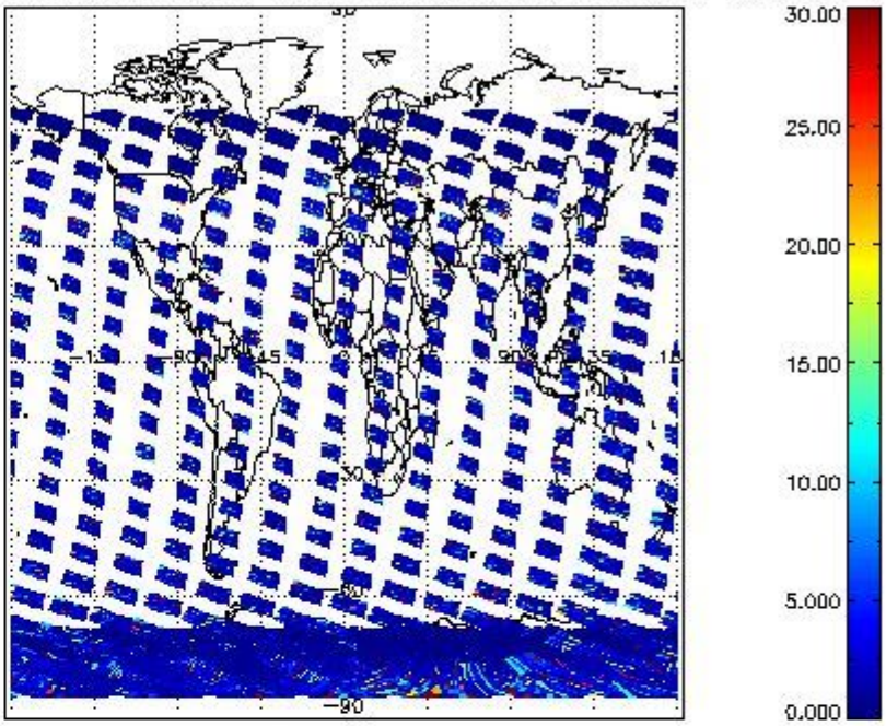
SCIOL2P_NADUV5S02_vcd_err for 02JAN2011 00:00:00 to 03JAN2011 00:00:00
