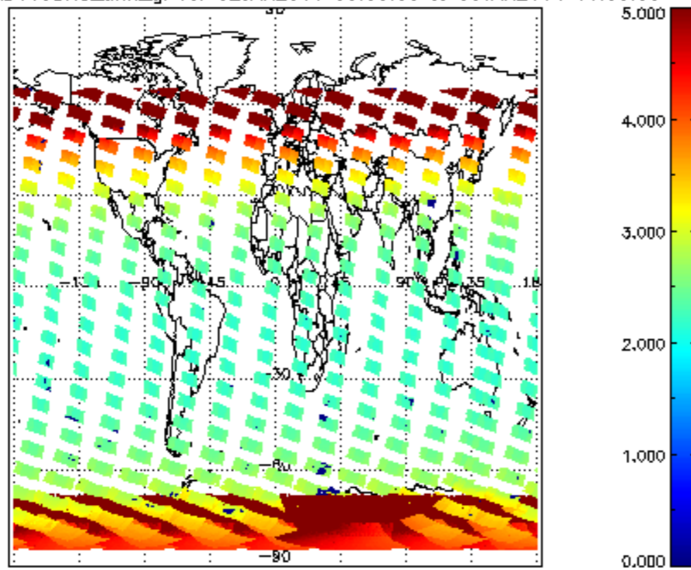
SCIOL2P_NADUV3BRO_amf_gr for 02JAN2011 00:00:00 to 03JAN2011 00:00:00
