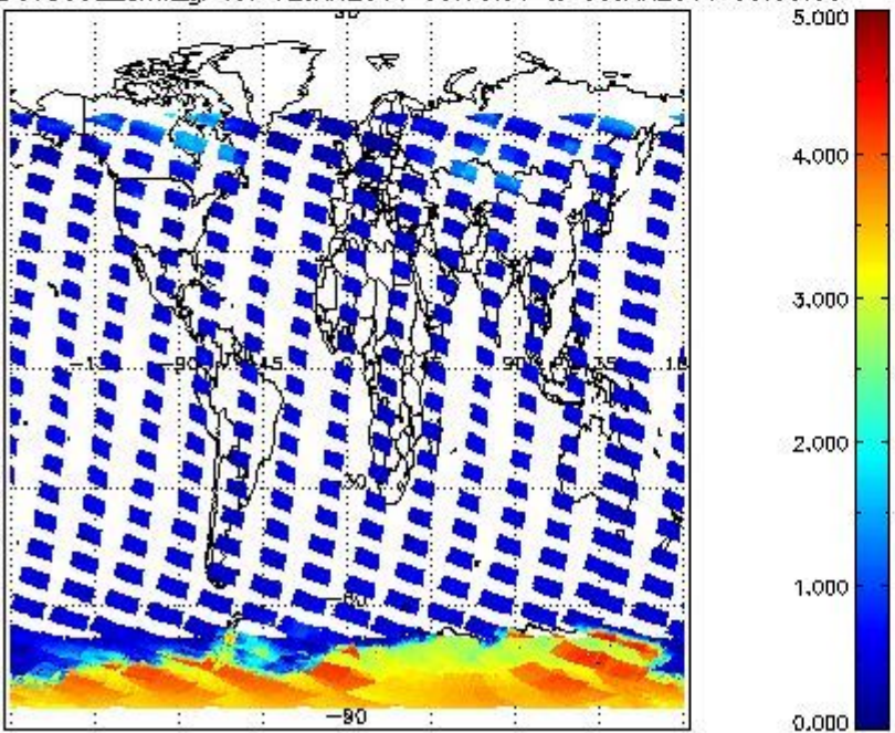
SCIOL2P_NADUV5S02_amf_gr for 02JAN2011 00:00:00 to 03JAN2011 00:00:00
