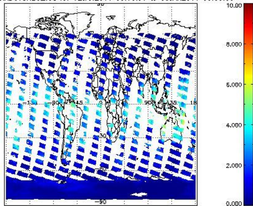
SCIOL2P_NADUV8H2O_vcd for 02JAN2011 00:00:00 to 03JAN2011 00:00:00
