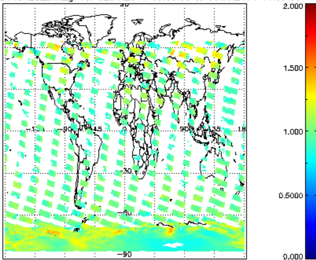
SCIOL2P_NADUV8H20_amf_gr for 02JAN2011 00:00:00 to 03JAN2011 00:00:00
