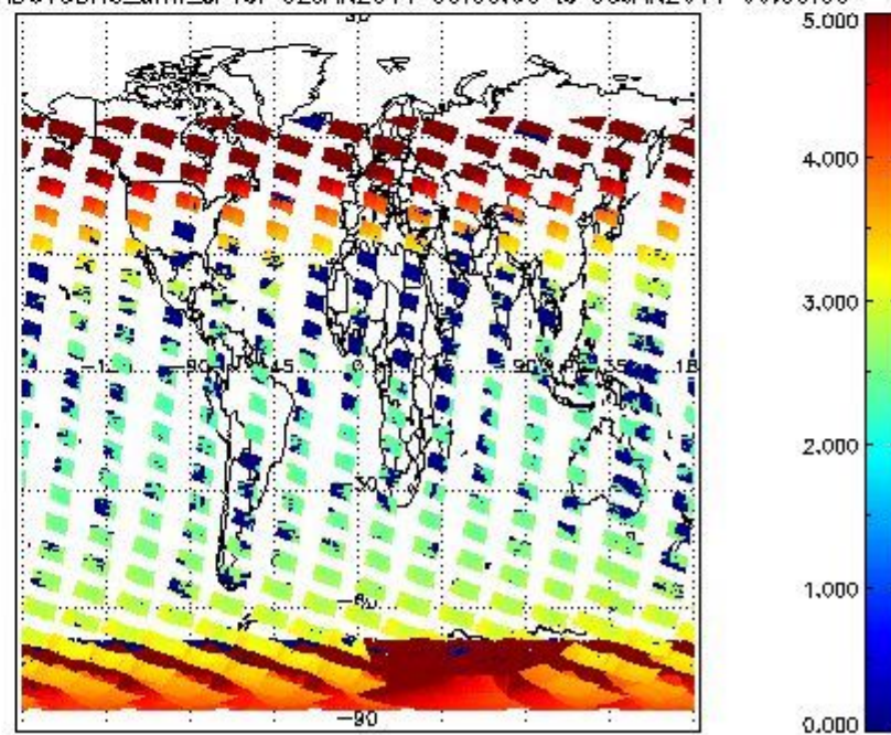
SCIOL2P_NADUV3BRO_amf_cl for 02JAN2011 00:00:00 to 03JAN2011 00:00:00
