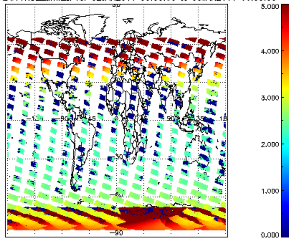
SCIOL2P_NADUV1NO2_amf_cl for 02JAN2011 00:00:00 to 03JAN2011 00:00:00
