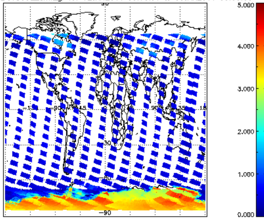
SCIOL2P_NADUV5S02_amf_gr for 02JAN2011 00:00:00 to 03JAN2011 00:00:00
