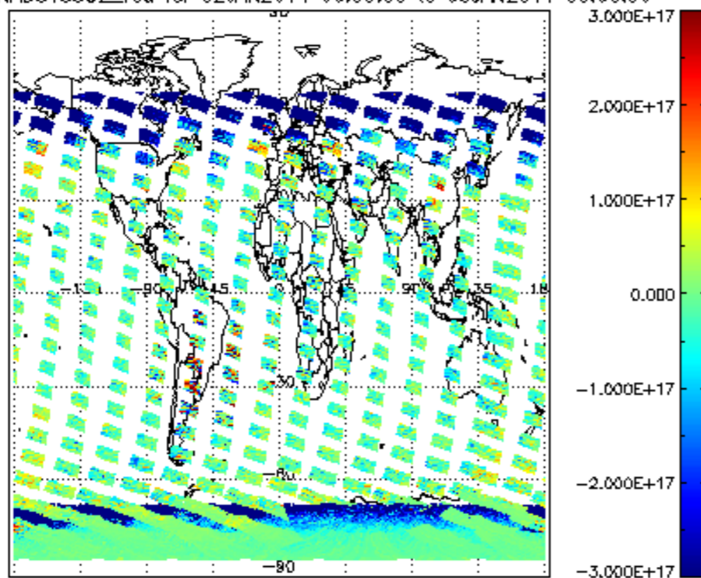
SCIOL2P_NADUV5S02_vcd for 02JAN2011 00:00:00 to 03JAN2011 00:00:00
