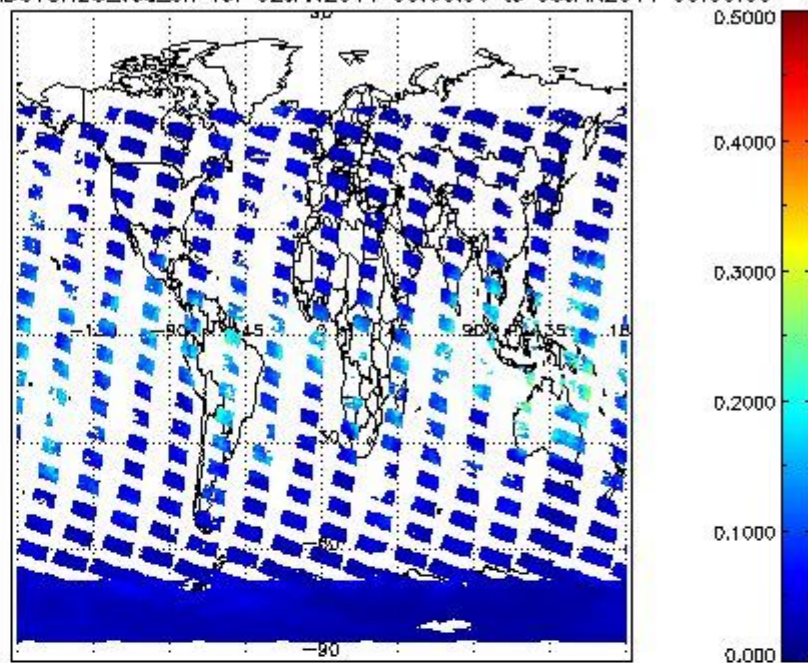
SCIOL2P_NADUV8H2O_vcd_err for 02JAN2011 00:00:00 to 03JAN2011 00:00:00
