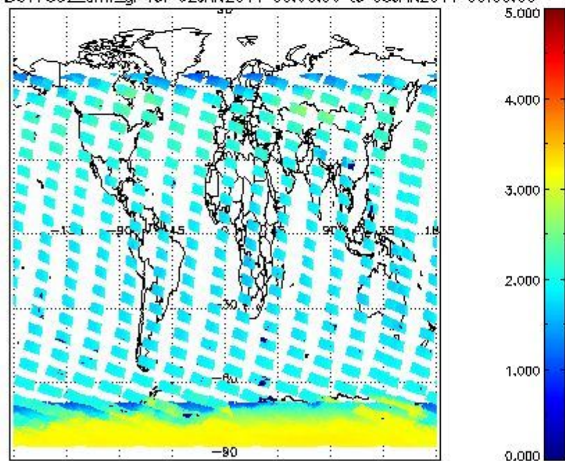
SCIOL2P_NADUV7S02_amf_gr for 02JAN2011 00:00:00 to 03JAN2011 00:00:00
