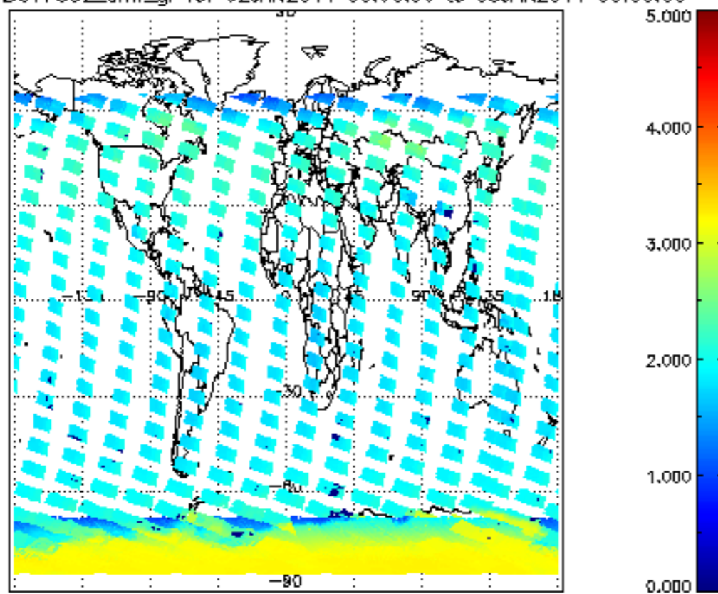
SCIOL2P_NADUV7S02_amf_gr for 02JAN2011 00:00:00 to 03JAN2011 00:00:00
