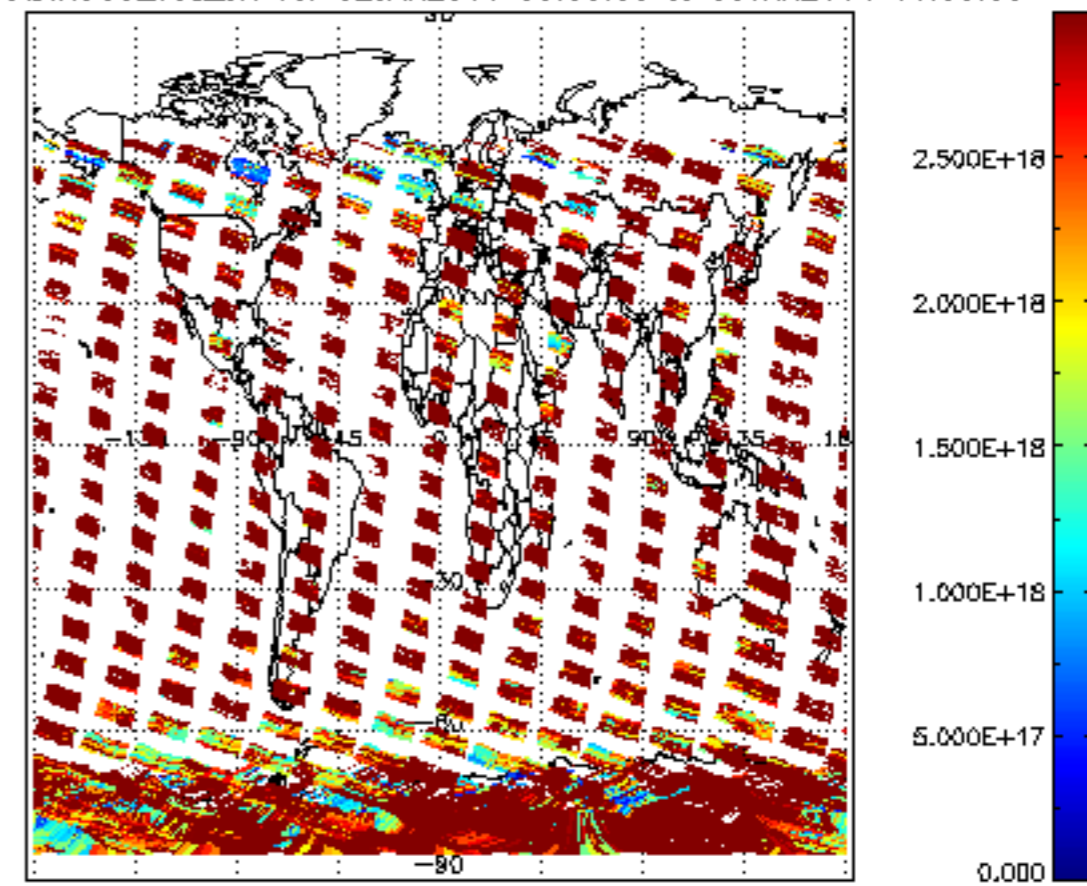
SCIOL2P_NADIR3CO_vcd_err for 02JAN2011 00:00:00 to 03JAN2011 00:00:00
