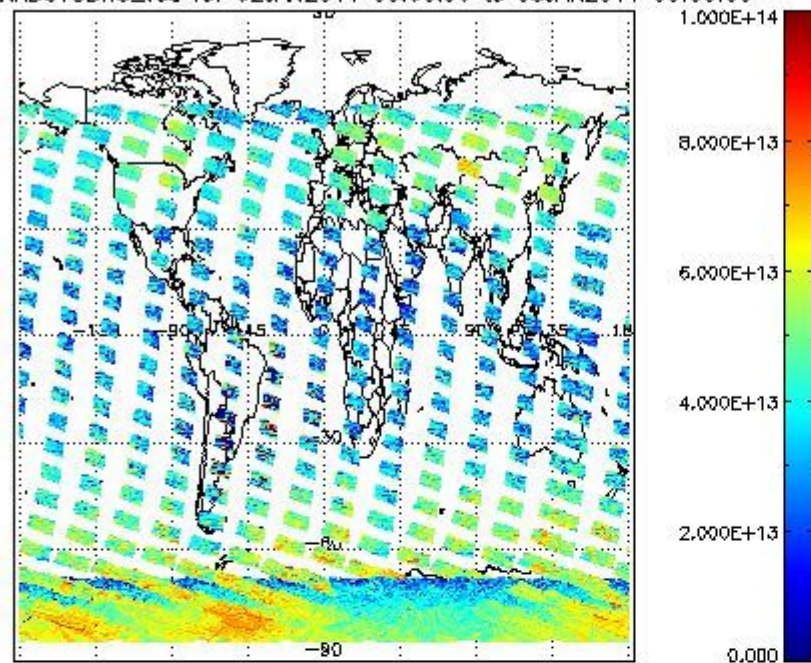
SCIOL2P_NADUV3BRO_vcd for 02JAN2011 00:00:00 to 03JAN2011 00:00:00
