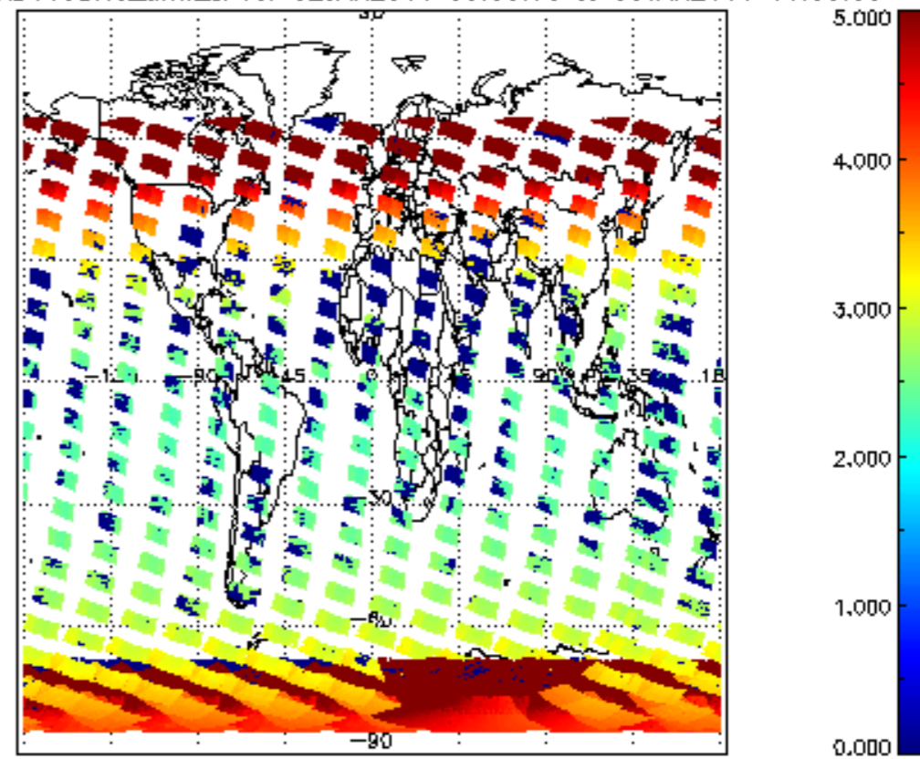
SCIOL2P_NADUV3BRO_amf_cl for 02JAN2011 00:00:00 to 03JAN2011 00:00:00
