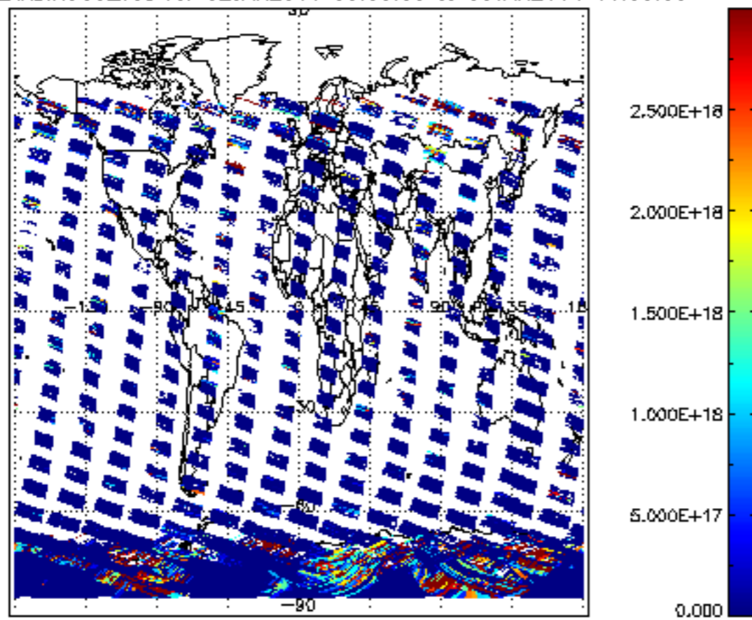
SCIOL2P_NADIR3CO_vcd for 02JAN2011 00:00:00 to 03JAN2011 00:00:00
