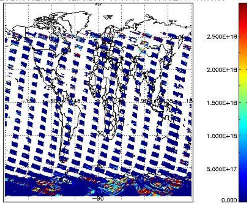
SCIDL2P_NADIR3CO_vcd for 02JAN2011 00:00:00 to 03JAN2011 00:00:00
