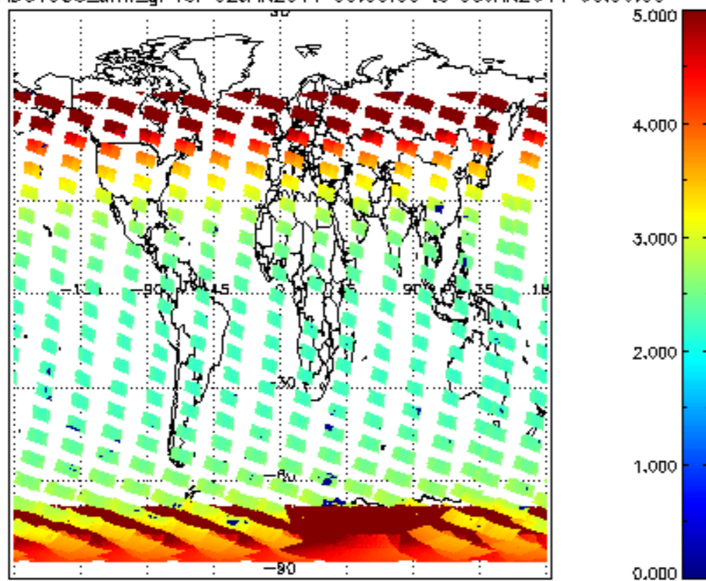
SCIOL2P_NADUV003_amf_gr for 02JAN2011 00:00:00 to 03JAN2011 00:00:00
