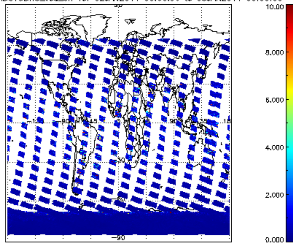
SCIOL2P_NADUV3BRO_vcd_err for 02JAN2011 00:00:00 to 03JAN2011 00:00:00
