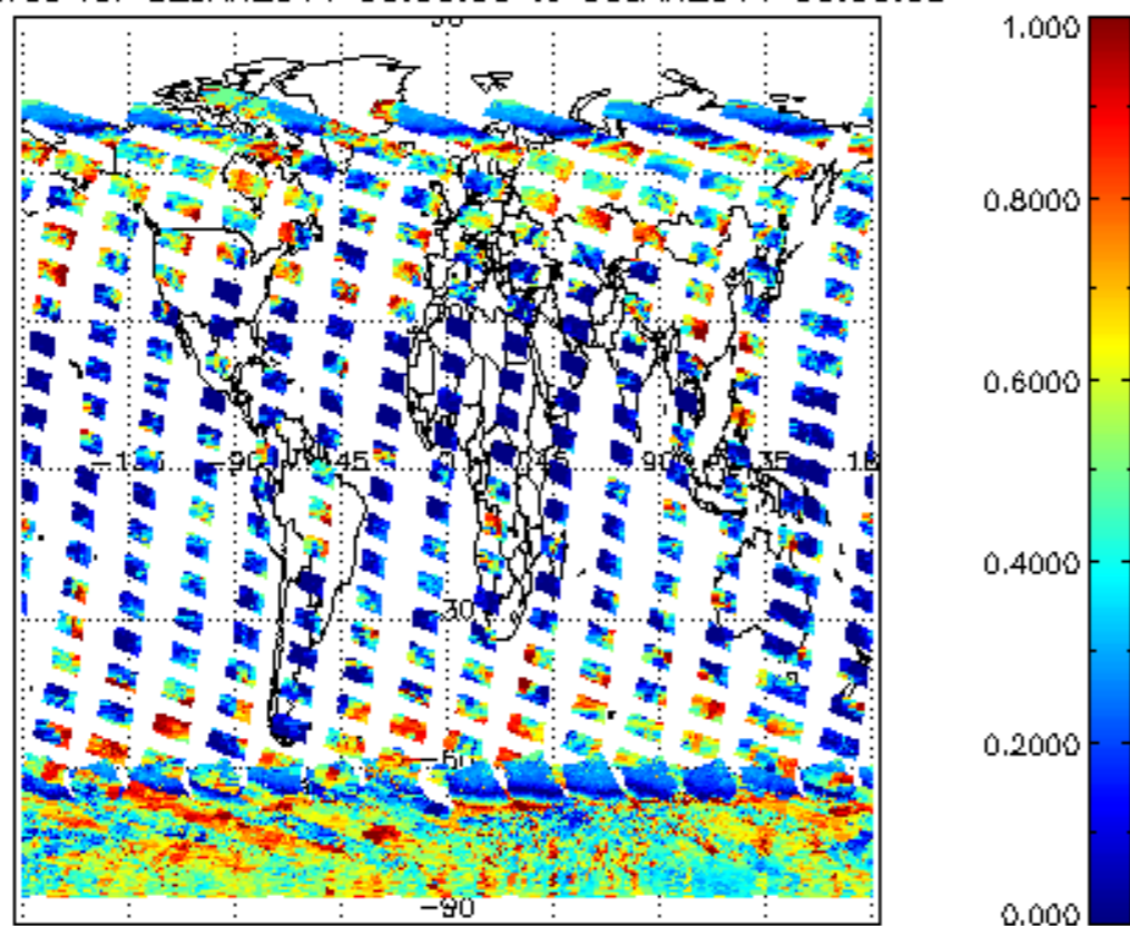
cL_frac for 02JAN2011 00:00:00 to 03JAN2011 00:00:00
