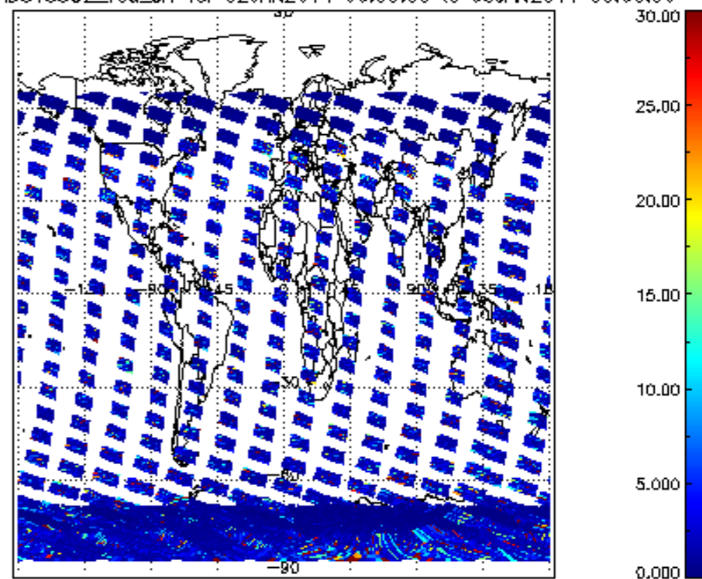
SCIOL2P_NADUV5S02_vcd_err for 02JAN2011 00:00:00 to 03JAN2011 00:00:00
