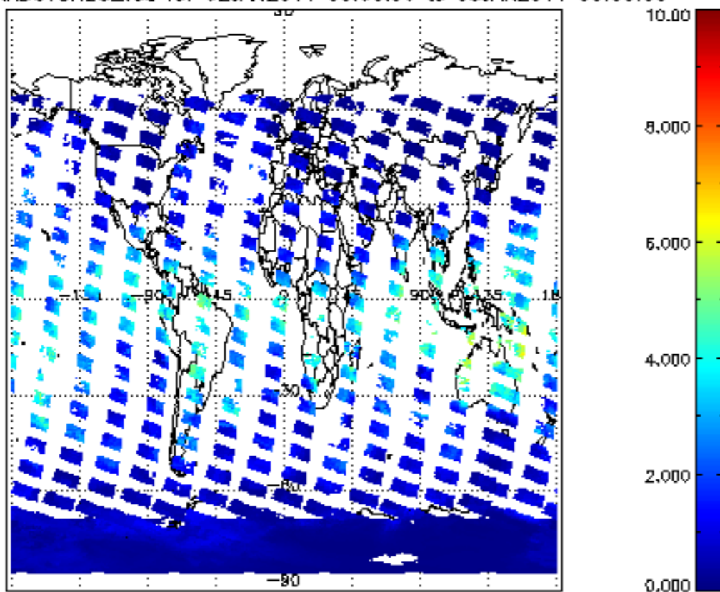
SCIOL2P_NADUV8H20_vcd for 02JAN2011 00:00:00 to 03JAN2011 00:00:00
