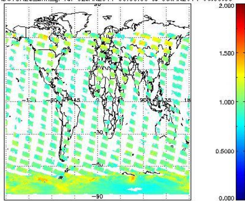
SCIOL2P_NADUV8H2O_amf_gr for 02JAN2011 00:00:00 to 03JAN2011 00:00:00
