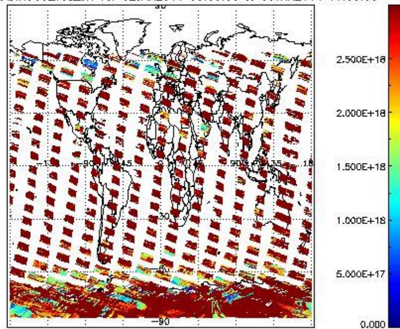
SCIDL2P_NADIR3CO_vcd_err for 02JAN2011 00:00:00 to 03JAN2011 00:00:00
