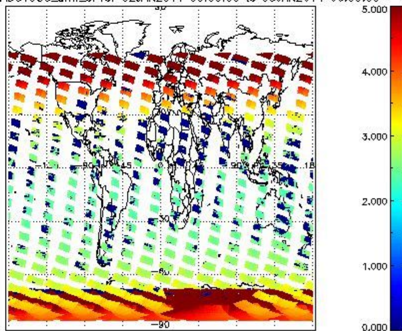
SCIOL2P_NADUV003_amf_cl for 02JAN2011 00:00:00 to 03JAN2011 00:00:00
