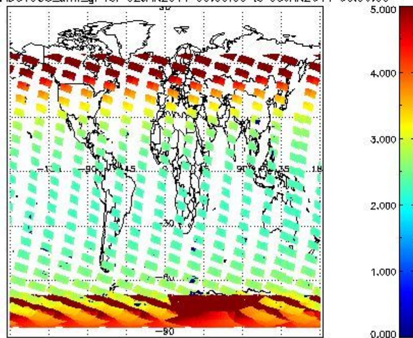
SCIOL2P_NADUV003_amf_gr for 02JAN2011 00:00:00 to 03JAN2011 00:00:00
