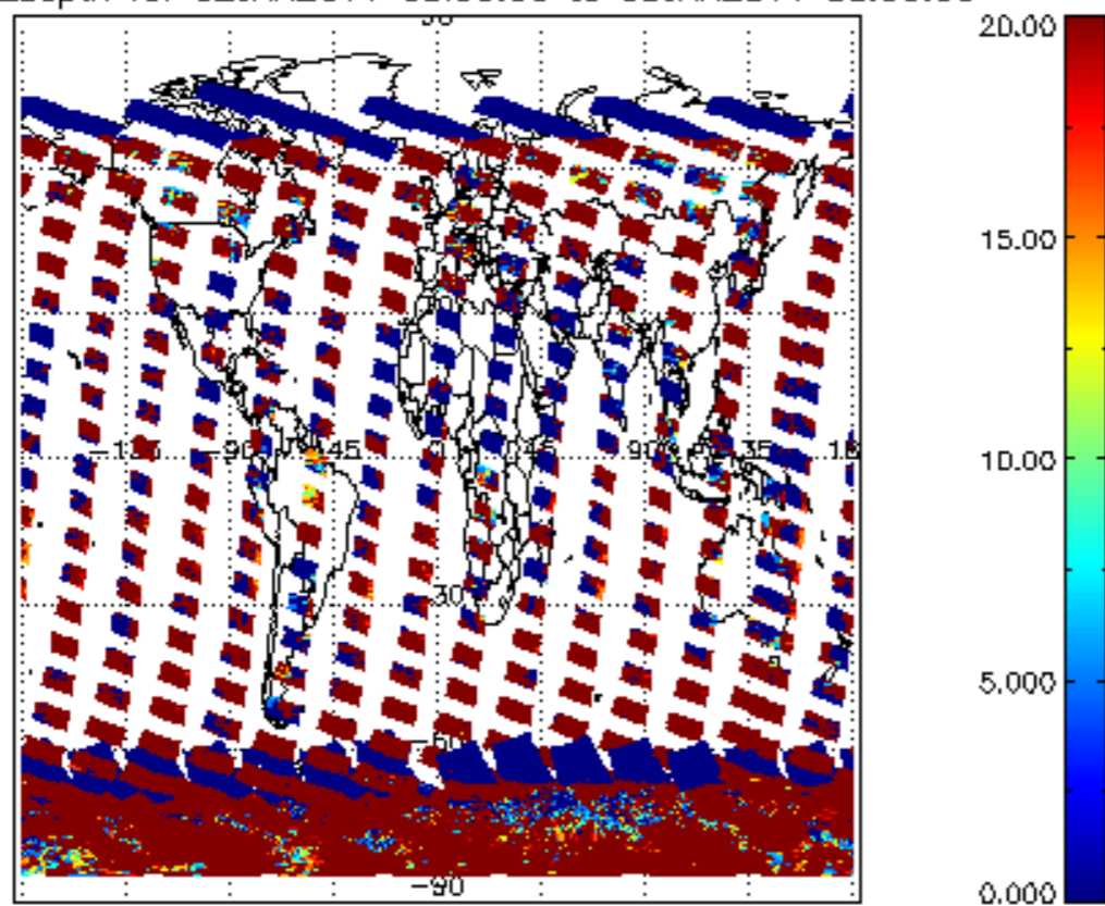
cLopt_depth for 02JAN2011 00:00:00 to 03JAN2011 00:00:00
