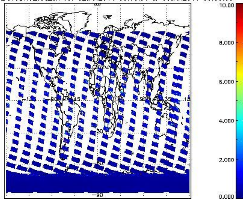
SCIOL2P_NADUV3BRO_vcd_err for 02JAN2011 00:00:00 to 03JAN2011 00:00:00
