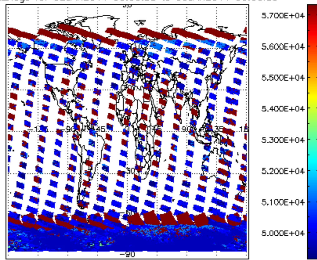
cloud_flags for 02JAN2011 00:00:00 to 03JAN2011 00:00:00
