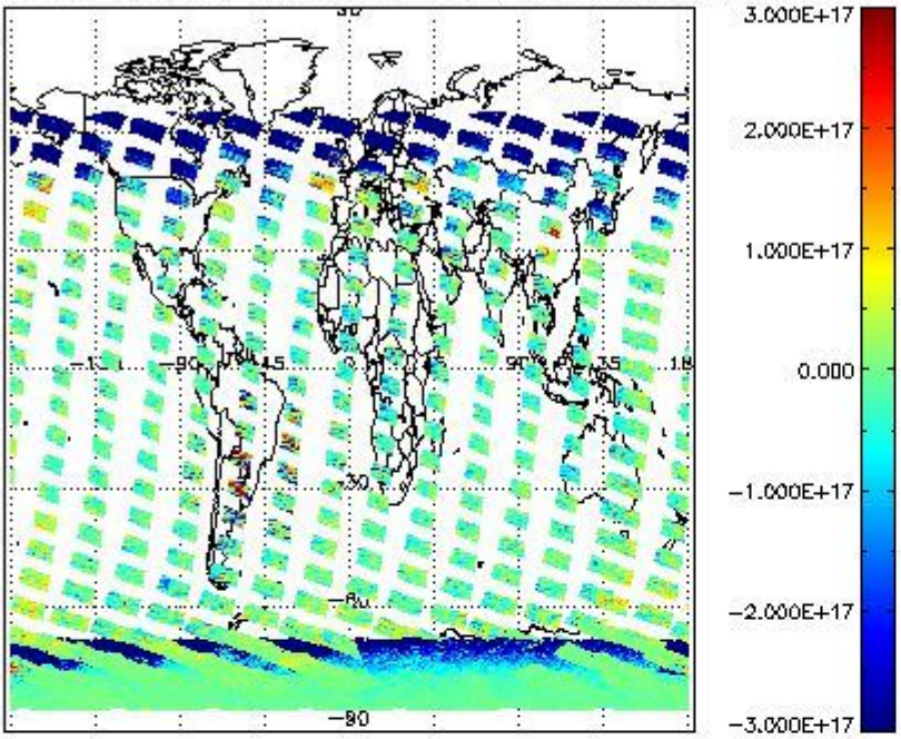
SCIOL2P_NADUV5S02_vcd for 02JAN2011 00:00:00 to 03JAN2011 00:00:00
