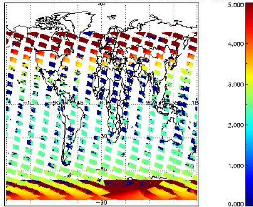
SCIOL2P_NADUV1NO2_amf_cl for 02JAN2011 00:00:00 to 03JAN2011 00:00:00
