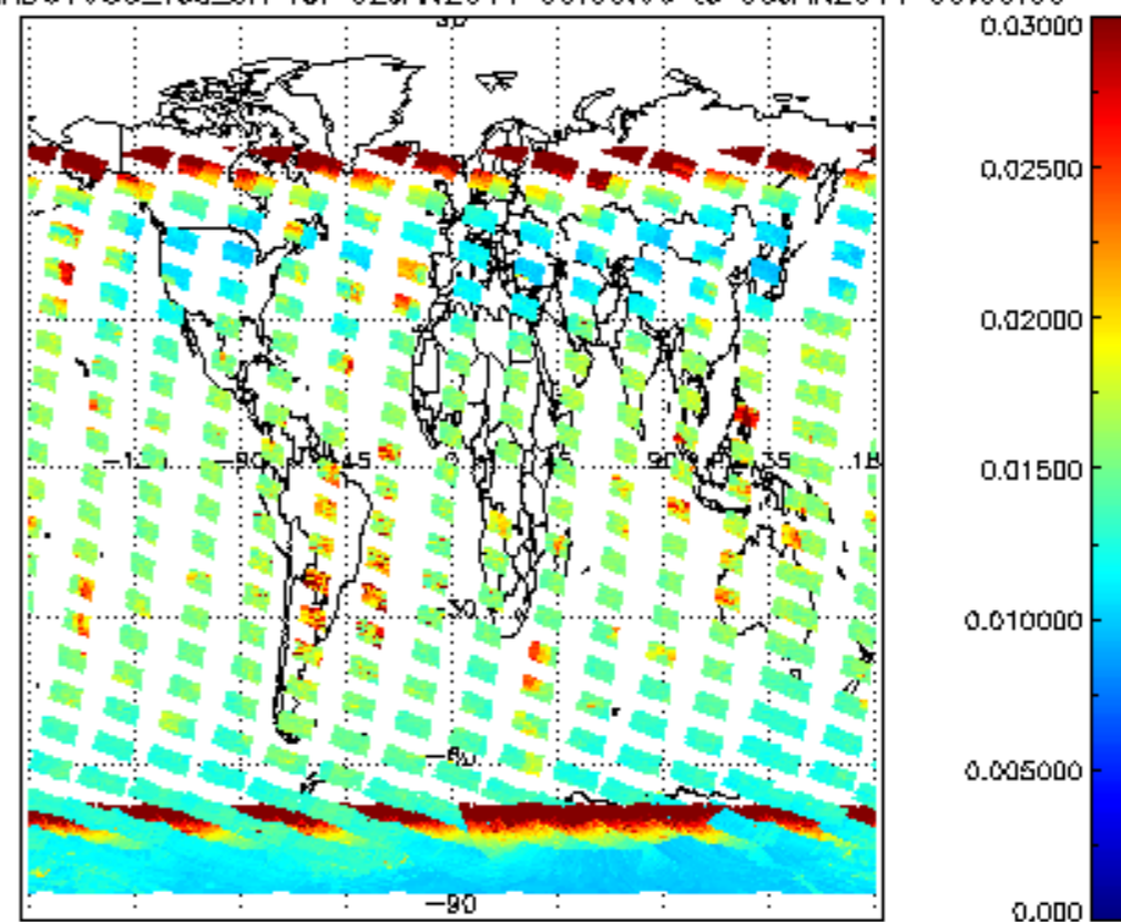
SCIOL2P_NADUV003_vcd_err for 02JAN2011 00:00:00 to 03JAN2011 00:00:00
