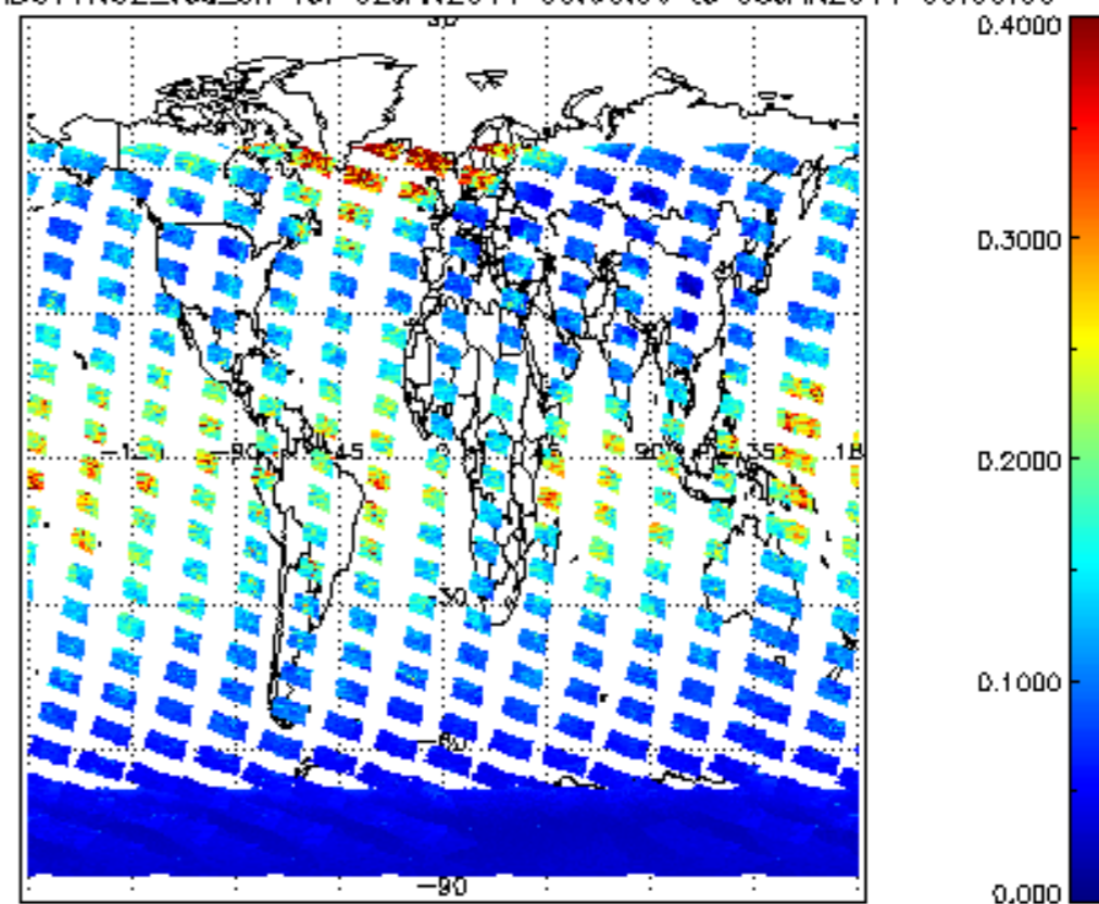
SCIOL2P_NADUV1NO2_vcd_err for 02JAN2011 00:00:00 to 03JAN2011 00:00:00
