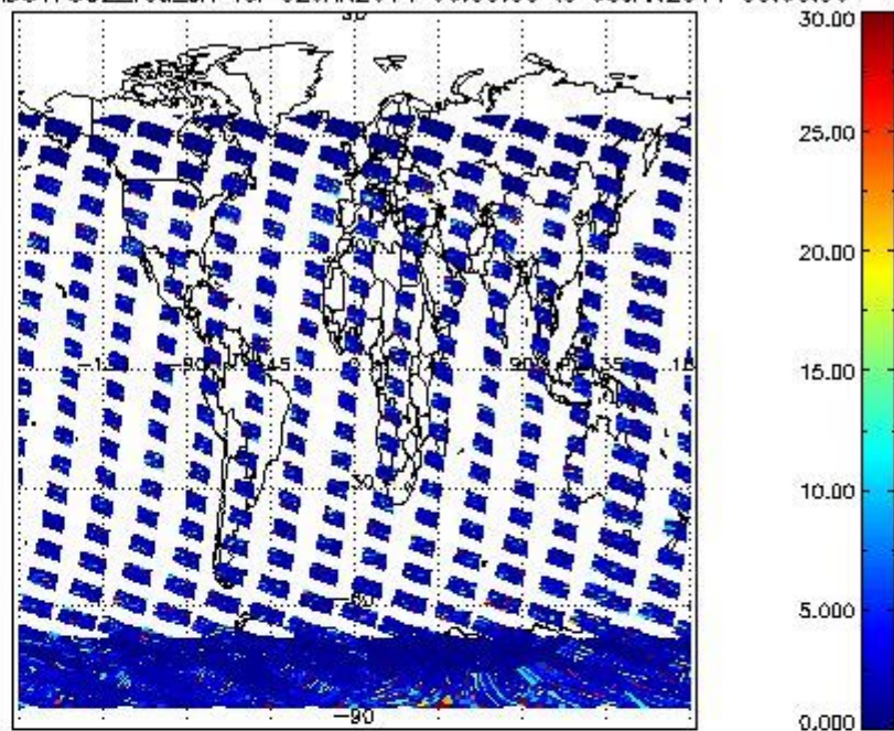
SCIOL2P_NADUV7S02_vcd_err for 02JAN2011 00:00:00 to 03JAN2011 00:00:00
