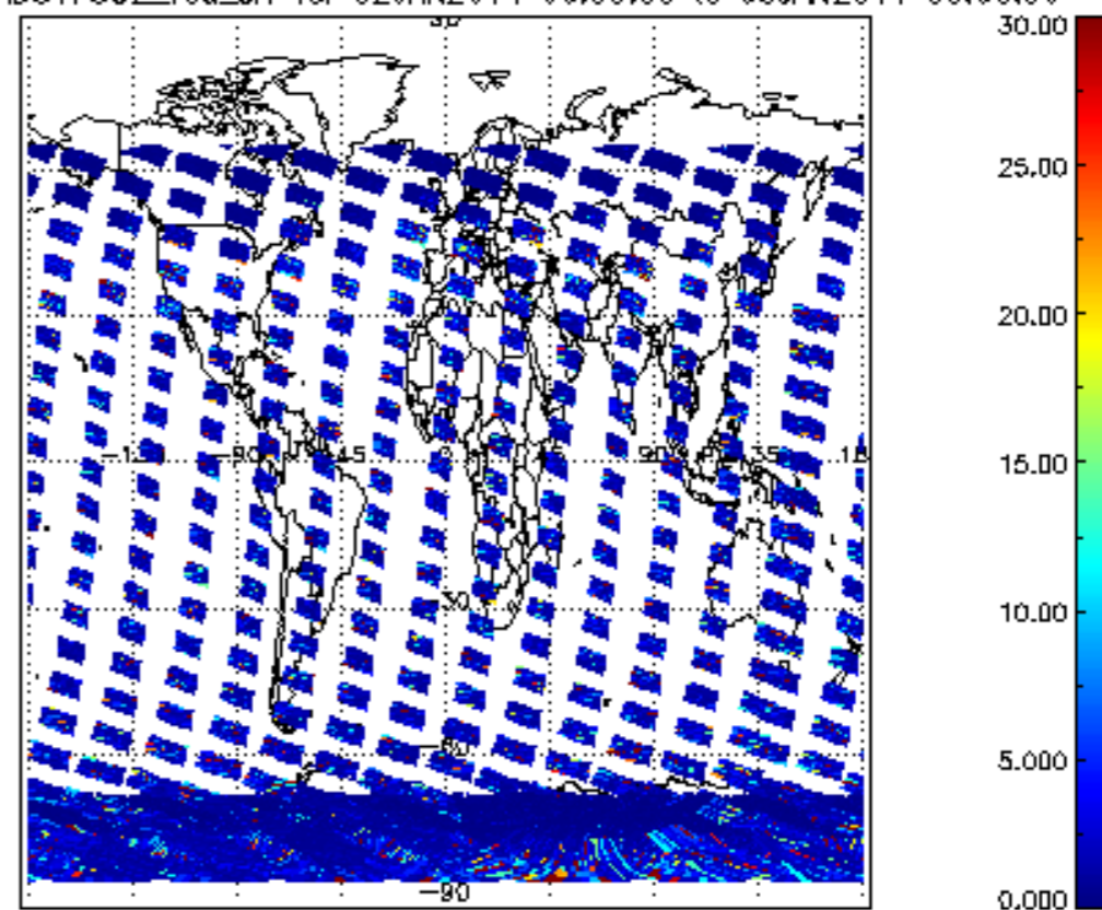
SCIOL2P_NADUV7S02_vcd_err for 02JAN2011 00:00:00 to 03JAN2011 00:00:00
