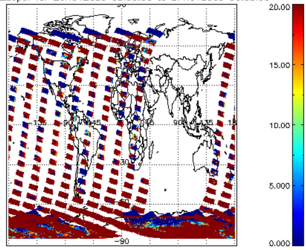
cL_opt_depth for 26NOV2009 00:00:00 to 27NOV2009 00:00:00
