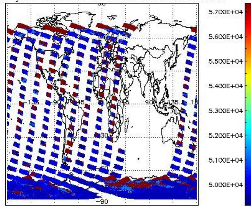
cloud_flags for 26NOV2009 00:00:00 to 27NOV2009 00:00:00
