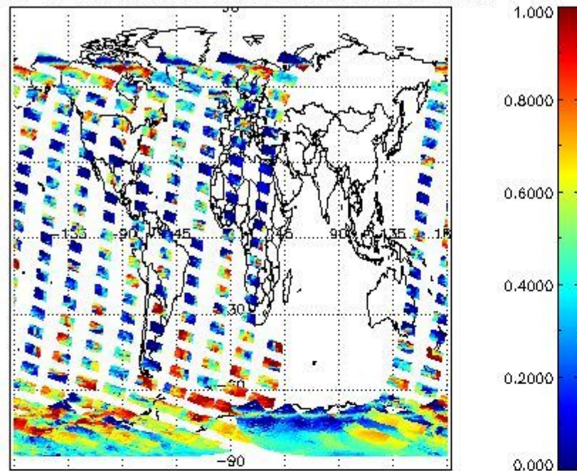
cLfrac for 26NOV2009 00:00:00 to 27NOV2009 00:00:00
