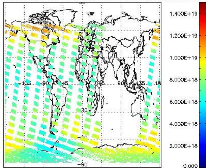
SCIOL2P_NADUV003_vcd for 26NOV2009 00:00:00 to 27NOV2009 00:00:00
