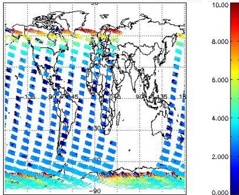
SCIOL2P_NADUV003_amf_cl for 26NOV2009 00:00:00 to 27NOV2009 00:00:00
