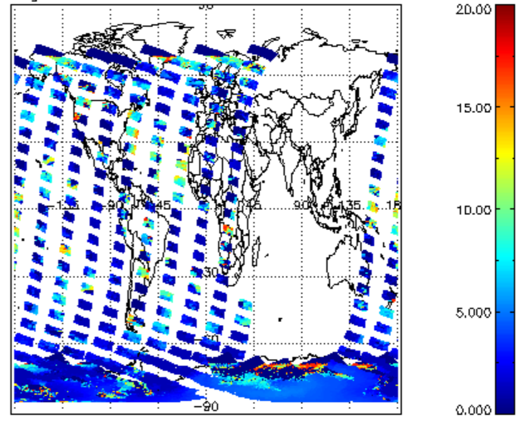
cL_top_height for 26NOV2009 00:00:00 to 27NOV2009 00:00:00
