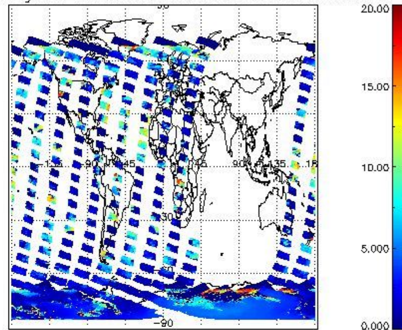
cL_top_height for 26NOV2009 00:00:00 to 27NOV2009 00:00:00
