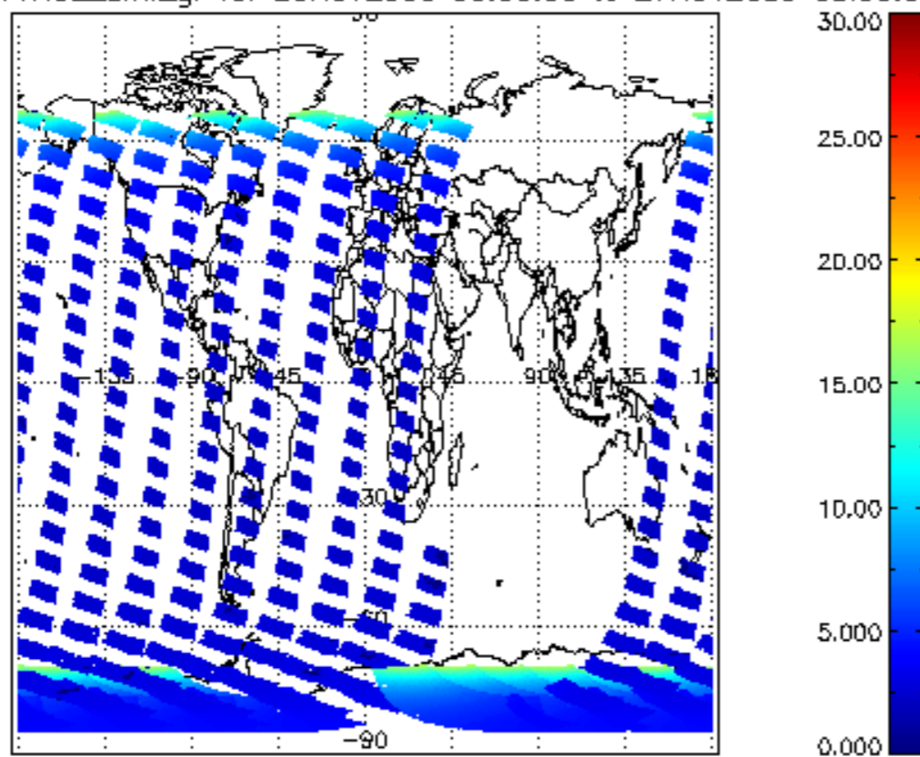
SCIOL2P_NADUV1NO2_amf_gr for 26NOV2009 00:00:00 to 27NOV2009 00:00:00
