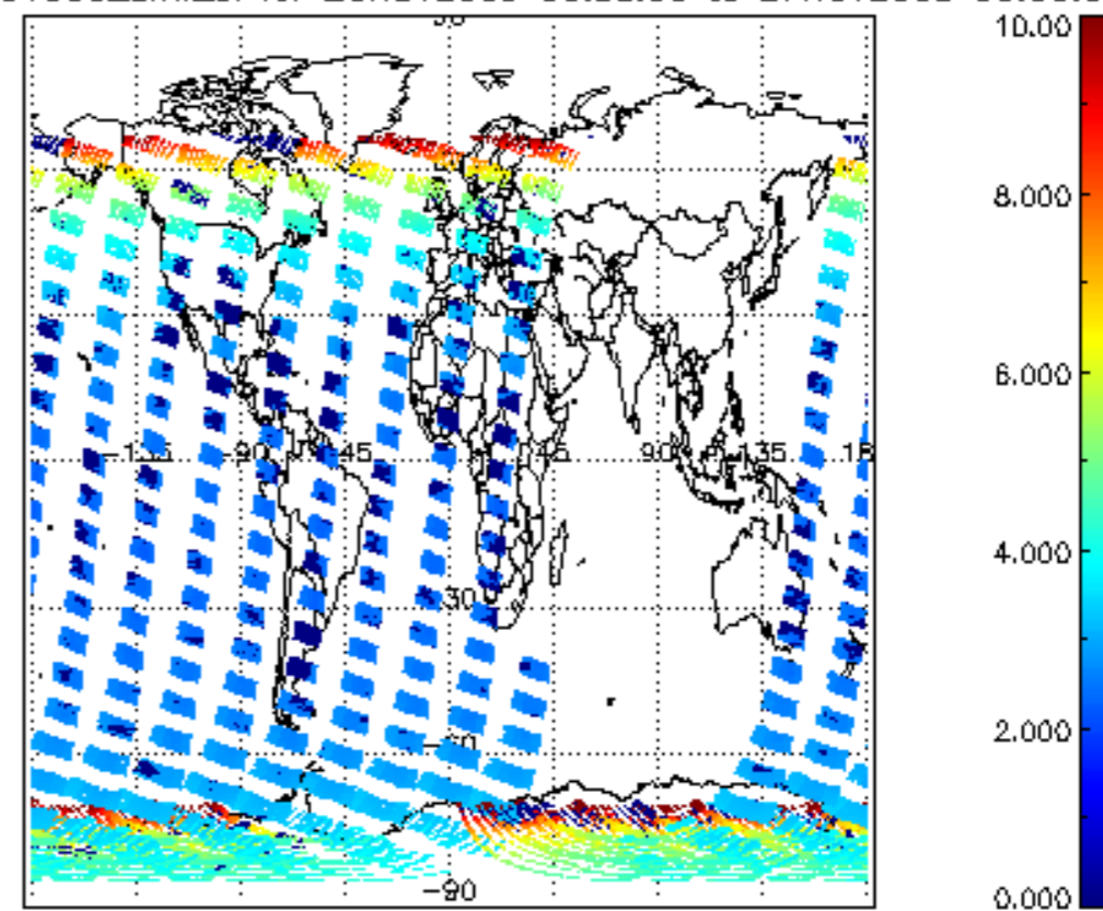
SCIOL2P_NADUV003_amf_cl for 26NOV2009 00:00:00 to 27NOV2009 00:00:00
