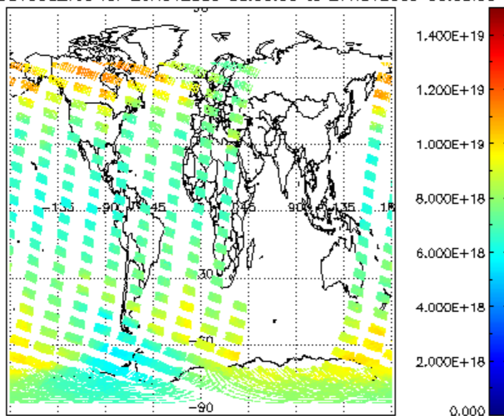
SCIOL2P_NADUV003_vcd for 26NOV2009 00:00:00 to 27NOV2009 00:00:00
