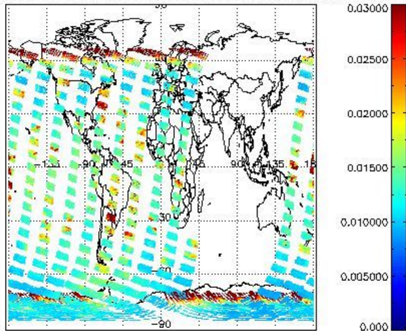
SCIOL2P_NADUV003_vcd_err for 26NOV2009 00:00:00 to 27NOV2009 00:00:00
