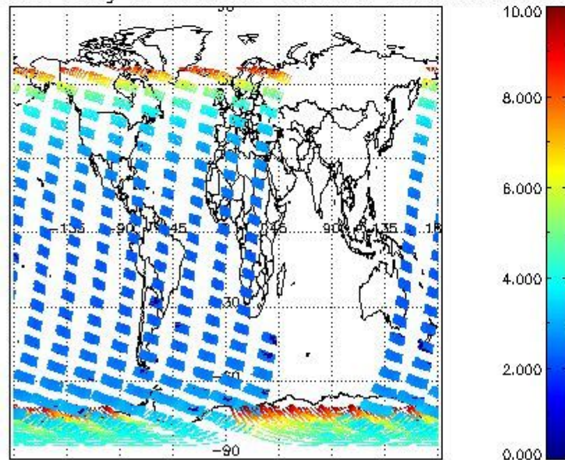
SCIOL2P_NADUV003_amf_gr for 26NOV2009 00:00:00 to 27NOV2009 00:00:00
