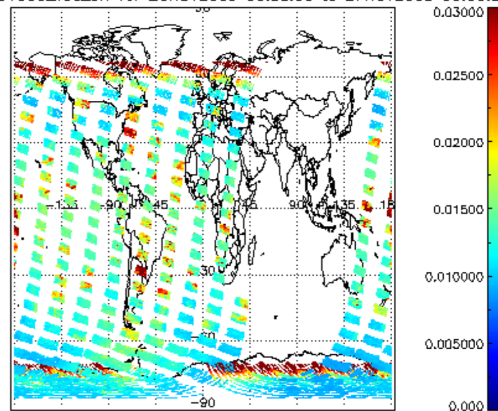
SCIOL2P_NADUV003_vcd_err for 26NOV2009 00:00:00 to 27NOV2009 00:00:00
