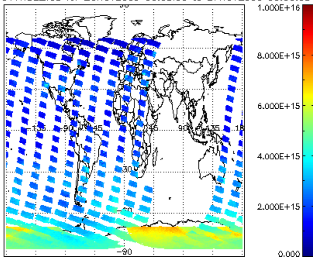
SCIOL2P_NADUV1NO2_vcd for 26NOV2009 00:00:00 to 27NOV2009 00:00:00
