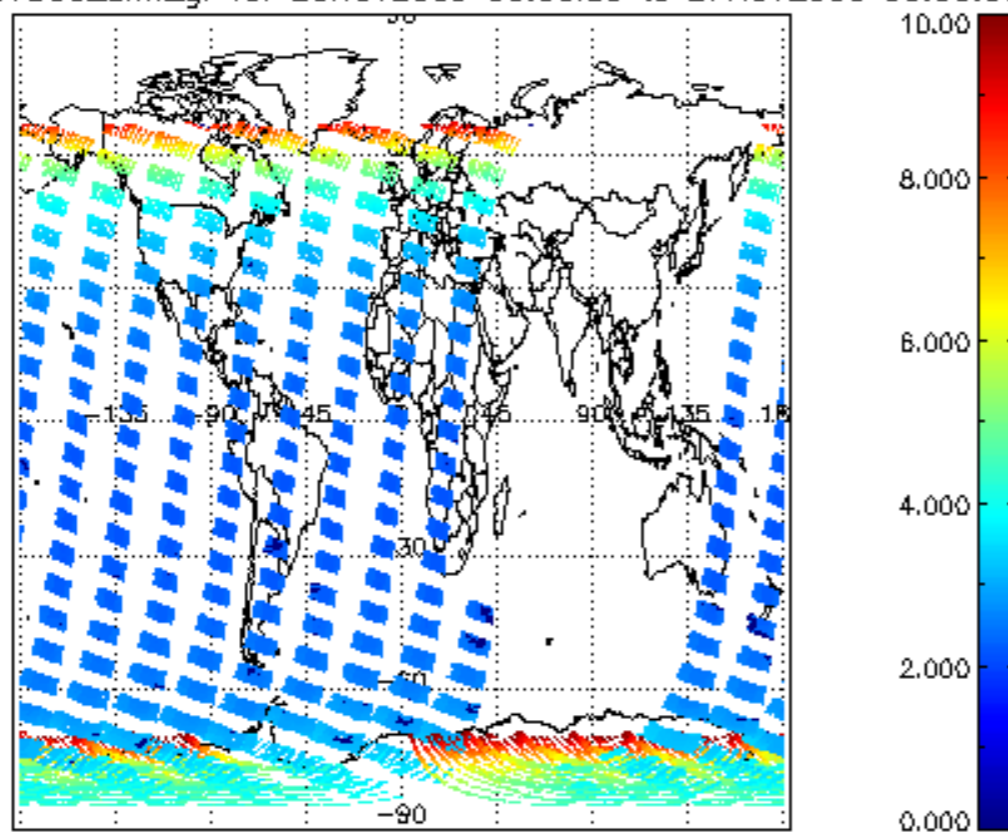
SCIOL2P_NADUV003_amf_gr for 26NOV2009 00:00:00 to 27NOV2009 00:00:00
