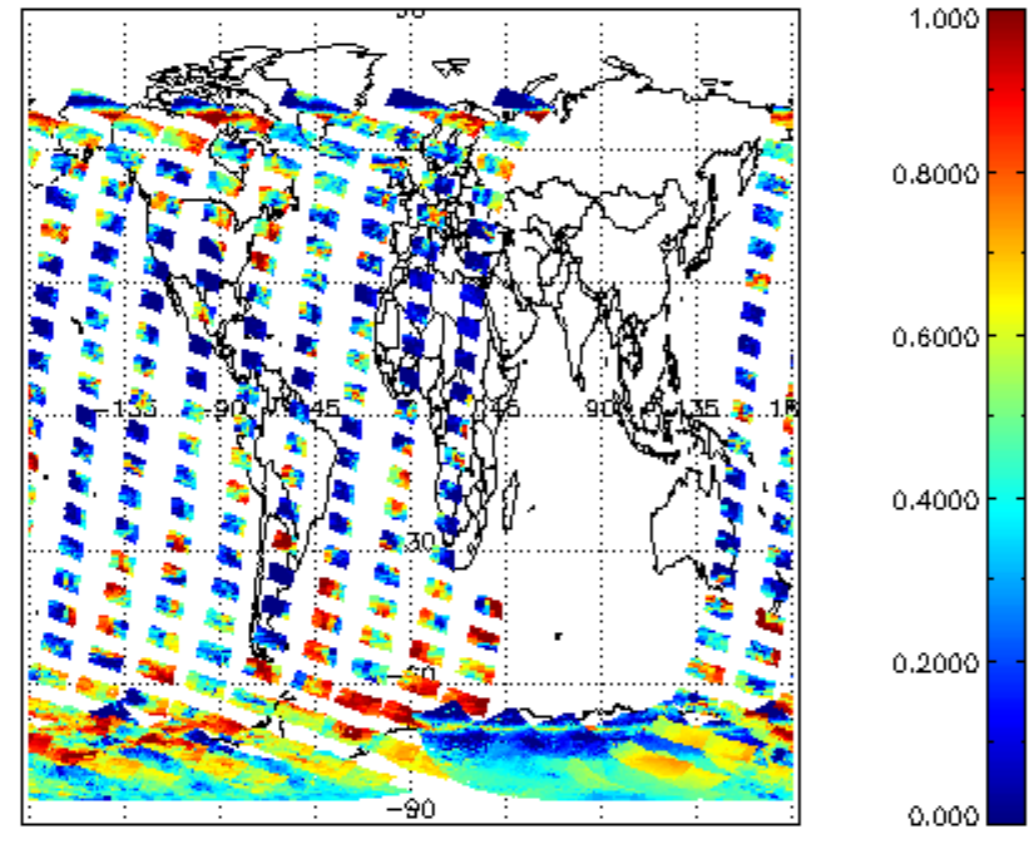
cLfrac for 26NOV2009 00:00:00 to 27NOV2009 00:00:00
