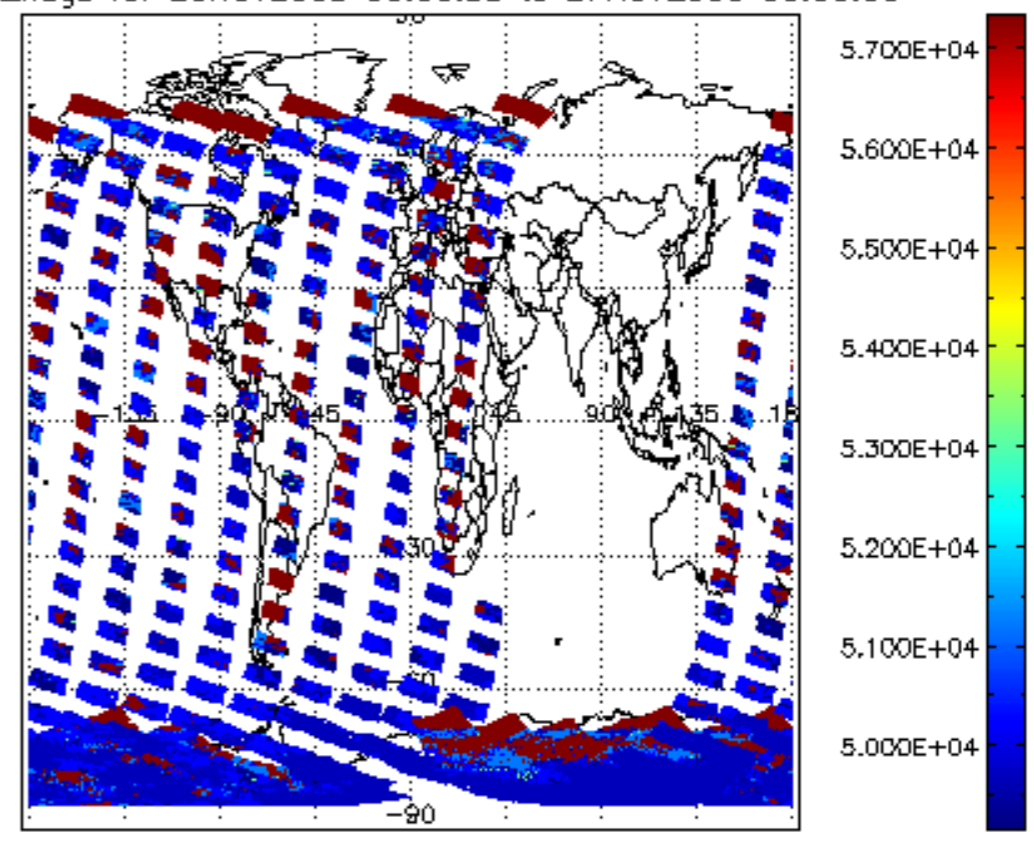
cloud_flags for 26NOV2009 00:00:00 to 27NOV2009 00:00:00
