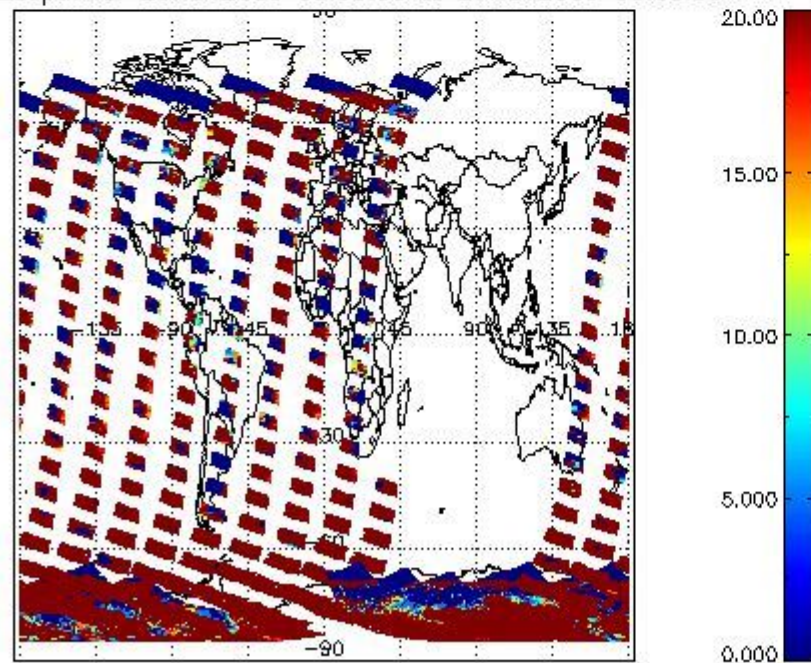
cLopt_depth for 26NOV2009 00:00:00 to 27NOV2009 00:00:00
