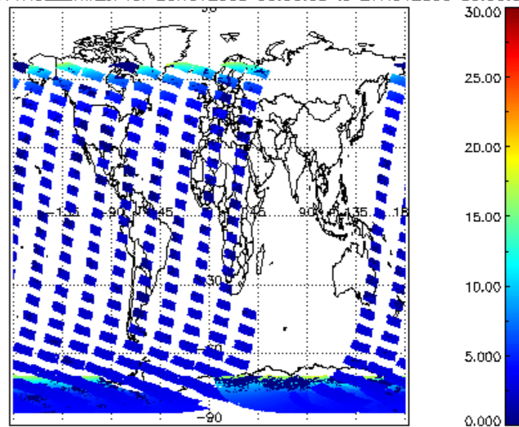
SCIOL2P_NADUV1NO2_amf_cl for 26NOV2009 00:00:00 to 27NOV2009 00:00:00
