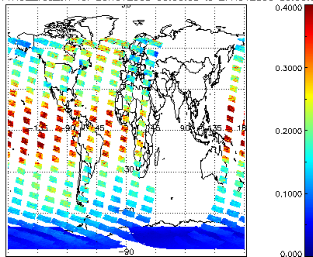
SCIOL2P_NADUV1NO2_vcd_err for 26NOV2009 00:00:00 to 27NOV2009 00:00:00
