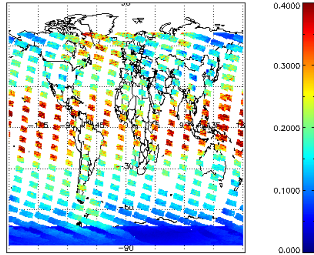
SCIOL2P_NADUV1NO2_vcd_err for 16NOV2009 00:00:00 to 17NOV2009 00:00:00
