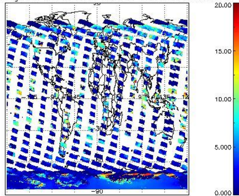
cL_top_height for 16NOV2009 00:00:00 to 17NOV2009 00:00:00
