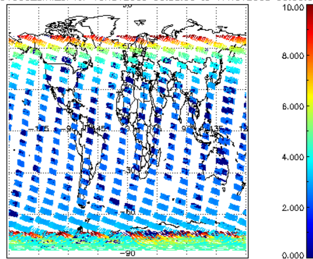
SCIOL2P_NADUV003_amf_cl for 16NOV2009 00:00:00 to 17NOV2009 00:00:00
