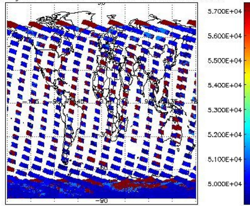
cloud_flags for 16NOV2009 00:00:00 to 17NOV2009 00:00:00
