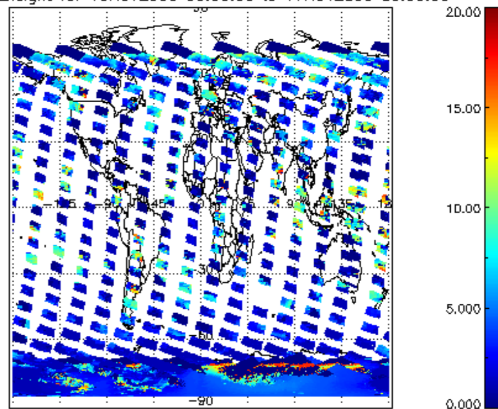
cL_top_height for 16NOV2009 00:00:00 to 17NOV2009 00:00:00
