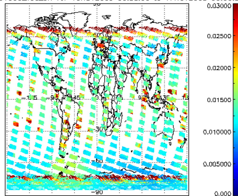
SCIOL2P_NADUV003_vcd_err for 16NOV2009 00:00:00 to 17NOV2009 00:00:00
