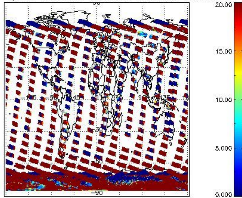
cLopt_depth for 16NOV2009 00:00:00 to 17NOV2009 00:00:00
