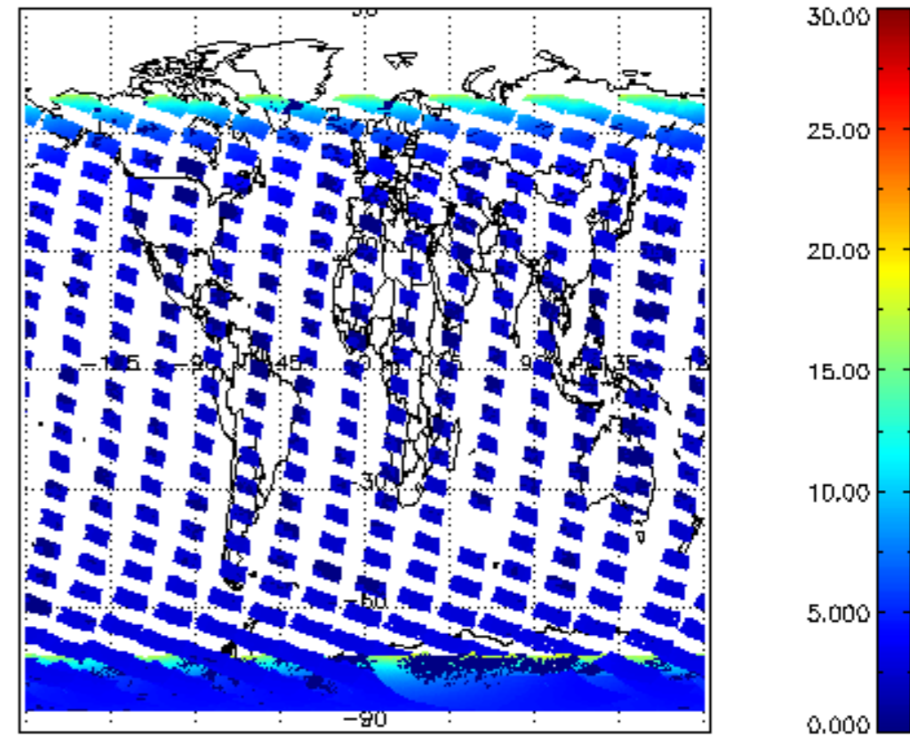
SCIOL2P_NADUV1NO2_amf_cl for 16NOV2009 00:00:00 to 17NOV2009 00:00:00
