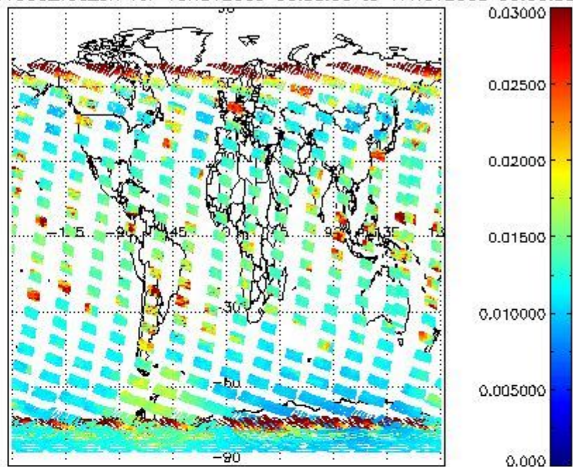
SCIOL2P_NADUV003_vcd_err for 16NOV2009 00:00:00 to 17NOV2009 00:00:00
