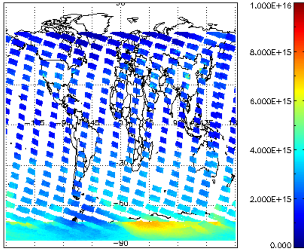
SCIOL2P_NADUV1NO2_vcd for 16NOV2009 00:00:00 to 17NOV2009 00:00:00
