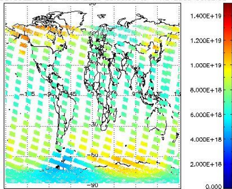
SCIOL2P_NADUV003_vcd for 16NOV2009 00:00:00 to 17NOV2009 00:00:00
