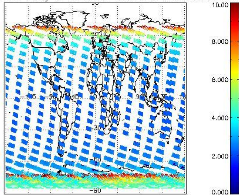
SCIOL2P_NADUV003_amf_gr for 16NOV2009 00:00:00 to 17NOV2009 00:00:00
