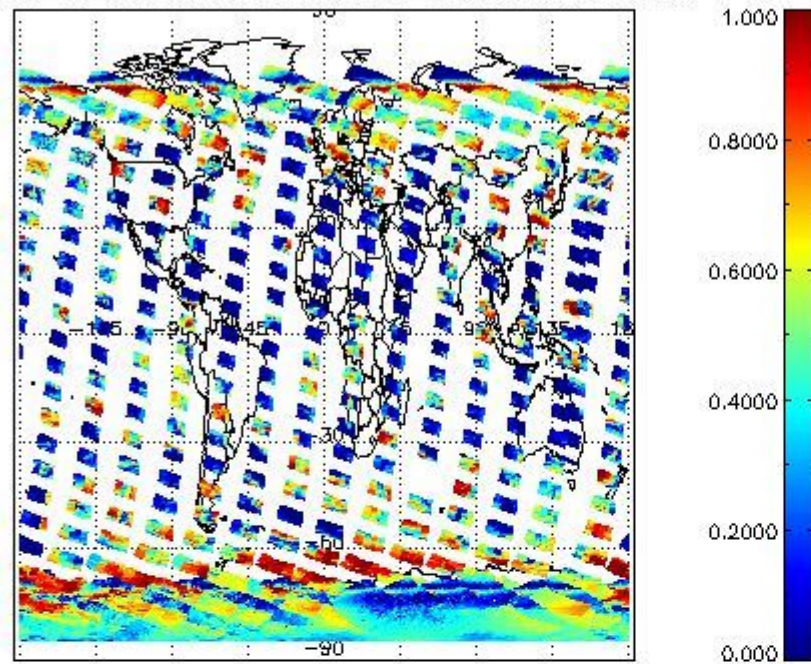
cLfrac for 16NOV2009 00:00:00 to 17NOV2009 00:00:00
