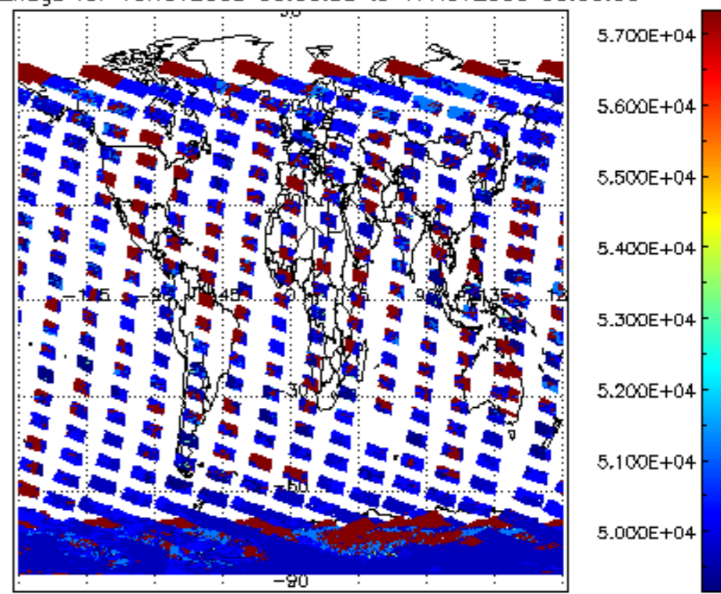
cloud_flags for 16NOV2009 00:00:00 to 17NOV2009 00:00:00
