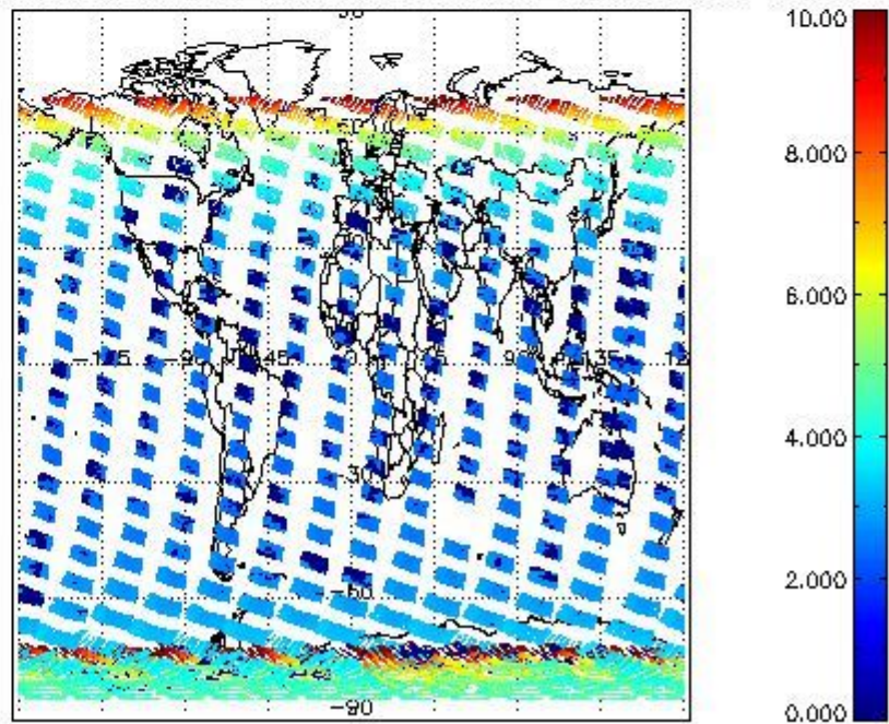
SCIOL2P_NADUV003_amf_cl for 16NOV2009 00:00:00 to 17NOV2009 00:00:00
