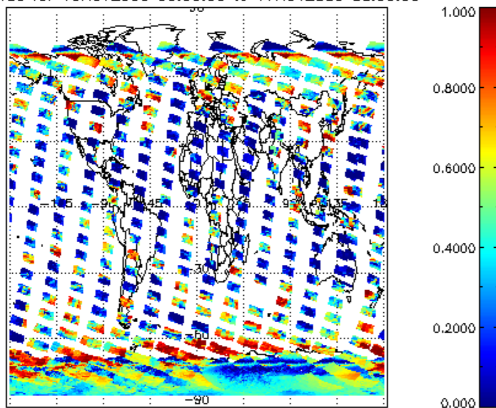
cLfrac for 16NOV2009 00:00:00 to 17NOV2009 00:00:00
