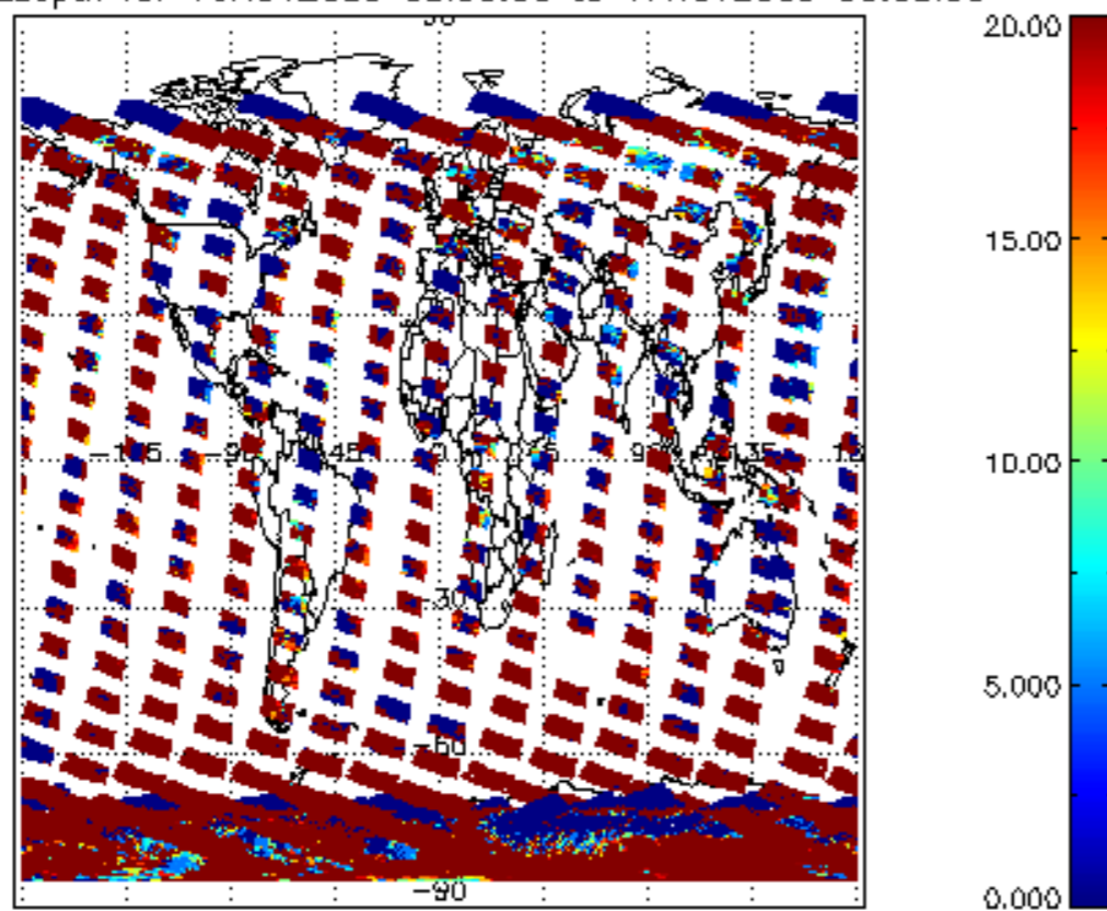
cL_opt_depth for 16NOV2009 00:00:00 to 17NOV2009 00:00:00
