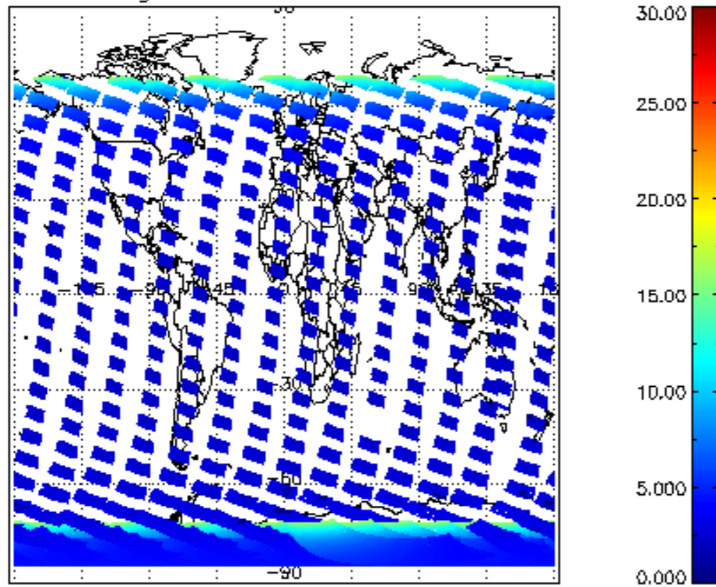
SCIOL2P_NADUV1NO2_amf_gr for 16NOV2009 00:00:00 to 17NOV2009 00:00:00
