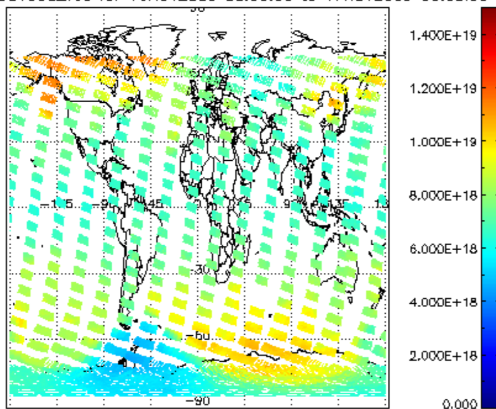
SCIOL2P_NADUV003_vcd for 16NOV2009 00:00:00 to 17NOV2009 00:00:00
