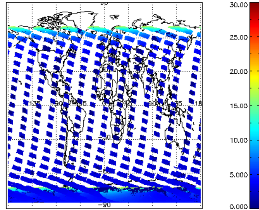
SCIOL2P_NADUV1NO2_amf_cl for 14NOV2009 00:00:00 to 15NOV2009 00:00:00
