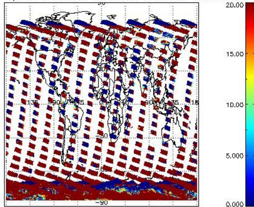
cLopt_depth for 14NOV2009 00:00:00 to 15NOV2009 00:00:00
