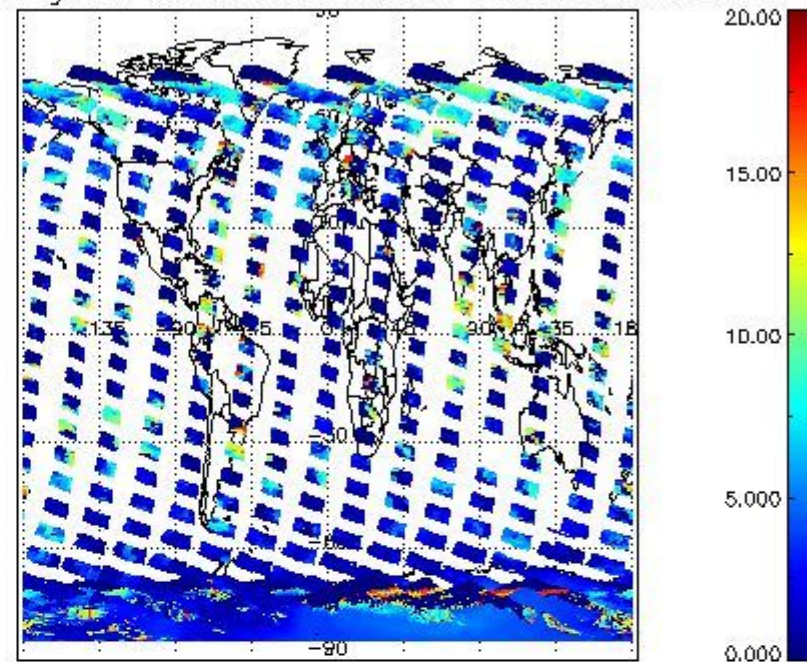
cL_top_height for 14NOV2009 00:00:00 to 15NOV2009 00:00:00
