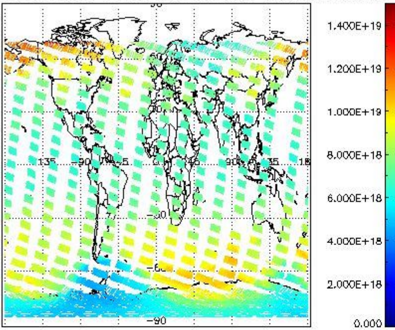
SCIOL2P_NADUV003_vcd for 14NOV2009 00:00:00 to 15NOV2009 00:00:00
