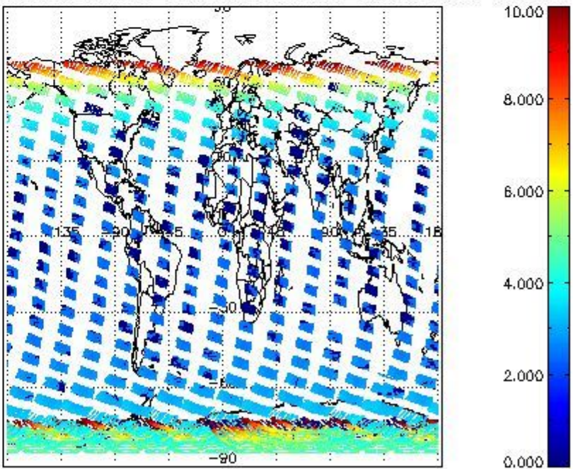
SCIOL2P_NADUV003_amf_cl for 14NOV2009 00:00:00 to 15NOV2009 00:00:00
