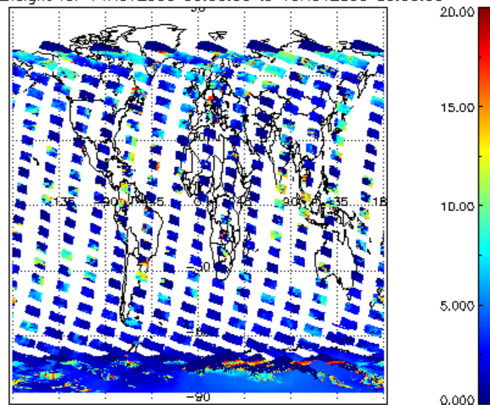
cL_top_height for 14NOV2009 00:00:00 to 15NOV2009 00:00:00
