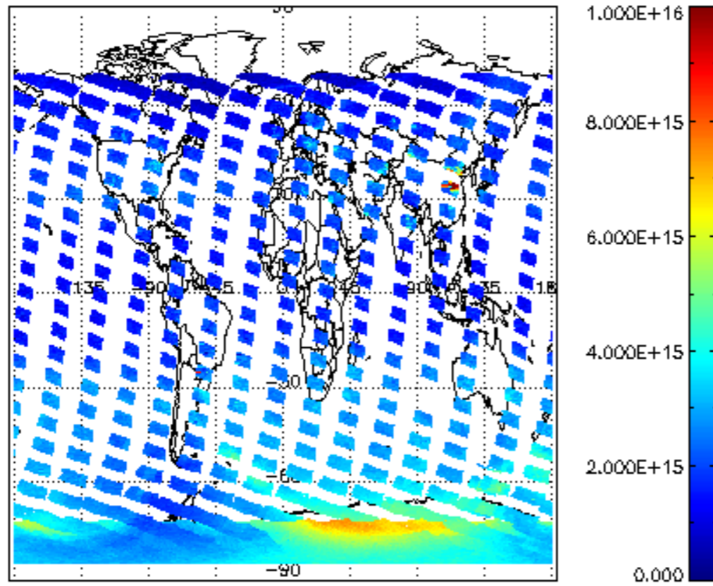
SCIOL2P_NADUV1NO2_vcd for 14NOV2009 00:00:00 to 15NOV2009 00:00:00
