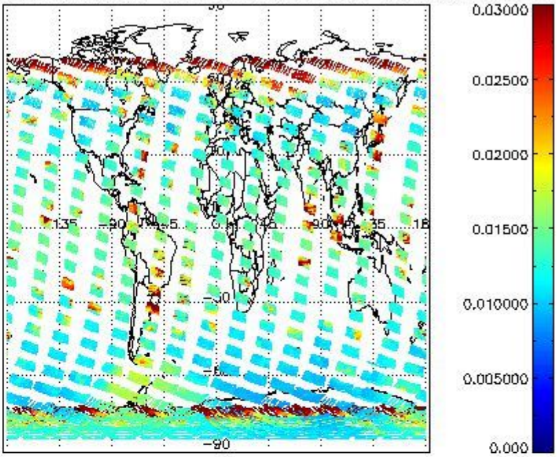
SCIOL2P_NADUV003_vcd_err for 14NOV2009 00:00:00 to 15NOV2009 00:00:00
