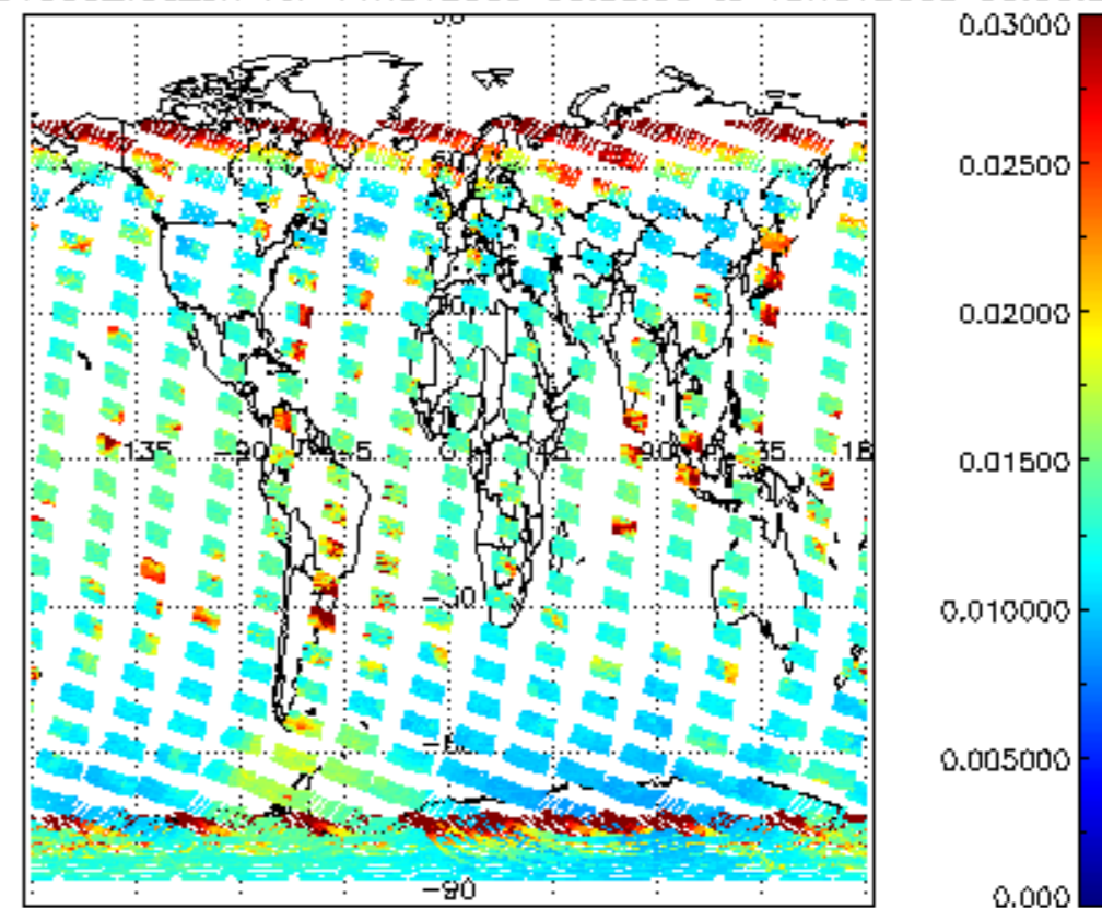
SCIOL2P_NADUV003_vcd_err for 14NOV2009 00:00:00 to 15NOV2009 00:00:00
