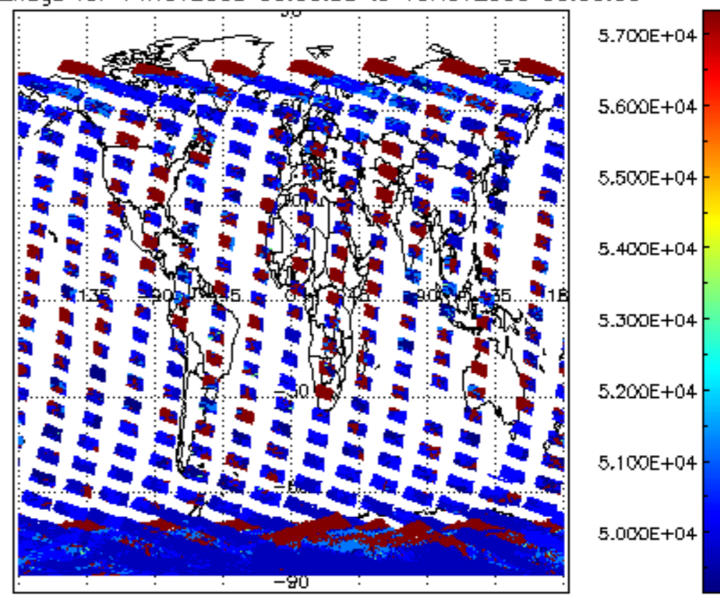
cloud_flags for 14NOV2009 00:00:00 to 15NOV2009 00:00:00
