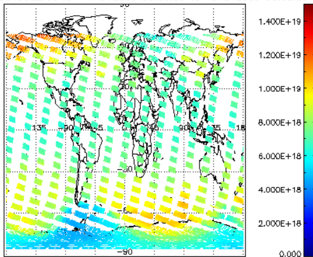
SCIOL2P_NADUV003_vcd for 14NOV2009 00:00:00 to 15NOV2009 00:00:00
