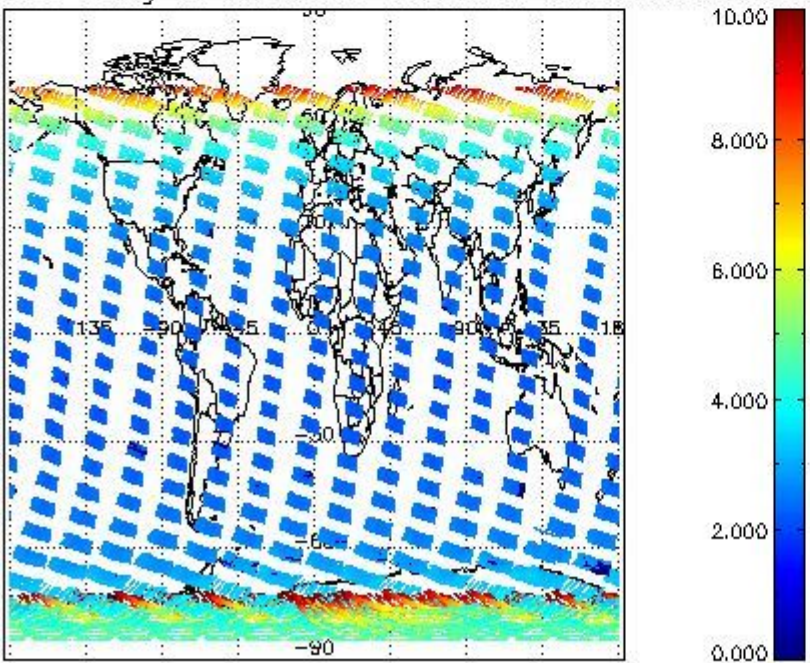
SCIOL2P_NADUV003_amf_gr for 14NOV2009 00:00:00 to 15NOV2009 00:00:00
