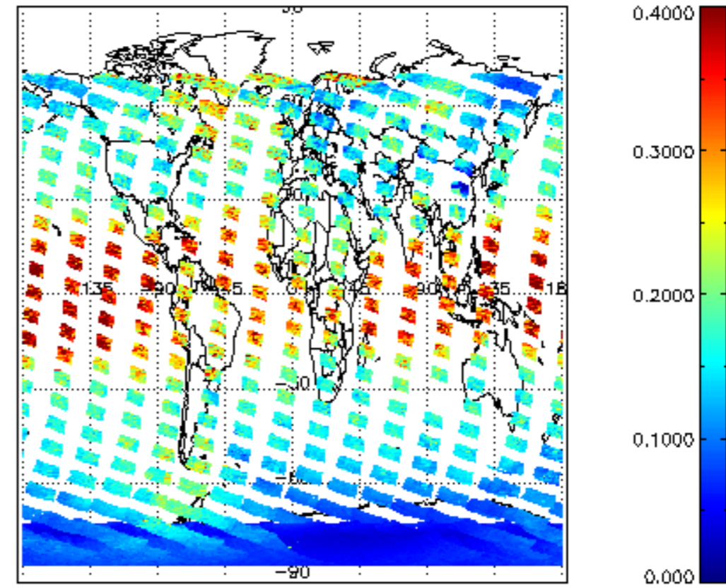
SCIOL2P_NADUV1NO2_vcd_err for 14NOV2009 00:00:00 to 15NOV2009 00:00:00
