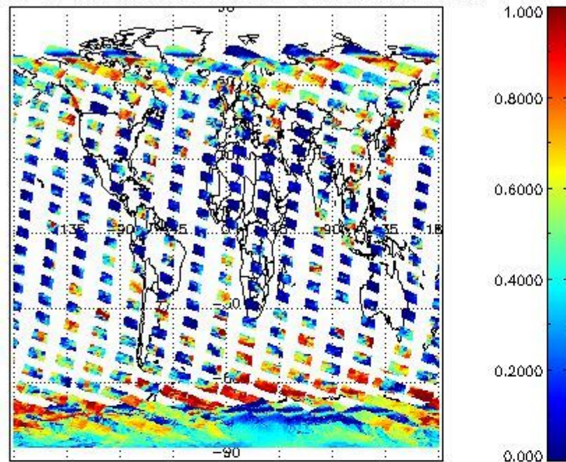
cLfrac for 14NOV2009 00:00:00 to 15NOV2009 00:00:00
