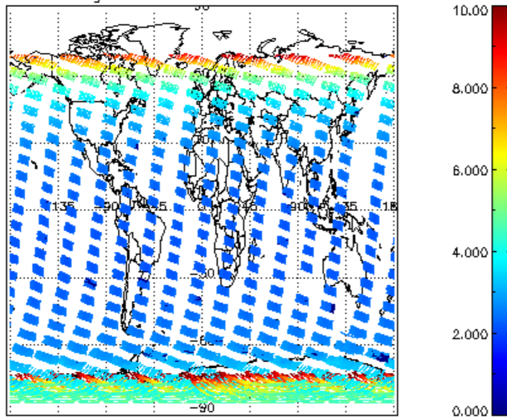
SCIOL2P_NADUV003_amf_gr for 14NOV2009 00:00:00 to 15NOV2009 00:00:00
