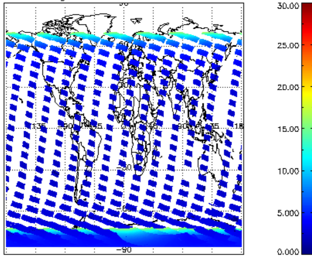
SCIOL2P_NADUV1NO2_amf_gr for 14NOV2009 00:00:00 to 15NOV2009 00:00:00
