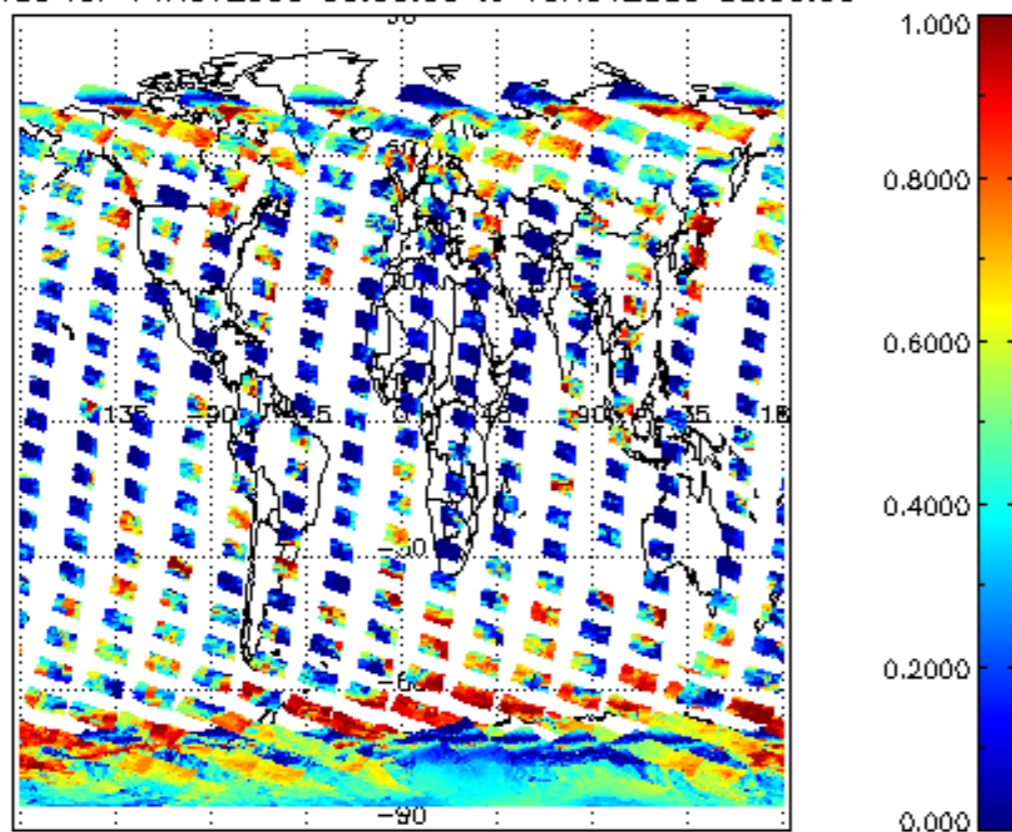
cLfrac for 14NOV2009 00:00:00 to 15NOV2009 00:00:00
