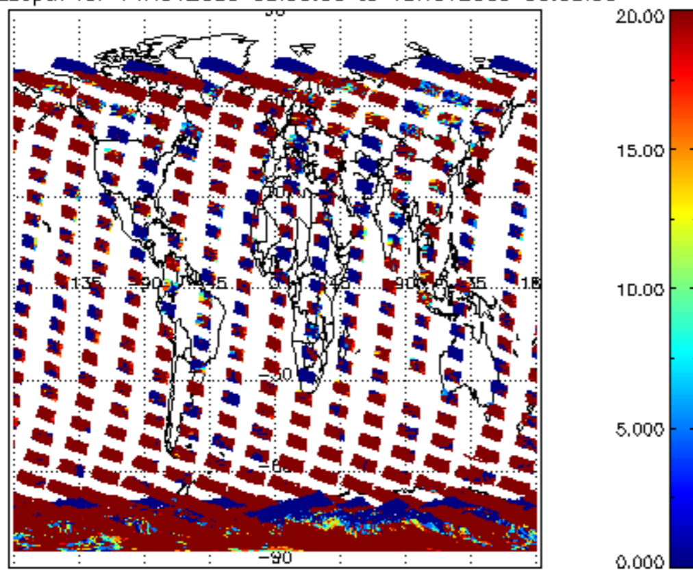
cL_opt_depth for 14NOV2009 00:00:00 to 15NOV2009 00:00:00
