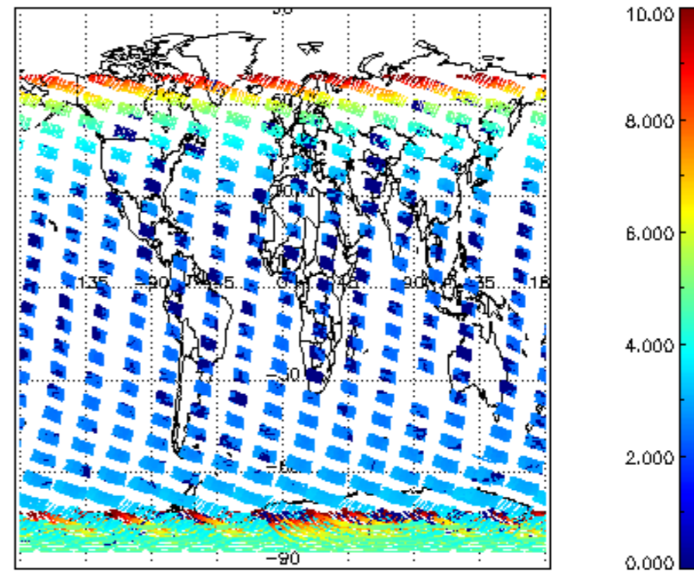
SCIOL2P_NADUV003_amf_cl for 14NOV2009 00:00:00 to 15NOV2009 00:00:00
