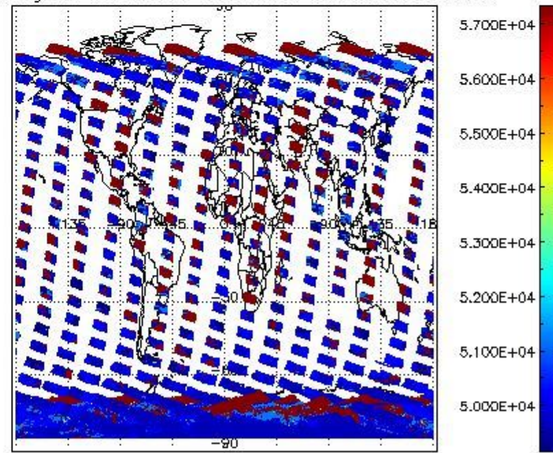
cloud_flags for 14NOV2009 00:00:00 to 15NOV2009 00:00:00
