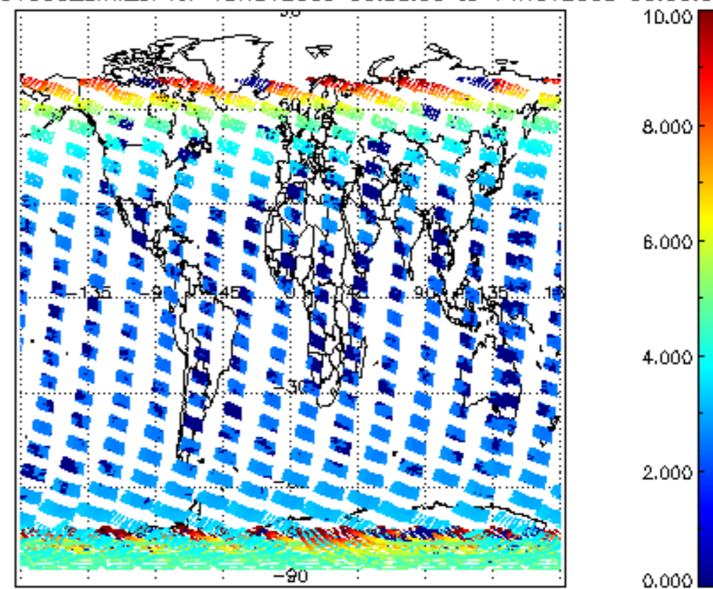
SCIOL2P_NADUV003_amf_cl for 13NOV2009 00:00:00 to 14NOV2009 00:00:00
