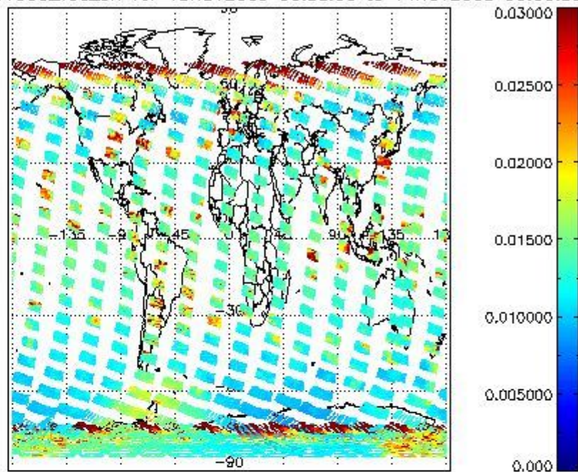
SCIOL2P_NADUV003_vcd_err for 13NOV2009 00:00:00 to 14NOV2009 00:00:00
