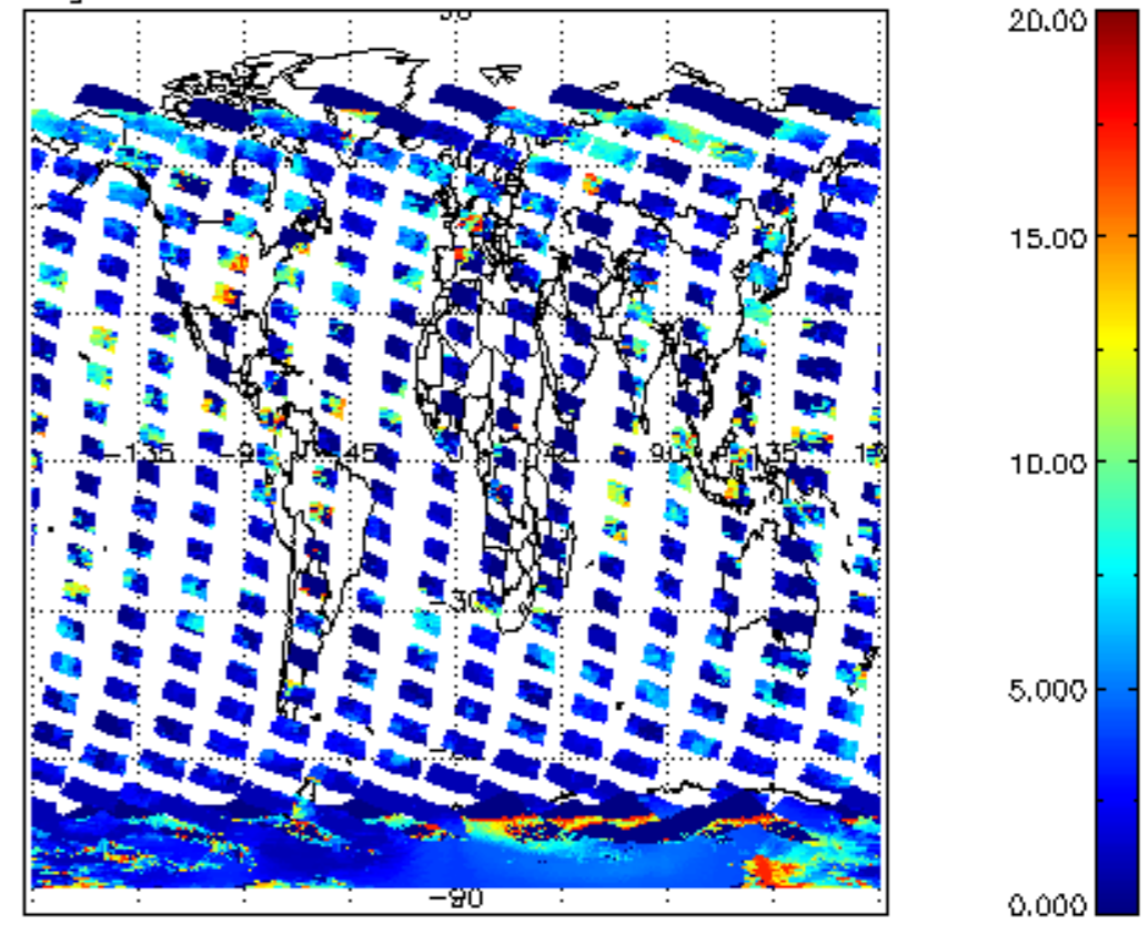
cL_top_height for 13NOV2009 00:00:00 to 14NOV2009 00:00:00
