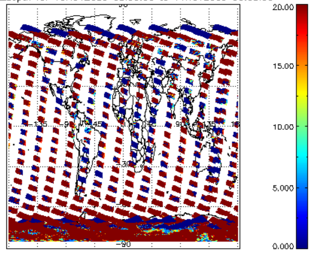
cL_opt_depth for 13NOV2009 00:00:00 to 14NOV2009 00:00:00
