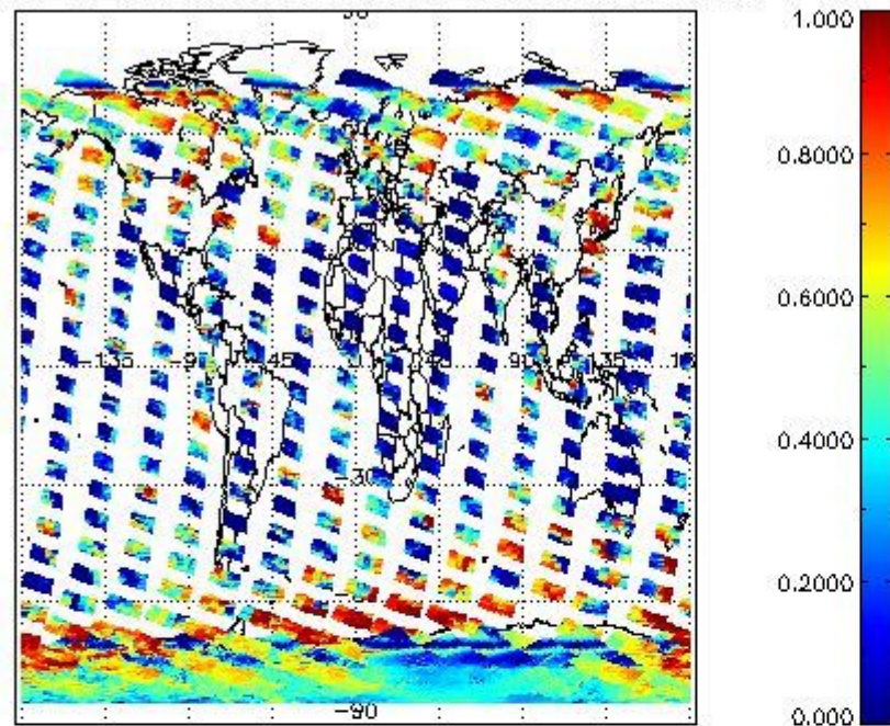
cLfrac for 13NOV2009 00:00:00 to 14NOV2009 00:00:00
