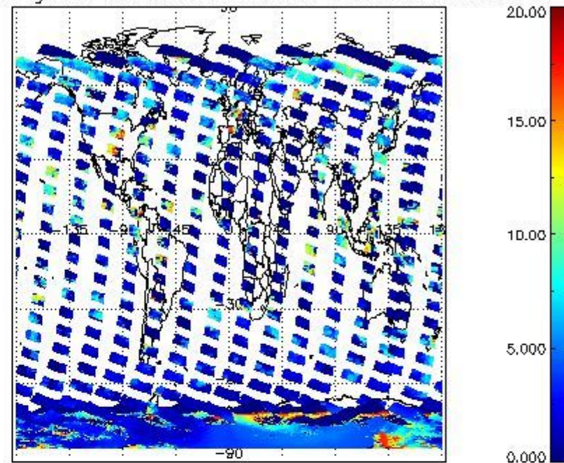
cL_top_height for 13NOV2009 00:00:00 to 14NOV2009 00:00:00
