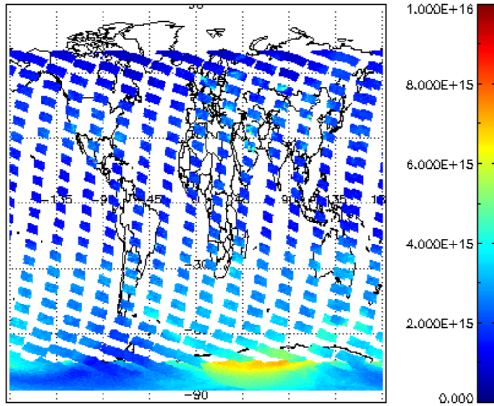
SCIOL2P_NADUV1NO2_vcd for 13NOV2009 00:00:00 to 14NOV2009 00:00:00
