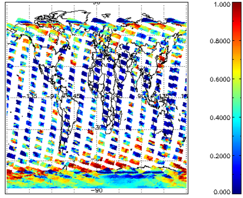
cLfrac for 13NOV2009 00:00:00 to 14NOV2009 00:00:00
