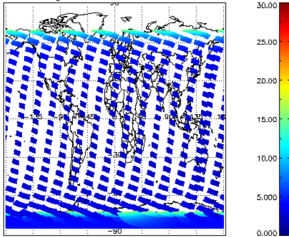
SCIOL2P_NADUV1NO2_amf_gr for 13NOV2009 00:00:00 to 14NOV2009 00:00:00
