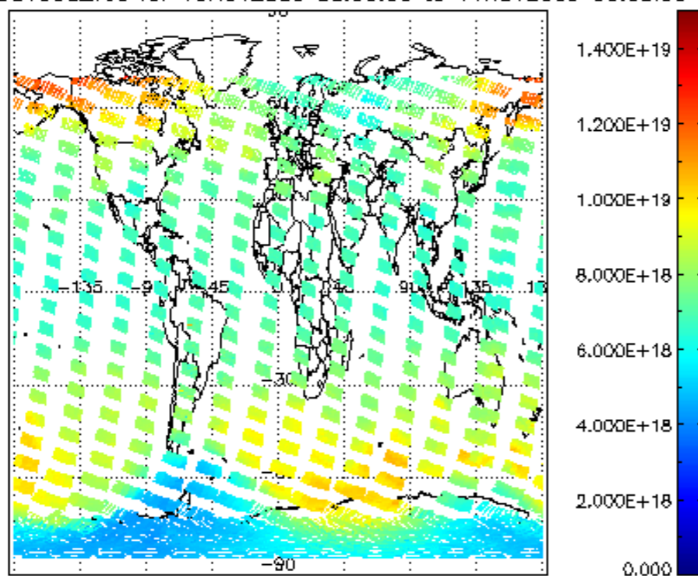
SCIOL2P_NADUV003_vcd for 13NOV2009 00:00:00 to 14NOV2009 00:00:00
