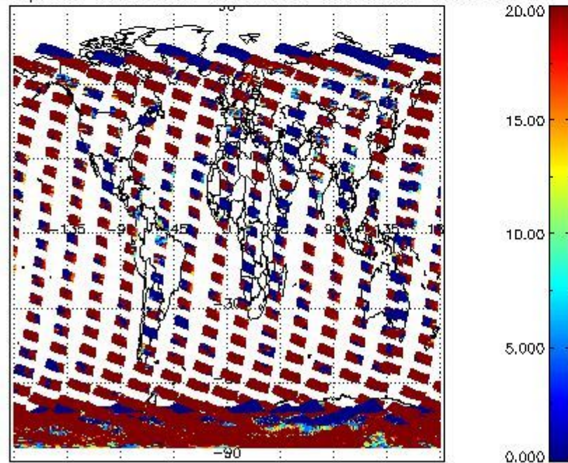
cLopt_depth for 13NOV2009 00:00:00 to 14NOV2009 00:00:00
