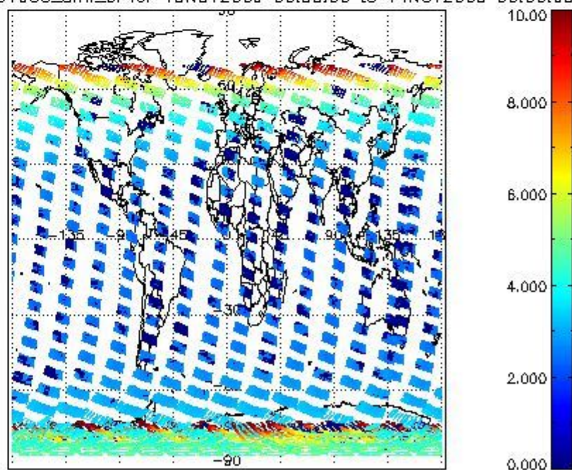
SCIOL2P_NADUV003_amf_cl for 13NOV2009 00:00:00 to 14NOV2009 00:00:00
