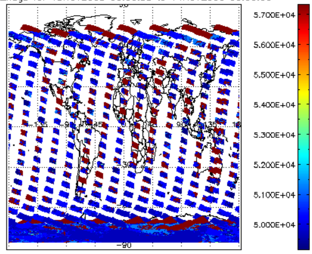
cloud_flags for 13NOV2009 00:00:00 to 14NOV2009 00:00:00
