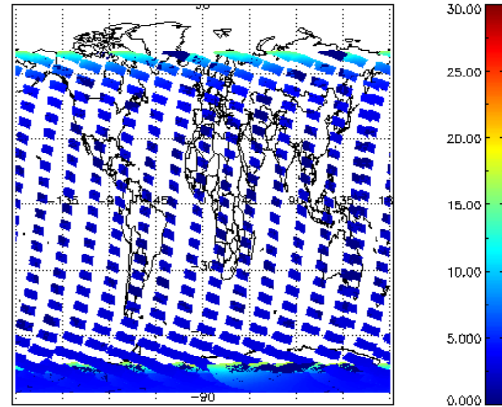
SCIOL2P_NADUV1NO2_amf_cl for 13NOV2009 00:00:00 to 14NOV2009 00:00:00
