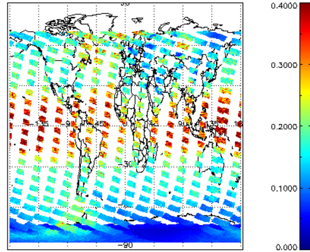
SCIOL2P_NADUV1NO2_vcd_err for 13NOV2009 00:00:00 to 14NOV2009 00:00:00
