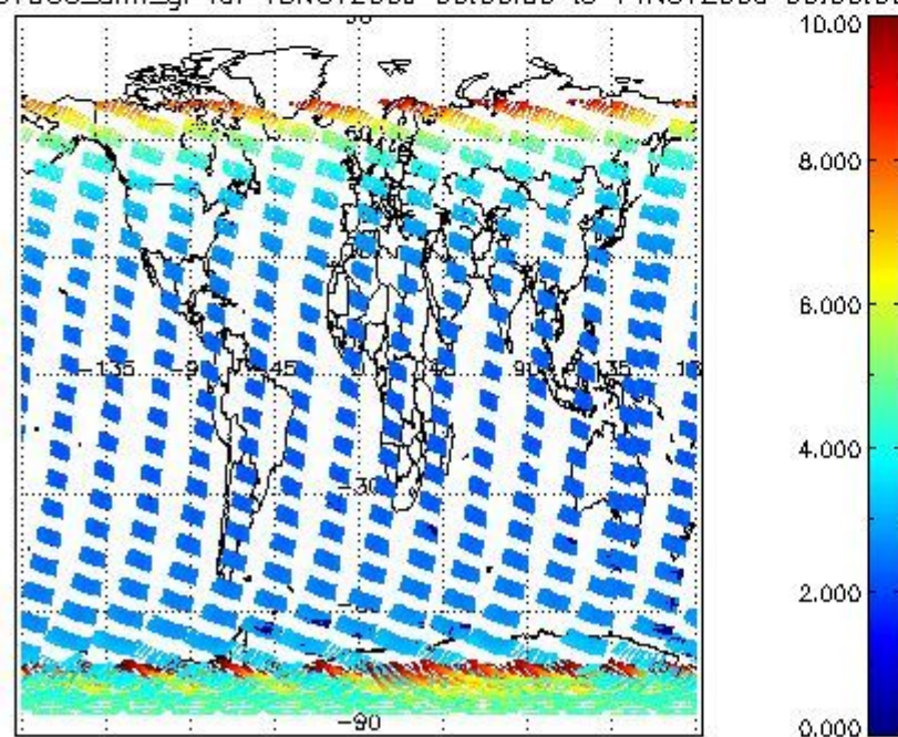
SCIOL2P_NADUV003_amf_gr for 13NOV2009 00:00:00 to 14NOV2009 00:00:00
