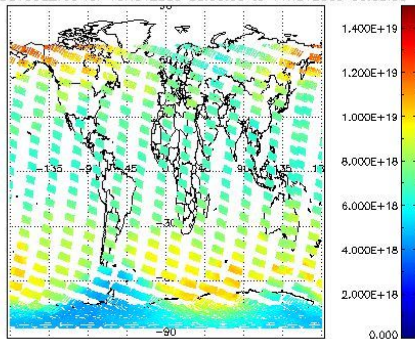
SCIOL2P_NADUV003_vcd for 13NOV2009 00:00:00 to 14NOV2009 00:00:00
