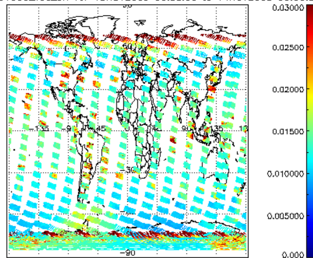
SCIOL2P_NADUV003_vcd_err for 13NOV2009 00:00:00 to 14NOV2009 00:00:00
