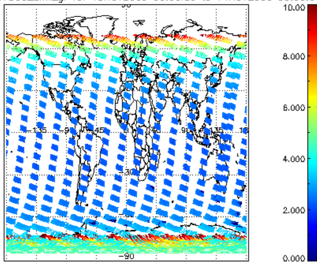
SCIOL2P_NADUV003_amf_gr for 13NOV2009 00:00:00 to 14NOV2009 00:00:00
