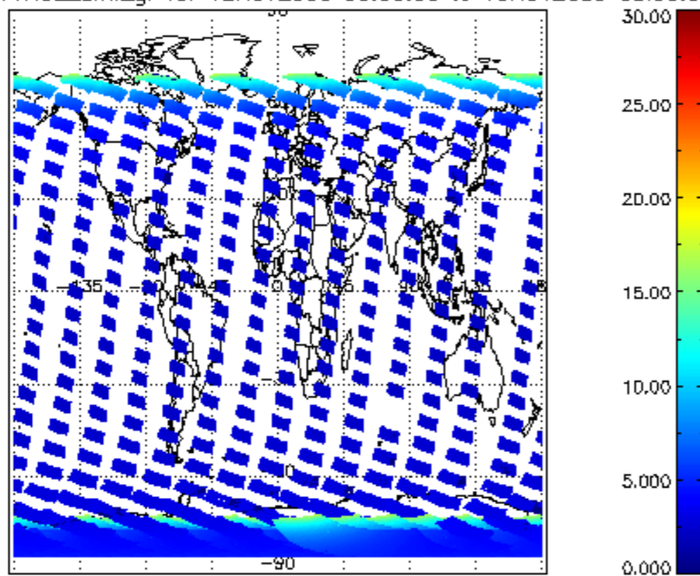
SCIOL2P_NADUV1NO2_amf_gr for 12NOV2009 00:00:00 to 13NOV2009 00:00:00
