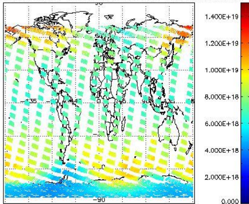
SCIOL2P_NADUV003_vcd for 12NOV2009 00:00:00 to 13NOV2009 00:00:00
