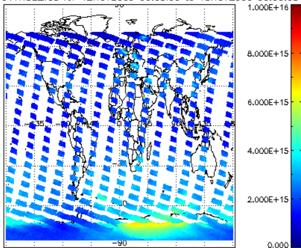
SCIOL2P_NADUV1NO2_vcd for 12NOV2009 00:00:00 to 13NOV2009 00:00:00
