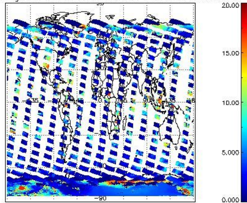
cL_top_height for 12NOV2009 00:00:00 to 13NOV2009 00:00:00
