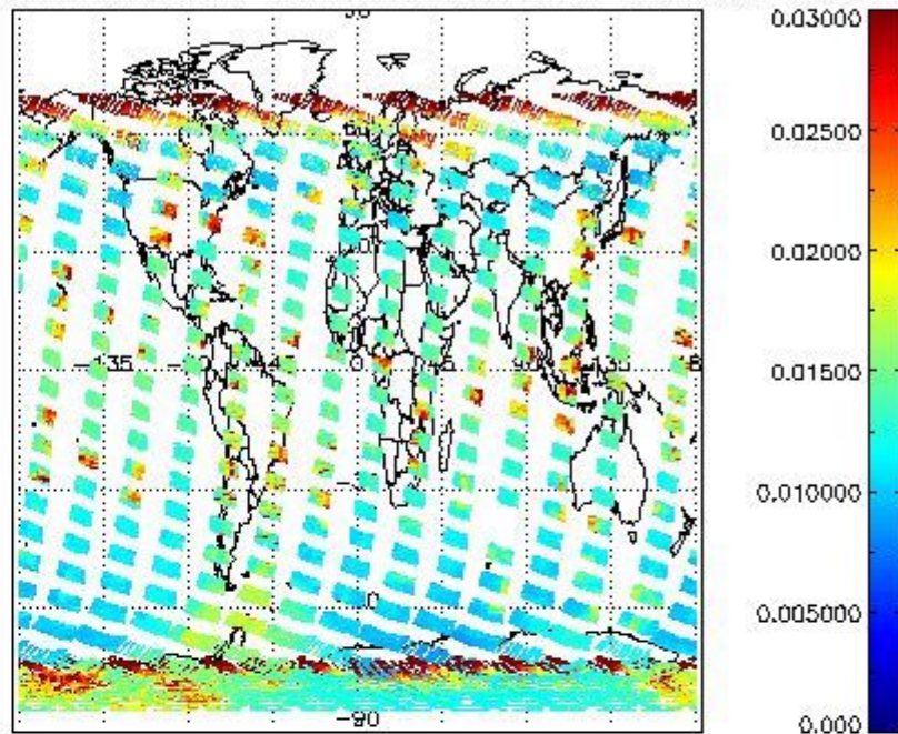
SCIOL2P_NADUV003_vcd_err for 12NOV2009 00:00:00 to 13NOV2009 00:00:00
