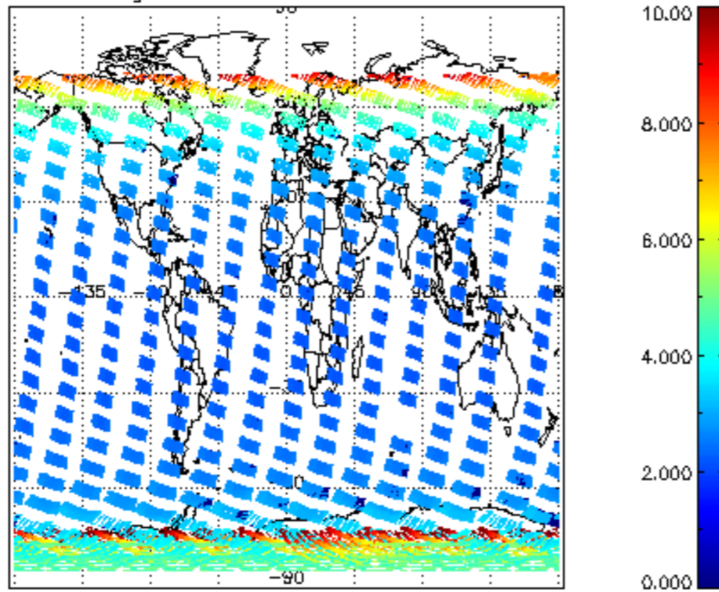
SCIOL2P_NADUV003_amf_gr for 12NOV2009 00:00:00 to 13NOV2009 00:00:00
