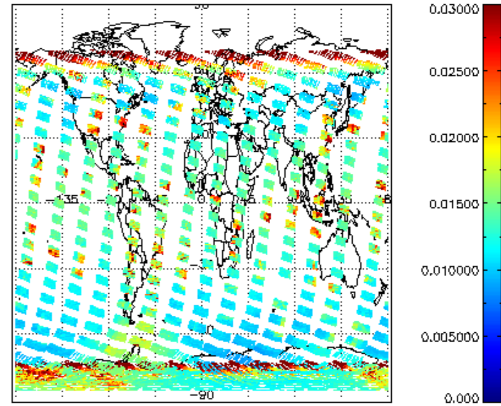
SCIOL2P_NADUV003_vcd_err for 12NOV2009 00:00:00 to 13NOV2009 00:00:00
