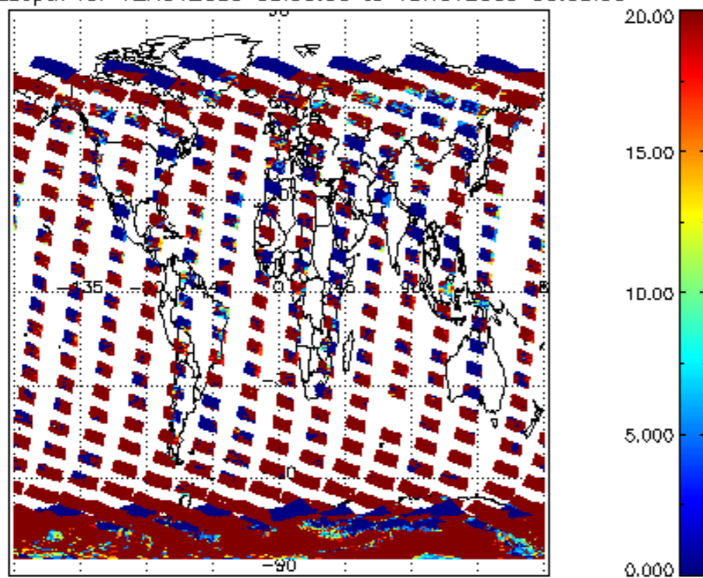
cL_opt_depth for 12NOV2009 00:00:00 to 13NOV2009 00:00:00
