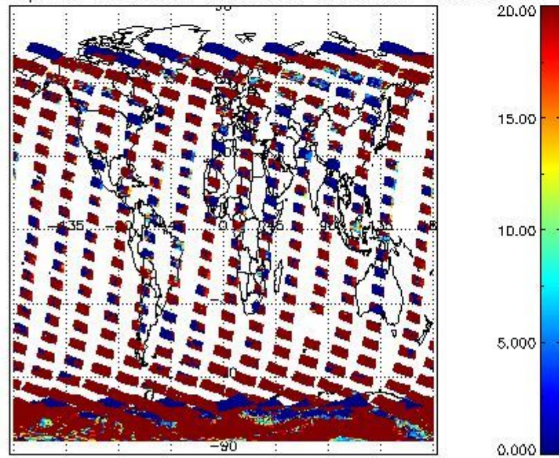
cLopt_depth for 12NOV2009 00:00:00 to 13NOV2009 00:00:00
