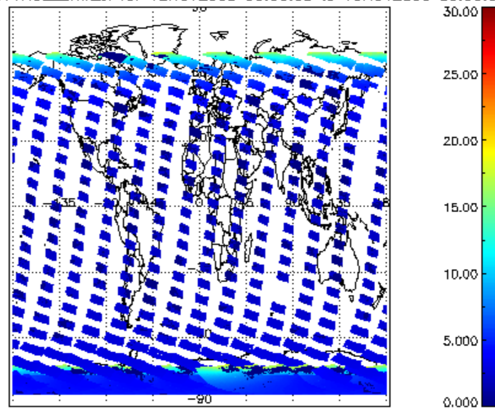
SCIOL2P_NADUV1NO2_amf_cl for 12NOV2009 00:00:00 to 13NOV2009 00:00:00
