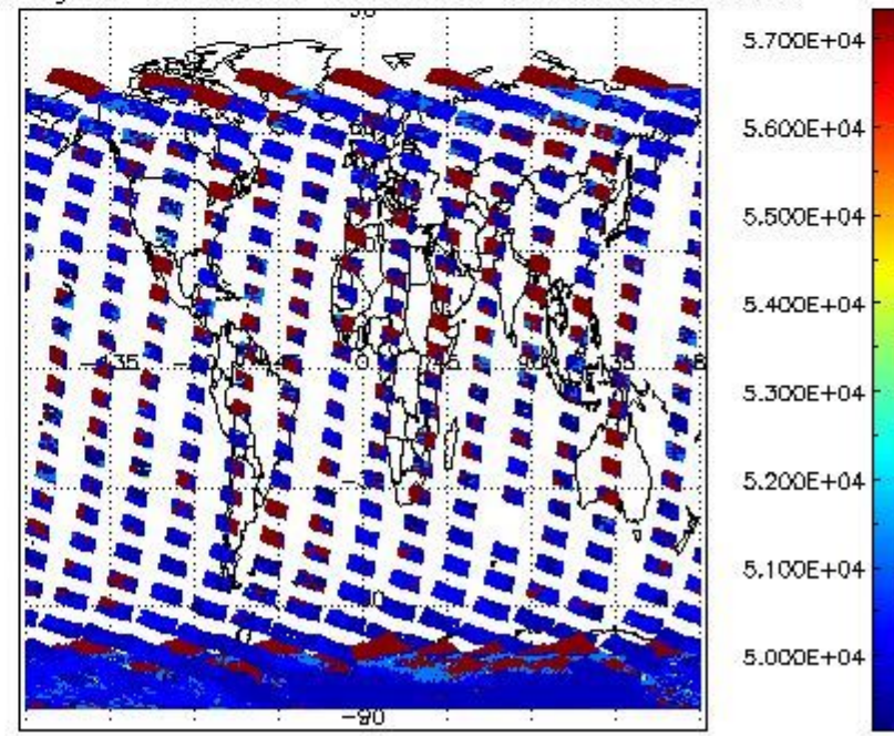
cloud_flags for 12NOV2009 00:00:00 to 13NOV2009 00:00:00
