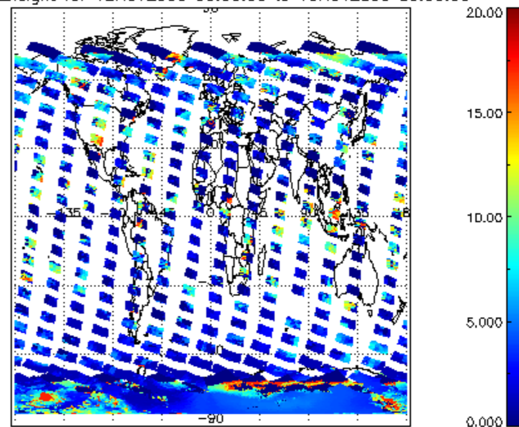
cL_top_height for 12NOV2009 00:00:00 to 13NOV2009 00:00:00
