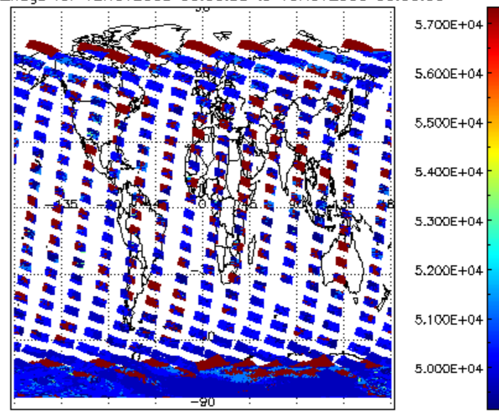
cloud_flags for 12NOV2009 00:00:00 to 13NOV2009 00:00:00
