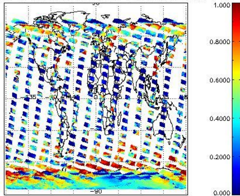
cLfrac for 12NOV2009 00:00:00 to 13NOV2009 00:00:00
