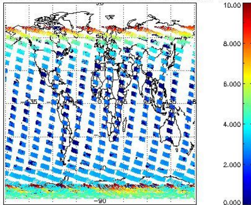
SCIOL2P_NADUV003_amf_cl for 12NOV2009 00:00:00 to 13NOV2009 00:00:00
