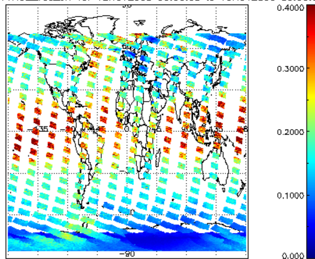
SCIOL2P_NADUV1NO2_vcd_err for 12NOV2009 00:00:00 to 13NOV2009 00:00:00
