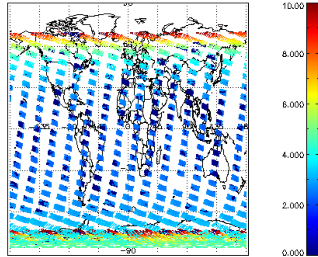
SCIOL2P_NADUV003_amf_cl for 12NOV2009 00:00:00 to 13NOV2009 00:00:00
