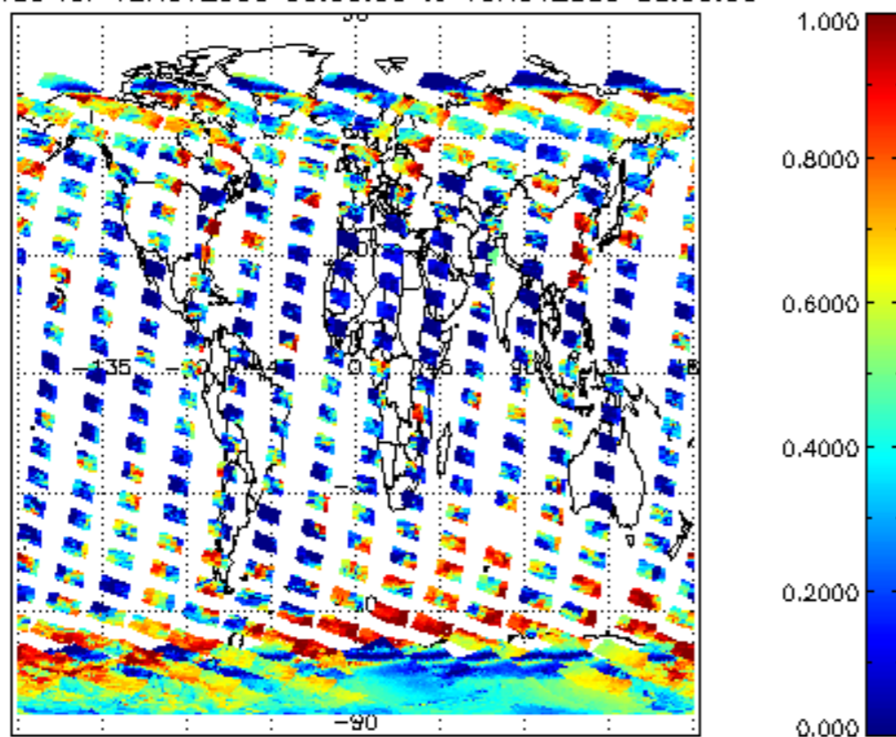
cLfrac for 12NOV2009 00:00:00 to 13NOV2009 00:00:00
