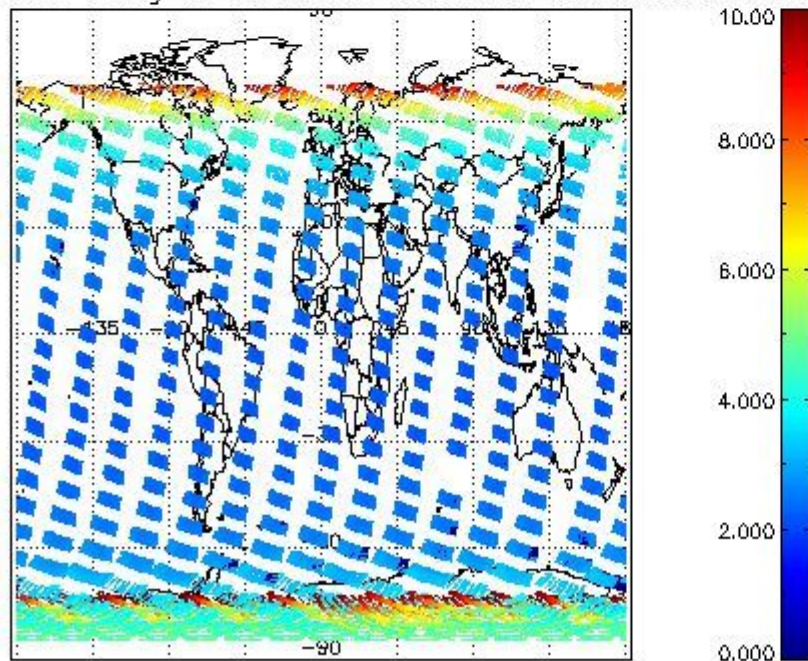
SCIOL2P_NADUV003_amf_gr for 12NOV2009 00:00:00 to 13NOV2009 00:00:00
