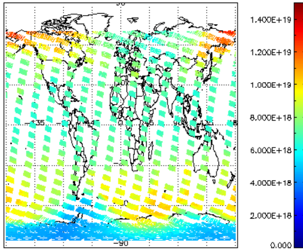
SCIOL2P_NADUV003_vcd for 12NOV2009 00:00:00 to 13NOV2009 00:00:00
