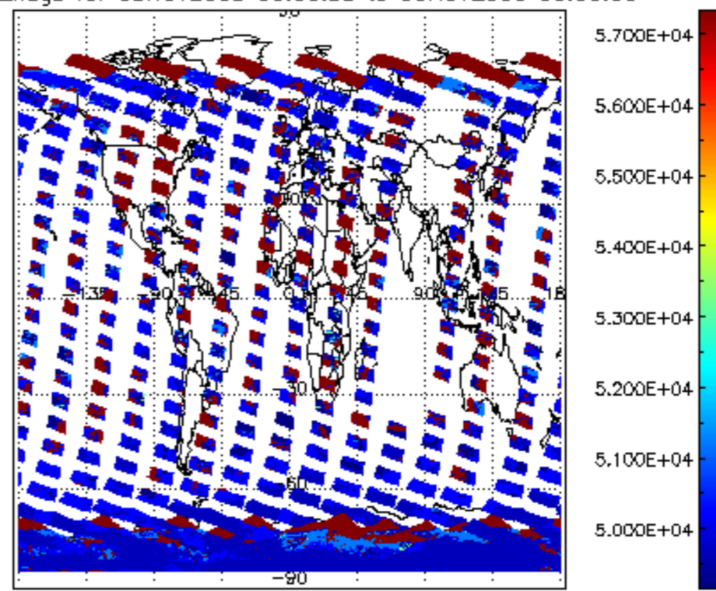
cloud_flags for 08NOV2009 00:00:00 to 09NOV2009 00:00:00
