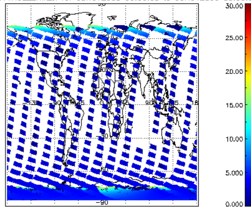
SCIOL2P_NADUV1NO2_amf_cl for 08NOV2009 00:00:00 to 09NOV2009 00:00:00
