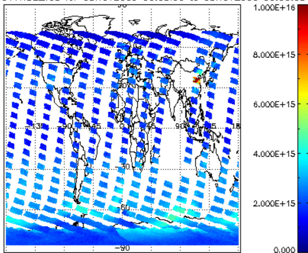
SCIOL2P_NADUV1NO2_vcd for 08NOV2009 00:00:00 to 09NOV2009 00:00:00
