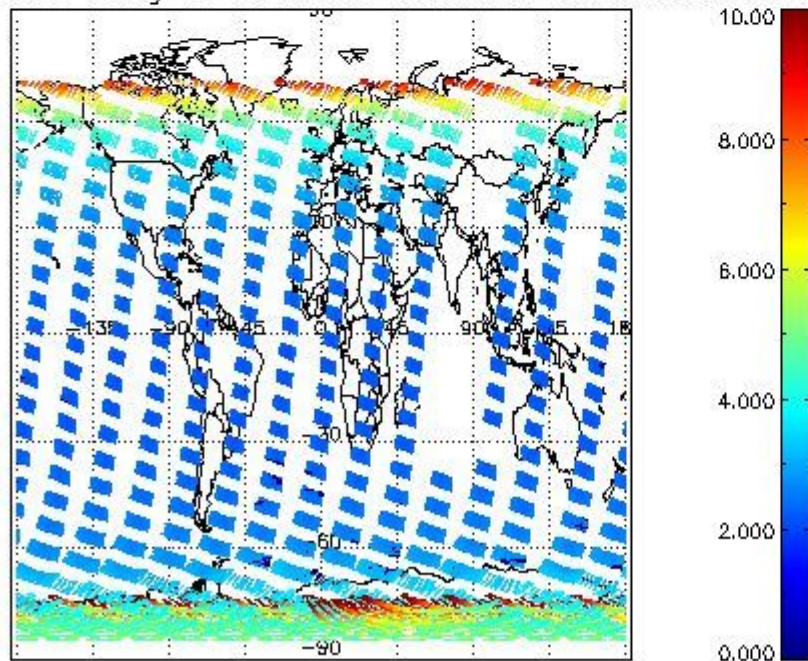
SCIOL2P_NADUV003_amf_gr for 08NOV2009 00:00:00 to 09NOV2009 00:00:00
