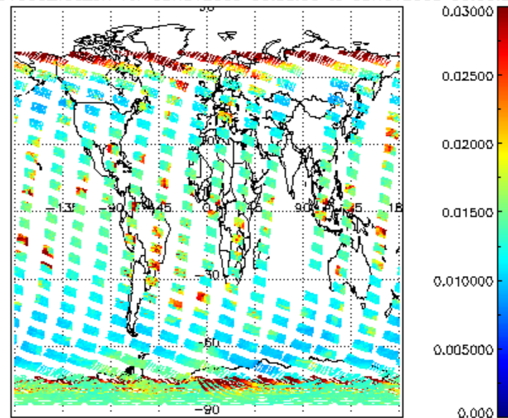
SCIOL2P_NADUV003_vcd_err for 08NOV2009 00:00:00 to 09NOV2009 00:00:00
