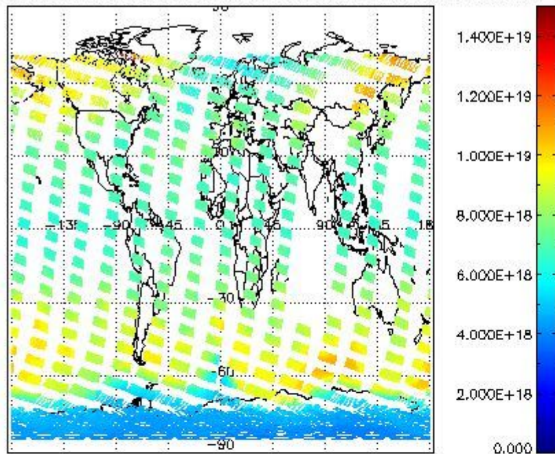
SCIOL2P_NADUV003_vcd for 08NOV2009 00:00:00 to 09NOV2009 00:00:00
