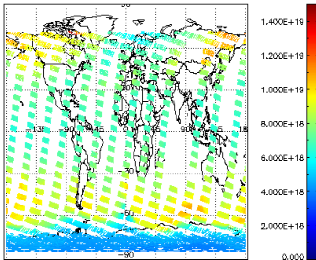
SCIOL2P_NADUV003_vcd for 08NOV2009 00:00:00 to 09NOV2009 00:00:00
