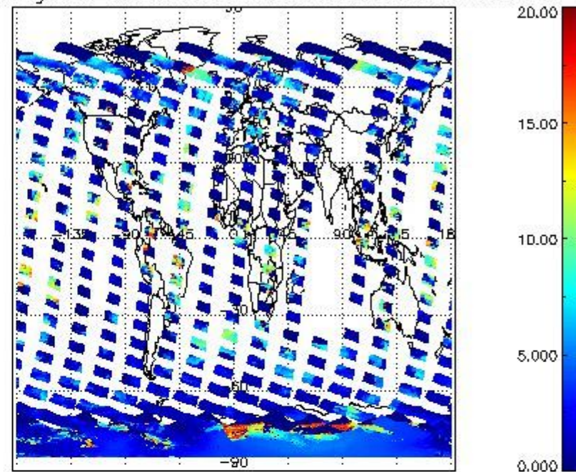
cL_top_height for 08NOV2009 00:00:00 to 09NOV2009 00:00:00
