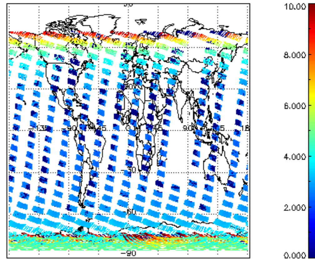
SCIOL2P_NADUV003_amf_cl for 08NOV2009 00:00:00 to 09NOV2009 00:00:00
