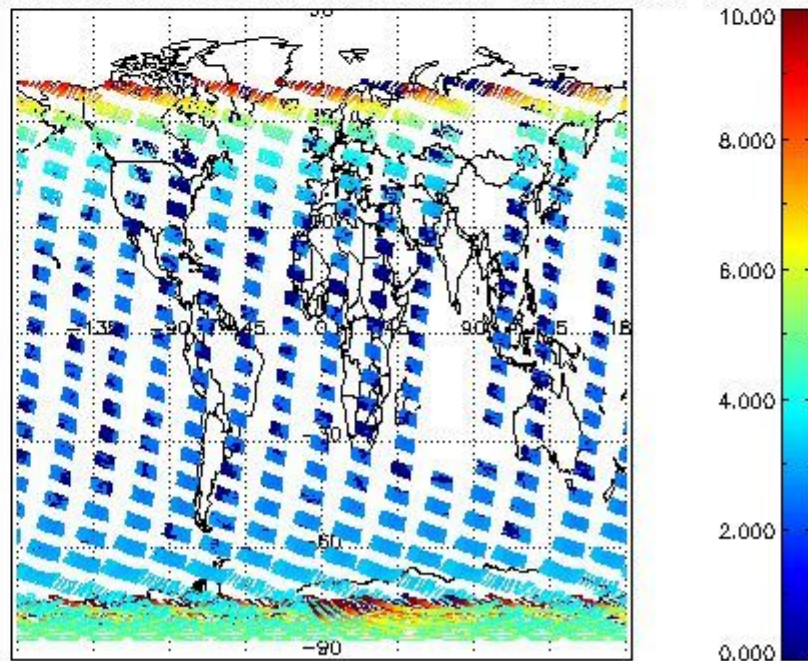
SCIOL2P_NADUV003_amf_cl for 08NOV2009 00:00:00 to 09NOV2009 00:00:00
