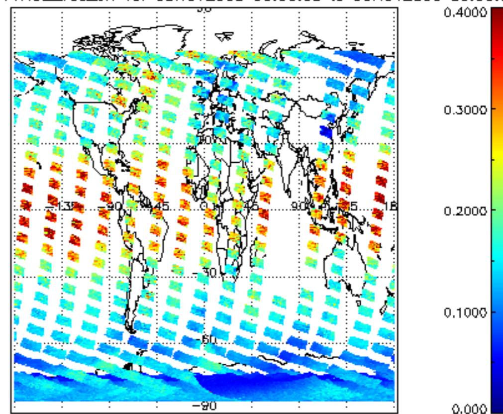
SCIOL2P_NADUV1NO2_vcd_err for 08NOV2009 00:00:00 to 09NOV2009 00:00:00
