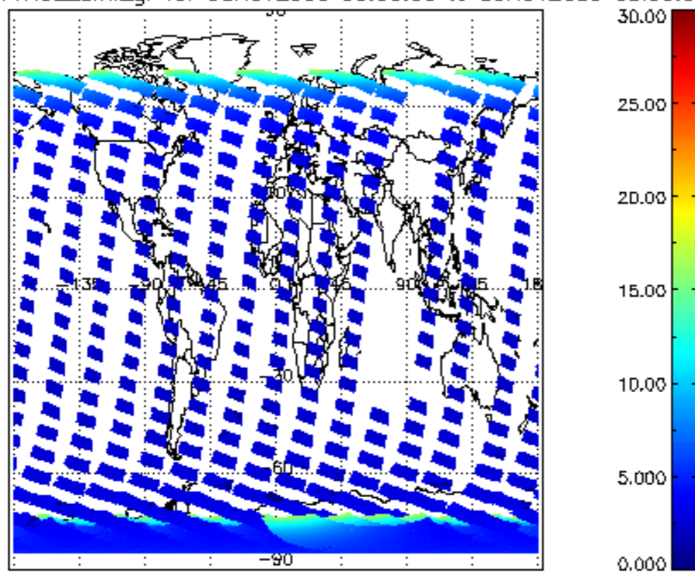
SCIOL2P_NADUV1NO2_amf_gr for 08NOV2009 00:00:00 to 09NOV2009 00:00:00
