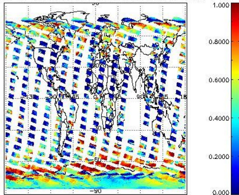
cLfrac for 08NOV2009 00:00:00 to 09NOV2009 00:00:00
