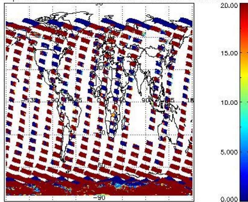
cLopt_depth for 08NOV2009 00:00:00 to 09NOV2009 00:00:00
