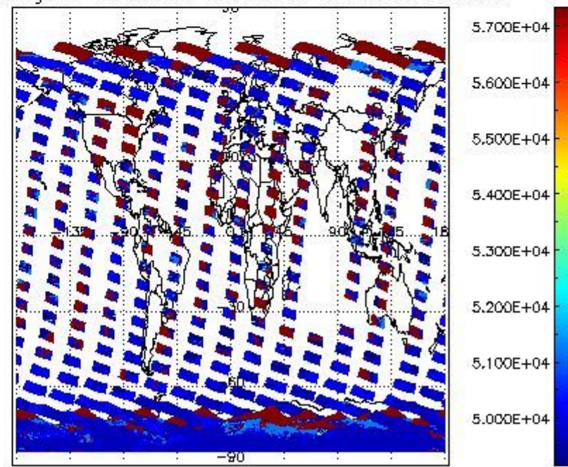
cloud_flags for 08NOV2009 00:00:00 to 09NOV2009 00:00:00
