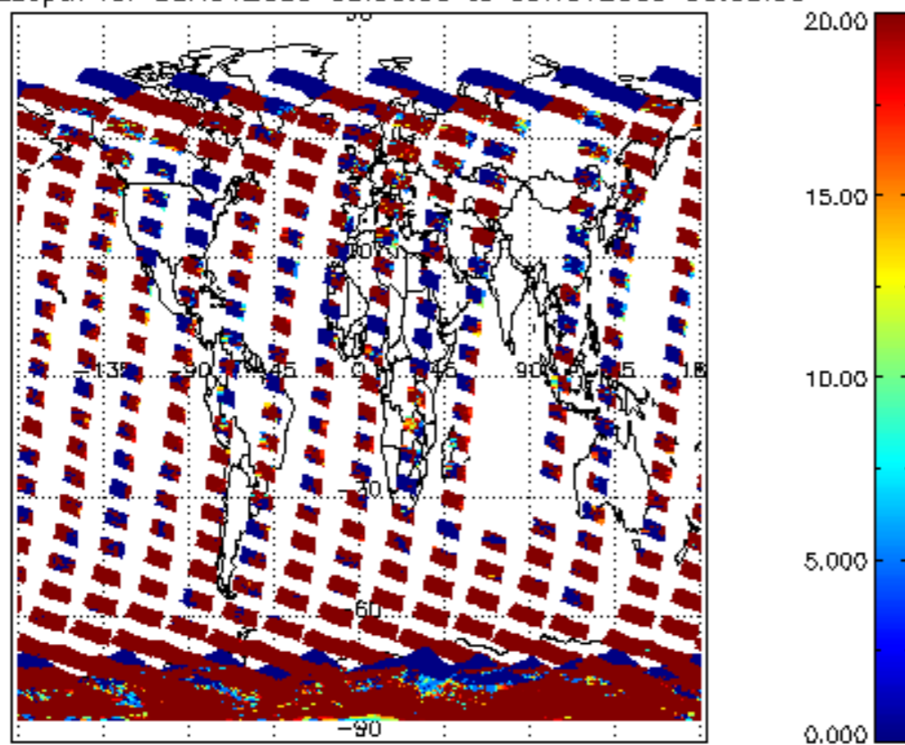
cl_opt_depth for 08NOV2009 00:00:00 to 09NOV2009 00:00:00
