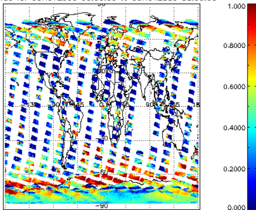
cLfrac for 08NOV2009 00:00:00 to 09NOV2009 00:00:00
