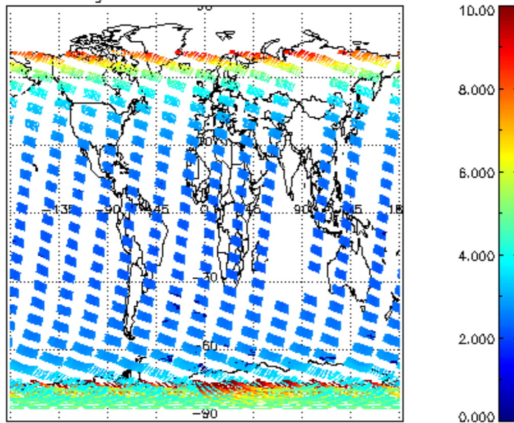
SCIOL2P_NADUV003_amf_gr for 08NOV2009 00:00:00 to 09NOV2009 00:00:00
