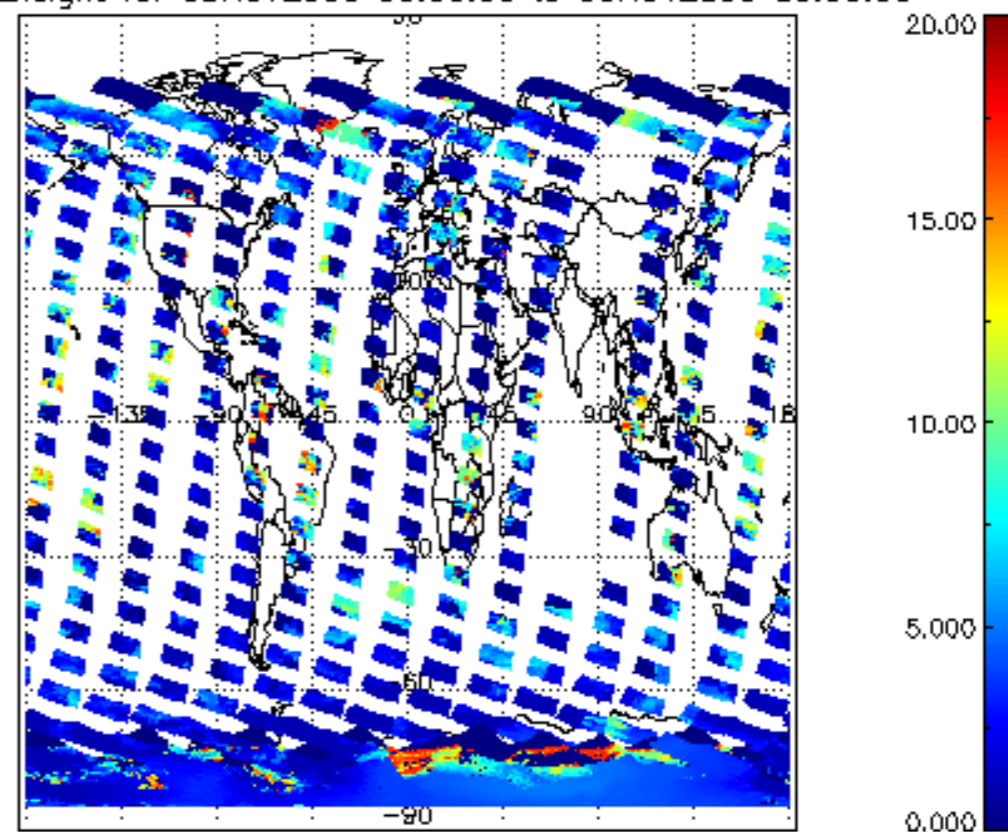
cl_top_height for 08NOV2009 00:00:00 to 09NOV2009 00:00:00
