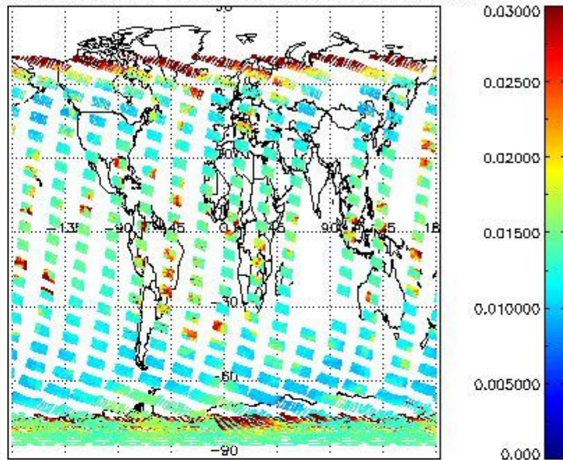
SCIOL2P_NADUV003_vcd_err for 08NOV2009 00:00:00 to 09NOV2009 00:00:00
