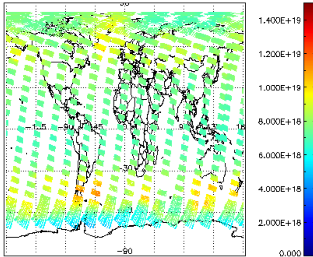
SCIOL2P_NADUV003_vcd for 22AUG2009 00:00:00 to 23AUG2009 00:00:00
