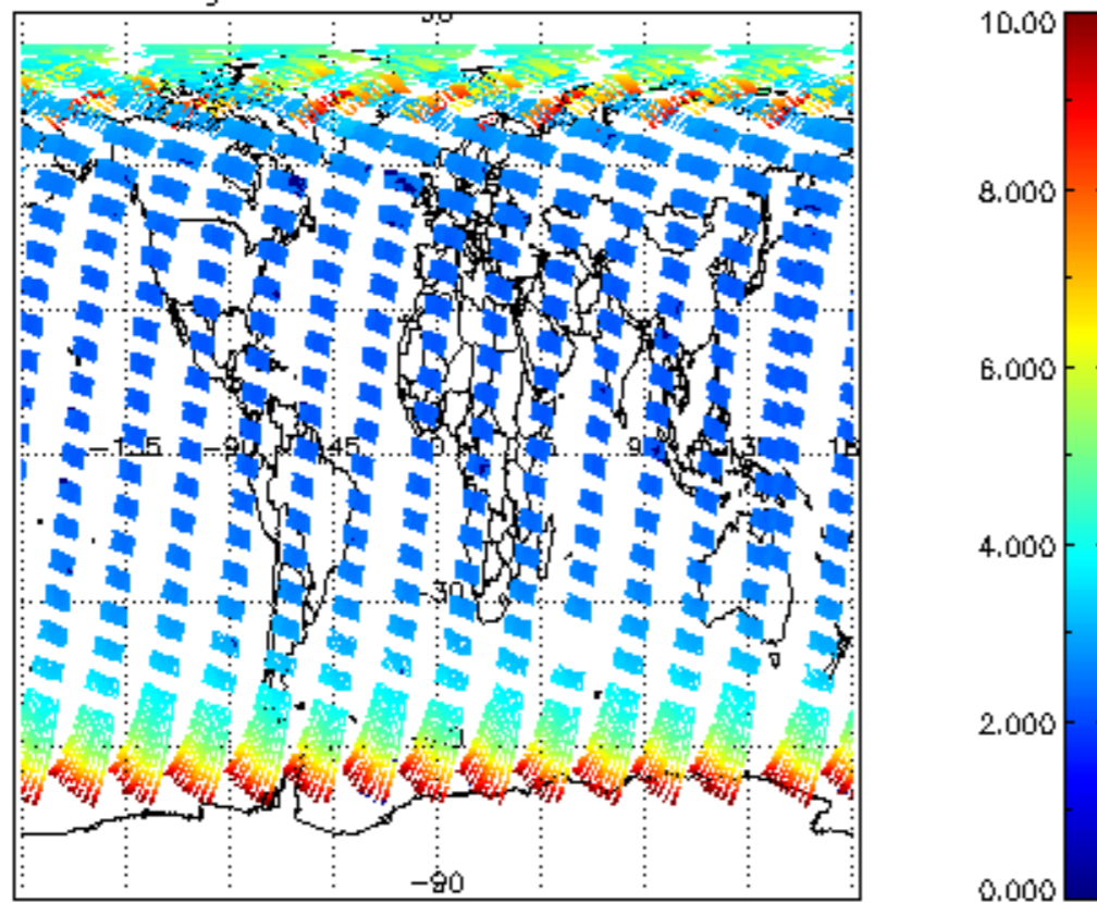
SCIOL2P_NADUV003_amf_gr for 22AUG2009 00:00:00 to 23AUG2009 00:00:00
