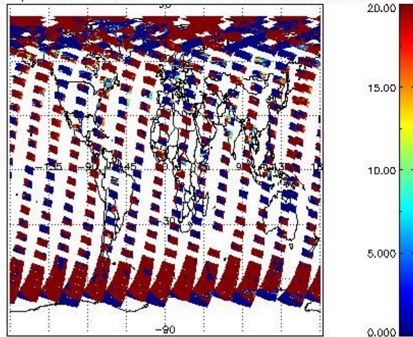
cL_opt_depth for 22AUG2009 00:00:00 to 23AUG2009 00:00:00
