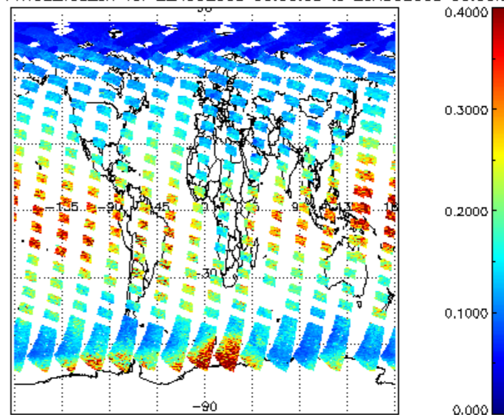
SCIOL2P_NADUV1NO2_vcd_err for 22AUG2009 00:00:00 to 23AUG2009 00:00:00
