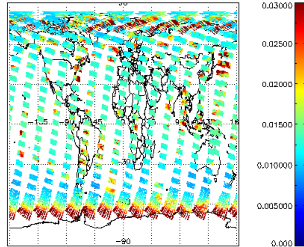
SCIOL2P_NADUV003_vcd_err for 22AUG2009 00:00:00 to 23AUG2009 00:00:00
