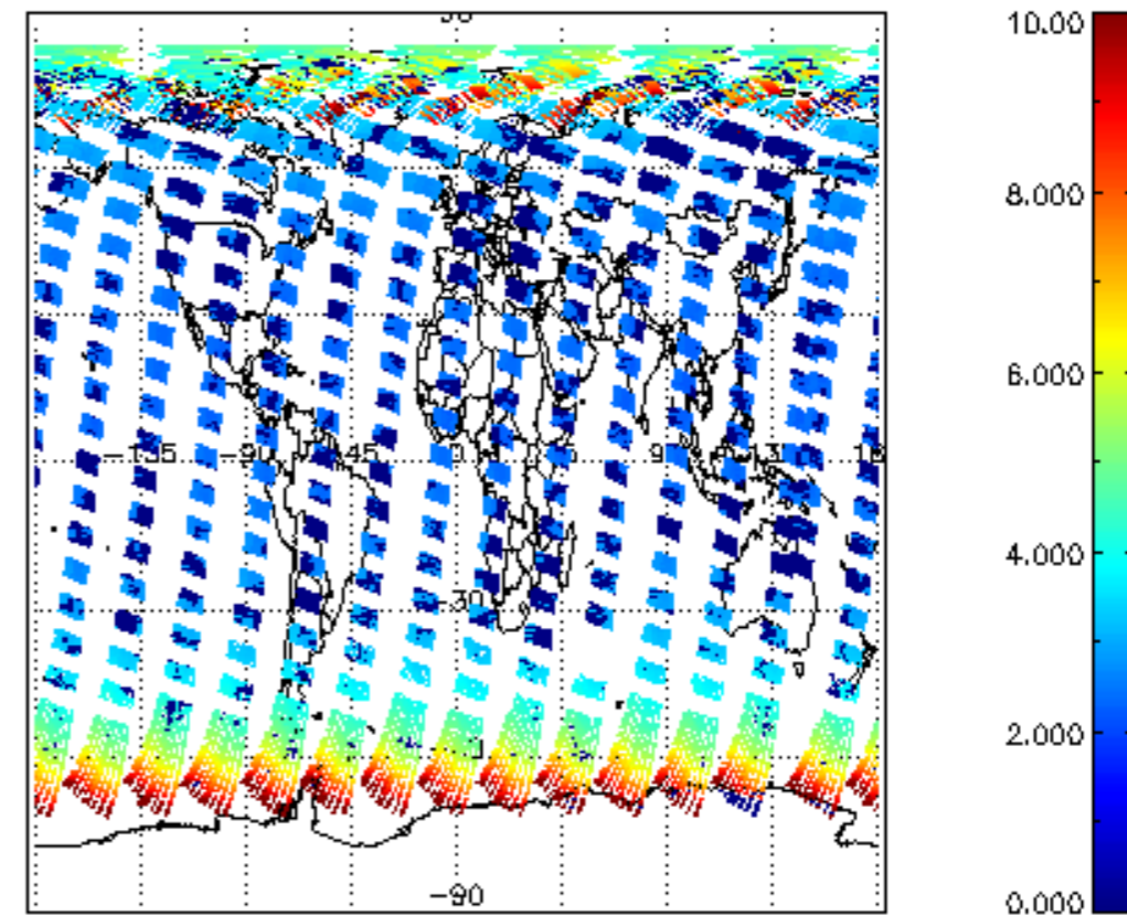
SCIOL2P_NADUV003_amf_cl for 22AUG2009 00:00:00 to 23AUG2009 00:00:00
