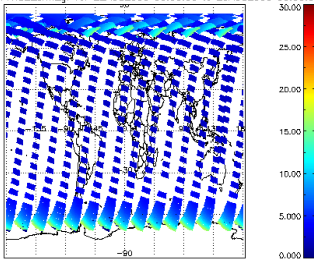
SCIOL2P_NADUV1NO2_amf_gr for 22AUG2009 00:00:00 to 23AUG2009 00:00:00
