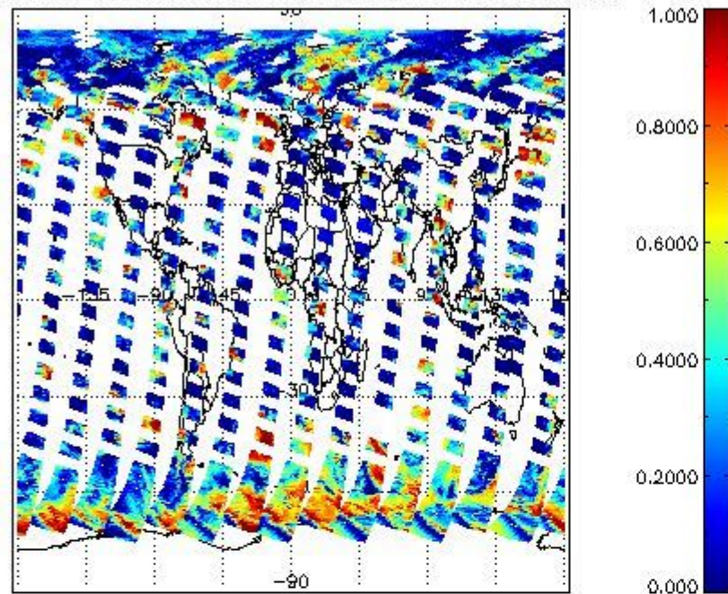
cL_frac for 22AUG2009 00:00:00 to 23AUG2009 00:00:00
