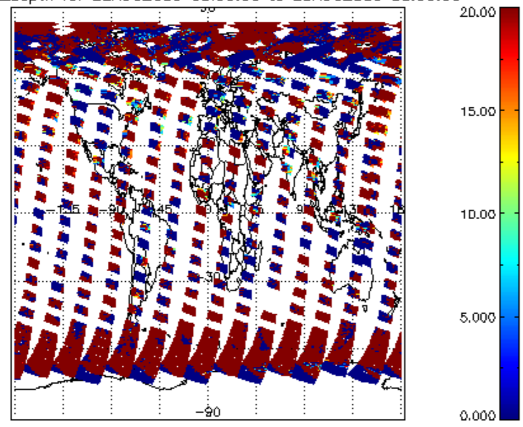
cI_opt_depth for 22AUG2009 00:00:00 to 23AUG2009 00:00:00
