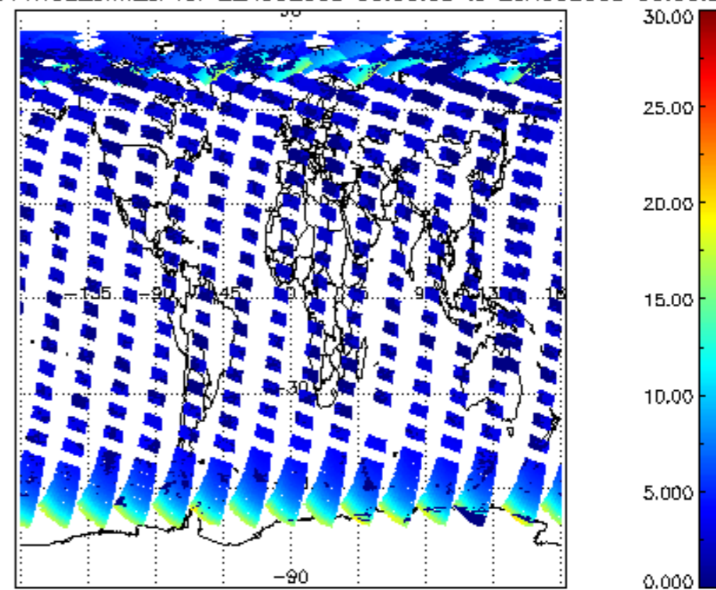
SCIOL2P_NADUV1NO2_amf_cl for 22AUG2009 00:00:00 to 23AUG2009 00:00:00
