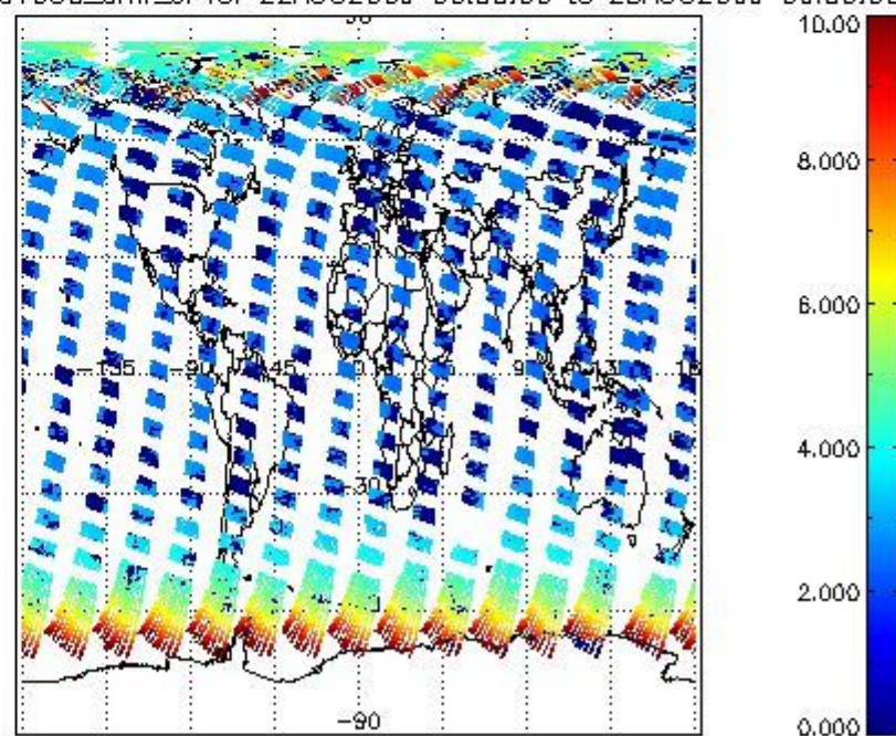
SCIOL2P_NADUV003_amf_gr for 22AUG2009 00:00:00 to 23AUG2009 00:00:00 SCIOL2P_NADUV003_amf_cl for 22AUG2009 00:00:00 to 23AUG2009 00:00:00
