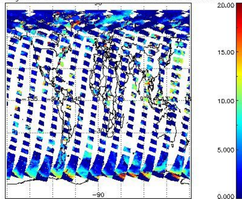
cL_top_height for 22AUG2009 00:00:00 to 23AUG2009 00:00:00
