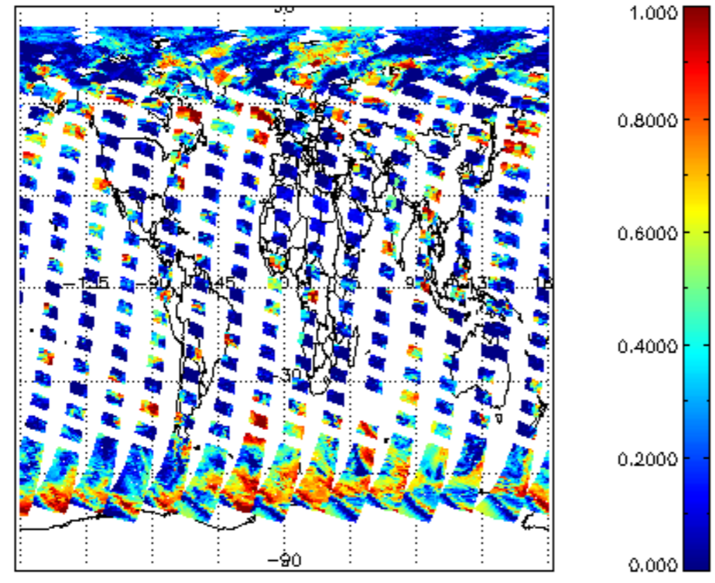
cI_frac for 22AUG2009 00:00:00 to 23AUG2009 00:00:00
