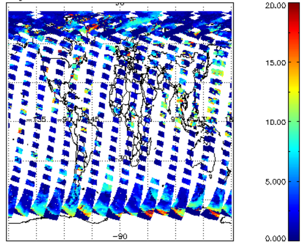
cI_top_height for 22AUG2009 00:00:00 to 23AUG2009 00:00:00
