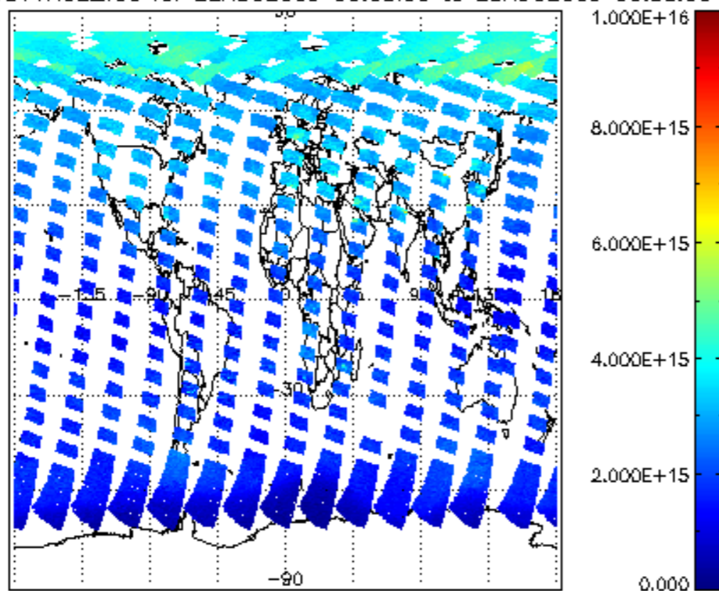
SCIOL2P_NADUV1NO2_vcd for 22AUG2009 00:00:00 to 23AUG2009 00:00:00
