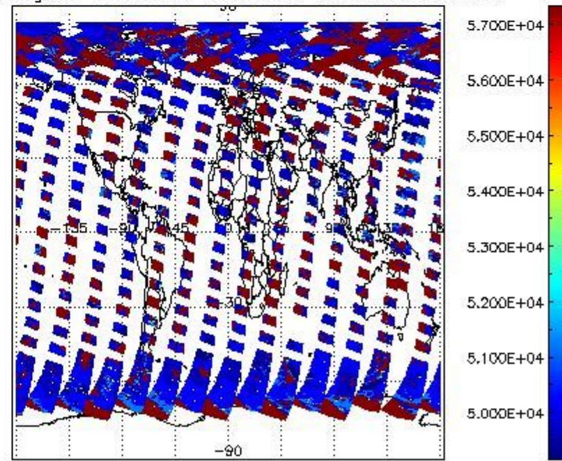
cloud_flags for 22AUG2009 00:00:00 to 23AUG2009 00:00:00
