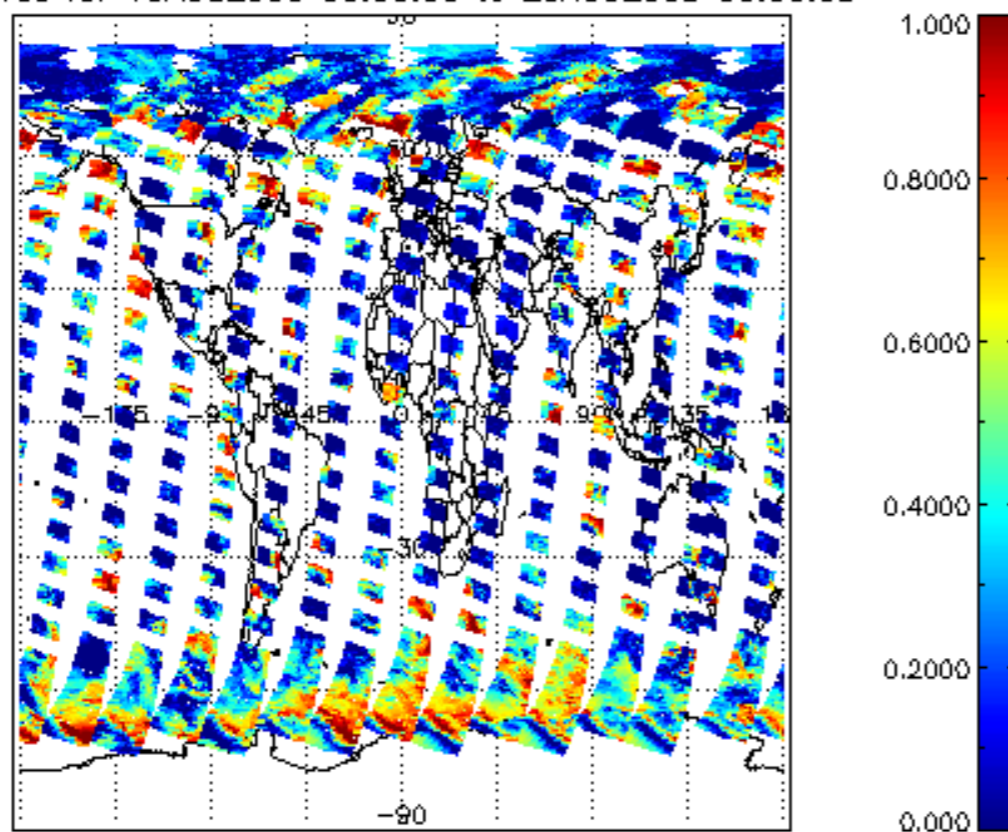
cL_frac for 19AUG2009 00:00:00 to 20AUG2009 00:00:00
