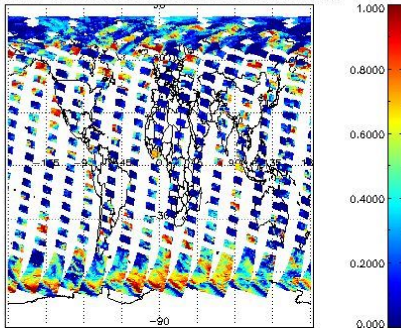
cL_frac for 19AUG2009 00:00:00 to 20AUG2009 00:00:00
