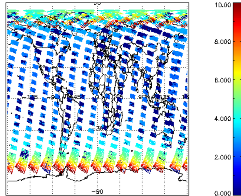
SCIOL2P_NADUV003_amf_cl for 19AUG2009 00:00:00 to 20AUG2009 00:00:00
