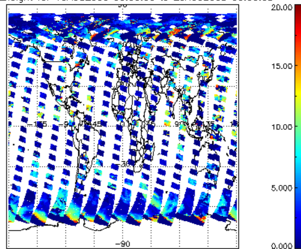
cL_top_height for 19AUG2009 00:00:00 to 20AUG2009 00:00:00
