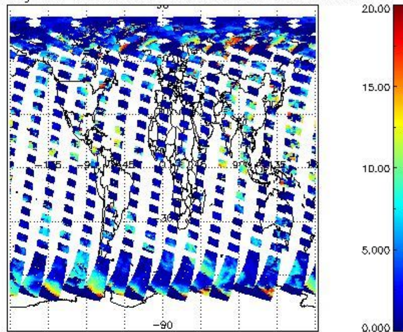
cL_top_height for 19AUG2009 00:00:00 to 20AUG2009 00:00:00
