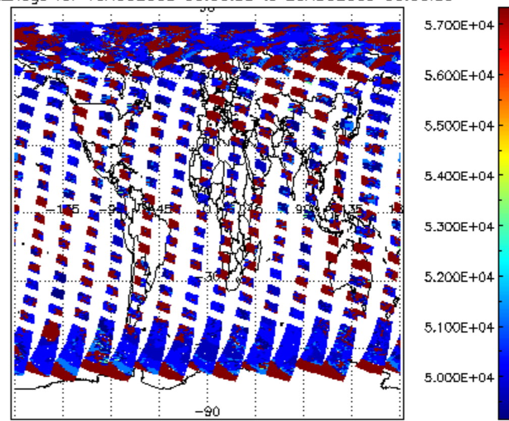
cloud_flags for 19AUG2009 00:00:00 to 20AUG2009 00:00:00
