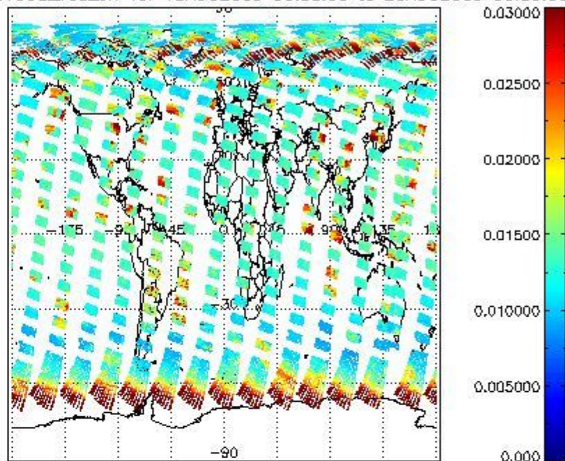
SCIOL2P_NADUV003_vcd for 19AUG2009 00:00:00 to 20AUG2009 00:00:00 SCIOL2P_NADUV003_vcd_err for 19AUG2009 00:00:00 to 20AUG2009 00:00:00
