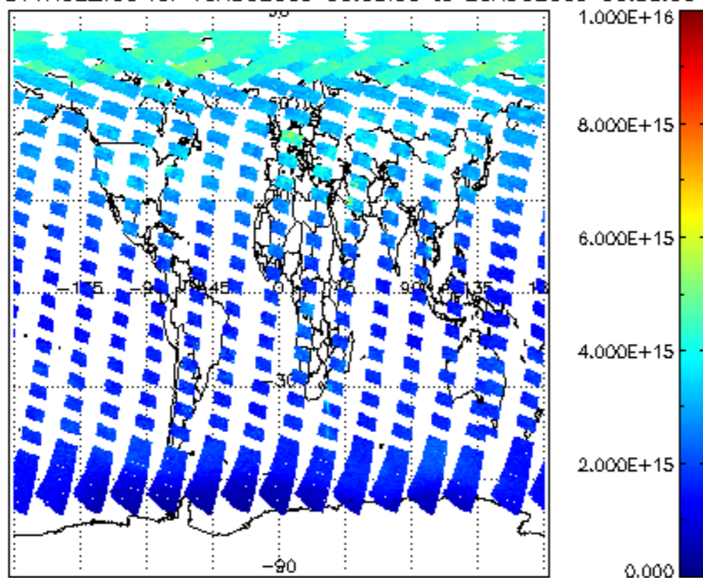
SCIOL2P_NADUV1NO2_vcd for 19AUG2009 00:00:00 to 20AUG2009 00:00:00
