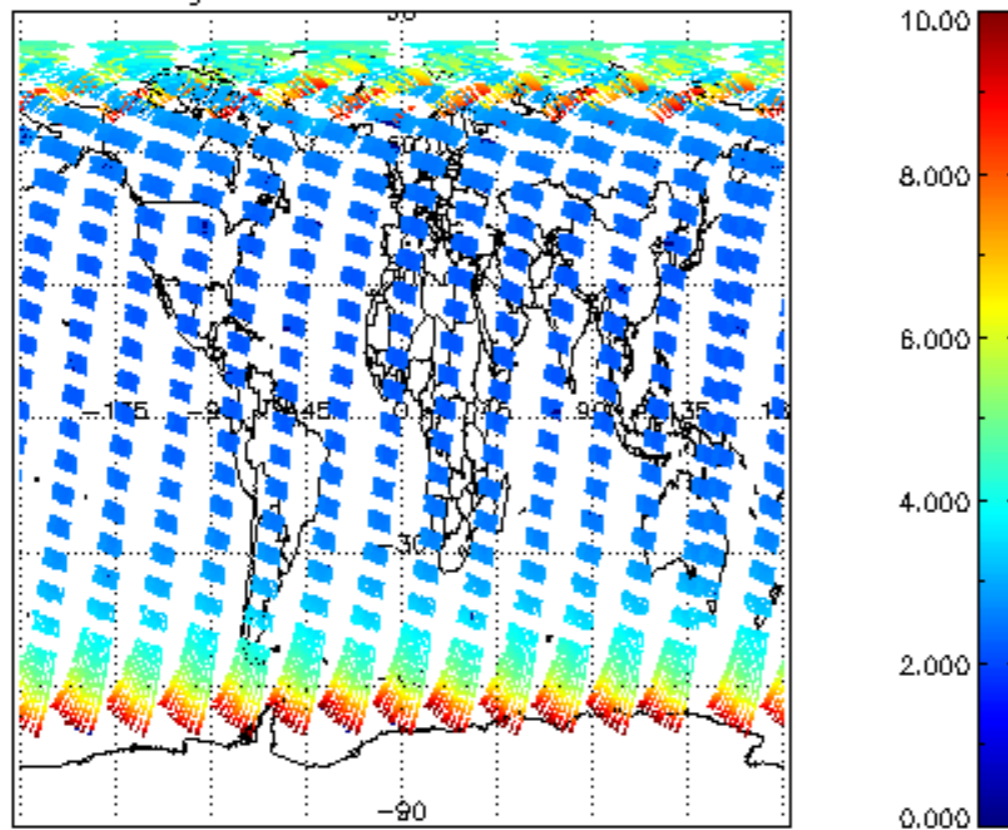
SCIOL2P_NADUV003_amf_gr for 19AUG2009 00:00:00 to 20AUG2009 00:00:00
