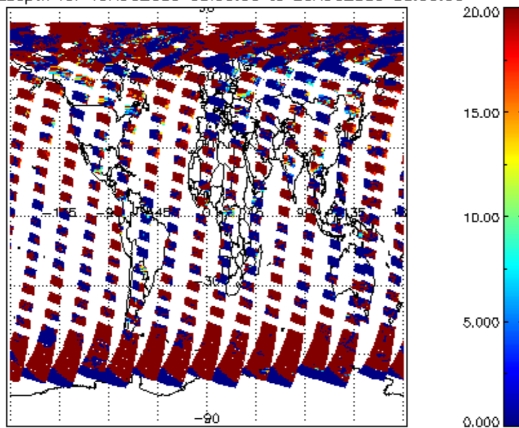
cL_opt_depth for 19AUG2009 00:00:00 to 20AUG2009 00:00:00
