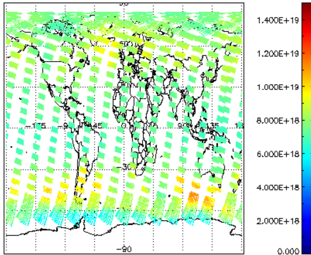
SCIOL2P_NADUV003_vcd for 19AUG2009 00:00:00 to 20AUG2009 00:00:00
