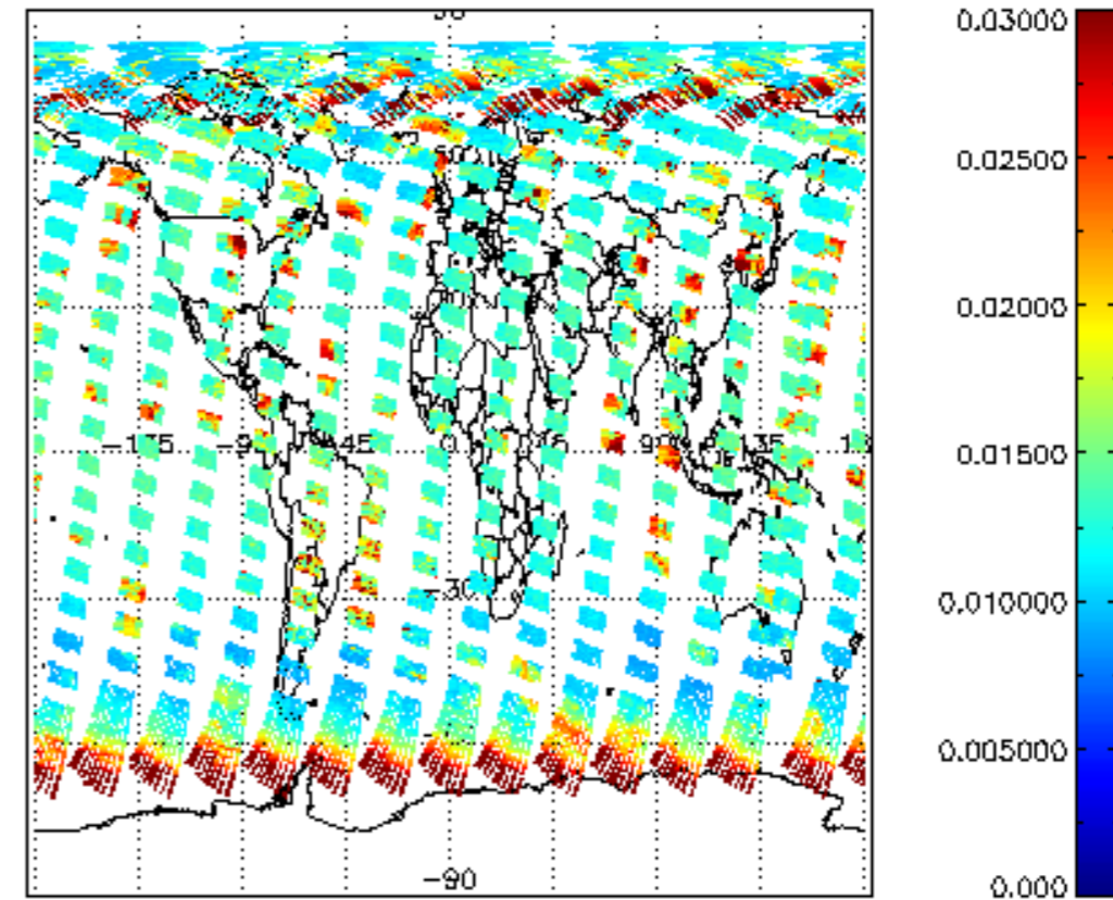
SCIOL2P_NADUV003_vcd_err for 19AUG2009 00:00:00 to 20AUG2009 00:00:00
