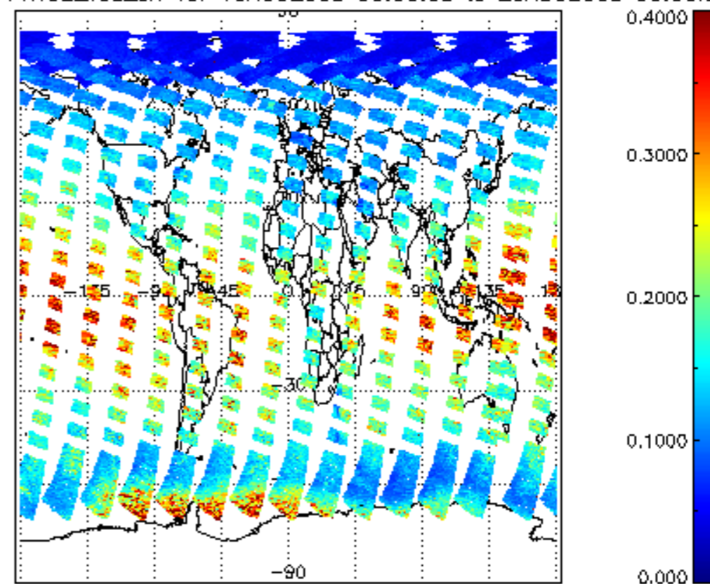
SCIOL2P_NADUV1NO2_vcd_err for 19AUG2009 00:00:00 to 20AUG2009 00:00:00
