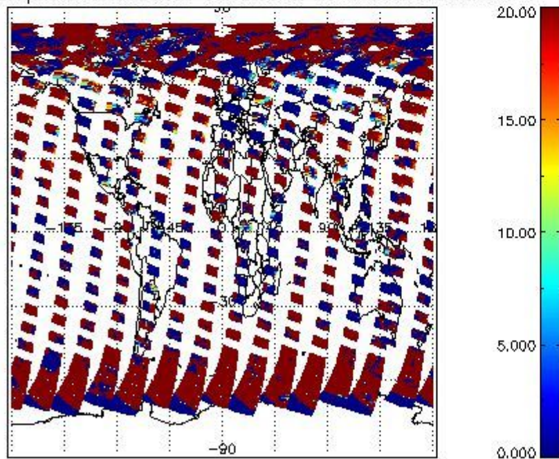
cL_opt_depth for 19AUG2009 00:00:00 to 20AUG2009 00:00:00
