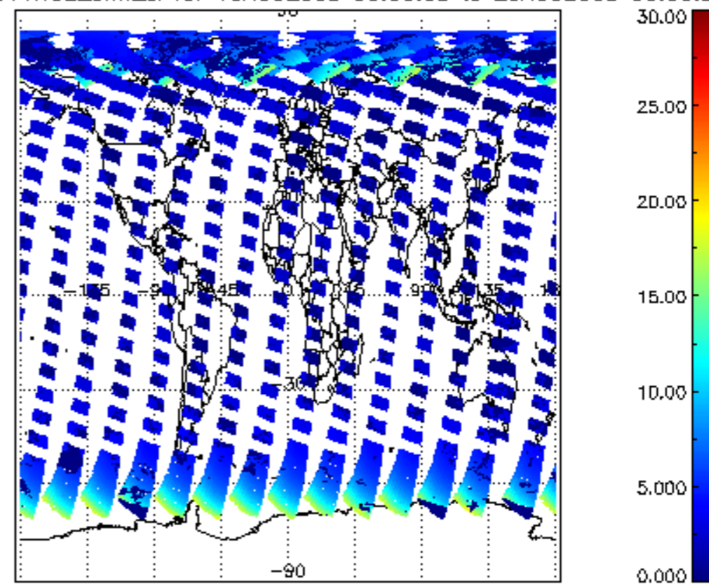
SCIOL2P_NADUV1NO2_amf_cl for 19AUG2009 00:00:00 to 20AUG2009 00:00:00
