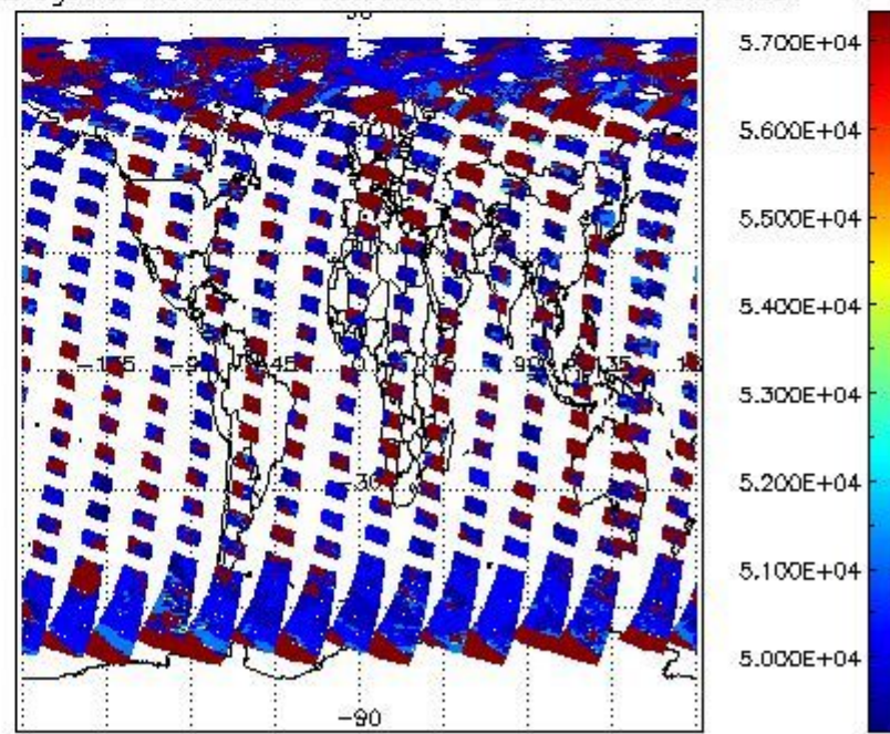
cloud_flags for 19AUG2009 00:00:00 to 20AUG2009 00:00:00
