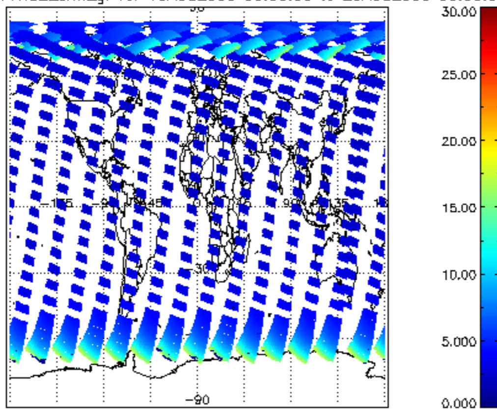
SCIOL2P_NADUV1NO2_amf_gr for 19AUG2009 00:00:00 to 20AUG2009 00:00:00
