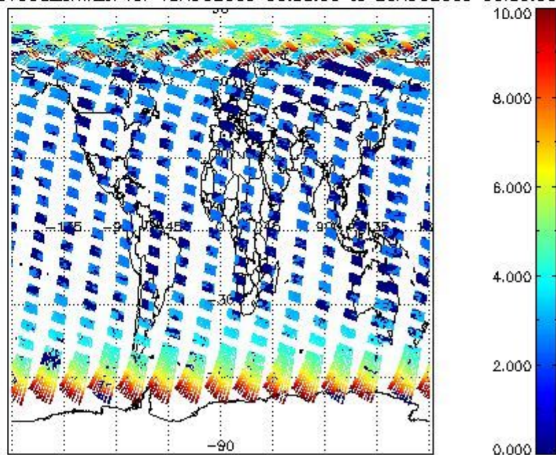
SCIOL2P_NADUV003_amf_gr for 19AUG2009 00:00:00 to 20AUG2009 00:00:00 SCIOL2P_NADUV003_amf_cl for 19AUG2009 00:00:00 to 20AUG2009 00:00:00
