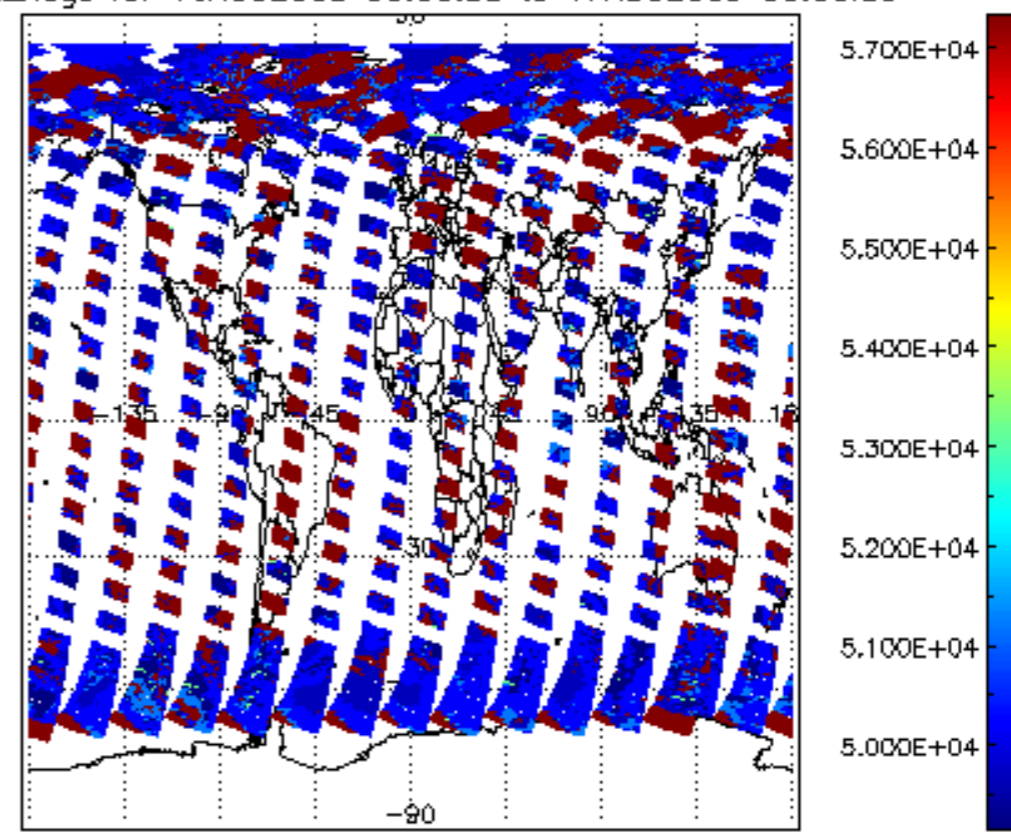
cloud_flags for 16AUG2009 00:00:00 to 17AUG2009 00:00:00
