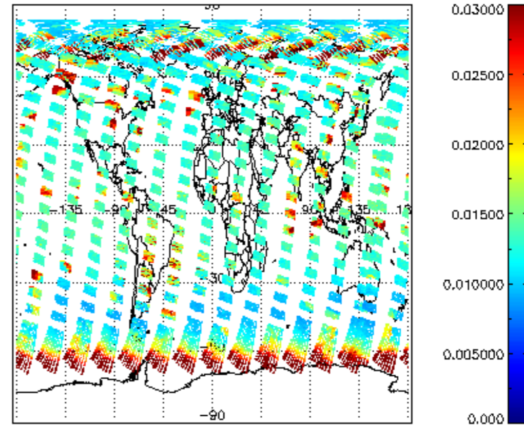
SCIOL2P_NADUV003_vcd_err for 16AUG2009 00:00:00 to 17AUG2009 00:00:00
