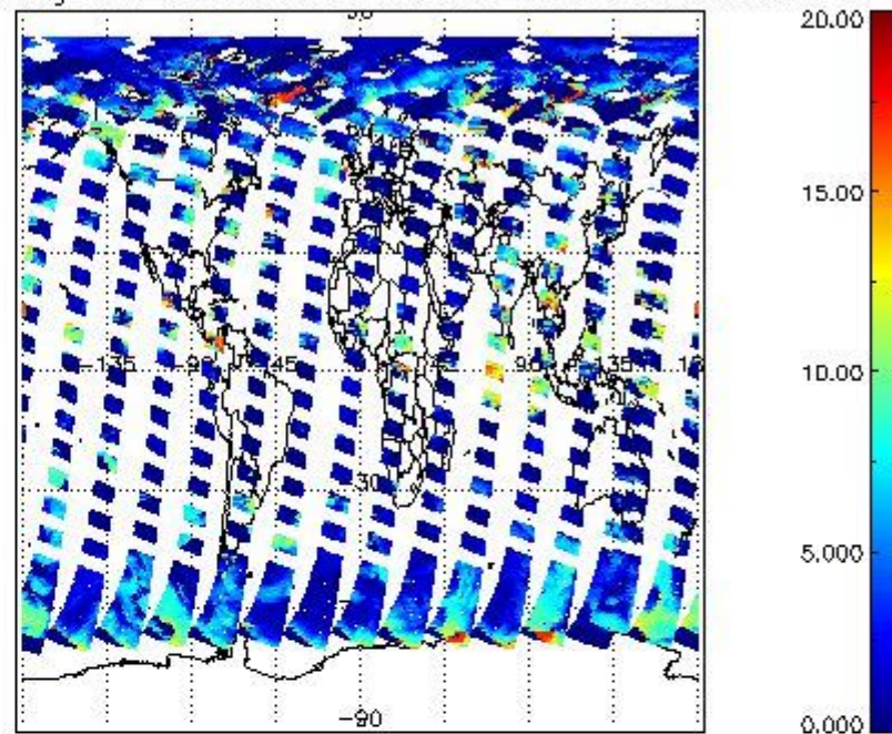
cL_top_height for 16AUG2009 00:00:00 to 17AUG2009 00:00:00
