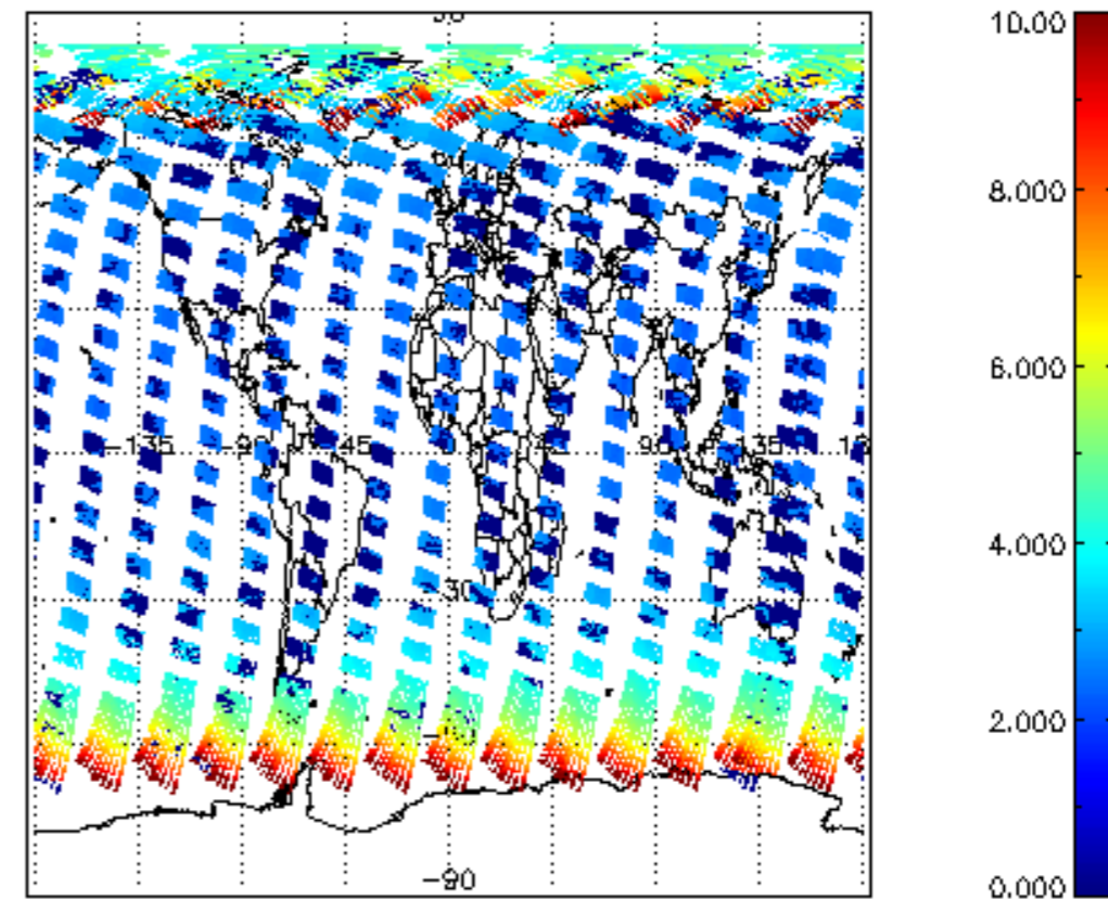
SCIOL2P_NADUV003_amf_cl for 16AUG2009 00:00:00 to 17AUG2009 00:00:00
