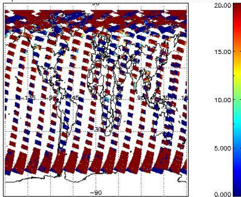
cL_opt_depth for 16AUG2009 00:00:00 to 17AUG2009 00:00:00
