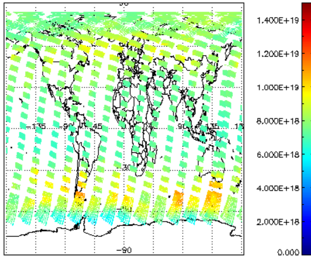
SCIOL2P_NADUV003_vcd for 16AUG2009 00:00:00 to 17AUG2009 00:00:00
