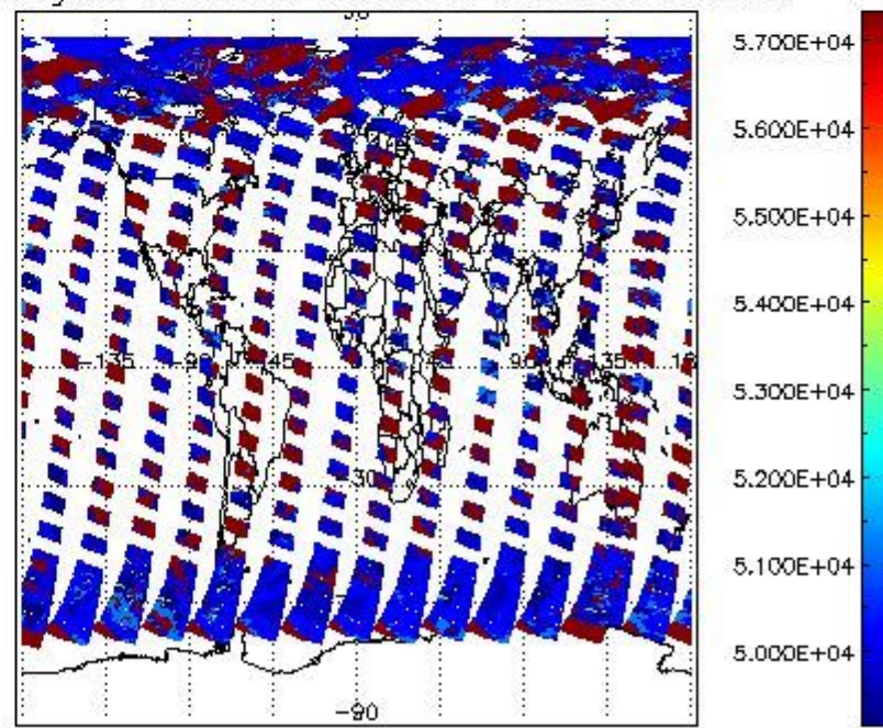
cloud_flags for 16AUG2009 00:00:00 to 17AUG2009 00:00:00
