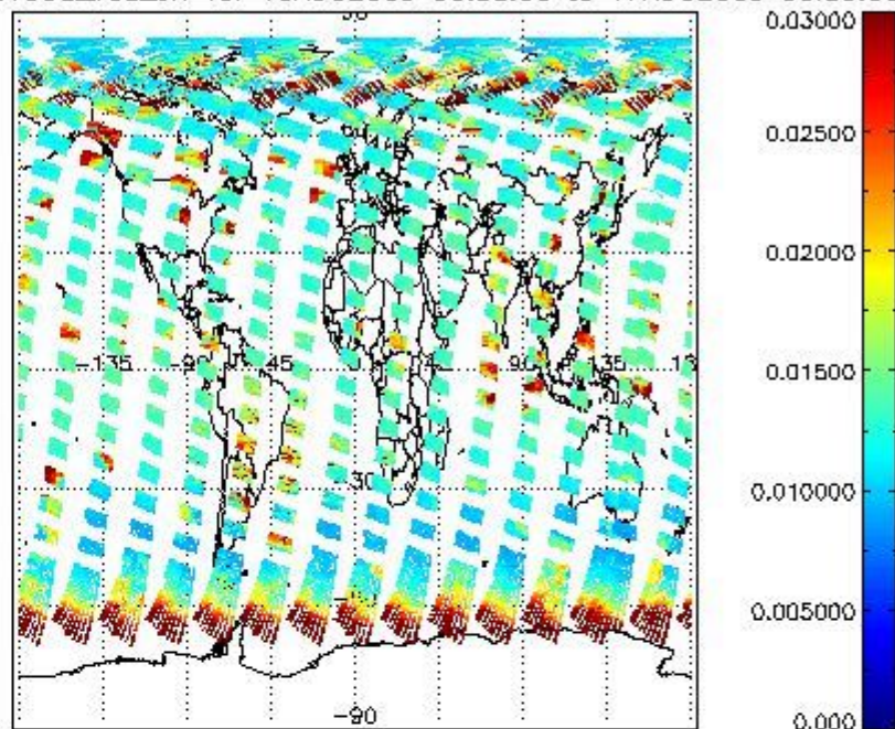
SCIOL2P_NADUV003_vcd_err for 16AUG2009 00:00:00 to 17AUG2009 00:00:00
