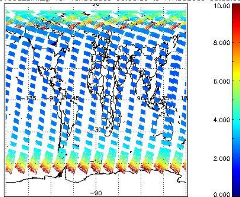
SCIOL2P_NADUV003_amf_gr for 16AUG2009 00:00:00 to 17AUG2009 00:00:00
