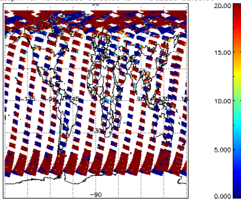
cL_opt_depth for 16AUG2009 00:00:00 to 17AUG2009 00:00:00
