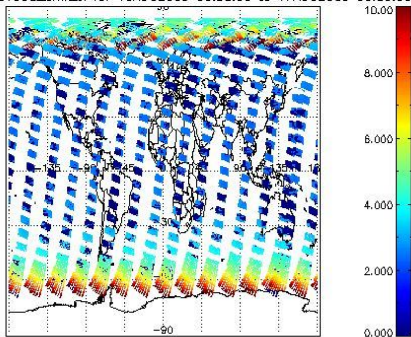
SCIOL2P_NADUV003_amf_cl for 16AUG2009 00:00:00 to 17AUG2009 00:00:00
