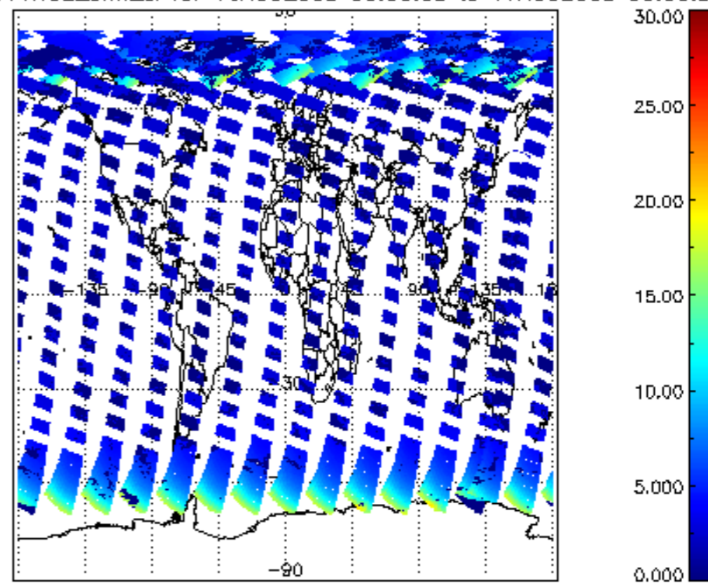
ICIOL2P_NADUV1NO2_amf_cl for 16AUG2009 00:00:00 to 17AUG2009 00:00:00
