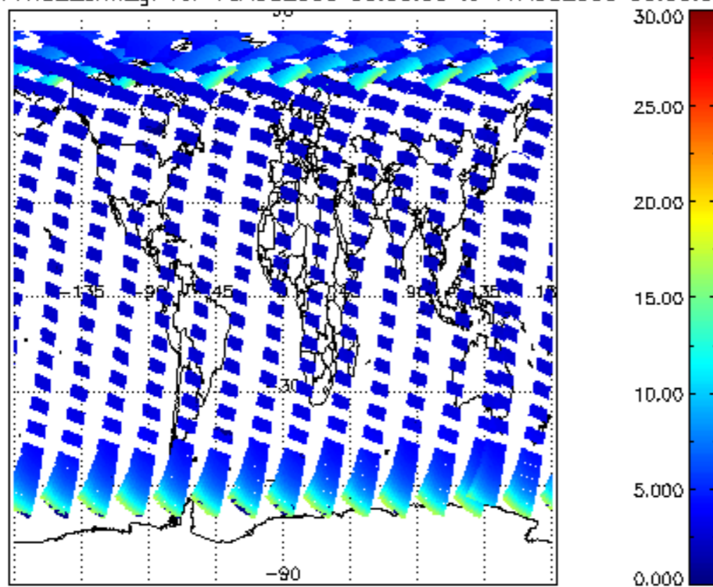
ICIOL2P_NADUV1NO2_amf_gr for 16AUG2009 00:00:00 to 17AUG2009 00:00:00
