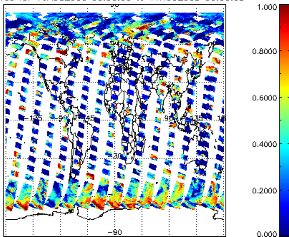
cL_frac for 16AUG2009 00:00:00 to 17AUG2009 00:00:00
