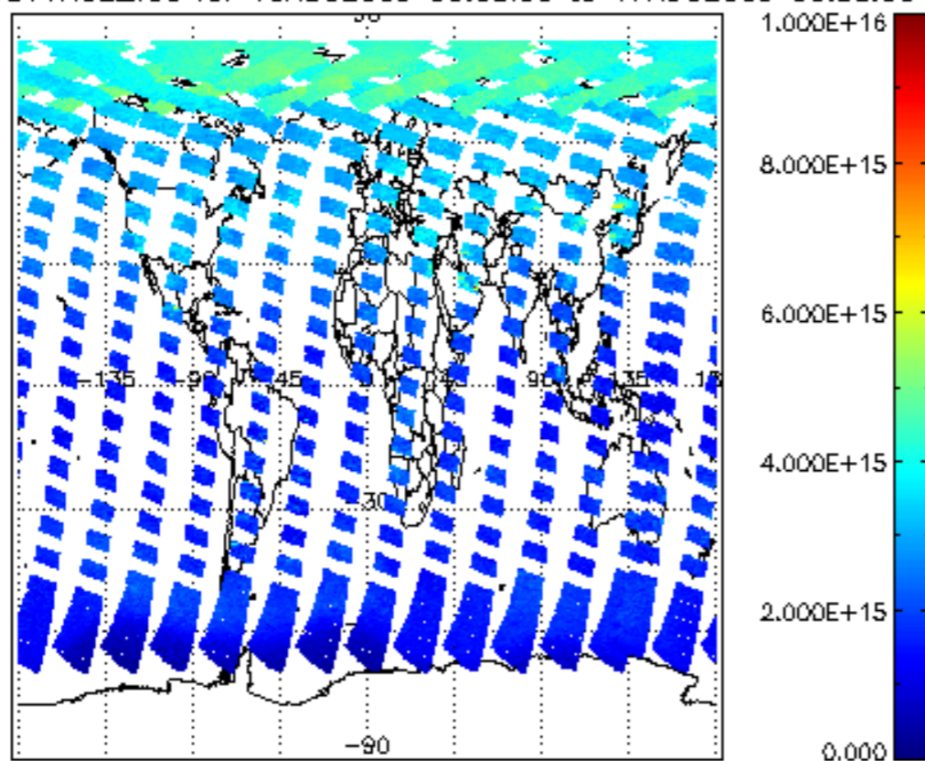
SCIOL2P_NADUV1NO2_vcd for 16AUG2009 00:00:00 to 17AUG2009 00:00:00
