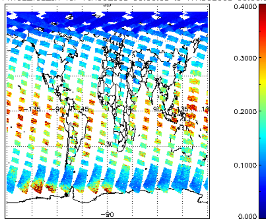
SCIOL2P_NADUV1NO2_vcd_err for 16AUG2009 00:00:00 to 17AUG2009 00:00:00
