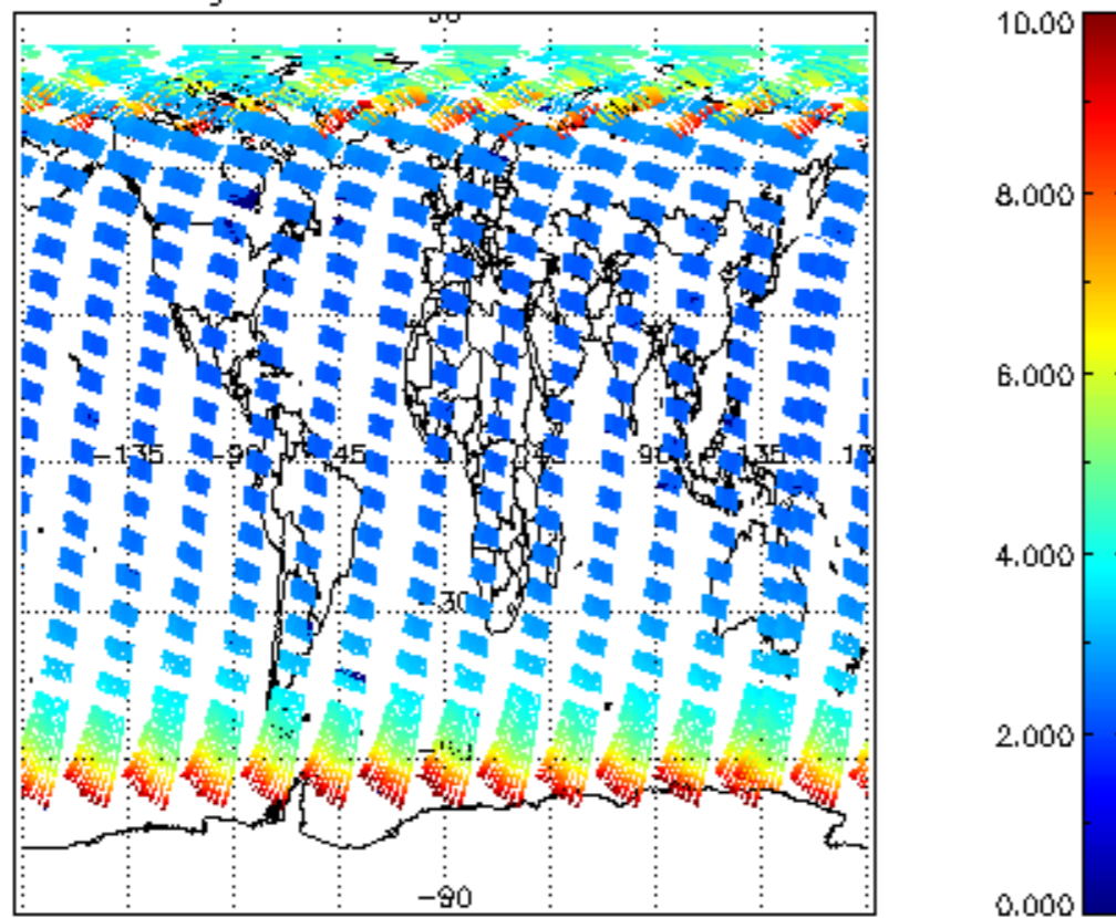
SCIOL2P_NADUV003_amf_gr for 16AUG2009 00:00:00 to 17AUG2009 00:00:00
