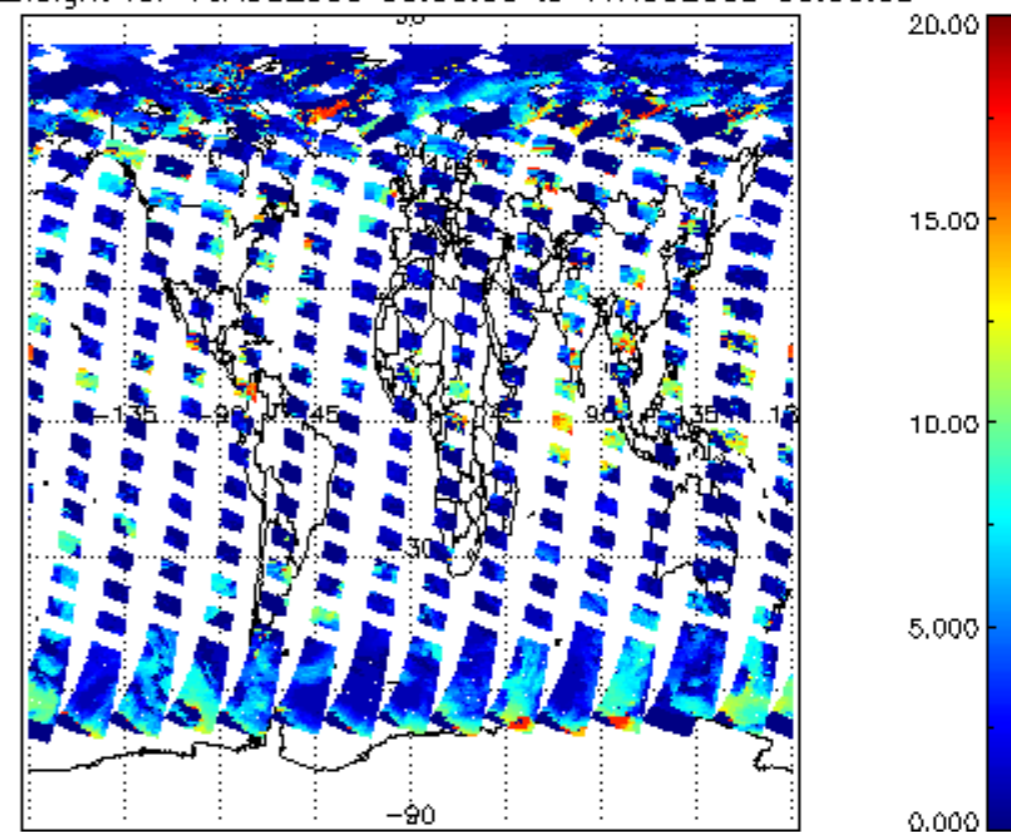
cL_top_height for 16AUG2009 00:00:00 to 17AUG2009 00:00:00
