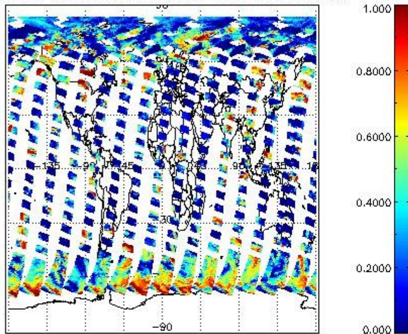
cL_frac for 16AUG2009 00:00:00 to 17AUG2009 00:00:00
