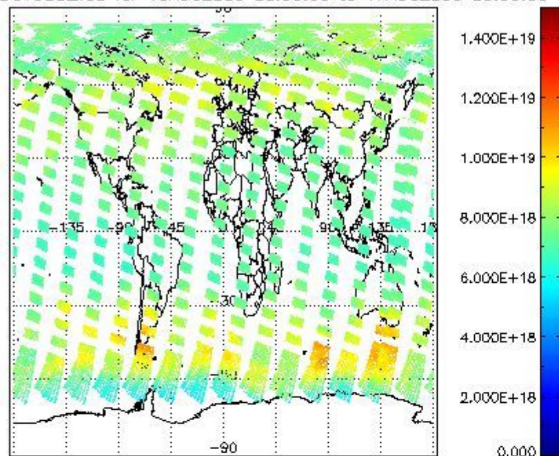
SCIOL2P_NADUV003_vcd for 16AUG2009 00:00:00 to 17AUG2009 00:00:00
