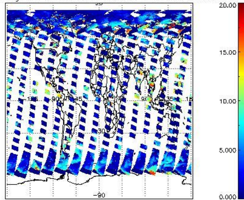
cL_top_height for 13AUG2009 00:00:00 to 14AUG2009 00:00:00
