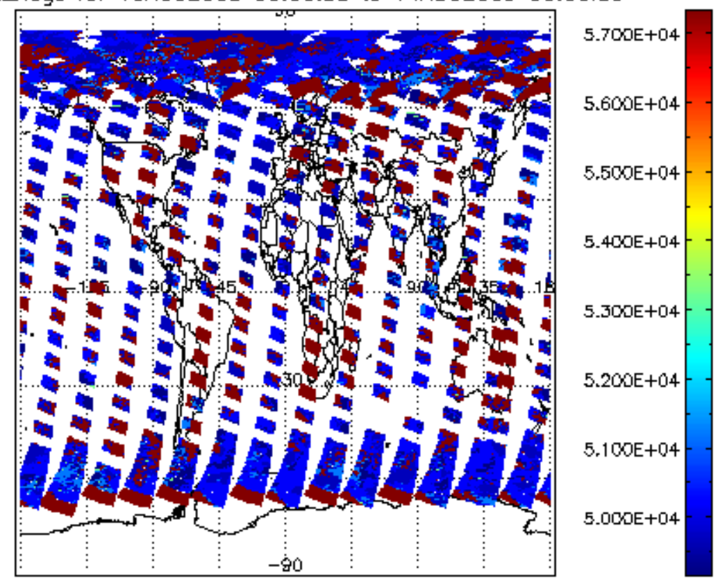
cloud_flags for 13AUG2009 00:00:00 to 14AUG2009 00:00:00
