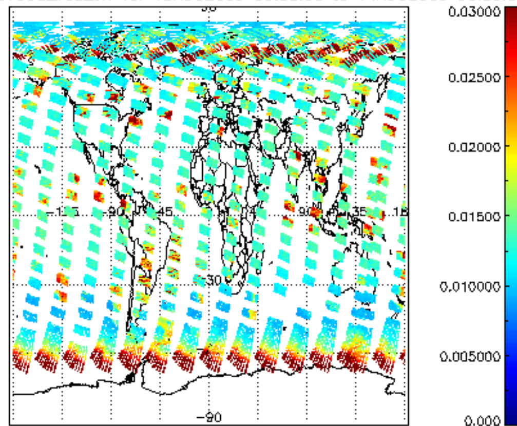
SCIOL2P_NADUV003_vcd_err for 13AUG2009 00:00:00 to 14AUG2009 00:00:00
