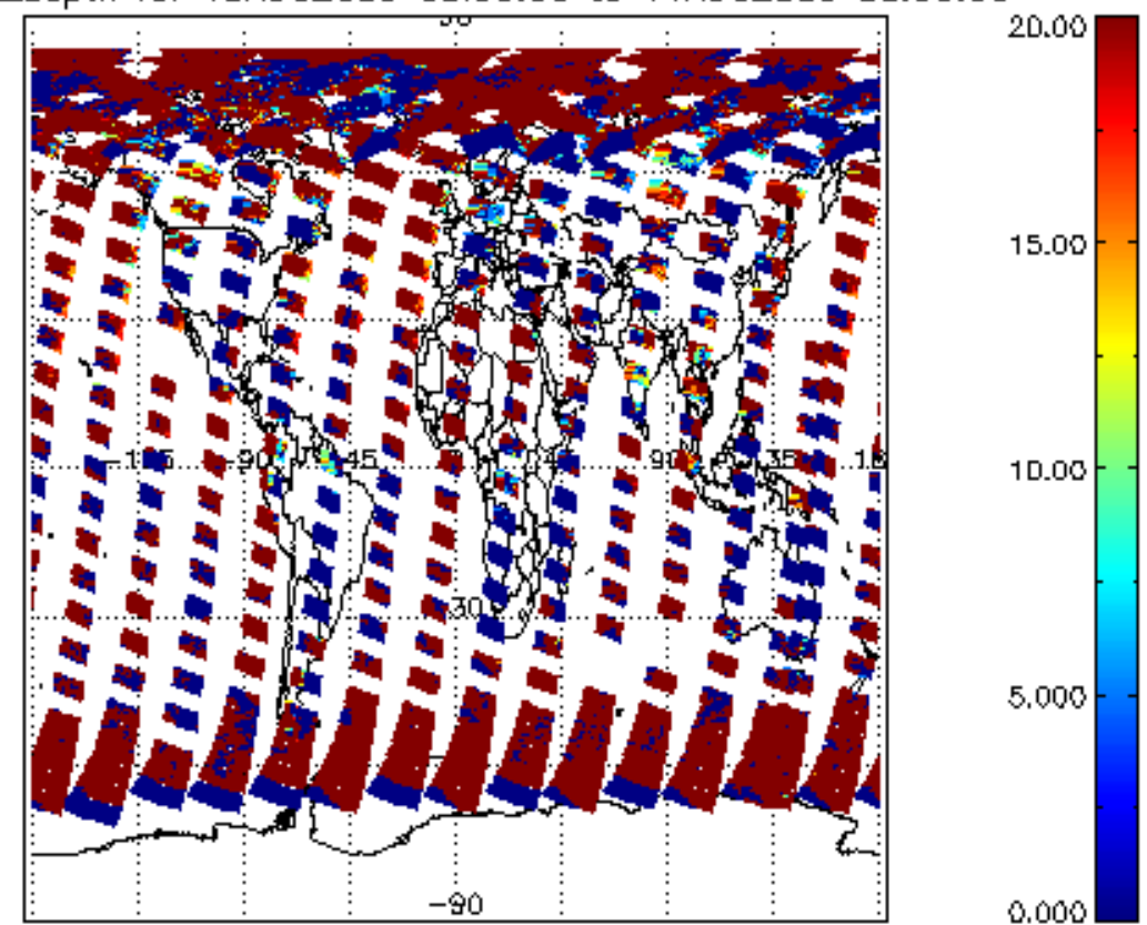
cL_opt_depth for 13AUG2009 00:00:00 to 14AUG2009 00:00:00
