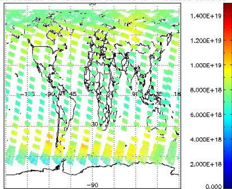
SCIOL2P_NADUV003_vcd for 13AUG2009 00:00:00 to 14AUG2009 00:00:00
