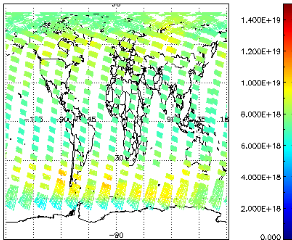
SCIOL2P_NADUV003_vcd for 13AUG2009 00:00:00 to 14AUG2009 00:00:00
