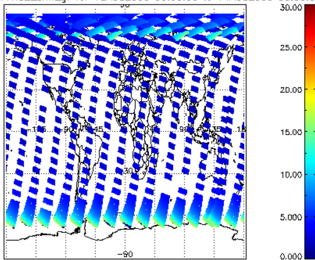
SCIOL2P_NADUV1NO2_amf_gr for 13AUG2009 00:00:00 to 14AUG2009 00:00:00
