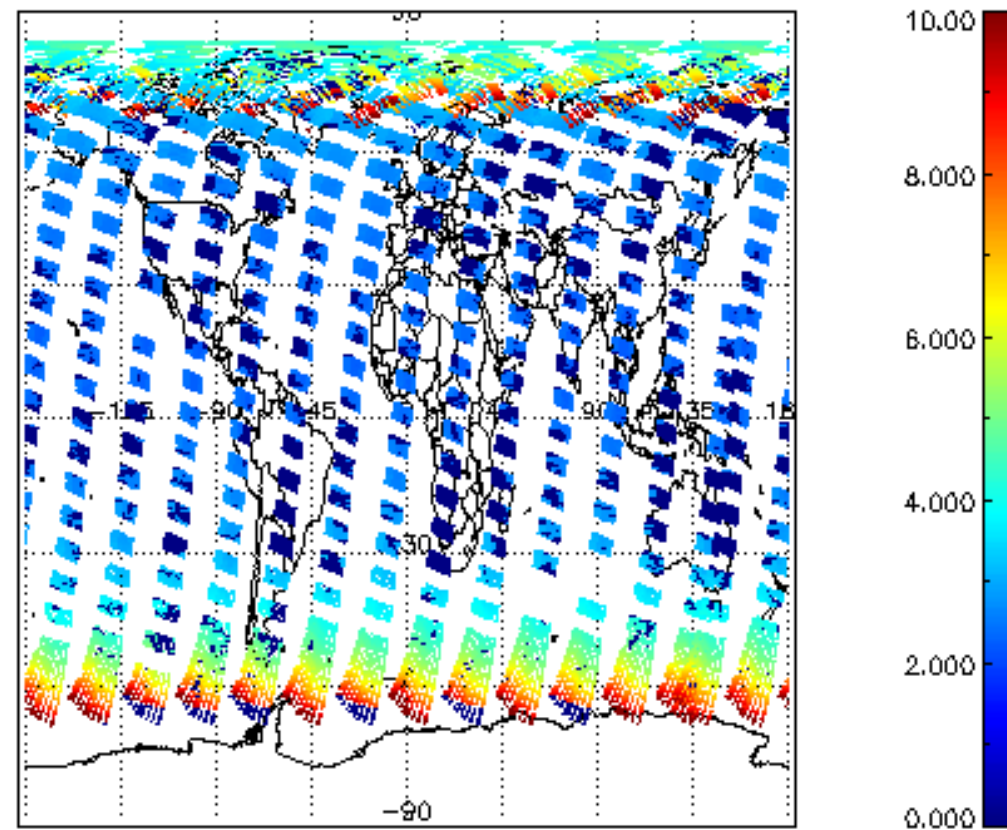
SCIOL2P_NADUV003_amf_cl for 13AUG2009 00:00:00 to 14AUG2009 00:00:00
