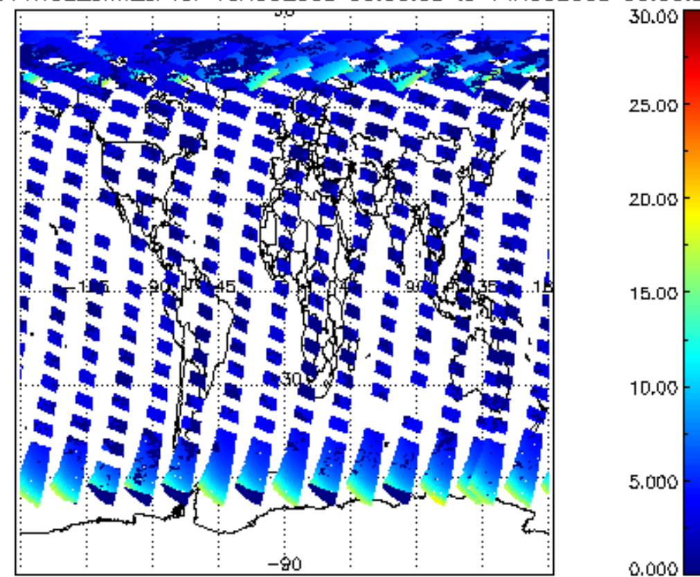
SCIOL2P_NADUV1NO2_amf_cl for 13AUG2009 00:00:00 to 14AUG2009 00:00:00
