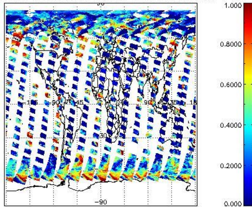
cL_frac for 13AUG2009 00:00:00 to 14AUG2009 00:00:00
