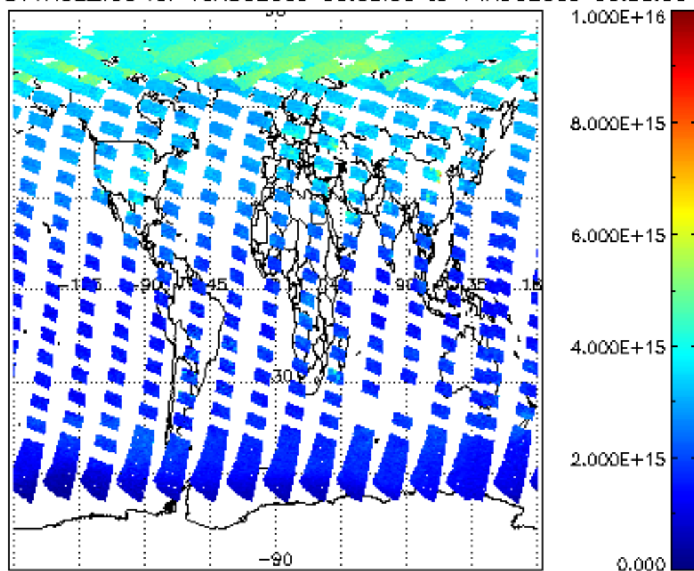
SCIOL2P_NADUV1NO2_vcd for 13AUG2009 00:00:00 to 14AUG2009 00:00:00
