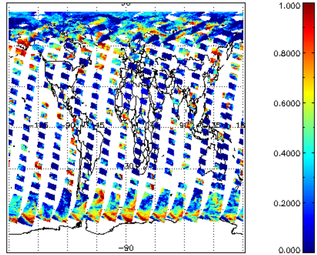
cL_frac for 13AUG2009 00:00:00 to 14AUG2009 00:00:00
