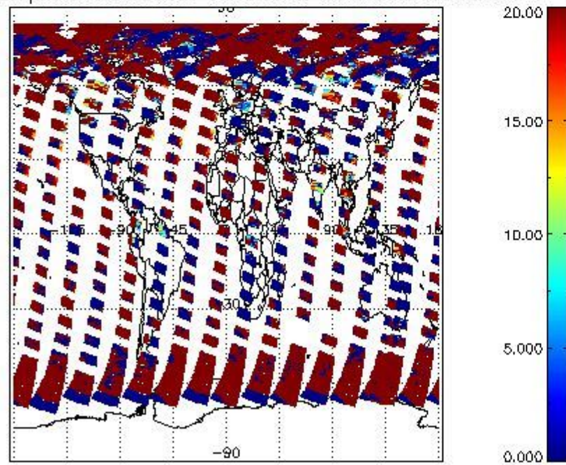
cL_opt_depth for 13AUG2009 00:00:00 to 14AUG2009 00:00:00
