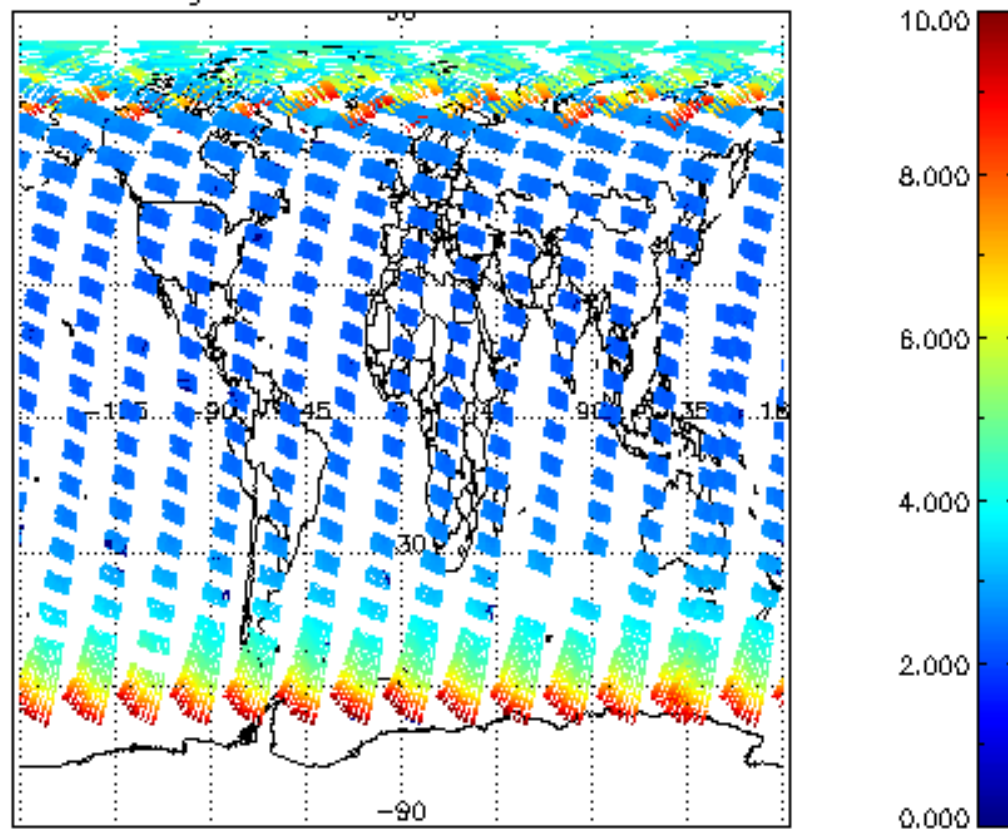
SCIOL2P_NADUV003_amf_gr for 13AUG2009 00:00:00 to 14AUG2009 00:00:00
