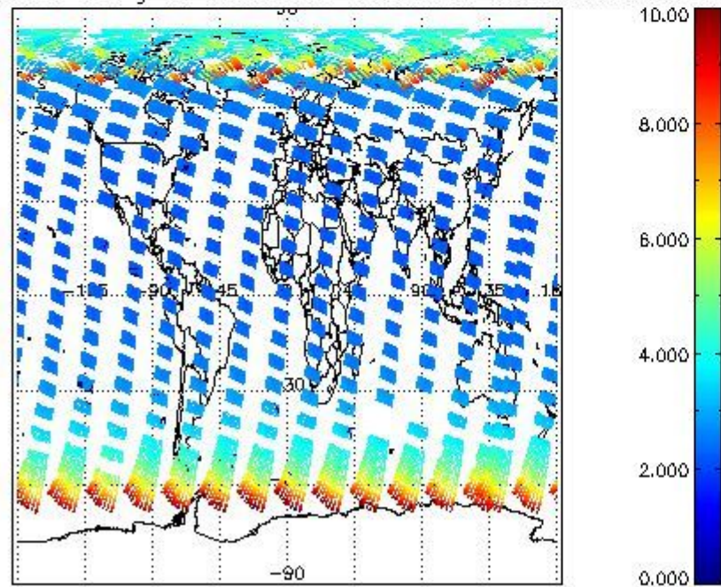
SCIOL2P_NADUV003_amf_gr for 13AUG2009 00:00:00 to 14AUG2009 00:00:00
