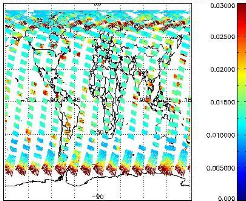
SCIOL2P_NADUV003_vcd_err for 13AUG2009 00:00:00 to 14AUG2009 00:00:00
