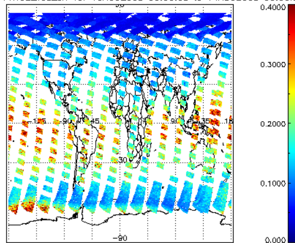
SCIOL2P_NADUV1NO2_vcd_err for 13AUG2009 00:00:00 to 14AUG2009 00:00:00
