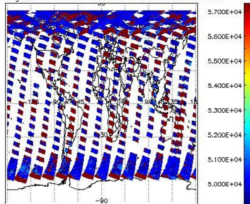
cloud_flags for 13AUG2009 00:00:00 to 14AUG2009 00:00:00
