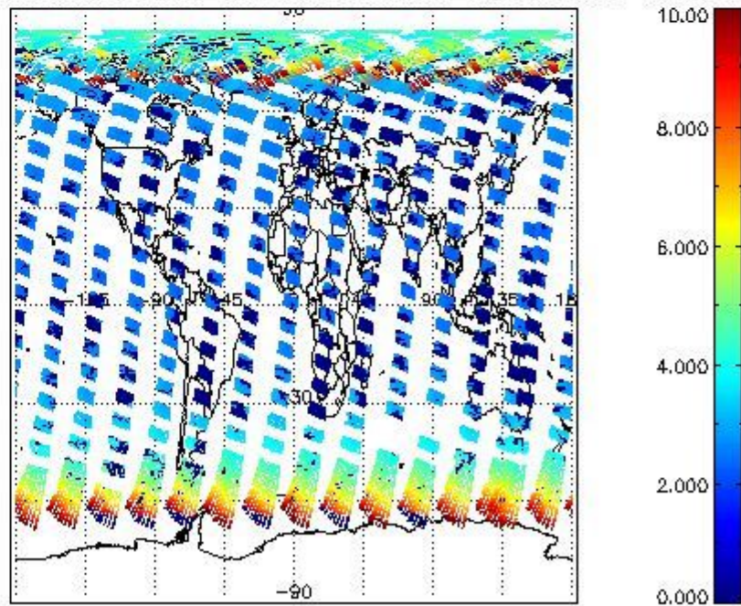
SCIOL2P_NADUV003_amf_cl for 13AUG2009 00:00:00 to 14AUG2009 00:00:00
