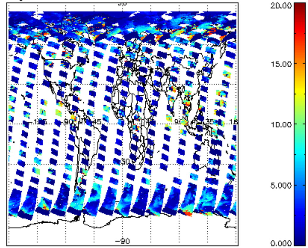
cL_top_height for 13AUG2009 00:00:00 to 14AUG2009 00:00:00
