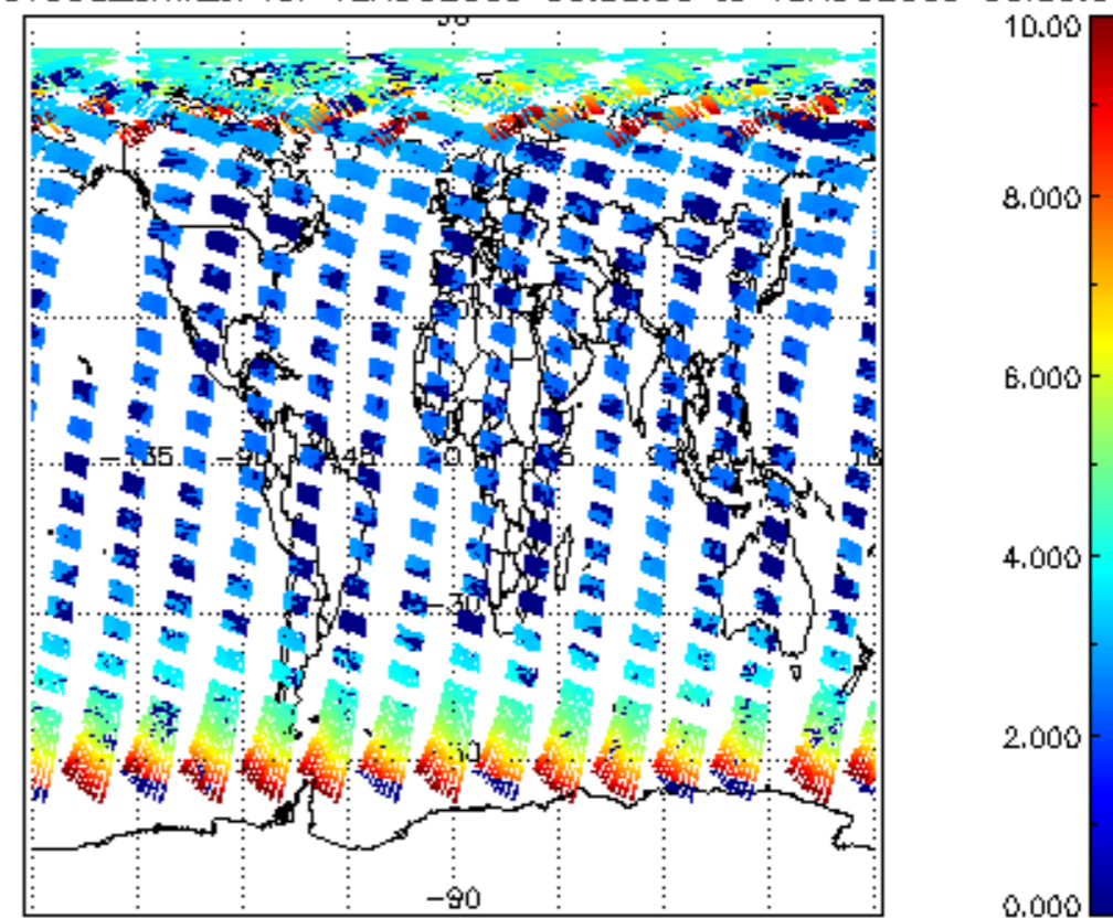
SCIOL2P_NADUV003_amf_cl for 12AUG2009 00:00:00 to 13AUG2009 00:00:00
