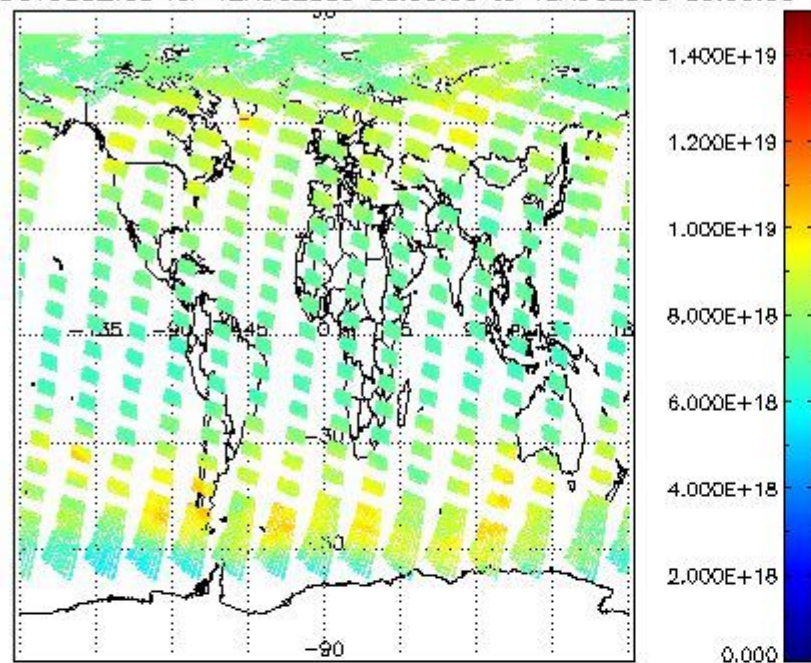
SCIOL2P_NADUV003_vcd for 12AUG2009 00:00:00 to 13AUG2009 00:00:00
