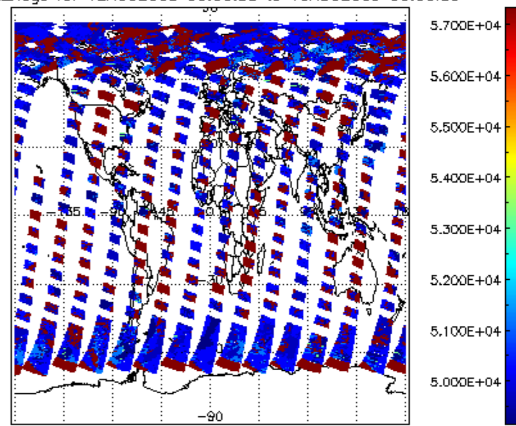
cloud_flags for 12AUG2009 00:00:00 to 13AUG2009 00:00:00
