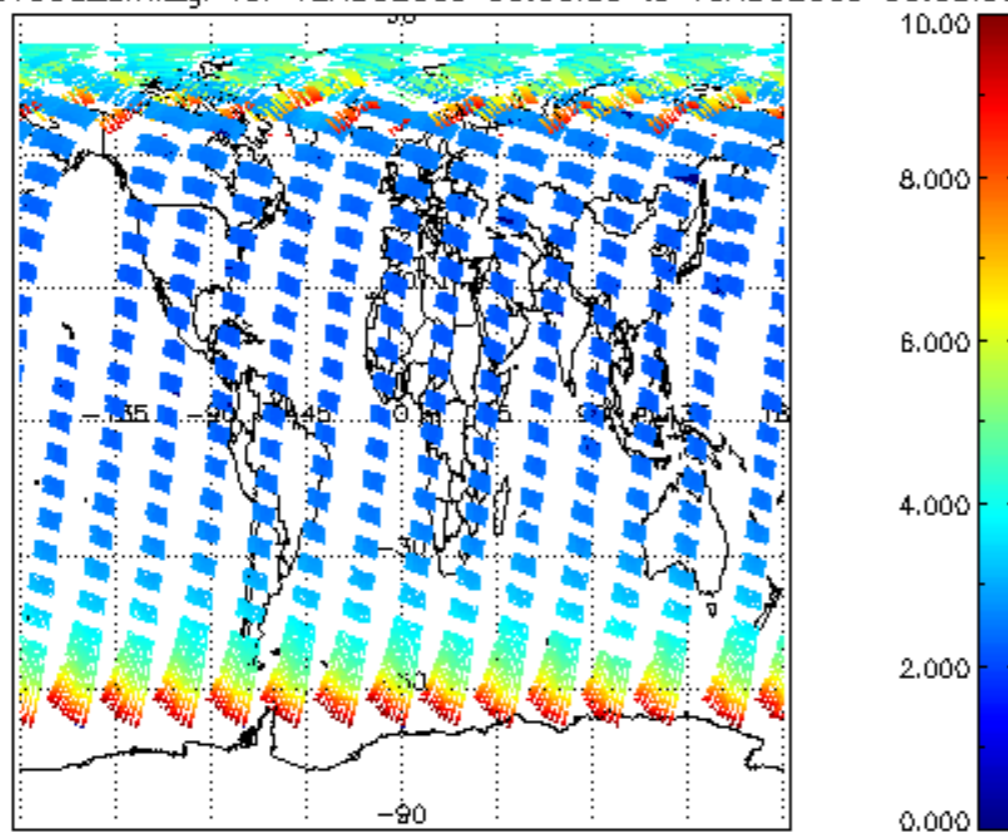
SCIOL2P_NADUV003_amf_gr for 12AUG2009 00:00:00 to 13AUG2009 00:00:00
