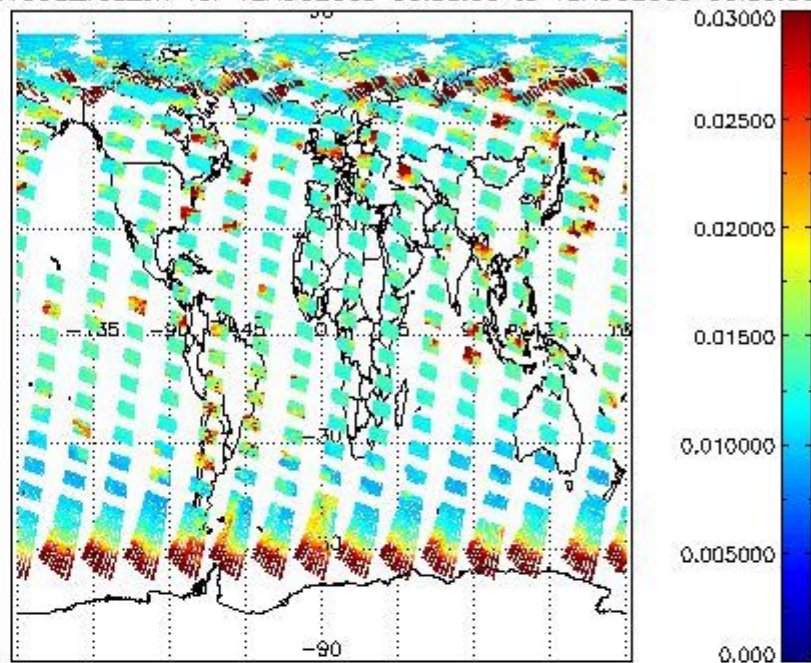
SCIOL2P_NADUV003_vcd_err for 12AUG2009 00:00:00 to 13AUG2009 00:00:00
