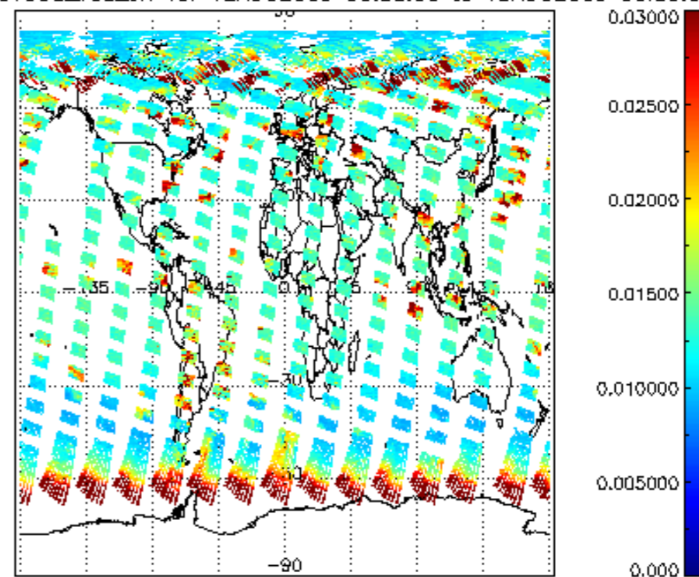
SCIOL2P_NADUV003_vcd_err for 12AUG2009 00:00:00 to 13AUG2009 00:00:00
