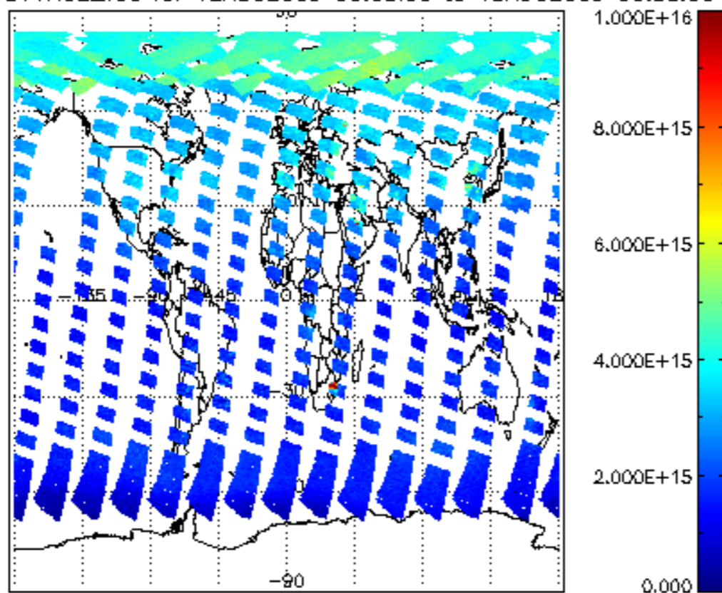
SCIOL2P_NADUV1NO2_vcd for 12AUG2009 00:00:00 to 13AUG2009 00:00:00
