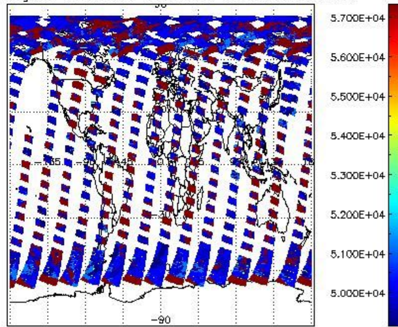
cloud_flags for 12AUG2009 00:00:00 to 13AUG2009 00:00:00
