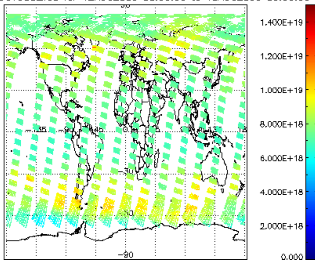
SCIOL2P_NADUV003_vcd for 12AUG2009 00:00:00 to 13AUG2009 00:00:00
