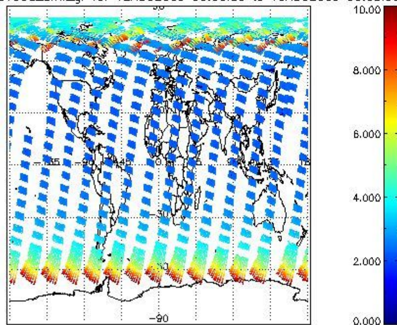
SCIOL2P_NADUV003_amf_gr for 12AUG2009 00:00:00 to 13AUG2009 00:00:00
