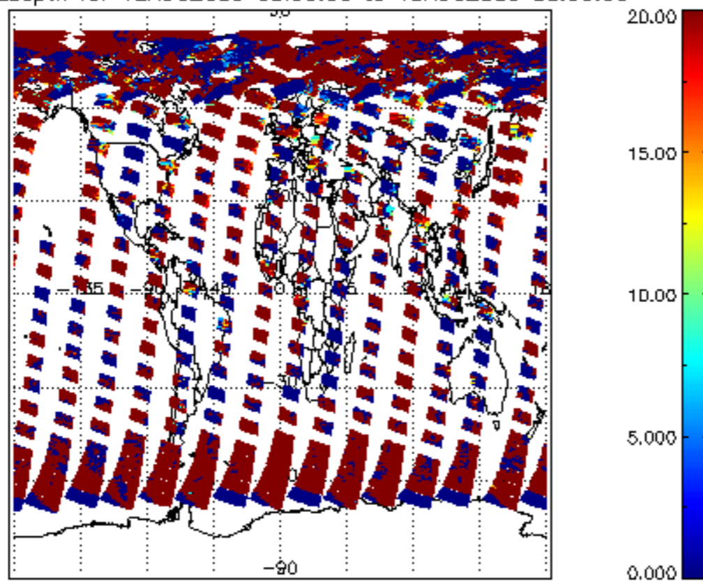
cL_opt_depth for 12AUG2009 00:00:00 to 13AUG2009 00:00:00
