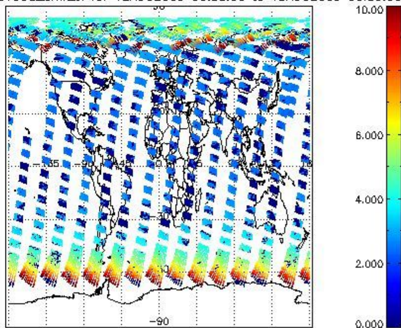
SCIOL2P_NADUV003_amf_cl for 12AUG2009 00:00:00 to 13AUG2009 00:00:00
