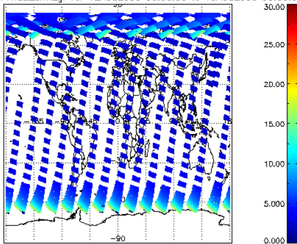
SCIOL2P_NADUV1NO2_amf_gr for 12AUG2009 00:00:00 to 13AUG2009 00:00:00
