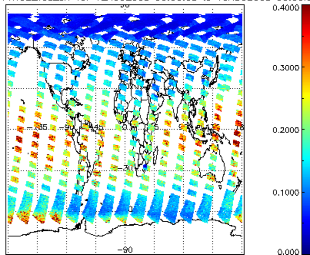
SCIOL2P_NADUV1NO2_vcd_err for 12AUG2009 00:00:00 to 13AUG2009 00:00:00
