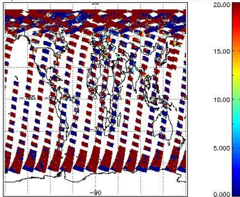
cL_opt_depth for 12AUG2009 00:00:00 to 13AUG2009 00:00:00
