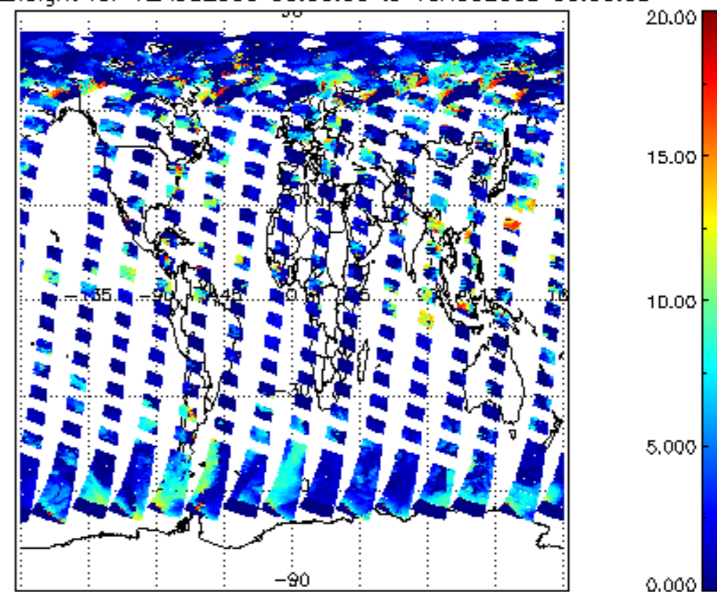
cL_top_height for 12AUG2009 00:00:00 to 13AUG2009 00:00:00
