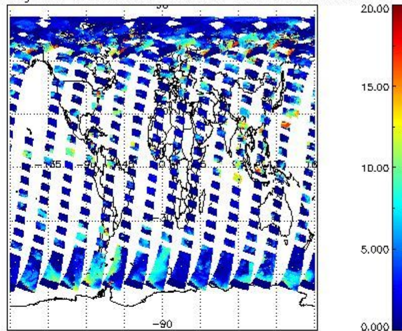
cL_top_height for 12AUG2009 00:00:00 to 13AUG2009 00:00:00
