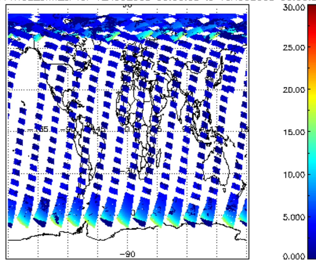
SCIOL2P_NADUV1NO2_amf_cl for 12AUG2009 00:00:00 to 13AUG2009 00:00:00
