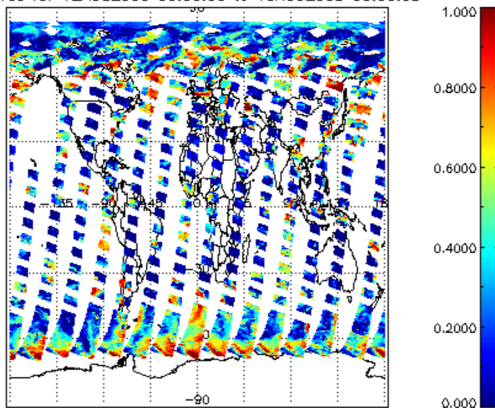
cL_frac for 12AUG2009 00:00:00 to 13AUG2009 00:00:00
