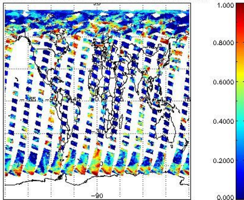
cL_frac for 12AUG2009 00:00:00 to 13AUG2009 00:00:00
