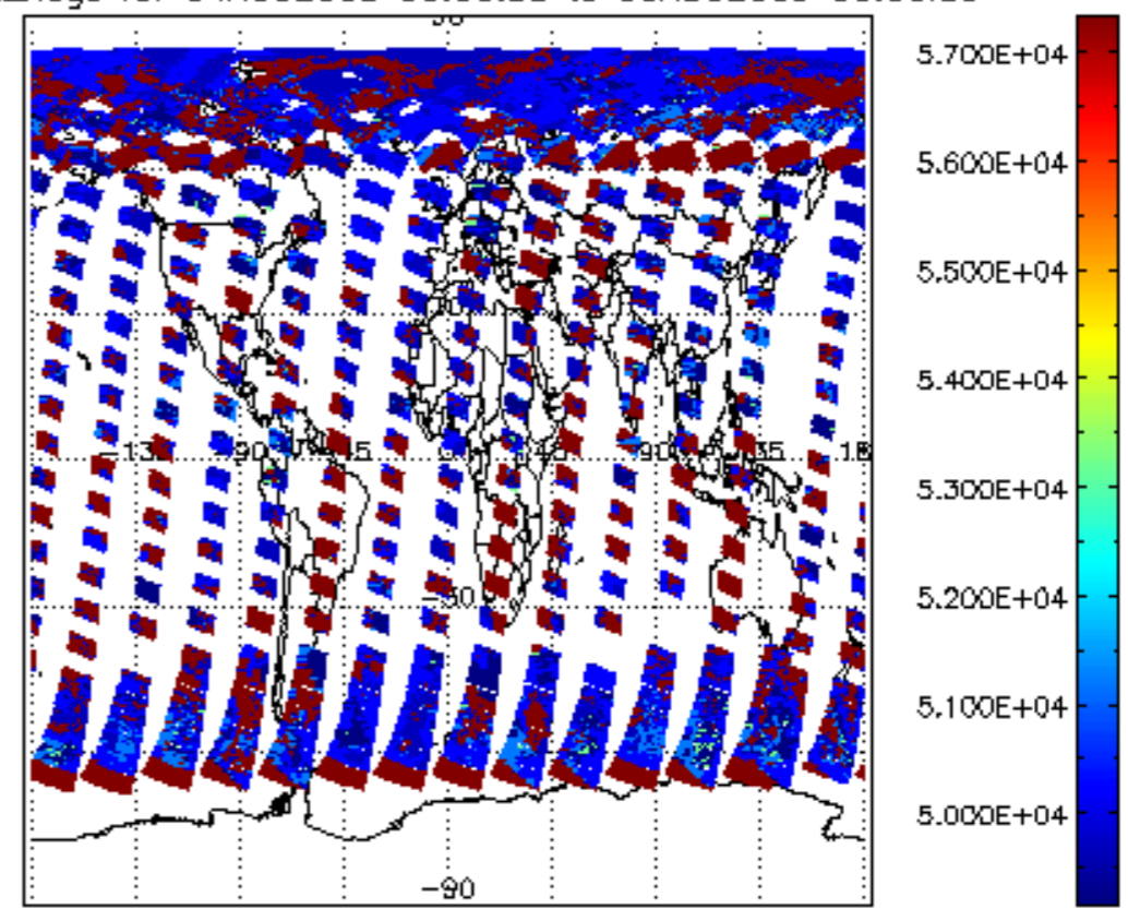
cloud_flags for 04AUG2009 00:00:00 to 05AUG2009 00:00:00
