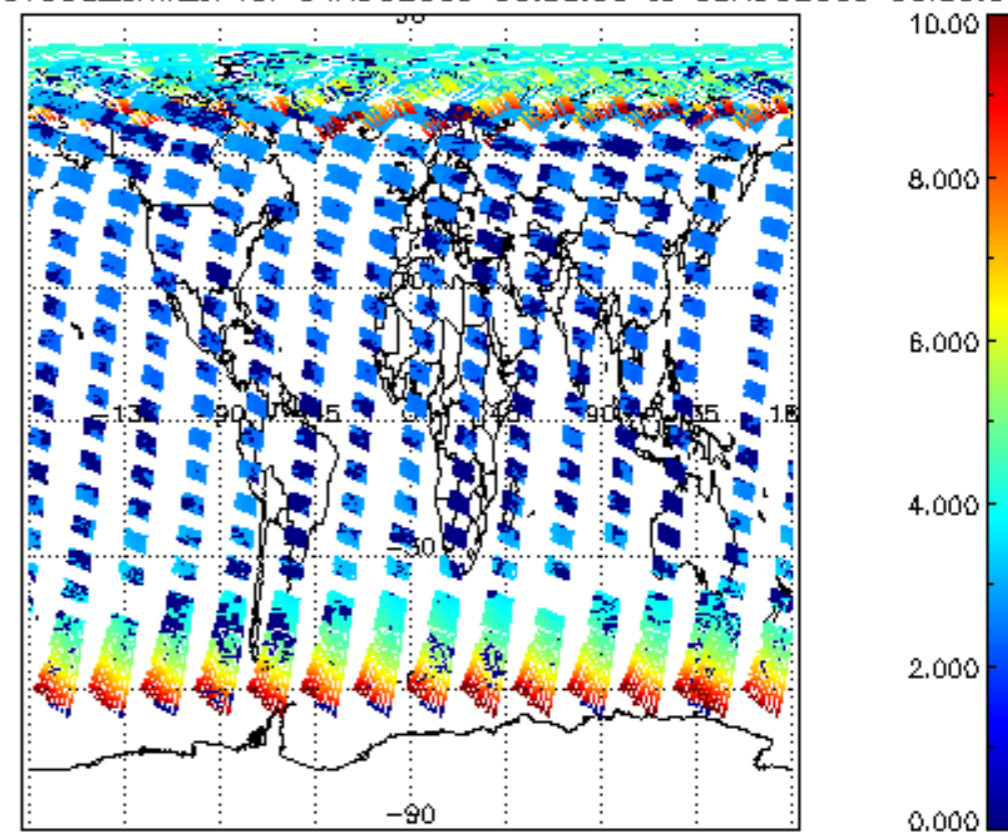
SCIOL2P_NADUV003_amf_cl for 04AUG2009 00:00:00 to 05AUG2009 00:00:00
