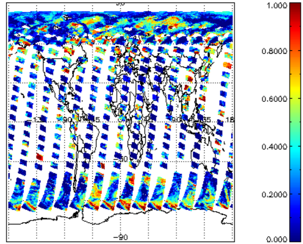
cL_frac for 04AUG2009 00:00:00 to 05AUG2009 00:00:00
