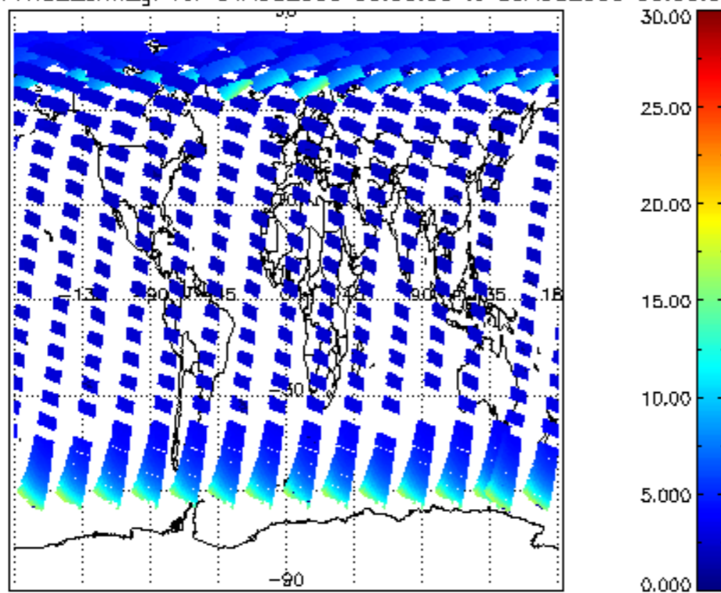
SCIOL2P_NADUV1NO2_amf_gr for 04AUG2009 00:00:00 to 05AUG2009 00:00:00
