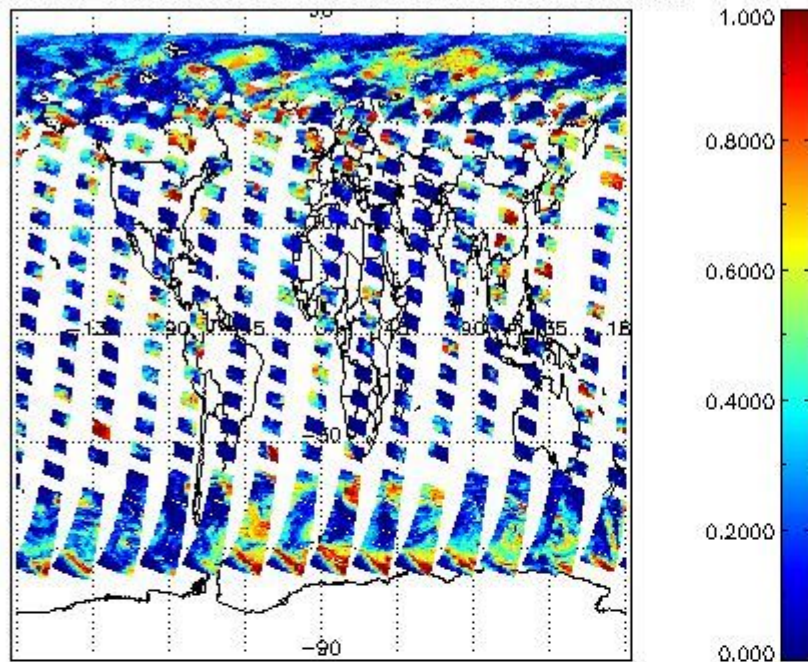
cL_frac for 04AUG2009 00:00:00 to 05AUG2009 00:00:00
