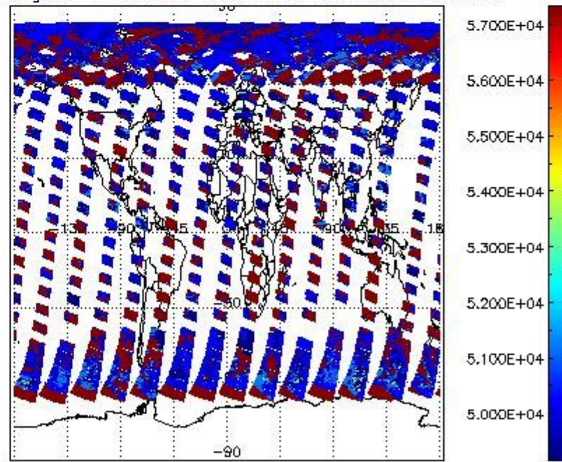
cloud_flags for 04AUG2009 00:00:00 to 05AUG2009 00:00:00
