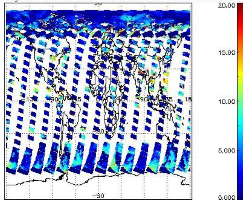
cL_top_height for 04AUG2009 00:00:00 to 05AUG2009 00:00:00
