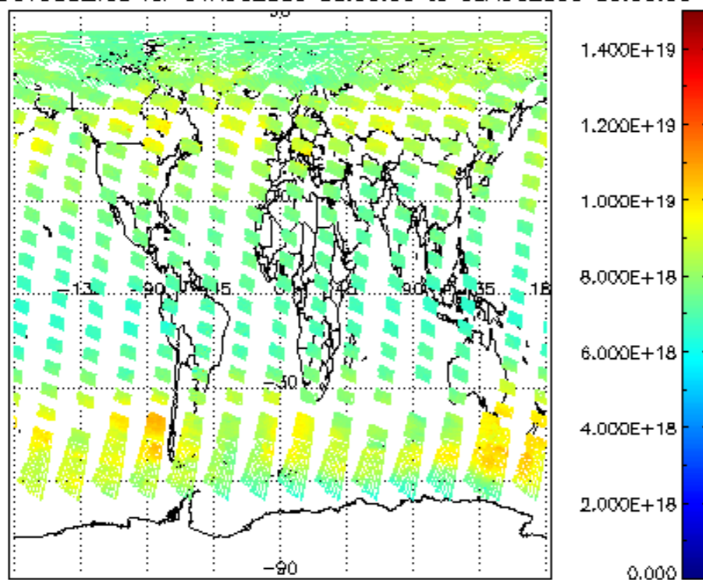
SCIOL2P_NADUV003_vcd for 04AUG2009 00:00:00 to 05AUG2009 00:00:00
