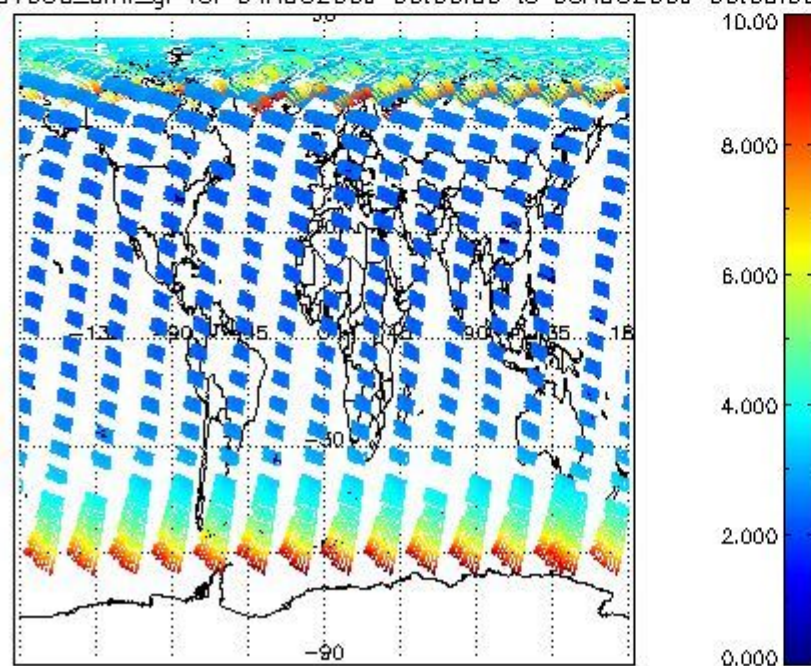
SCIOL2P_NADUV003_amf_gr for 04AUG2009 00:00:00 to 05AUG2009 00:00:00 SCIOL2P_NADUV003_amf_cl for 04AUG2009 00:00:00 to 05AUG2009 00:00:00
