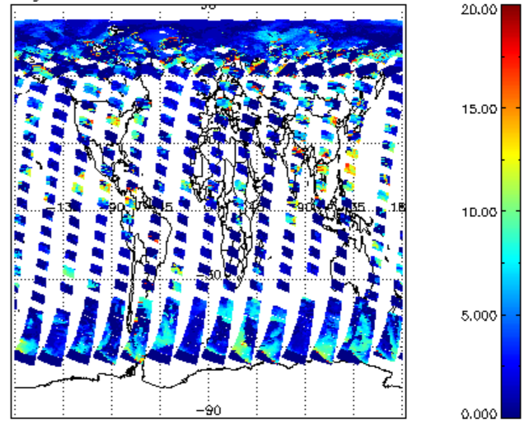
cL_top_height for 04AUG2009 00:00:00 to 05AUG2009 00:00:00
