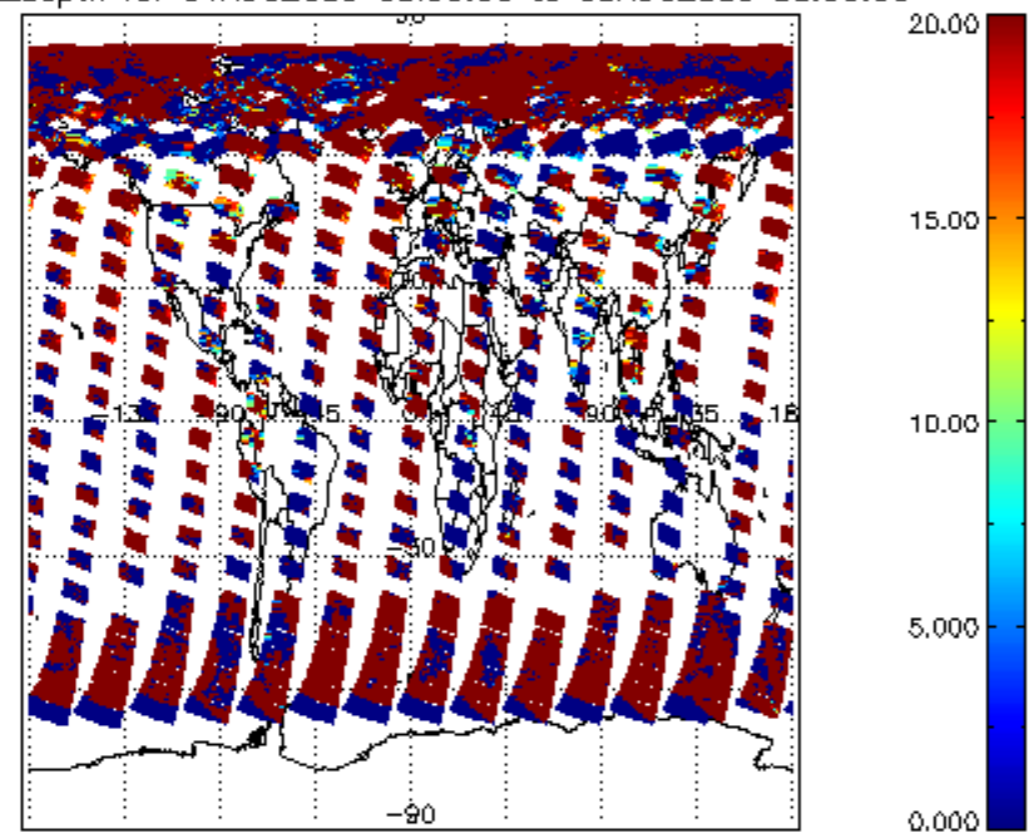
cL_opt_depth for 04AUG2009 00:00:00 to 05AUG2009 00:00:00
