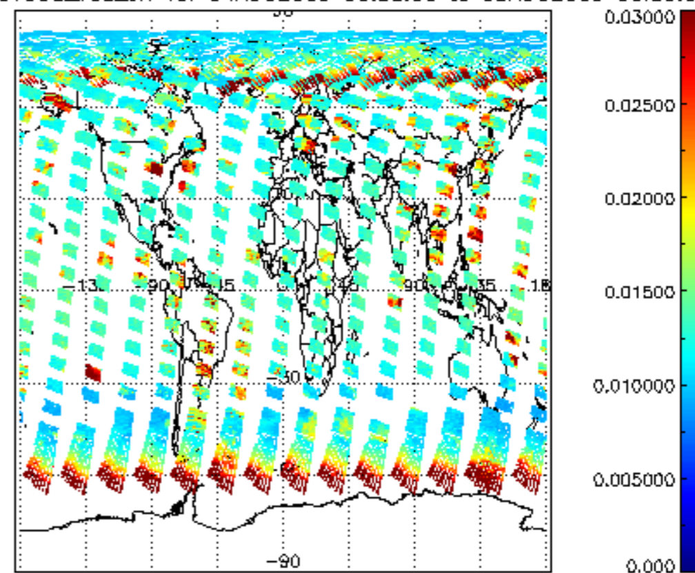
SCIOL2P_NADUV003_vcd_err for 04AUG2009 00:00:00 to 05AUG2009 00:00:00
