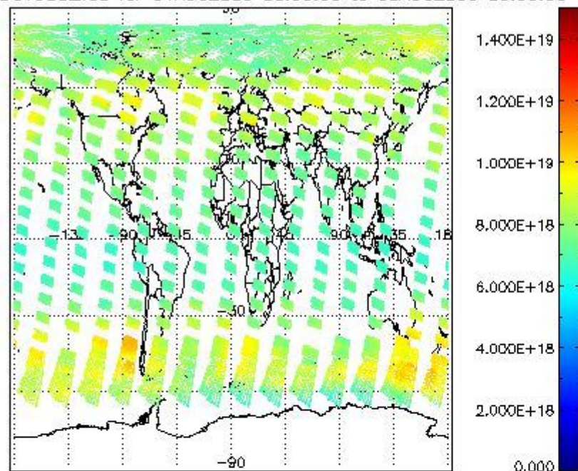
SCIOL2P_NADUV003_vcd for 04AUG2009 00:00:00 to 05AUG2009 00:00:00 SCIOL2P_NADUV003_vcd_err for 04AUG2009 00:00:00 to 05AUG2009 00:00:00
