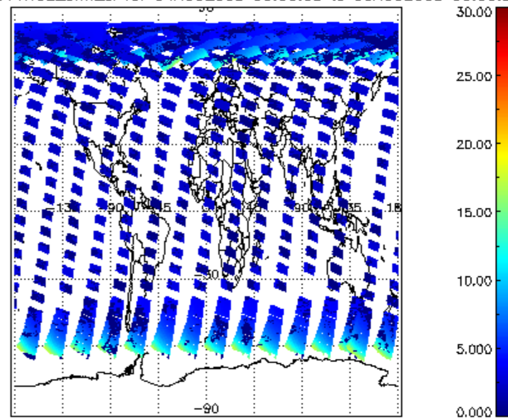
SCIOL2P_NADUV1NO2_amf_cl for 04AUG2009 00:00:00 to 05AUG2009 00:00:00
