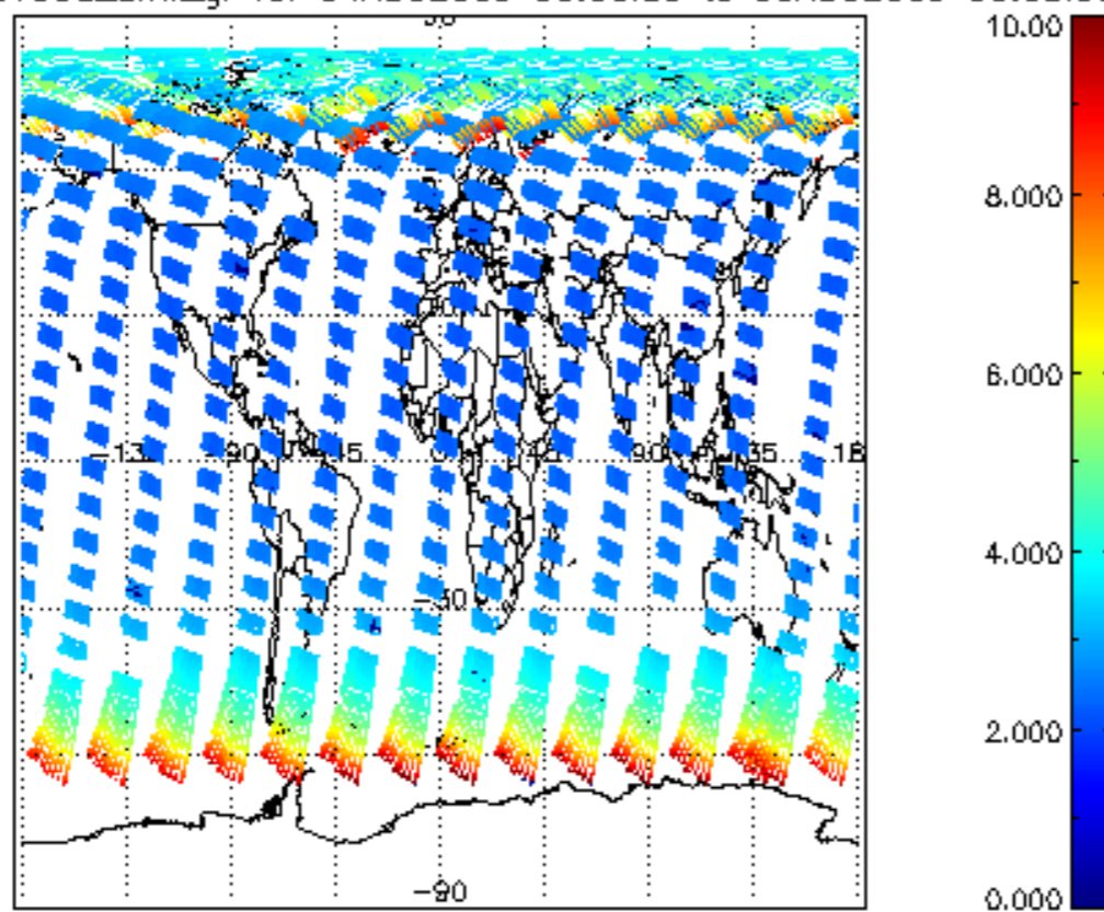
SCIOL2P_NADUV003_amf_gr for 04AUG2009 00:00:00 to 05AUG2009 00:00:00
