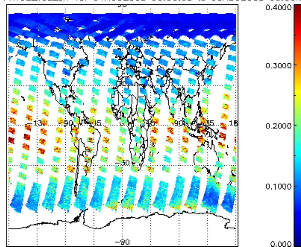
SCIOL2P_NADUV1NO2_vcd_err for 04AUG2009 00:00:00 to 05AUG2009 00:00:00
