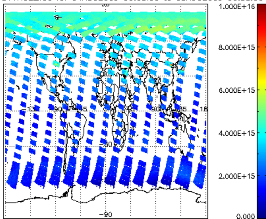
SCIOL2P_NADUV1NO2_vcd for 04AUG2009 00:00:00 to 05AUG2009 00:00:00
