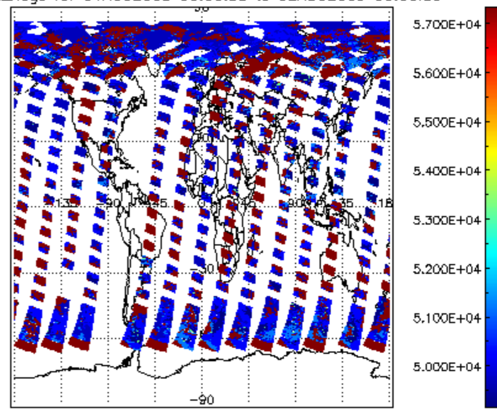
cloud_flags for 01AUG2009 00:00:00 to 02AUG2009 00:00:00
