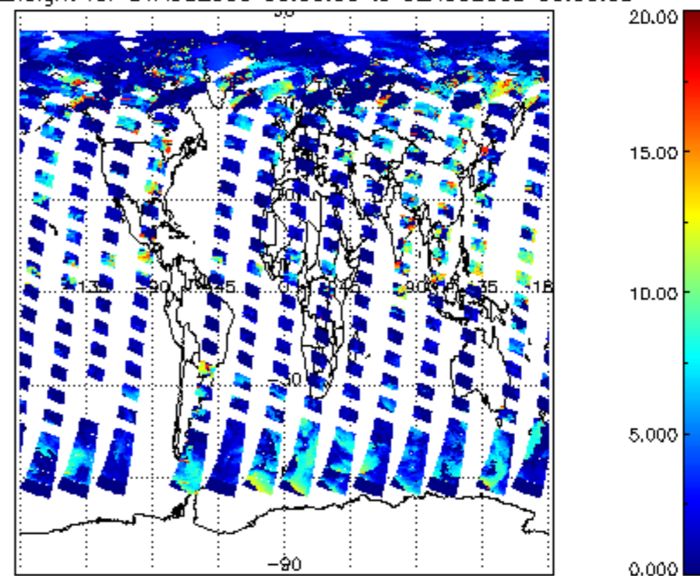
cL_top_height for 01AUG2009 00:00:00 to 02AUG2009 00:00:00
