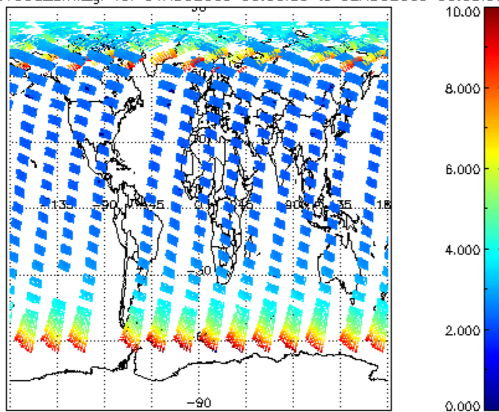
SCIOL2P_NADUV003_amf_gr for 01AUG2009 00:00:00 to 02AUG2009 00:00:00
