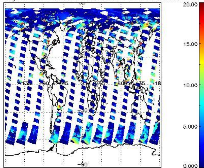
cL_top_height for 01AUG2009 00:00:00 to 02AUG2009 00:00:00
