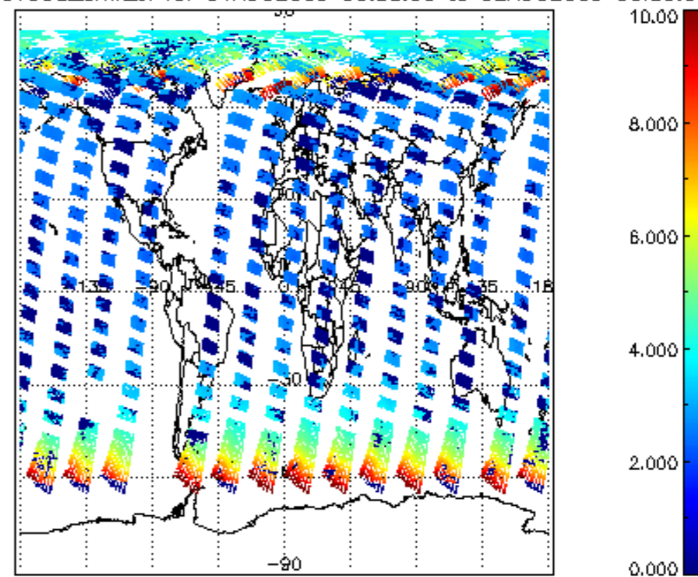
SCIOL2P_NADUV003_amf_cl for 01AUG2009 00:00:00 to 02AUG2009 00:00:00
