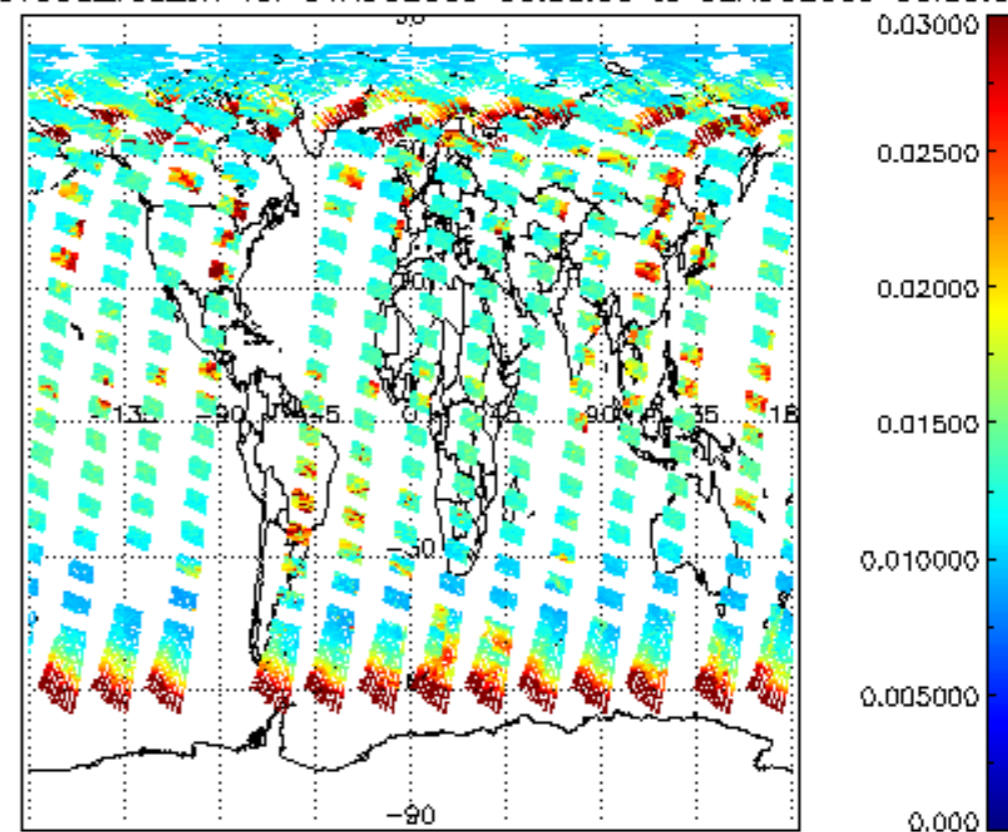
SCIOL2P_NADUV003_vcd_err for 01AUG2009 00:00:00 to 02AUG2009 00:00:00
