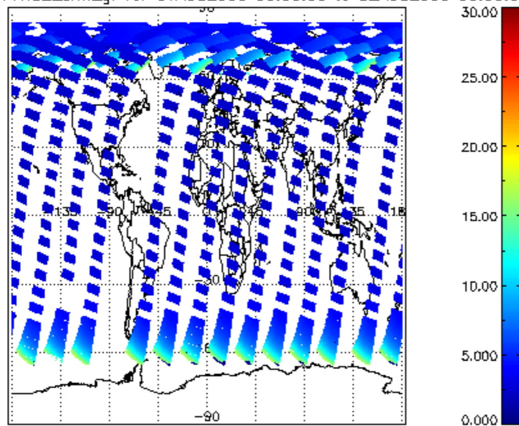
SCIOL2P_NADUV1NO2_amf_gr for 01AUG2009 00:00:00 to 02AUG2009 00:00:00
