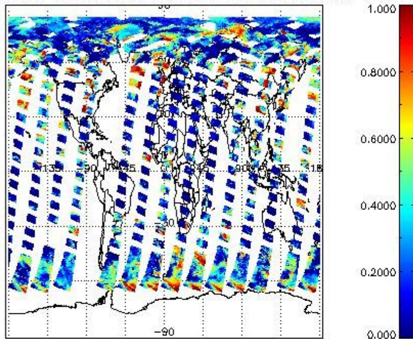
cL_frac for 01AUG2009 00:00:00 to 02AUG2009 00:00:00
