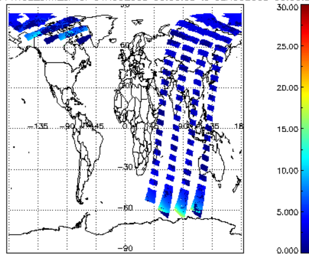
SCIOL2P_NADUV1NO2_amf_cl for 01AUG2009 00:00:00 to 02AUG2009 00:00:00
