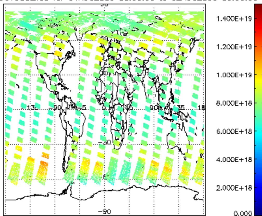
SCIOL2P_NADUV003_vcd for 01AUG2009 00:00:00 to 02AUG2009 00:00:00
