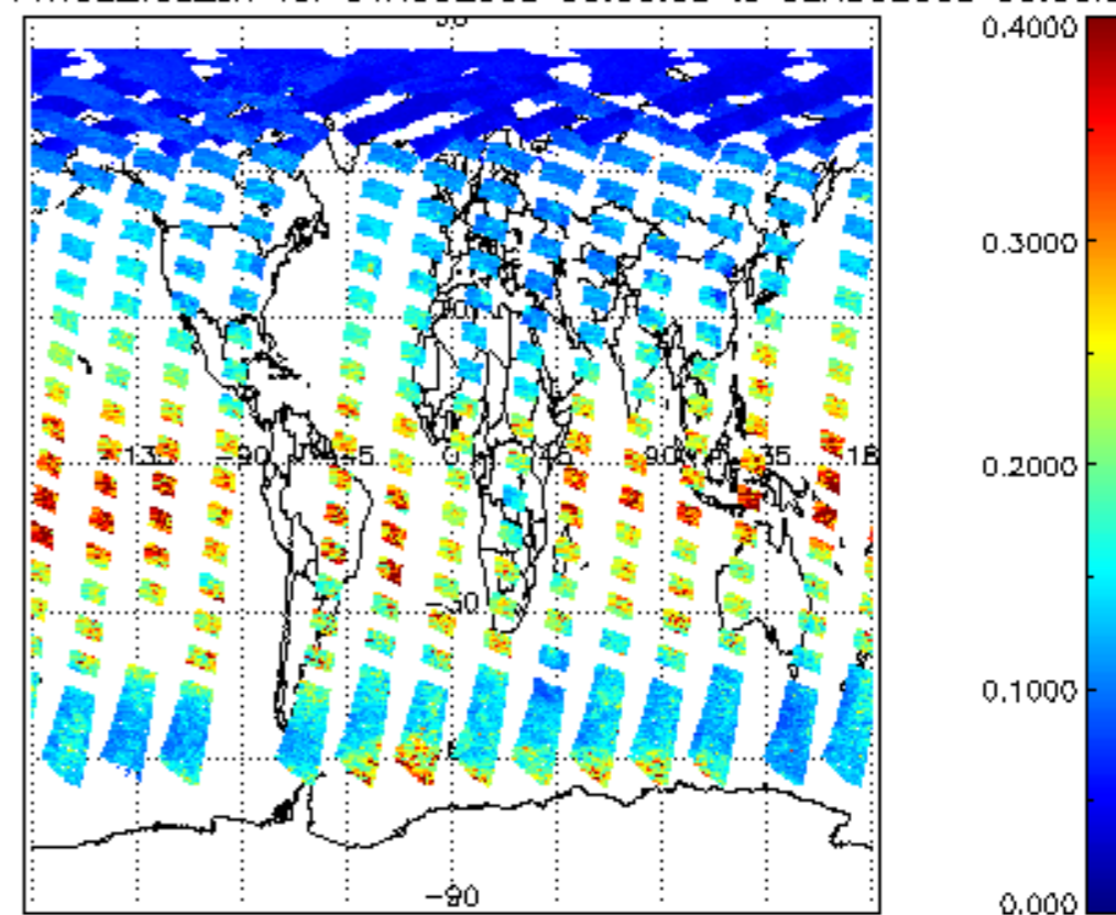
SCIOL2P_NADUV1NO2_vcd_err for 01AUG2009 00:00:00 to 02AUG2009 00:00:00
