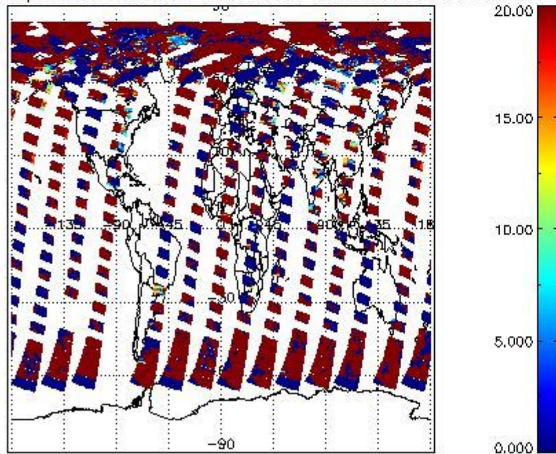
cL_opt_depth for 01AUG2009 00:00:00 to 02AUG2009 00:00:00
