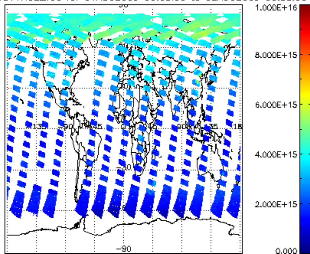
SCIOL2P_NADUV1NO2_vcd for 01AUG2009 00:00:00 to 02AUG2009 00:00:00
