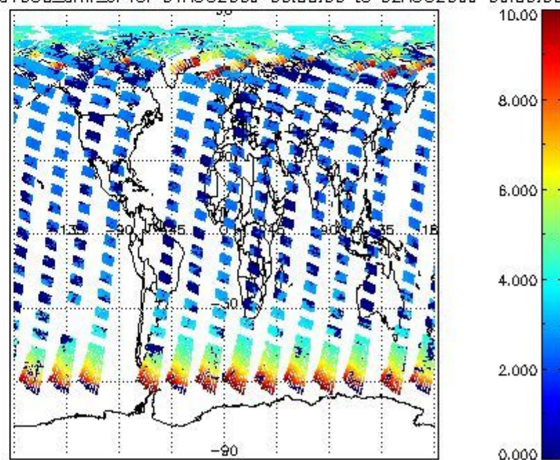
SCIOL2P_NADUV003_amf_gr for 01AUG2009 00:00:00 to 02AUG2009 00:00:00 SCIOL2P_NADUV003_amf_cl for 01AUG2009 00:00:00 to 02AUG2009 00:00:00
