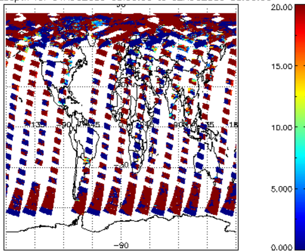
cL_opt_depth for 01AUG2009 00:00:00 to 02AUG2009 00:00:00
