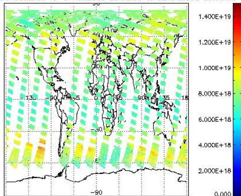
SCIOL2P_NADUV003_vcd for 01AUG2009 00:00:00 to 02AUG2009 00:00:00 SCIOL2P_NADUV003_vcd_err for 01AUG2009 00:00:00 to 02AUG2009 00:00:00
