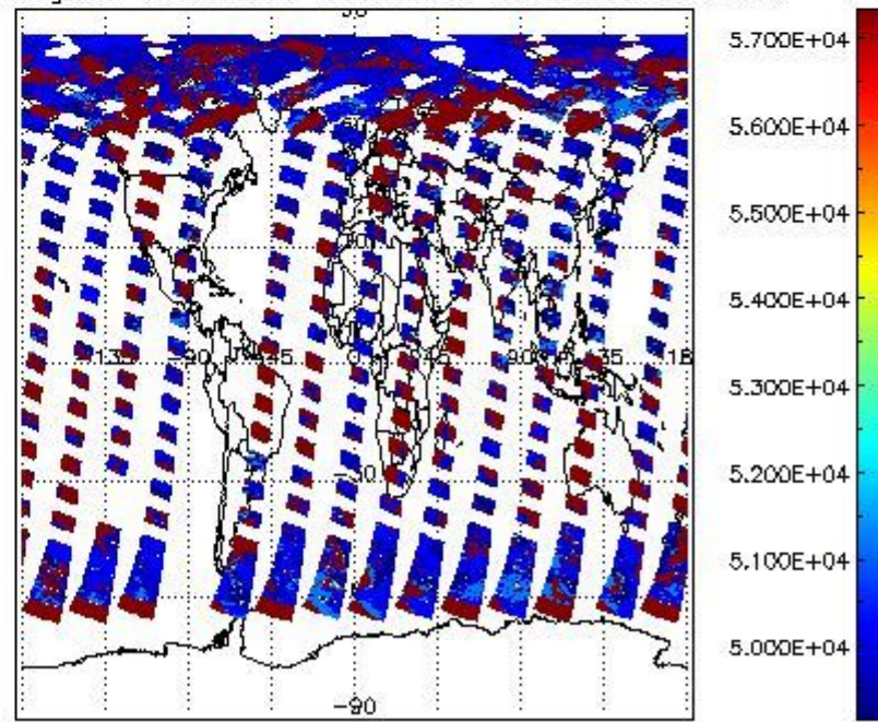
cloud_flags for 01AUG2009 00:00:00 to 02AUG2009 00:00:00
