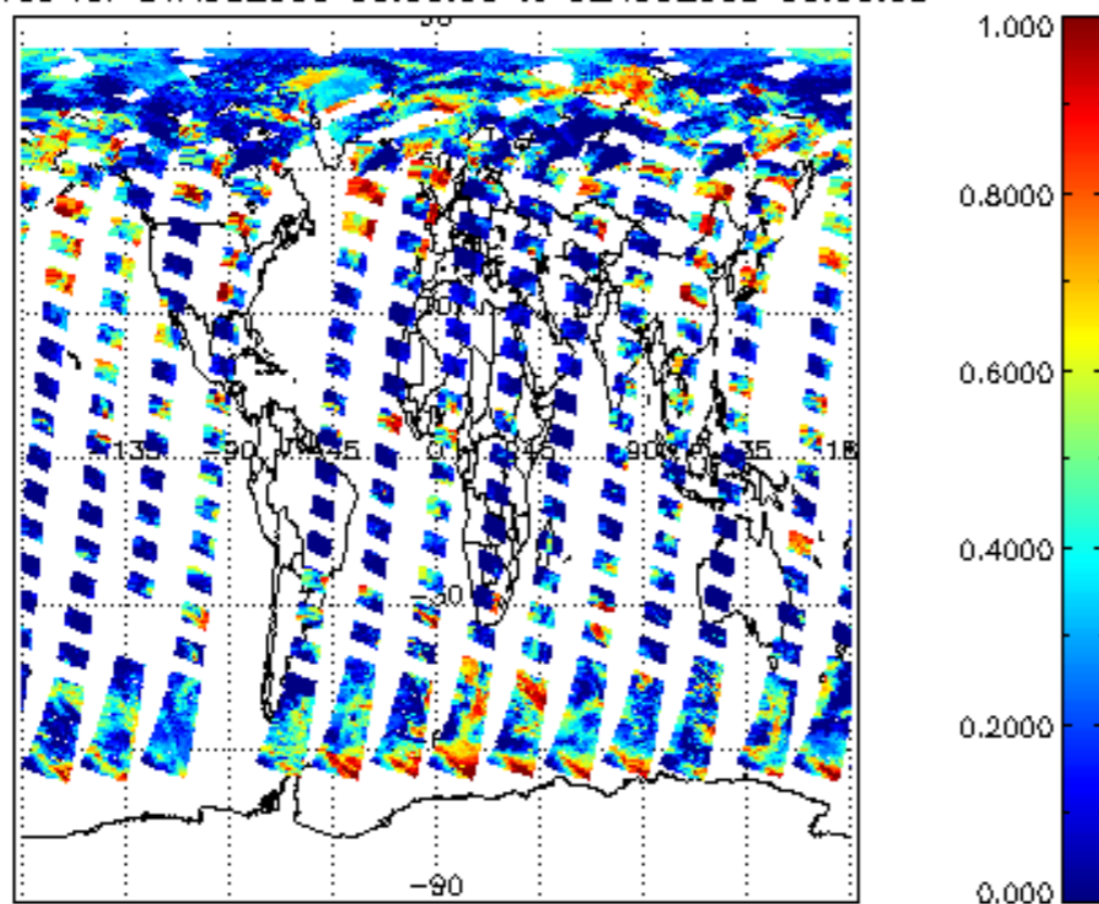
cL_frac for 01AUG2009 00:00:00 to 02AUG2009 00:00:00
