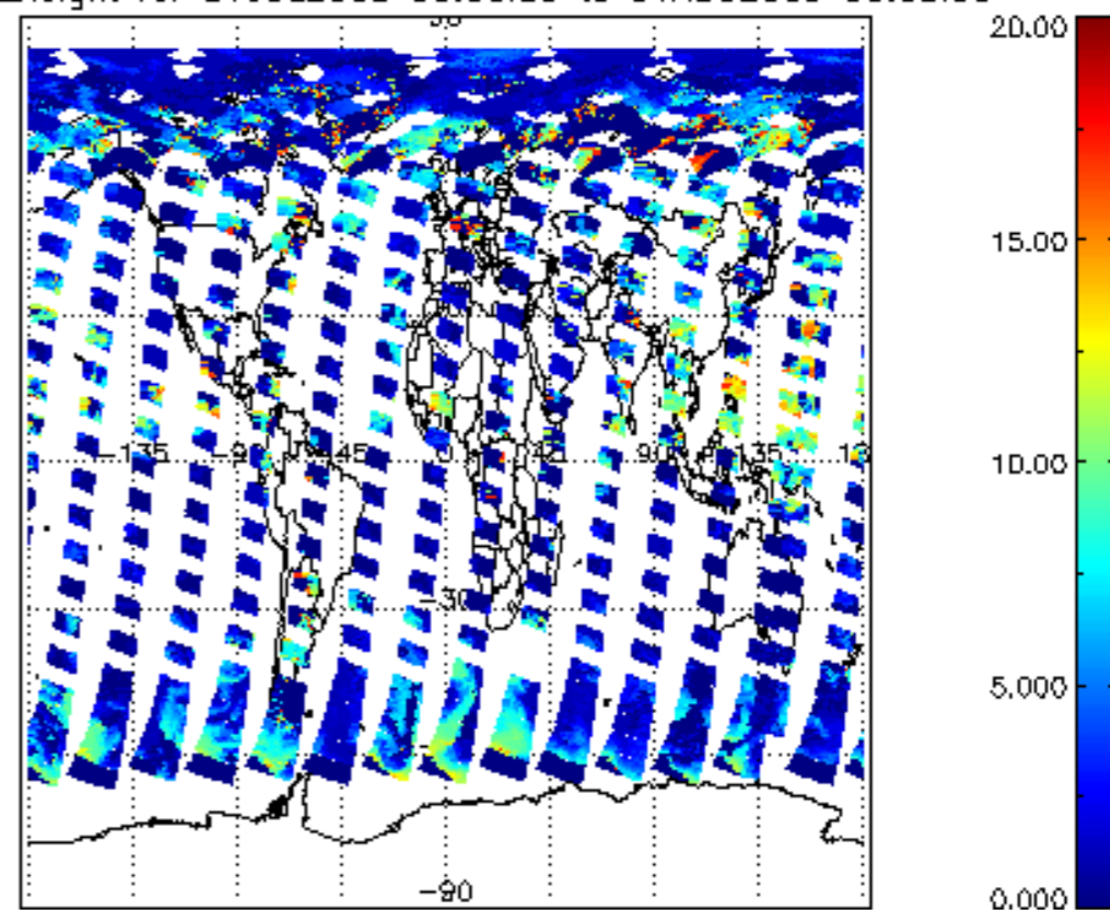
cl_top_height for 31JUL2009 00:00:00 to 01AUG2009 00:00:00
