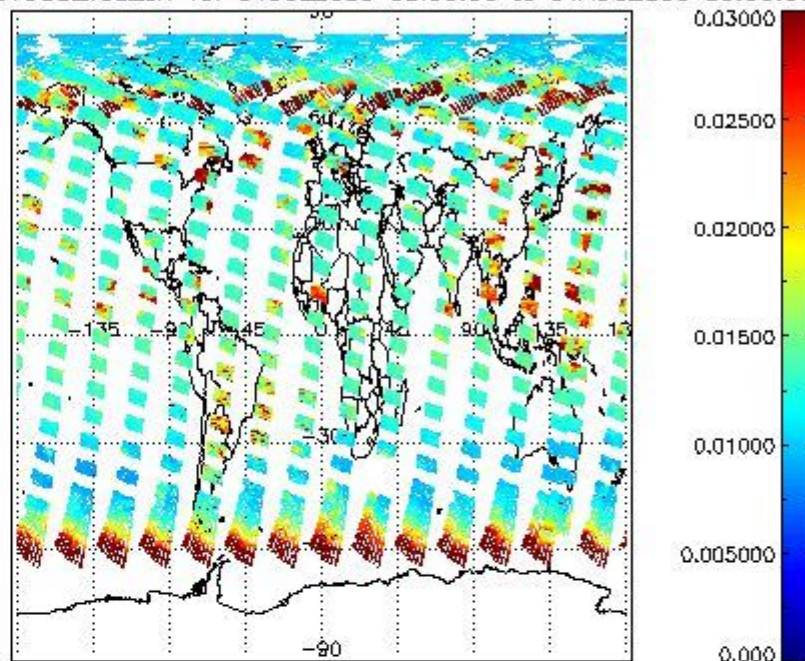
SCIOL2P_NADUV003_vcd_err for 31JUL2009 00:00:00 to 01AUG2009 00:00:00
