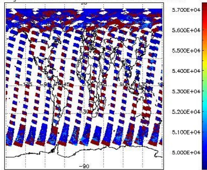
cloud_flags for 31JUL2009 00:00:00 to 01AUG2009 00:00:00
