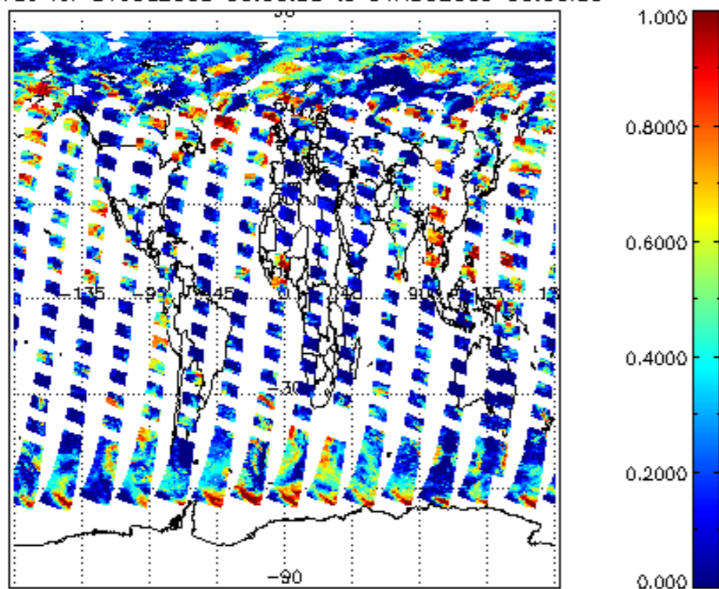
cl_frac for 31JUL2009 00:00:00 to 01AUG2009 00:00:00
