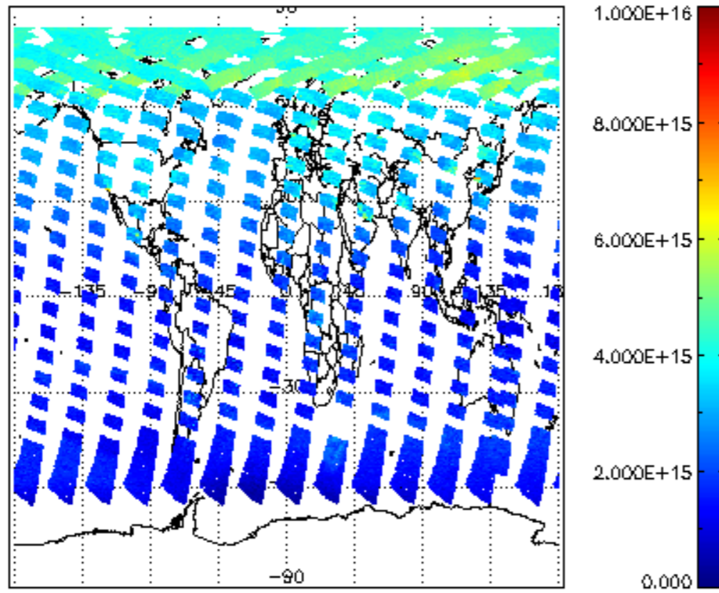
SCIOL2P_NADUV1NO2_vcd for 31JUL2009 00:00:00 to 01AUG2009 00:00:00
