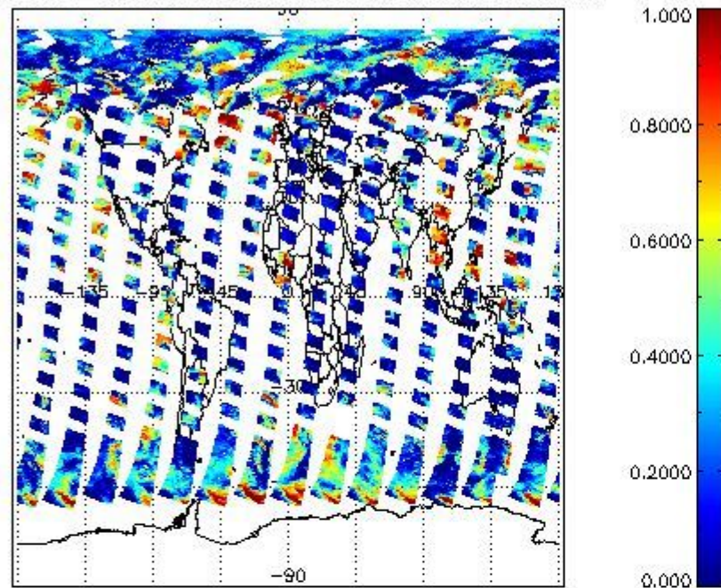
cL_frac for 31JUL2009 00:00:00 to 01AUG2009 00:00:00
