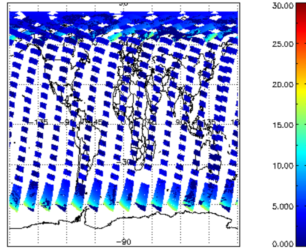
SCIOL2P_NADUV1NO2_amf_cl for 31JUL2009 00:00:00 to 01AUG2009 00:00:00
