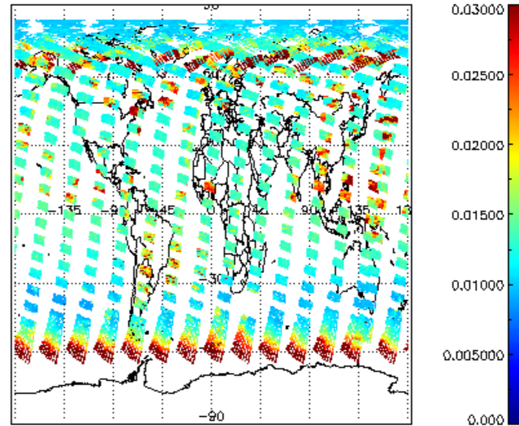
SCIOL2P_NADUV003_vcd_err for 31JUL2009 00:00:00 to 01AUG2009 00:00:00
