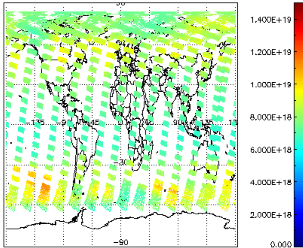
SCIOL2P_NADUV003_vcd for 31JUL2009 00:00:00 to 01AUG2009 00:00:00
