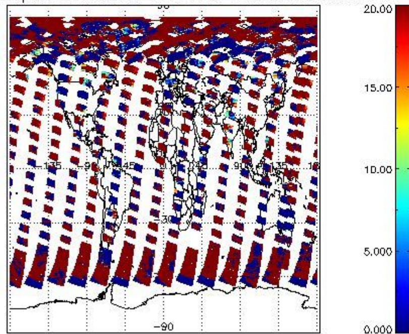
cL_opt_depth for 31JUL2009 00:00:00 to 01AUG2009 00:00:00
