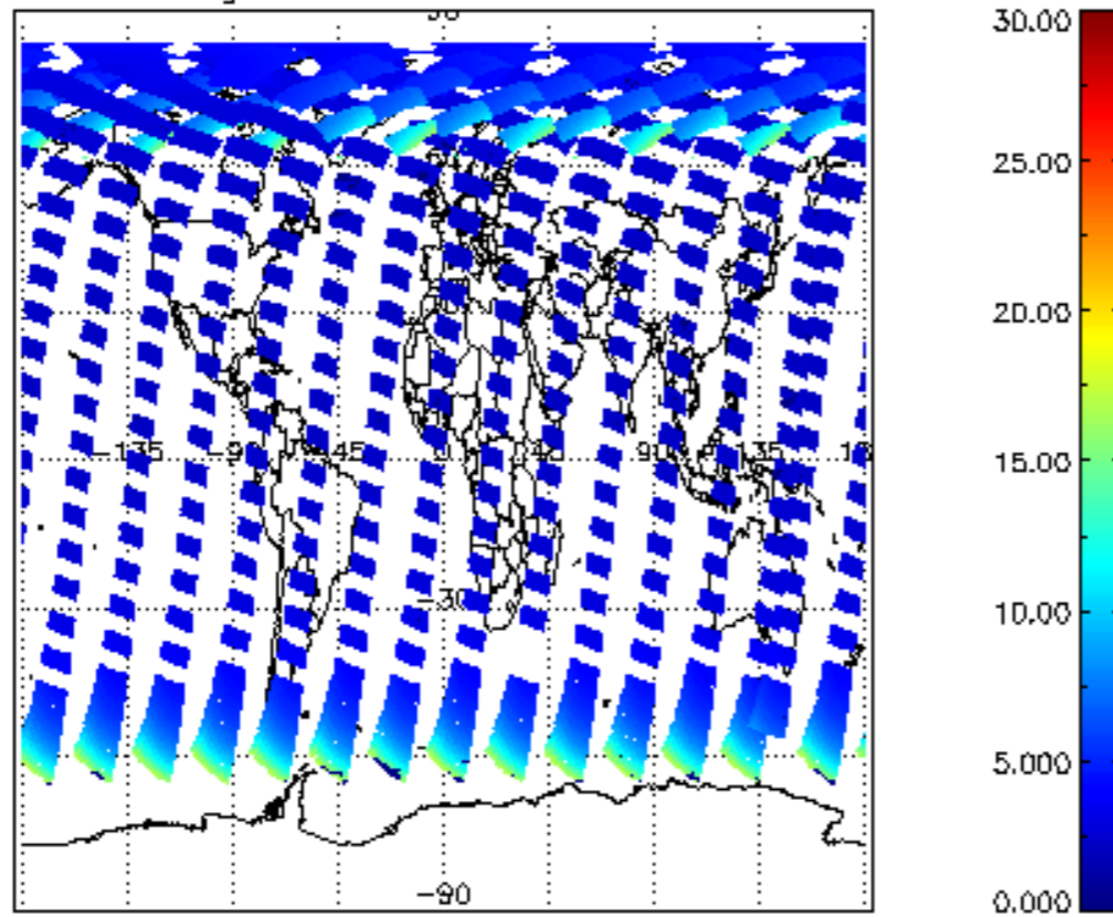
SCIOL2P_NADUV1NO2_amf_gr for 31JUL2009 00:00:00 to 01AUG2009 00:00:00
