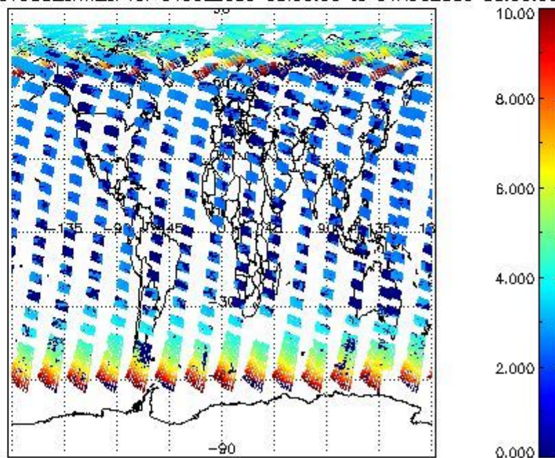
SCIOL2P_NADUV003_amf_cl for 31JUL2009 00:00:00 to 01AUG2009 00:00:00
