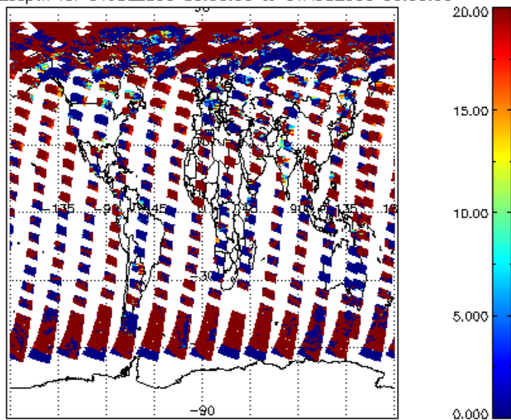
cl_opt_depth for 31JUL2009 00:00:00 to 01AUG2009 00:00:00
