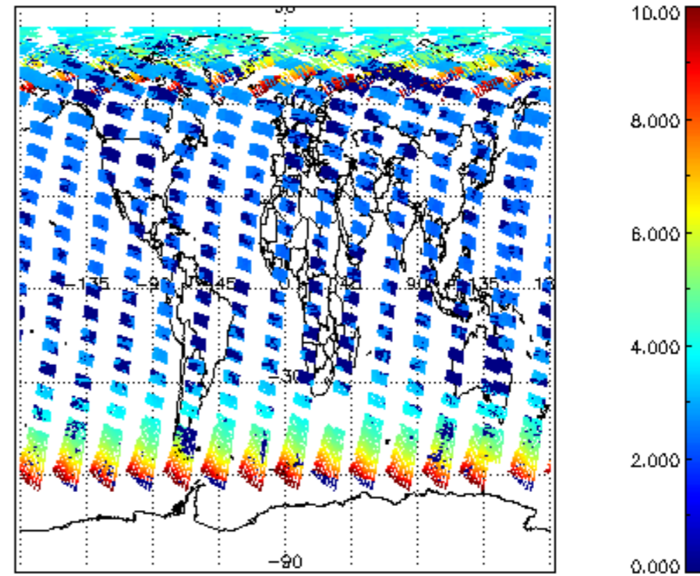
SCIOL2P_NADUV003_amf_el for 31JUL2009 00:00:00 to 01AUG2009 00:00:00
