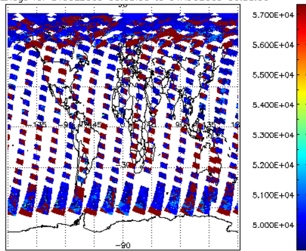
cloud_flags for 31JUL2009 00:00:00 to 01AUG2009 00:00:00
