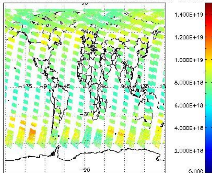
SCIOL2P_NADUV003_vcd for 31JUL2009 00:00:00 to 01AUG2009 00:00:00
