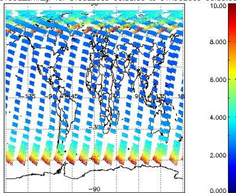
SCIOL2P_NADUV003_amf_gr for 31JUL2009 00:00:00 to 01AUG2009 00:00:00
