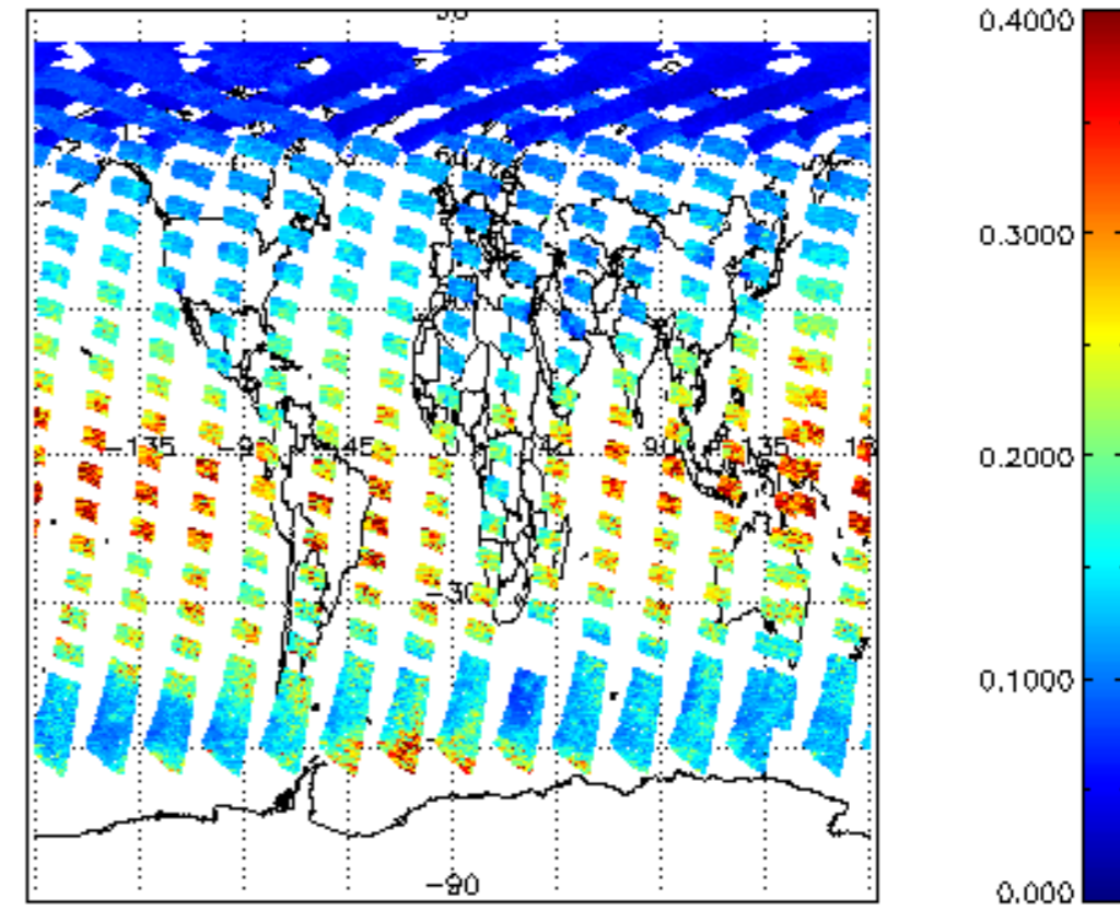
SCIOL2P_NADUV1NO2_vcd_err for 31JUL2009 00:00:00 to 01AUG2009 00:00:00
