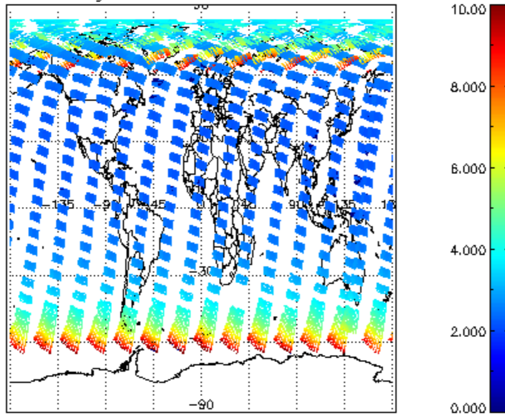
SCIOL2P_NADUV003_amf_gr for 31JUL2009 00:00:00 to 01AUG2009 00:00:00
