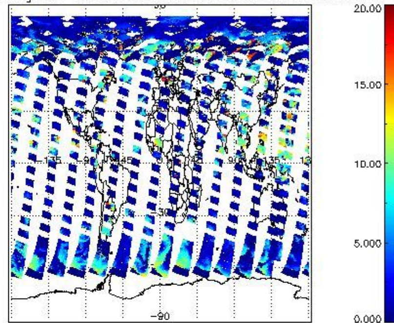
cL_top_height for 31JUL2009 00:00:00 to 01AUG2009 00:00:00
