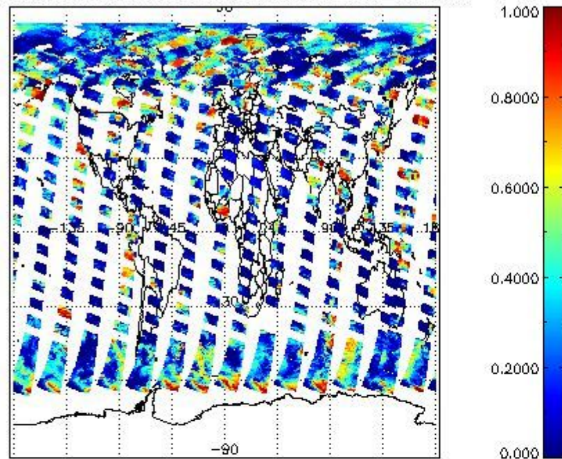
cL_frac for 28JUL2009 00:00:00 to 29JUL2009 00:00:00
