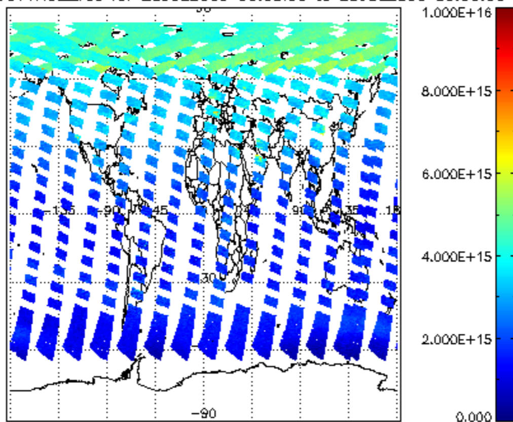
SCIOL2P_NADUV1NO2_vcd for 28JUL2009 00:00:00 to 29JUL2009 00:00:00
