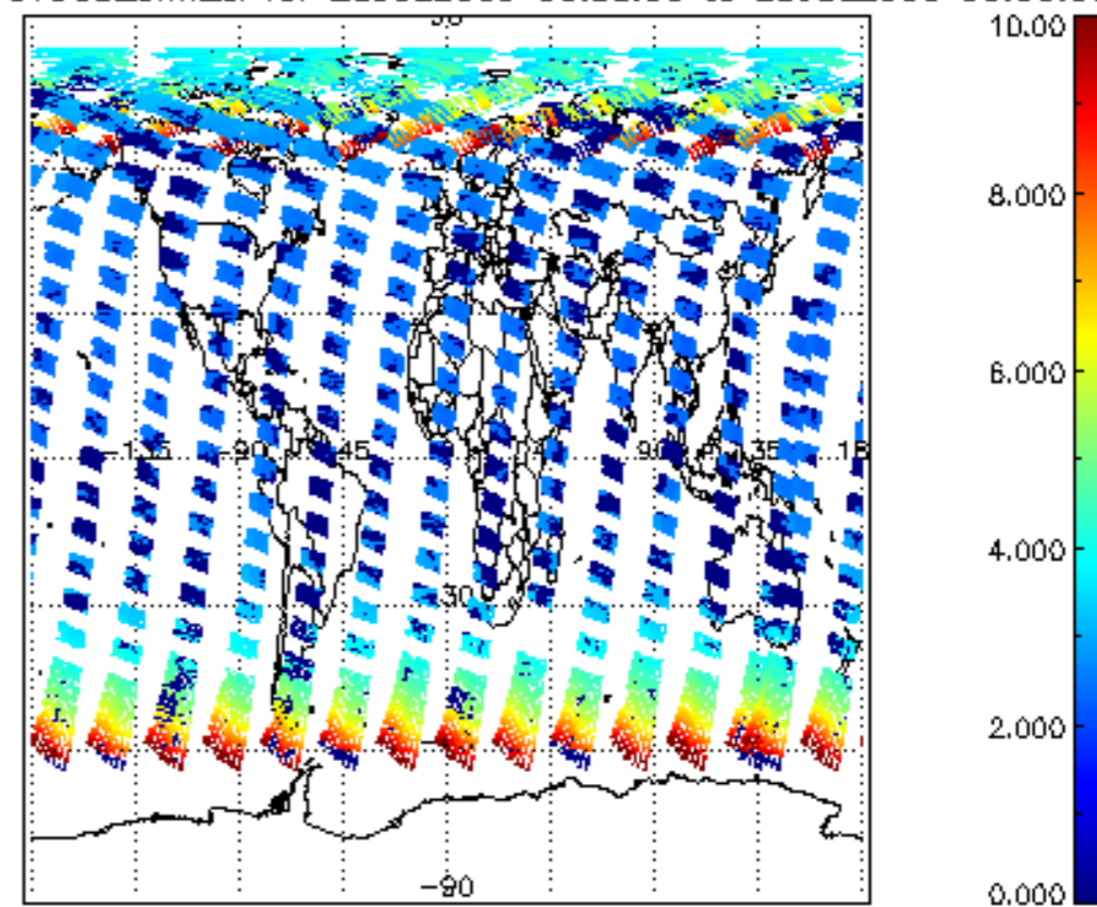
SCIOL2P_NADUV003_amf_cl for 28JUL2009 00:00:00 to 29JUL2009 00:00:00
