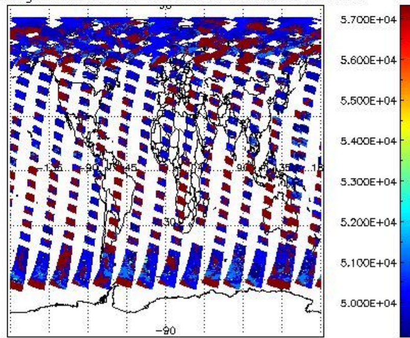
cloud_flags for 28JUL2009 00:00:00 to 29JUL2009 00:00:00
