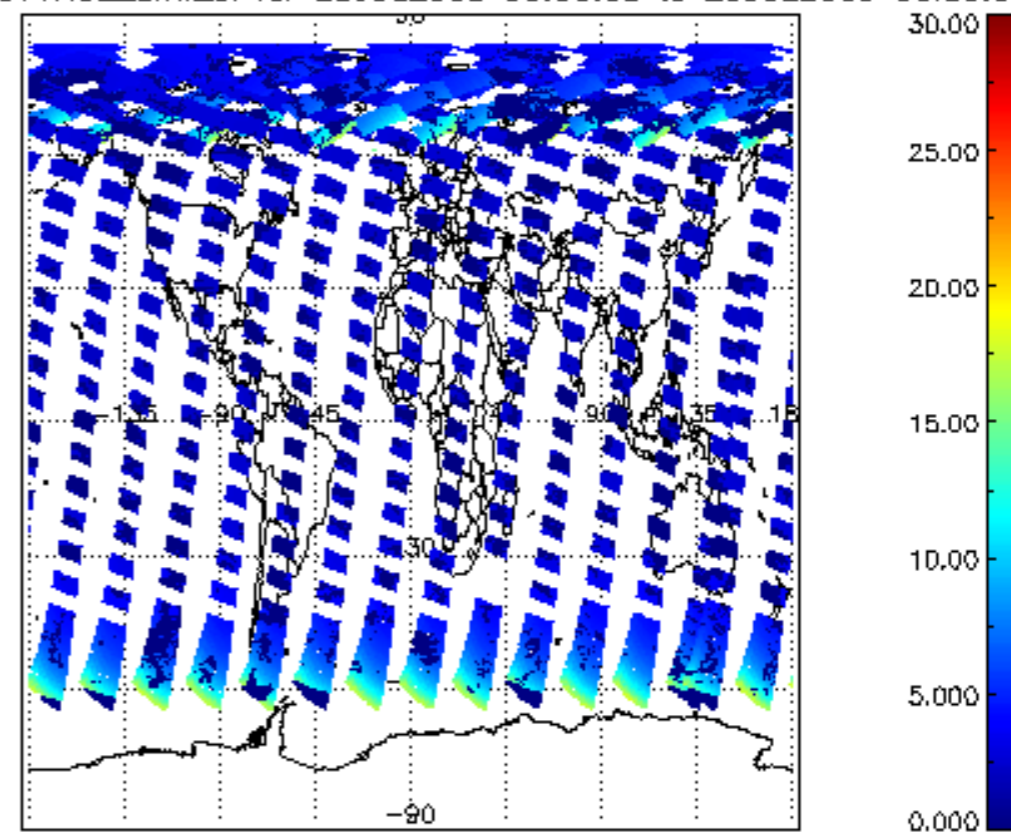
SCIOL2P_NADUV1NO2_amf_cl for 28JUL2009 00:00:00 to 29JUL2009 00:00:00
