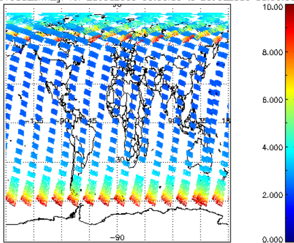
SCIOL2P_NADUV003_amf_gr for 28JUL2009 00:00:00 to 29JUL2009 00:00:00
