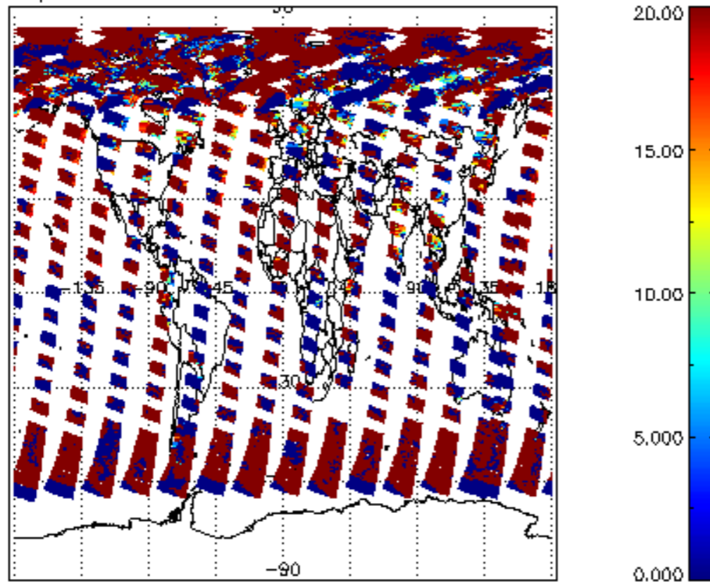
cl_opt_depth for 28JUL2009 00:00:00 to 29JUL2009 00:00:00
