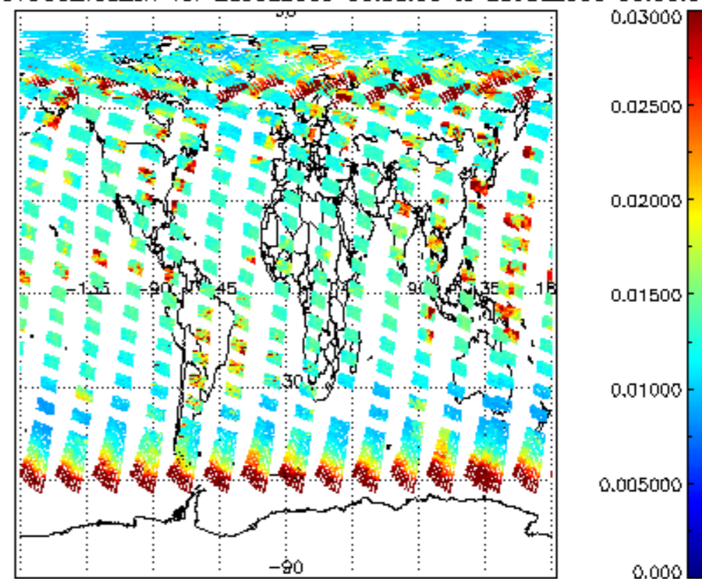
SCIOL2P_NADUV003_vcd_err for 28JUL2009 00:00:00 to 29JUL2009 00:00:00
