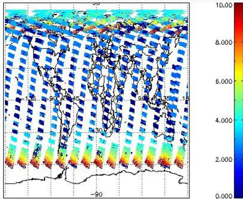
SCIOL2P_NADUV003_amf_cl for 28JUL2009 00:00:00 to 29JUL2009 00:00:00
