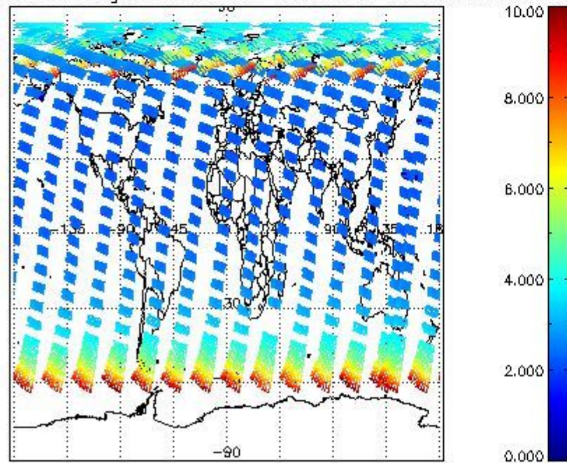
SCIOL2P_NADUV003_amf_gr for 28JUL2009 00:00:00 to 29JUL2009 00:00:00
