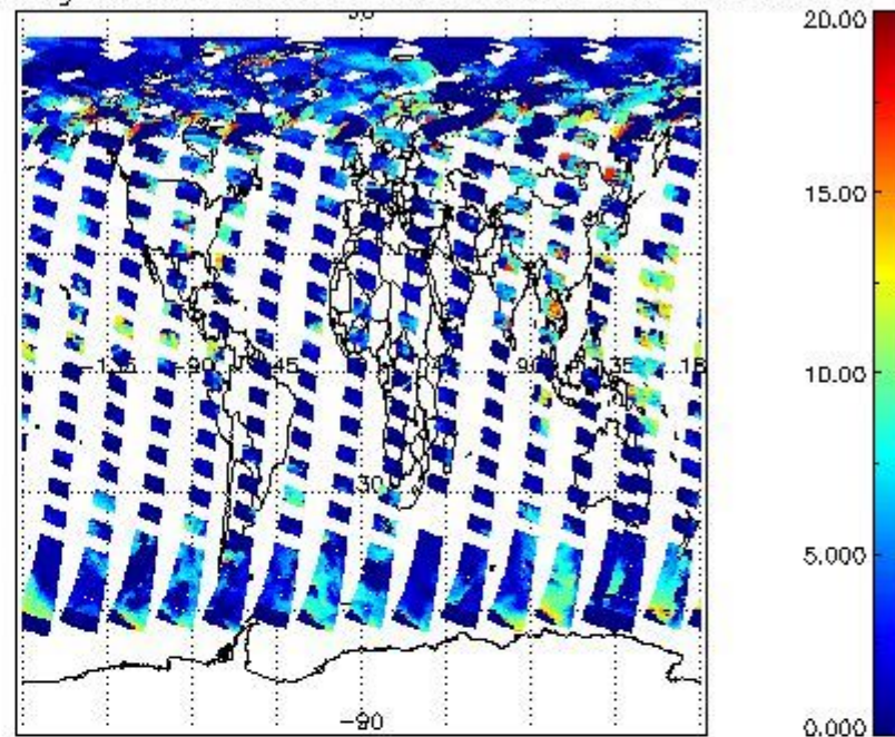
cL_top_height for 28JUL2009 00:00:00 to 29JUL2009 00:00:00
