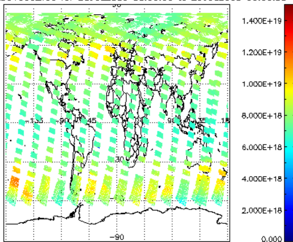
SCIOL2P_NADUV003_vcd for 28JUL2009 00:00:00 to 29JUL2009 00:00:00
