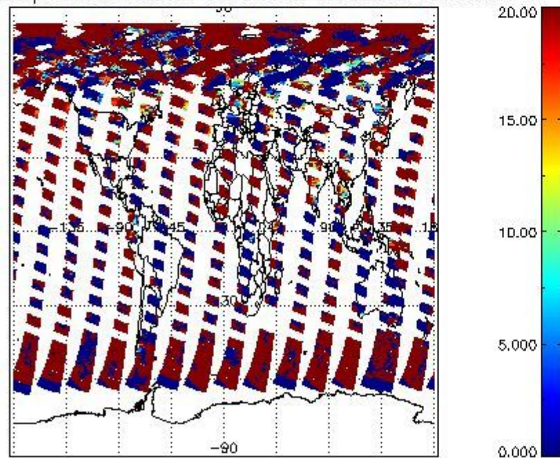
cL_opt_depth for 28JUL2009 00:00:00 to 29JUL2009 00:00:00
