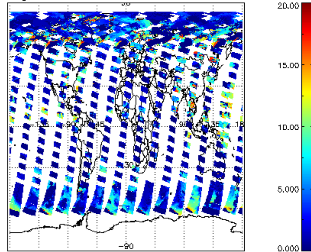
cl_top_height for 28JUL2009 00:00:00 to 29JUL2009 00:00:00
