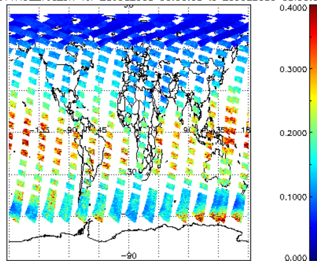
SCIOL2P_NADUV1NO2_vcd_err for 28JUL2009 00:00:00 to 29JUL2009 00:00:00
