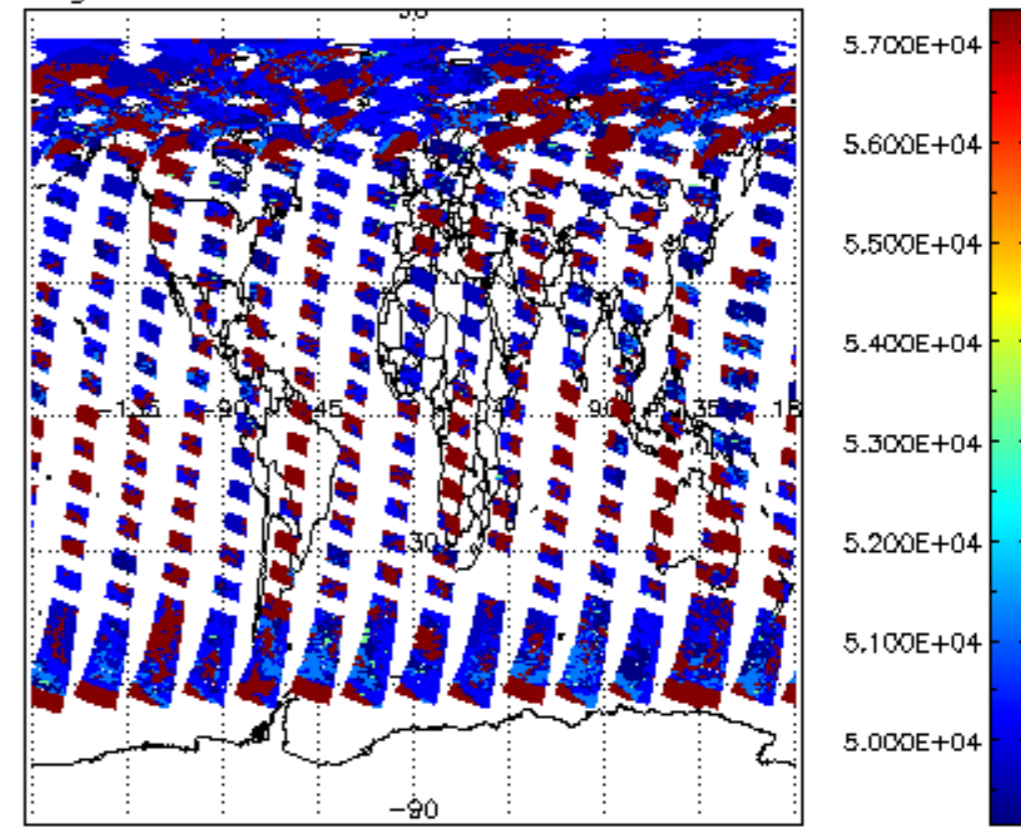
cloud_flags for 28JUL2009 00:00:00 to 29JUL2009 00:00:00
