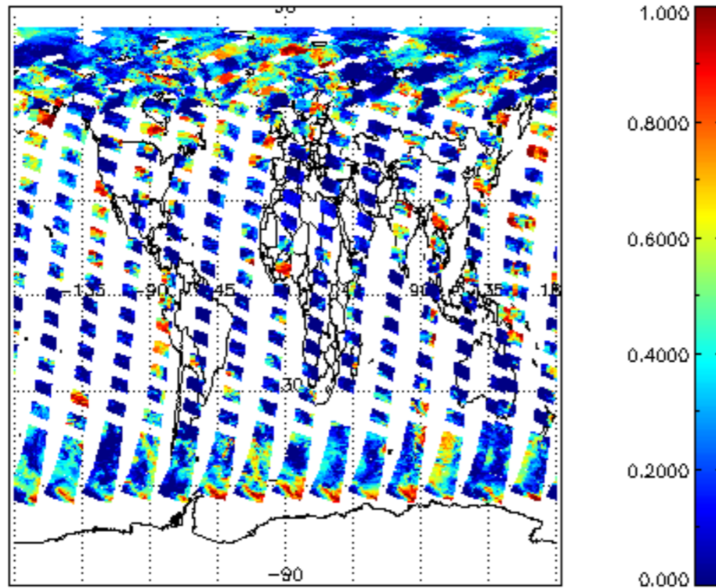
cl_frac for 28JUL2009 00:00:00 to 29JUL2009 00:00:00
