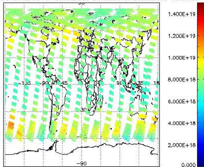
SCIOL2P_NADUV003_vcd for 28JUL2009 00:00:00 to 29JUL2009 00:00:00
