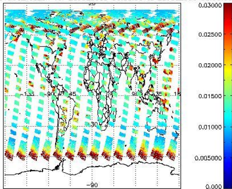
SCIOL2P_NADUV003_vcd_err for 28JUL2009 00:00:00 to 29JUL2009 00:00:00
