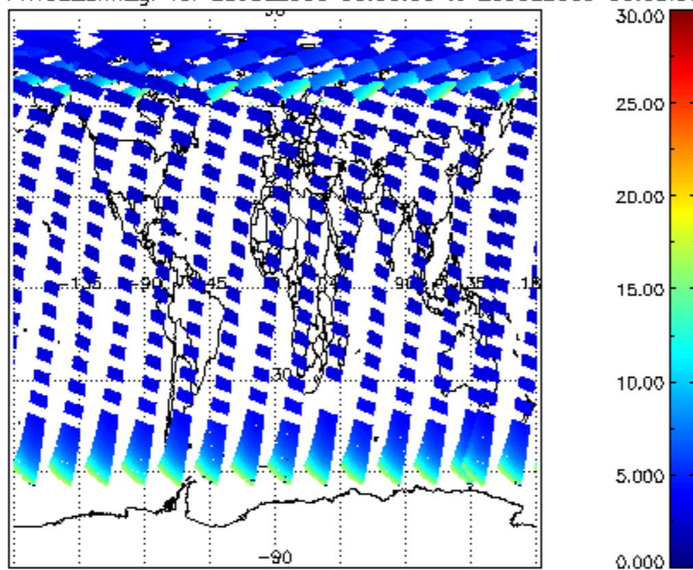
SCIOL2P_NADUV1NO2_amf_gr for 28JUL2009 00:00:00 to 29JUL2009 00:00:00
