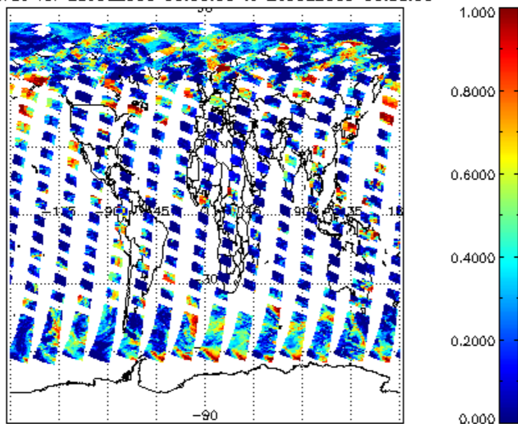
cl_frac for 25JUL2009 00:00:00 to 26JUL2009 00:00:00
