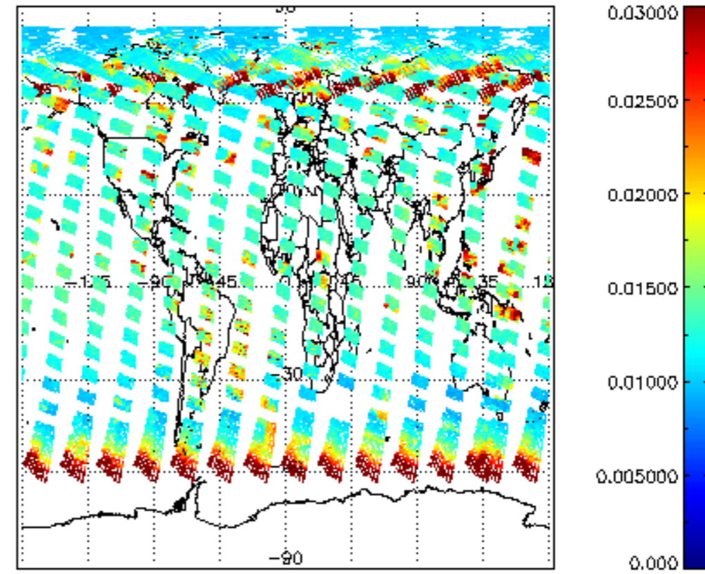
SCIOL2P_NADUV003_vcd_err for 25JUL2009 00:00:00 to 26JUL2009 00:00:00
