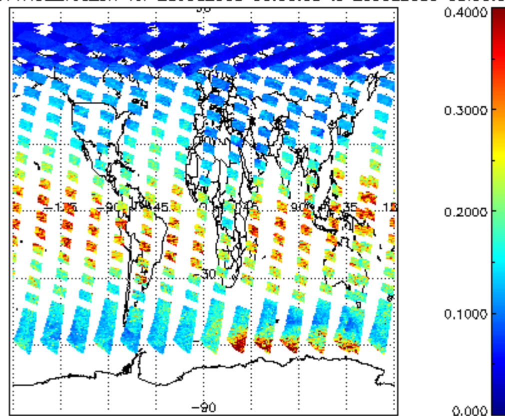
SCIOL2P_NADUV1NO2_vcd_err for 25JUL2009 00:00:00 to 26JUL2009 00:00:00
