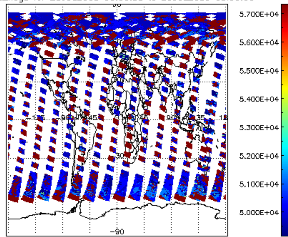
cloud_flags for 25JUL2009 00:00:00 to 26JUL2009 00:00:00
