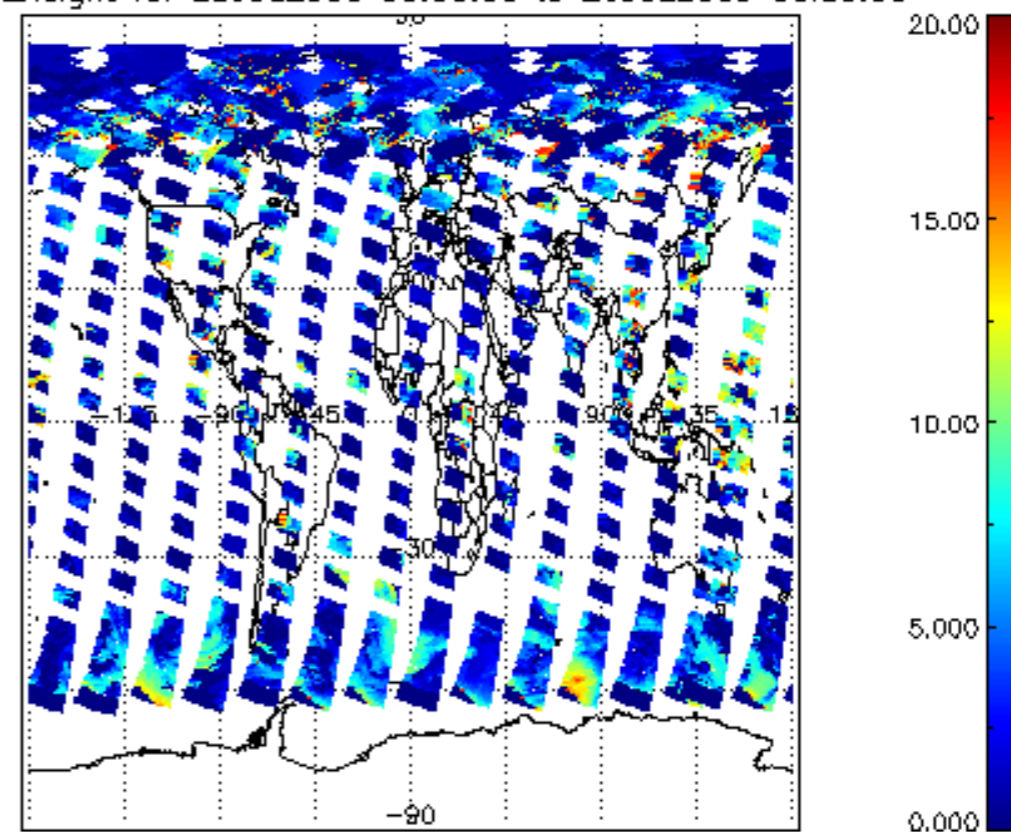
cl_top_height for 25JUL2009 00:00:00 to 26JUL2009 00:00:00
