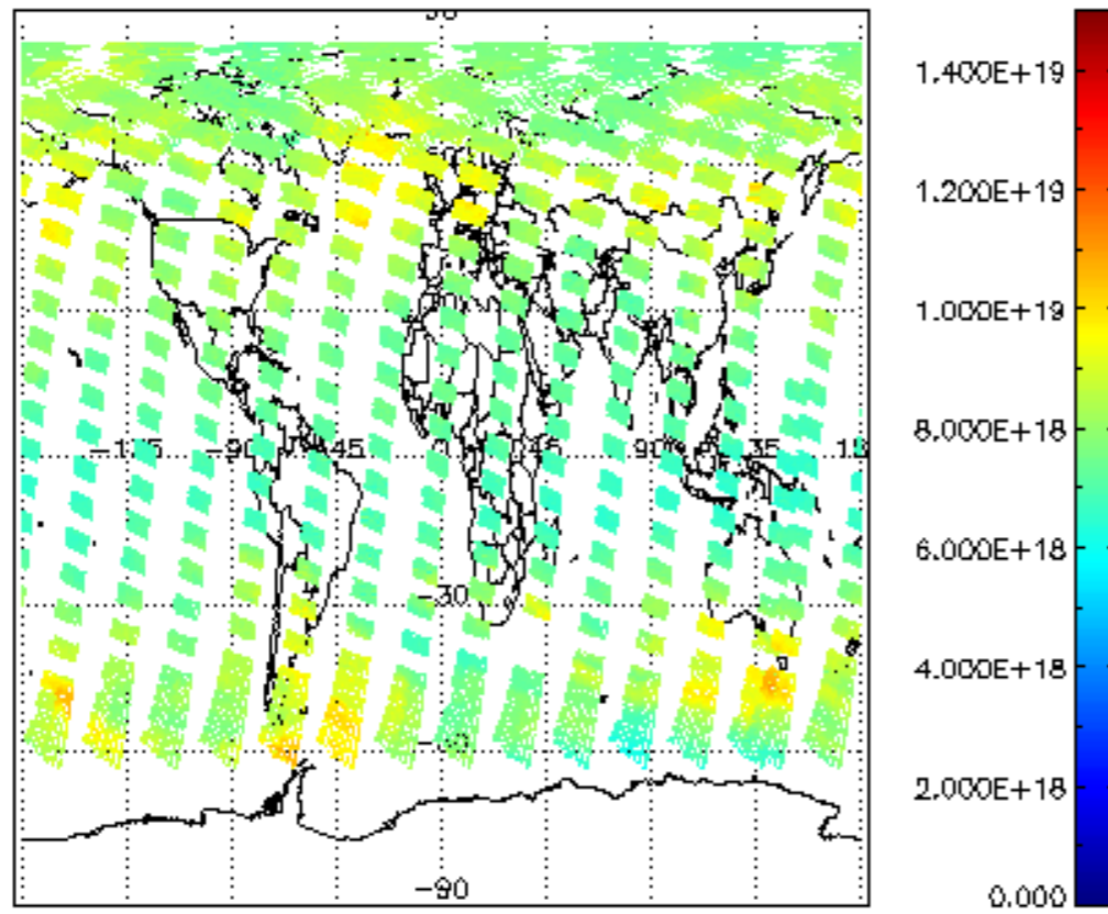
SCIOL2P_NADUV003_vcd for 25JUL2009 00:00:00 to 26JUL2009 00:00:00
