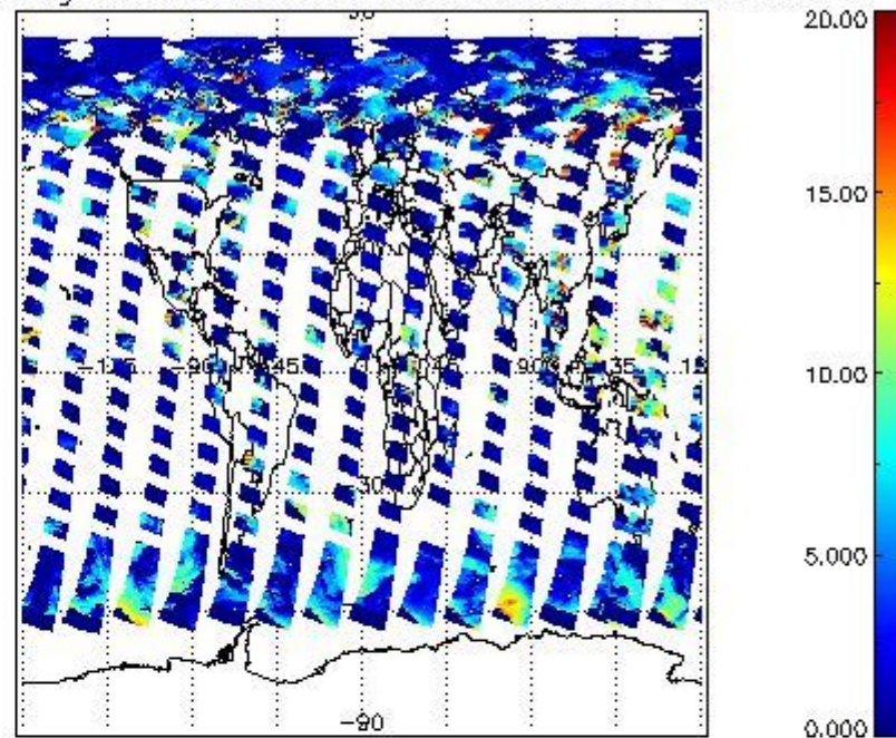
cL_top_height for 25JUL2009 00:00:00 to 26JUL2009 00:00:00
