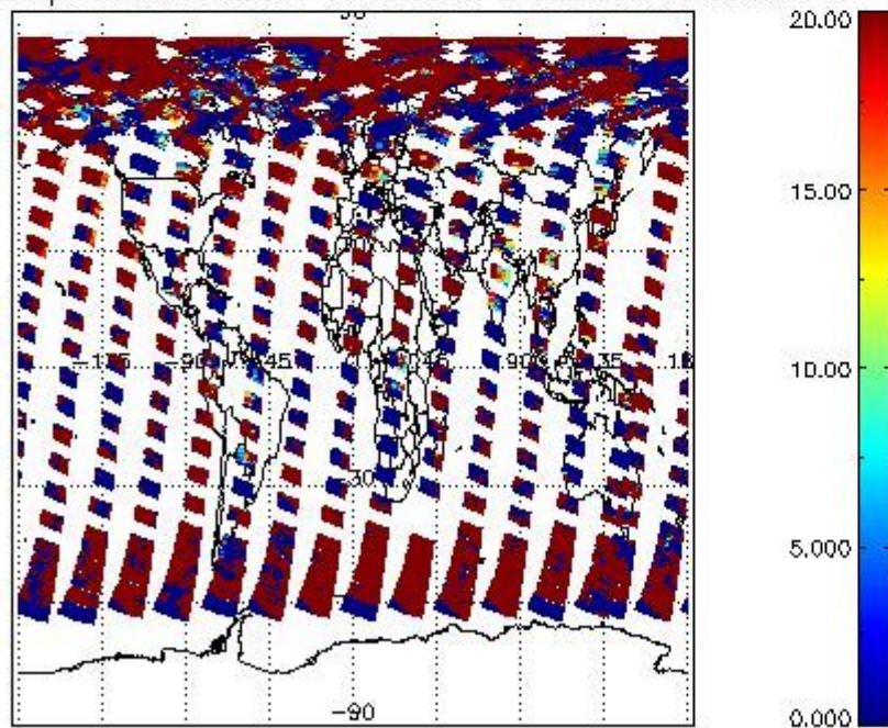
cL_opt_depth for 25JUL2009 00:00:00 to 26JUL2009 00:00:00
