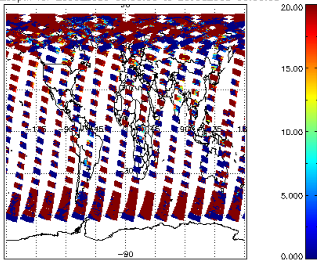
cl_lopt_depth for 25JUL2009 00:00:00 to 26JUL2009 00:00:00
