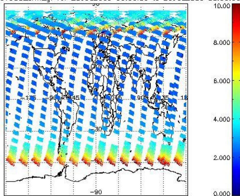
SCIOL2P_NADUV003_amf_gr for 25JUL2009 00:00:00 to 26JUL2009 00:00:00
