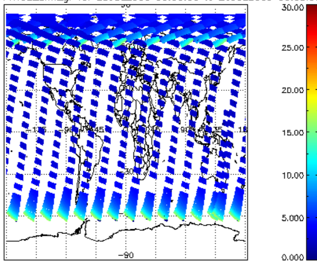
SCIOL2P_NADUV1NO2_amf_gr for 25JUL2009 00:00:00 to 26JUL2009 00:00:00
