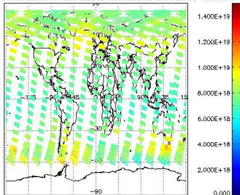
SCIOL2P_NADUV003_vcd for 25JUL2009 00:00:00 to 26JUL2009 00:00:00
