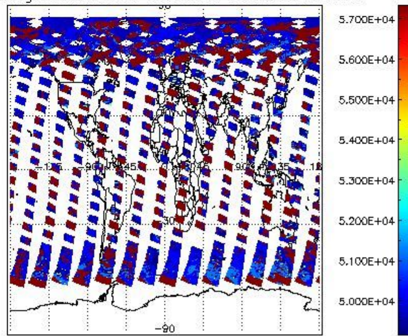
cloud_flags for 25JUL2009 00:00:00 to 26JUL2009 00:00:00
