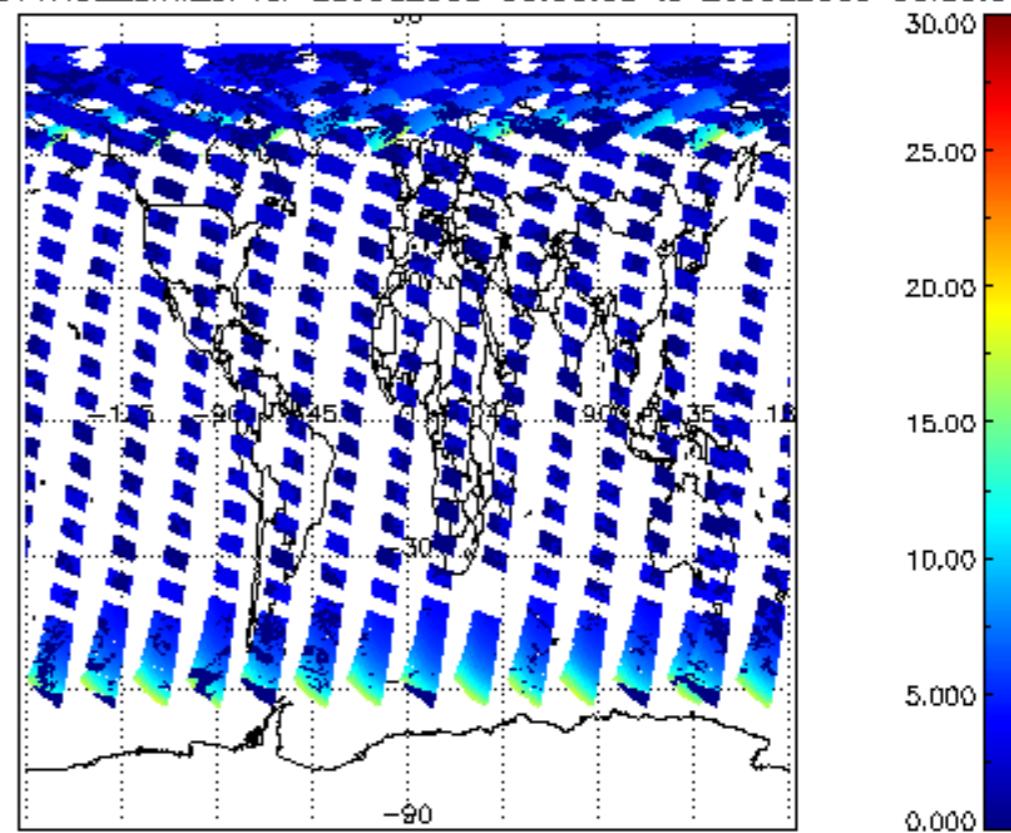
SCIOL2P_NADUV1NO2_amf_cl for 25JUL2009 00:00:00 to 26JUL2009 00:00:00
