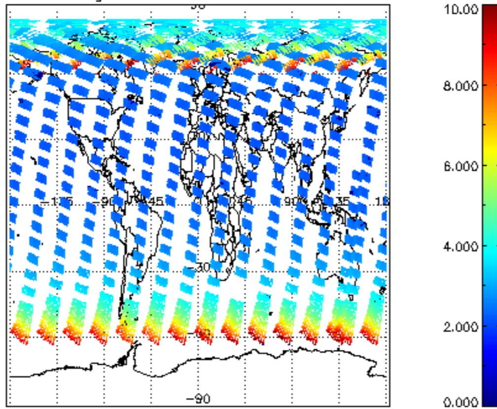
SCIOL2P_NADUV003_amf_gr for 25JUL2009 00:00:00 to 26JUL2009 00:00:00
