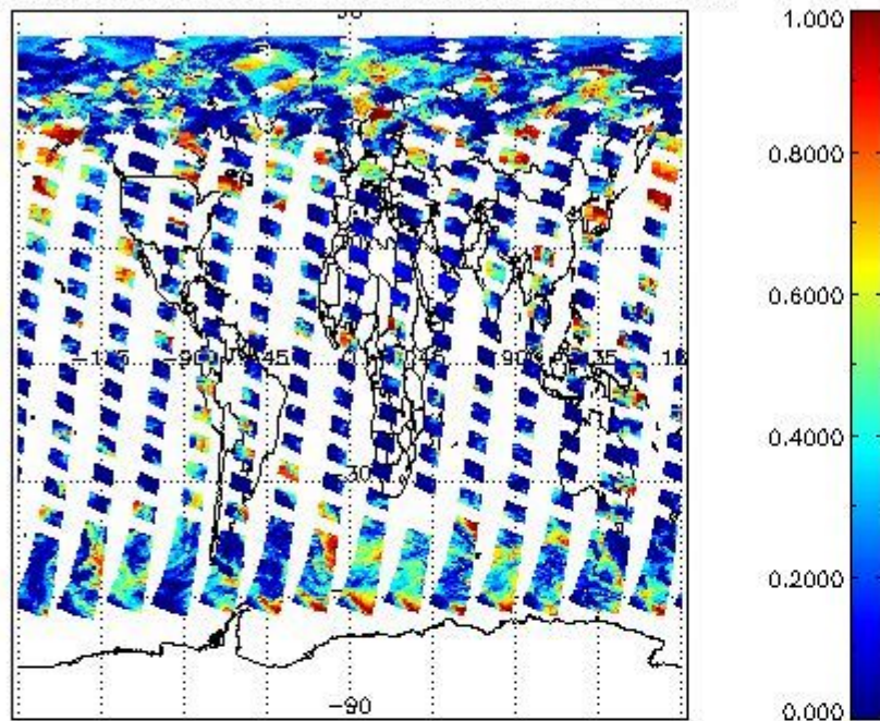
cL_frac for 25JUL2009 00:00:00 to 26JUL2009 00:00:00
