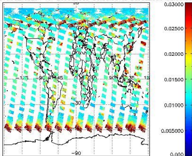
SCIOL2P_NADUV003_vcd_err for 25JUL2009 00:00:00 to 26JUL2009 00:00:00
