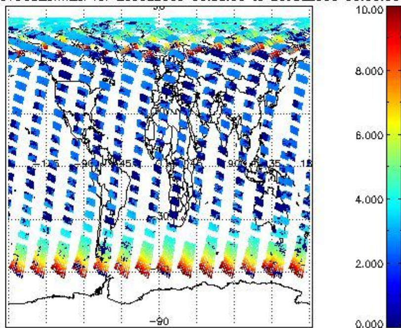
SCIOL2P_NADUV003_amf_cl for 25JUL2009 00:00:00 to 26JUL2009 00:00:00
