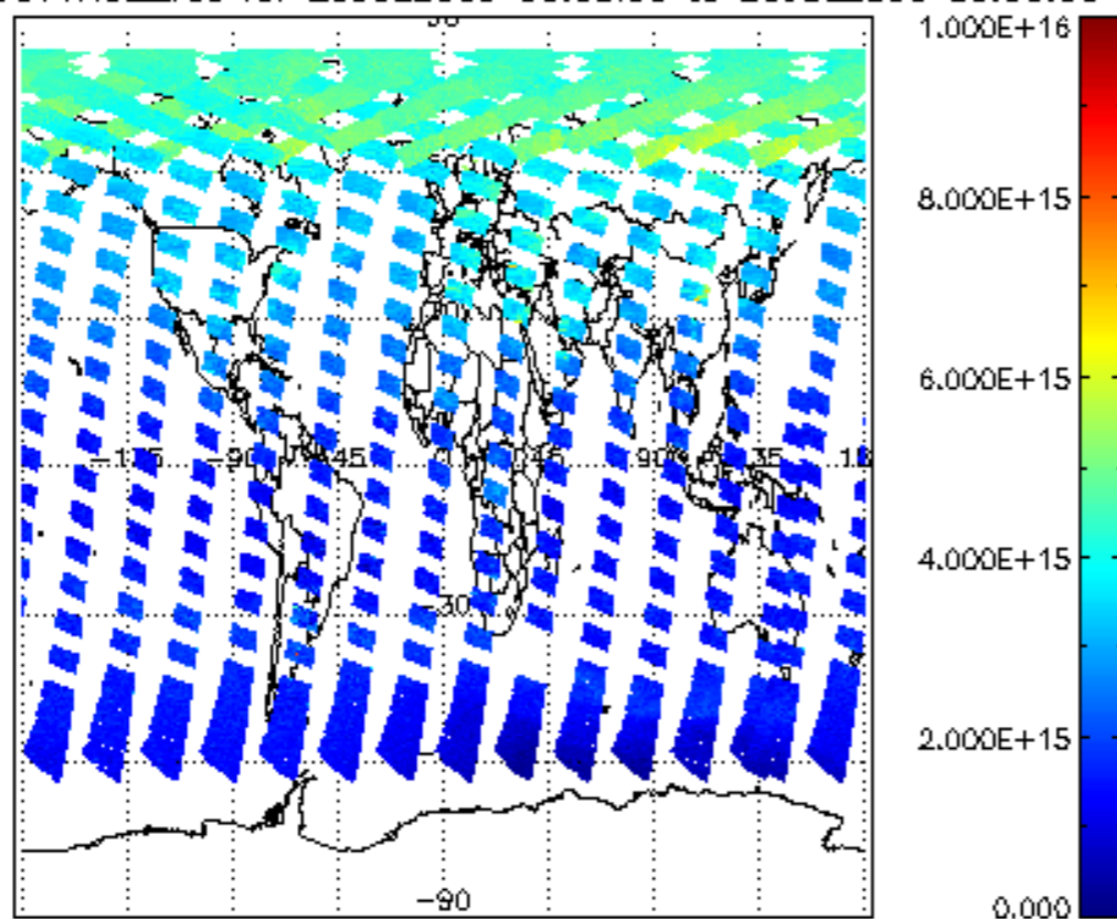
SCIOL2P_NADUV1NO2_vcd for 25JUL2009 00:00:00 to 26JUL2009 00:00:00
