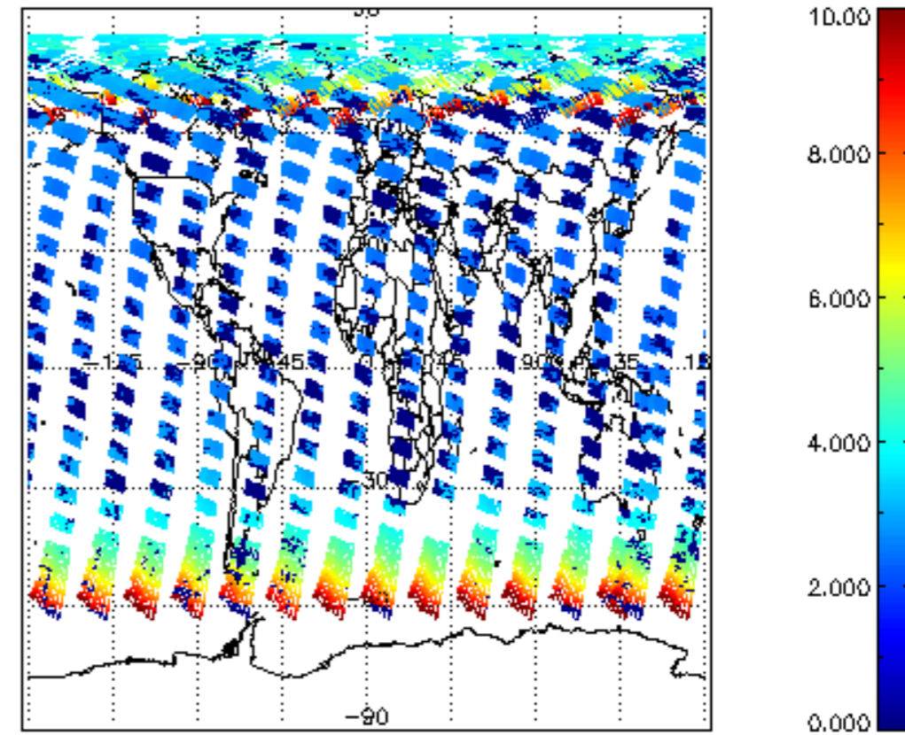
SCIOL2P_NADUV003_amf_cl for 25JUL2009 00:00:00 to 26JUL2009 00:00:00
