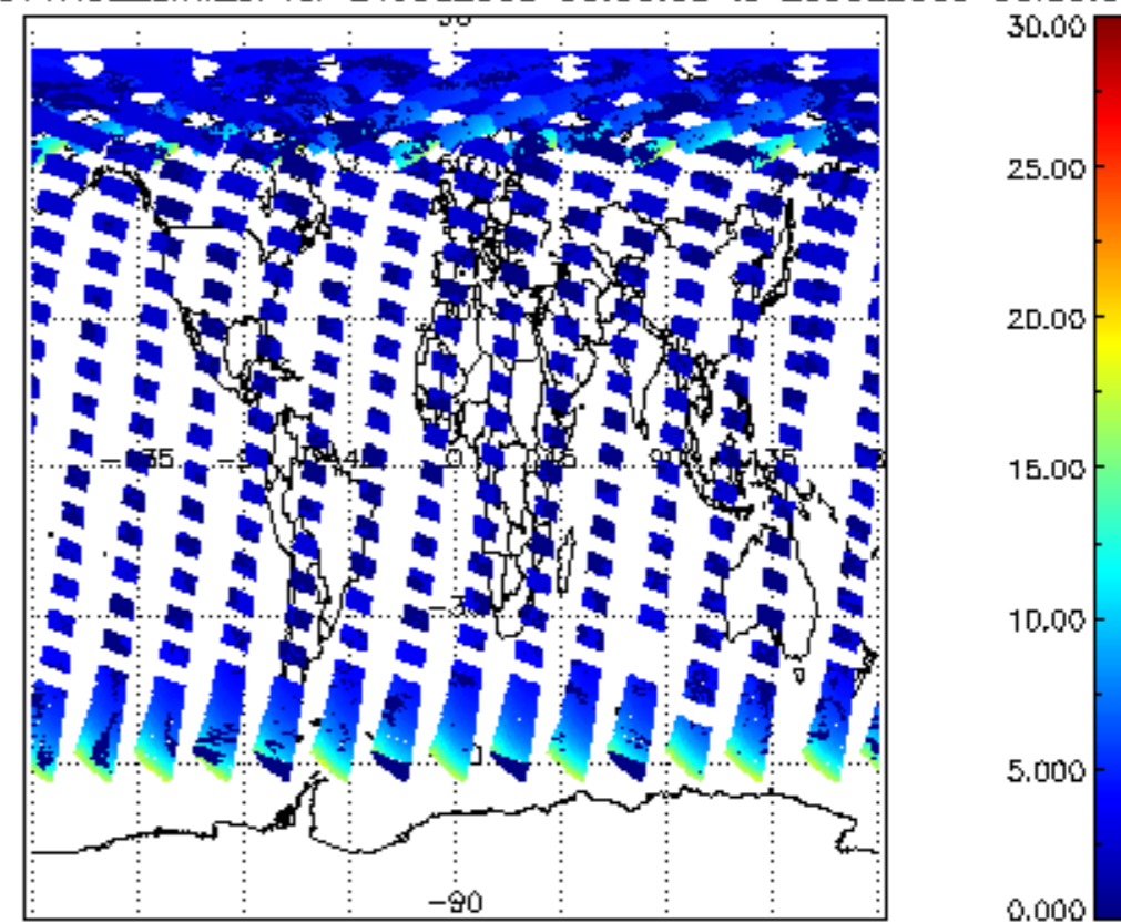
SCIOL2P_NADUV1NO2_amf_cl for 24JUL2009 00:00:00 to 25JUL2009 00:00:00
