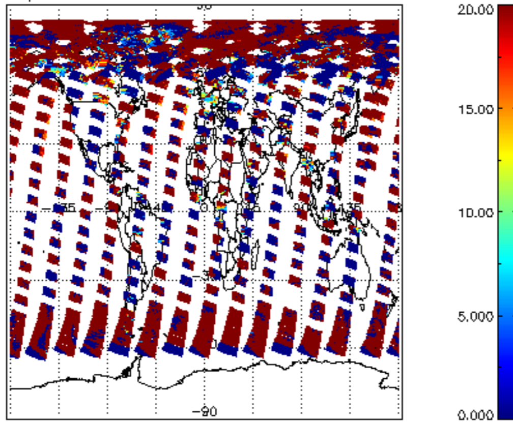
cl_lopt_depth for 24JUL2009 00:00:00 to 25JUL2009 00:00:00
