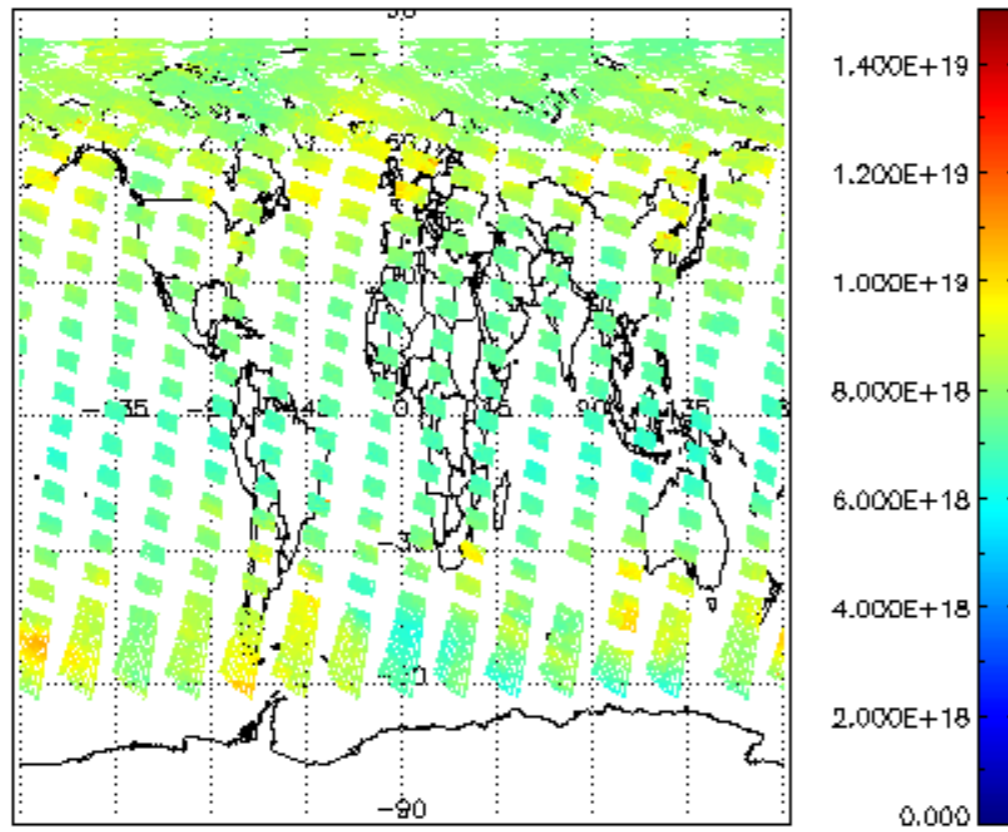
SCIOL2P_NADUV003_vcd for 24JUL2009 00:00:00 to 25JUL2009 00:00:00
