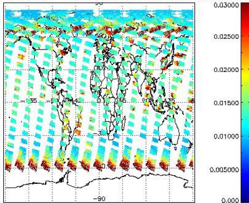
SCIOL2P_NADUV003_vcd_err for 24JUL2009 00:00:00 to 25JUL2009 00:00:00
