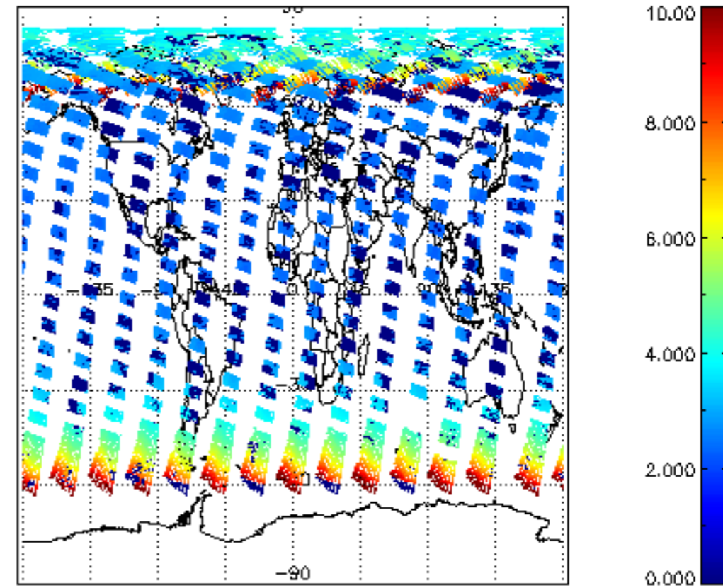
SCIOL2P_NADUV003_amf_cl for 24JUL2009 00:00:00 to 25JUL2009 00:00:00
