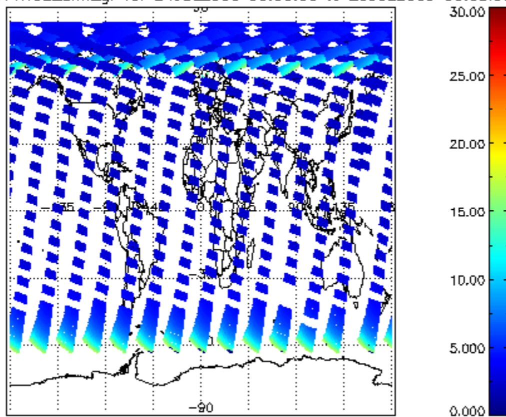
SCIOL2P_NADUV1NO2_amf_gr for 24JUL2009 00:00:00 to 25JUL2009 00:00:00
