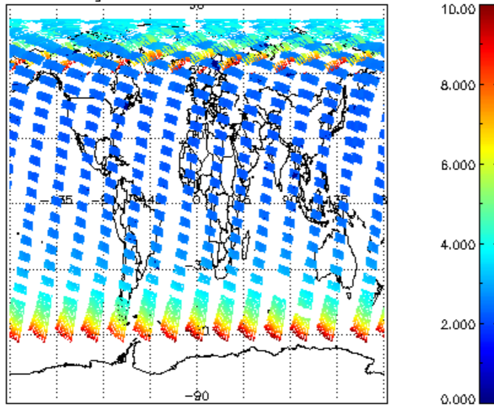
SCIOL2P_NADUV003_amf_gr for 24JUL2009 00:00:00 to 25JUL2009 00:00:00
