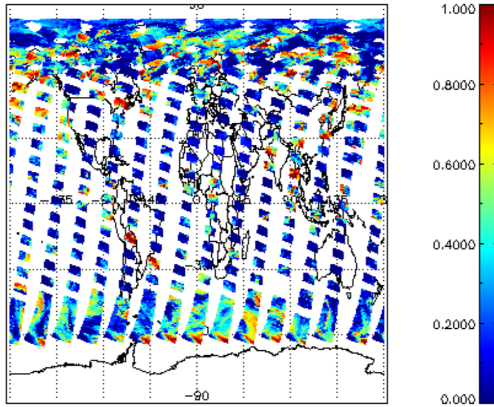
cl_frac for 24JUL2009 00:00:00 to 25JUL2009 00:00:00
