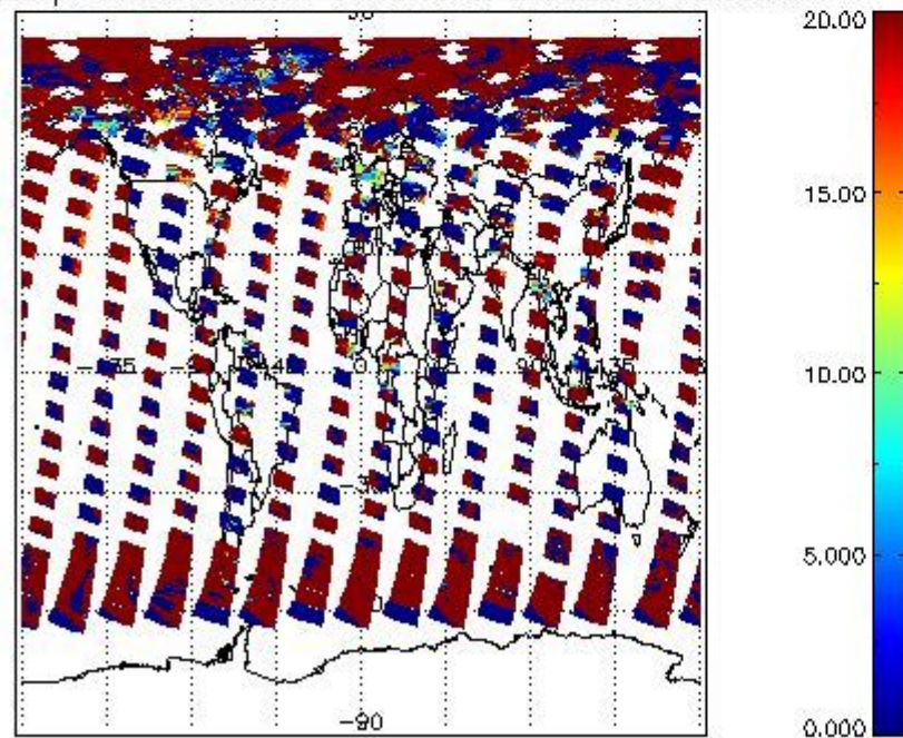
cL_opt_depth for 24JUL2009 00:00:00 to 25JUL2009 00:00:00
