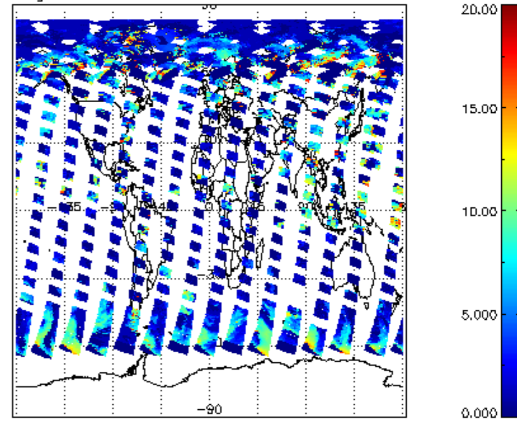
cl_top_height for 24JUL2009 00:00:00 to 25JUL2009 00:00:00
