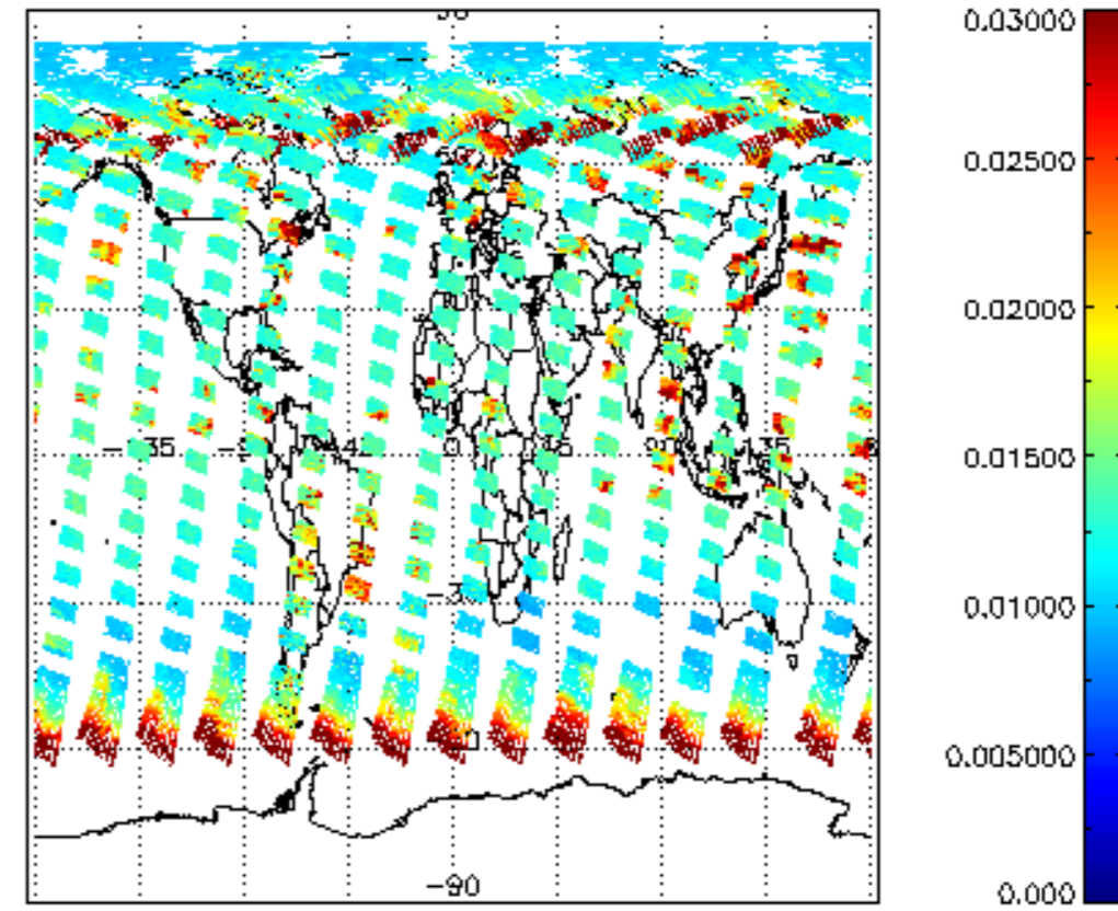
SCIOL2P_NADUV003_vcd_err for 24JUL2009 00:00:00 to 25JUL2009 00:00:00
