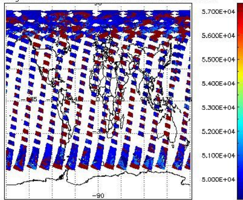
cloud_flags for 24JUL2009 00:00:00 to 25JUL2009 00:00:00
