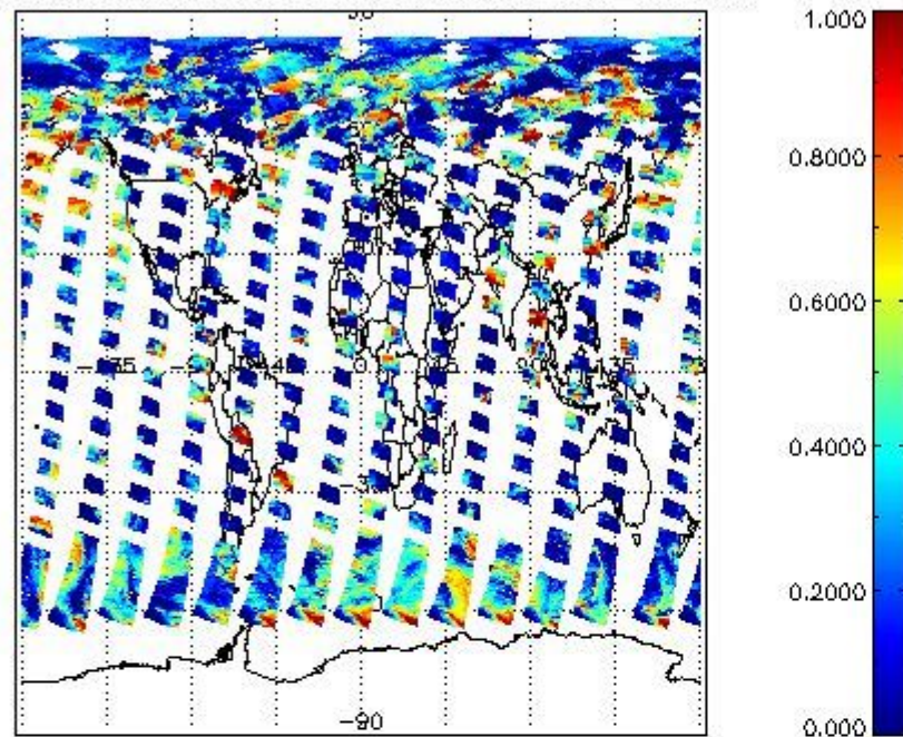
cL_frac for 24JUL2009 00:00:00 to 25JUL2009 00:00:00
