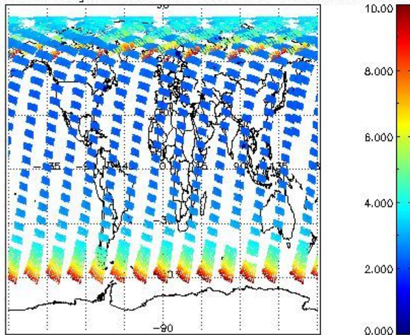
SCIOL2P_NADUV003_amf_gr for 24JUL2009 00:00:00 to 25JUL2009 00:00:00
