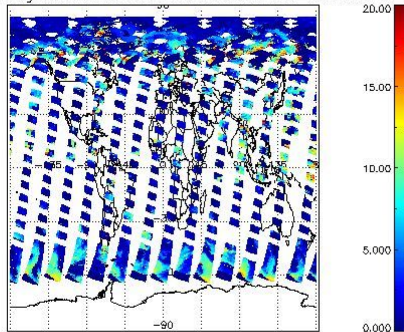
cL_top_height for 24JUL2009 00:00:00 to 25JUL2009 00:00:00
