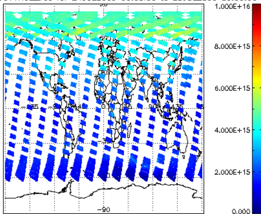
SCIOL2P_NADUV1NO2_vcd for 24JUL2009 00:00:00 to 25JUL2009 00:00:00
