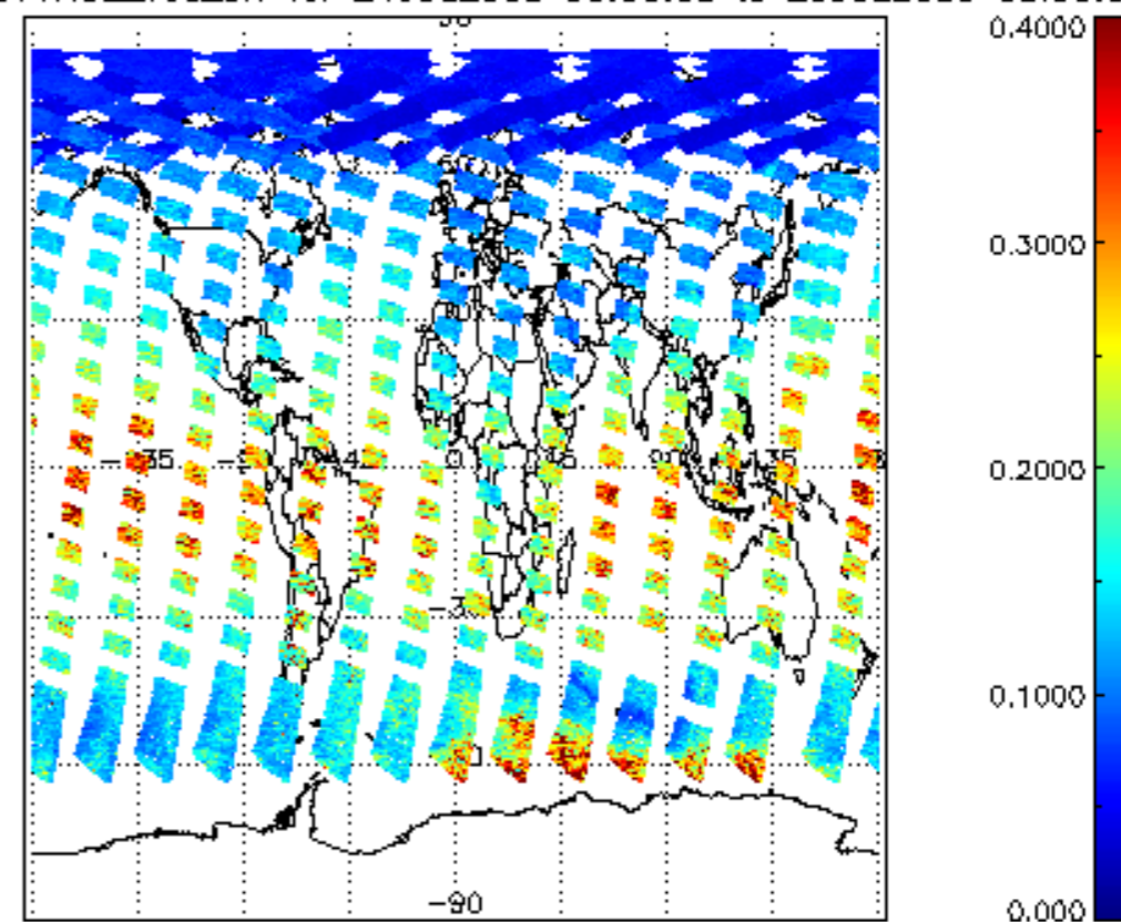
SCIOL2P_NADUV1NO2_vcd_err for 24JUL2009 00:00:00 to 25JUL2009 00:00:00
