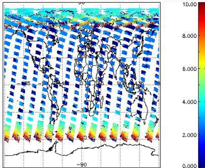
SCIOL2P_NADUV003_amf_cl for 24JUL2009 00:00:00 to 25JUL2009 00:00:00
