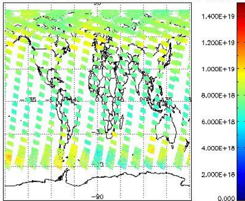
SCIOL2P_NADUV003_vcd for 24JUL2009 00:00:00 to 25JUL2009 00:00:00
