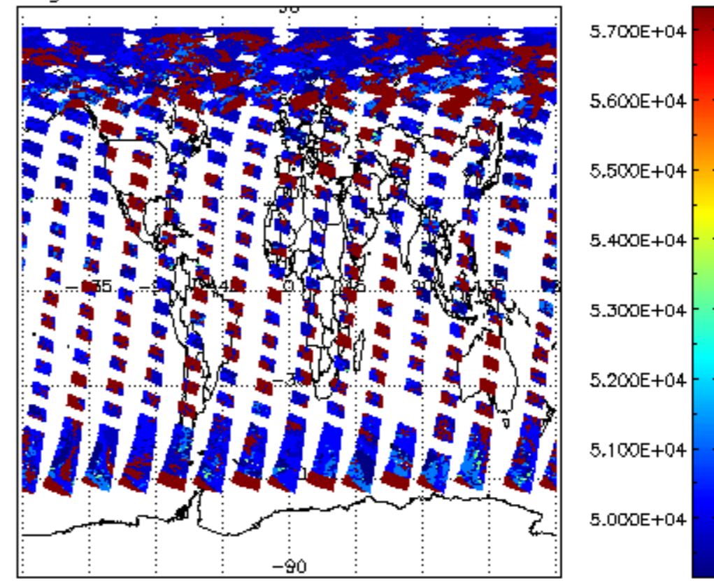
cloud_flags for 24JUL2009 00:00:00 to 25JUL2009 00:00:00
