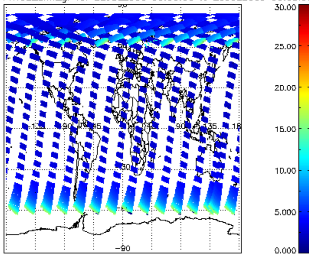
SCIOL2P_NADUV1NO2_amf_gr for 22JUL2009 00:00:00 to 23JUL2009 00:00:00
