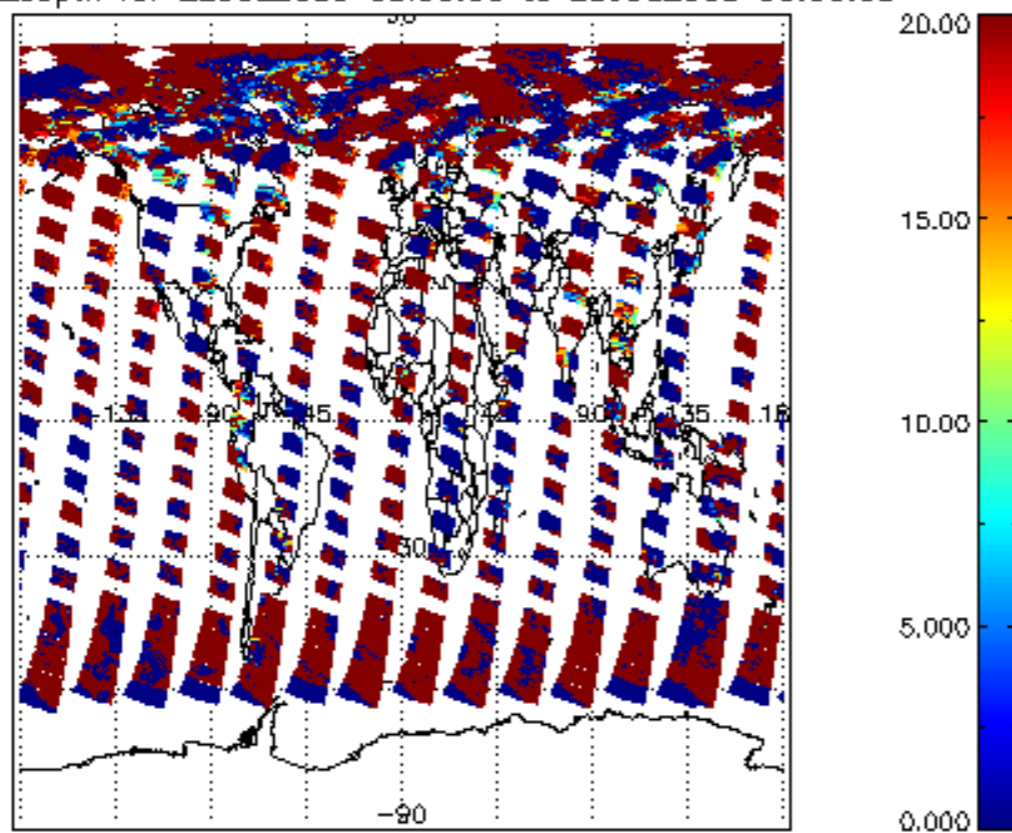
cl_opt_depth for 22JUL2009 00:00:00 to 23JUL2009 00:00:00
