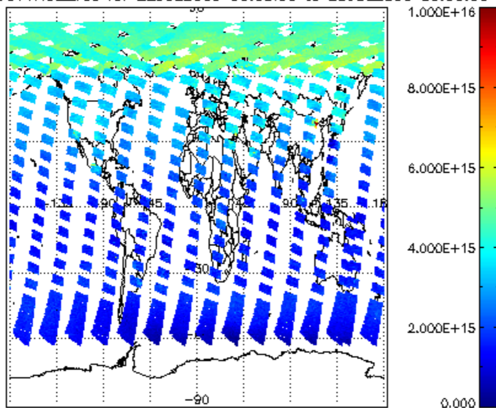
SCIOL2P_NADUV1NO2_vcd for 22JUL2009 00:00:00 to 23JUL2009 00:00:00
