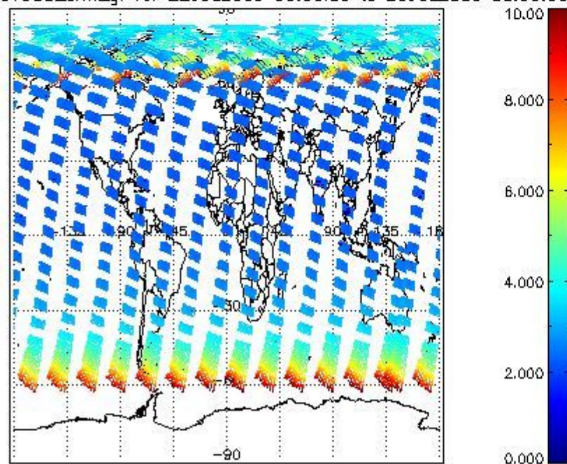
SCIOL2P_NADUV003_amf_gr for 22JUL2009 00:00:00 to 23JUL2009 00:00:00
