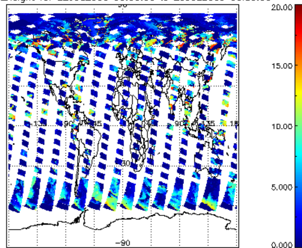
cl_top_height for 22JUL2009 00:00:00 to 23JUL2009 00:00:00
