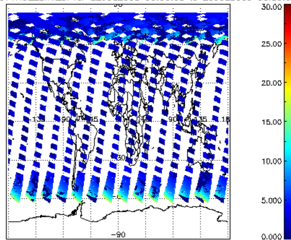
SCIOL2P_NADUV1NO2_amf_cl for 22JUL2009 00:00:00 to 23JUL2009 00:00:00
