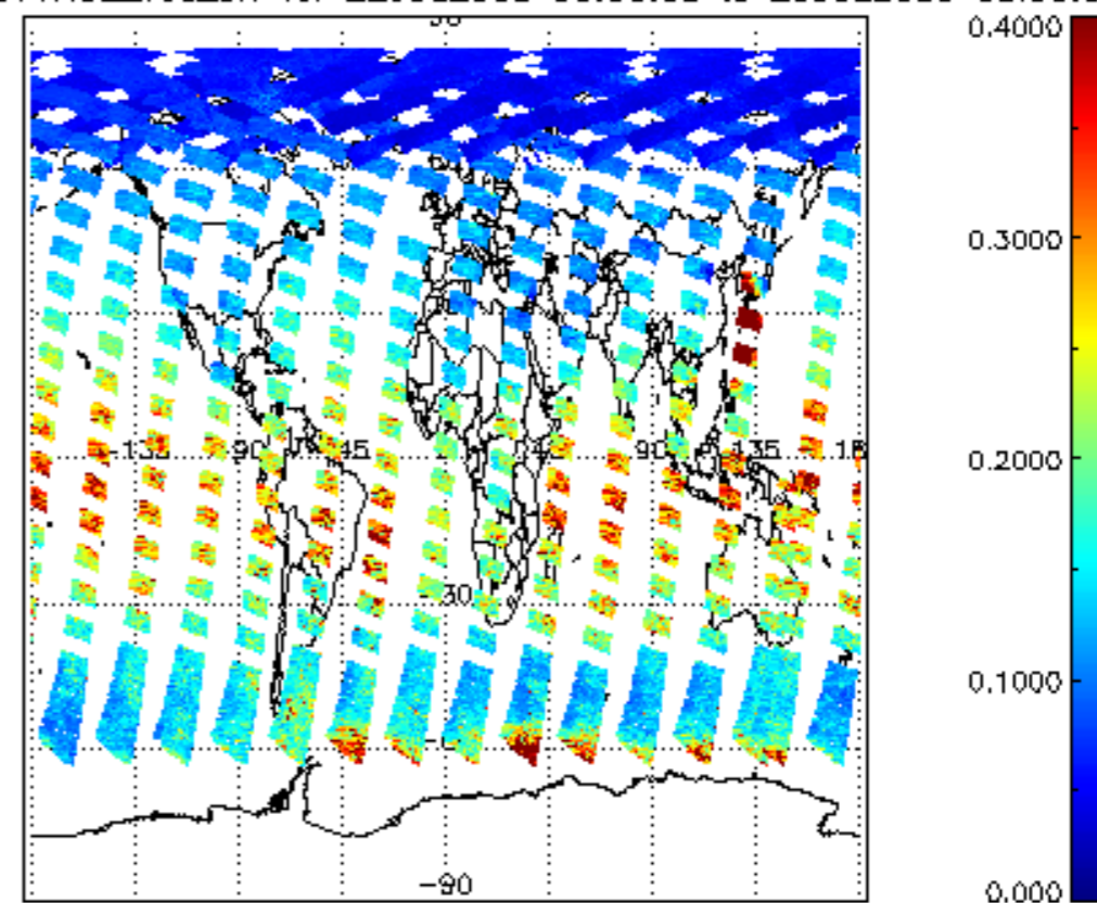
SCIOL2P_NADUV1NO2_vcd_err for 22JUL2009 00:00:00 to 23JUL2009 00:00:00
