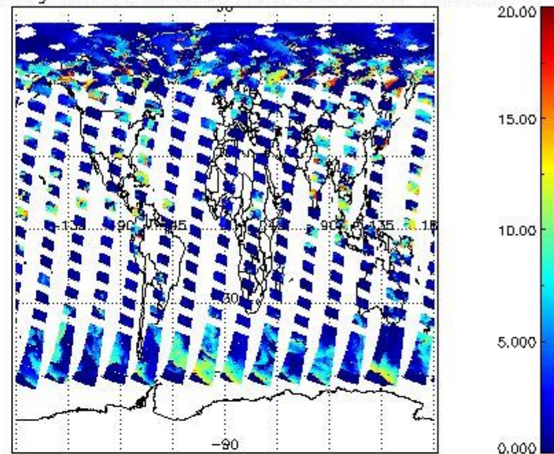
cL_top_height for 22JUL2009 00:00:00 to 23JUL2009 00:00:00
