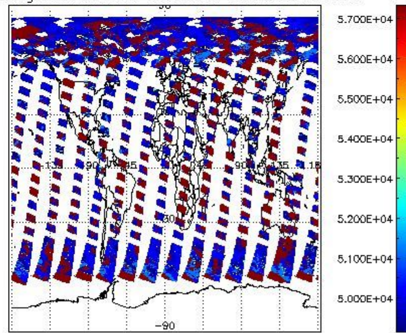
cloud_flags for 22JUL2009 00:00:00 to 23JUL2009 00:00:00
