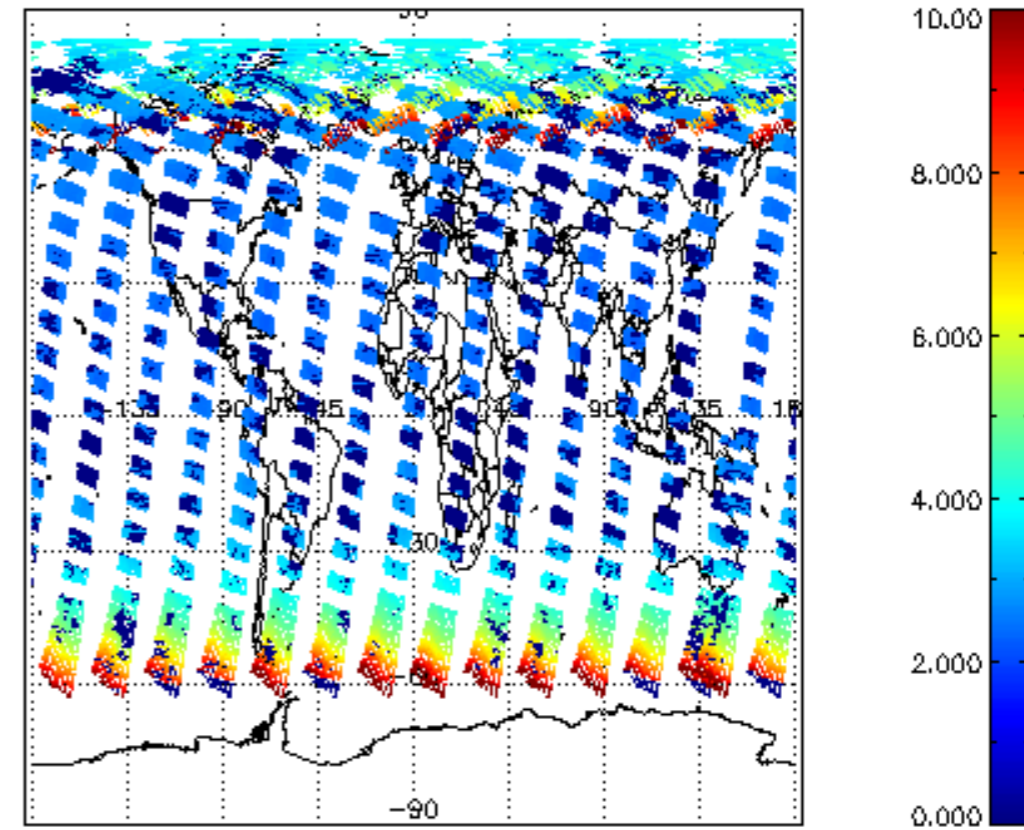
SCIOL2P_NADUV003_amf_cl for 22JUL2009 00:00:00 to 23JUL2009 00:00:00
