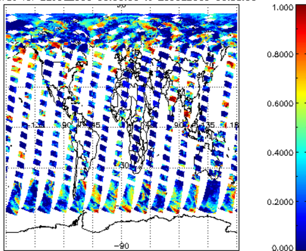
cl_frac for 22JUL2009 00:00:00 to 23JUL2009 00:00:00
