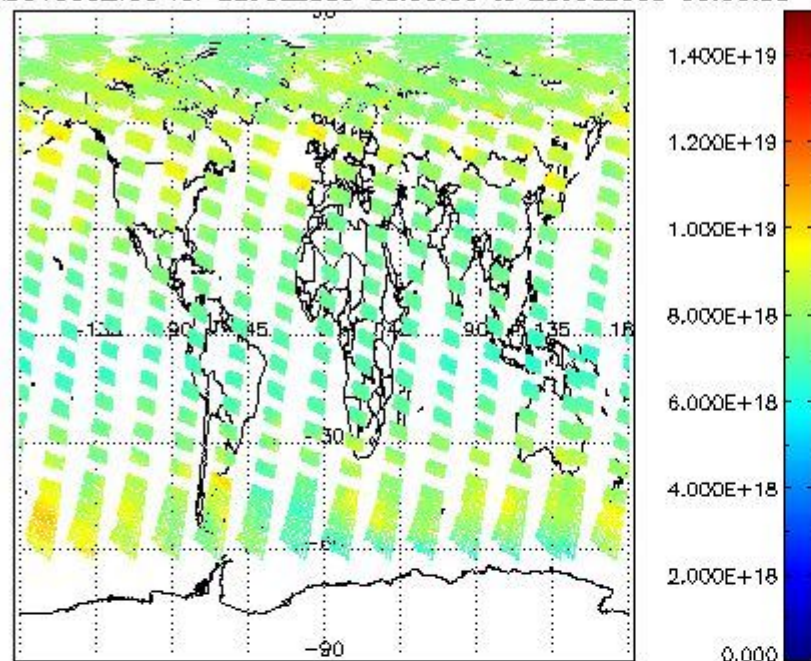
SCIOL2P_NADUV003_vcd for 22JUL2009 00:00:00 to 23JUL2009 00:00:00
