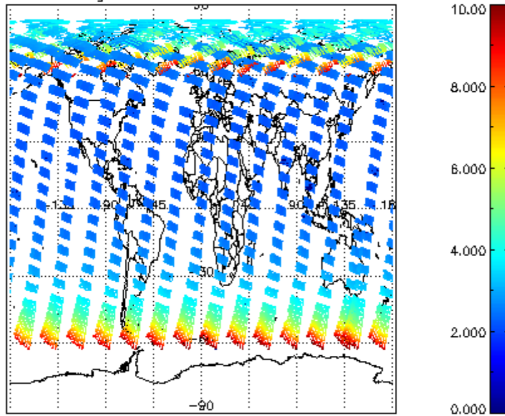
SCIOL2P_NADUV003_amf_gr for 22JUL2009 00:00:00 to 23JUL2009 00:00:00
