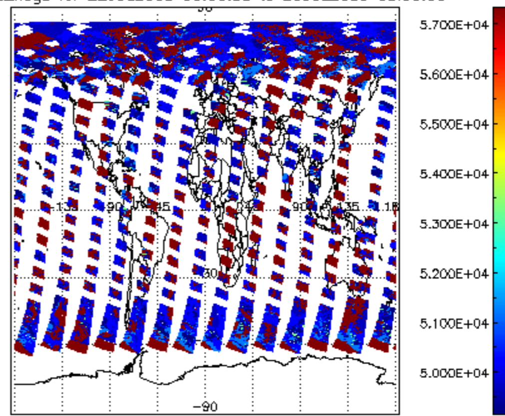
cloud_flags for 22JUL2009 00:00:00 to 23JUL2009 00:00:00
