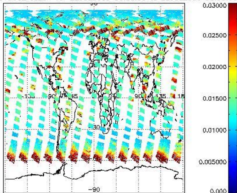
SCIOL2P_NADUV003_vcd_err for 22JUL2009 00:00:00 to 23JUL2009 00:00:00
