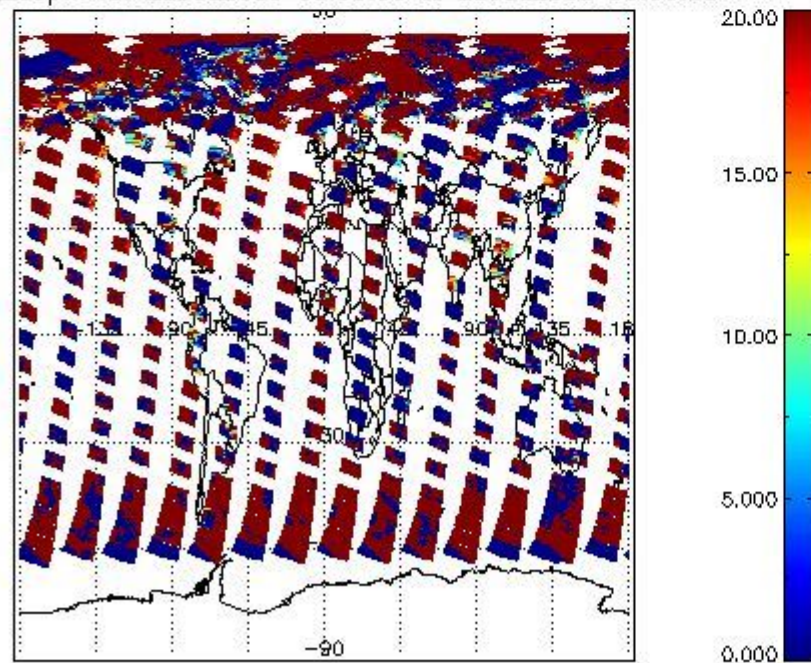
cL_opt_depth for 22JUL2009 00:00:00 to 23JUL2009 00:00:00
