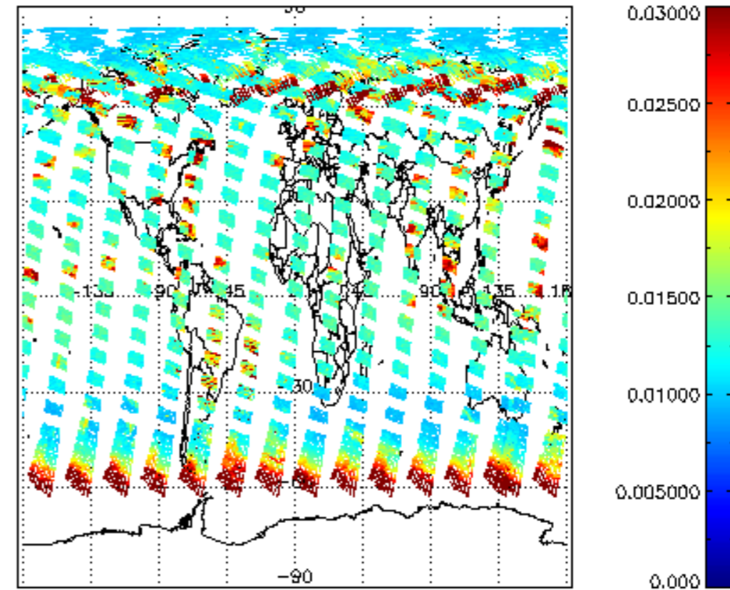
SCIOL2P_NADUV003_vcd_err for 22JUL2009 00:00:00 to 23JUL2009 00:00:00
