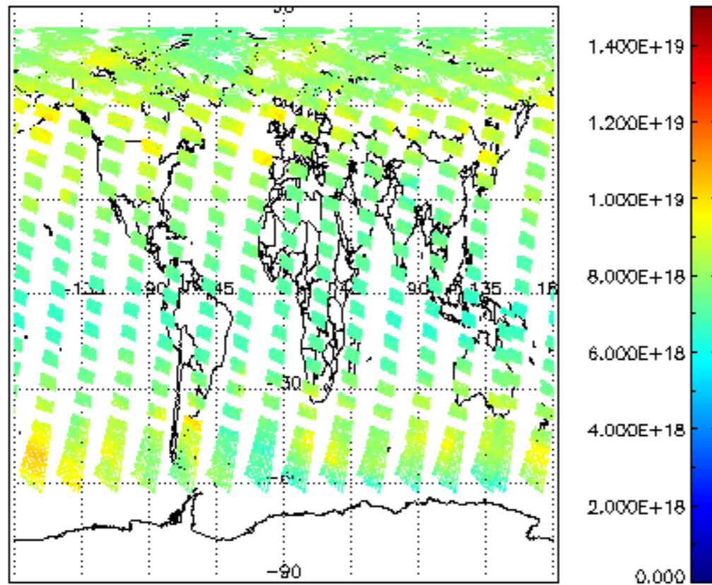
SCIOL2P_NADUV003_vcd for 22JUL2009 00:00:00 to 23JUL2009 00:00:00
