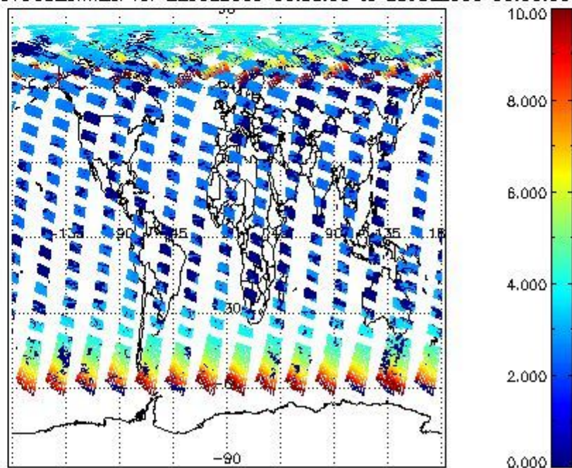
SCIOL2P_NADUV003_amf_cl for 22JUL2009 00:00:00 to 23JUL2009 00:00:00
