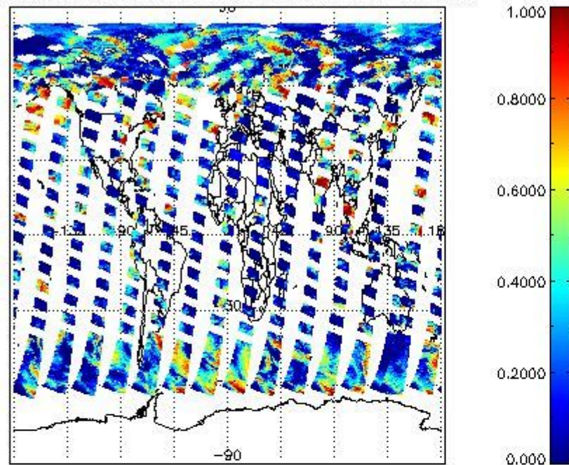
cL_frac for 22JUL2009 00:00:00 to 23JUL2009 00:00:00
