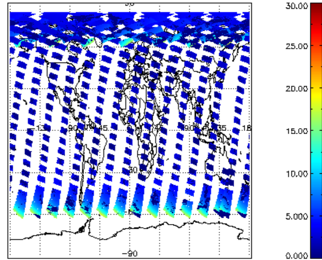
SCIOL2P_NADUV1NO2_amf_cl for 19JUL2009 00:00:00 to 20JUL2009 00:00:00
