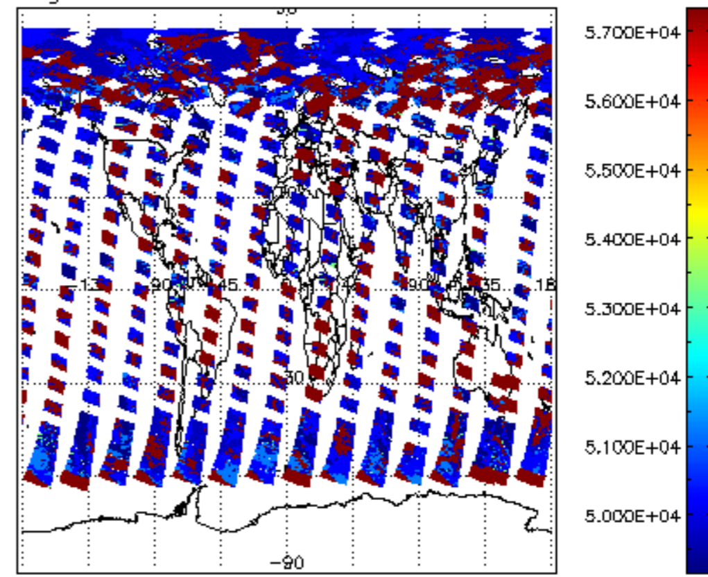
cloud_flags for 19JUL2009 00:00:00 to 20JUL2009 00:00:00
