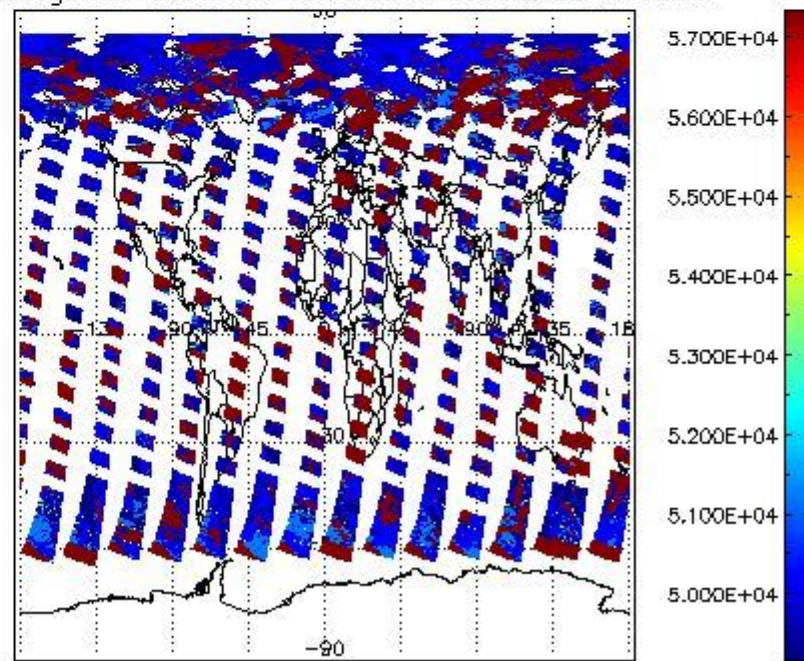
cloud_flags for 19JUL2009 00:00:00 to 20JUL2009 00:00:00
