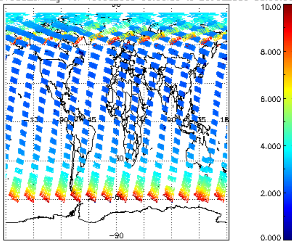
SCIOL2P_NADUV003_amf_gr for 19JUL2009 00:00:00 to 20JUL2009 00:00:00
