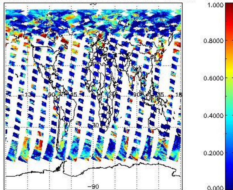
cL_frac for 19JUL2009 00:00:00 to 20JUL2009 00:00:00
