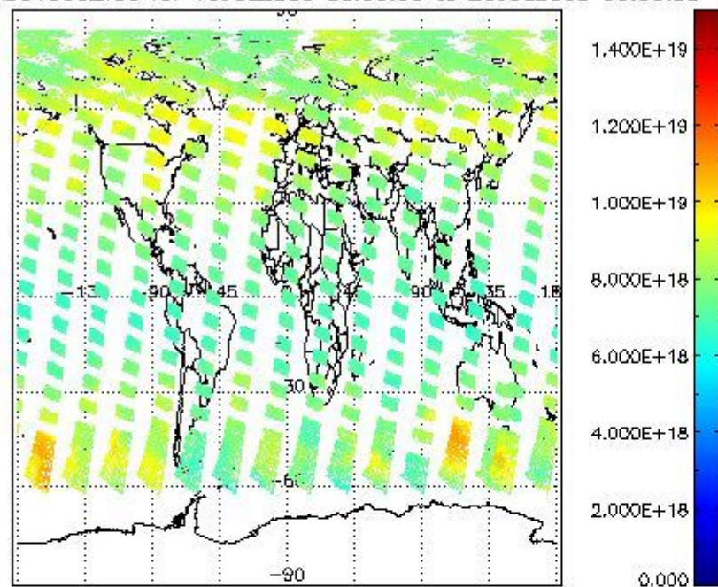
SCIOL2P_NADUV003_vcd for 19JUL2009 00:00:00 to 20JUL2009 00:00:00
