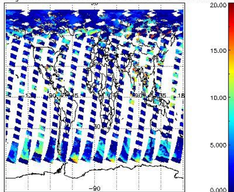
cL_top_height for 19JUL2009 00:00:00 to 20JUL2009 00:00:00
