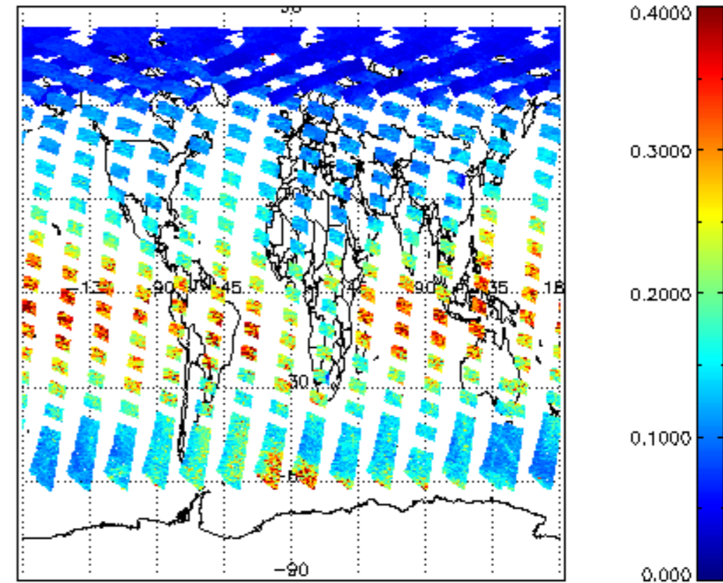
SCIOL2P_NADUV1NO2_vcd_err for 19JUL2009 00:00:00 to 20JUL2009 00:00:00
