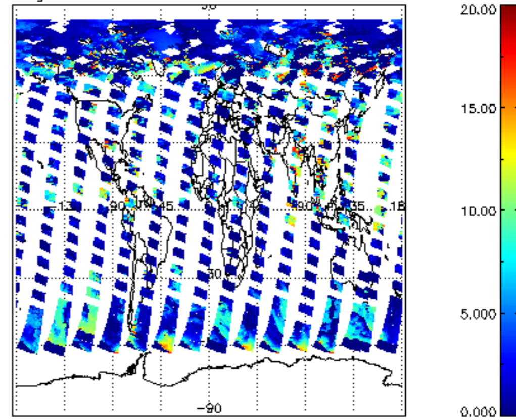
cl_top_height for 19JUL2009 00:00:00 to 20JUL2009 00:00:00
