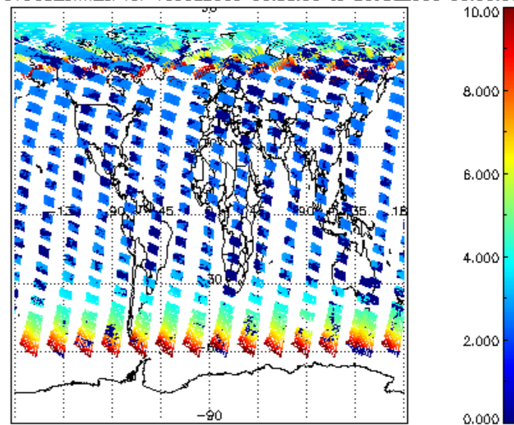
SCIOL2P_NADUV003_amf_cl for 19JUL2009 00:00:00 to 20JUL2009 00:00:00
