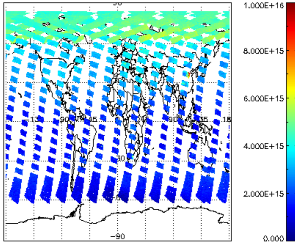
SCIOL2P_NADUV1NO2_vcd for 19JUL2009 00:00:00 to 20JUL2009 00:00:00
