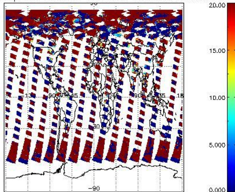
cL_opt_depth for 19JUL2009 00:00:00 to 20JUL2009 00:00:00
