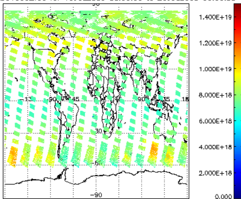
SCIOL2P_NADUV003_vcd for 19JUL2009 00:00:00 to 20JUL2009 00:00:00
