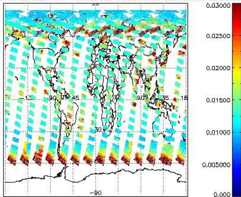
SCIOL2P_NADUV003_vcd_err for 19JUL2009 00:00:00 to 20JUL2009 00:00:00
