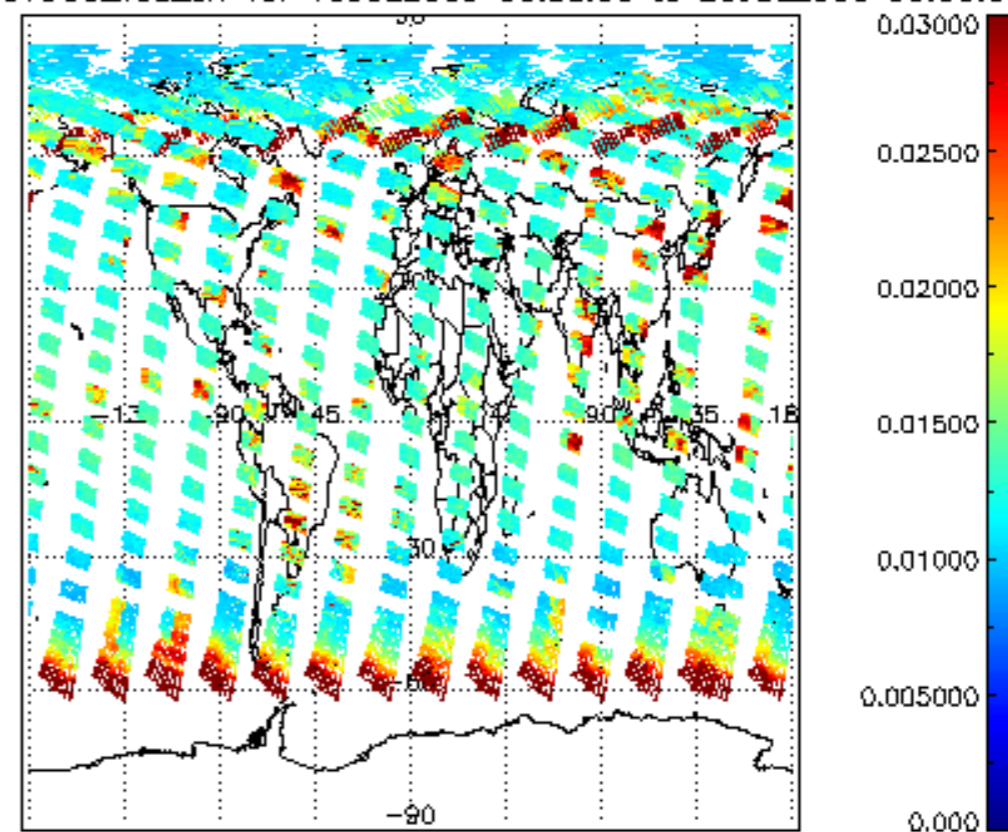
SCIOL2P_NADUV003_vcd_err for 19JUL2009 00:00:00 to 20JUL2009 00:00:00
