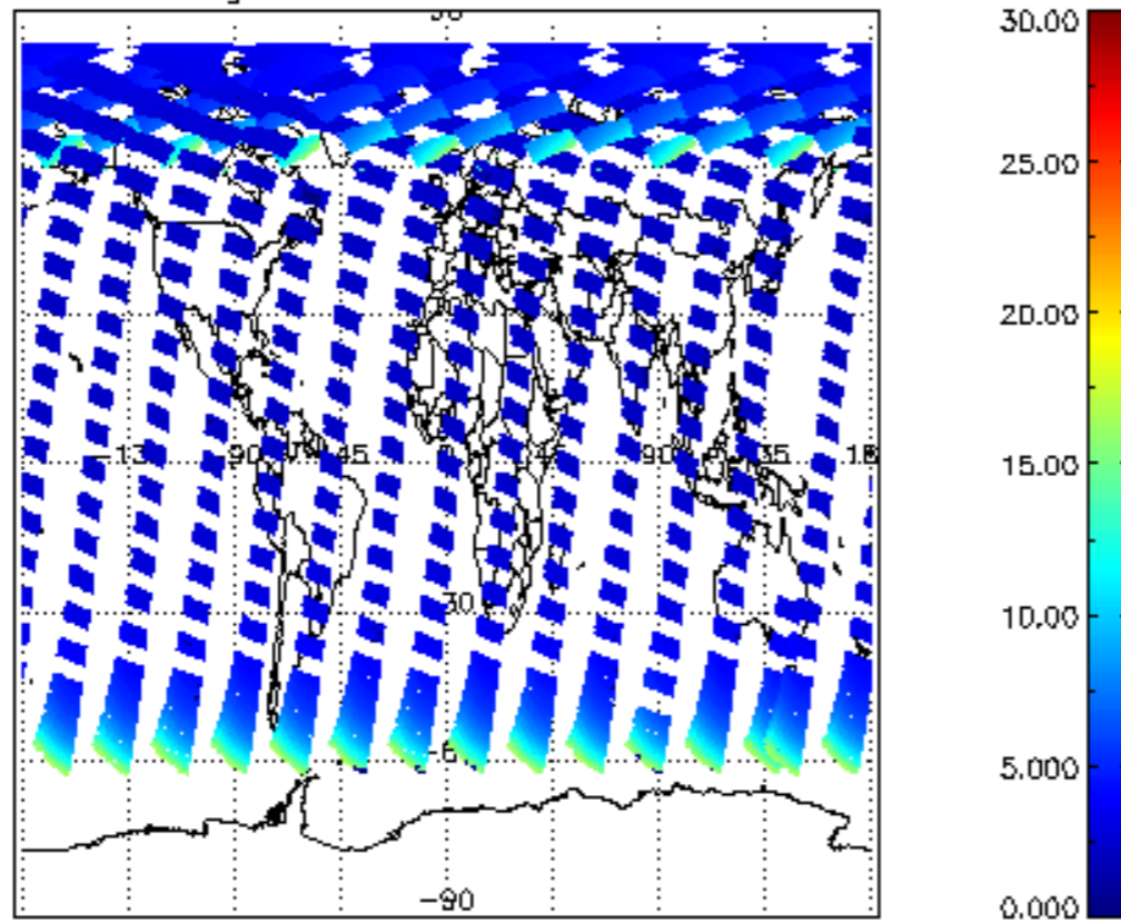
SCIOL2P_NADUV1NO2_amf_gr for 19JUL2009 00:00:00 to 20JUL2009 00:00:00
