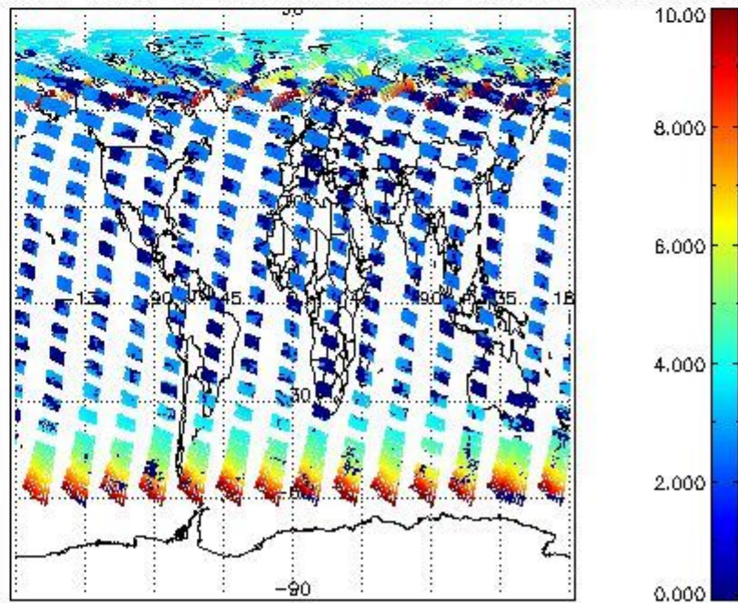
SCIOL2P_NADUV003_amf_cl for 19JUL2009 00:00:00 to 20JUL2009 00:00:00
