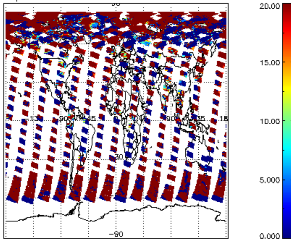
cl_lopt_depth for 19JUL2009 00:00:00 to 20JUL2009 00:00:00
