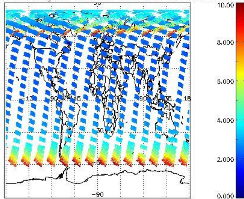
SCIOL2P_NADUV003_amf_gr for 19JUL2009 00:00:00 to 20JUL2009 00:00:00
