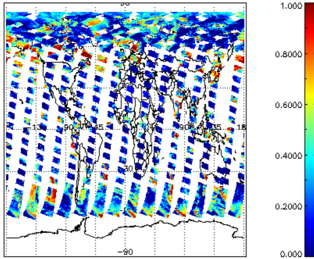
cl_frac for 19JUL2009 00:00:00 to 20JUL2009 00:00:00
