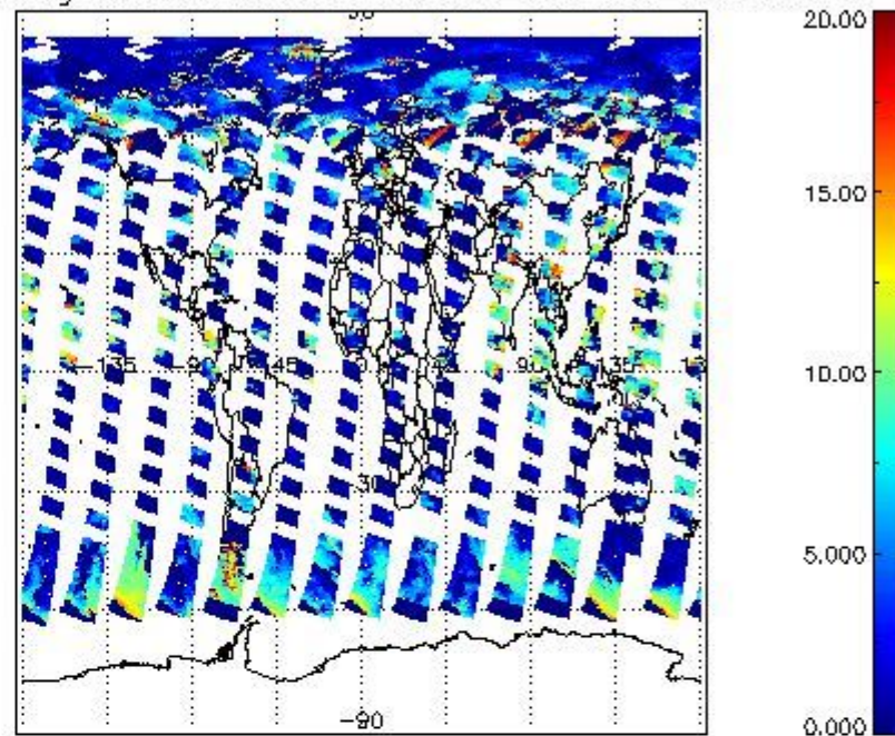
cL_top_height for 15JUL2009 00:00:00 to 16JUL2009 00:00:00
