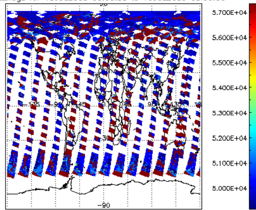
cloud_flags for 15JUL2009 00:00:00 to 16JUL2009 00:00:00
