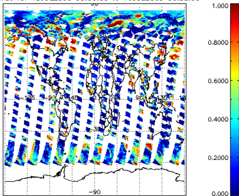
cl_frac for 15JUL2009 00:00:00 to 16JUL2009 00:00:00
