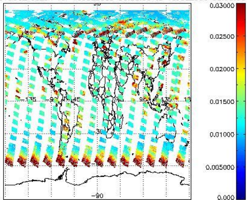
SCIOL2P_NADUV003_vcd_err for 15JUL2009 00:00:00 to 16JUL2009 00:00:00
