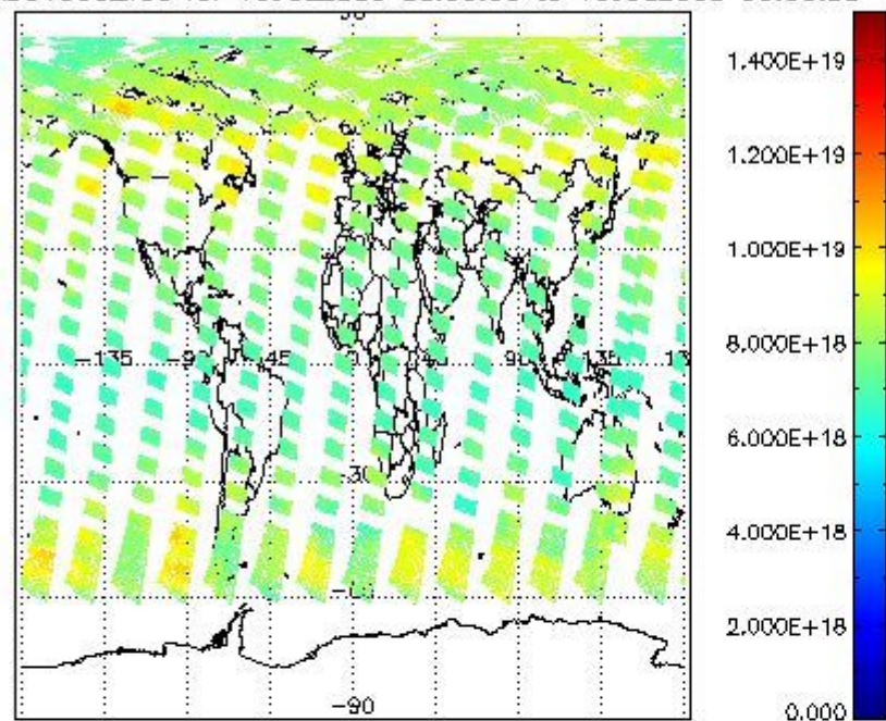
SCIOL2P_NADUV003_vcd for 15JUL2009 00:00:00 to 16JUL2009 00:00:00
