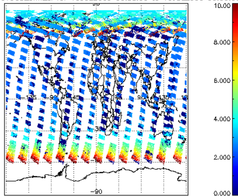
SCIOL2P_NADUV003_amf_cl for 15JUL2009 00:00:00 to 16JUL2009 00:00:00
