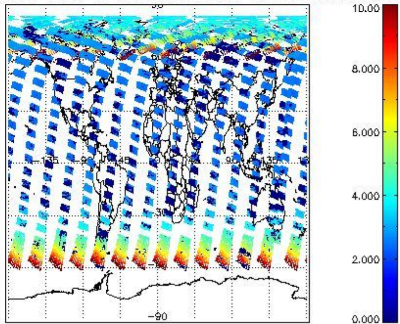
SCIOL2P_NADUV003_amf_cl for 15JUL2009 00:00:00 to 16JUL2009 00:00:00
