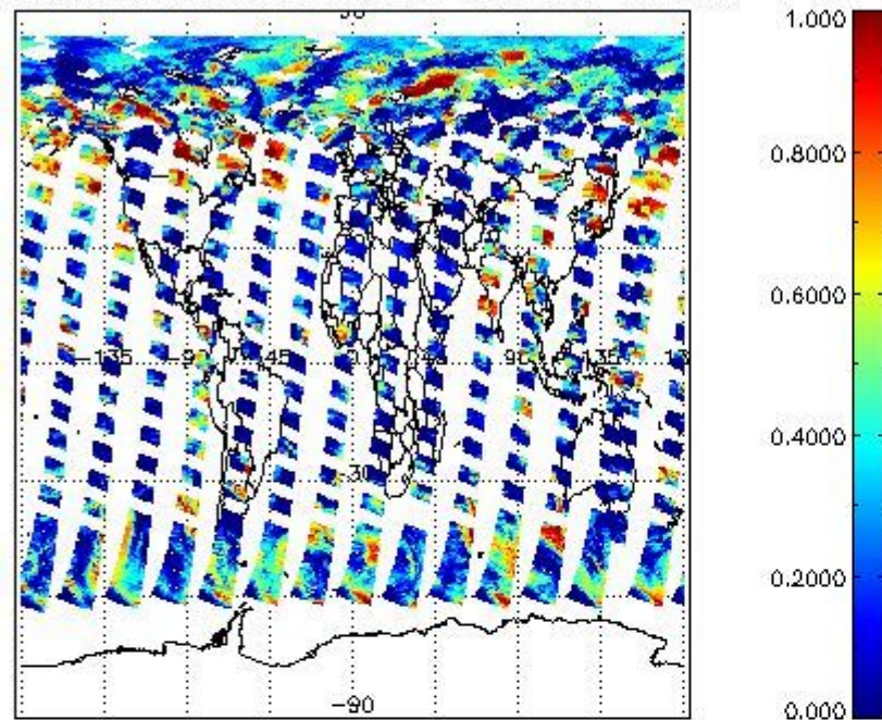
cL_frac for 15JUL2009 00:00:00 to 16JUL2009 00:00:00
