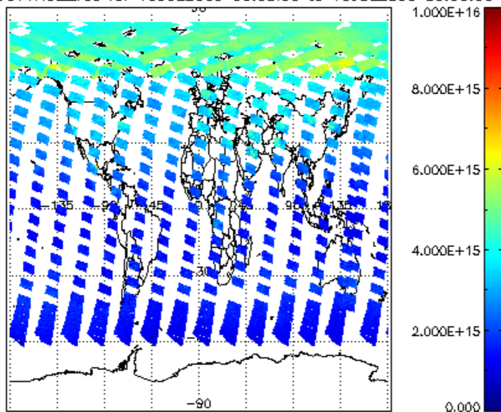
SCIOL2P_NADUV1NO2_vcd for 15JUL2009 00:00:00 to 16JUL2009 00:00:00
