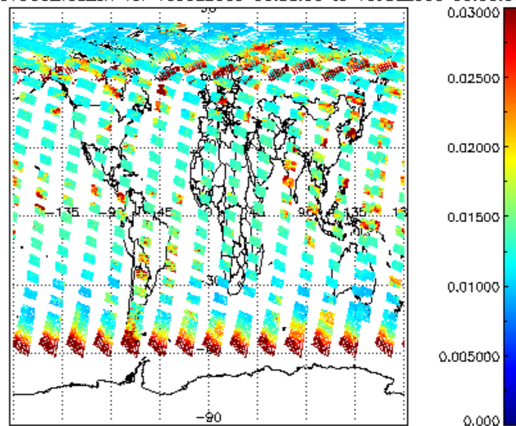
SCIOL2P_NADUV003_vcd_err for 15JUL2009 00:00:00 to 16JUL2009 00:00:00
