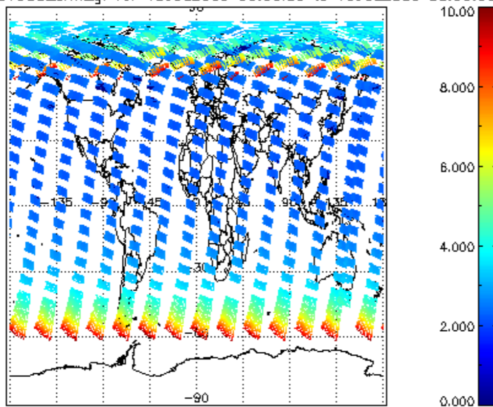
SCIOL2P_NADUV003_amf_gr for 15JUL2009 00:00:00 to 16JUL2009 00:00:00
