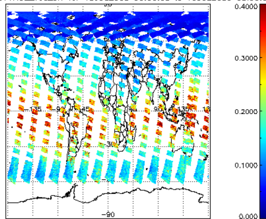
SCIOL2P_NADUV1NO2_vcd_err for 15JUL2009 00:00:00 to 16JUL2009 00:00:00
