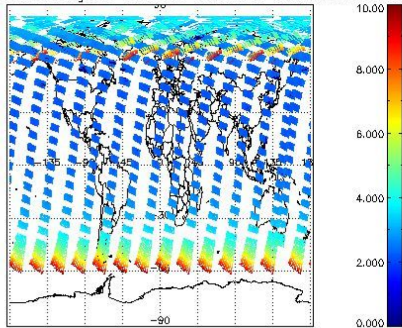
SCIOL2P_NADUV003_amf_gr for 15JUL2009 00:00:00 to 16JUL2009 00:00:00
