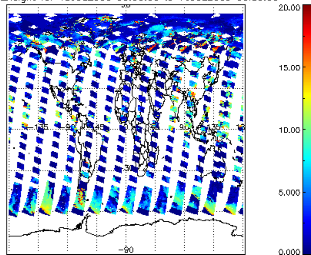
cl_top_height for 15JUL2009 00:00:00 to 16JUL2009 00:00:00
