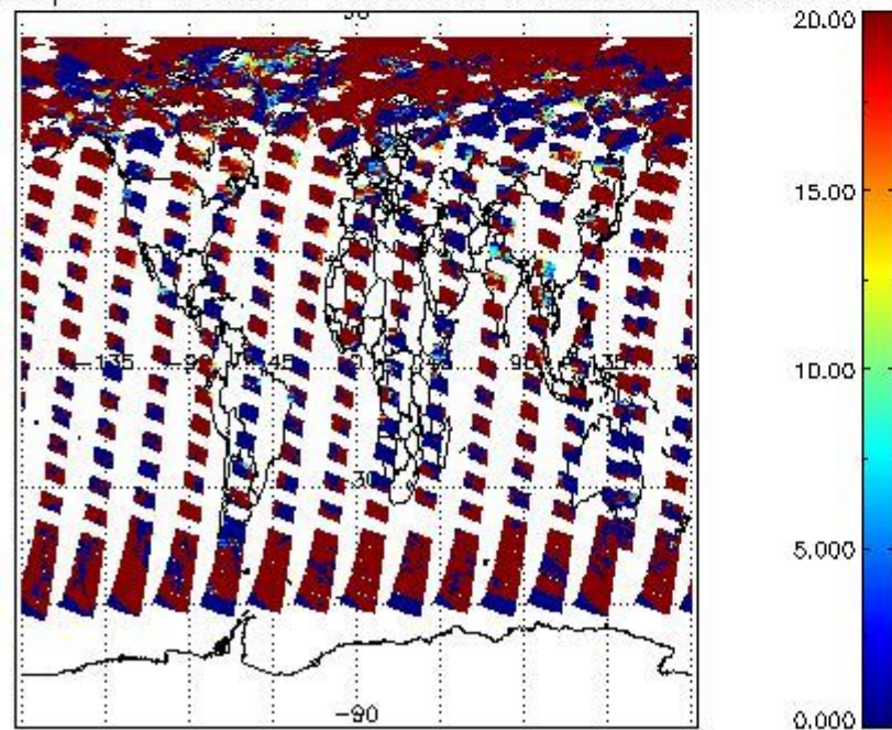
cL_opt_depth for 15JUL2009 00:00:00 to 16JUL2009 00:00:00
