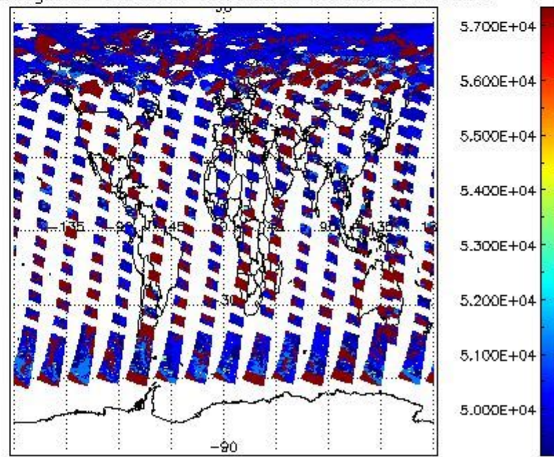
cloud_flags for 15JUL2009 00:00:00 to 16JUL2009 00:00:00
