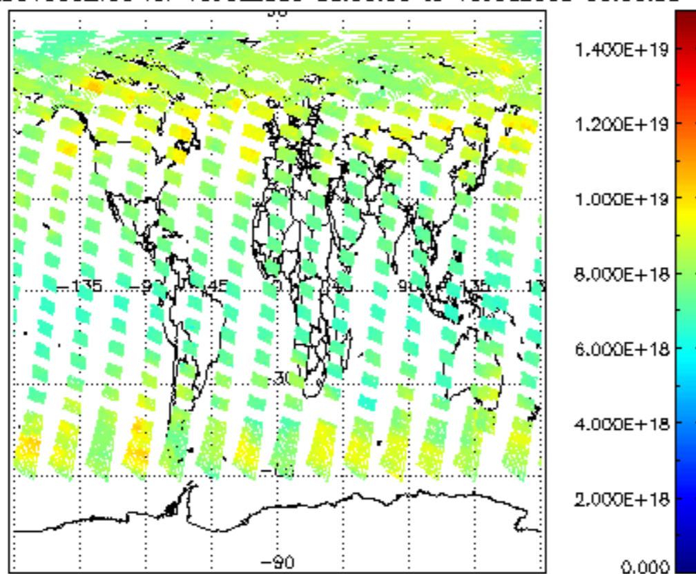
SCIOL2P_NADUV003_vcd for 15JUL2009 00:00:00 to 16JUL2009 00:00:00
