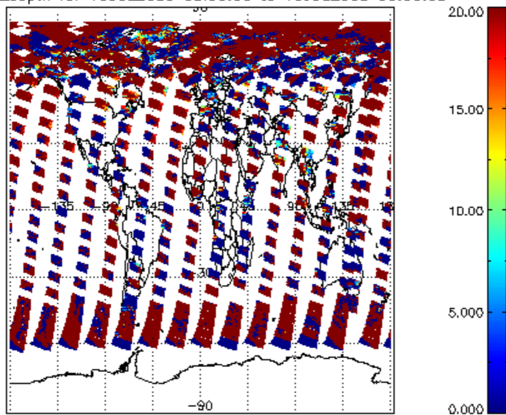
cl_lopt_depth for 15JUL2009 00:00:00 to 16JUL2009 00:00:00
