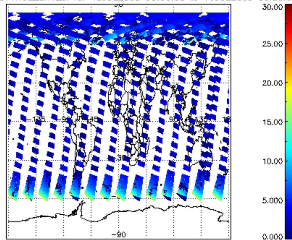
SCIOL2P_NADUV1NO2_amf_cl for 15JUL2009 00:00:00 to 16JUL2009 00:00:00
