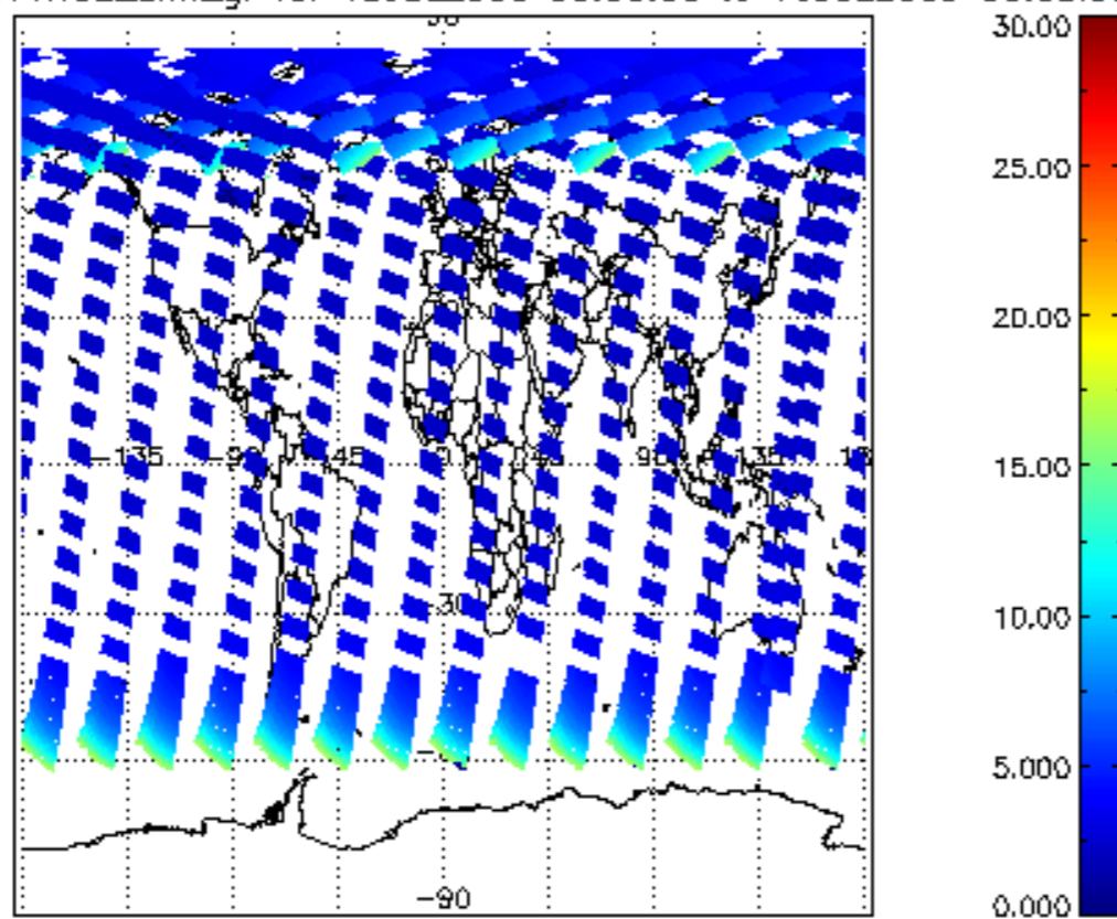
SCIOL2P_NADUV1NO2_amf_gr for 15JUL2009 00:00:00 to 16JUL2009 00:00:00
