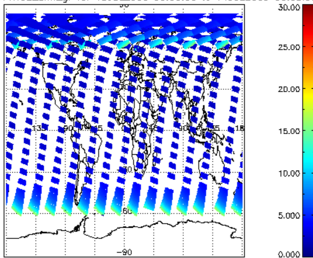
SCIOL2P_NADUV1NO2_amf_gr for 13JUL2009 00:00:00 to 14JUL2009 00:00:00
