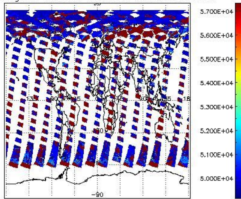
cloud_flags for 13JUL2009 00:00:00 to 14JUL2009 00:00:00
