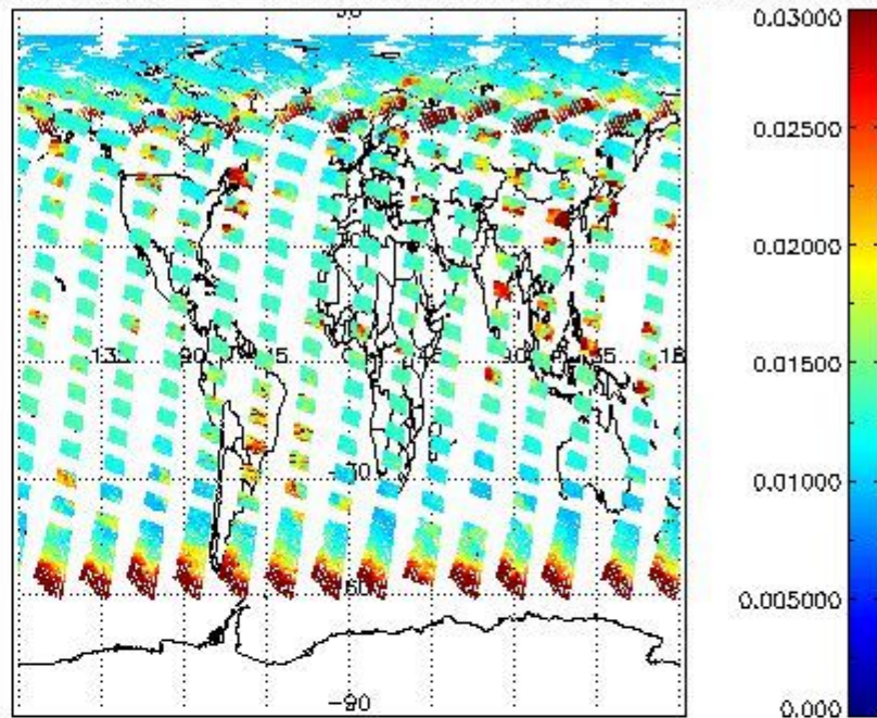
SCIOL2P_NADUV003_vcd_err for 13JUL2009 00:00:00 to 14JUL2009 00:00:00
