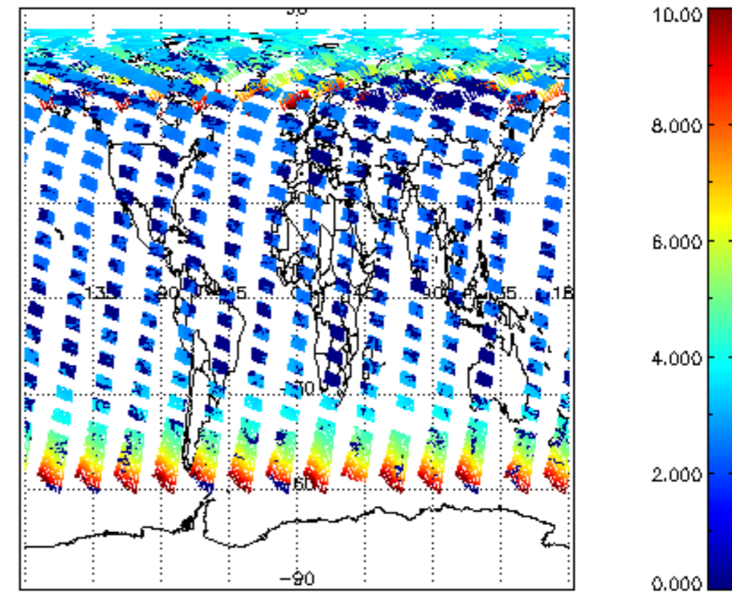
SCIOL2P_NADUV003_amf_cl for 13JUL2009 00:00:00 to 14JUL2009 00:00:00
