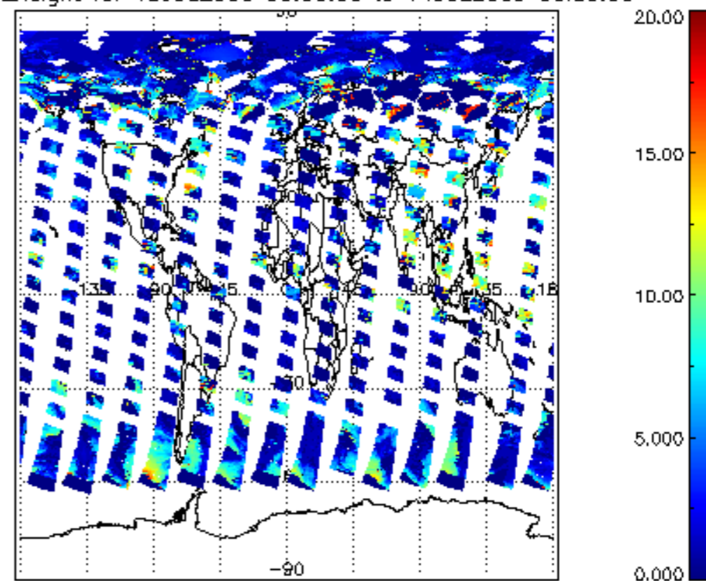
cl_top_height for 13JUL2009 00:00:00 to 14JUL2009 00:00:00
