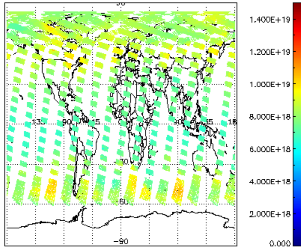
SCIOL2P_NADUV003_vcd for 13JUL2009 00:00:00 to 14JUL2009 00:00:00
