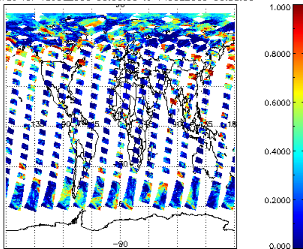
cl_frac for 13JUL2009 00:00:00 to 14JUL2009 00:00:00
