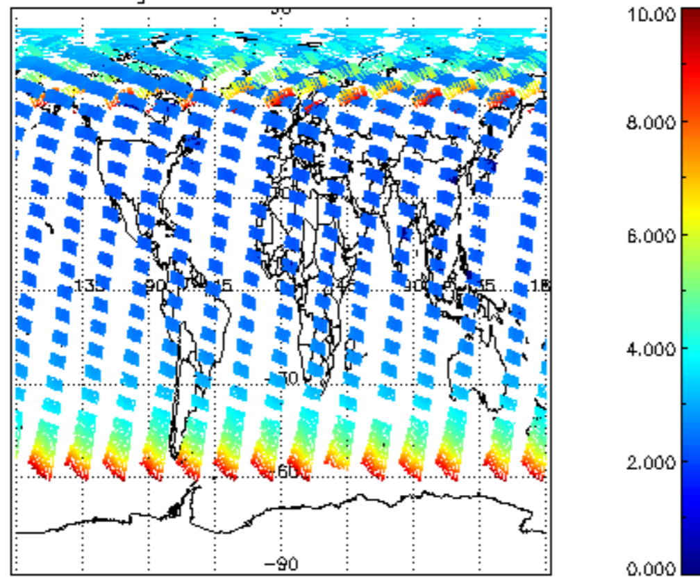
SCIOL2P_NADUV003_amf_gr for 13JUL2009 00:00:00 to 14JUL2009 00:00:00
