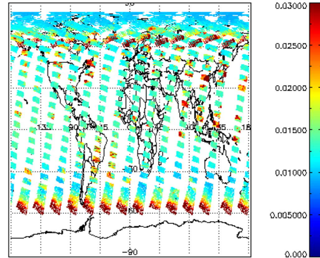
SCIOL2P_NADUV003_vcd_err for 13JUL2009 00:00:00 to 14JUL2009 00:00:00
