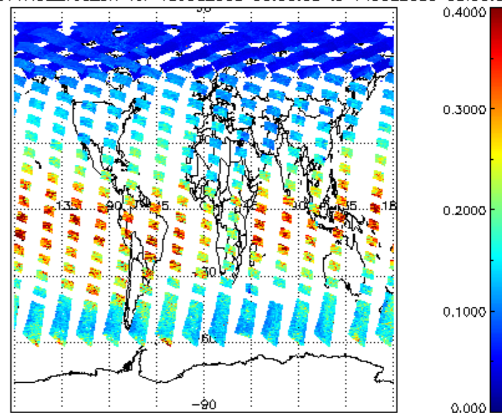
SCIOL2P_NADUV1NO2_vcd_err for 13JUL2009 00:00:00 to 14JUL2009 00:00:00
