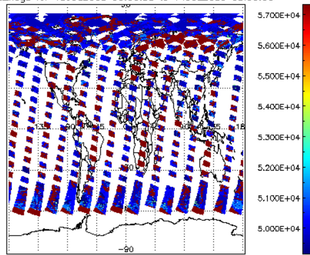
cloud_flags for 13JUL2009 00:00:00 to 14JUL2009 00:00:00
