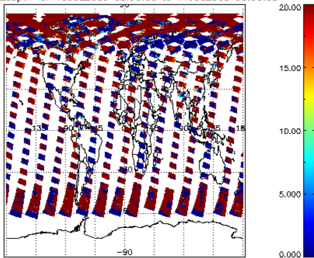
cl_lopt_depth for 13JUL2009 00:00:00 to 14JUL2009 00:00:00
