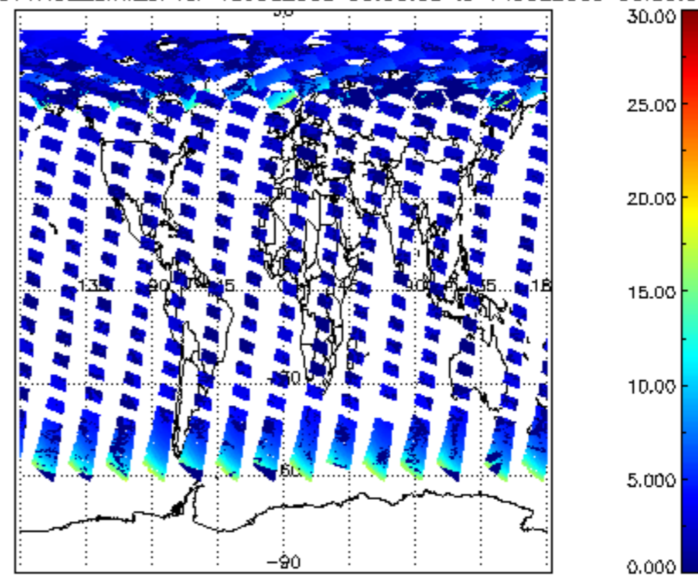
SCIOL2P_NADUV1NO2_amf_cl for 13JUL2009 00:00:00 to 14JUL2009 00:00:00
