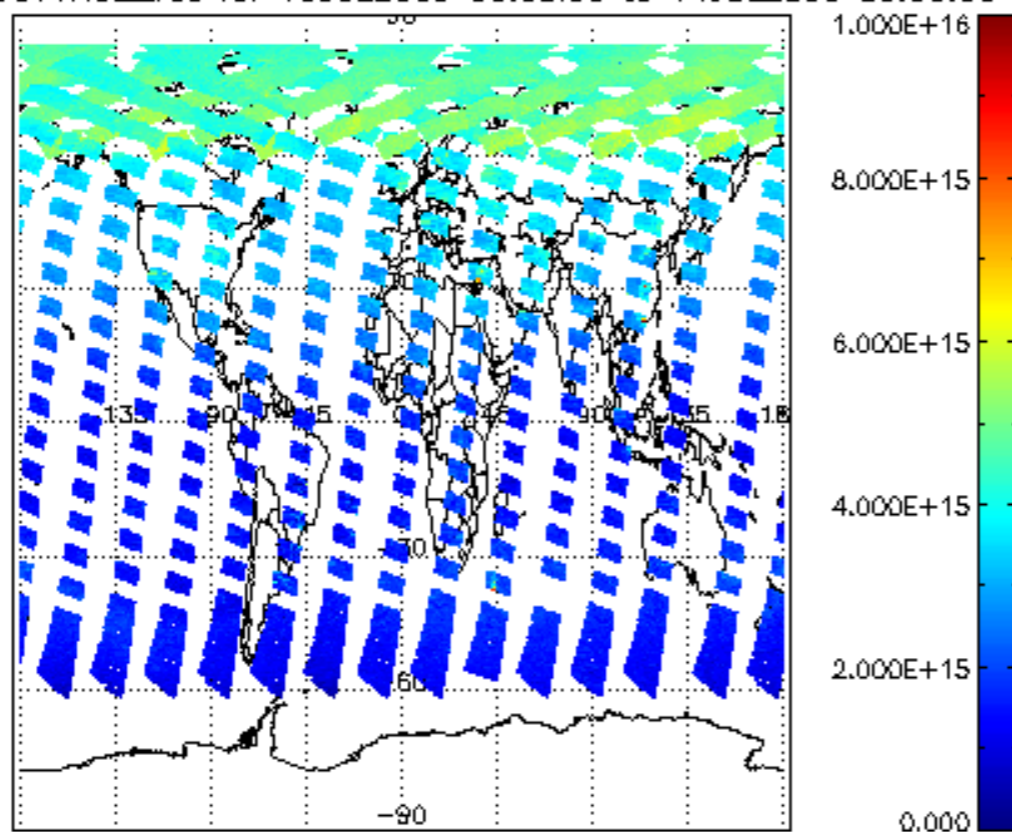
SCIOL2P_NADUV1NO2_vcd for 13JUL2009 00:00:00 to 14JUL2009 00:00:00
