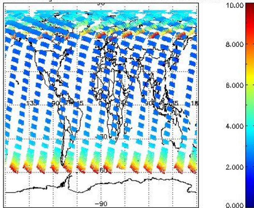
SCIOL2P_NADUV003_amf_gr for 13JUL2009 00:00:00 to 14JUL2009 00:00:00
