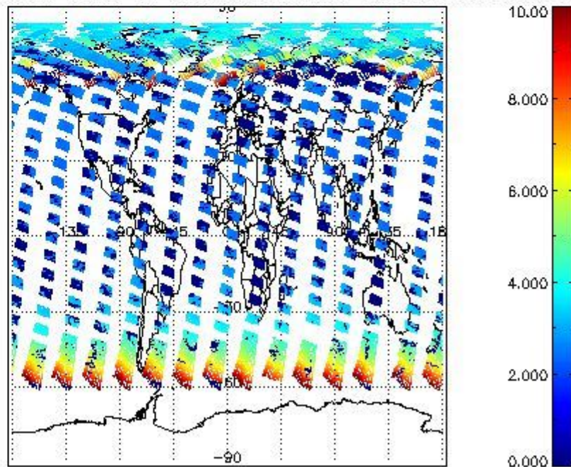
SCIOL2P_NADUV003_amf_cl for 13JUL2009 00:00:00 to 14JUL2009 00:00:00
