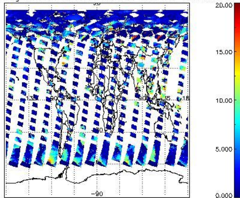
cL_top_height for 13JUL2009 00:00:00 to 14JUL2009 00:00:00
