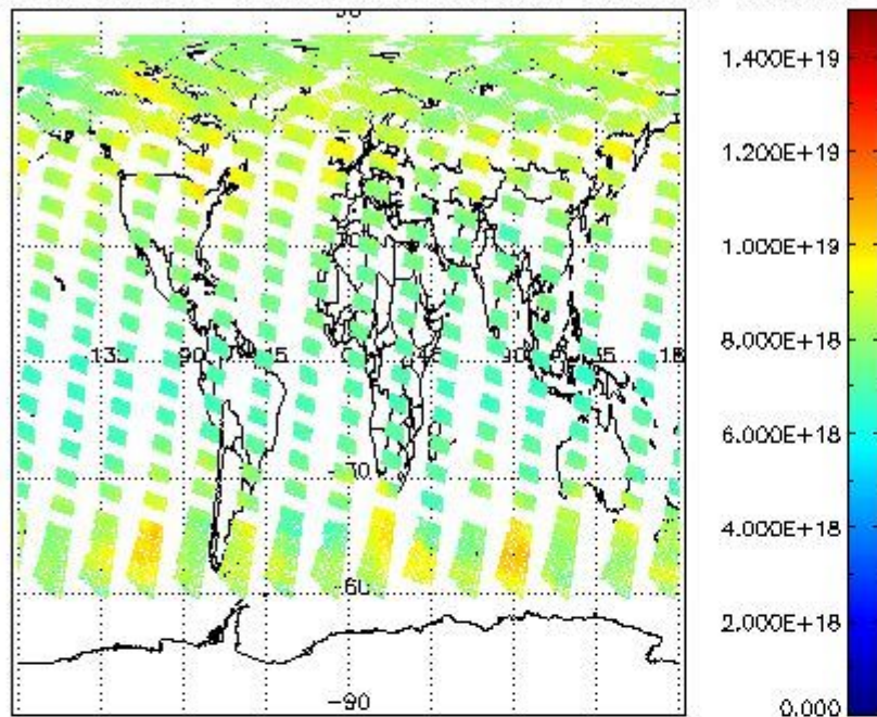
SCIOL2P_NADUV003_vcd for 13JUL2009 00:00:00 to 14JUL2009 00:00:00
