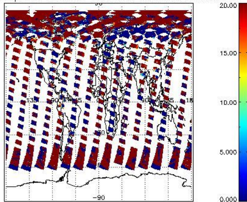
cL_opt_depth for 13JUL2009 00:00:00 to 14JUL2009 00:00:00
