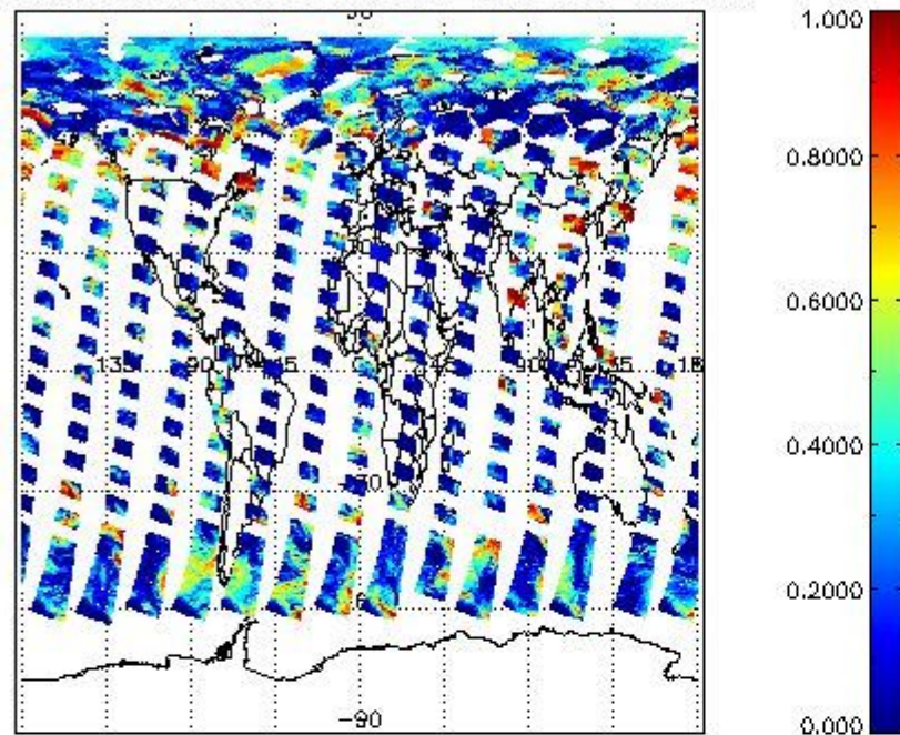
cL_frac for 13JUL2009 00:00:00 to 14JUL2009 00:00:00
