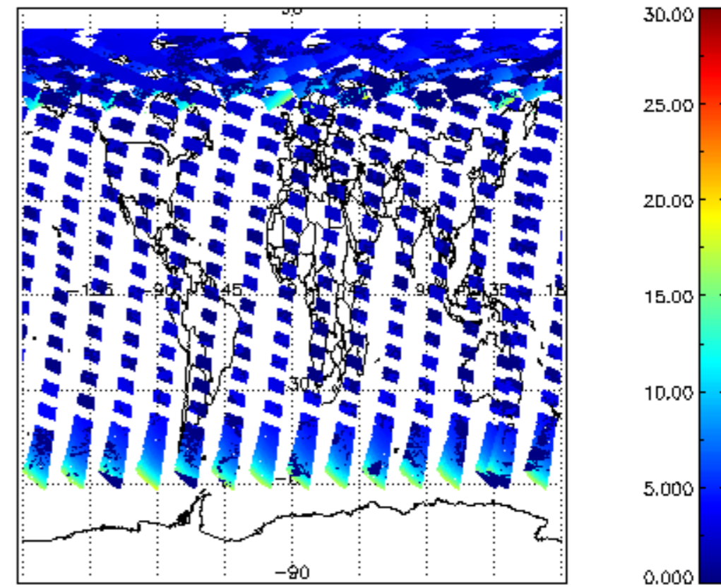
SCIOL2P_NADUV1NO2_amf_cl for 12JUL2009 00:00:00 to 13JUL2009 00:00:00
