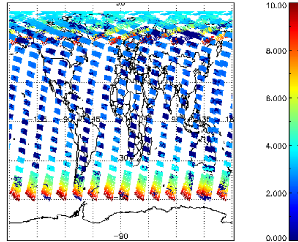
SCIOL2P_NADUV003_amf_cl for 12JUL2009 00:00:00 to 13JUL2009 00:00:00
