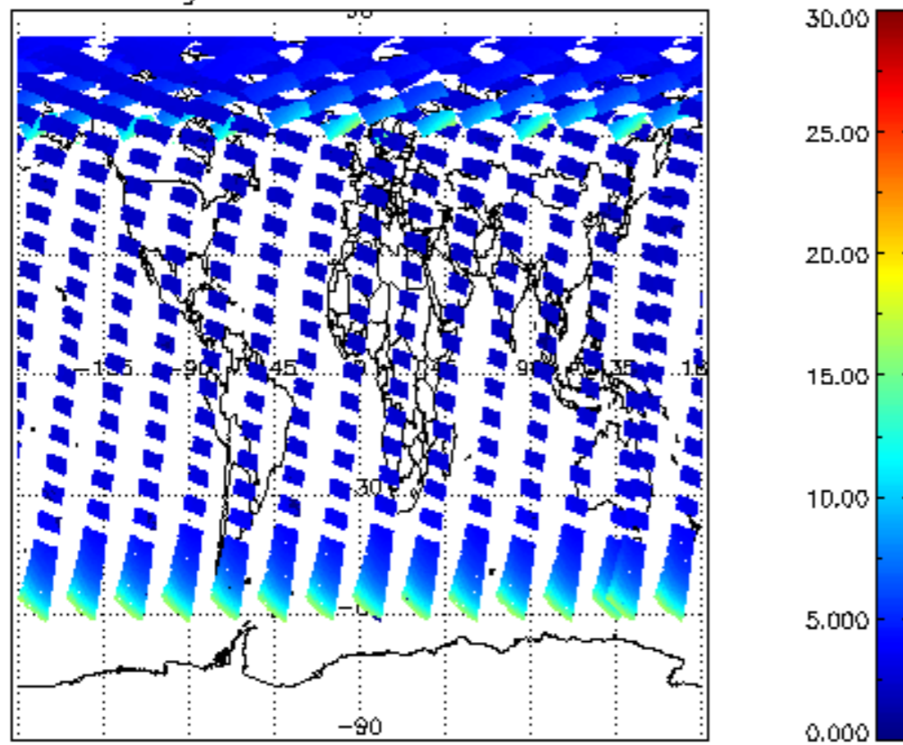
SCIOL2P_NADUV1NO2_amf_gr for 12JUL2009 00:00:00 to 13JUL2009 00:00:00
