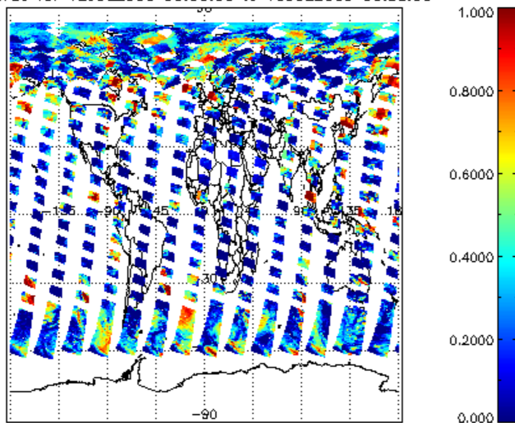
cl_frac for 12JUL2009 00:00:00 to 13JUL2009 00:00:00
