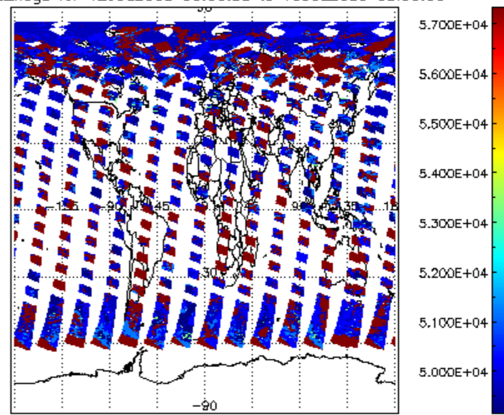
cloud_flags for 12JUL2009 00:00:00 to 13JUL2009 00:00:00
