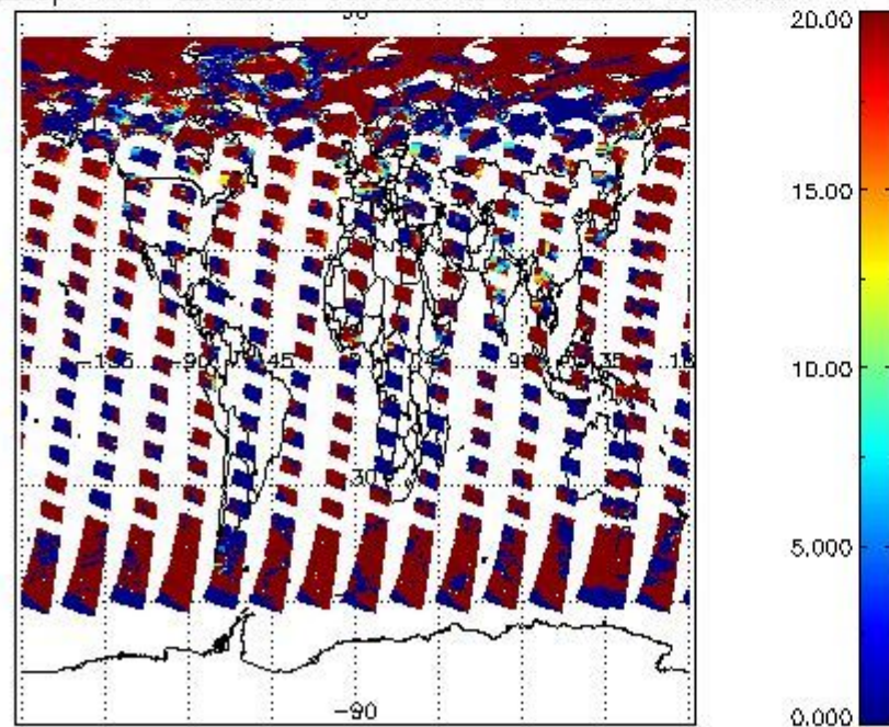
cL_opt_depth for 12JUL2009 00:00:00 to 13JUL2009 00:00:00
