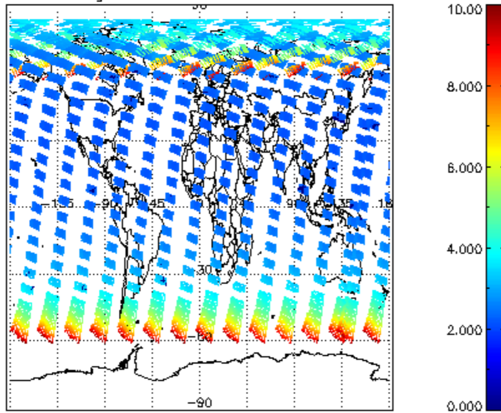
SCIOL2P_NADUV003_amf_gr for 12JUL2009 00:00:00 to 13JUL2009 00:00:00
