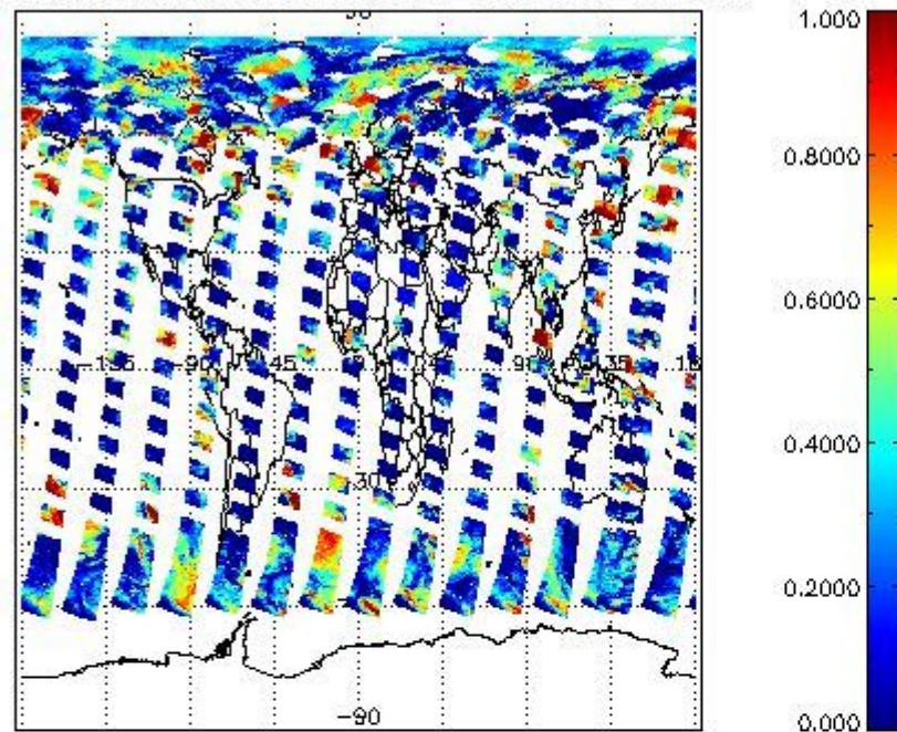
cL_frac for 12JUL2009 00:00:00 to 13JUL2009 00:00:00
