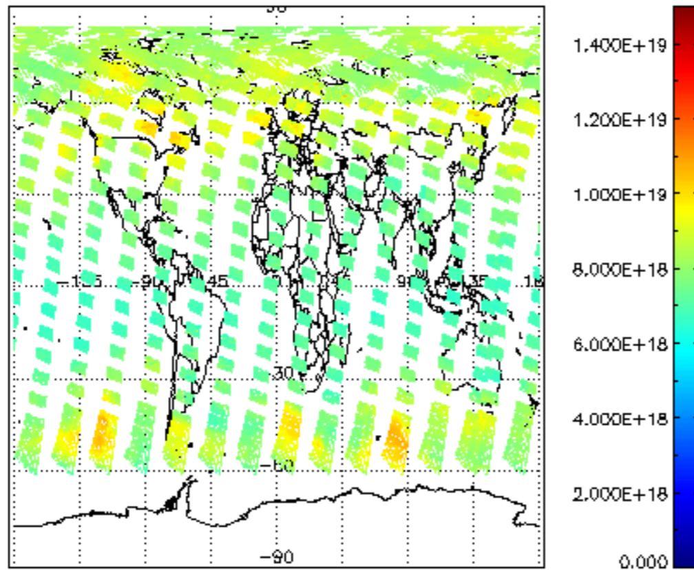
SCIOL2P_NADUV003_vcd for 12JUL2009 00:00:00 to 13JUL2009 00:00:00
