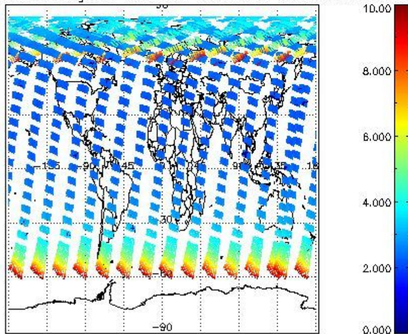
SCIOL2P_NADUV003_amf_gr for 12JUL2009 00:00:00 to 13JUL2009 00:00:00
