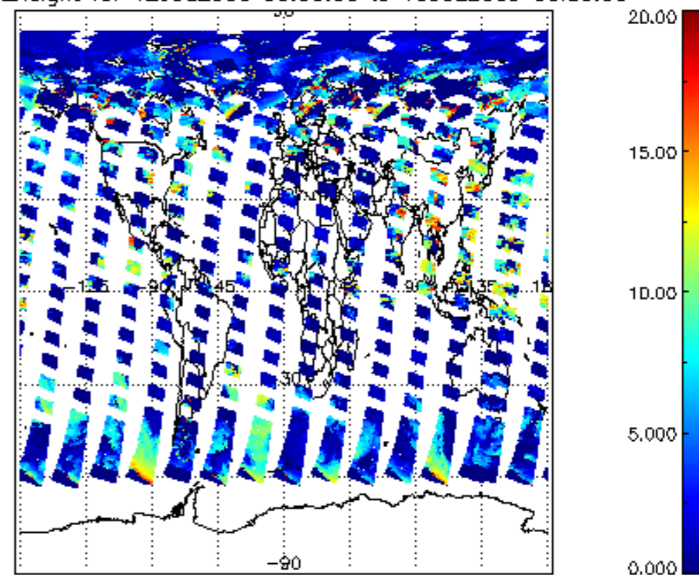
cl_top_height for 12JUL2009 00:00:00 to 13JUL2009 00:00:00
