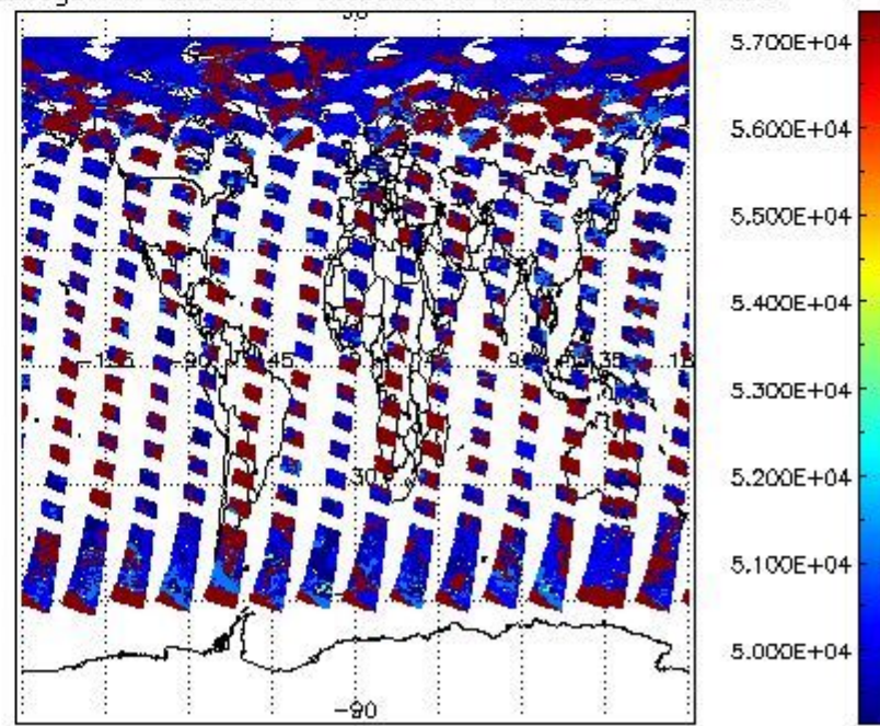
cloud_flags for 12JUL2009 00:00:00 to 13JUL2009 00:00:00
