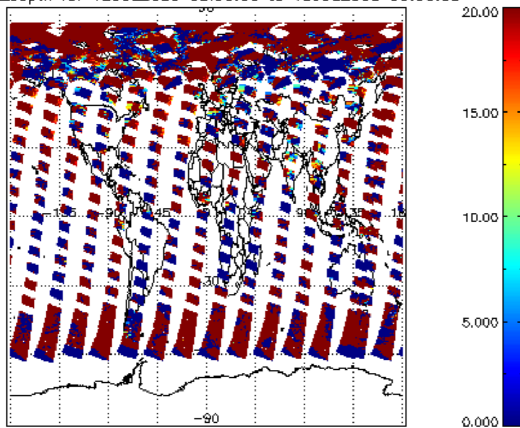
cl_lopt_depth for 12JUL2009 00:00:00 to 13JUL2009 00:00:00
