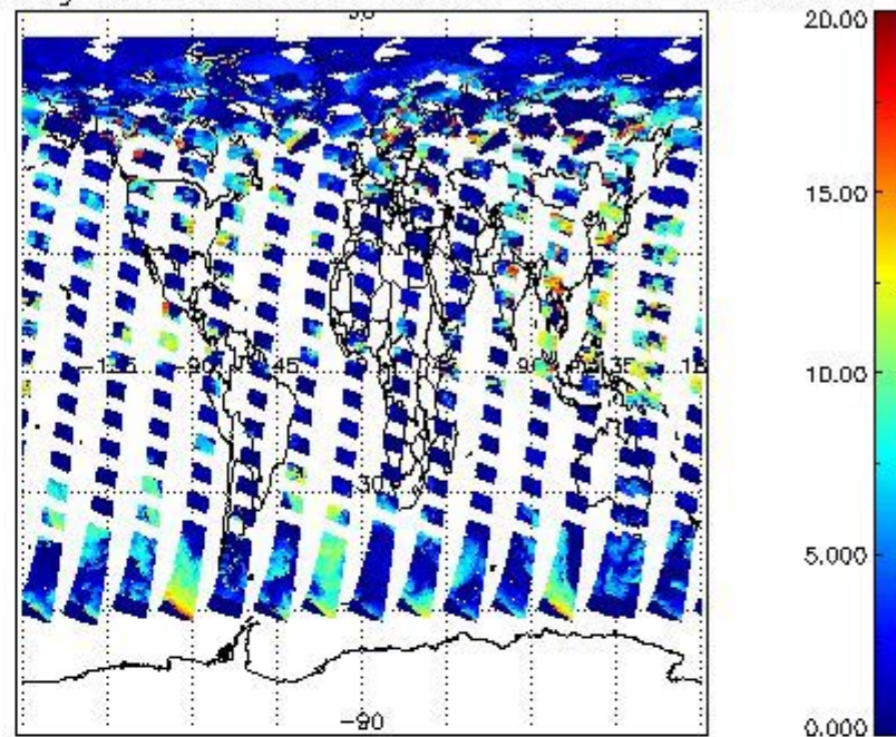
cL_top_height for 12JUL2009 00:00:00 to 13JUL2009 00:00:00
