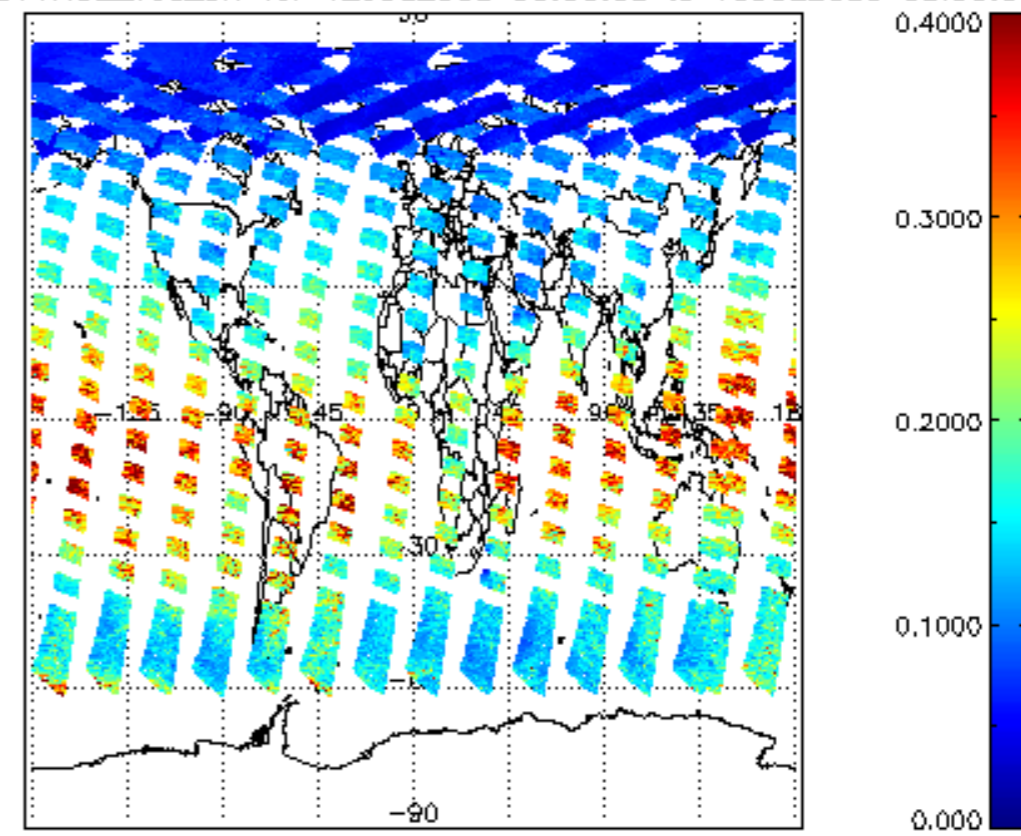
SCIOL2P_NADUV1NO2_vcd_err for 12JUL2009 00:00:00 to 13JUL2009 00:00:00
