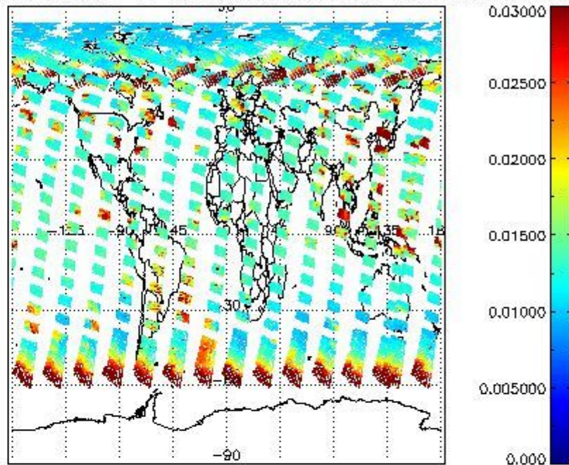
SCIOL2P_NADUV003_vcd_err for 12JUL2009 00:00:00 to 13JUL2009 00:00:00
