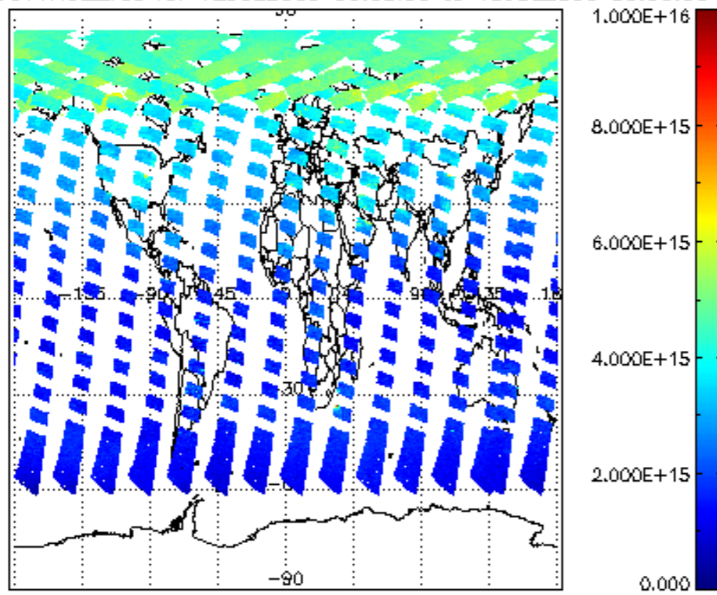
SCIOL2P_NADUV1NO2_vcd for 12JUL2009 00:00:00 to 13JUL2009 00:00:00
