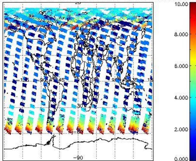
SCIOL2P_NADUV003_amf_cl for 12JUL2009 00:00:00 to 13JUL2009 00:00:00
