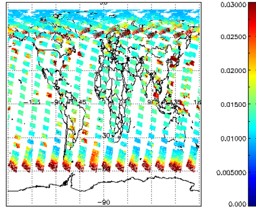
SCIOL2P_NADUV003_vcd_err for 12JUL2009 00:00:00 to 13JUL2009 00:00:00
