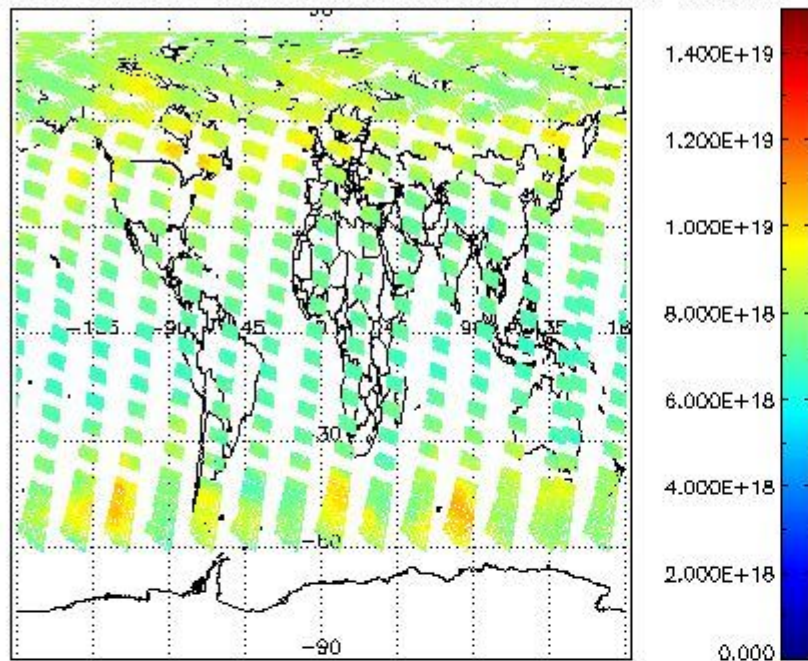
SCIOL2P_NADUV003_vcd for 12JUL2009 00:00:00 to 13JUL2009 00:00:00
