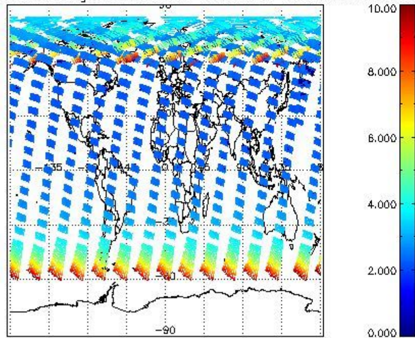
SCIOL2P_NADUV003_amf_gr for 08JUL2009 00:00:00 to 09JUL2009 00:00:00
