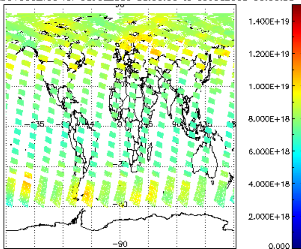
SCIOL2P_NADUV003_vcd for 08JUL2009 00:00:00 to 09JUL2009 00:00:00
