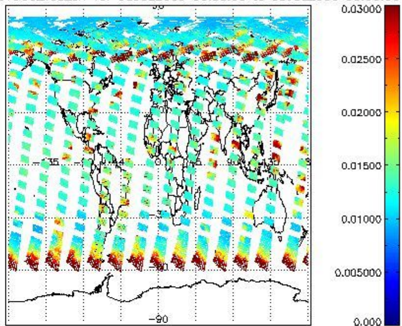
SCIOL2P_NADUV003_vcd_err for 08JUL2009 00:00:00 to 09JUL2009 00:00:00
