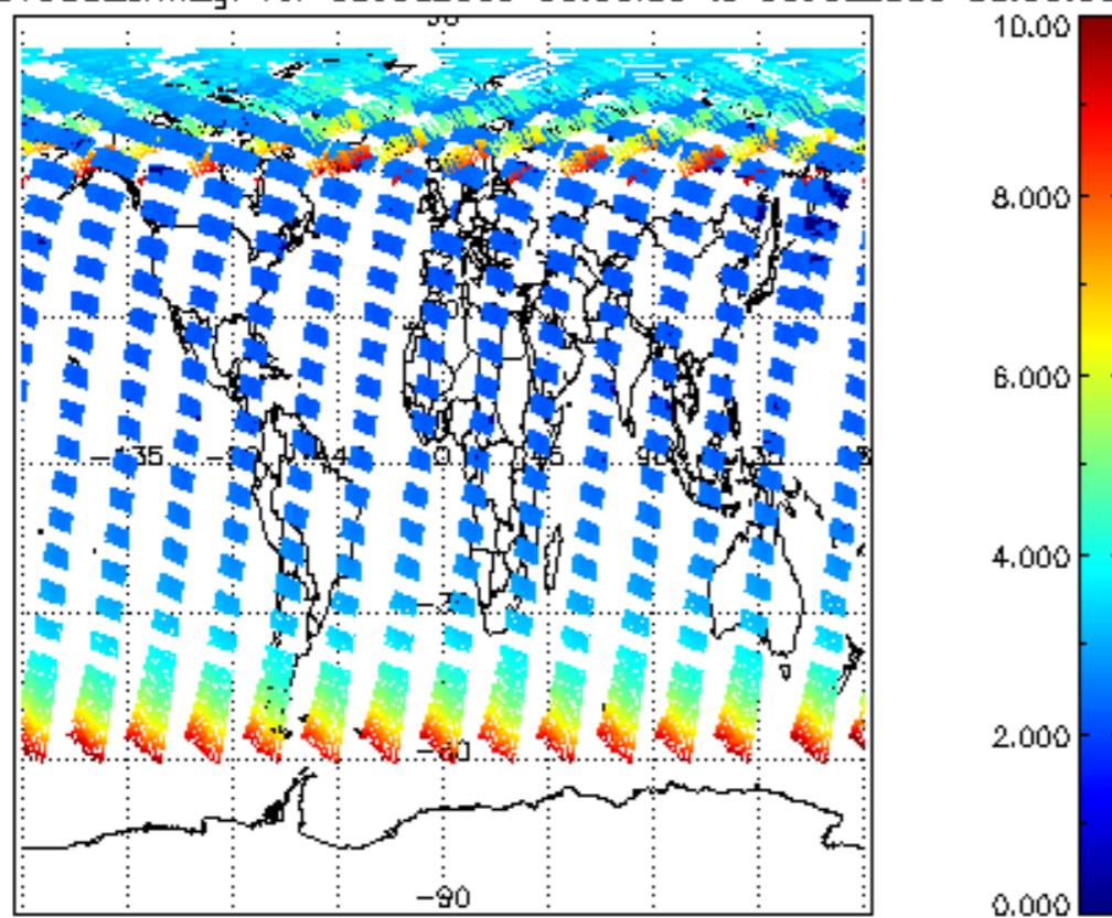
SCIOL2P_NADUV003_amf_gr for 08JUL2009 00:00:00 to 09JUL2009 00:00:00
