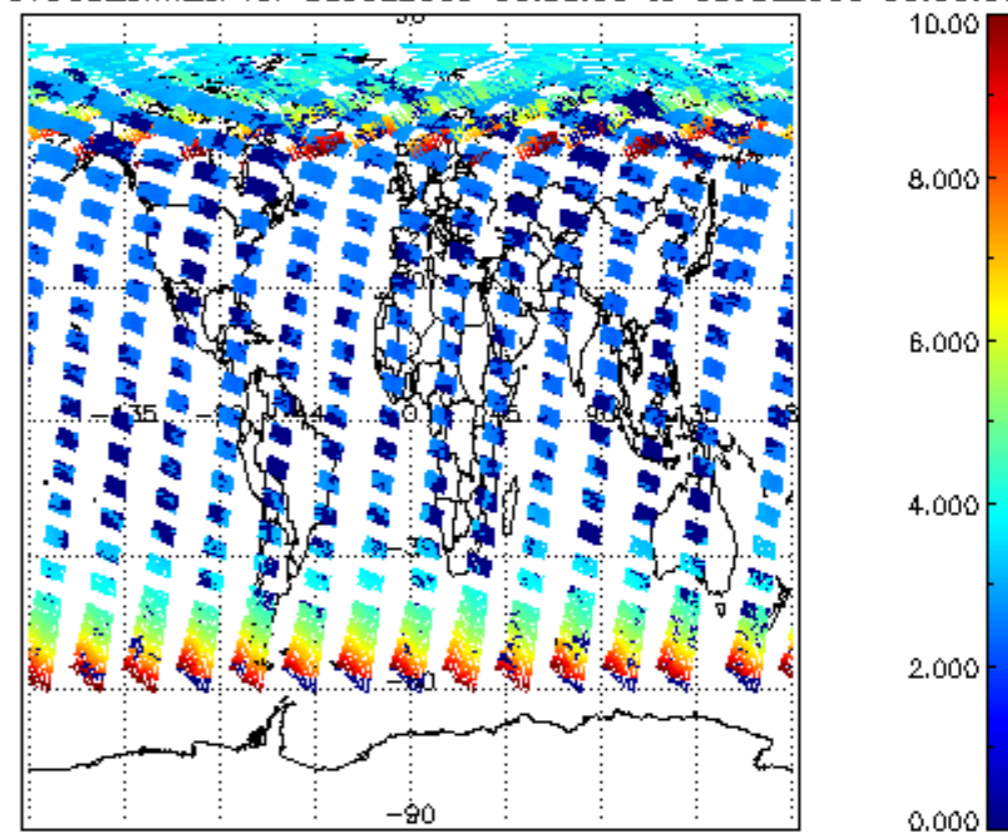
SCIOL2P_NADUV003_amf_cl for 08JUL2009 00:00:00 to 09JUL2009 00:00:00
