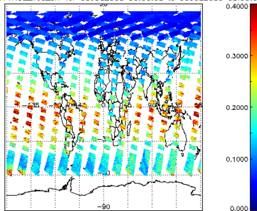
SCIOL2P_NADUV1NO2_vcd_err for 08JUL2009 00:00:00 to 09JUL2009 00:00:00
