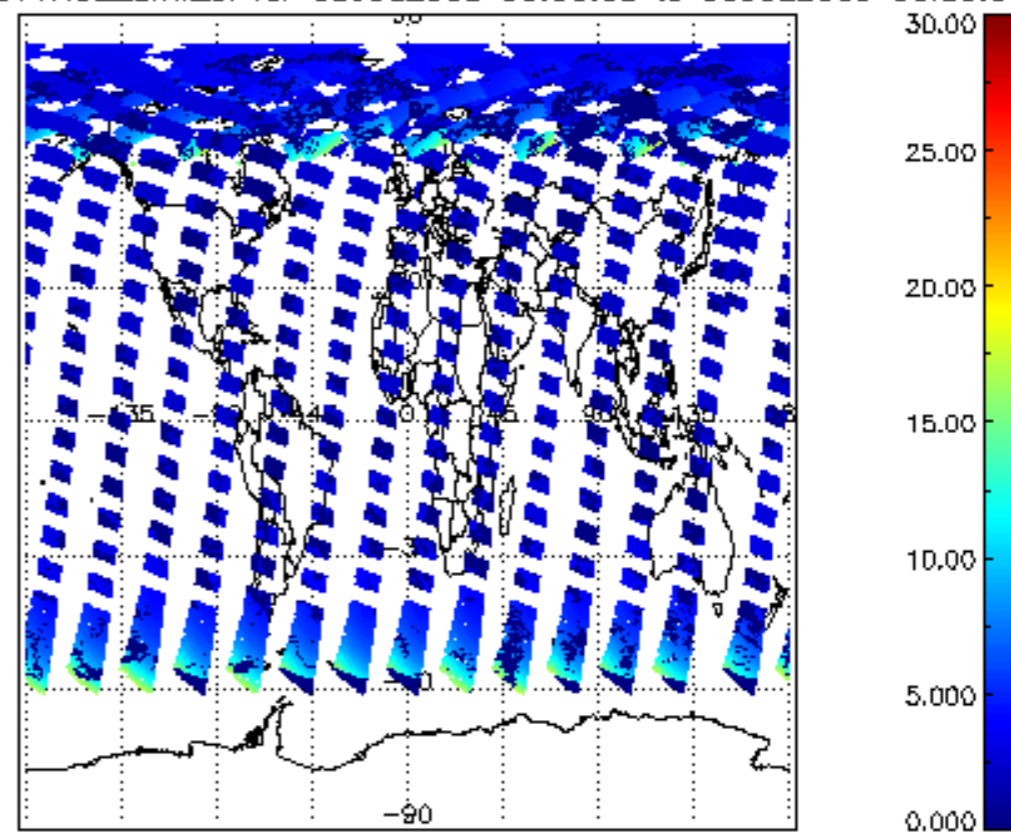
SCIOL2P_NADUV1NO2_amf_cl for 08JUL2009 00:00:00 to 09JUL2009 00:00:00
