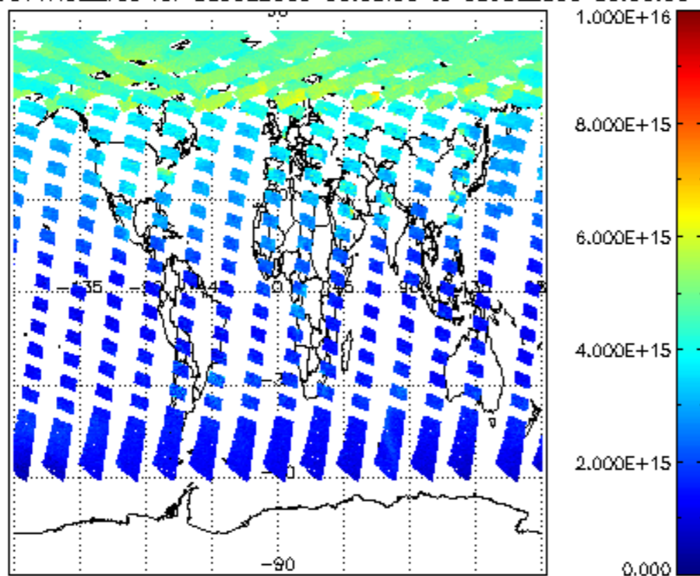
SCIOL2P_NADUV1NO2_vcd for 08JUL2009 00:00:00 to 09JUL2009 00:00:00
