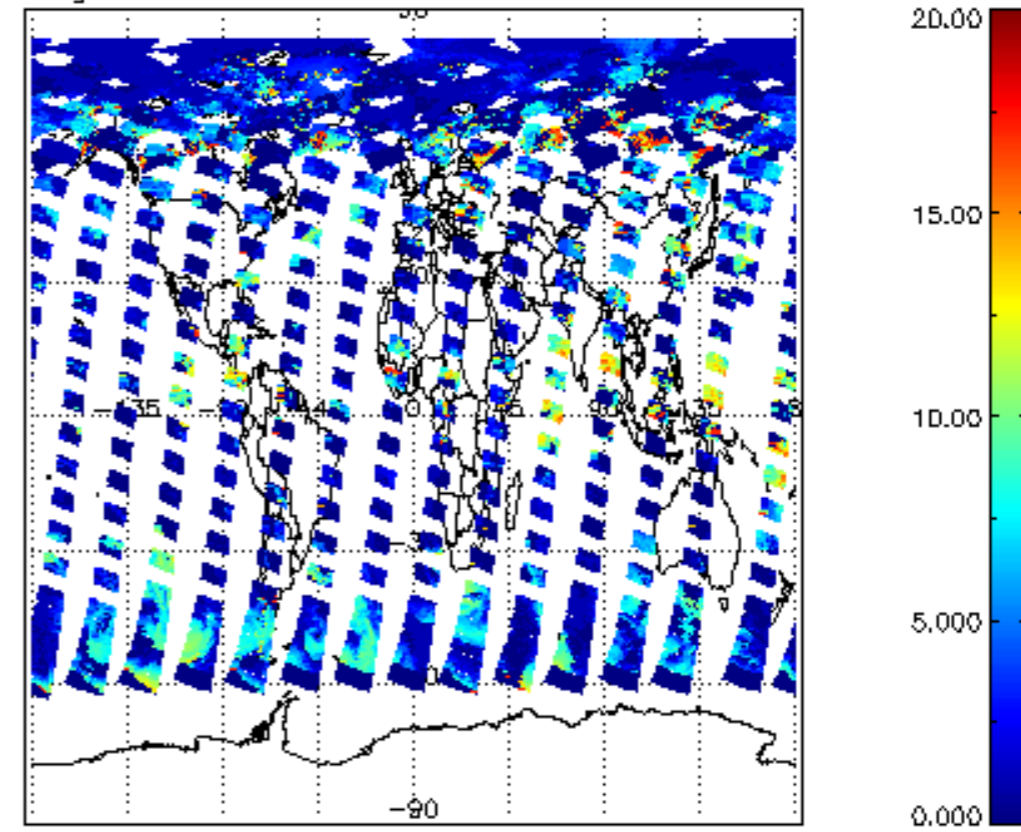
cl_top_height for 08JUL2009 00:00:00 to 09JUL2009 00:00:00
