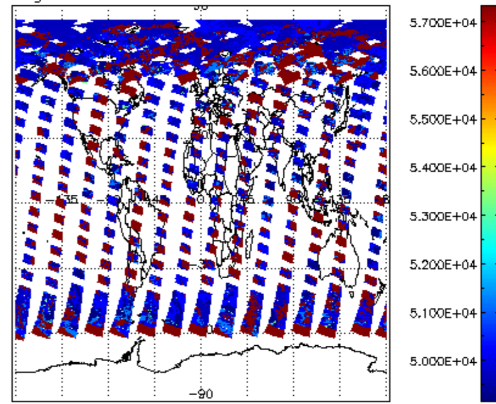
cloud_flags for 08JUL2009 00:00:00 to 09JUL2009 00:00:00
