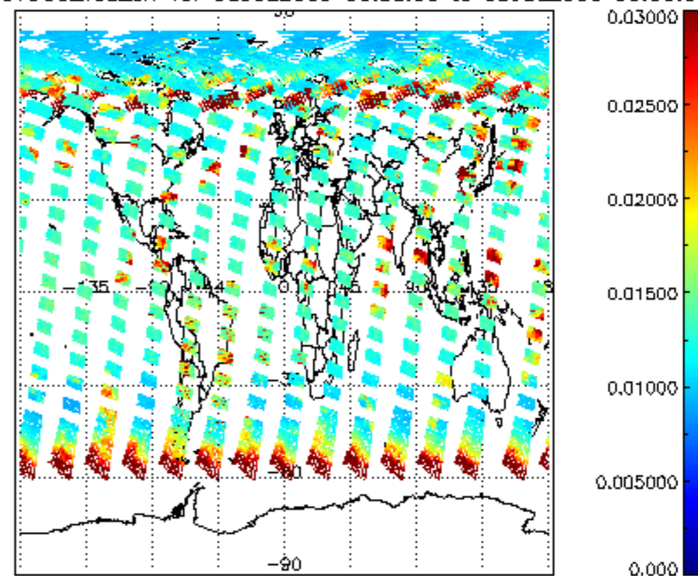
SCIOL2P_NADUV003_vcd_err for 08JUL2009 00:00:00 to 09JUL2009 00:00:00
