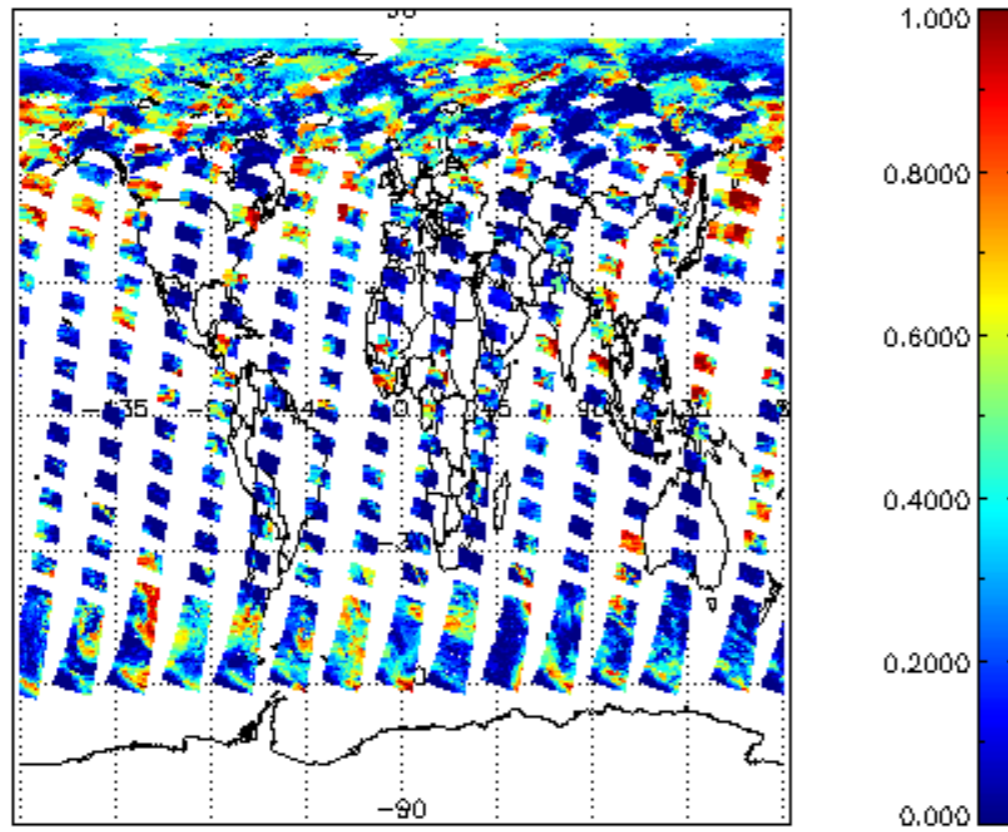
cl_frac for 08JUL2009 00:00:00 to 09JUL2009 00:00:00
