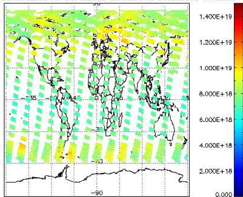
SCIOL2P_NADUV003_vcd for 08JUL2009 00:00:00 to 09JUL2009 00:00:00
