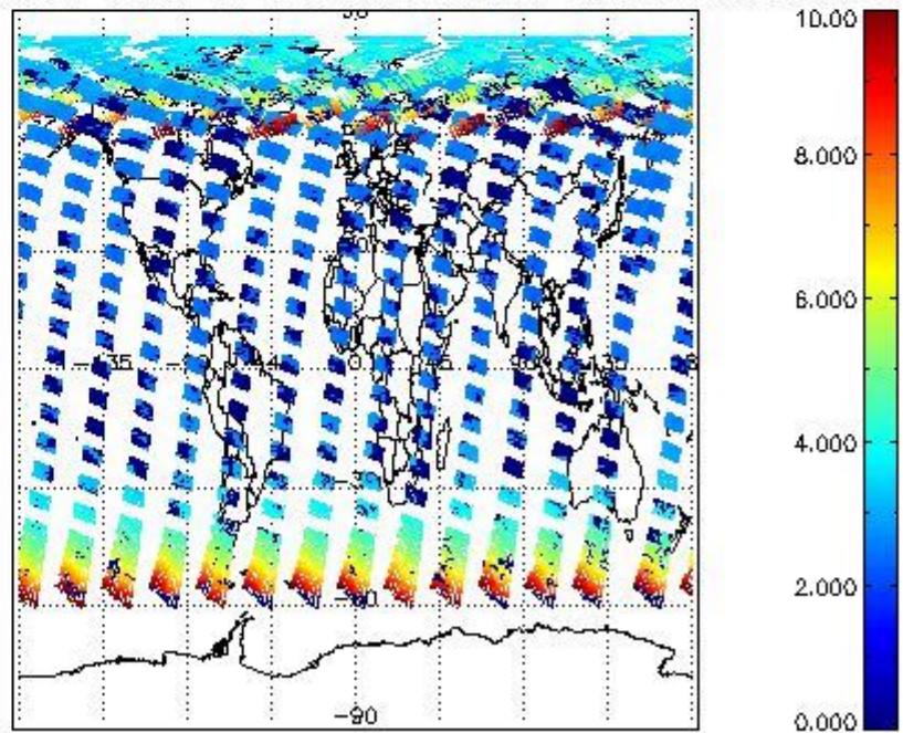
SCIOL2P_NADUV003_amf_cl for 08JUL2009 00:00:00 to 09JUL2009 00:00:00
