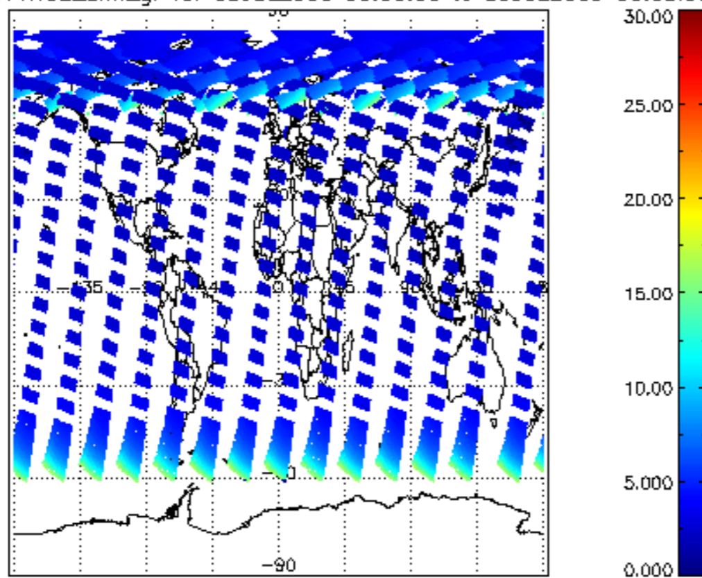
SCIOL2P_NADUV1NO2_amf_gr for 08JUL2009 00:00:00 to 09JUL2009 00:00:00
