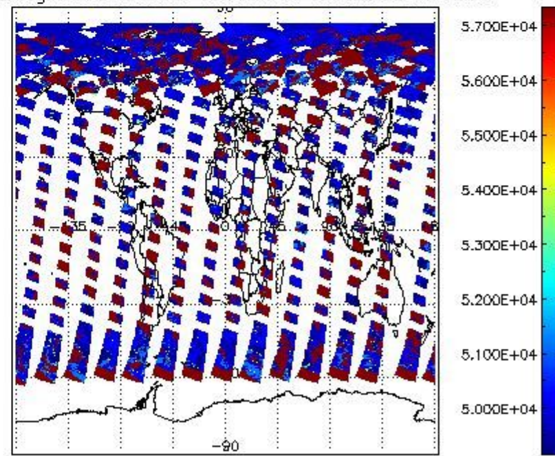
cloud_flags for 08JUL2009 00:00:00 to 09JUL2009 00:00:00
