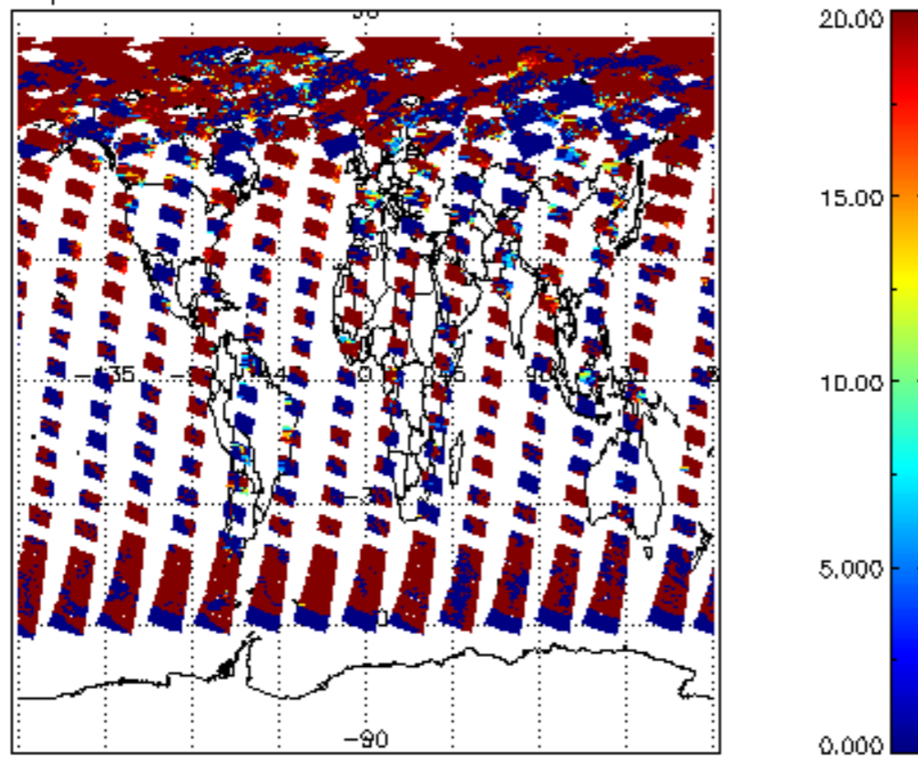
cl_lopt_depth for 08JUL2009 00:00:00 to 09JUL2009 00:00:00
