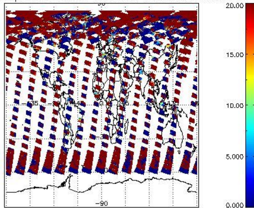
cL_opt_depth for 08JUL2009 00:00:00 to 09JUL2009 00:00:00
