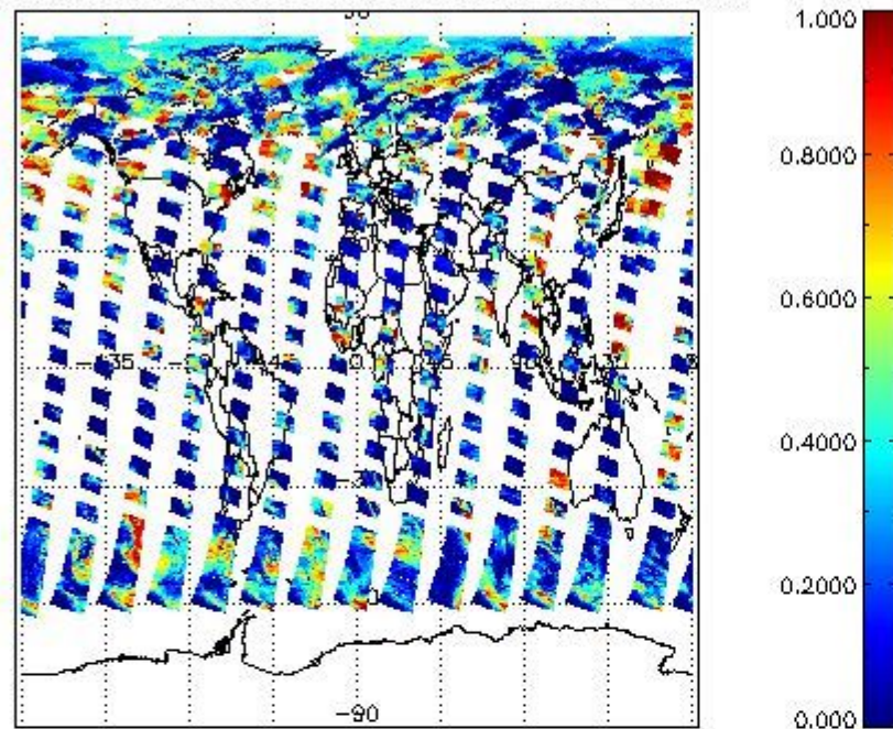
cL_frac for 08JUL2009 00:00:00 to 09JUL2009 00:00:00
