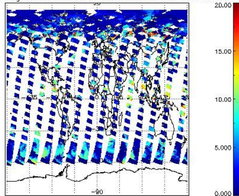
cL_top_height for 08JUL2009 00:00:00 to 09JUL2009 00:00:00
