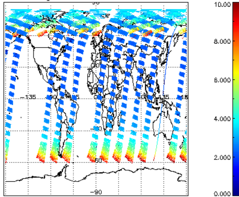
SCIOL2P_NADUV003_amf_gr for 07JUL2009 00:00:00 to 08JUL2009 00:00:00
