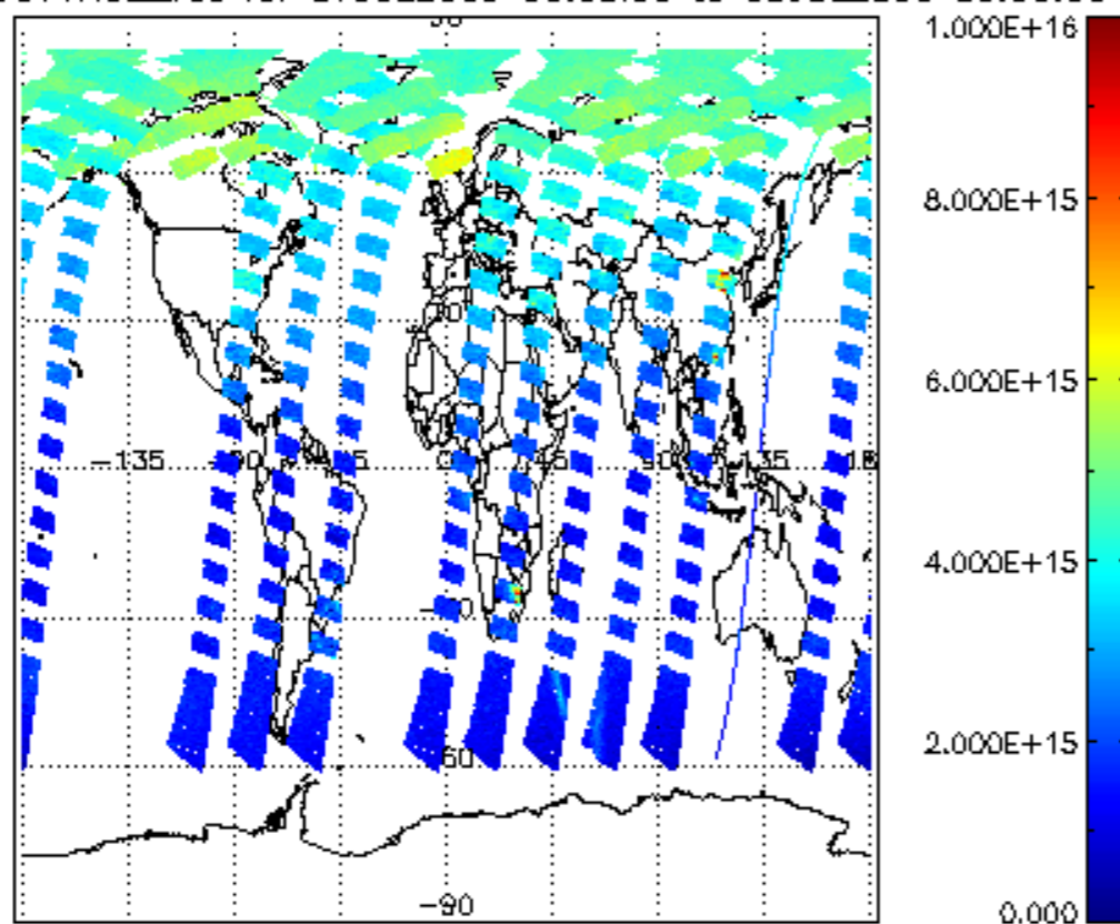
SCIOL2P_NADUV1NO2_vcd for 07JUL2009 00:00:00 to 08JUL2009 00:00:00
