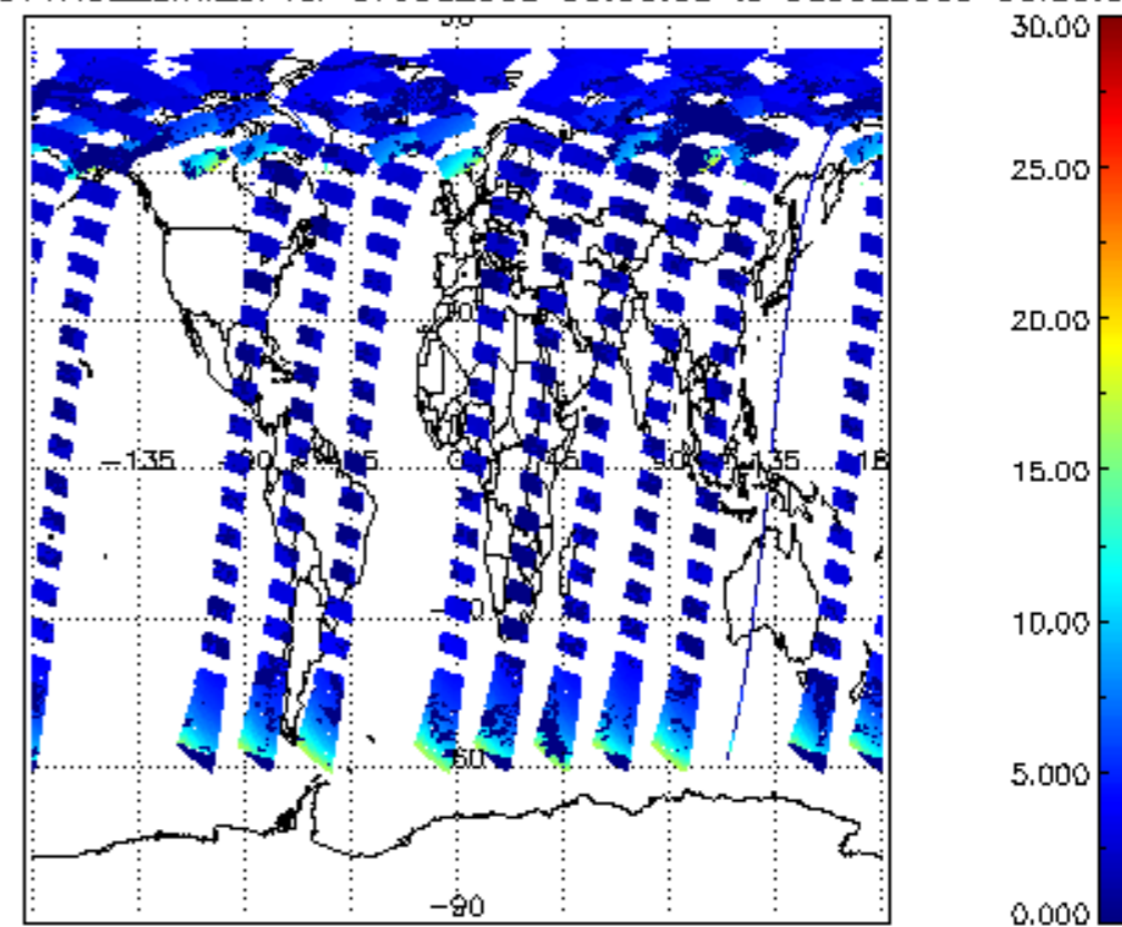
SCIOL2P_NADUV1NO2_amf_cl for 07JUL2009 00:00:00 to 08JUL2009 00:00:00
