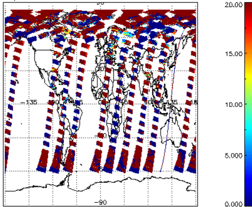
cl_lopt_depth for 07JUL2009 00:00:00 to 08JUL2009 00:00:00
