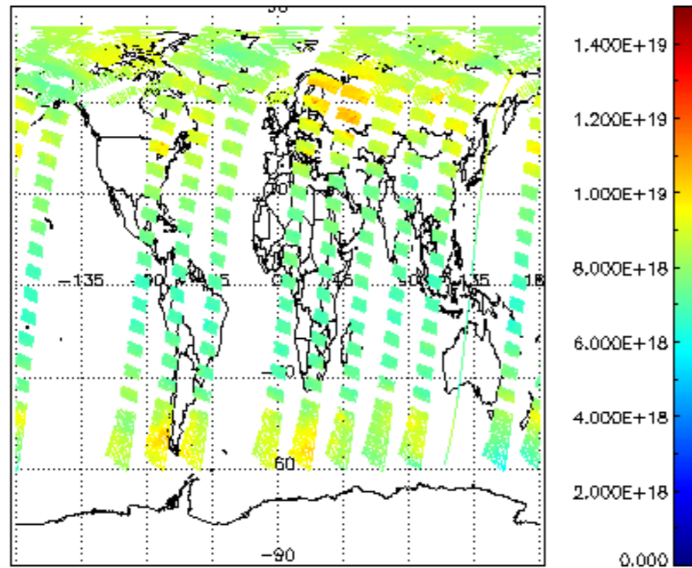
SCIOL2P_NADUV003_vcd for 07JUL2009 00:00:00 to 08JUL2009 00:00:00
