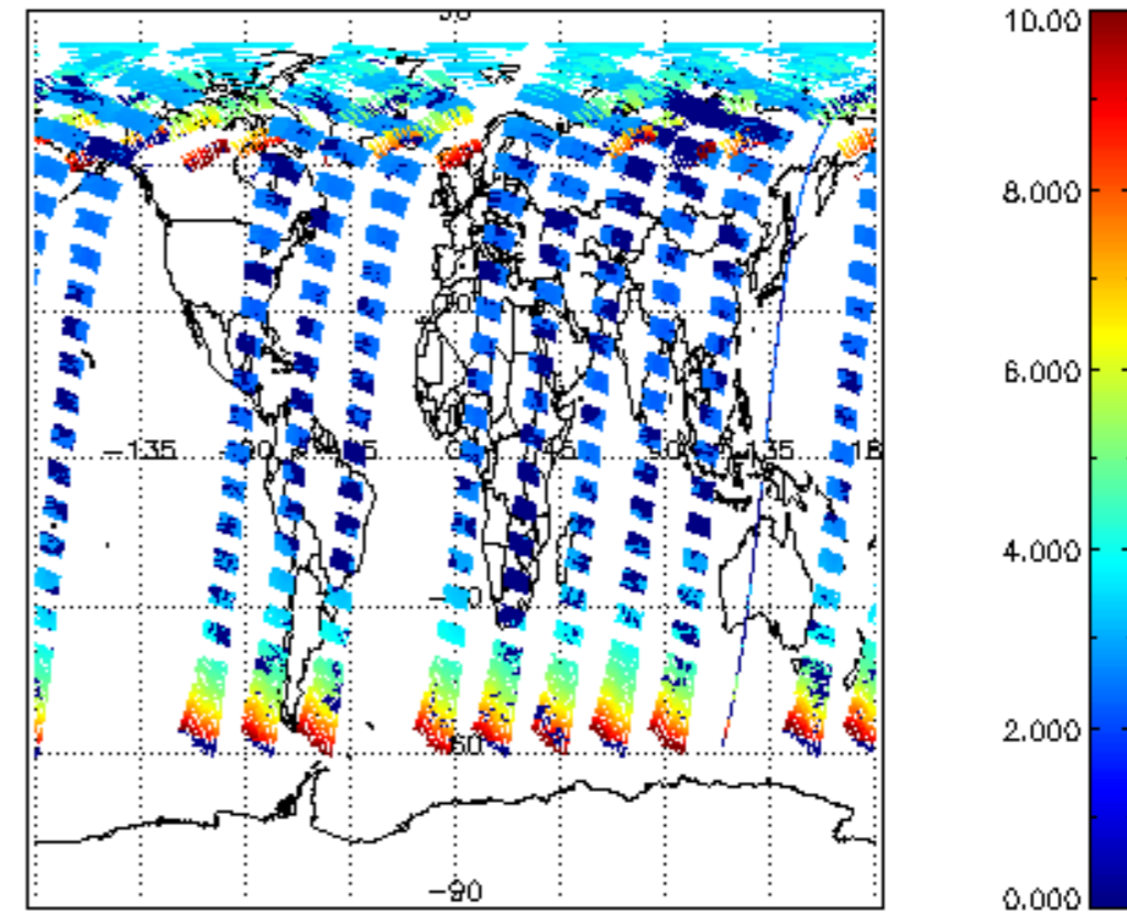
SCIOL2P_NADUV003_amf_cl for 07JUL2009 00:00:00 to 08JUL2009 00:00:00
