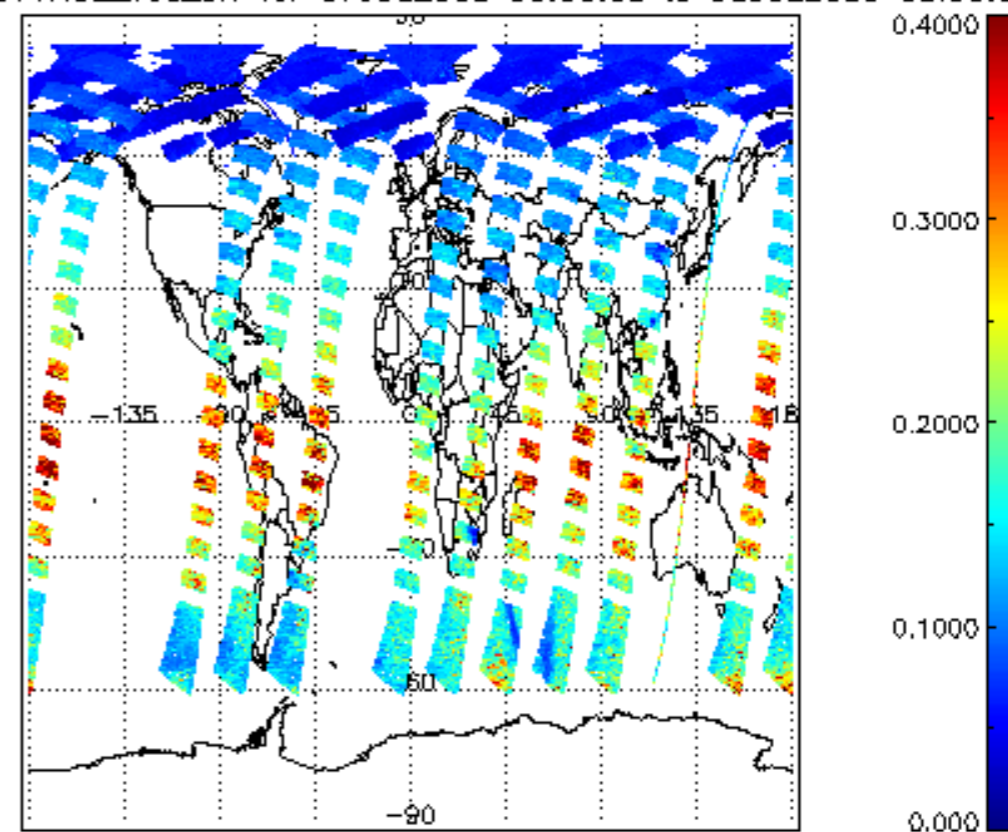
SCIOL2P_NADUV1NO2_vcd_err for 07JUL2009 00:00:00 to 08JUL2009 00:00:00
