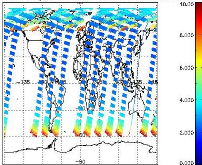
SCIOL2P_NADUV003_amf_gr for 07JUL2009 00:00:00 to 08JUL2009 00:00:00
