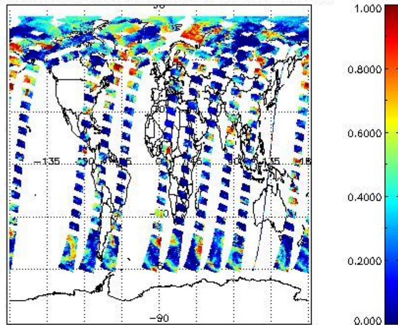
cL_frac for 07JUL2009 00:00:00 to 08JUL2009 00:00:00
