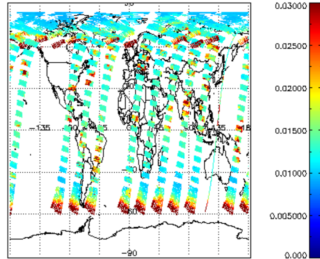
SCIOL2P_NADUV003_vcd_err for 07JUL2009 00:00:00 to 08JUL2009 00:00:00
