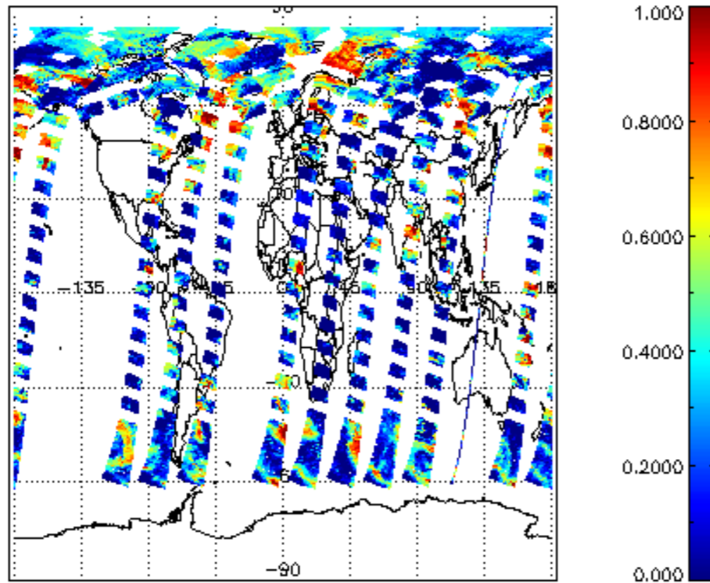
cl_frac for 07JUL2009 00:00:00 to 08JUL2009 00:00:00
