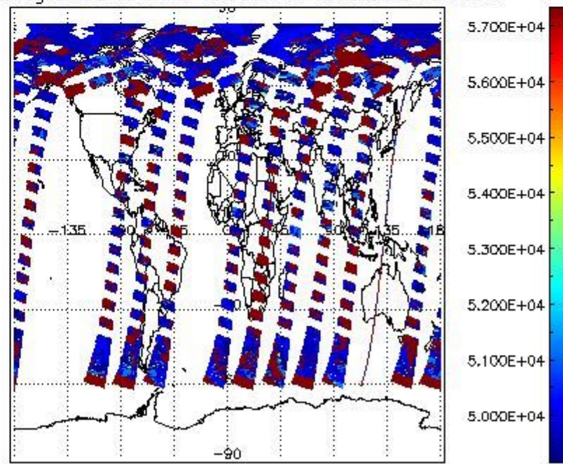
cloud_flags for 07JUL2009 00:00:00 to 08JUL2009 00:00:00
