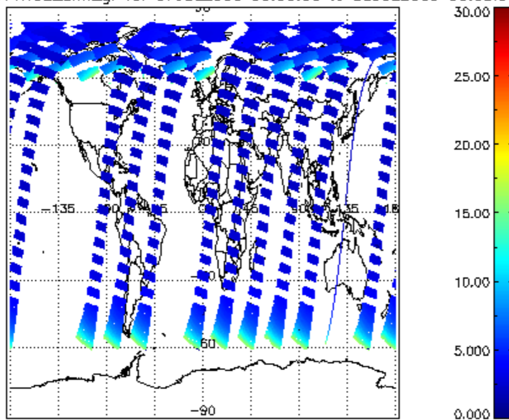
SCIOL2P_NADUV1NO2_amf_gr for 07JUL2009 00:00:00 to 08JUL2009 00:00:00
