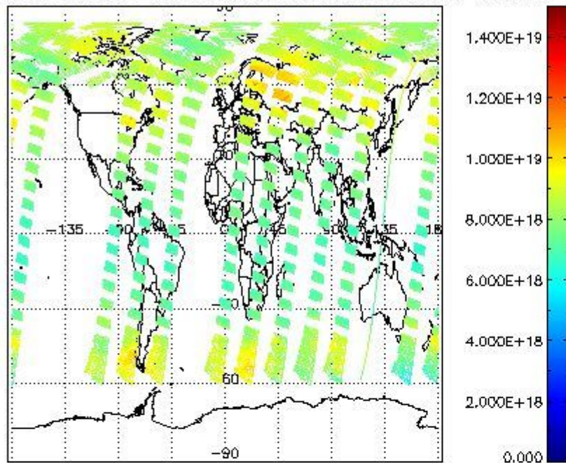
SCIOL2P_NADUV003_vcd for 07JUL2009 00:00:00 to 08JUL2009 00:00:00
