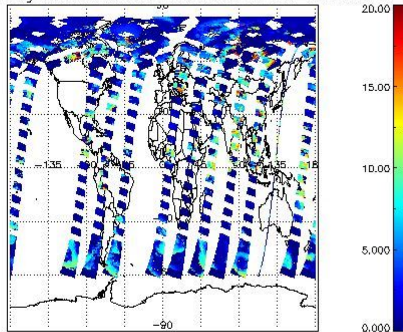
cL_top_height for 07JUL2009 00:00:00 to 08JUL2009 00:00:00
