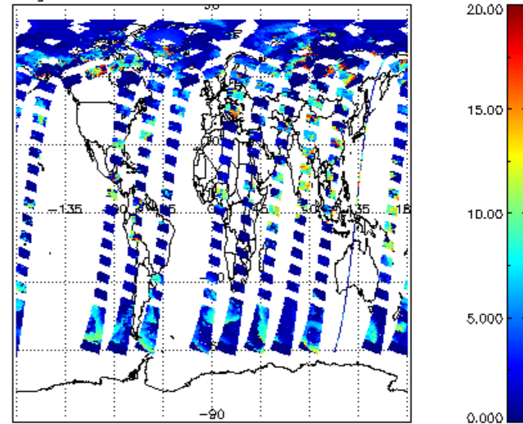
cl_top_height for 07JUL2009 00:00:00 to 08JUL2009 00:00:00
