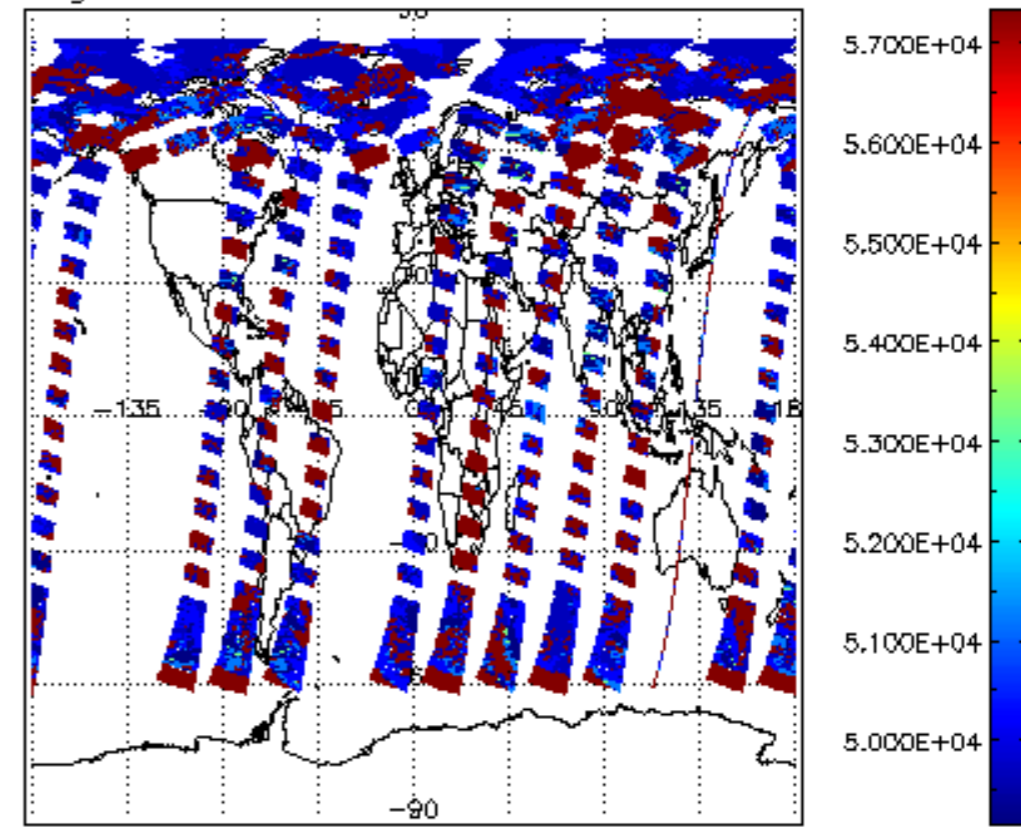
cloud_flags for 07JUL2009 00:00:00 to 08JUL2009 00:00:00
