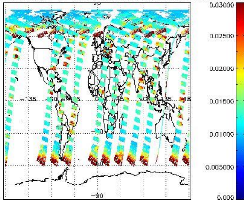
SCIOL2P_NADUV003_vcd_err for 07JUL2009 00:00:00 to 08JUL2009 00:00:00
