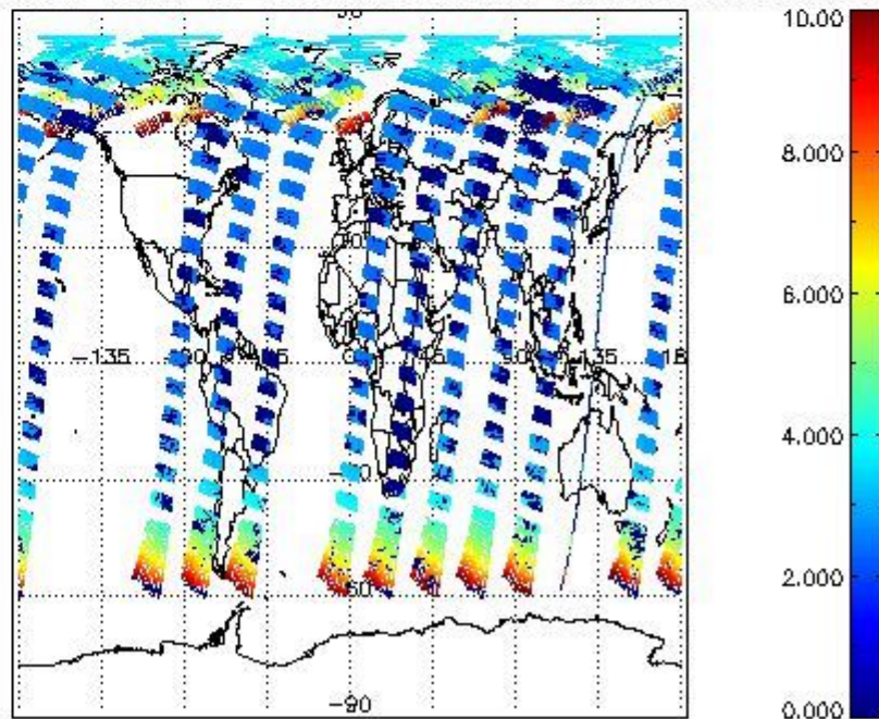
SCIOL2P_NADUV003_amf_cl for 07JUL2009 00:00:00 to 08JUL2009 00:00:00
