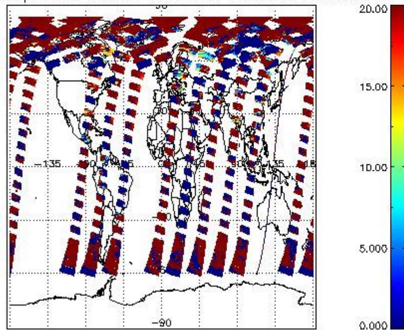
cL_opt_depth for 07JUL2009 00:00:00 to 08JUL2009 00:00:00
