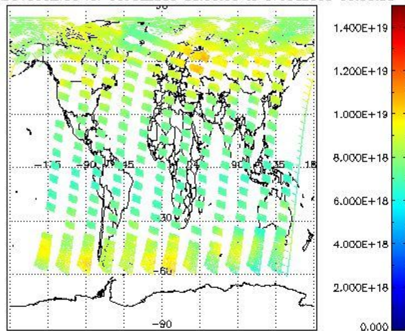
SCIOL2P_NADUV003_vcd for 06JUL2009 00:00:00 to 07JUL2009 00:00:00
