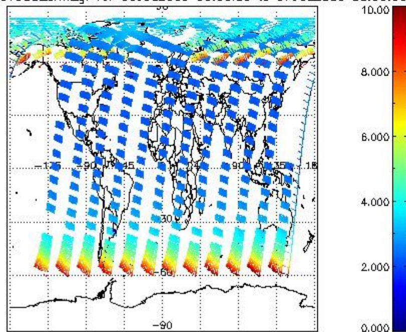
SCIOL2P_NADUV003_amf_gr for 06JUL2009 00:00:00 to 07JUL2009 00:00:00
