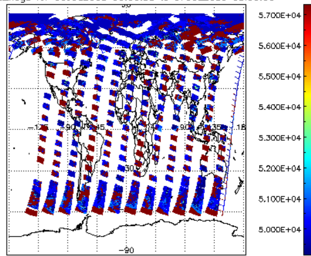
cloud_flags for 06JUL2009 00:00:00 to 07JUL2009 00:00:00
