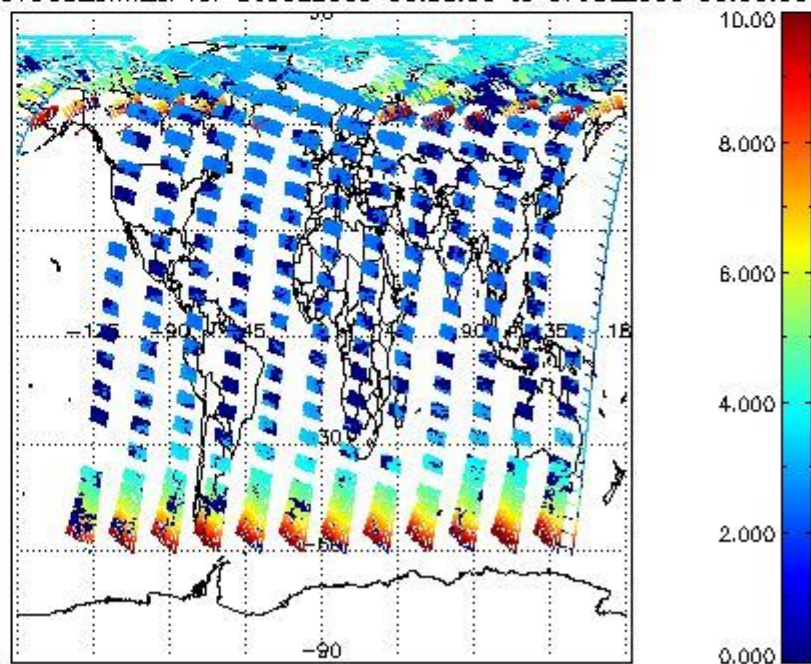
SCIOL2P_NADUV003_amf_cl for 06JUL2009 00:00:00 to 07JUL2009 00:00:00
