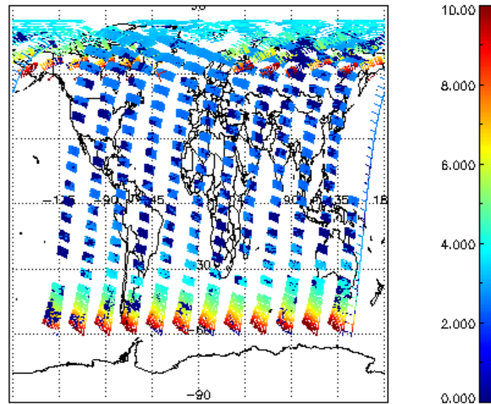
SCIOL2P_NADUV003_amf_cl for 06JUL2009 00:00:00 to 07JUL2009 00:00:00
