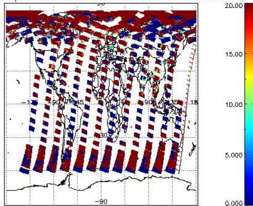
cL_opt_depth for 06JUL2009 00:00:00 to 07JUL2009 00:00:00
