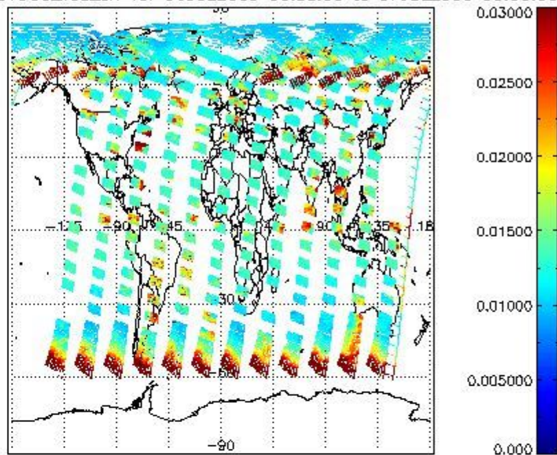
SCIOL2P_NADUV003_vcd_err for 06JUL2009 00:00:00 to 07JUL2009 00:00:00
