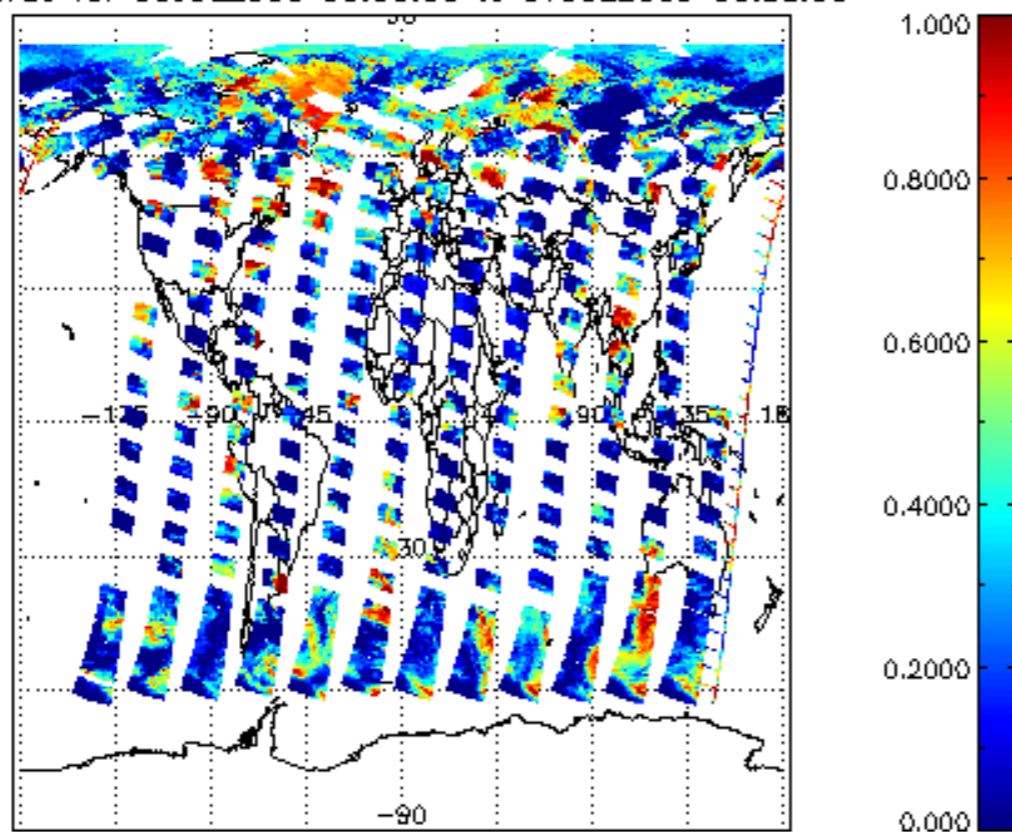
cl_frac for 06JUL2009 00:00:00 to 07JUL2009 00:00:00
