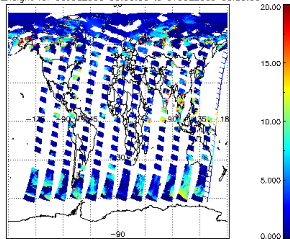
cl_top_height for 06JUL2009 00:00:00 to 07JUL2009 00:00:00
