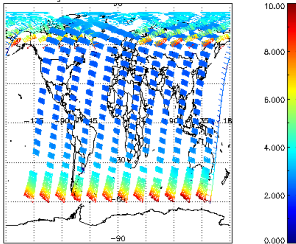
SCIOL2P_NADUV003_amf_gr for 06JUL2009 00:00:00 to 07JUL2009 00:00:00
