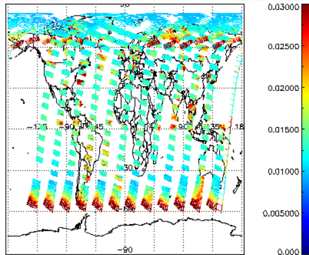
SCIOL2P_NADUV003_vcd_err for 06JUL2009 00:00:00 to 07JUL2009 00:00:00
