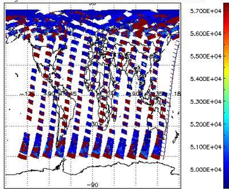
cloud_flags for 06JUL2009 00:00:00 to 07JUL2009 00:00:00
