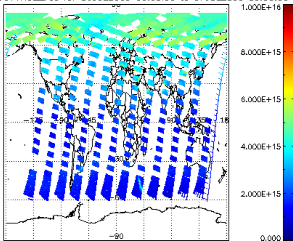
SCIOL2P_NADUV1NO2_vcd for 06JUL2009 00:00:00 to 07JUL2009 00:00:00
