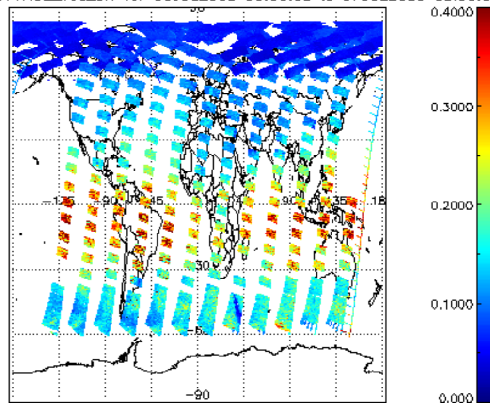
SCIOL2P_NADUV1NO2_vcd_err for 06JUL2009 00:00:00 to 07JUL2009 00:00:00
