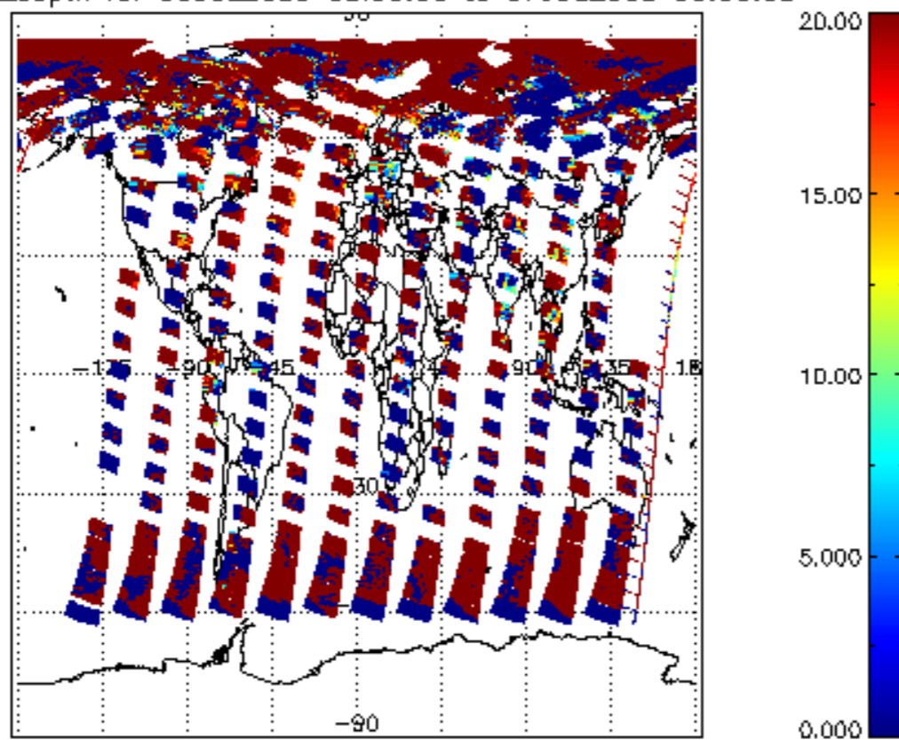
cl_lopt_depth for 06JUL2009 00:00:00 to 07JUL2009 00:00:00
