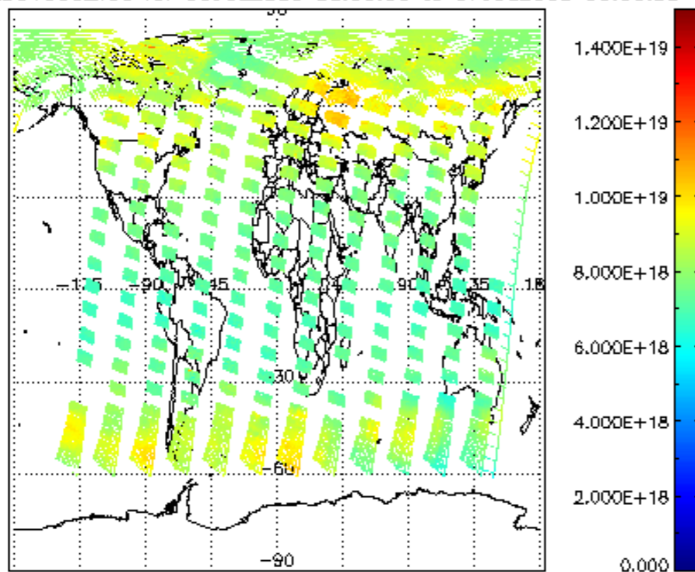
SCIOL2P_NADUV003_vcd for 06JUL2009 00:00:00 to 07JUL2009 00:00:00
