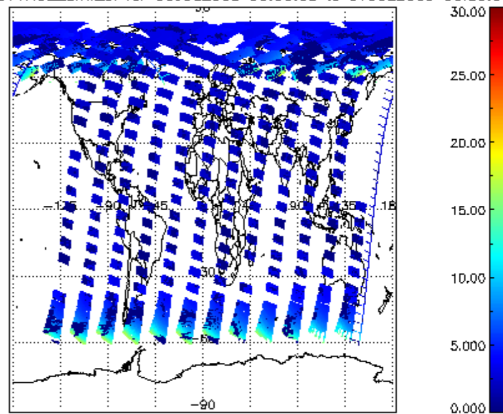
SCIOL2P_NADUV1NO2_amf_cl for 06JUL2009 00:00:00 to 07JUL2009 00:00:00
