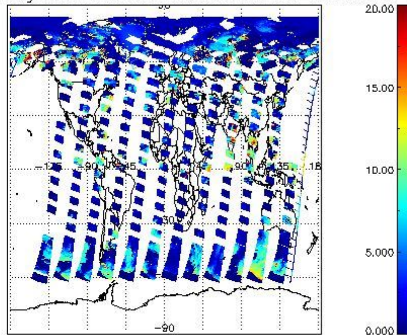
cL_top_height for 06JUL2009 00:00:00 to 07JUL2009 00:00:00
