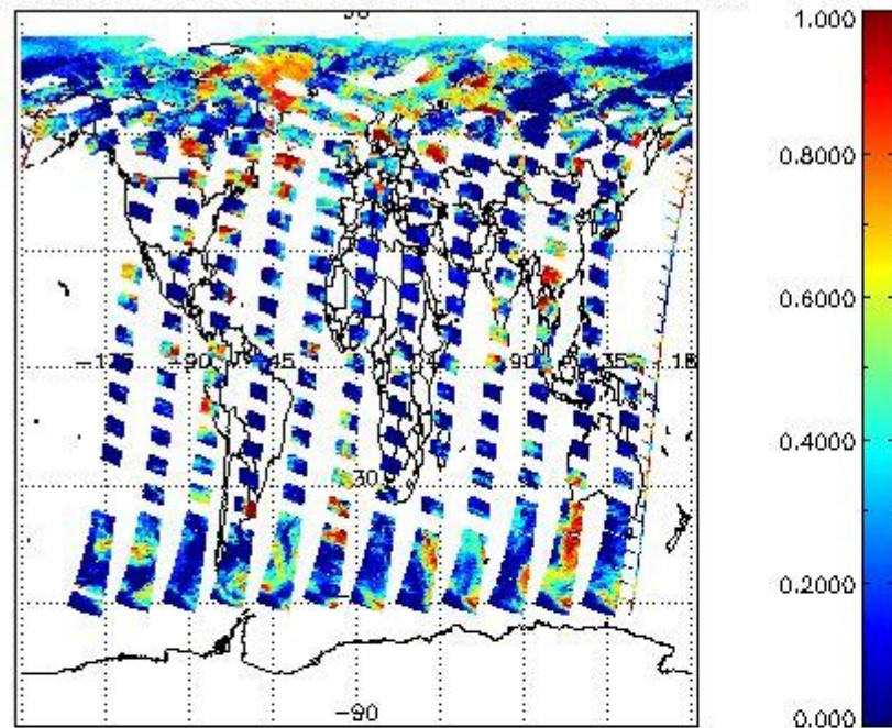
cL_frac for 06JUL2009 00:00:00 to 07JUL2009 00:00:00
